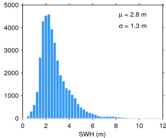
Figure 20. Histogram of science-valid SWH over oceans and lakes for 31/01/2019. The mean ( \mu ) and standard deviation ( \sigma ) are also shown. Note that values larger than 12 m are excluded from the histogram for the sake of readability but not from the computation of \mu and \sigma .
