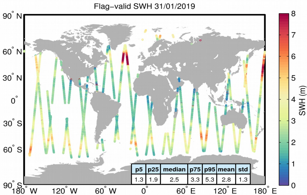
Figure 15. Geographical distribution of flag-valid SWH data over oceans and lakes for 31/01/2019. The statistical values shown in the table refer to the SWH in m and are calculated over all measurements shown in the figure.
