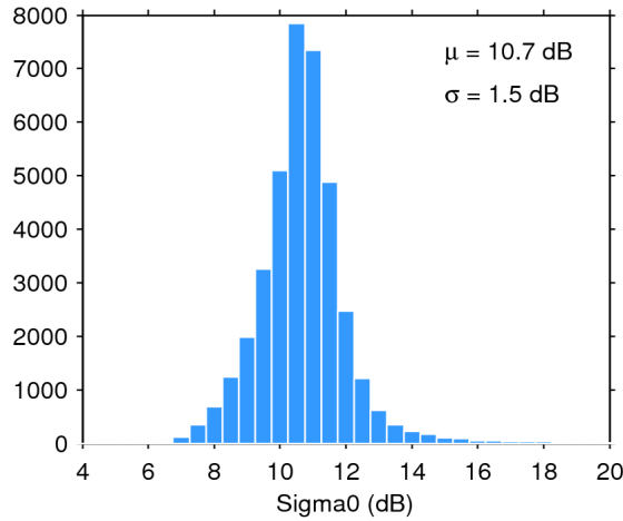
Figure 28. Histogram of science-valid sigma0 over oceans and lakes for 31/01/2019. The mean ( \mu ) and standard deviation ( \sigma ) are also shown. Note that values outside [4 20] dB are excluded from the histogram for the sake of readability but not from the computation of \mu and \sigma .
