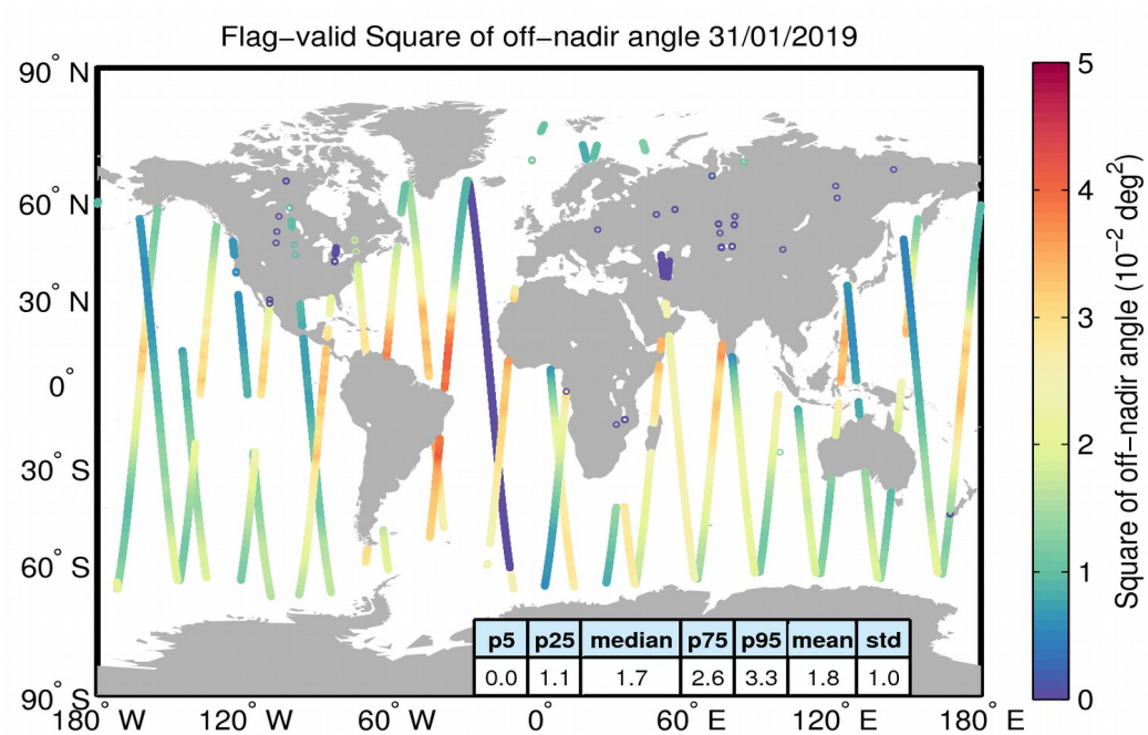
Figure 37. Geographical distribution of flag-valid mispointing data over oceans and lakes for 31/01/2019. The statistical values shown in the table refer to the mispointing in 10^{-2} \text{ deg}^2 and are calculated over all measurements shown in the figure.
