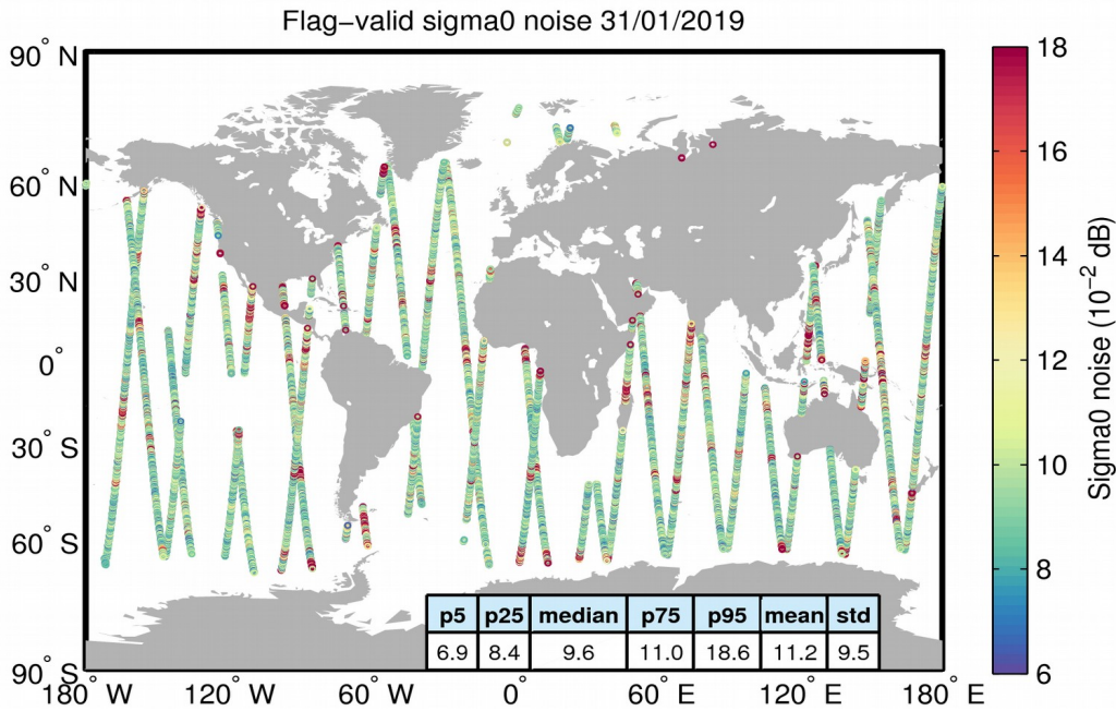
Figure 26. Geographical distribution of flag-valid 20-Hz sigma0 measurement noise over oceans and lakes for 31/01/2019. The statistical values shown in the table refer to the sigma0 noise and are calculated over all measurements shown in the figure.
