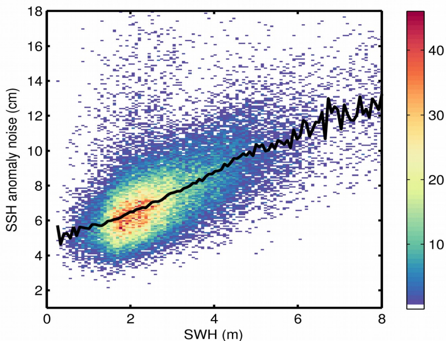
Figure 9. 2D histogram showing flag-valid SSH anomaly noise as a function of SWH for 31/01/2019. The black line denotes the median SSH anomaly noise as a function of SWH.
