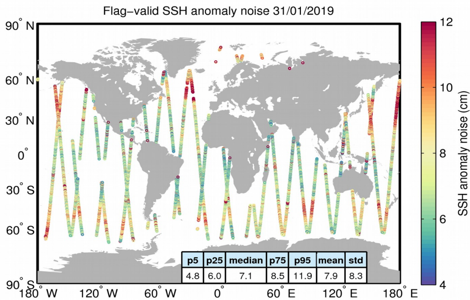
Figure 8. Geographical distribution of flag-valid 20-Hz SSH anomaly measurement noise over oceans and lakes for 31/01/2019. The statistical values shown in the table refer to the SSH anomaly noise and are calculated over all measurements shown in the figure.
