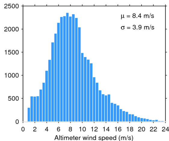
Figure 35. Histogram of science-valid wind over oceans and lakes for 31/01/2019. The mean ( \mu ) and standard deviation ( \sigma ) are also shown. Note that values larger than 24 m/s are excluded from the histogram for the sake of readability but not from the computation of \mu and \sigma .
