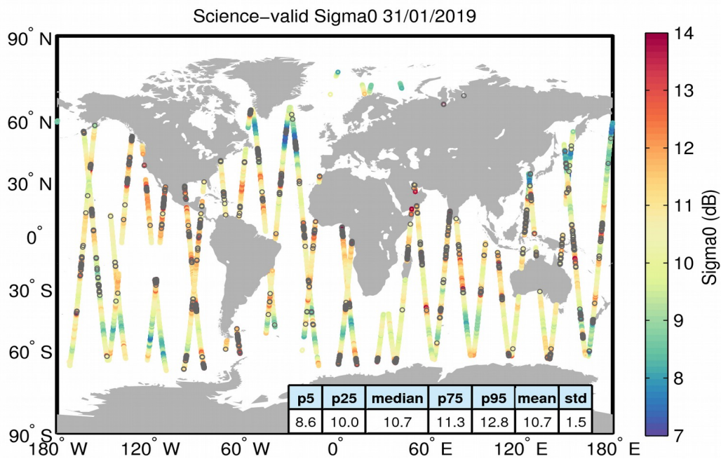
Figure 27. Geographical distribution of science-valid sigma0 data over oceans and lakes for 31/01/2019. The statistical values shown in the table refer to the sigma0 in dB and are calculated over all measurements shown in the figure. Gray circles denote records that have been rejected based on the editing criteria described in Table 4.
