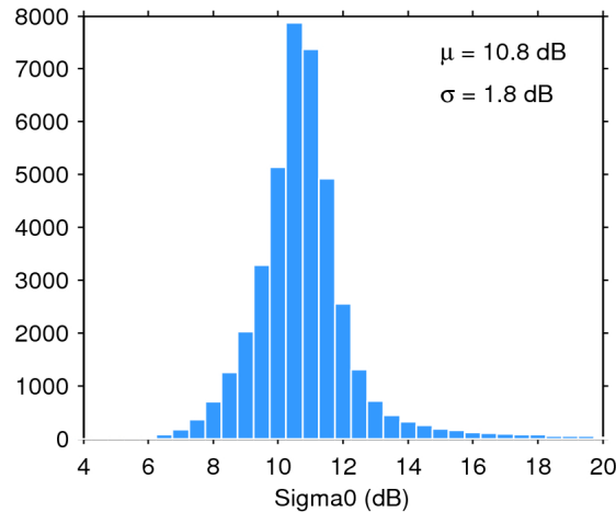
Figure 25. Histogram of flag-valid sigma0 over oceans and lakes for 31/01/2019. The mean ( \mu ) and standard deviation ( \sigma ) are also shown. Note that values outside [4 20] dB are excluded from the histogram for the sake of readability but not from the computation of \mu and \sigma .
