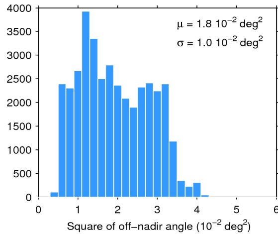
Figure 39. Histogram of flag-valid mispointing over oceans and lakes for 31/01/2019. The mean ( \mu ) and standard deviation ( \sigma ) are also shown. Note that values larger than 6 \cdot 10^{-2} \text{ deg}^2 are excluded from the histogram for the sake of readability but not from the computation of \mu and \sigma .
