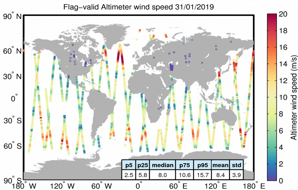
Figure 31. Geographical distribution of flag-valid wind data over oceans and lakes for 31/01/2019. The statistical values shown in the table refer to the wind in m/s and are calculated over all measurements shown in the figure.
