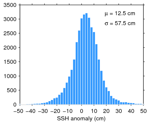
Figure 7. Histogram of flag-valid SSH anomaly over oceans and lakes for 31/01/2019. The mean ( \mu ) and standard deviation ( \sigma ) are also shown. Note that values outside [-50 50] cm are excluded from the histogram for the sake of readability but not from the computation of \mu and \sigma .
