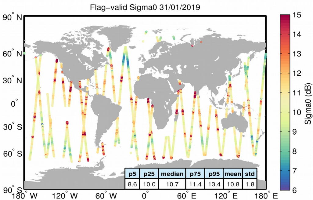
Figure 23. Geographical distribution of flag-valid sigma0 data over oceans and lakes for 31/01/2019. The statistical values shown in the table refer to the sigma0 in dB and are calculated over all measurements shown in the figure.
