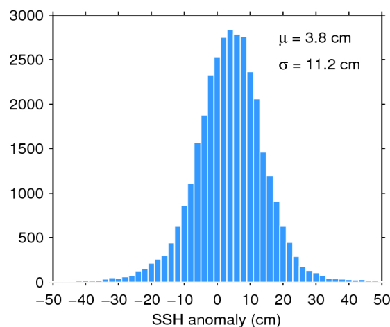
Figure 11. Histogram of science-valid SSH anomaly over oceans and lakes for 29/01/2019. The mean ( \mu ) and standard deviation ( \sigma ) are also shown. Note that values outside [-50 50] cm are excluded from the histogram for the sake of readability but not from the computation of \mu and \sigma .
