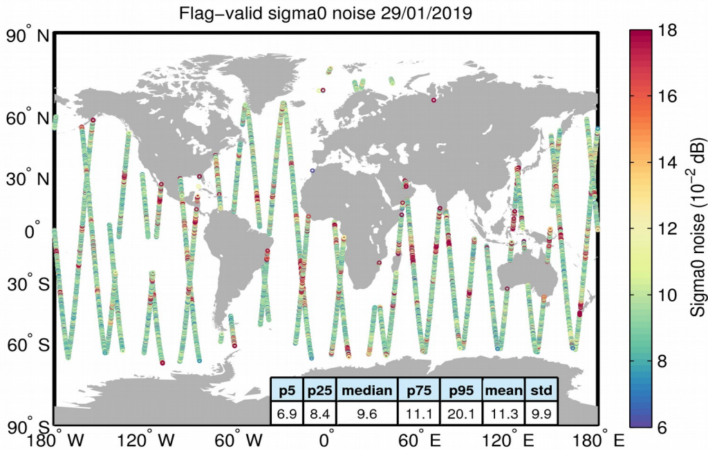
Figure 26. Geographical distribution of flag-valid 20-Hz sigma0 measurement noise over oceans and lakes for 29/01/2019. The statistical values shown in the table refer to the sigma0 noise and are calculated over all measurements shown in the figure.
