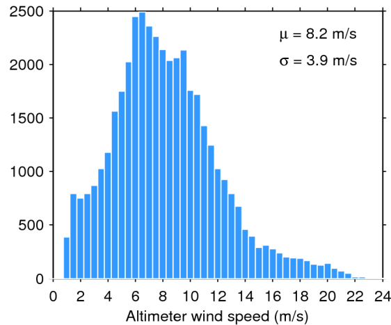
Figure 33. Histogram of flag-valid wind over oceans and lakes for 29/01/2019. The mean ( \mu ) and standard deviation ( \sigma ) are also shown. Note that values larger than 24 m/s are excluded from the histogram for the sake of readability but not from the computation of \mu and \sigma .
