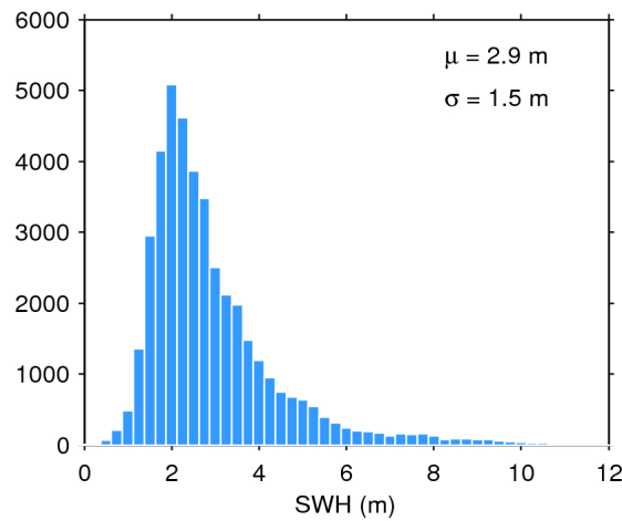
Figure 17. Histogram of flag-valid SWH over oceans and lakes for 29/01/2019. The mean ( \mu ) and standard deviation ( \sigma ) are also shown. Note that values larger than 12 m are excluded from the histogram for the sake of readability but not from the computation of \mu and \sigma .
