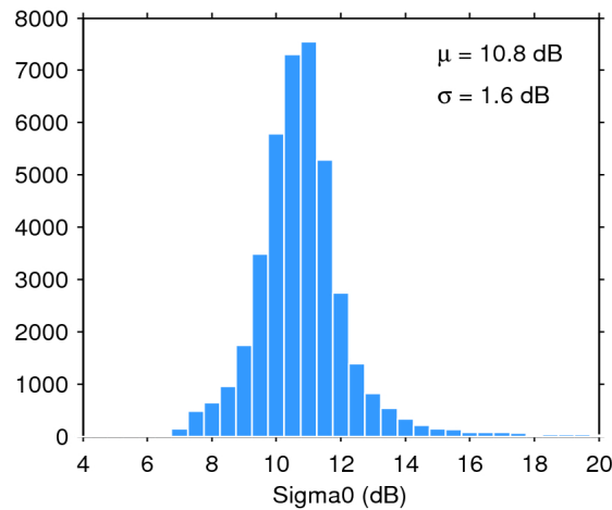
Figure 28. Histogram of science-valid sigma0 over oceans and lakes for 29/01/2019. The mean ( \mu ) and standard deviation ( \sigma ) are also shown. Note that values outside [4 20] dB are excluded from the histogram for the sake of readability but not from the computation of \mu and \sigma .
