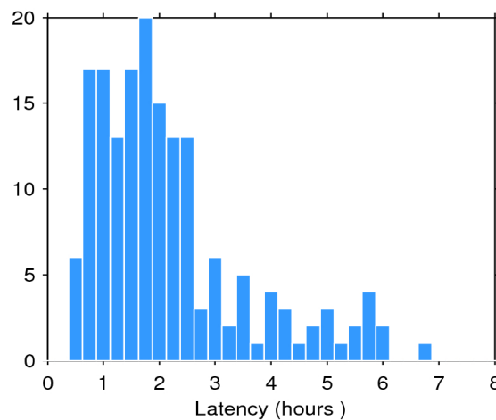
Figure 2. Histogram of the data latency for 29/01/2019. The y-axis denotes the number of files that are made available with a delay of x-hours with respect to the mean time of the records stored in the file.
