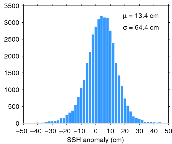
Figure 7. Histogram of flag-valid SSH anomaly over oceans and lakes for 29/01/2019. The mean ( \mu ) and standard deviation ( \sigma ) are also shown. Note that values outside [-50 50] cm are excluded from the histogram for the sake of readability but not from the computation of \mu and \sigma .
