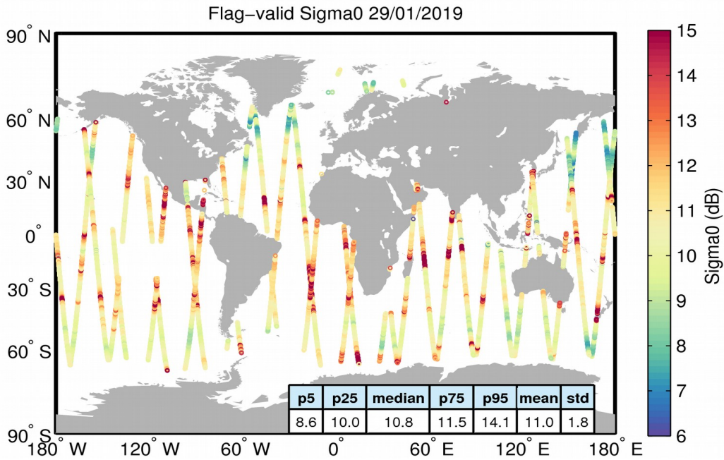
Figure 23. Geographical distribution of flag-valid sigma0 data over oceans and lakes for 29/01/2019. The statistical values shown in the table refer to the sigma0 in dB and are calculated over all measurements shown in the figure.
