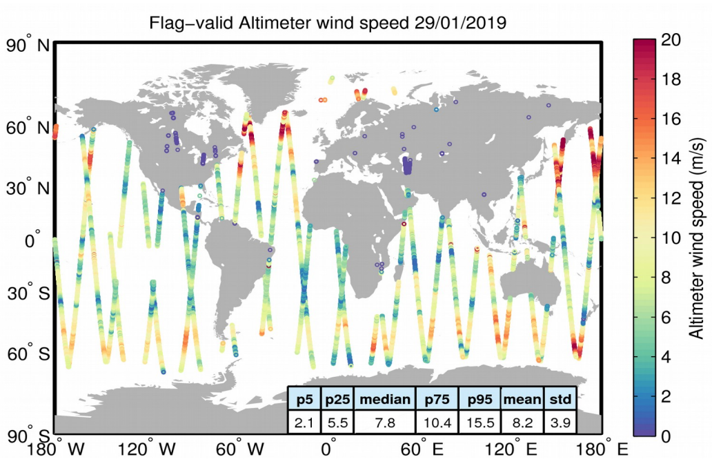
Figure 31. Geographical distribution of flag-valid wind data over oceans and lakes for 29/01/2019. The statistical values shown in the table refer to the wind in m/s and are calculated over all measurements shown in the figure.
