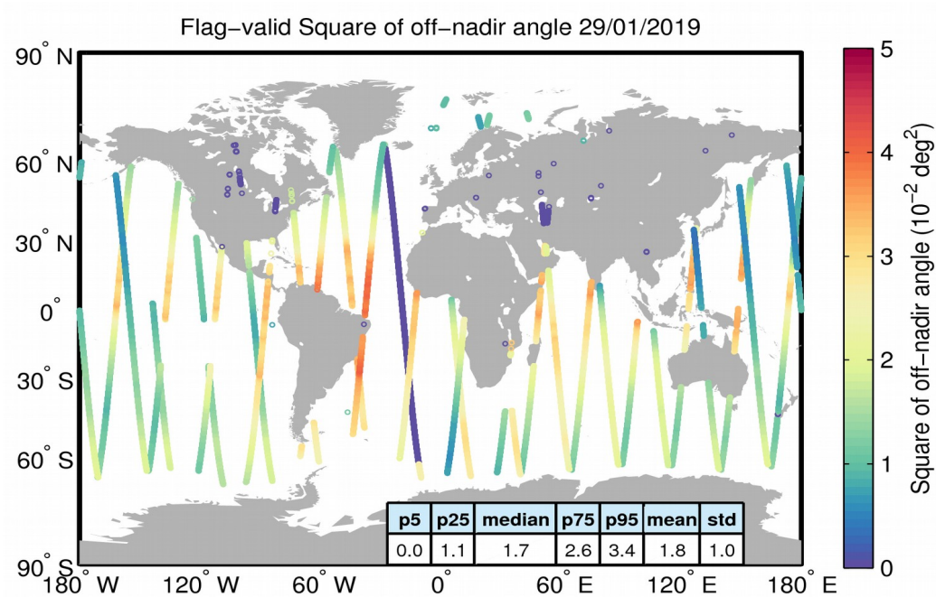
Figure 37. Geographical distribution of flag-valid mispointing data over oceans and lakes for 29/01/2019. The statistical values shown in the table refer to the mispointing in 10^{-2} \text{deg}^2 and are calculated over all measurements shown in the figure.
