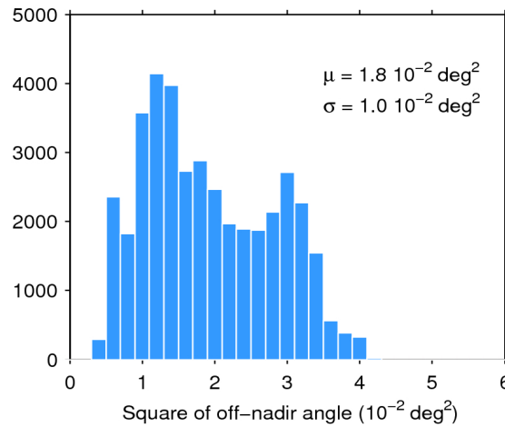
Figure 39. Histogram of flag-valid mispointing over oceans and lakes for 29/01/2019. The mean ( \mu ) and standard deviation ( \sigma ) are also shown. Note that values larger than 6 \cdot 10^{-2} \text{ deg}^2 are excluded from the histogram for the sake of readability but not from the computation of \mu and \sigma .
