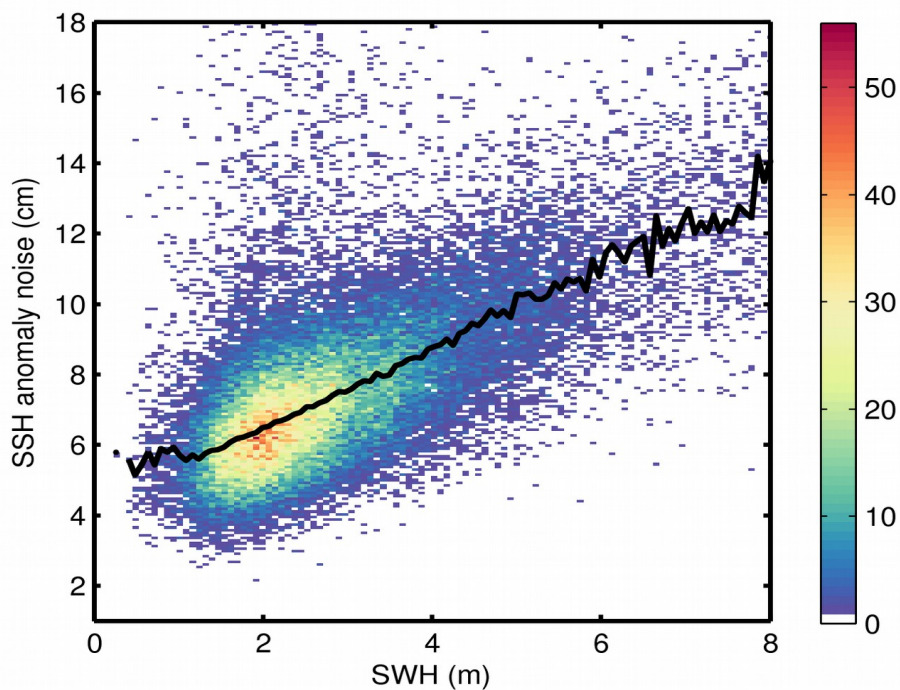
Figure 9. 2D histogram showing flag-valid SSH anomaly noise as a function of SWH for 29/01/2019. The black line denotes the median SSH anomaly noise as a function of SWH.
