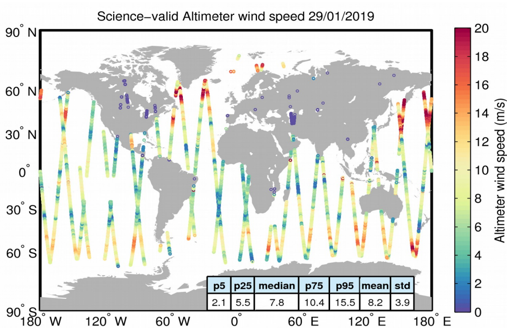
Figure 34. Geographical distribution of science-valid wind data over oceans and lakes for 29/01/2019. The statistical values shown in the table refer to the wind in m/s and are calculated over all measurements shown in the figure. Gray circles denote records that have been rejected based on the editing criteria described in Table 5.
