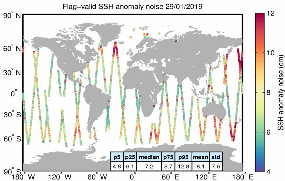
Figure 8. Geographical distribution of flag-valid 20-Hz SSH anomaly measurement noise over oceans and lakes for 29/01/2019. The statistical values shown in the table refer to the SSH anomaly noise and are calculated over all measurements shown in the figure.
