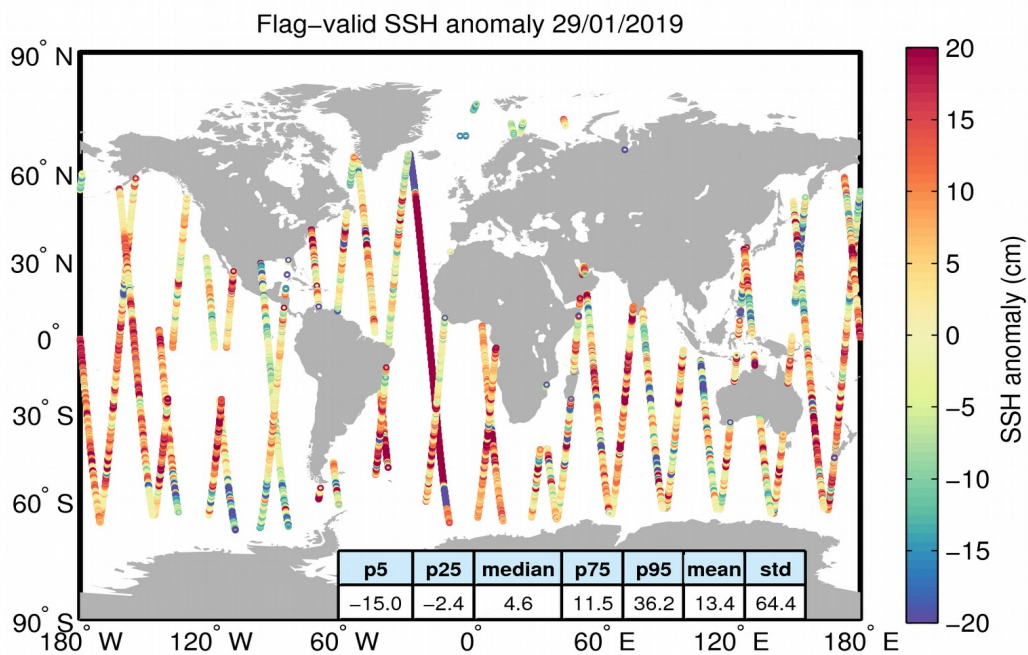
Figure 5. Geographical distribution of flag-valid 1-Hz SSH anomaly data over oceans and lakes for 29/01/2019. The statistical values shown in the table refer to the SSH anomaly in cm and are calculated over all measurements shown in the figure.
