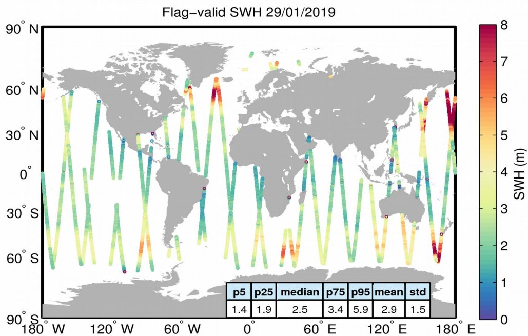
Figure 15. Geographical distribution of flag-valid SWH data over oceans and lakes for 29/01/2019. The statistical values shown in the table refer to the SWH in m and are calculated over all measurements shown in the figure.
