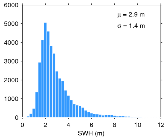
Figure 20. Histogram of science-valid SWH over oceans and lakes for 29/01/2019. The mean ( \mu ) and standard deviation ( \sigma ) are also shown. Note that values larger than 12 m are excluded from the histogram for the sake of readability but not from the computation of \mu and \sigma .
