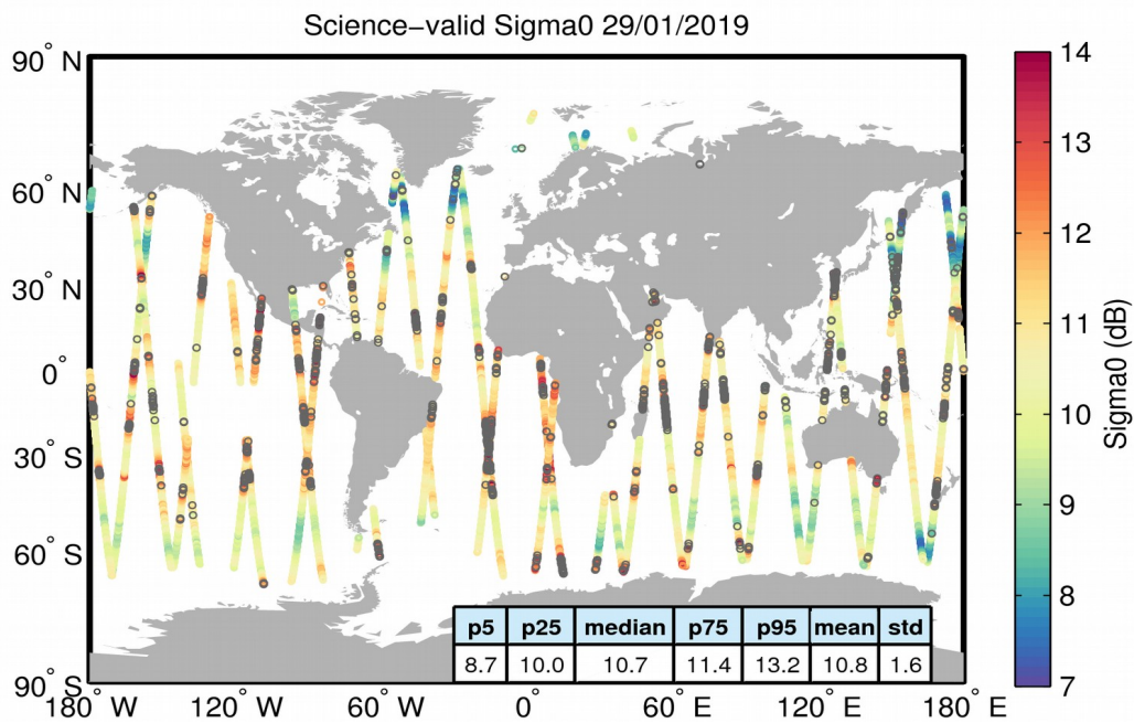
Figure 27. Geographical distribution of science-valid sigma0 data over oceans and lakes for 29/01/2019. The statistical values shown in the table refer to the sigma0 in dB and are calculated over all measurements shown in the figure. Gray circles denote records that have been rejected based on the editing criteria described in Table 4.
