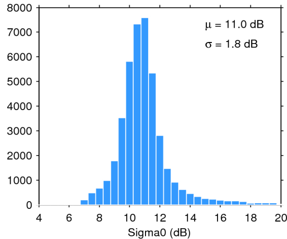
Figure 25. Histogram of flag-valid sigma0 over oceans and lakes for 29/01/2019. The mean ( \mu ) and standard deviation ( \sigma ) are also shown. Note that values outside [4 20] dB are excluded from the histogram for the sake of readability but not from the computation of \mu and \sigma .
