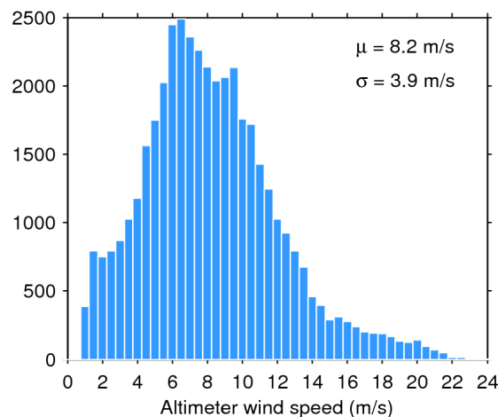
Figure 35. Histogram of science-valid wind over oceans and lakes for 29/01/2019. The mean ( \mu ) and standard deviation ( \sigma ) are also shown. Note that values larger than 24 m/s are excluded from the histogram for the sake of readability but not from the computation of \mu and \sigma .
