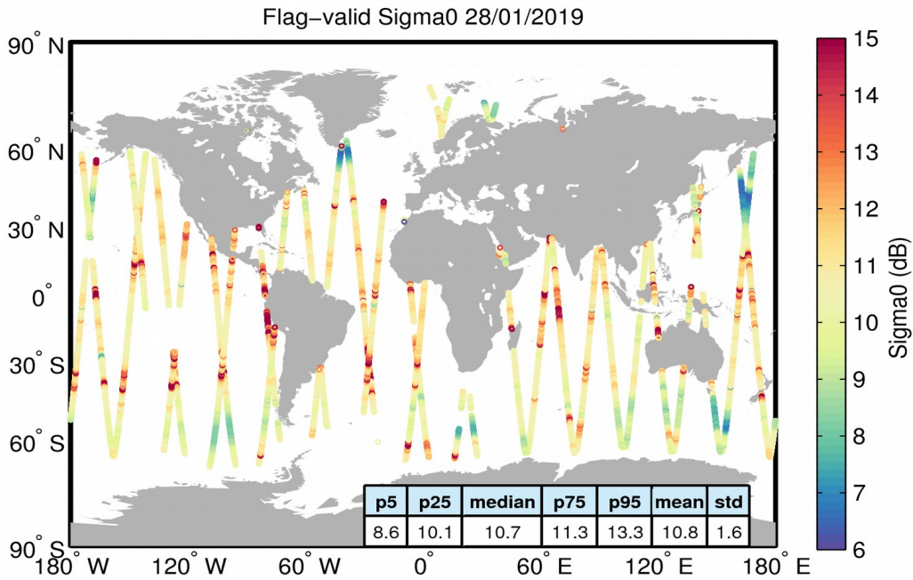
Figure 23. Geographical distribution of flag-valid sigma0 data over oceans and lakes for 28/01/2019. The statistical values shown in the table refer to the sigma0 in dB and are calculated over all measurements shown in the figure.
