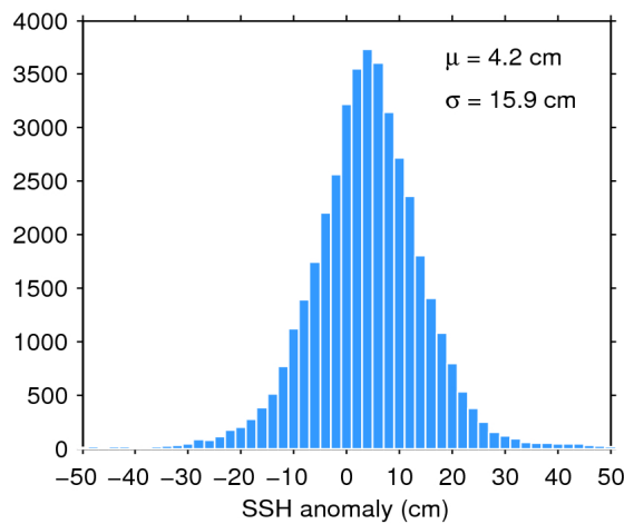
Figure 7. Histogram of flag-valid SSH anomaly over oceans and lakes for 28/01/2019. The mean ( \mu ) and standard deviation ( \sigma ) are also shown. Note that values outside [-50 50] cm are excluded from the histogram for the sake of readability but not from the computation of \mu and \sigma .
