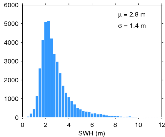
Figure 20. Histogram of science-valid SWH over oceans and lakes for 28/01/2019. The mean ( \mu ) and standard deviation ( \sigma ) are also shown. Note that values larger than 12 m are excluded from the histogram for the sake of readability but not from the computation of \mu and \sigma .
