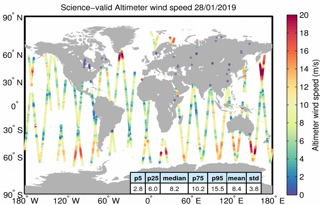
Figure 34. Geographical distribution of science-valid wind data over oceans and lakes for 28/01/2019. The statistical values shown in the table refer to the wind in m/s and are calculated over all measurements shown in the figure. Gray circles denote records that have been rejected based on the editing criteria described in Table 5.
