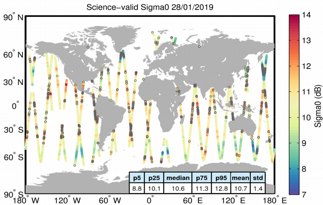
Figure 27. Geographical distribution of science-valid sigma0 data over oceans and lakes for 28/01/2019. The statistical values shown in the table refer to the sigma0 in dB and are calculated over all measurements shown in the figure. Gray circles denote records that have been rejected based on the editing criteria described in Table 4.
