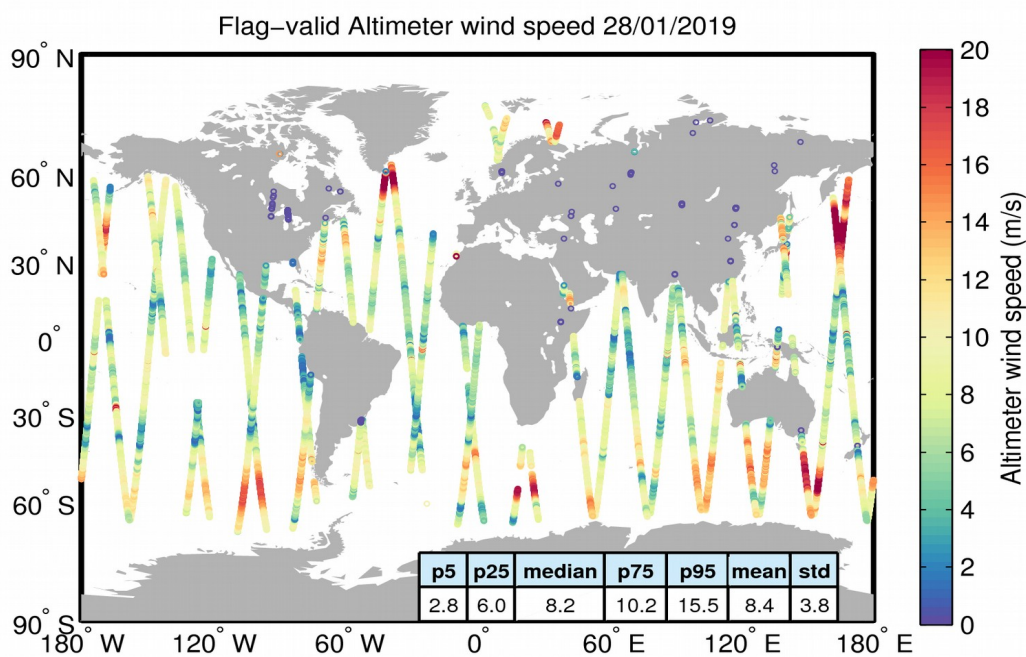
Figure 31. Geographical distribution of flag-valid wind data over oceans and lakes for 28/01/2019. The statistical values shown in the table refer to the wind in m/s and are calculated over all measurements shown in the figure.
