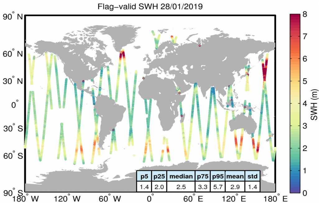
Figure 15. Geographical distribution of flag-valid SWH data over oceans and lakes for 28/01/2019. The statistical values shown in the table refer to the SWH in m and are calculated over all measurements shown in the figure.
