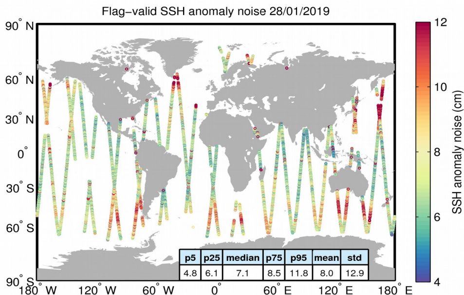
Figure 8. Geographical distribution of flag-valid 20-Hz SSH anomaly measurement noise over oceans and lakes for 28/01/2019. The statistical values shown in the table refer to the SSH anomaly noise and are calculated over all measurements shown in the figure.
