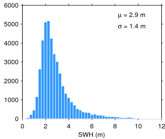
Figure 17. Histogram of flag-valid SWH over oceans and lakes for 28/01/2019. The mean ( \mu ) and standard deviation ( \sigma ) are also shown. Note that values larger than 12 m are excluded from the histogram for the sake of readability but not from the computation of \mu and \sigma .
