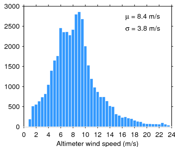
Figure 35. Histogram of science-valid wind over oceans and lakes for 28/01/2019. The mean ( \mu ) and standard deviation ( \sigma ) are also shown. Note that values larger than 24 m/s are excluded from the histogram for the sake of readability but not from the computation of \mu and \sigma .
