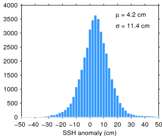
Figure 11. Histogram of science-valid SSH anomaly over oceans and lakes for 28/01/2019. The mean ( \mu ) and standard deviation ( \sigma ) are also shown. Note that values outside [-50 50] cm are excluded from the histogram for the sake of readability but not from the computation of \mu and \sigma .
