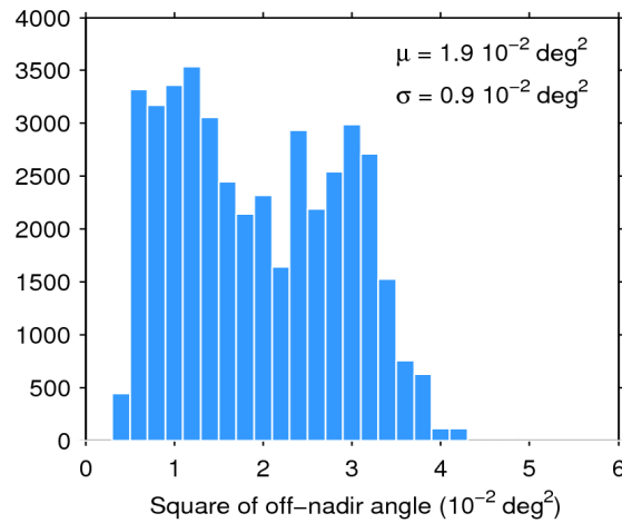
Figure 39. Histogram of flag-valid mispointing over oceans and lakes for 28/01/2019. The mean ( \mu ) and standard deviation ( \sigma ) are also shown. Note that values larger than 6 \cdot 10^{-2} \text{ deg}^2 are excluded from the histogram for the sake of readability but not from the computation of \mu and \sigma .
