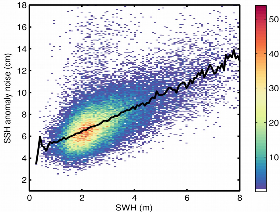
Figure 9. 2D histogram showing flag-valid SSH anomaly noise as a function of SWH for 28/01/2019. The black line denotes the median SSH anomaly noise as a function of SWH.
