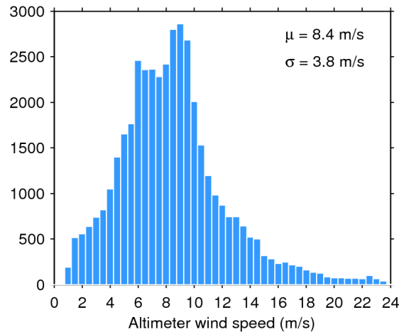
Figure 33. Histogram of flag-valid wind over oceans and lakes for 28/01/2019. The mean ( \mu ) and standard deviation ( \sigma ) are also shown. Note that values larger than 24 m/s are excluded from the histogram for the sake of readability but not from the computation of \mu and \sigma .
