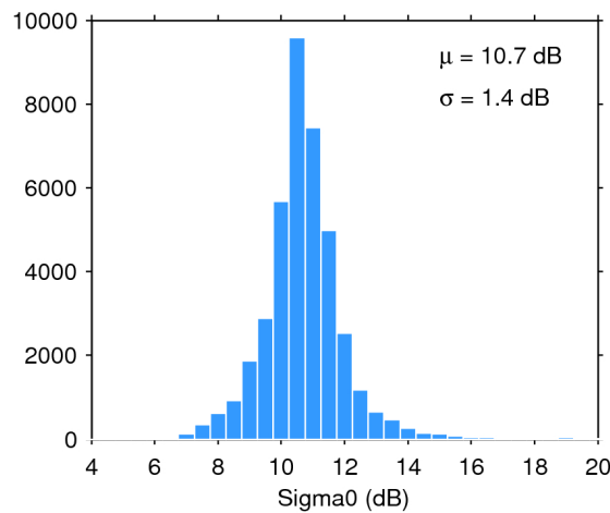
Figure 28. Histogram of science-valid sigma0 over oceans and lakes for 28/01/2019. The mean ( \mu ) and standard deviation ( \sigma ) are also shown. Note that values outside [4 20] dB are excluded from the histogram for the sake of readability but not from the computation of \mu and \sigma .
