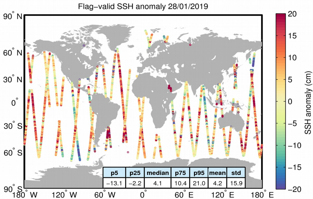
Figure 5. Geographical distribution of flag-valid 1-Hz SSH anomaly data over oceans and lakes for 28/01/2019. The statistical values shown in the table refer to the SSH anomaly in cm and are calculated over all measurements shown in the figure.
