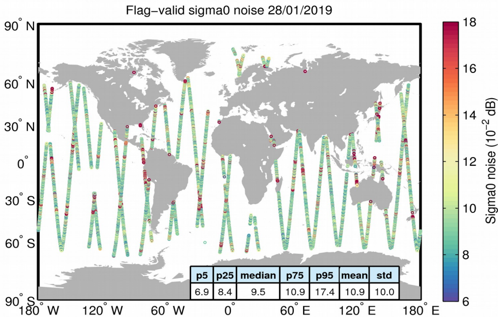
Figure 26. Geographical distribution of flag-valid 20-Hz sigma0 measurement noise over oceans and lakes for 28/01/2019. The statistical values shown in the table refer to the sigma0 noise and are calculated over all measurements shown in the figure.
