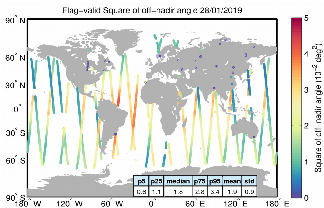
Figure 37. Geographical distribution of flag-valid mispointing data over oceans and lakes for 28/01/2019. The statistical values shown in the table refer to the mispointing in 10^{-2} deg 2 and are calculated over all measurements shown in the figure.
