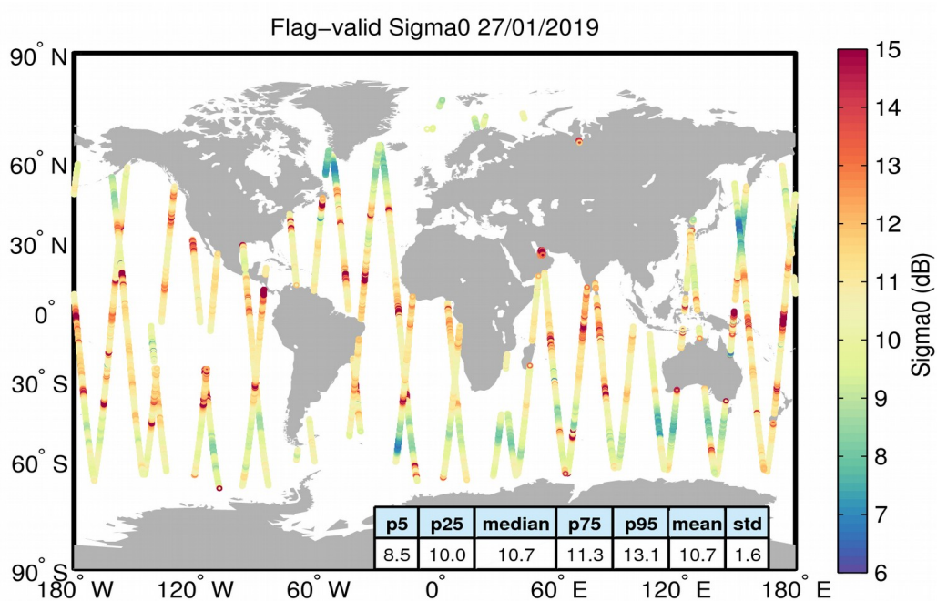
Figure 23. Geographical distribution of flag-valid sigma0 data over oceans and lakes for 27/01/2019. The statistical values shown in the table refer to the sigma0 in dB and are calculated over all measurements shown in the figure.
