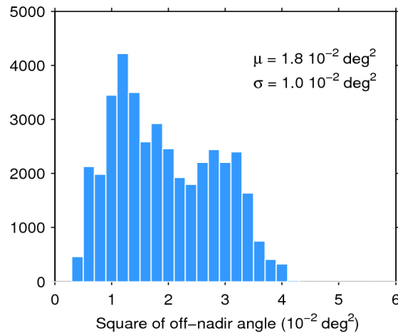
Figure 39. Histogram of flag-valid mispointing over oceans and lakes for 27/01/2019. The mean ( \mu ) and standard deviation ( \sigma ) are also shown. Note that values larger than 6 \cdot 10^{-2} \text{ deg}^2 are excluded from the histogram for the sake of readability but not from the computation of \mu and \sigma .
