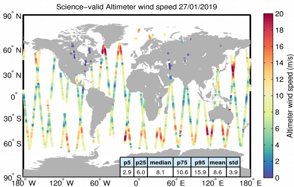
Figure 34. Geographical distribution of science-valid wind data over oceans and lakes for 27/01/2019. The statistical values shown in the table refer to the wind in m/s and are calculated over all measurements shown in the figure. Gray circles denote records that have been rejected based on the editing criteria described in Table 5.
