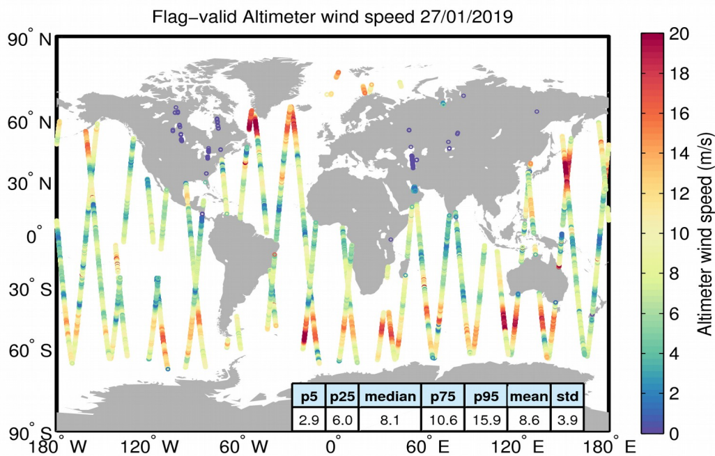
Figure 31. Geographical distribution of flag-valid wind data over oceans and lakes for 27/01/2019. The statistical values shown in the table refer to the wind in m/s and are calculated over all measurements shown in the figure.
