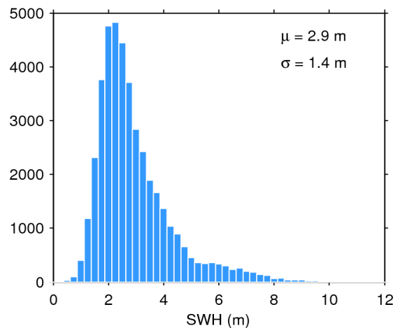
Figure 17. Histogram of flag-valid SWH over oceans and lakes for 27/01/2019. The mean ( \mu ) and standard deviation ( \sigma ) are also shown. Note that values larger than 12 m are excluded from the histogram for the sake of readability but not from the computation of \mu and \sigma .
