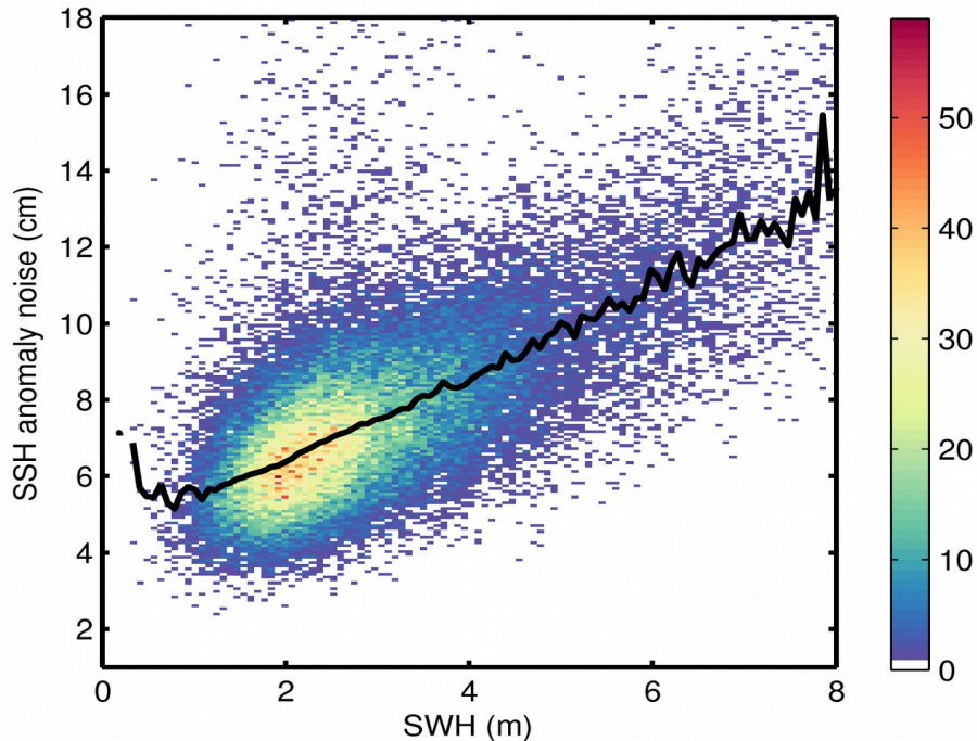
Figure 9. 2D histogram showing flag-valid SSH anomaly noise as a function of SWH for 27/01/2019. The black line denotes the median SSH anomaly noise as a function of SWH.
