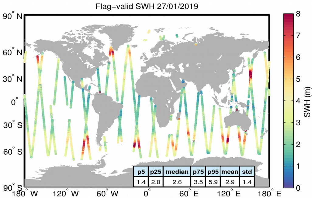
Figure 15. Geographical distribution of flag-valid SWH data over oceans and lakes for 27/01/2019. The statistical values shown in the table refer to the SWH in m and are calculated over all measurements shown in the figure.
