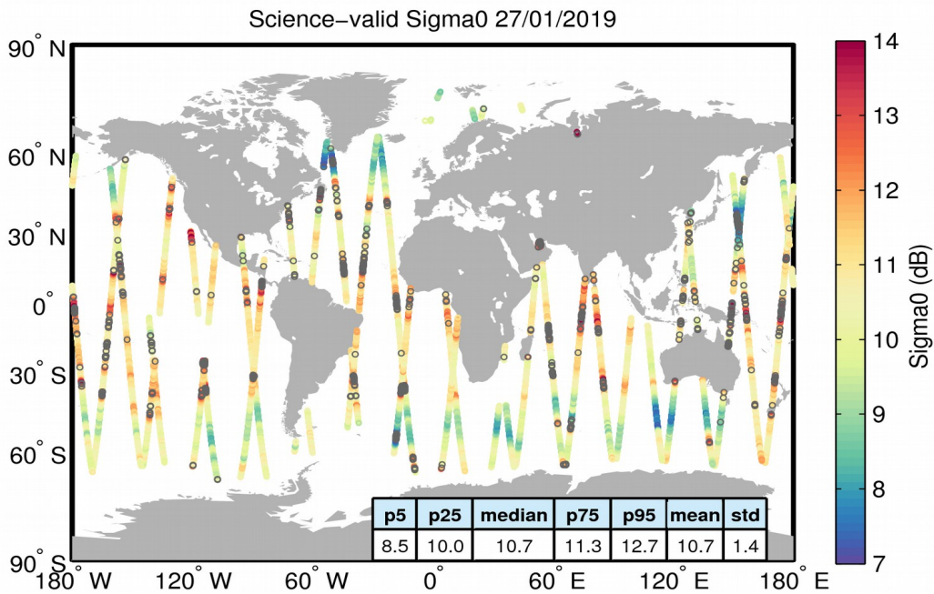
Figure 27. Geographical distribution of science-valid sigma0 data over oceans and lakes for 27/01/2019. The statistical values shown in the table refer to the sigma0 in dB and are calculated over all measurements shown in the figure. Gray circles denote records that have been rejected based on the editing criteria described in Table 4.
