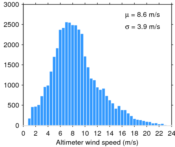
Figure 33. Histogram of flag-valid wind over oceans and lakes for 27/01/2019. The mean ( \mu ) and standard deviation ( \sigma ) are also shown. Note that values larger than 24 m/s are excluded from the histogram for the sake of readability but not from the computation of \mu and \sigma .
