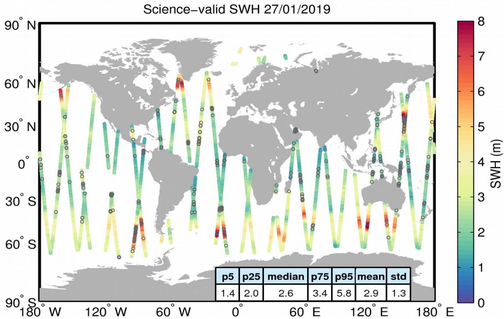
Figure 19. Geographical distribution of science-valid SWH data over oceans and lakes for 27/01/2019. The statistical values shown in the table refer to the SWH in m and are calculated over all measurements shown in the figure. Gray circles denote records that have been rejected based on the editing criteria described in Table 3.
