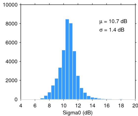
Figure 28. Histogram of science-valid sigma0 over oceans and lakes for 27/01/2019. The mean ( \mu ) and standard deviation ( \sigma ) are also shown. Note that values outside [4 20] dB are excluded from the histogram for the sake of readability but not from the computation of \mu and \sigma .
