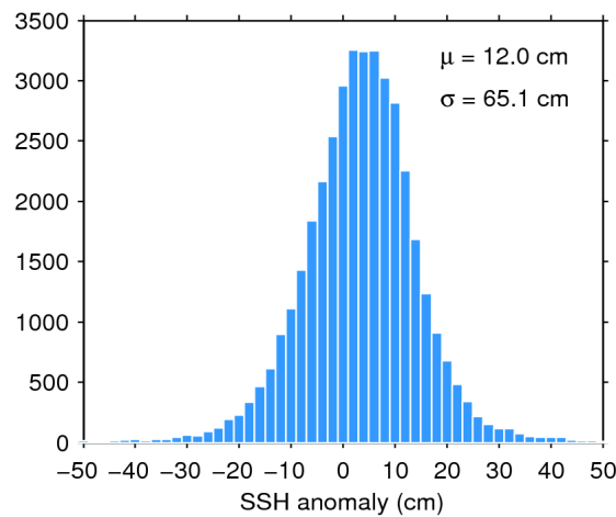
Figure 7. Histogram of flag-valid SSH anomaly over oceans and lakes for 27/01/2019. The mean ( \mu ) and standard deviation ( \sigma ) are also shown. Note that values outside [-50\ 50] cm are excluded from the histogram for the sake of readability but not from the computation of \mu and \sigma .
