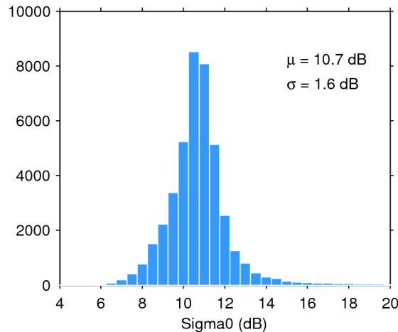
Figure 25. Histogram of flag-valid sigma0 over oceans and lakes for 27/01/2019. The mean ( \mu ) and standard deviation ( \sigma ) are also shown. Note that values outside [4 20] dB are excluded from the histogram for the sake of readability but not from the computation of \mu and \sigma .
