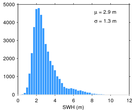
Figure 20. Histogram of science-valid SWH over oceans and lakes for 27/01/2019. The mean ( \mu ) and standard deviation ( \sigma ) are also shown. Note that values larger than 12 m are excluded from the histogram for the sake of readability but not from the computation of \mu and \sigma .
