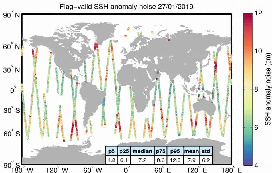
Figure 8. Geographical distribution of flag-valid 20-Hz SSH anomaly measurement noise over oceans and lakes for 27/01/2019. The statistical values shown in the table refer to the SSH anomaly noise and are calculated over all measurements shown in the figure.
