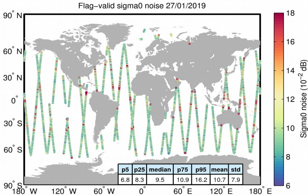
Figure 26. Geographical distribution of flag-valid 20-Hz sigma0 measurement noise over oceans and lakes for 27/01/2019. The statistical values shown in the table refer to the sigma0 noise and are calculated over all measurements shown in the figure.
