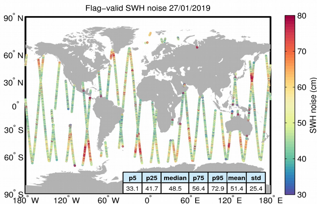
Figure 18. Geographical distribution of flag-valid 20-Hz SWH measurement noise over oceans and lakes for 27/01/2019. The statistical values shown in the table refer to the SWH noise and are calculated over all measurements shown in the figure.
