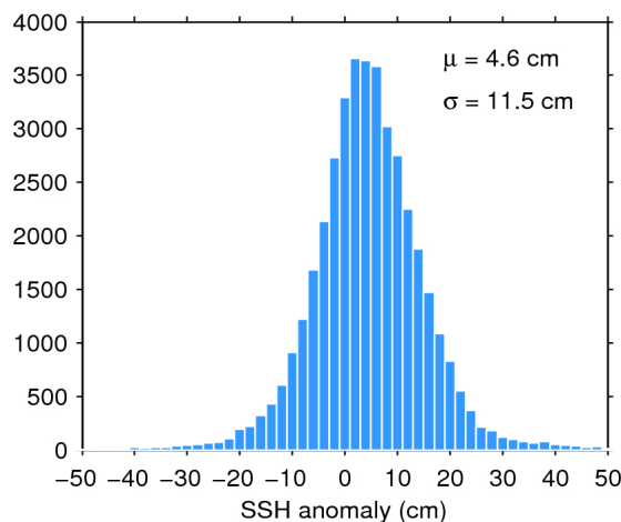
Figure 11. Histogram of science-valid SSH anomaly over oceans and lakes for 26/01/2019. The mean ( \mu ) and standard deviation ( \sigma ) are also shown. Note that values outside [-50 50] cm are excluded from the histogram for the sake of readability but not from the computation of \mu and \sigma .
