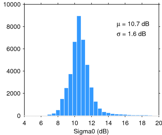
Figure 25. Histogram of flag-valid sigma0 over oceans and lakes for 26/01/2019. The mean ( \mu ) and standard deviation ( \sigma ) are also shown. Note that values outside [4 20] dB are excluded from the histogram for the sake of readability but not from the computation of \mu and \sigma .
