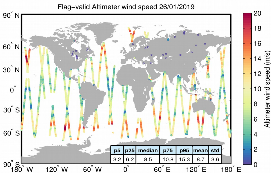
Figure 31. Geographical distribution of flag-valid wind data over oceans and lakes for 26/01/2019. The statistical values shown in the table refer to the wind in m/s and are calculated over all measurements shown in the figure.
