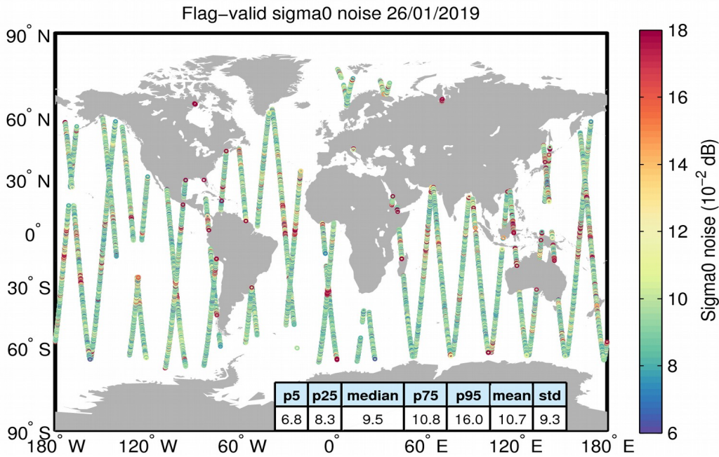
Figure 26. Geographical distribution of flag-valid 20-Hz sigma0 measurement noise over oceans and lakes for 26/01/2019. The statistical values shown in the table refer to the sigma0 noise and are calculated over all measurements shown in the figure.
