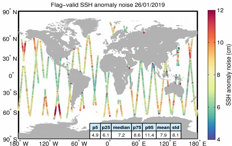
Figure 8. Geographical distribution of flag-valid 20-Hz SSH anomaly measurement noise over oceans and lakes for 26/01/2019. The statistical values shown in the table refer to the SSH anomaly noise and are calculated over all measurements shown in the figure.
