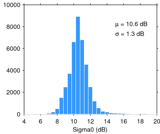
Figure 28. Histogram of science-valid sigma0 over oceans and lakes for 26/01/2019. The mean ( \mu ) and standard deviation ( \sigma ) are also shown. Note that values outside [4 20] dB are excluded from the histogram for the sake of readability but not from the computation of \mu and \sigma .
