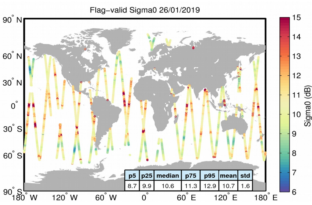
Figure 23. Geographical distribution of flag-valid sigma0 data over oceans and lakes for 26/01/2019. The statistical values shown in the table refer to the sigma0 in dB and are calculated over all measurements shown in the figure.
