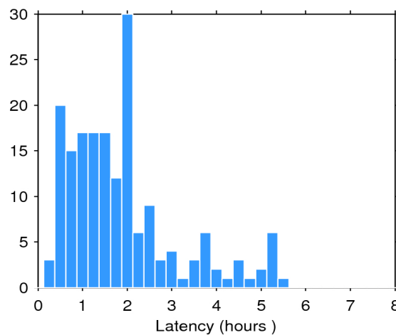
Figure 2. Histogram of the data latency for 26/01/2019. The y-axis denotes the number of files that are made available with a delay of x-hours with respect to the mean time of the records stored in the file.
