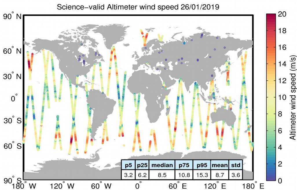
Figure 34. Geographical distribution of science-valid wind data over oceans and lakes for 26/01/2019. The statistical values shown in the table refer to the wind in m/s and are calculated over all measurements shown in the figure. Gray circles denote records that have been rejected based on the editing criteria described in Table 5.
