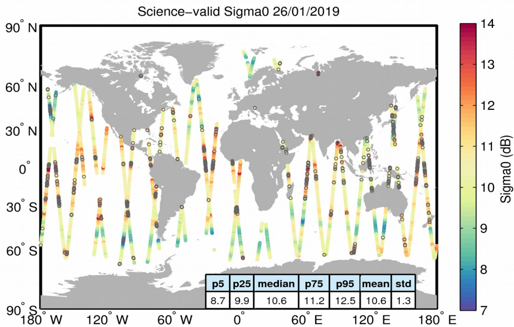
Figure 27. Geographical distribution of science-valid sigma0 data over oceans and lakes for 26/01/2019. The statistical values shown in the table refer to the sigma0 in dB and are calculated over all measurements shown in the figure. Gray circles denote records that have been rejected based on the editing criteria described in Table 4.
