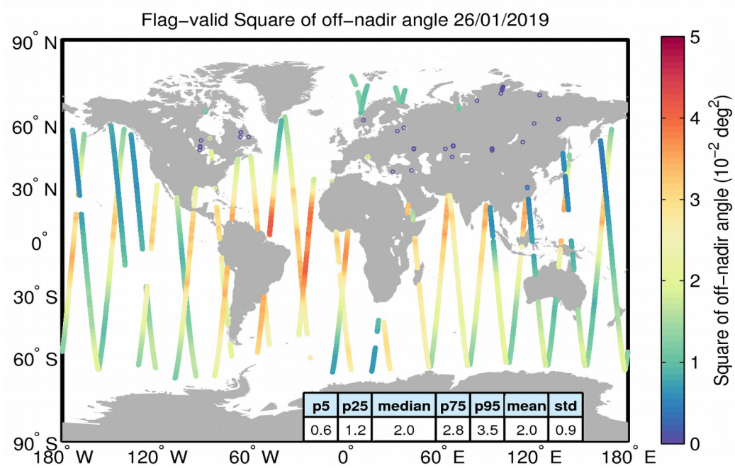
Figure 37. Geographical distribution of flag-valid mispointing data over oceans and lakes for 26/01/2019. The statistical values shown in the table refer to the mispointing in 10^{-2} \text{ deg}^2 and are calculated over all measurements shown in the figure.
