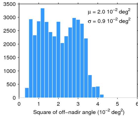
Figure 39. Histogram of flag-valid mispointing over oceans and lakes for 26/01/2019. The mean ( \mu ) and standard deviation ( \sigma ) are also shown. Note that values larger than 6 \cdot 10^{-2} \text{ deg}^2 are excluded from the histogram for the sake of readability but not from the computation of \mu and \sigma .
