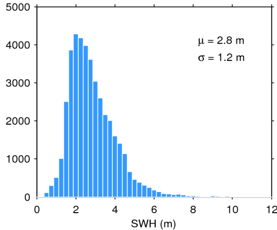
Figure 20. Histogram of science-valid SWH over oceans and lakes for 26/01/2019. The mean ( \mu ) and standard deviation ( \sigma ) are also shown. Note that values larger than 12 m are excluded from the histogram for the sake of readability but not from the computation of \mu and \sigma .
