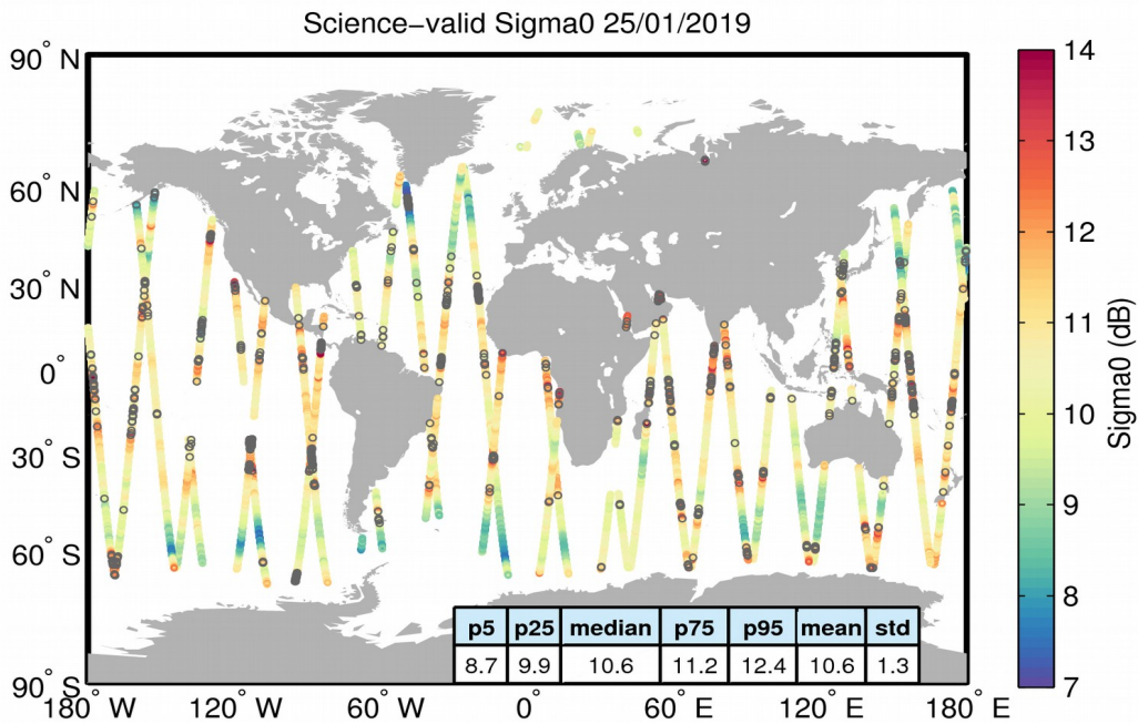
Figure 27. Geographical distribution of science-valid sigma0 data over oceans and lakes for 25/01/2019. The statistical values shown in the table refer to the sigma0 in dB and are calculated over all measurements shown in the figure. Gray circles denote records that have been rejected based on the editing criteria described in Table 4.
