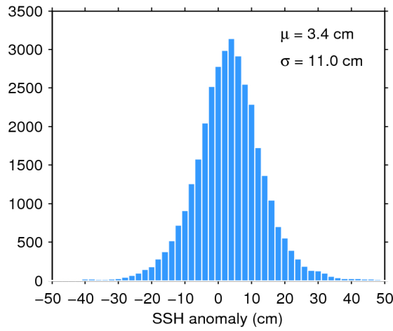
Figure 11. Histogram of science-valid SSH anomaly over oceans and lakes for 25/01/2019. The mean ( \mu ) and standard deviation ( \sigma ) are also shown. Note that values outside [-50 50] cm are excluded from the histogram for the sake of readability but not from the computation of \mu and \sigma .
