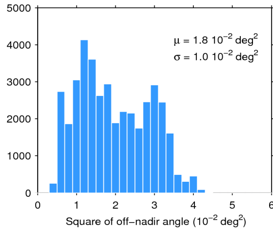
Figure 39. Histogram of flag-valid mispointing over oceans and lakes for 25/01/2019. The mean ( \mu ) and standard deviation ( \sigma ) are also shown. Note that values larger than 6 \cdot 10^{-2} \text{ deg}^2 are excluded from the histogram for the sake of readability but not from the computation of \mu and \sigma .
