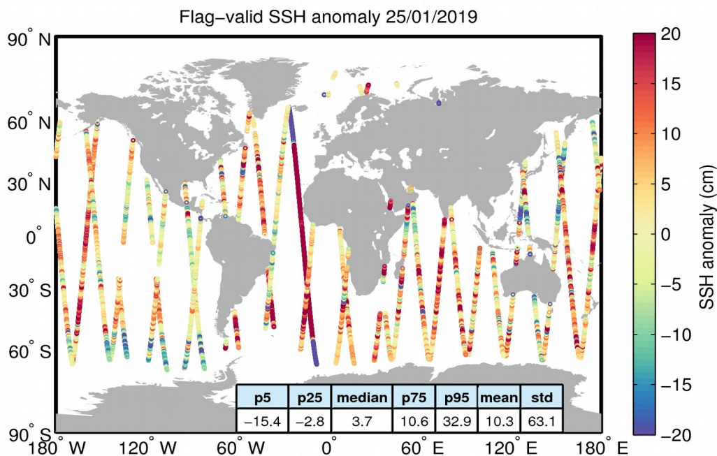
Figure 5. Geographical distribution of flag-valid 1-Hz SSH anomaly data over oceans and lakes for 25/01/2019. The statistical values shown in the table refer to the SSH anomaly in cm and are calculated over all measurements shown in the figure.
