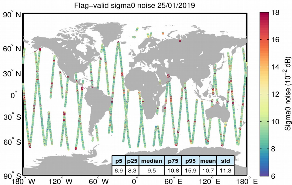
Figure 26. Geographical distribution of flag-valid 20-Hz sigma0 measurement noise over oceans and lakes for 25/01/2019. The statistical values shown in the table refer to the sigma0 noise and are calculated over all measurements shown in the figure.
