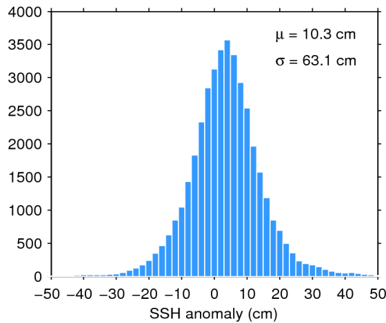
Figure 7. Histogram of flag-valid SSH anomaly over oceans and lakes for 25/01/2019. The mean ( \mu ) and standard deviation ( \sigma ) are also shown. Note that values outside [-50 50] cm are excluded from the histogram for the sake of readability but not from the computation of \mu and \sigma .
