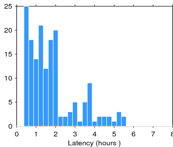
Figure 2. Histogram of the data latency for 25/01/2019. The y-axis denotes the number of files that are made available with a delay of x-hours with respect to the mean time of the records stored in the file.
