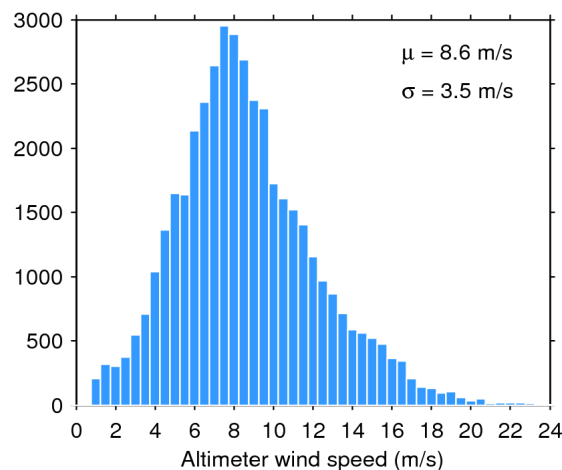
Figure 35. Histogram of science-valid wind over oceans and lakes for 25/01/2019. The mean ( \mu ) and standard deviation ( \sigma ) are also shown. Note that values larger than 24 m/s are excluded from the histogram for the sake of readability but not from the computation of \mu and \sigma .
