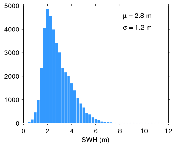
Figure 17. Histogram of flag-valid SWH over oceans and lakes for 25/01/2019. The mean ( \mu ) and standard deviation ( \sigma ) are also shown. Note that values larger than 12 m are excluded from the histogram for the sake of readability but not from the computation of \mu and \sigma .
