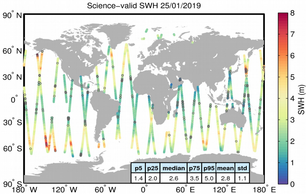
Figure 19. Geographical distribution of science-valid SWH data over oceans and lakes for 25/01/2019. The statistical values shown in the table refer to the SWH in m and are calculated over all measurements shown in the figure. Gray circles denote records that have been rejected based on the editing criteria described in Table 3.
