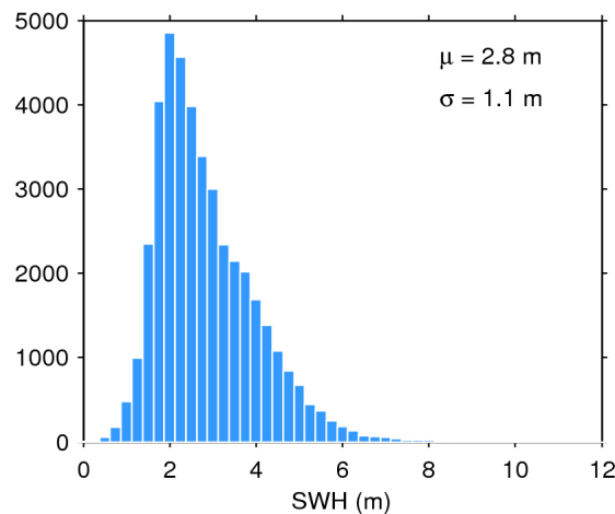
Figure 20. Histogram of science-valid SWH over oceans and lakes for 25/01/2019. The mean ( \mu ) and standard deviation ( \sigma ) are also shown. Note that values larger than 12 m are excluded from the histogram for the sake of readability but not from the computation of \mu and \sigma .
