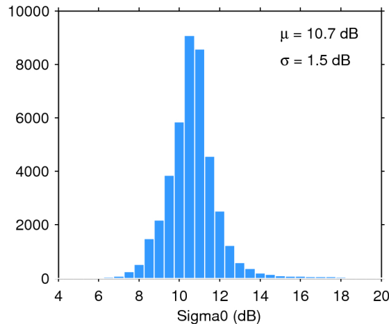
Figure 25. Histogram of flag-valid sigma0 over oceans and lakes for 25/01/2019. The mean ( \mu ) and standard deviation ( \sigma ) are also shown. Note that values outside [4 20] dB are excluded from the histogram for the sake of readability but not from the computation of \mu and \sigma .
