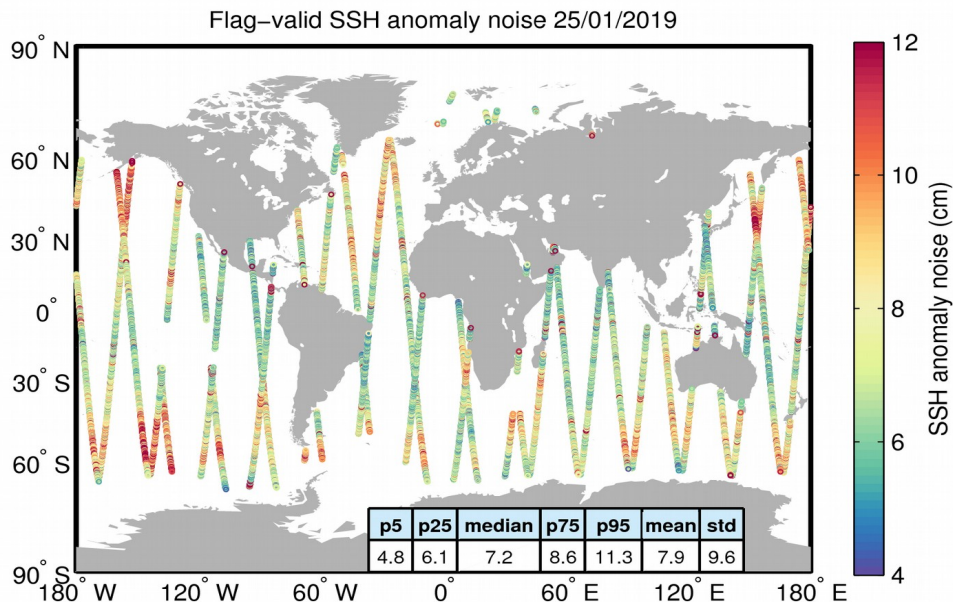
Figure 8. Geographical distribution of flag-valid 20-Hz SSH anomaly measurement noise over oceans and lakes for 25/01/2019. The statistical values shown in the table refer to the SSH anomaly noise and are calculated over all measurements shown in the figure.
