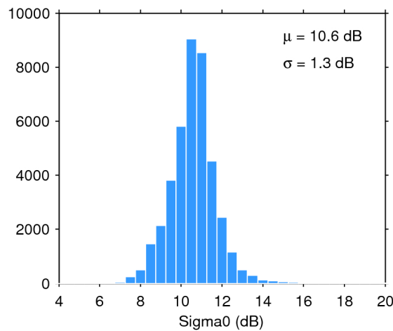
Figure 28. Histogram of science-valid sigma0 over oceans and lakes for 25/01/2019. The mean ( \mu ) and standard deviation ( \sigma ) are also shown. Note that values outside [4 20] dB are excluded from the histogram for the sake of readability but not from the computation of \mu and \sigma .
