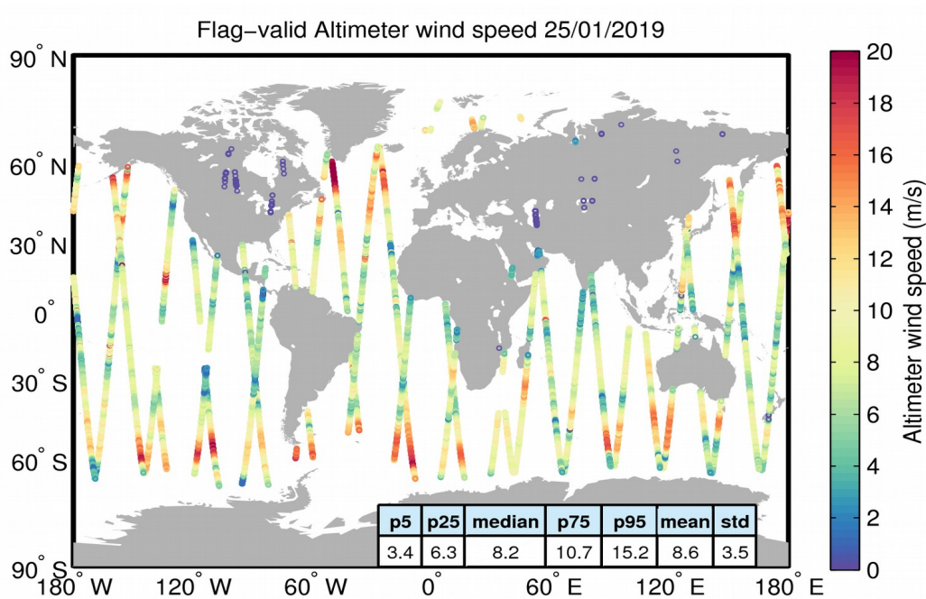
Figure 31. Geographical distribution of flag-valid wind data over oceans and lakes for 25/01/2019. The statistical values shown in the table refer to the wind in m/s and are calculated over all measurements shown in the figure.
