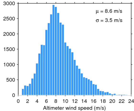
Figure 33. Histogram of flag-valid wind over oceans and lakes for 25/01/2019. The mean ( \mu ) and standard deviation ( \sigma ) are also shown. Note that values larger than 24 m/s are excluded from the histogram for the sake of readability but not from the computation of \mu and \sigma .
