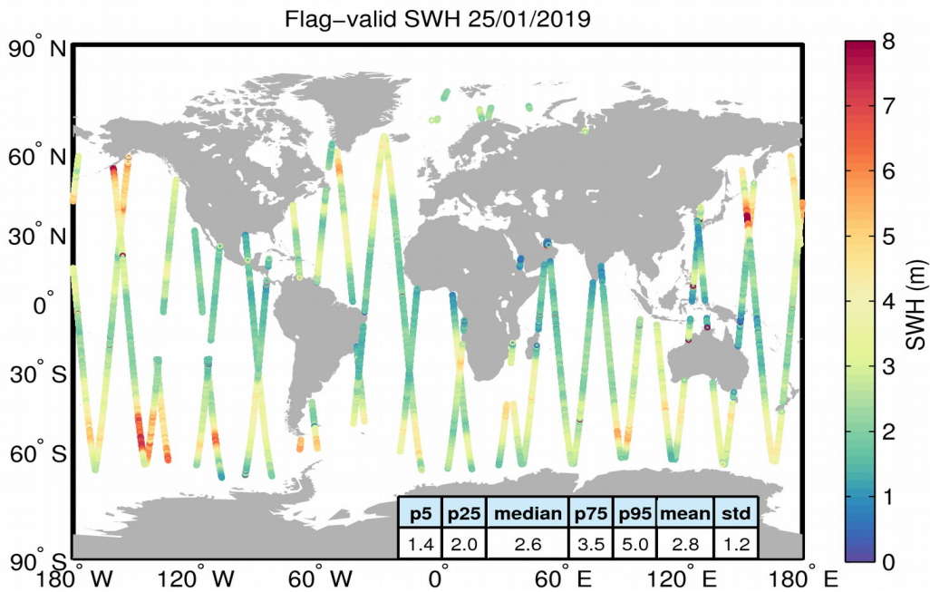
Figure 15. Geographical distribution of flag-valid SWH data over oceans and lakes for 25/01/2019. The statistical values shown in the table refer to the SWH in m and are calculated over all measurements shown in the figure.
