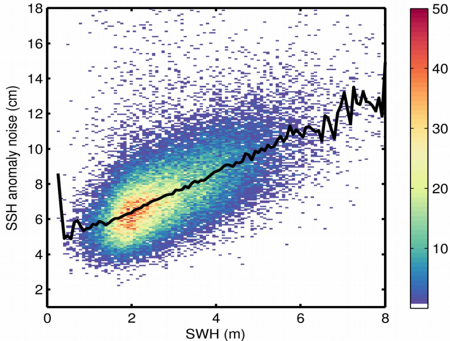
Figure 9. 2D histogram showing flag-valid SSH anomaly noise as a function of SWH for 25/01/2019. The black line denotes the median SSH anomaly noise as a function of SWH.
