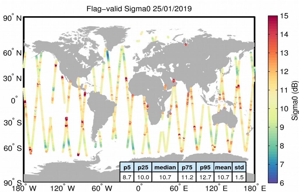
Figure 23. Geographical distribution of flag-valid sigma0 data over oceans and lakes for 25/01/2019. The statistical values shown in the table refer to the sigma0 in dB and are calculated over all measurements shown in the figure.
