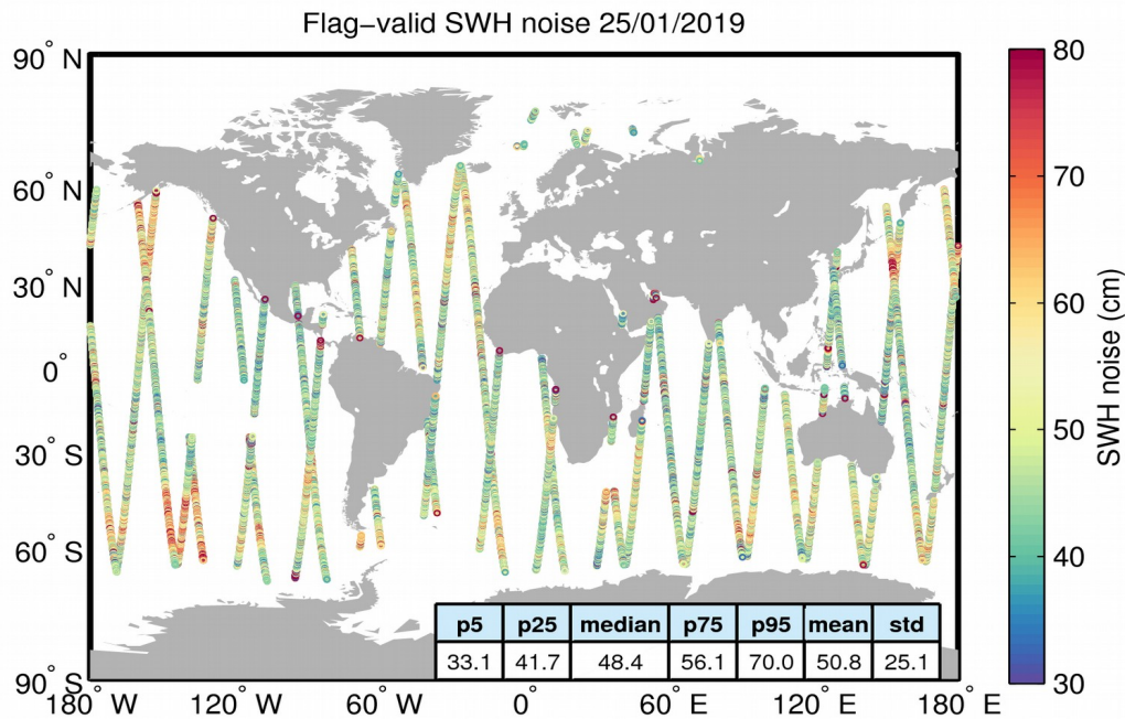
Figure 18. Geographical distribution of flag-valid 20-Hz SWH measurement noise over oceans and lakes for 25/01/2019. The statistical values shown in the figure refer to the SWH noise and are calculated over all measurements shown in the figure.
