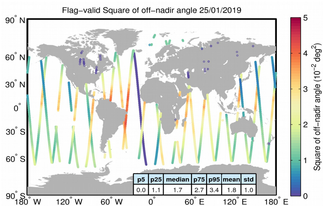
Figure 37. Geographical distribution of flag-valid mispointing data over oceans and lakes for 25/01/2019. The statistical values shown in the table refer to the mispointing in 10^{-2} \text{ deg}^2 and are calculated over all measurements shown in the figure.
