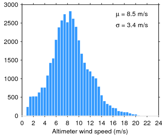
Figure 33. Histogram of flag-valid wind over oceans and lakes for 24/01/2019. The mean ( \mu ) and standard deviation ( \sigma ) are also shown. Note that values larger than 24 m/s are excluded from the histogram for the sake of readability but not from the computation of \mu and \sigma .
