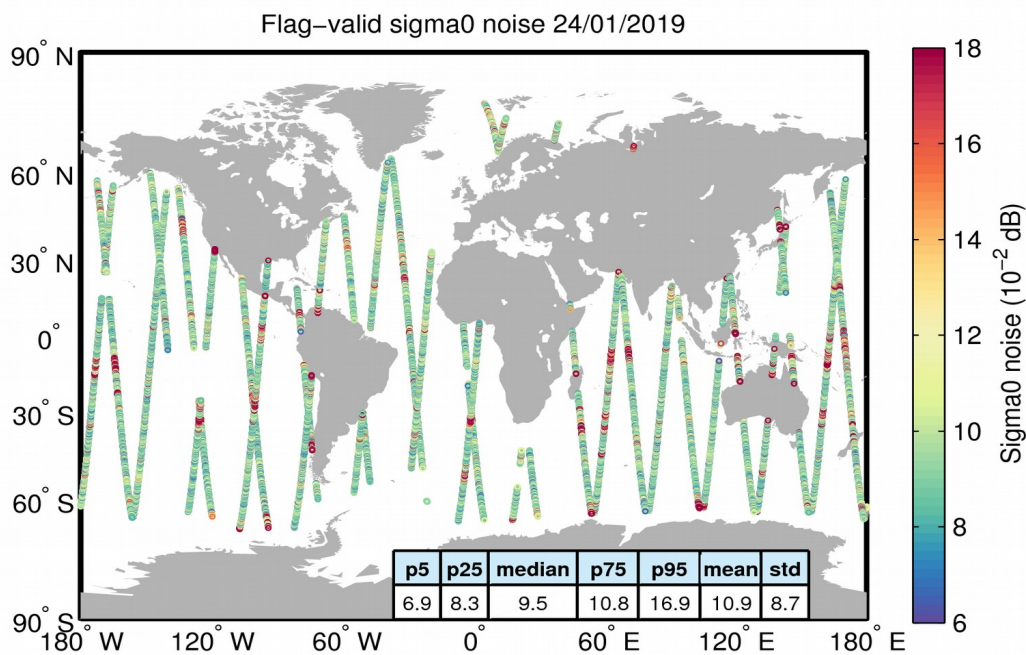
Figure 26. Geographical distribution of flag-valid 20-Hz sigma0 measurement noise over oceans and lakes for 24/01/2019. The statistical values shown in the table refer to the sigma0 noise and are calculated over all measurements shown in the figure.
