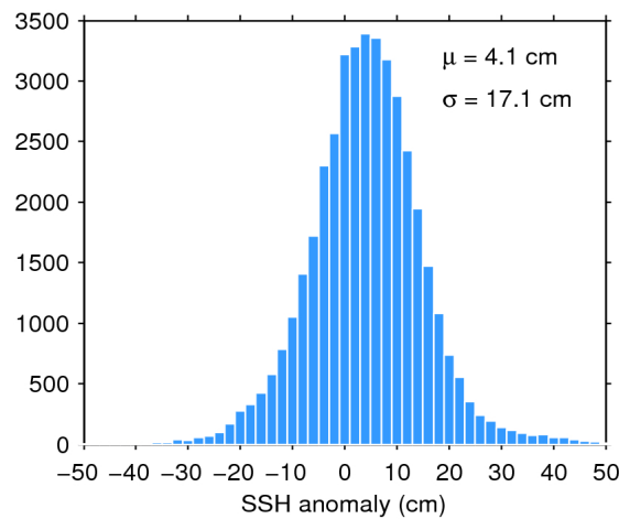
Figure 7. Histogram of flag-valid SSH anomaly over oceans and lakes for 24/01/2019. The mean ( \mu ) and standard deviation ( \sigma ) are also shown. Note that values outside [-50\ 50] cm are excluded from the histogram for the sake of readability but not from the computation of \mu and \sigma .
