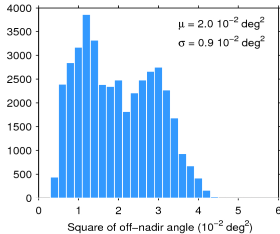
Figure 39. Histogram of flag-valid mispointing over oceans and lakes for 24/01/2019. The mean ( \mu ) and standard deviation ( \sigma ) are also shown. Note that values larger than 6 \cdot 10^{-2} \text{ deg}^2 are excluded from the histogram for the sake of readability but not from the computation of \mu and \sigma .
