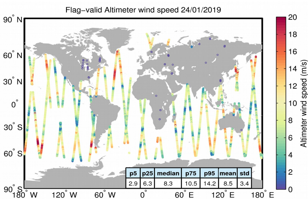
Figure 31. Geographical distribution of flag-valid wind data over oceans and lakes for 24/01/2019. The statistical values shown in the table refer to the wind in m/s and are calculated over all measurements shown in the figure.
