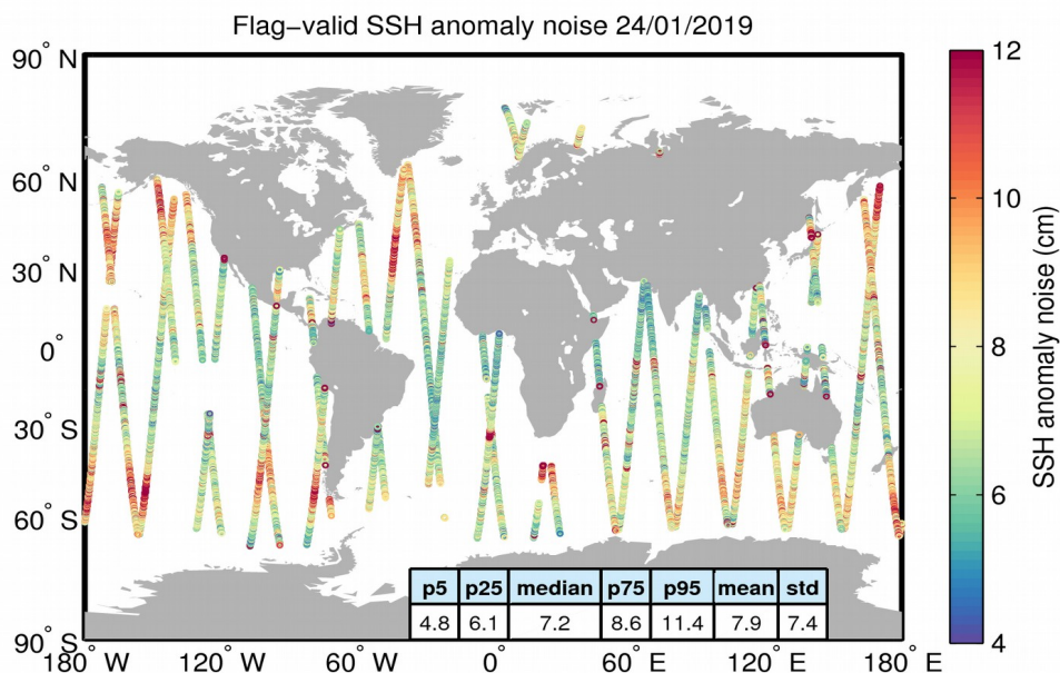
Figure 8. Geographical distribution of flag-valid 20-Hz SSH anomaly measurement noise over oceans and lakes for 24/01/2019. The statistical values shown in the table refer to the SSH anomaly noise and are calculated over all measurements shown in the figure.
