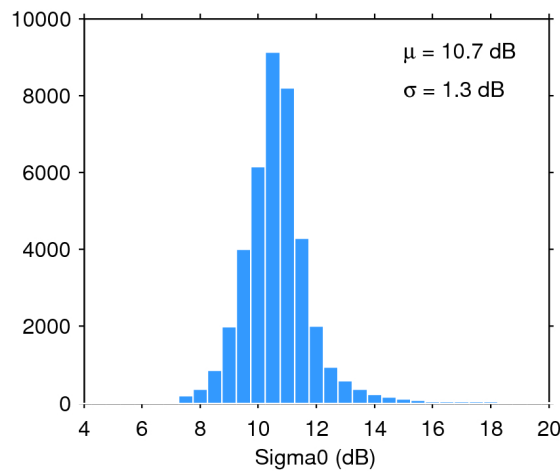
Figure 28. Histogram of science-valid sigma0 over oceans and lakes for 24/01/2019. The mean ( \mu ) and standard deviation ( \sigma ) are also shown. Note that values outside [4 20] dB are excluded from the histogram for the sake of readability but not from the computation of \mu and \sigma .
