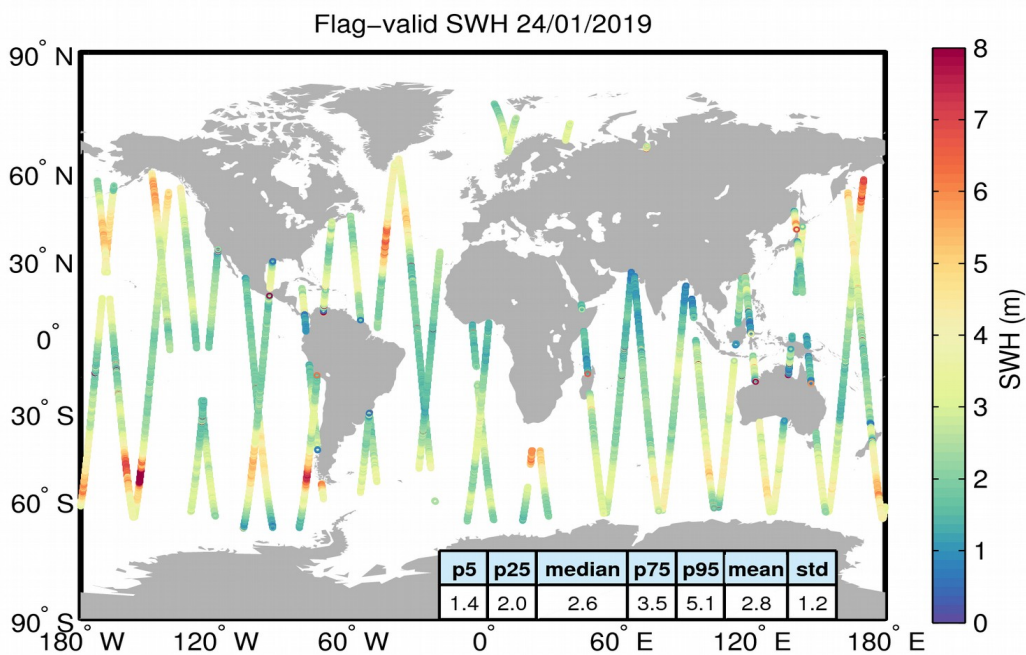
Figure 15. Geographical distribution of flag-valid SWH data over oceans and lakes for 24/01/2019. The statistical values shown in the table refer to the SWH in m and are calculated over all measurements shown in the figure.
