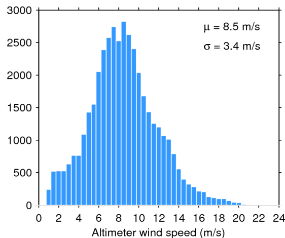
Figure 35. Histogram of science-valid wind over oceans and lakes for 24/01/2019. The mean ( \mu ) and standard deviation ( \sigma ) are also shown. Note that values larger than 24 m/s are excluded from the histogram for the sake of readability but not from the computation of \mu and \sigma .
