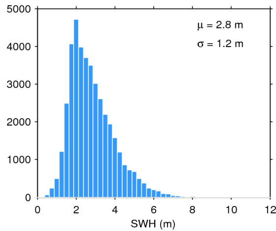
Figure 17. Histogram of flag-valid SWH over oceans and lakes for 24/01/2019. The mean ( \mu ) and standard deviation ( \sigma ) are also shown. Note that values larger than 12 m are excluded from the histogram for the sake of readability but not from the computation of \mu and \sigma .
