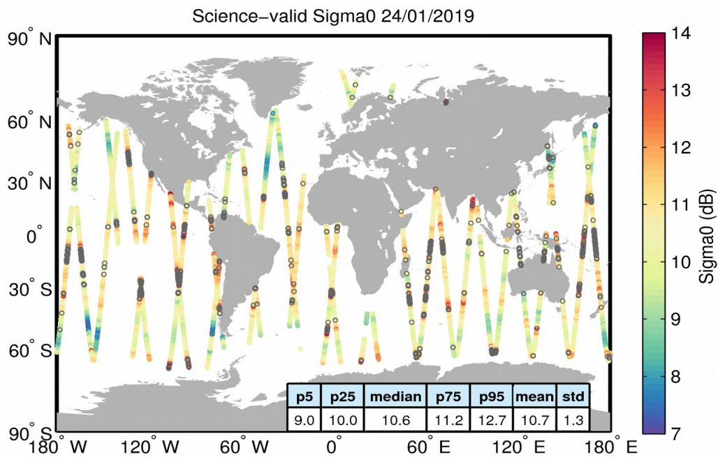
Figure 27. Geographical distribution of science-valid sigma0 data over oceans and lakes for 24/01/2019. The statistical values shown in the table refer to the sigma0 in dB and are calculated over all measurements shown in the figure. Gray circles denote records that have been rejected based on the editing criteria described in Table 4.
