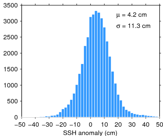
Figure 11. Histogram of science-valid SSH anomaly over oceans and lakes for 24/01/2019. The mean ( \mu ) and standard deviation ( \sigma ) are also shown. Note that values outside [-50 50] cm are excluded from the histogram for the sake of readability but not from the computation of \mu and \sigma .
