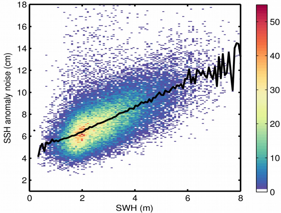
Figure 9. 2D histogram showing flag-valid SSH anomaly noise as a function of SWH for 24/01/2019. The black line denotes the median SSH anomaly noise as a function of SWH.
