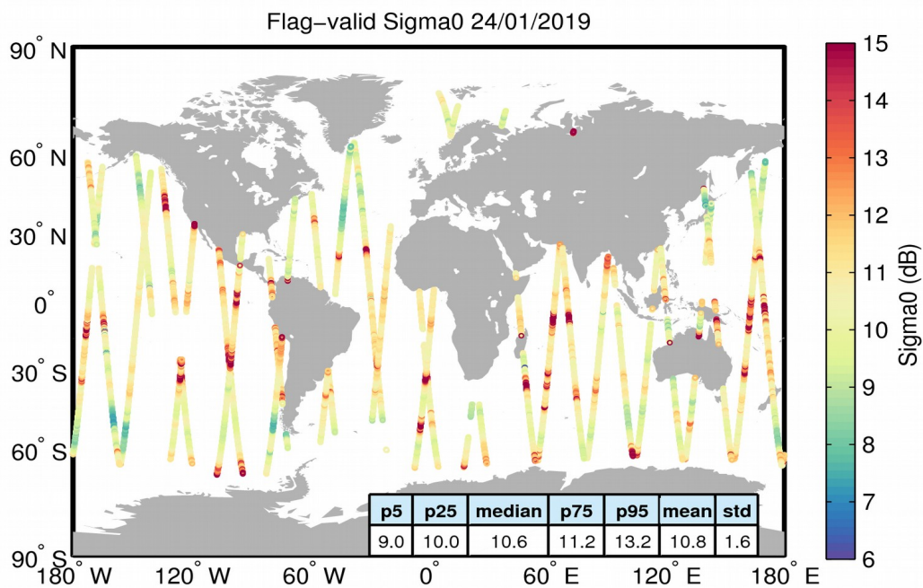
Figure 23. Geographical distribution of flag-valid sigma0 data over oceans and lakes for 24/01/2019. The statistical values shown in the table refer to the sigma0 in dB and are calculated over all measurements shown in the figure.
