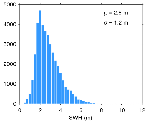
Figure 20. Histogram of science-valid SWH over oceans and lakes for 24/01/2019. The mean ( \mu ) and standard deviation ( \sigma ) are also shown. Note that values larger than 12 m are excluded from the histogram for the sake of readability but not from the computation of \mu and \sigma .
