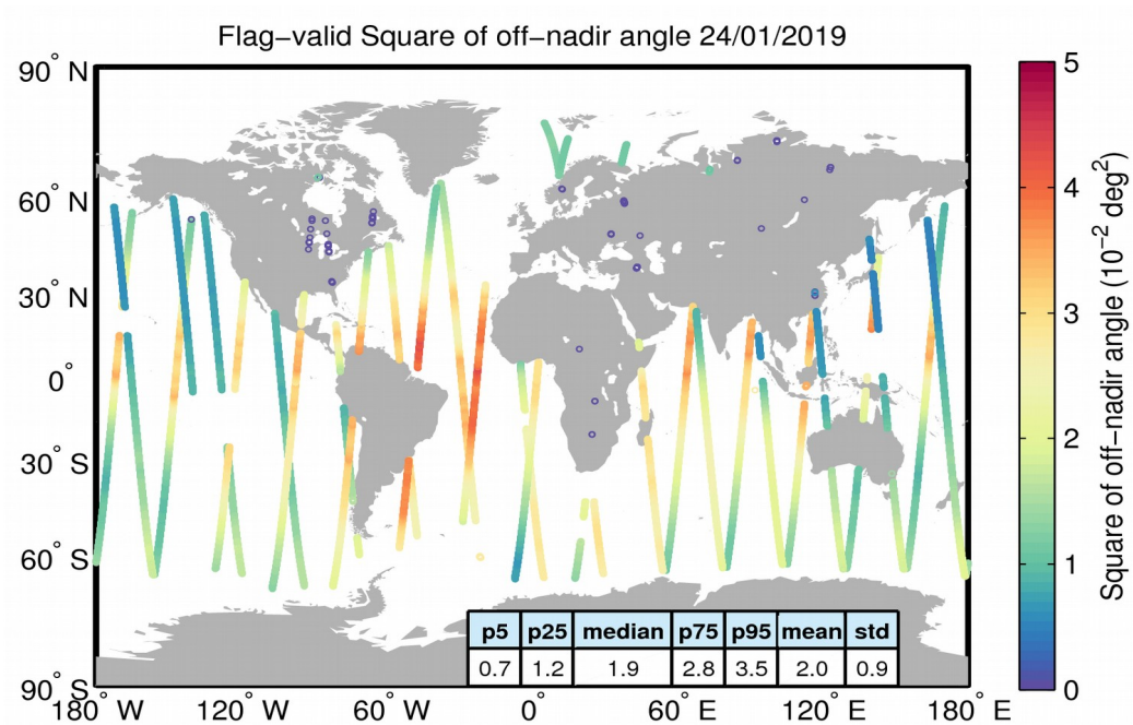
Figure 37. Geographical distribution of flag-valid mispointing data over oceans and lakes for 24/01/2019. The statistical values shown in the table refer to the mispointing in 10^{-2} \text{ deg}^2 and are calculated over all measurements shown in the figure.
