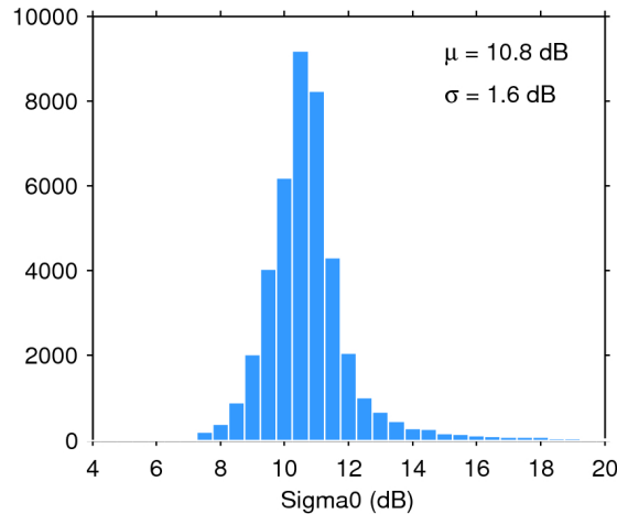
Figure 25. Histogram of flag-valid sigma0 over oceans and lakes for 24/01/2019. The mean ( \mu ) and standard deviation ( \sigma ) are also shown. Note that values outside [4 20] dB are excluded from the histogram for the sake of readability but not from the computation of \mu and \sigma .
