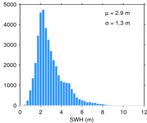
Figure 20. Histogram of science-valid SWH over oceans and lakes for 22/01/2019. The mean ( \mu ) and standard deviation ( \sigma ) are also shown. Note that values larger than 12 m are excluded from the histogram for the sake of readability but not from the computation of \mu and \sigma .
