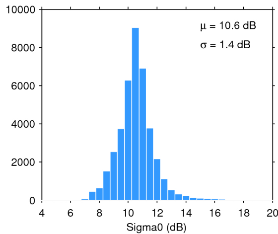
Figure 28. Histogram of science-valid sigma0 over oceans and lakes for 22/01/2019. The mean ( \mu ) and standard deviation ( \sigma ) are also shown. Note that values outside [4 20] dB are excluded from the histogram for the sake of readability but not from the computation of \mu and \sigma .
