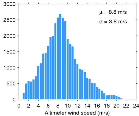
Figure 33. Histogram of flag-valid wind over oceans and lakes for 22/01/2019. The mean ( \mu ) and standard deviation ( \sigma ) are also shown. Note that values larger than 24 m/s are excluded from the histogram for the sake of readability but not from the computation of \mu and \sigma .
