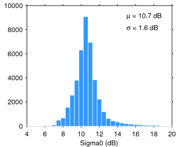
Figure 25. Histogram of flag-valid sigma0 over oceans and lakes for 22/01/2019. The mean ( \mu ) and standard deviation ( \sigma ) are also shown. Note that values outside [4 20] dB are excluded from the histogram for the sake of readability but not from the computation of \mu and \sigma .
