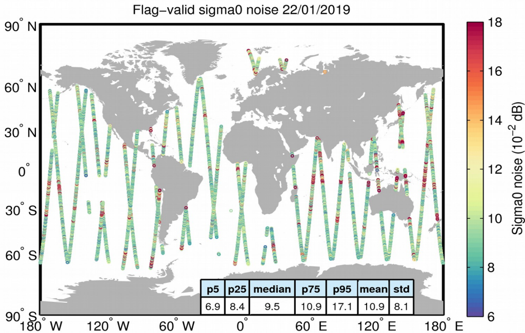
Figure 26. Geographical distribution of flag-valid 20-Hz sigma0 measurement noise over oceans and lakes for 22/01/2019. The statistical values shown in the table refer to the sigma0 noise and are calculated over all measurements shown in the figure.
