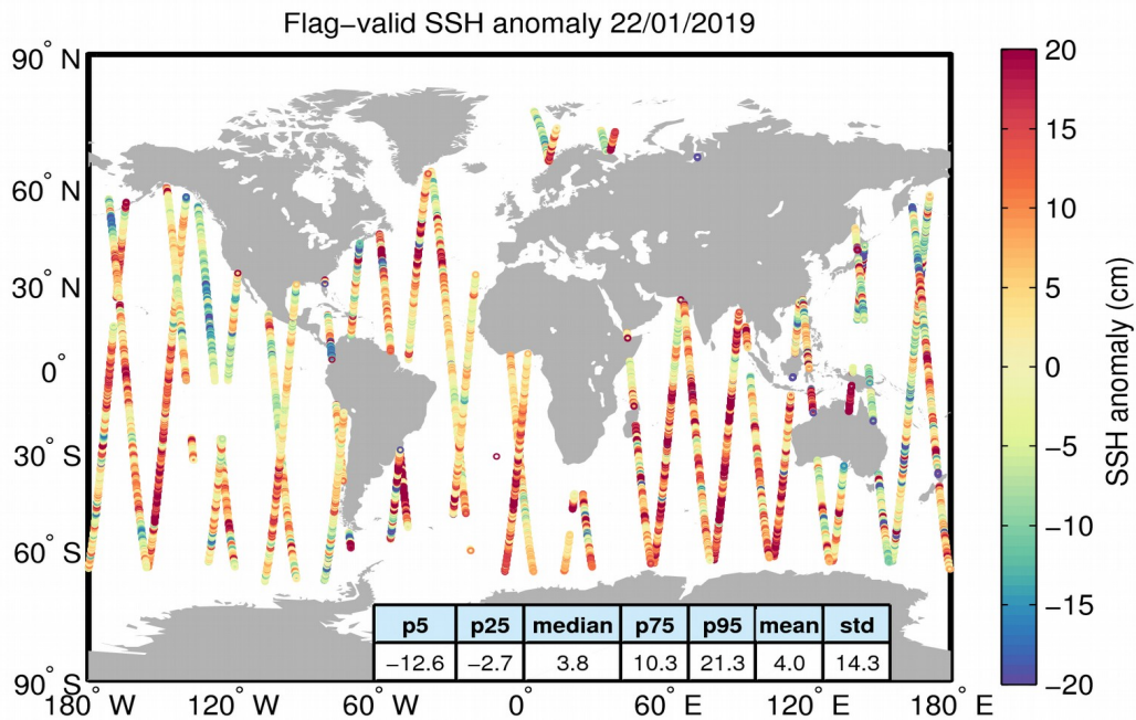
Figure 5. Geographical distribution of flag-valid 1-Hz SSH anomaly data over oceans and lakes for 22/01/2019. The statistical values shown in the table refer to the SSH anomaly in cm and are calculated over all measurements shown in the figure.
