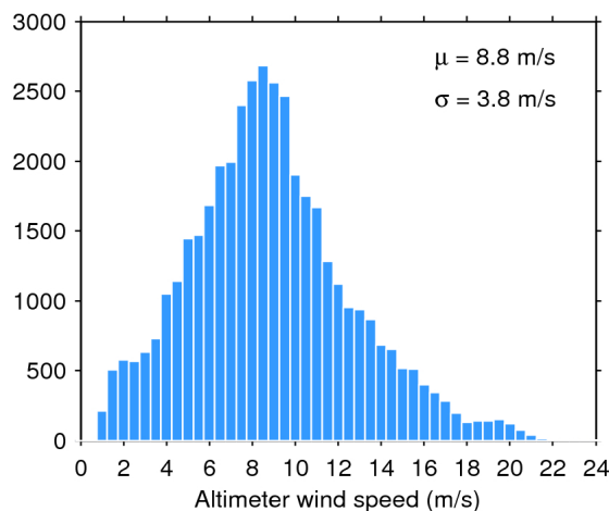
Figure 35. Histogram of science-valid wind over oceans and lakes for 22/01/2019. The mean ( \mu ) and standard deviation ( \sigma ) are also shown. Note that values larger than 24 m/s are excluded from the histogram for the sake of readability but not from the computation of \mu and \sigma .
