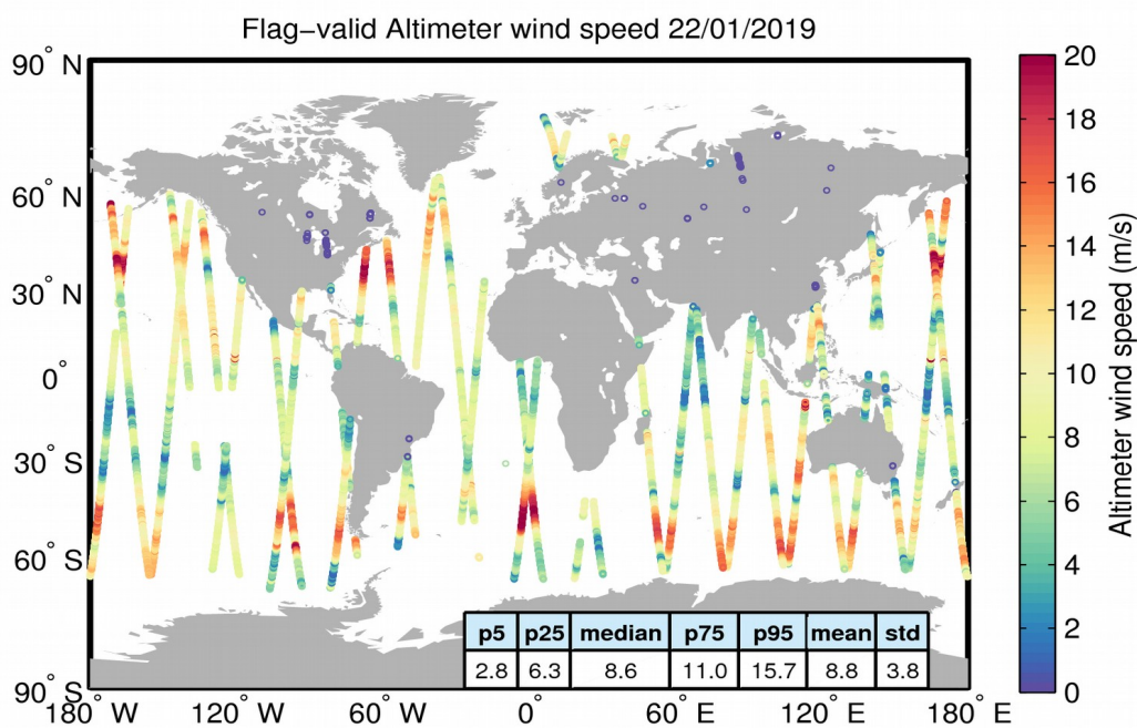
Figure 31. Geographical distribution of flag-valid wind data over oceans and lakes for 22/01/2019. The statistical values shown in the table refer to the wind in m/s and are calculated over all measurements shown in the figure.
