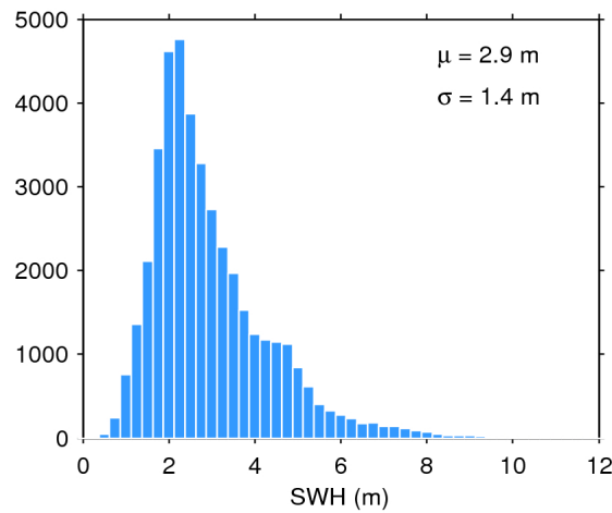
Figure 17. Histogram of flag-valid SWH over oceans and lakes for 22/01/2019. The mean ( \mu ) and standard deviation ( \sigma ) are also shown. Note that values larger than 12 m are excluded from the histogram for the sake of readability but not from the computation of \mu and \sigma .
