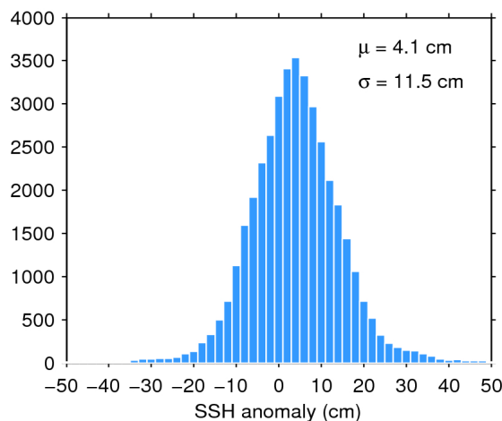
Figure 11. Histogram of science-valid SSH anomaly over oceans and lakes for 22/01/2019. The mean ( \mu ) and standard deviation ( \sigma ) are also shown. Note that values outside [-50 50] cm are excluded from the histogram for the sake of readability but not from the computation of \mu and \sigma .
