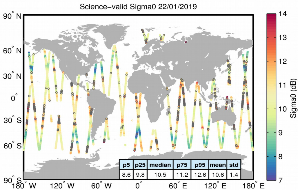
Figure 27. Geographical distribution of science-valid sigma0 data over oceans and lakes for 22/01/2019. The statistical values shown in the table refer to the sigma0 in dB and are calculated over all measurements shown in the figure. Gray circles denote records that have been rejected based on the editing criteria described in Table 4.
