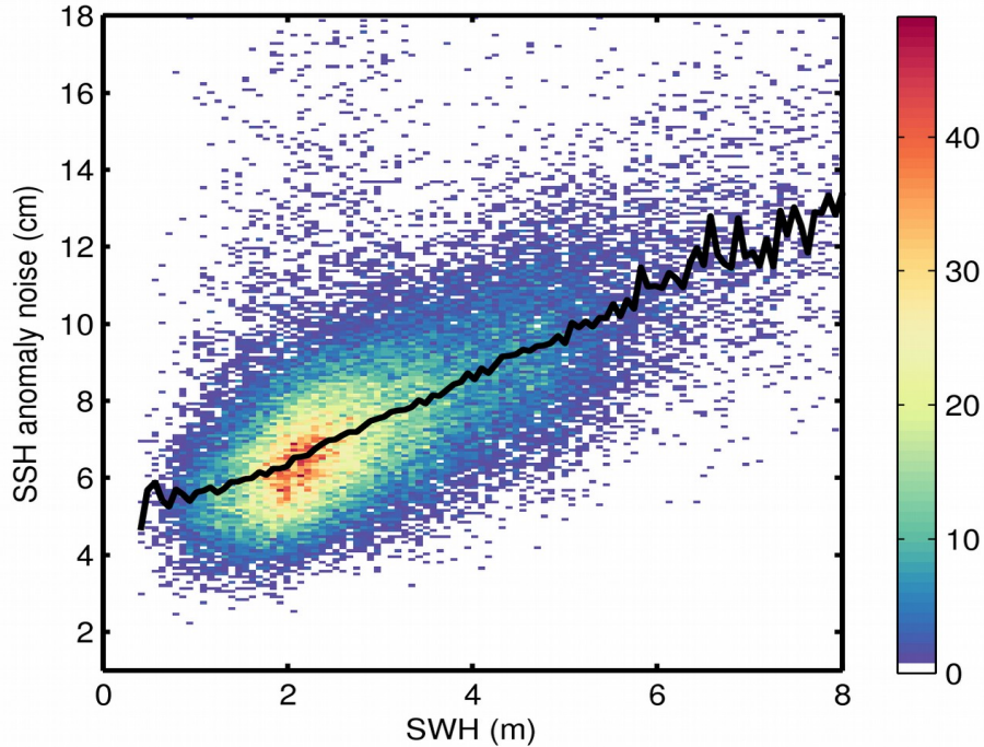
Figure 9. 2D histogram showing flag-valid SSH anomaly noise as a function of SWH for 22/01/2019. The black line denotes the median SSH anomaly noise as a function of SWH.
