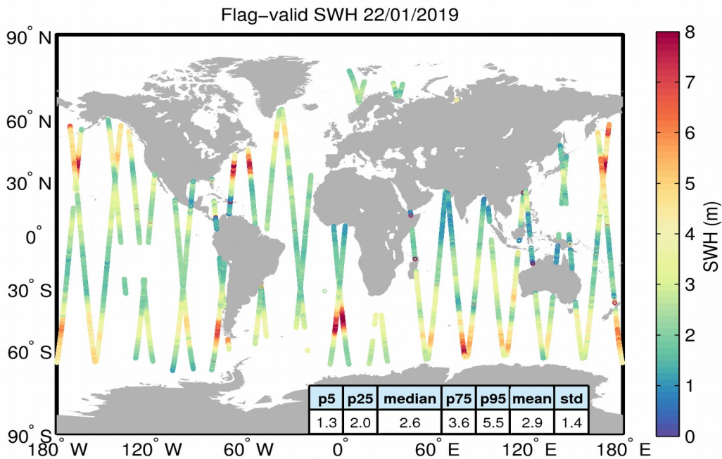
Figure 15. Geographical distribution of flag-valid SWH data over oceans and lakes for 22/01/2019. The statistical values shown in the table refer to the SWH in m and are calculated over all measurements shown in the figure.
