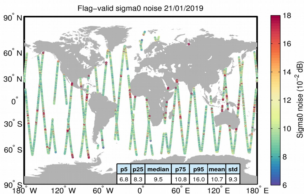
Figure 26. Geographical distribution of flag-valid 20-Hz sigma0 measurement noise over oceans and lakes for 21/01/2019. The statistical values shown in the table refer to the sigma0 noise and are calculated over all measurements shown in the figure.
