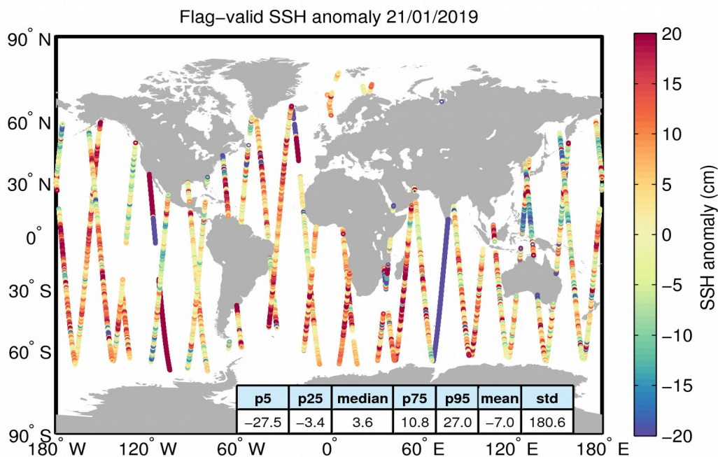
Figure 5. Geographical distribution of flag-valid 1-Hz SSH anomaly data over oceans and lakes for 21/01/2019. The statistical values shown in the table refer to the SSH anomaly in cm and are calculated over all measurements shown in the figure.
