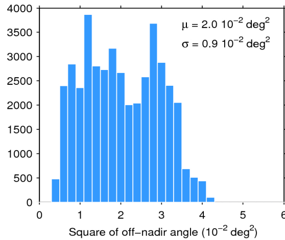
Figure 39. Histogram of flag-valid mispointing over oceans and lakes for 21/01/2019. The mean ( \mu ) and standard deviation ( \sigma ) are also shown. Note that values larger than 6 \cdot 10^{-2} \text{ deg}^2 are excluded from the histogram for the sake of readability but not from the computation of \mu and \sigma .
