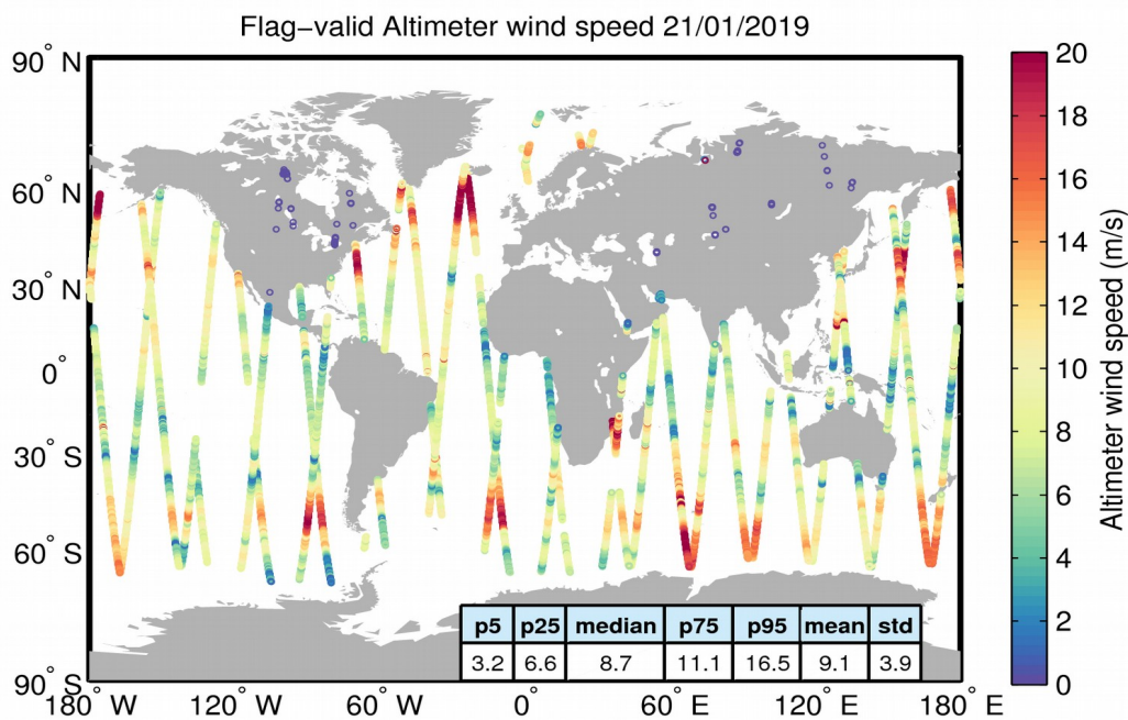
Figure 31. Geographical distribution of flag-valid wind data over oceans and lakes for 21/01/2019. The statistical values shown in the table refer to the wind in m/s and are calculated over all measurements shown in the figure.
