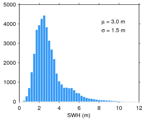
Figure 17. Histogram of flag-valid SWH over oceans and lakes for 21/01/2019. The mean ( \mu ) and standard deviation ( \sigma ) are also shown. Note that values larger than 12 m are excluded from the histogram for the sake of readability but not from the computation of \mu and \sigma .
