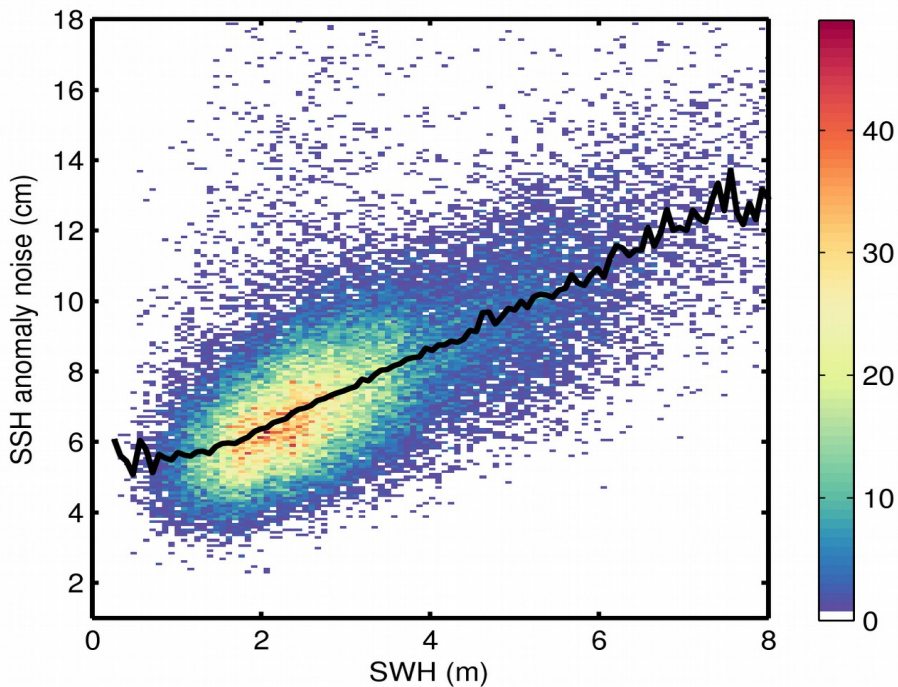
Figure 9. 2D histogram showing flag-valid SSH anomaly noise as a function of SWH for 21/01/2019. The black line denotes the median SSH anomaly noise as a function of SWH.
