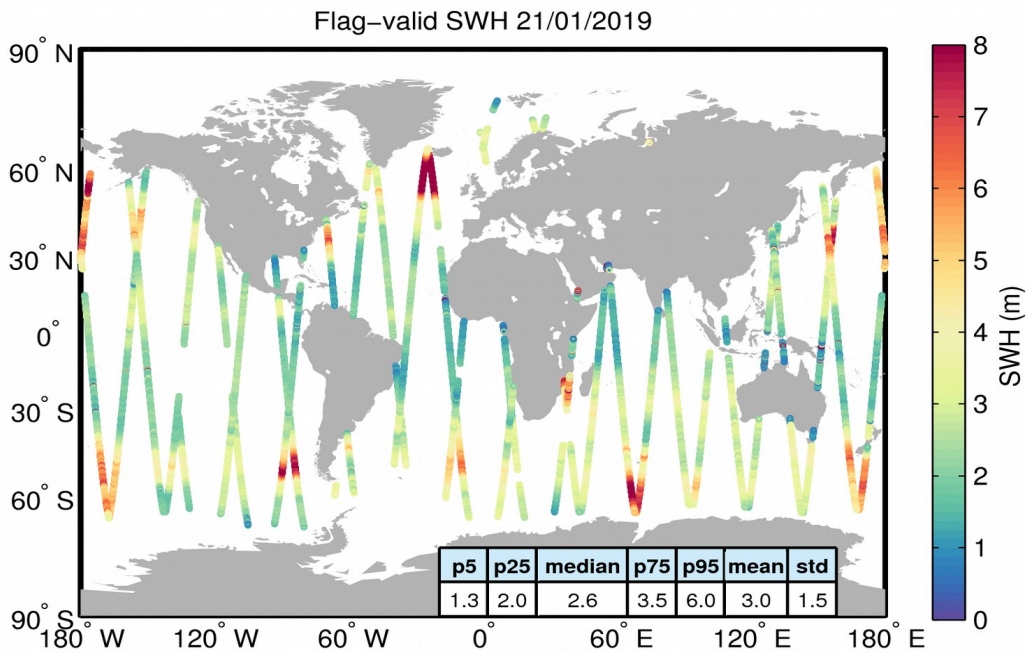
Figure 15. Geographical distribution of flag-valid SWH data over oceans and lakes for 21/01/2019. The statistical values shown in the table refer to the SWH in m and are calculated over all measurements shown in the figure.
