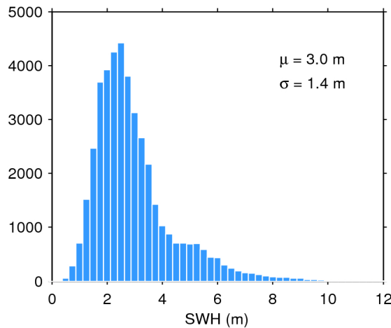
Figure 20. Histogram of science-valid SWH over oceans and lakes for 21/01/2019. The mean ( \mu ) and standard deviation ( \sigma ) are also shown. Note that values larger than 12 m are excluded from the histogram for the sake of readability but not from the computation of \mu and \sigma .
