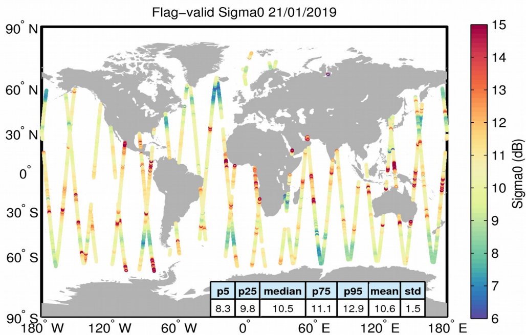
Figure 23. Geographical distribution of flag-valid sigma0 data over oceans and lakes for 21/01/2019. The statistical values shown in the table refer to the sigma0 in dB and are calculated over all measurements shown in the figure.
