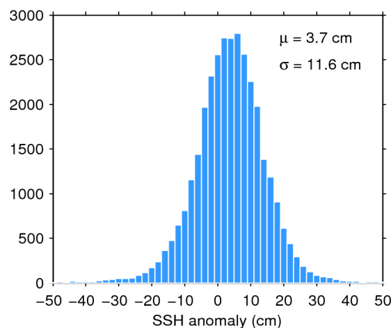
Figure 11. Histogram of science-valid SSH anomaly over oceans and lakes for 21/01/2019. The mean ( \mu ) and standard deviation ( \sigma ) are also shown. Note that values outside [-50 50] cm are excluded from the histogram for the sake of readability but not from the computation of \mu and \sigma .
