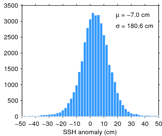
Figure 7. Histogram of flag-valid SSH anomaly over oceans and lakes for 21/01/2019. The mean ( \mu ) and standard deviation ( \sigma ) are also shown. Note that values outside [-50 50] cm are excluded from the histogram for the sake of readability but not from the computation of \mu and \sigma .
