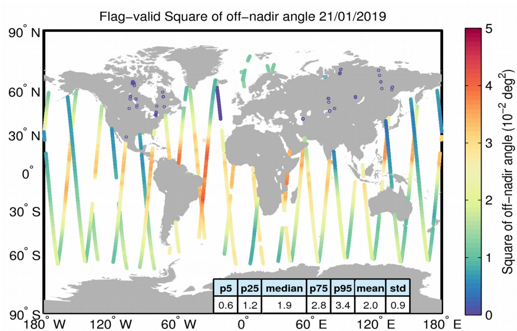
Figure 37. Geographical distribution of flag-valid mispointing data over oceans and lakes for 21/01/2019. The statistical values shown in the table refer to the mispointing in 10^{-2} deg 2 and are calculated over all measurements shown in the figure.
