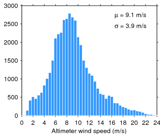
Figure 35. Histogram of science-valid wind over oceans and lakes for 21/01/2019. The mean ( \mu ) and standard deviation ( \sigma ) are also shown. Note that values larger than 24 m/s are excluded from the histogram for the sake of readability but not from the computation of \mu and \sigma .
