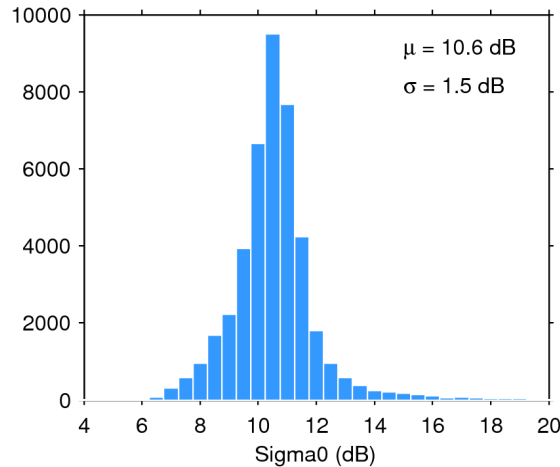
Figure 25. Histogram of flag-valid sigma0 over oceans and lakes for 21/01/2019. The mean ( \mu ) and standard deviation ( \sigma ) are also shown. Note that values outside [4 20] dB are excluded from the histogram for the sake of readability but not from the computation of \mu and \sigma .
