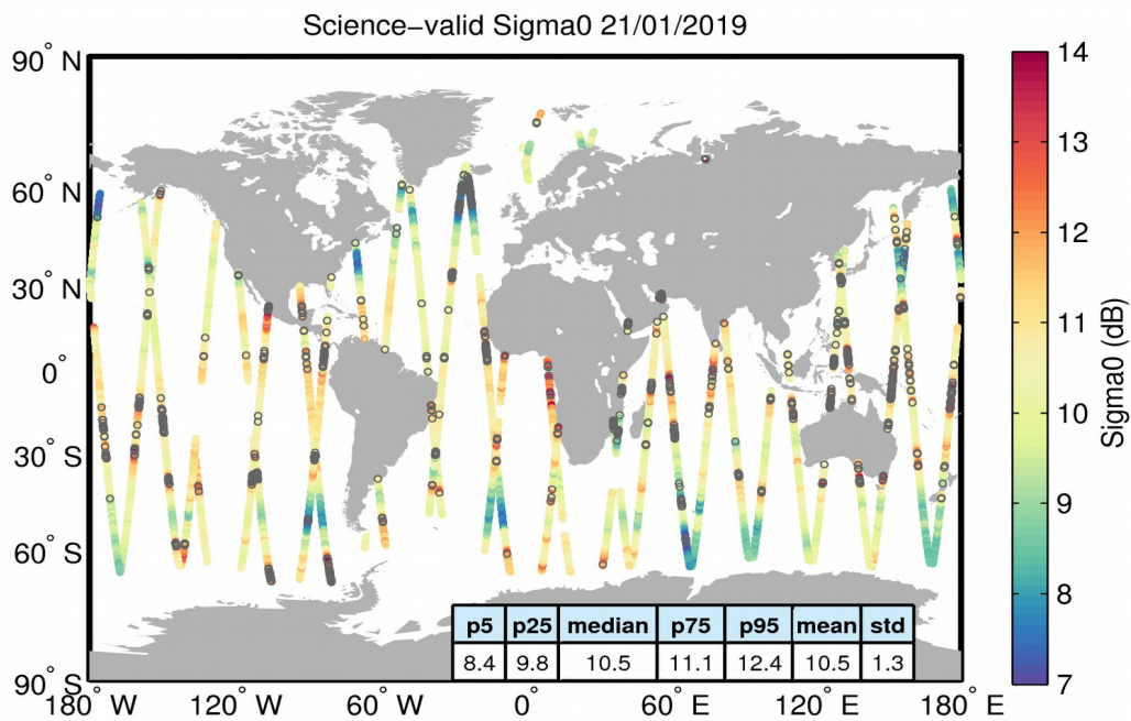
Figure 27. Geographical distribution of science-valid sigma0 data over oceans and lakes for 21/01/2019. The statistical values shown in the table refer to the sigma0 in dB and are calculated over all measurements shown in the figure. Gray circles denote records that have been rejected based on the editing criteria described in Table 4.
