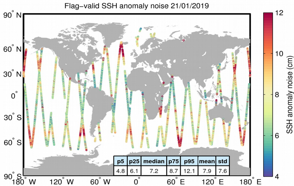
Figure 8. Geographical distribution of flag-valid 20-Hz SSH anomaly measurement noise over oceans and lakes for 21/01/2019. The statistical values shown in the table refer to the SSH anomaly noise and are calculated over all measurements shown in the figure.
