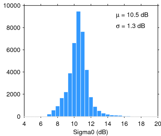
Figure 28. Histogram of science-valid sigma0 over oceans and lakes for 21/01/2019. The mean ( \mu ) and standard deviation ( \sigma ) are also shown. Note that values outside [4 20] dB are excluded from the histogram for the sake of readability but not from the computation of \mu and \sigma .
