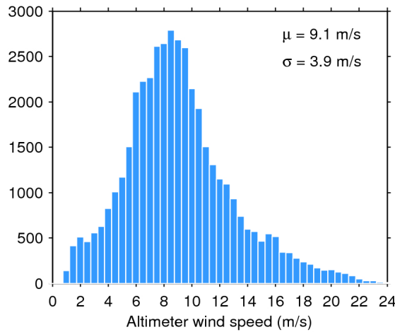
Figure 33. Histogram of flag-valid wind over oceans and lakes for 21/01/2019. The mean ( \mu ) and standard deviation ( \sigma ) are also shown. Note that values larger than 24 m/s are excluded from the histogram for the sake of readability but not from the computation of \mu and \sigma .
