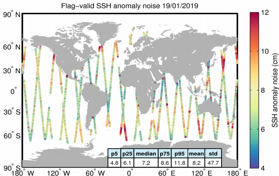
Figure 8. Geographical distribution of flag-valid 20-Hz SSH anomaly measurement noise over oceans and lakes for 19/01/2019. The statistical values shown in the table refer to the SSH anomaly noise and are calculated over all measurements shown in the figure.
