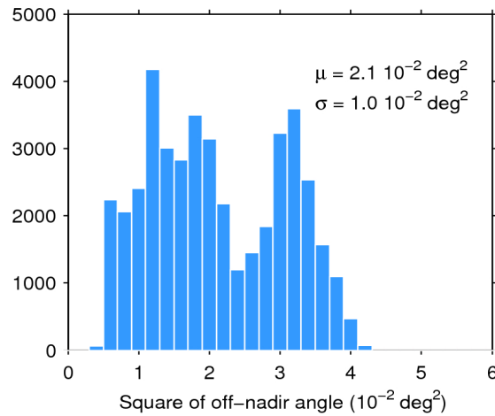
Figure 39. Histogram of flag-valid mispointing over oceans and lakes for 19/01/2019. The mean ( \mu ) and standard deviation ( \sigma ) are also shown. Note that values larger than 6 \cdot 10^{-2} \text{ deg}^2 are excluded from the histogram for the sake of readability but not from the computation of \mu and \sigma .
