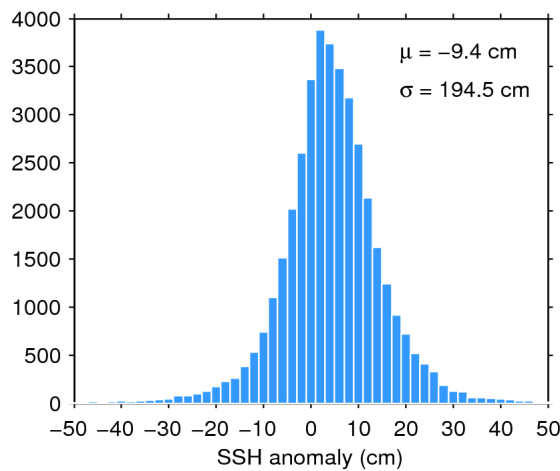
Figure 7. Histogram of flag-valid SSH anomaly over oceans and lakes for 19/01/2019. The mean ( \mu ) and standard deviation ( \sigma ) are also shown. Note that values outside [-50\ 50] cm are excluded from the histogram for the sake of readability but not from the computation of \mu and \sigma .
