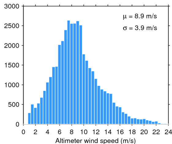
Figure 35. Histogram of science-valid wind over oceans and lakes for 19/01/2019. The mean ( \mu ) and standard deviation ( \sigma ) are also shown. Note that values larger than 24 m/s are excluded from the histogram for the sake of readability but not from the computation of \mu and \sigma .
