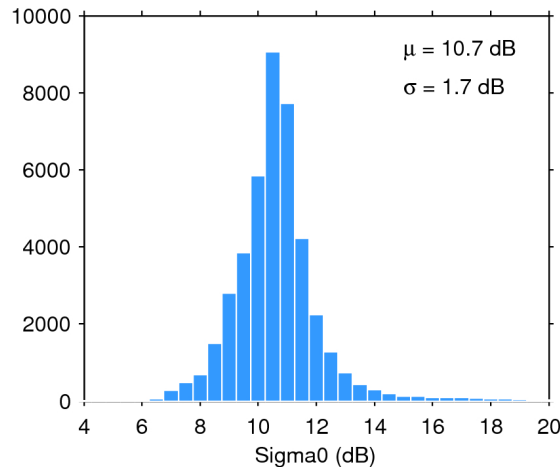
Figure 25. Histogram of flag-valid sigma0 over oceans and lakes for 19/01/2019. The mean ( \mu ) and standard deviation ( \sigma ) are also shown. Note that values outside [4 20] dB are excluded from the histogram for the sake of readability but not from the computation of \mu and \sigma .
