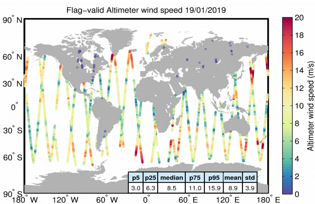
Figure 31. Geographical distribution of flag-valid wind data over oceans and lakes for 19/01/2019. The statistical values shown in the table refer to the wind in m/s and are calculated over all measurements shown in the figure.
