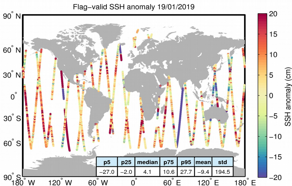
Figure 5. Geographical distribution of flag-valid 1-Hz SSH anomaly data over oceans and lakes for 19/01/2019. The statistical values shown in the table refer to the SSH anomaly in cm and are calculated over all measurements shown in the figure.
