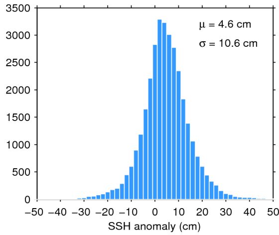
Figure 11. Histogram of science-valid SSH anomaly over oceans and lakes for 19/01/2019. The mean ( \mu ) and standard deviation ( \sigma ) are also shown. Note that values outside [-50 50] cm are excluded from the histogram for the sake of readability but not from the computation of \mu and \sigma .
