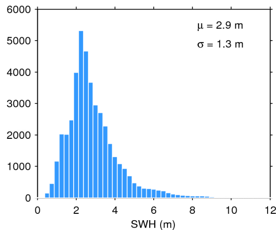
Figure 17. Histogram of flag-valid SWH over oceans and lakes for 19/01/2019. The mean ( \mu ) and standard deviation ( \sigma ) are also shown. Note that values larger than 12 m are excluded from the histogram for the sake of readability but not from the computation of \mu and \sigma .
