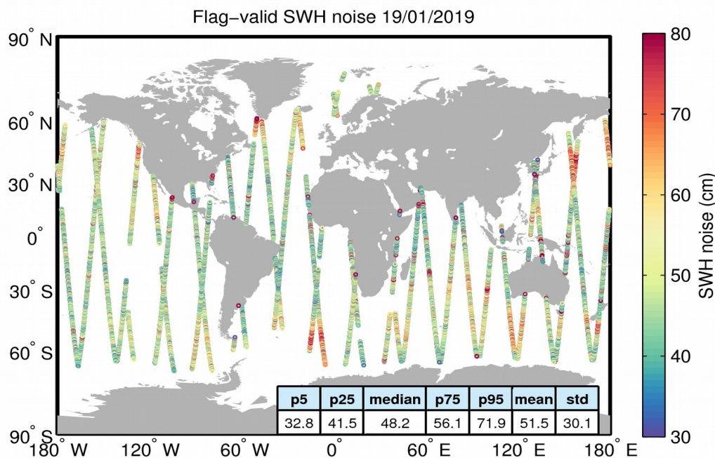
Figure 18. Geographical distribution of flag-valid 20-Hz SWH measurement noise over oceans and lakes for 19/01/2019. The statistical values shown in the figure refer to the SWH noise and are calculated over all measurements shown in the figure.
