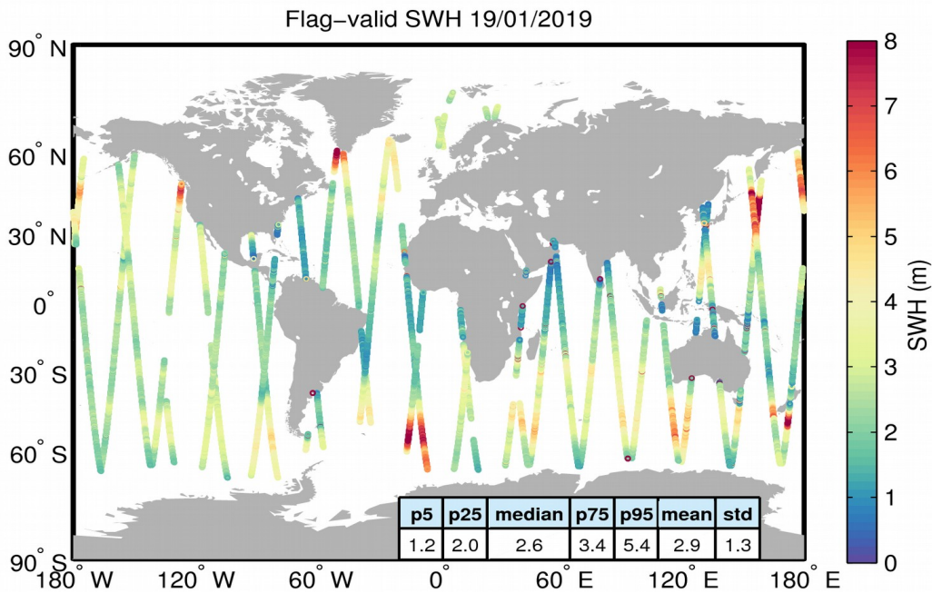
Figure 15. Geographical distribution of flag-valid SWH data over oceans and lakes for 19/01/2019. The statistical values shown in the table refer to the SWH in m and are calculated over all measurements shown in the figure.
