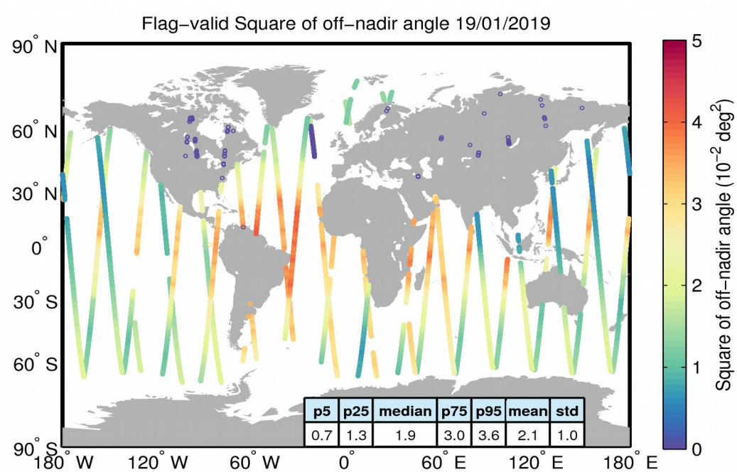
Figure 37. Geographical distribution of flag-valid mispointing data over oceans and lakes for 19/01/2019. The statistical values shown in the table refer to the mispointing in 10^{-2} deg 2 and are calculated over all measurements shown in the figure.
