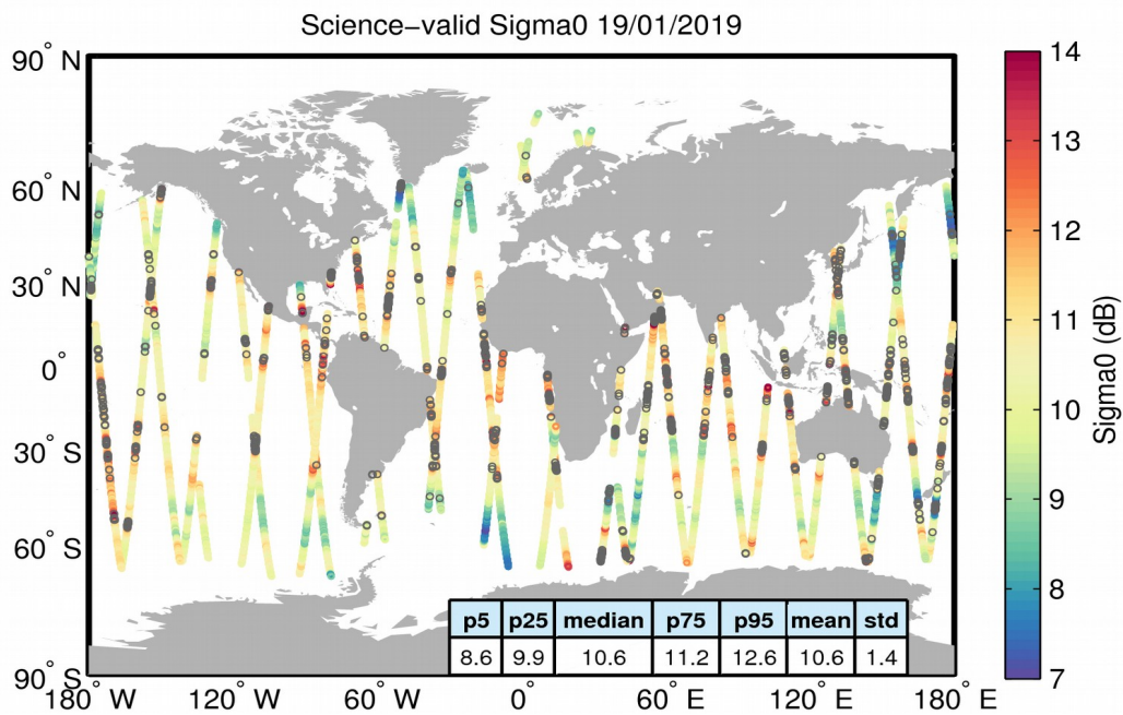
Figure 27. Geographical distribution of science-valid sigma0 data over oceans and lakes for 19/01/2019. The statistical values shown in the table refer to the sigma0 in dB and are calculated over all measurements shown in the figure. Gray circles denote records that have been rejected based on the editing criteria described in Table 4.
