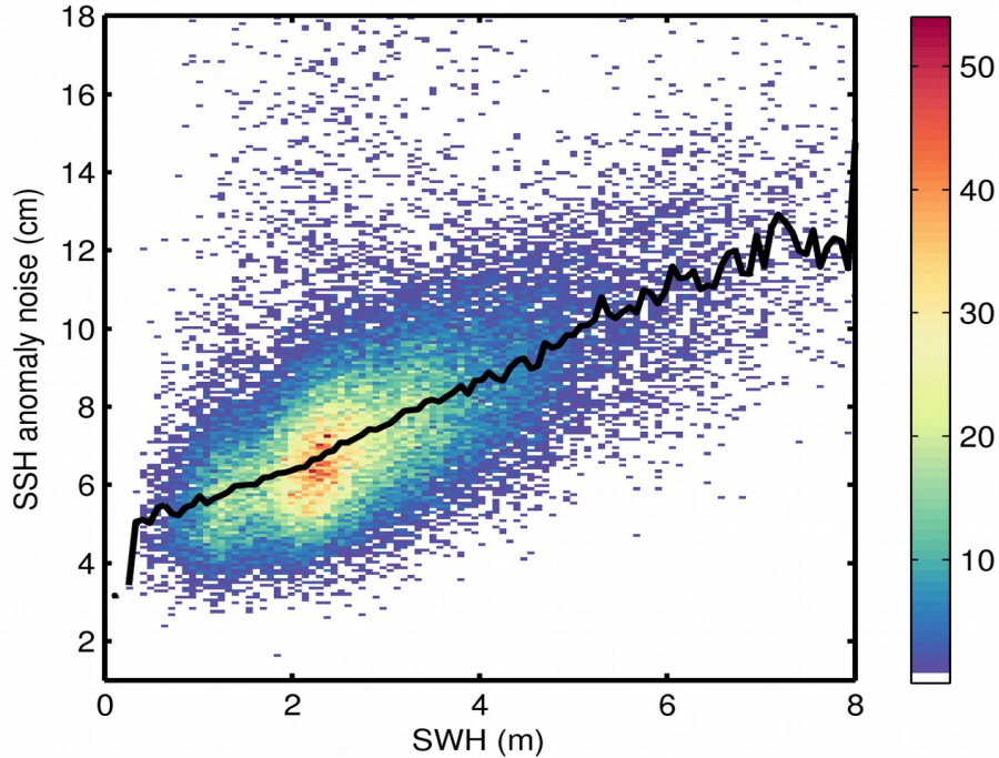
Figure 9. 2D histogram showing flag-valid SSH anomaly noise as a function of SWH for 19/01/2019. The black line denotes the median SSH anomaly noise as a function of SWH.
