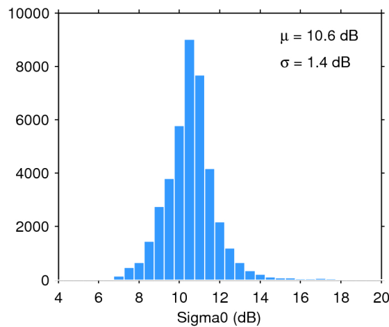
Figure 28. Histogram of science-valid sigma0 over oceans and lakes for 19/01/2019. The mean ( \mu ) and standard deviation ( \sigma ) are also shown. Note that values outside [4 20] dB are excluded from the histogram for the sake of readability but not from the computation of \mu and \sigma .
