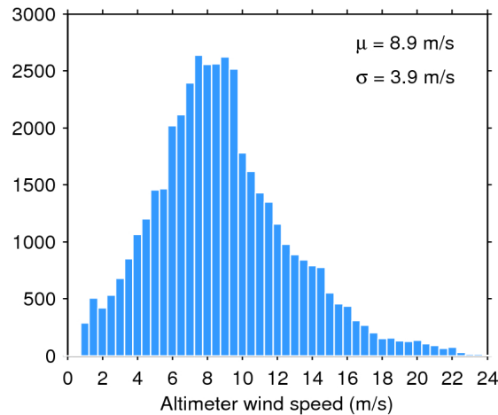
Figure 33. Histogram of flag-valid wind over oceans and lakes for 19/01/2019. The mean ( \mu ) and standard deviation ( \sigma ) are also shown. Note that values larger than 24 m/s are excluded from the histogram for the sake of readability but not from the computation of \mu and \sigma .
