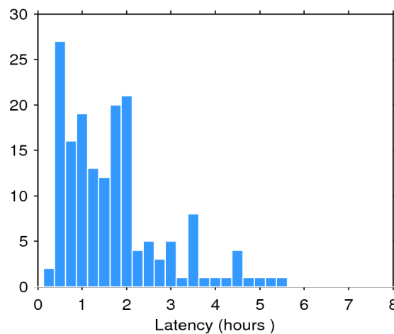
Figure 2. Histogram of the data latency for 18/01/2019. The y-axis denotes the number of files that are made available with a delay of x-hours with respect to the mean time of the records stored in the file.
