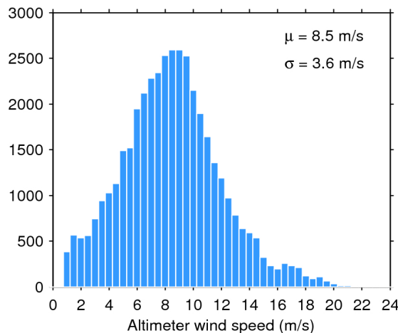
Figure 35. Histogram of science-valid wind over oceans and lakes for 18/01/2019. The mean ( \mu ) and standard deviation ( \sigma ) are also shown. Note that values larger than 24 m/s are excluded from the histogram for the sake of readability but not from the computation of \mu and \sigma .
