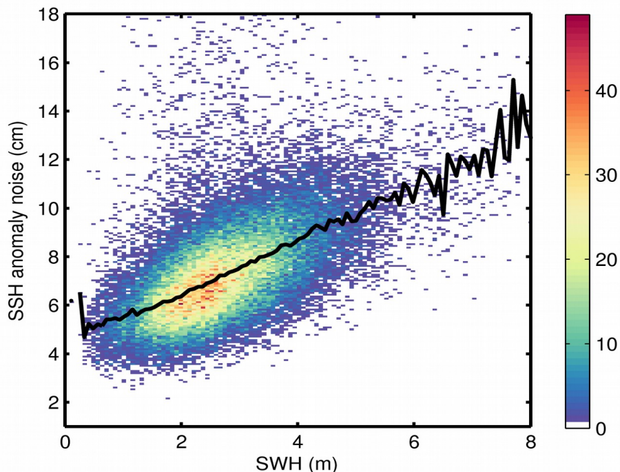
Figure 9. 2D histogram showing flag-valid SSH anomaly noise as a function of SWH for 18/01/2019. The black line denotes the median SSH anomaly noise as a function of SWH.
