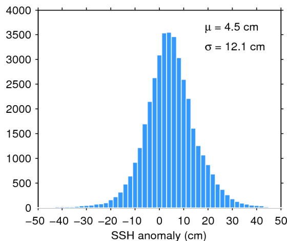
Figure 11. Histogram of science-valid SSH anomaly over oceans and lakes for 18/01/2019. The mean ( \mu ) and standard deviation ( \sigma ) are also shown. Note that values outside [-50 50] cm are excluded from the histogram for the sake of readability but not from the computation of \mu and \sigma .
