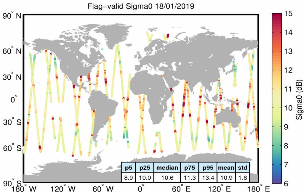
Figure 23. Geographical distribution of flag-valid sigma0 data over oceans and lakes for 18/01/2019. The statistical values shown in the table refer to the sigma0 in dB and are calculated over all measurements shown in the figure.
