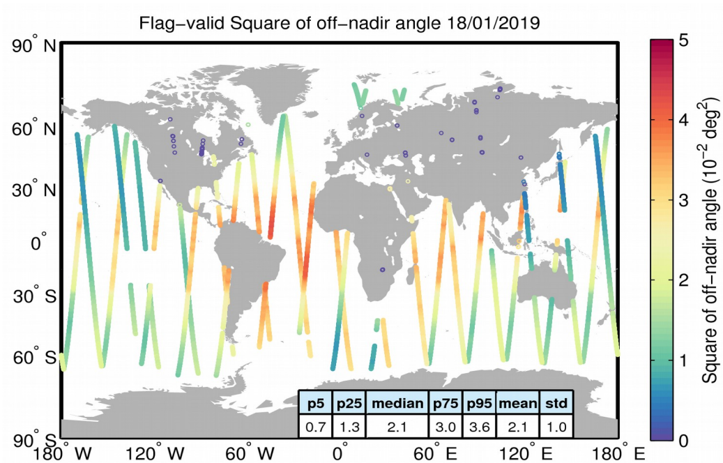
Figure 37. Geographical distribution of flag-valid mispointing data over oceans and lakes for 18/01/2019. The statistical values shown in the table refer to the mispointing in 10^{-2} \text{ deg}^2 and are calculated over all measurements shown in the figure.
