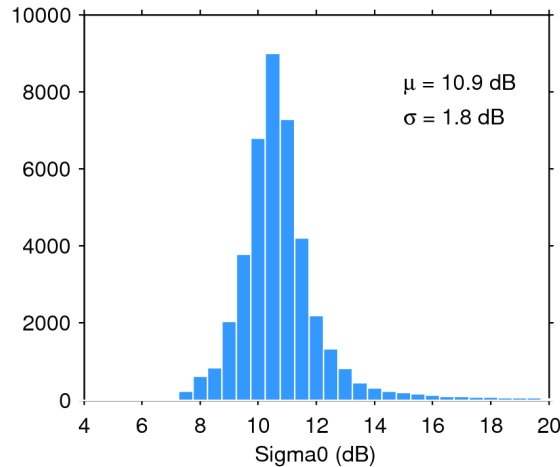
Figure 25. Histogram of flag-valid sigma0 over oceans and lakes for 18/01/2019. The mean ( \mu ) and standard deviation ( \sigma ) are also shown. Note that values outside [4 20] dB are excluded from the histogram for the sake of readability but not from the computation of \mu and \sigma .
