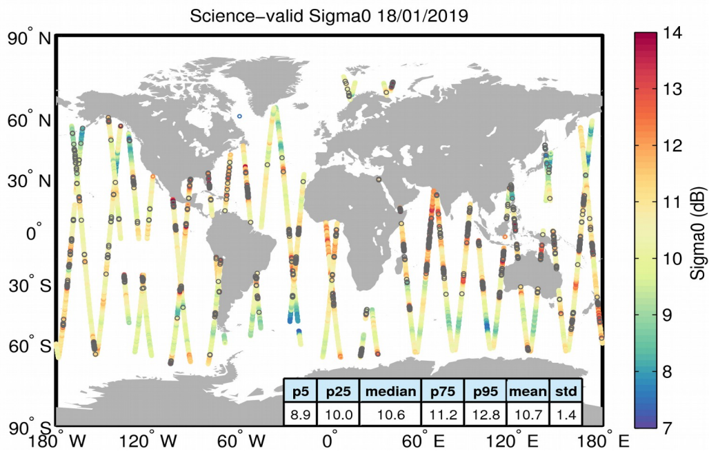
Figure 27. Geographical distribution of science-valid sigma0 data over oceans and lakes for 18/01/2019. The statistical values shown in the table refer to the sigma0 in dB and are calculated over all measurements shown in the figure. Gray circles denote records that have been rejected based on the editing criteria described in Table 4.
