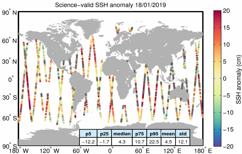
Figure 10. Geographical distribution of science-valid SSH anomaly data over oceans and lakes for 18/01/2019. The statistical values shown in the table refer to the SSH anomaly in cm and are calculated over all measurements shown in the figure. Gray circles denote records that have been rejected based on the editing criteria described in Table 2.
