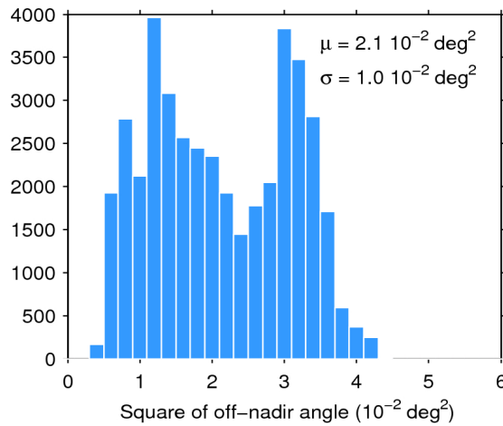
Figure 39. Histogram of flag-valid mispointing over oceans and lakes for 18/01/2019. The mean ( \mu ) and standard deviation ( \sigma ) are also shown. Note that values larger than 6 \cdot 10^{-2} \text{ deg}^2 are excluded from the histogram for the sake of readability but not from the computation of \mu and \sigma .
