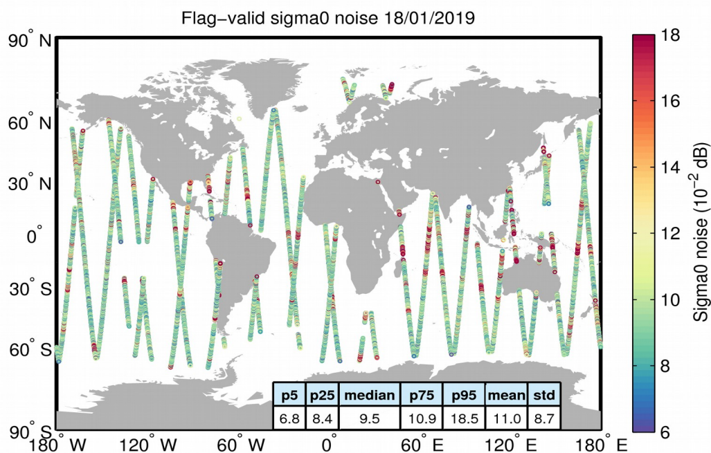
Figure 26. Geographical distribution of flag-valid 20-Hz sigma0 measurement noise over oceans and lakes for 18/01/2019. The statistical values shown in the table refer to the sigma0 noise and are calculated over all measurements shown in the figure.
