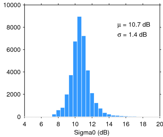
Figure 28. Histogram of science-valid sigma0 over oceans and lakes for 18/01/2019. The mean ( \mu ) and standard deviation ( \sigma ) are also shown. Note that values outside [4 20] dB are excluded from the histogram for the sake of readability but not from the computation of \mu and \sigma .
