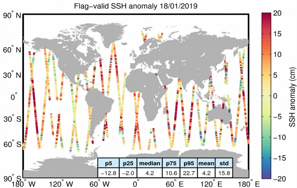
Figure 5. Geographical distribution of flag-valid 1-Hz SSH anomaly data over oceans and lakes for 18/01/2019. The statistical values shown in the table refer to the SSH anomaly in cm and are calculated over all measurements shown in the figure.
