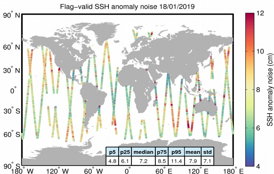
Figure 8. Geographical distribution of flag-valid 20-Hz SSH anomaly measurement noise over oceans and lakes for 18/01/2019. The statistical values shown in the table refer to the SSH anomaly noise and are calculated over all measurements shown in the figure.
