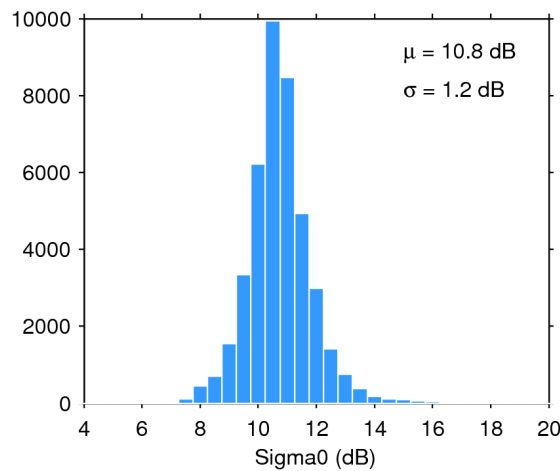
Figure 28. Histogram of science-valid sigma0 over oceans and lakes for 17/01/2019. The mean ( \mu ) and standard deviation ( \sigma ) are also shown. Note that values outside [4 20] dB are excluded from the histogram for the sake of readability but not from the computation of \mu and \sigma .
