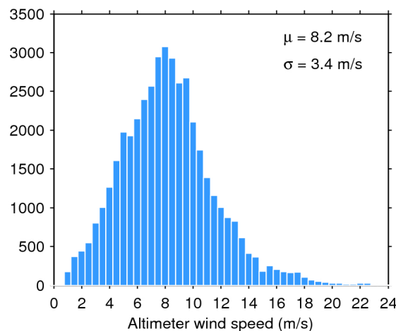
Figure 35. Histogram of science-valid wind over oceans and lakes for 17/01/2019. The mean ( \mu ) and standard deviation ( \sigma ) are also shown. Note that values larger than 24 m/s are excluded from the histogram for the sake of readability but not from the computation of \mu and \sigma .
