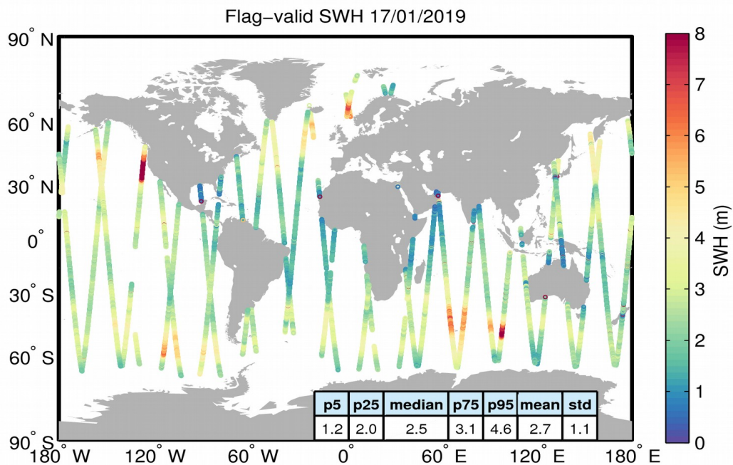
Figure 15. Geographical distribution of flag-valid SWH data over oceans and lakes for 17/01/2019. The statistical values shown in the table refer to the SWH in m and are calculated over all measurements shown in the figure.
