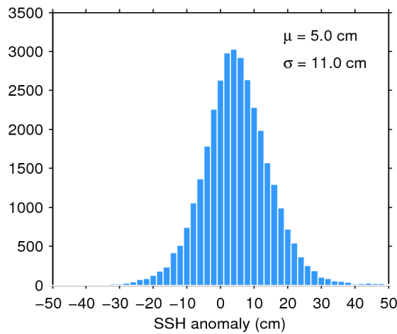
Figure 11. Histogram of science-valid SSH anomaly over oceans and lakes for 17/01/2019. The mean ( \mu ) and standard deviation ( \sigma ) are also shown. Note that values outside [-50 50] cm are excluded from the histogram for the sake of readability but not from the computation of \mu and \sigma .
