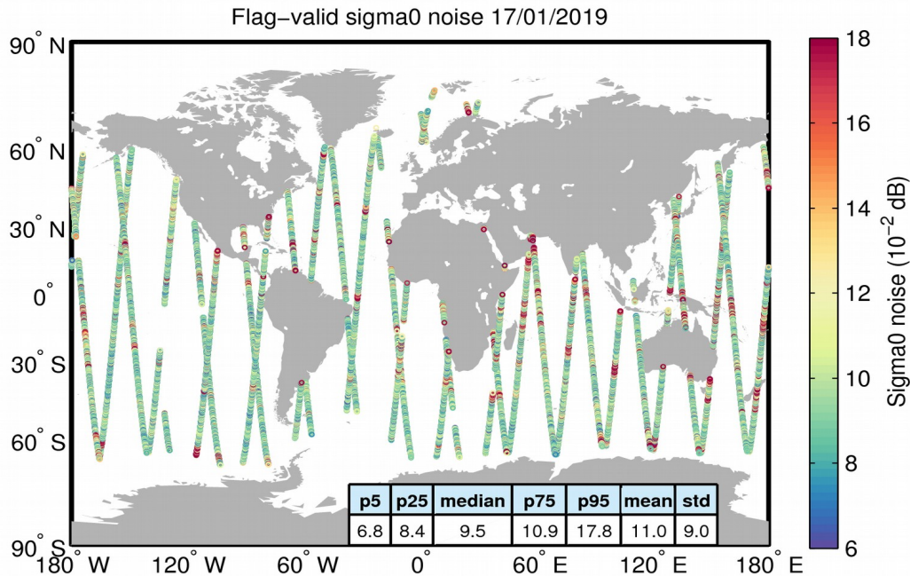
Figure 26. Geographical distribution of flag-valid 20-Hz sigma0 measurement noise over oceans and lakes for 17/01/2019. The statistical values shown in the table refer to the sigma0 noise and are calculated over all measurements shown in the figure.
