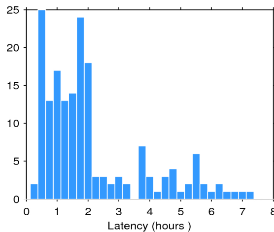
Figure 2. Histogram of the data latency for 17/01/2019. The y-axis denotes the number of files that are made available with a delay of x-hours with respect to the mean time of the records stored in the file.
