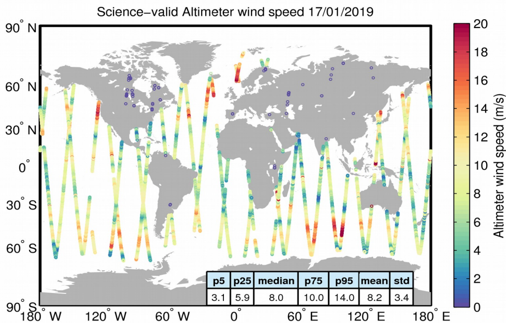
Figure 34. Geographical distribution of science-valid wind data over oceans and lakes for 17/01/2019. The statistical values shown in the table refer to the wind in m/s and are calculated over all measurements shown in the figure. Gray circles denote records that have been rejected based on the editing criteria described in Table 5.
