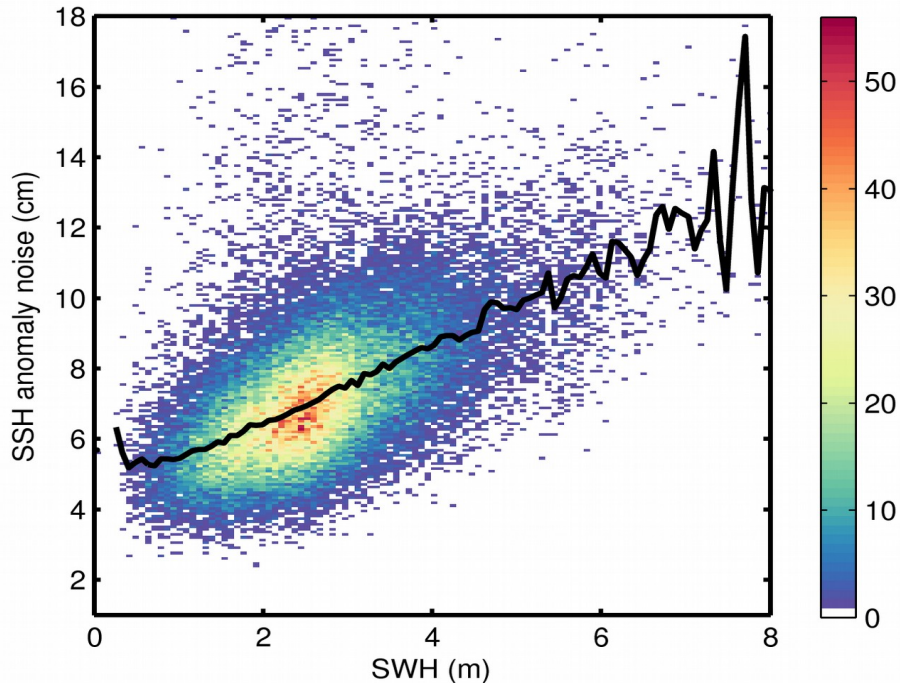
Figure 9. 2D histogram showing flag-valid SSH anomaly noise as a function of SWH for 17/01/2019. The black line denotes the median SSH anomaly noise as a function of SWH.
