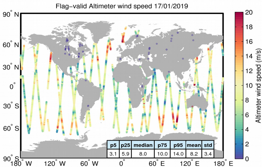
Figure 31. Geographical distribution of flag-valid wind data over oceans and lakes for 17/01/2019. The statistical values shown in the table refer to the wind in m/s and are calculated over all measurements shown in the figure.
