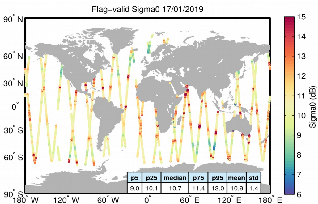
Figure 23. Geographical distribution of flag-valid sigma0 data over oceans and lakes for 17/01/2019. The statistical values shown in the table refer to the sigma0 in dB and are calculated over all measurements shown in the figure.
