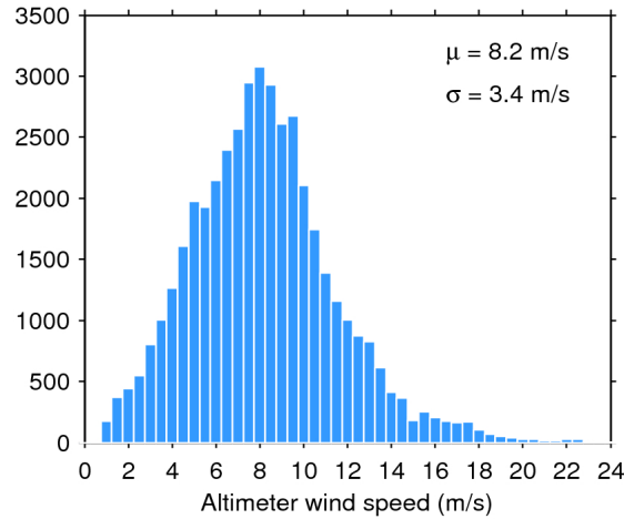
Figure 33. Histogram of flag-valid wind over oceans and lakes for 17/01/2019. The mean ( \mu ) and standard deviation ( \sigma ) are also shown. Note that values larger than 24 m/s are excluded from the histogram for the sake of readability but not from the computation of \mu and \sigma .
