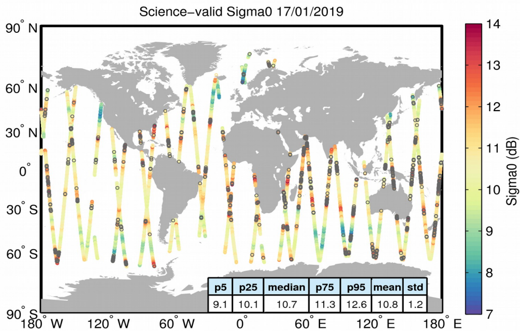
Figure 27. Geographical distribution of science-valid sigma0 data over oceans and lakes for 17/01/2019. The statistical values shown in the table refer to the sigma0 in dB and are calculated over all measurements shown in the figure. Gray circles denote records that have been rejected based on the editing criteria described in Table 4.
