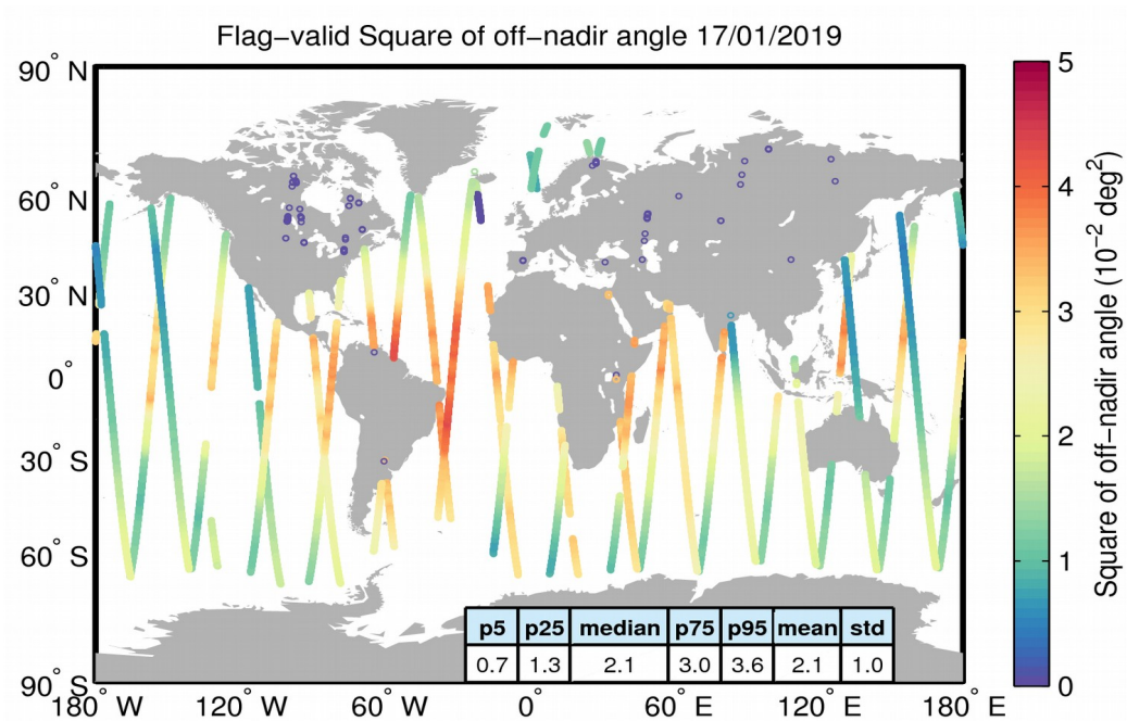
Figure 37. Geographical distribution of flag-valid mispointing data over oceans and lakes for 17/01/2019. The statistical values shown in the table refer to the mispointing in 10^{-2} deg 2 and are calculated over all measurements shown in the figure.
