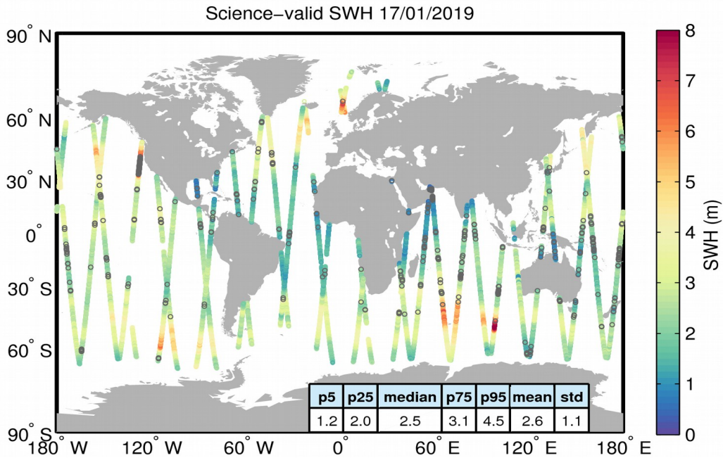
Figure 19. Geographical distribution of science-valid SWH data over oceans and lakes for 17/01/2019. The statistical values shown in the table refer to the SWH in m and are calculated over all measurements shown in the figure. Gray circles denote records that have been rejected based on the editing criteria described in Table 3.
