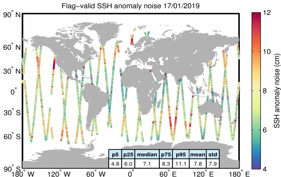
Figure 8. Geographical distribution of flag-valid 20-Hz SSH anomaly measurement noise over oceans and lakes for 17/01/2019. The statistical values shown in the table refer to the SSH anomaly noise and are calculated over all measurements shown in the figure.
