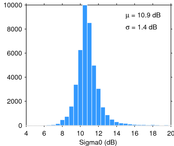
Figure 25. Histogram of flag-valid sigma0 over oceans and lakes for 17/01/2019. The mean ( \mu ) and standard deviation ( \sigma ) are also shown. Note that values outside [4 20] dB are excluded from the histogram for the sake of readability but not from the computation of \mu and \sigma .
