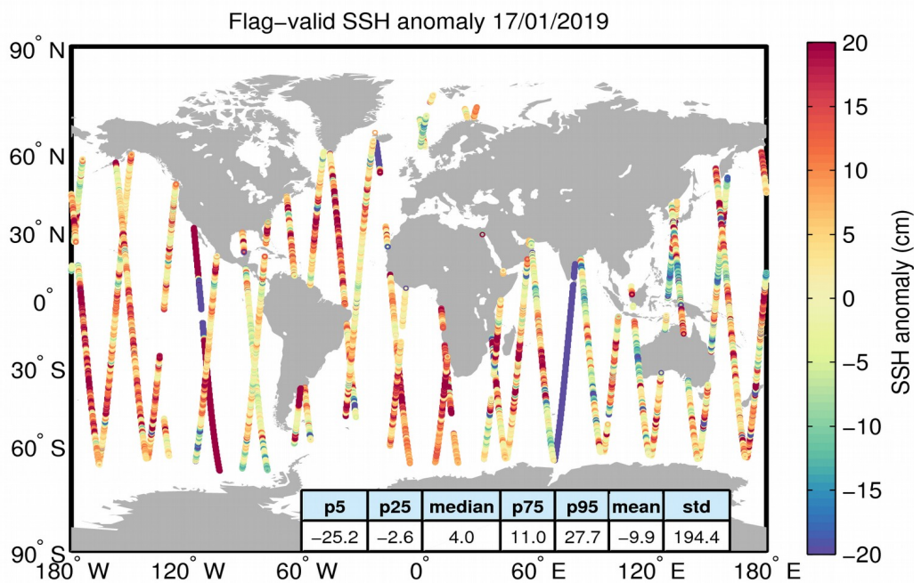
Figure 5. Geographical distribution of flag-valid 1-Hz SSH anomaly data over oceans and lakes for 17/01/2019. The statistical values shown in the table refer to the SSH anomaly in cm and are calculated over all measurements shown in the figure.
