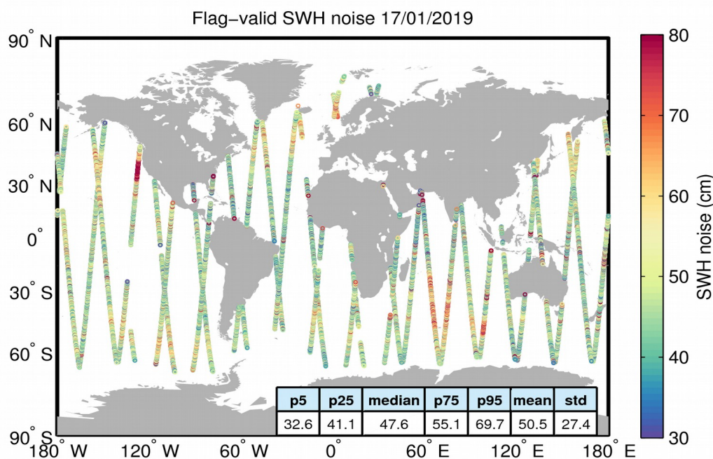
Figure 18. Geographical distribution of flag-valid 20-Hz SWH measurement noise over oceans and lakes for 17/01/2019. The statistical values shown in the figure refer to the SWH noise and are calculated over all measurements shown in the figure.
