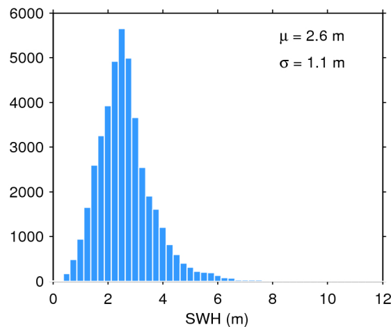
Figure 20. Histogram of science-valid SWH over oceans and lakes for 17/01/2019. The mean ( \mu ) and standard deviation ( \sigma ) are also shown. Note that values larger than 12 m are excluded from the histogram for the sake of readability but not from the computation of \mu and \sigma .
