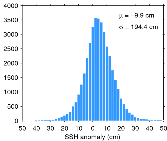
Figure 7. Histogram of flag-valid SSH anomaly over oceans and lakes for 17/01/2019. The mean ( \mu ) and standard deviation ( \sigma ) are also shown. Note that values outside [-50\ 50] cm are excluded from the histogram for the sake of readability but not from the computation of \mu and \sigma .
