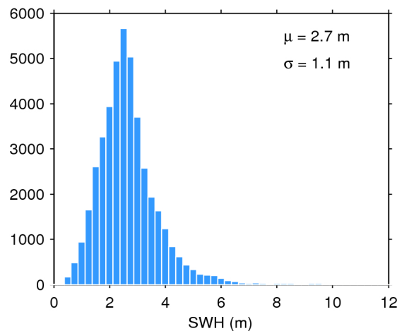
Figure 17. Histogram of flag-valid SWH over oceans and lakes for 17/01/2019. The mean ( \mu ) and standard deviation ( \sigma ) are also shown. Note that values larger than 12 m are excluded from the histogram for the sake of readability but not from the computation of \mu and \sigma .
