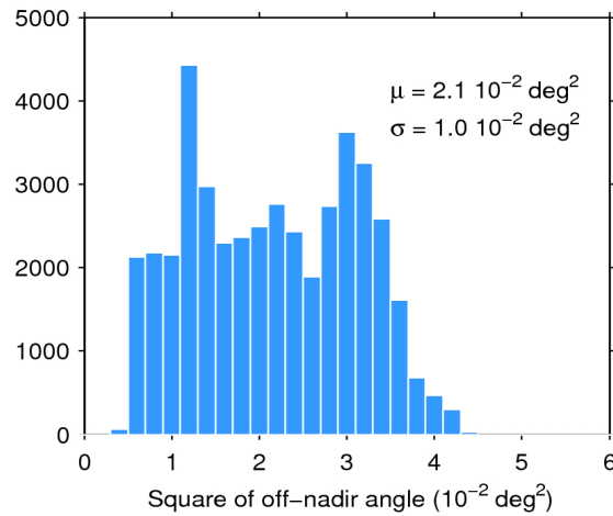
Figure 39. Histogram of flag-valid mispointing over oceans and lakes for 17/01/2019. The mean ( \mu ) and standard deviation ( \sigma ) are also shown. Note that values larger than 6 \cdot 10^{-2} \text{ deg}^2 are excluded from the histogram for the sake of readability but not from the computation of \mu and \sigma .
