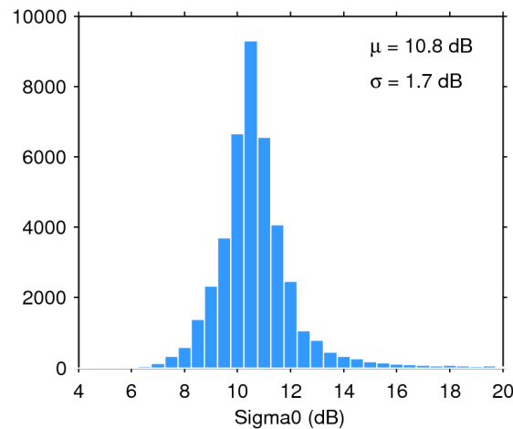
Figure 25. Histogram of flag-valid sigma0 over oceans and lakes for 16/01/2019. The mean ( \mu ) and standard deviation ( \sigma ) are also shown. Note that values outside [4 20] dB are excluded from the histogram for the sake of readability but not from the computation of \mu and \sigma .
