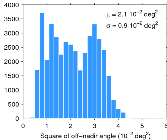
Figure 39. Histogram of flag-valid mispointing over oceans and lakes for 16/01/2019. The mean ( \mu ) and standard deviation ( \sigma ) are also shown. Note that values larger than 6 \cdot 10^{-2} \text{ deg}^2 are excluded from the histogram for the sake of readability but not from the computation of \mu and \sigma .
