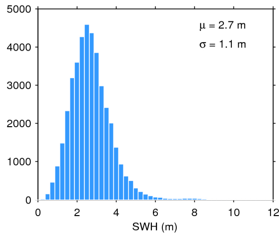
Figure 17. Histogram of flag-valid SWH over oceans and lakes for 16/01/2019. The mean ( \mu ) and standard deviation ( \sigma ) are also shown. Note that values larger than 12 m are excluded from the histogram for the sake of readability but not from the computation of \mu and \sigma .
