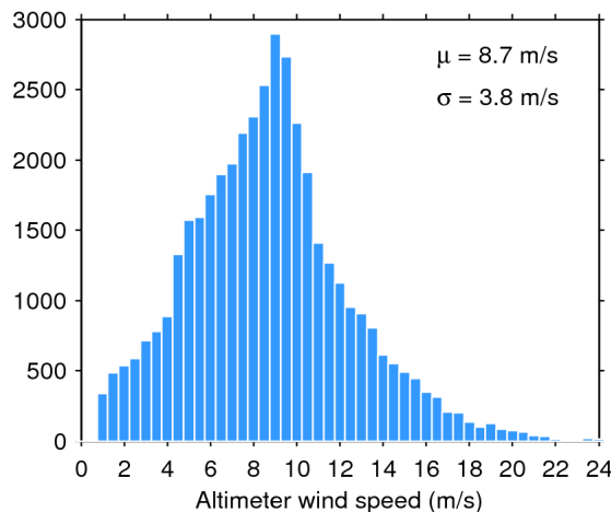
Figure 35. Histogram of science-valid wind over oceans and lakes for 16/01/2019. The mean ( \mu ) and standard deviation ( \sigma ) are also shown. Note that values larger than 24 m/s are excluded from the histogram for the sake of readability but not from the computation of \mu and \sigma .
