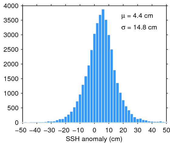
Figure 7. Histogram of flag-valid SSH anomaly over oceans and lakes for 16/01/2019. The mean ( \mu ) and standard deviation ( \sigma ) are also shown. Note that values outside [-50 50] cm are excluded from the histogram for the sake of readability but not from the computation of \mu and \sigma .
