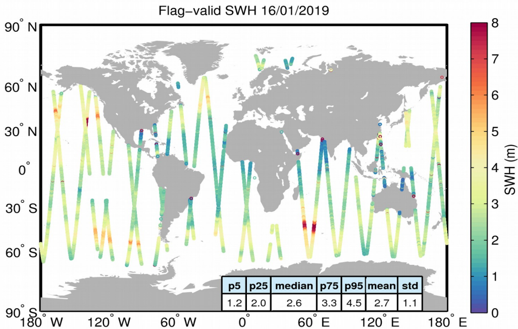
Figure 15. Geographical distribution of flag-valid SWH data over oceans and lakes for 16/01/2019. The statistical values shown in the table refer to the SWH in m and are calculated over all measurements shown in the figure.
