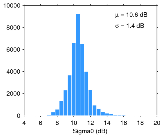
Figure 28. Histogram of science-valid sigma0 over oceans and lakes for 16/01/2019. The mean ( \mu ) and standard deviation ( \sigma ) are also shown. Note that values outside [4 20] dB are excluded from the histogram for the sake of readability but not from the computation of \mu and \sigma .
