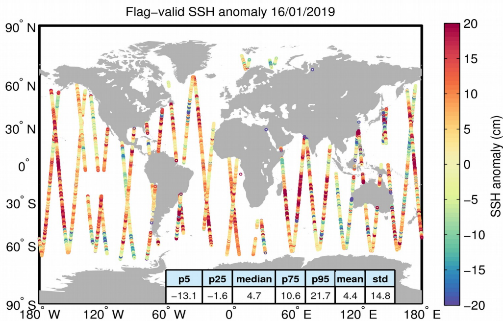
Figure 5. Geographical distribution of flag-valid 1-Hz SSH anomaly data over oceans and lakes for 16/01/2019. The statistical values shown in the table refer to the SSH anomaly in cm and are calculated over all measurements shown in the figure.
