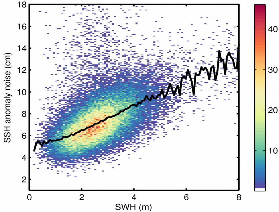
Figure 9. 2D histogram showing flag-valid SSH anomaly noise as a function of SWH for 16/01/2019. The black line denotes the median SSH anomaly noise as a function of SWH.
