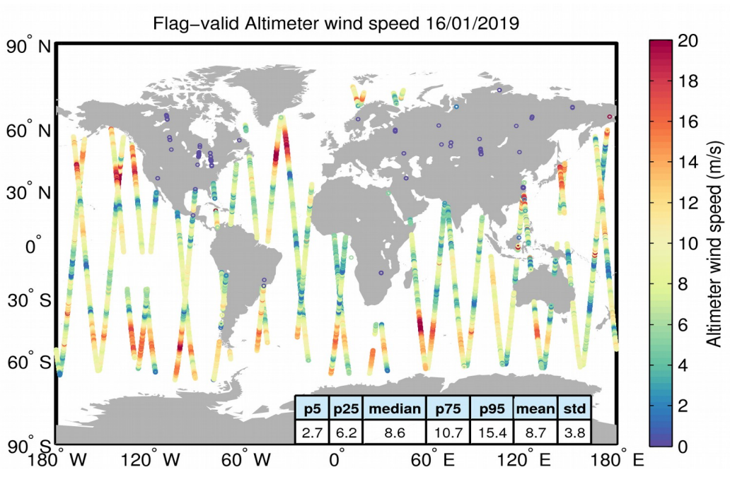
Figure 31. Geographical distribution of flag-valid wind data over oceans and lakes for 16/01/2019. The statistical values shown in the table refer to the wind in m/s and are calculated over all measurements shown in the figure.
