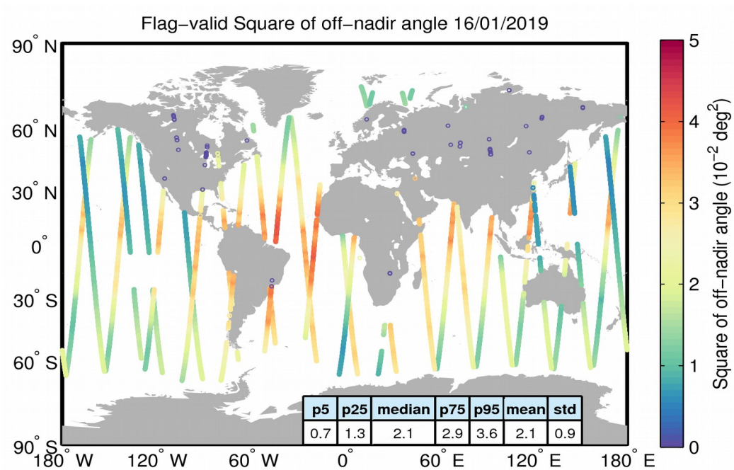
Figure 37. Geographical distribution of flag-valid mispointing data over oceans and lakes for 16/01/2019. The statistical values shown in the table refer to the mispointing in 10^{-2} \text{ deg}^2 and are calculated over all measurements shown in the figure.
