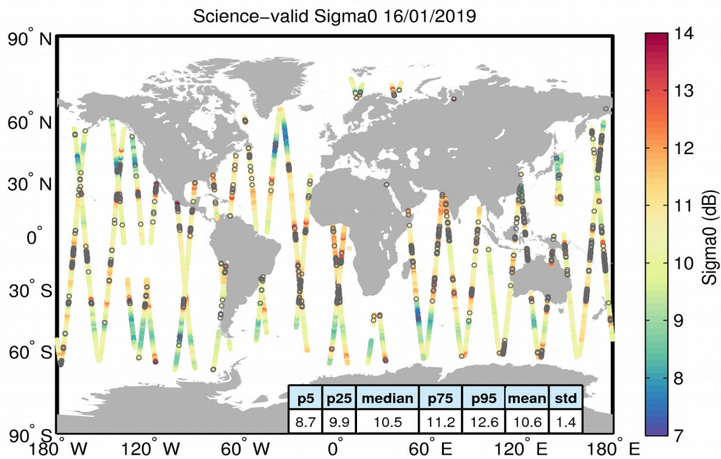
Figure 27. Geographical distribution of science-valid sigma0 data over oceans and lakes for 16/01/2019. The statistical values shown in the table refer to the sigma0 in dB and are calculated over all measurements shown in the figure. Gray circles denote records that have been rejected based on the editing criteria described in Table 4.
