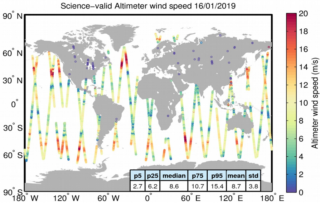
Figure 34. Geographical distribution of science-valid wind data over oceans and lakes for 16/01/2019. The statistical values shown in the table refer to the wind in m/s and are calculated over all measurements shown in the figure. Gray circles denote records that have been rejected based on the editing criteria described in Table 5.
