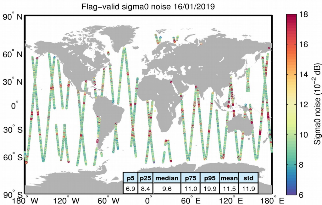
Figure 26. Geographical distribution of flag-valid 20-Hz sigma0 measurement noise over oceans and lakes for 16/01/2019. The statistical values shown in the table refer to the sigma0 noise and are calculated over all measurements shown in the figure.
