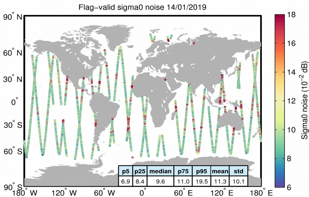
Figure 26. Geographical distribution of flag-valid 20-Hz sigma0 measurement noise over oceans and lakes for 14/01/2019. The statistical values shown in the table refer to the sigma0 noise and are calculated over all measurements shown in the figure.
