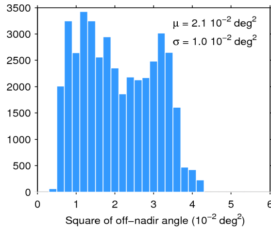
Figure 39. Histogram of flag-valid mispointing over oceans and lakes for 14/01/2019. The mean ( \mu ) and standard deviation ( \sigma ) are also shown. Note that values larger than 6 \cdot 10^{-2} \text{ deg}^2 are excluded from the histogram for the sake of readability but not from the computation of \mu and \sigma .
