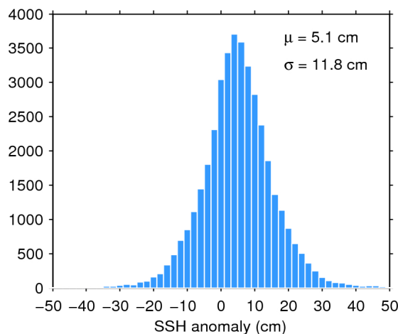
Figure 11. Histogram of science-valid SSH anomaly over oceans and lakes for 14/01/2019. The mean ( \mu ) and standard deviation ( \sigma ) are also shown. Note that values outside [-50 50] cm are excluded from the histogram for the sake of readability but not from the computation of \mu and \sigma .
