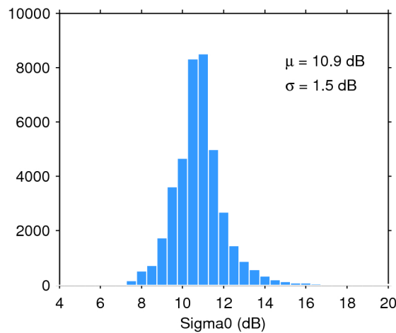
Figure 28. Histogram of science-valid sigma0 over oceans and lakes for 14/01/2019. The mean ( \mu ) and standard deviation ( \sigma ) are also shown. Note that values outside [4 20] dB are excluded from the histogram for the sake of readability but not from the computation of \mu and \sigma .
