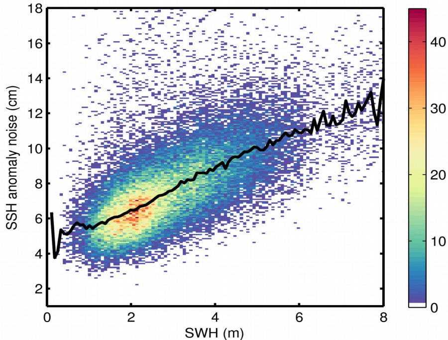
Figure 9. 2D histogram showing flag-valid SSH anomaly noise as a function of SWH for 14/01/2019. The black line denotes the median SSH anomaly noise as a function of SWH.
