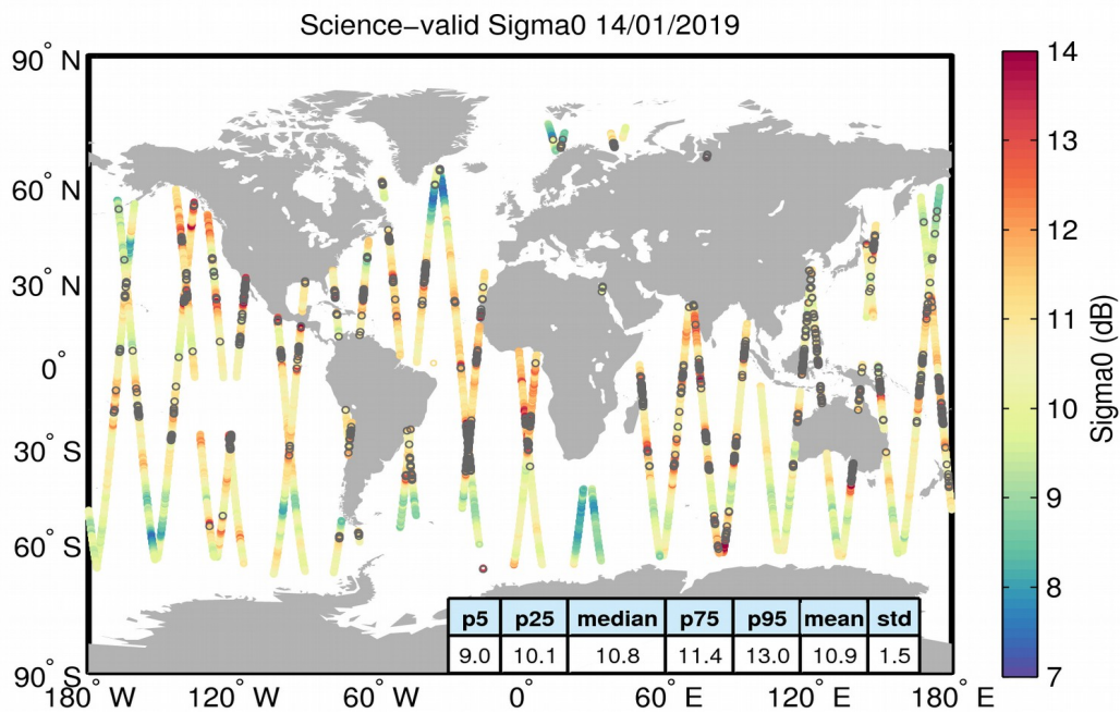
Figure 27. Geographical distribution of science-valid sigma0 data over oceans and lakes for 14/01/2019. The statistical values shown in the table refer to the sigma0 in dB and are calculated over all measurements shown in the figure. Gray circles denote records that have been rejected based on the editing criteria described in Table 4.
