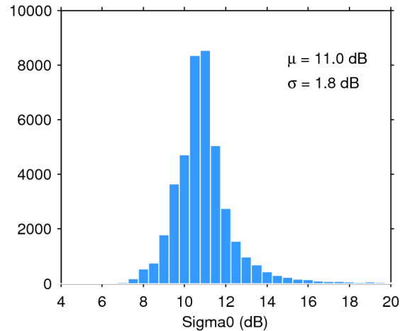
Figure 25. Histogram of flag-valid sigma0 over oceans and lakes for 14/01/2019. The mean ( \mu ) and standard deviation ( \sigma ) are also shown. Note that values outside [4 20] dB are excluded from the histogram for the sake of readability but not from the computation of \mu and \sigma .
