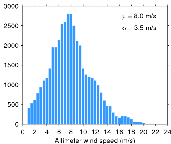
Figure 35. Histogram of science-valid wind over oceans and lakes for 14/01/2019. The mean ( \mu ) and standard deviation ( \sigma ) are also shown. Note that values larger than 24 m/s are excluded from the histogram for the sake of readability but not from the computation of \mu and \sigma .
