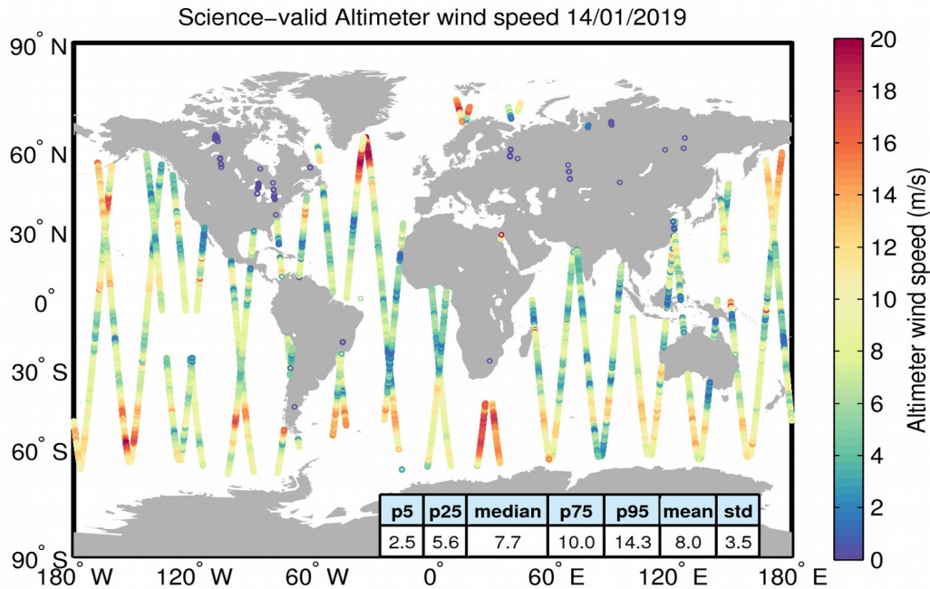
Figure 34. Geographical distribution of science-valid wind data over oceans and lakes for 14/01/2019. The statistical values shown in the table refer to the wind in m/s and are calculated over all measurements shown in the figure. Gray circles denote records that have been rejected based on the editing criteria described in Table 5.
