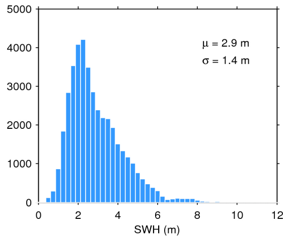
Figure 17. Histogram of flag-valid SWH over oceans and lakes for 14/01/2019. The mean ( \mu ) and standard deviation ( \sigma ) are also shown. Note that values larger than 12 m are excluded from the histogram for the sake of readability but not from the computation of \mu and \sigma .
