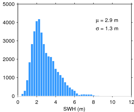
Figure 20. Histogram of science-valid SWH over oceans and lakes for 14/01/2019. The mean ( \mu ) and standard deviation ( \sigma ) are also shown. Note that values larger than 12 m are excluded from the histogram for the sake of readability but not from the computation of \mu and \sigma .
