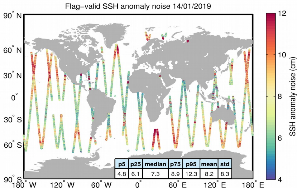
Figure 8. Geographical distribution of flag-valid 20-Hz SSH anomaly measurement noise over oceans and lakes for 14/01/2019. The statistical values shown in the table refer to the SSH anomaly noise and are calculated over all measurements shown in the figure.
