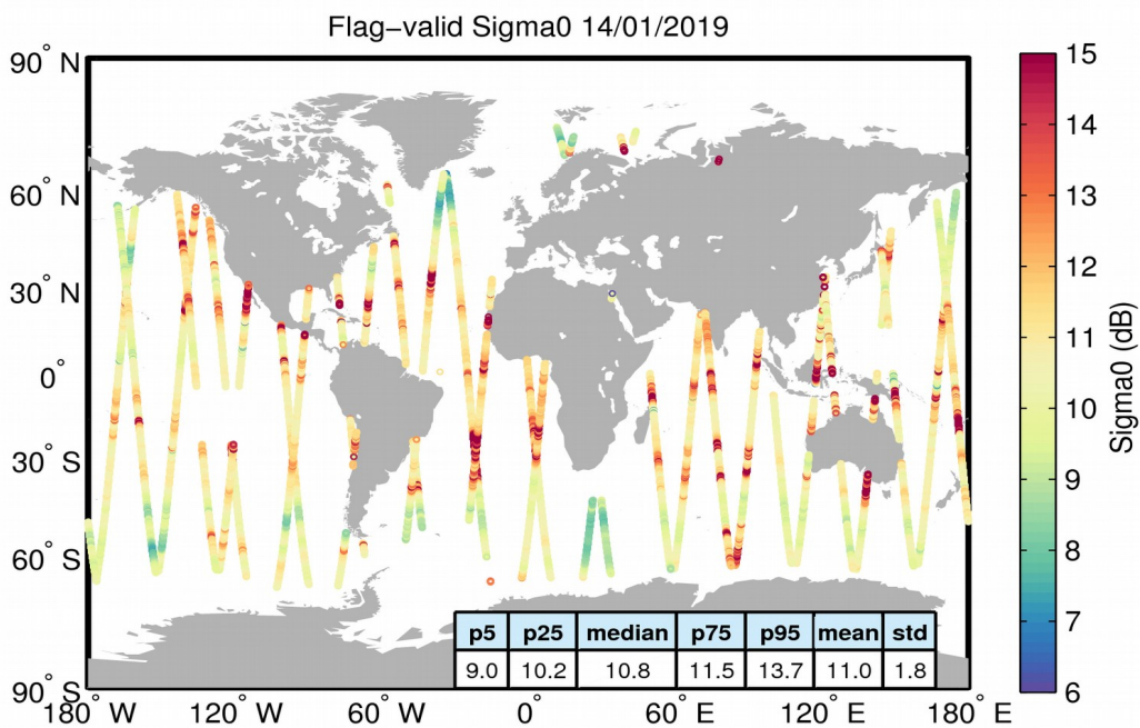
Figure 23. Geographical distribution of flag-valid sigma0 data over oceans and lakes for 14/01/2019. The statistical values shown in the table refer to the sigma0 in dB and are calculated over all measurements shown in the figure.
