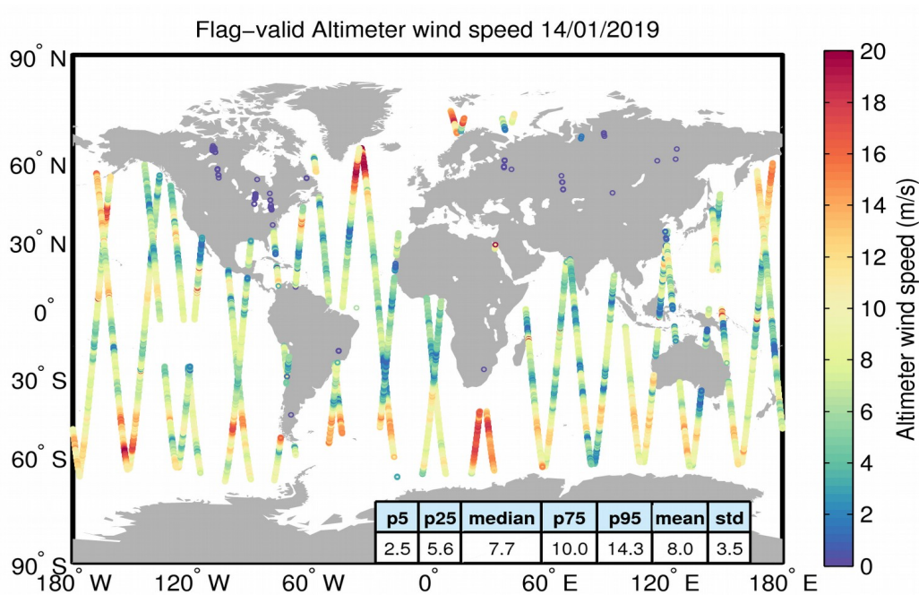
Figure 31. Geographical distribution of flag-valid wind data over oceans and lakes for 14/01/2019. The statistical values shown in the table refer to the wind in m/s and are calculated over all measurements shown in the figure.
