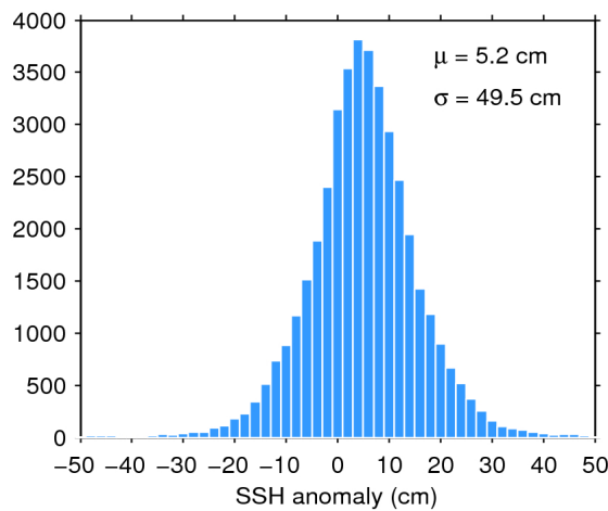
Figure 7. Histogram of flag-valid SSH anomaly over oceans and lakes for 14/01/2019. The mean ( \mu ) and standard deviation ( \sigma ) are also shown. Note that values outside [-50 50] cm are excluded from the histogram for the sake of readability but not from the computation of \mu and \sigma .
