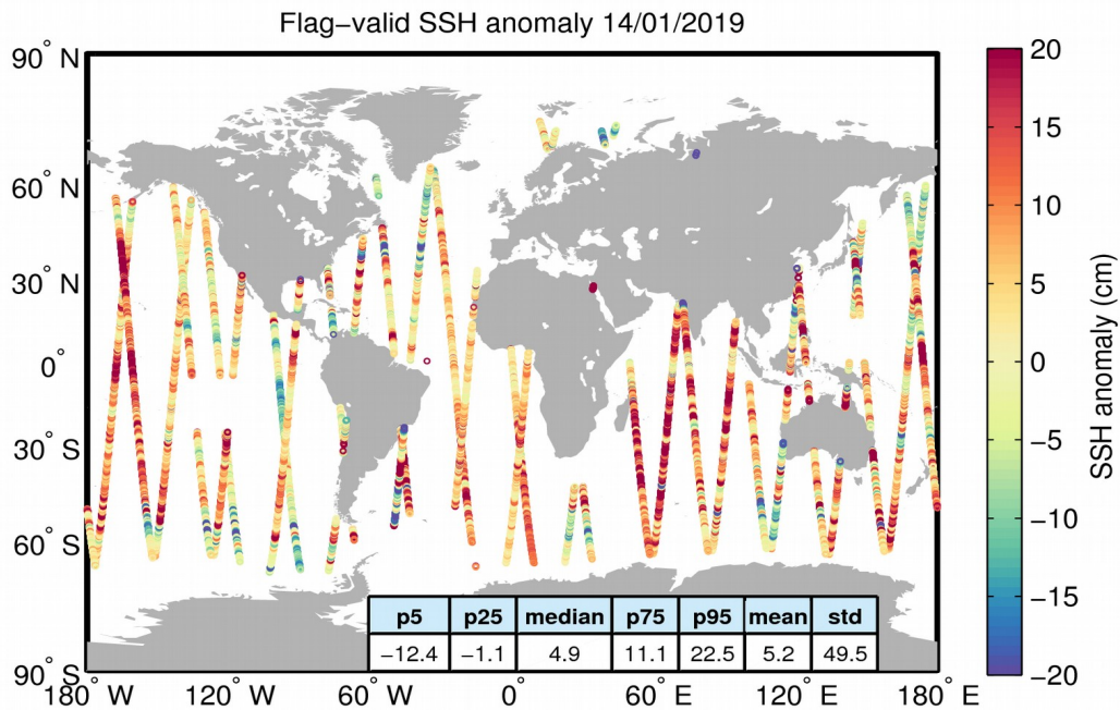
Figure 5. Geographical distribution of flag-valid 1-Hz SSH anomaly data over oceans and lakes for 14/01/2019. The statistical values shown in the table refer to the SSH anomaly in cm and are calculated over all measurements shown in the figure.
