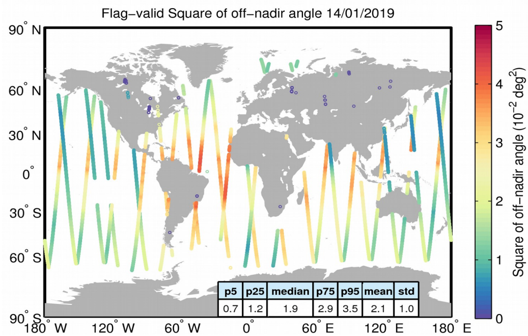
Figure 37. Geographical distribution of flag-valid mispointing data over oceans and lakes for 14/01/2019. The statistical values shown in the table refer to the mispointing in 10^{-2} \text{ deg}^2 and are calculated over all measurements shown in the figure.
