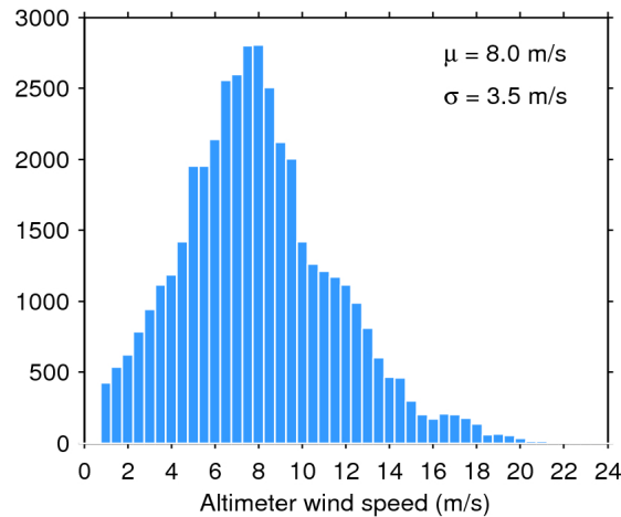
Figure 33. Histogram of flag-valid wind over oceans and lakes for 14/01/2019. The mean ( \mu ) and standard deviation ( \sigma ) are also shown. Note that values larger than 24 m/s are excluded from the histogram for the sake of readability but not from the computation of \mu and \sigma .
