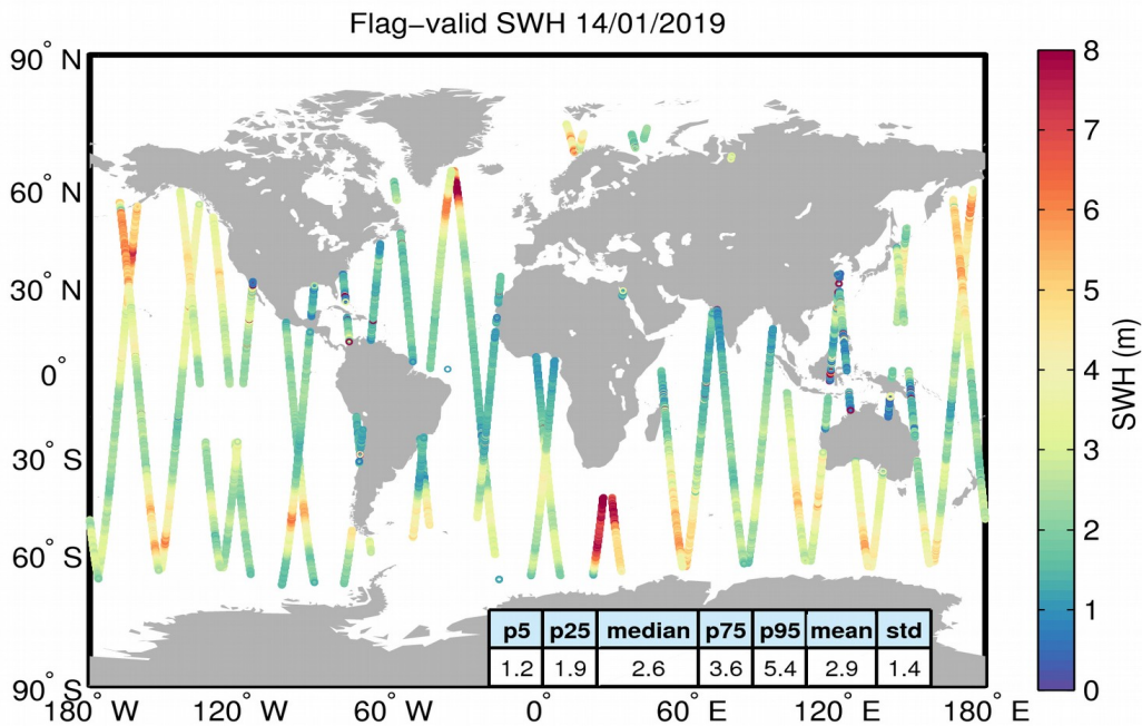
Figure 15. Geographical distribution of flag-valid SWH data over oceans and lakes for 14/01/2019. The statistical values shown in the table refer to the SWH in m and are calculated over all measurements shown in the figure.
