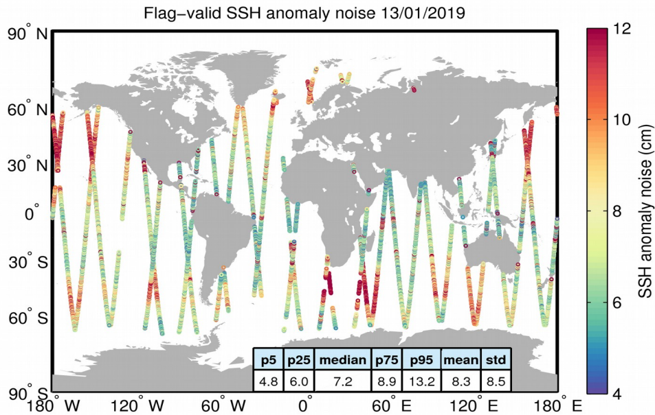
Figure 8. Geographical distribution of flag-valid 20-Hz SSH anomaly measurement noise over oceans and lakes for 13/01/2019. The statistical values shown in the table refer to the SSH anomaly noise and are calculated over all measurements shown in the figure.
