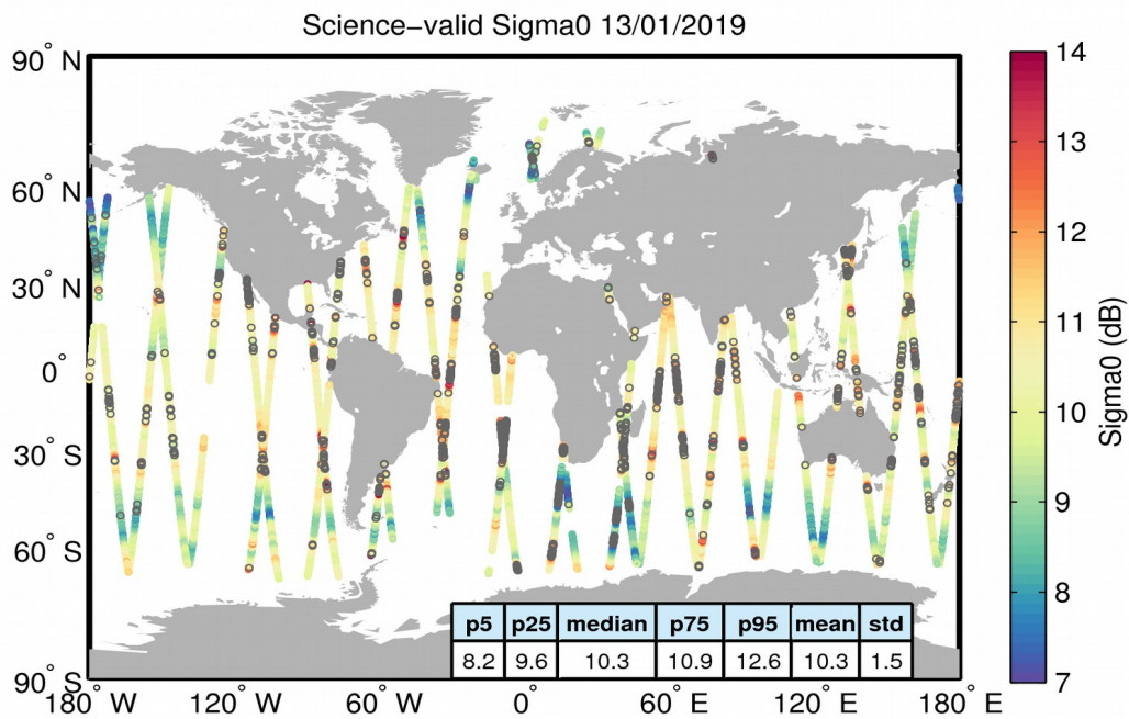
Figure 27. Geographical distribution of science-valid sigma0 data over oceans and lakes for 13/01/2019. The statistical values shown in the table refer to the sigma0 in dB and are calculated over all measurements shown in the figure. Gray circles denote records that have been rejected based on the editing criteria described in Table 4.
