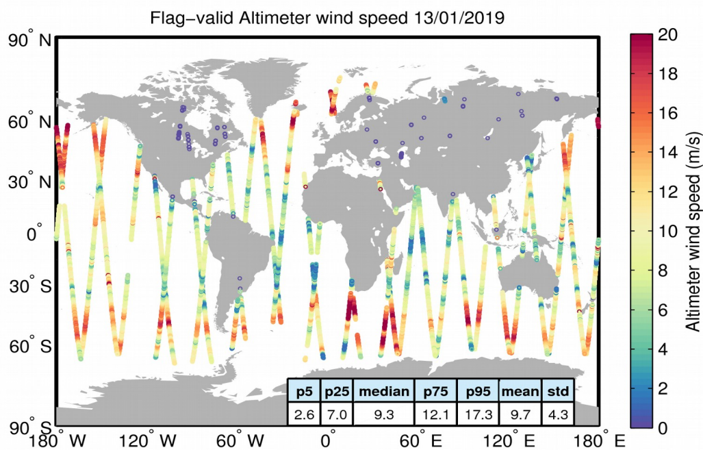
Figure 31. Geographical distribution of flag-valid wind data over oceans and lakes for 13/01/2019. The statistical values shown in the table refer to the wind in m/s and are calculated over all measurements shown in the figure.
