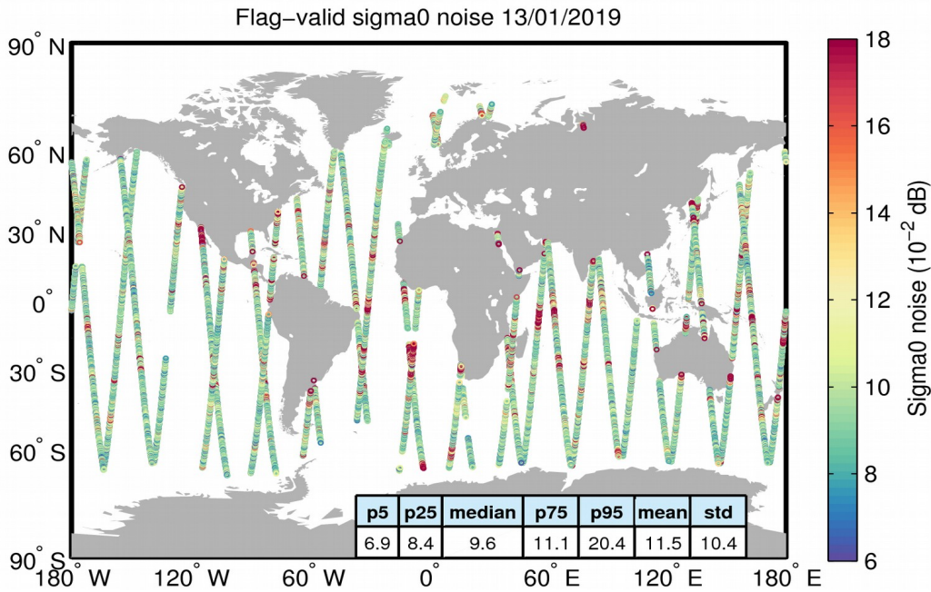
Figure 26. Geographical distribution of flag-valid 20-Hz sigma0 measurement noise over oceans and lakes for 13/01/2019. The statistical values shown in the table refer to the sigma0 noise and are calculated over all measurements shown in the figure.
