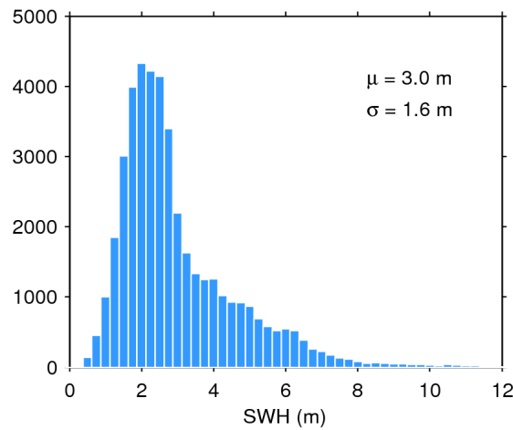
Figure 17. Histogram of flag-valid SWH over oceans and lakes for 13/01/2019. The mean ( \mu ) and standard deviation ( \sigma ) are also shown. Note that values larger than 12 m are excluded from the histogram for the sake of readability but not from the computation of \mu and \sigma .
