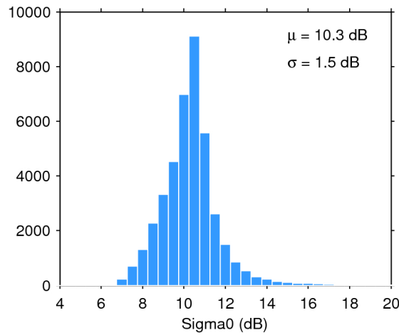
Figure 28. Histogram of science-valid sigma0 over oceans and lakes for 13/01/2019. The mean ( \mu ) and standard deviation ( \sigma ) are also shown. Note that values outside [4 20] dB are excluded from the histogram for the sake of readability but not from the computation of \mu and \sigma .
