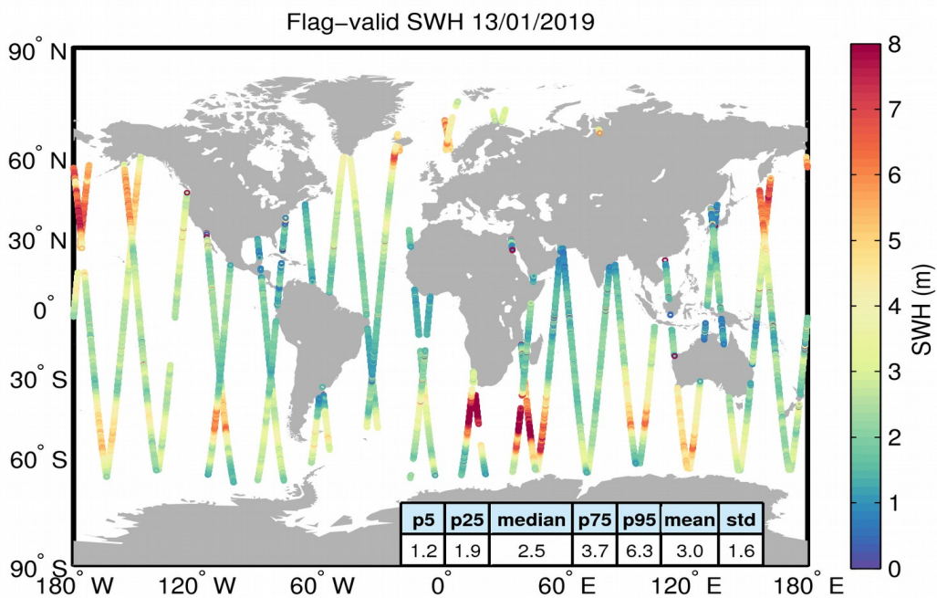
Figure 15. Geographical distribution of flag-valid SWH data over oceans and lakes for 13/01/2019. The statistical values shown in the table refer to the SWH in m and are calculated over all measurements shown in the figure.
