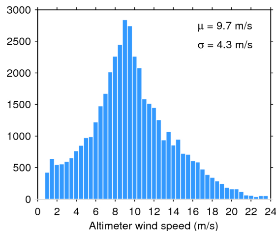
Figure 35. Histogram of science-valid wind over oceans and lakes for 13/01/2019. The mean ( \mu ) and standard deviation ( \sigma ) are also shown. Note that values larger than 24 m/s are excluded from the histogram for the sake of readability but not from the computation of \mu and \sigma .
