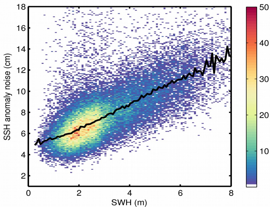
Figure 9. 2D histogram showing flag-valid SSH anomaly noise as a function of SWH for 13/01/2019. The black line denotes the median SSH anomaly noise as a function of SWH.
