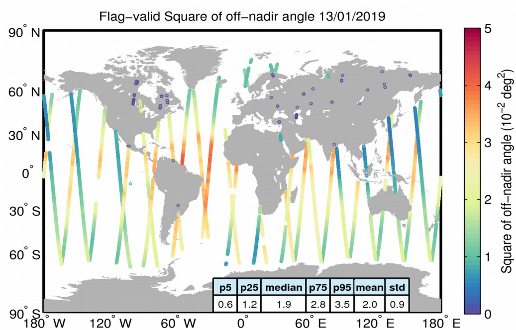
Figure 37. Geographical distribution of flag-valid mispointing data over oceans and lakes for 13/01/2019. The statistical values shown in the table refer to the mispointing in 10^{-2} deg 2 and are calculated over all measurements shown in the figure.
