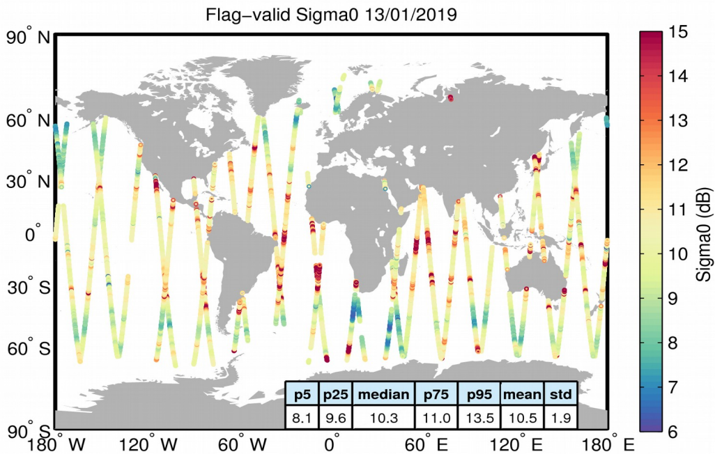
Figure 23. Geographical distribution of flag-valid sigma0 data over oceans and lakes for 13/01/2019. The statistical values shown in the table refer to the sigma0 in dB and are calculated over all measurements shown in the figure.
