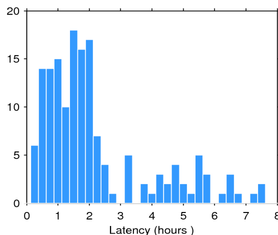
Figure 2. Histogram of the data latency for 13/01/2019. The y-axis denotes the number of files that are made available with a delay of x-hours with respect to the mean time of the records stored in the file.
