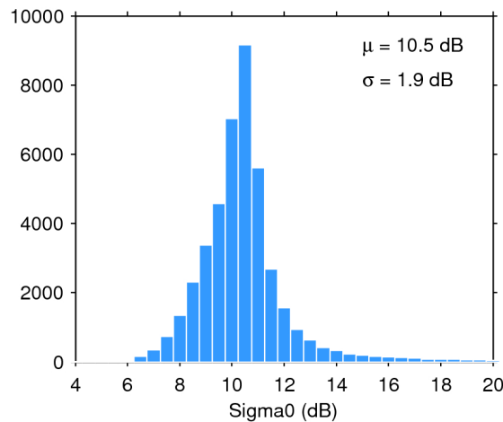
Figure 25. Histogram of flag-valid sigma0 over oceans and lakes for 13/01/2019. The mean ( \mu ) and standard deviation ( \sigma ) are also shown. Note that values outside [4 20] dB are excluded from the histogram for the sake of readability but not from the computation of \mu and \sigma .
