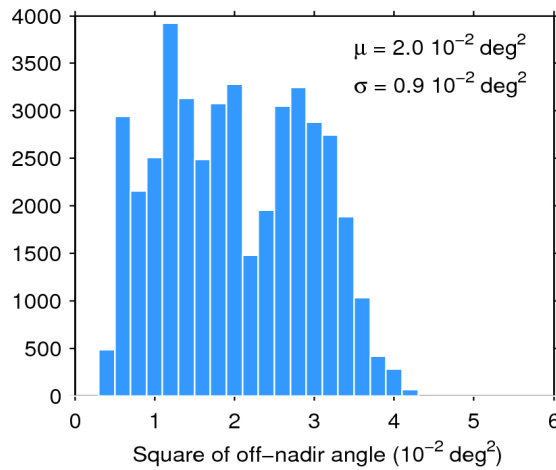
Figure 39. Histogram of flag-valid mispointing over oceans and lakes for 13/01/2019. The mean ( \mu ) and standard deviation ( \sigma ) are also shown. Note that values larger than 6 \cdot 10^{-2} \text{ deg}^2 are excluded from the histogram for the sake of readability but not from the computation of \mu and \sigma .
