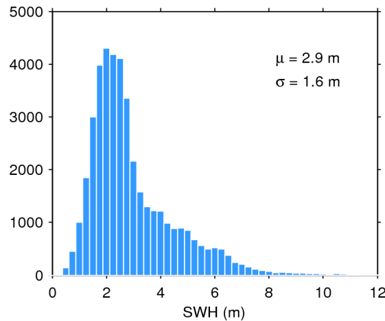
Figure 20. Histogram of science-valid SWH over oceans and lakes for 13/01/2019. The mean ( \mu ) and standard deviation ( \sigma ) are also shown. Note that values larger than 12 m are excluded from the histogram for the sake of readability but not from the computation of \mu and \sigma .
