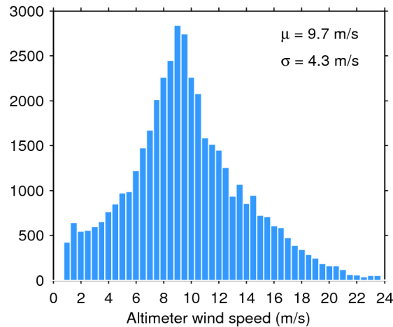
Figure 33. Histogram of flag-valid wind over oceans and lakes for 13/01/2019. The mean ( \mu ) and standard deviation ( \sigma ) are also shown. Note that values larger than 24 m/s are excluded from the histogram for the sake of readability but not from the computation of \mu and \sigma .
