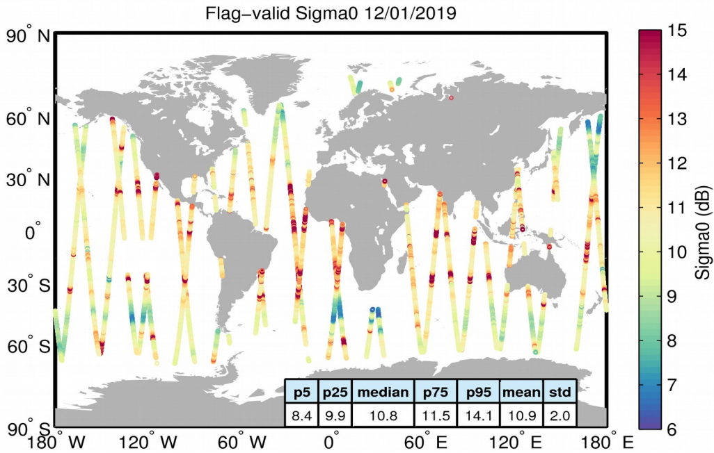
Figure 23. Geographical distribution of flag-valid sigma0 data over oceans and lakes for 12/01/2019. The statistical values shown in the table refer to the sigma0 in dB and are calculated over all measurements shown in the figure.
