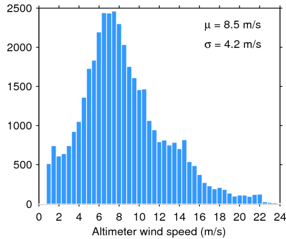
Figure 33. Histogram of flag-valid wind over oceans and lakes for 12/01/2019. The mean ( \mu ) and standard deviation ( \sigma ) are also shown. Note that values larger than 24 m/s are excluded from the histogram for the sake of readability but not from the computation of \mu and \sigma .
