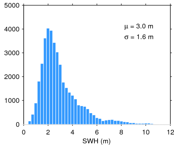
Figure 20. Histogram of science-valid SWH over oceans and lakes for 12/01/2019. The mean ( \mu ) and standard deviation ( \sigma ) are also shown. Note that values larger than 12 m are excluded from the histogram for the sake of readability but not from the computation of \mu and \sigma .
