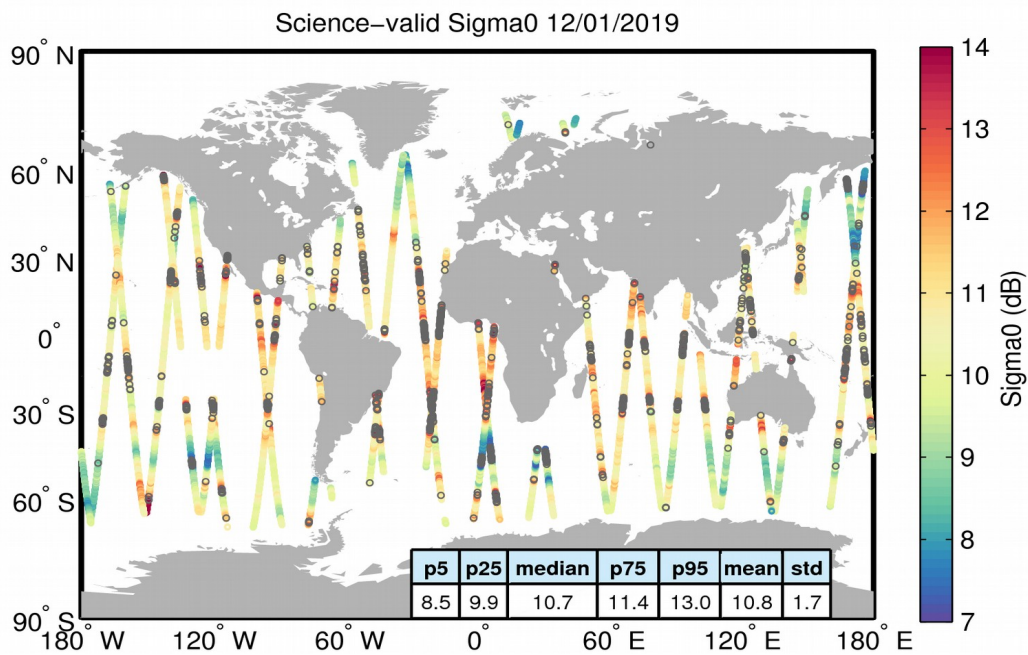
Figure 27. Geographical distribution of science-valid sigma0 data over oceans and lakes for 12/01/2019. The statistical values shown in the table refer to the sigma0 in dB and are calculated over all measurements shown in the figure. Gray circles denote records that have been rejected based on the editing criteria described in Table 4.
