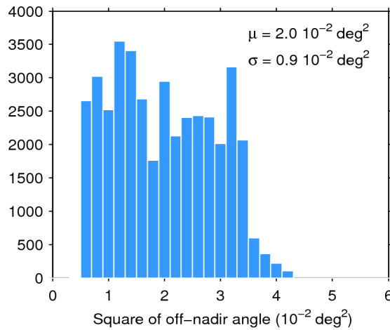
Figure 39. Histogram of flag-valid mispointing over oceans and lakes for 12/01/2019. The mean ( \mu ) and standard deviation ( \sigma ) are also shown. Note that values larger than 6 \cdot 10^{-2} \text{ deg}^2 are excluded from the histogram for the sake of readability but not from the computation of \mu and \sigma .
