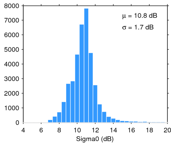
Figure 28. Histogram of science-valid sigma0 over oceans and lakes for 12/01/2019. The mean ( \mu ) and standard deviation ( \sigma ) are also shown. Note that values outside [4 20] dB are excluded from the histogram for the sake of readability but not from the computation of \mu and \sigma .
