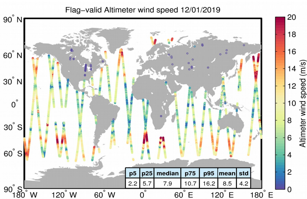
Figure 31. Geographical distribution of flag-valid wind data over oceans and lakes for 12/01/2019. The statistical values shown in the table refer to the wind in m/s and are calculated over all measurements shown in the figure.
