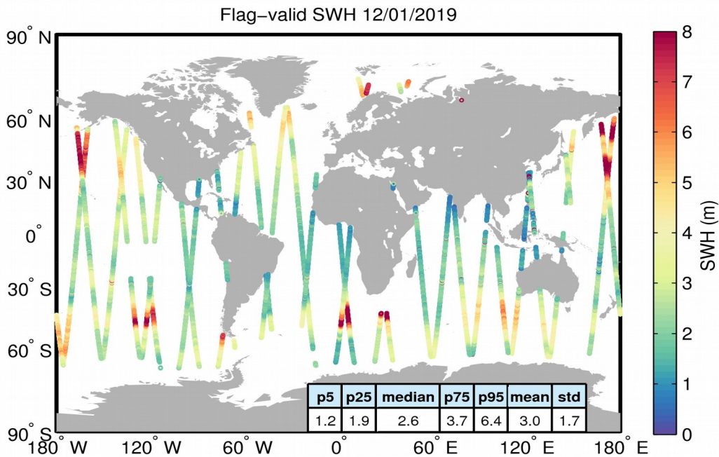
Figure 15. Geographical distribution of flag-valid SWH data over oceans and lakes for 12/01/2019. The statistical values shown in the table refer to the SWH in m and are calculated over all measurements shown in the figure.
