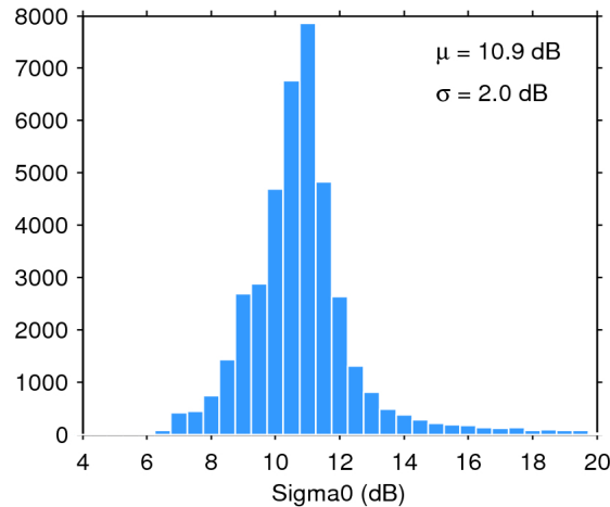
Figure 25. Histogram of flag-valid sigma0 over oceans and lakes for 12/01/2019. The mean ( \mu ) and standard deviation ( \sigma ) are also shown. Note that values outside [4 20] dB are excluded from the histogram for the sake of readability but not from the computation of \mu and \sigma .
