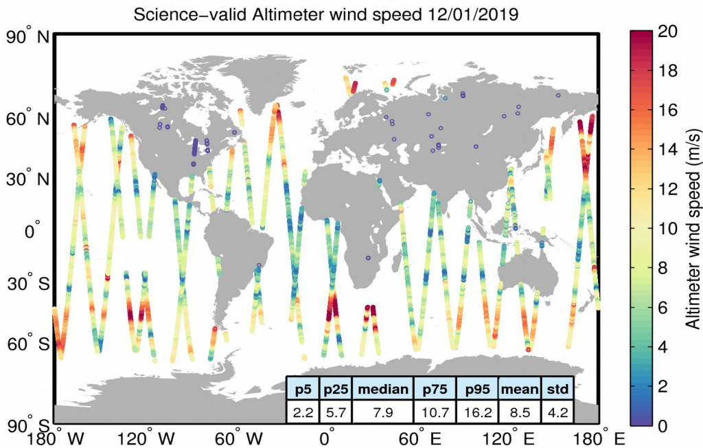
Figure 34. Geographical distribution of science-valid wind data over oceans and lakes for 12/01/2019. The statistical values shown in the table refer to the wind in m/s and are calculated over all measurements shown in the figure. Gray circles denote records that have been rejected based on the editing criteria described in Table 5.
