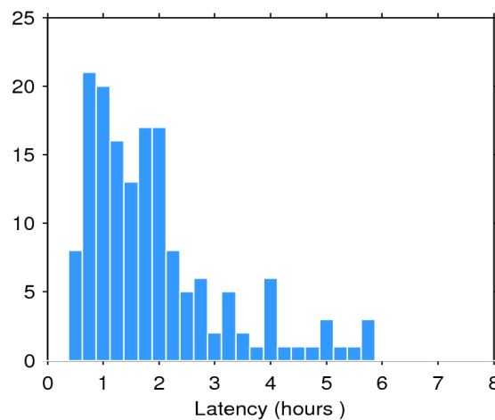
Figure 2. Histogram of the data latency for 12/01/2019. The y-axis denotes the number of files that are made available with a delay of x-hours with respect to the mean time of the records stored in the file.
