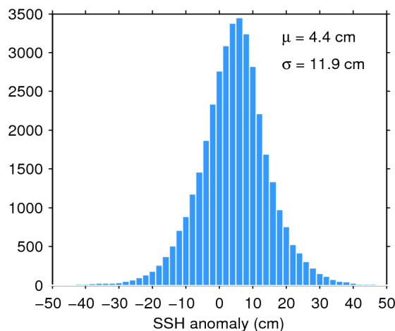
Figure 11. Histogram of science-valid SSH anomaly over oceans and lakes for 12/01/2019. The mean ( \mu ) and standard deviation ( \sigma ) are also shown. Note that values outside [-50 50] cm are excluded from the histogram for the sake of readability but not from the computation of \mu and \sigma .
