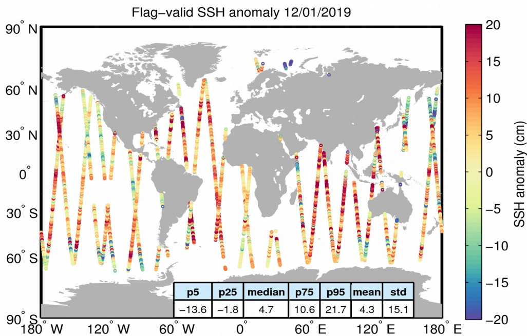
Figure 5. Geographical distribution of flag-valid 1-Hz SSH anomaly data over oceans and lakes for 12/01/2019. The statistical values shown in the table refer to the SSH anomaly in cm and are calculated over all measurements shown in the figure.
