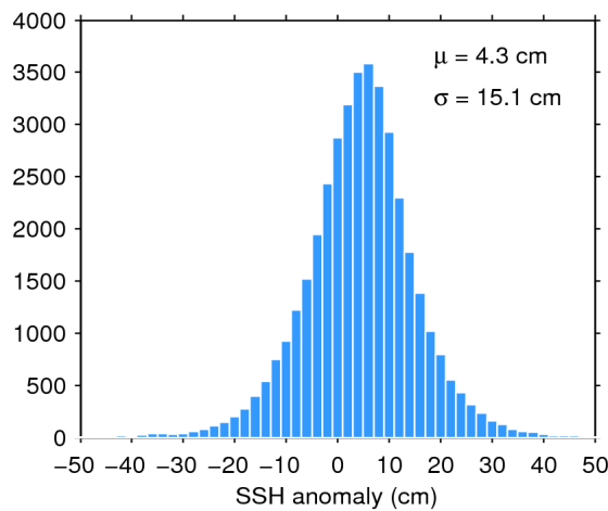
Figure 7. Histogram of flag-valid SSH anomaly over oceans and lakes for 12/01/2019. The mean ( \mu ) and standard deviation ( \sigma ) are also shown. Note that values outside [-50\ 50] cm are excluded from the histogram for the sake of readability but not from the computation of \mu and \sigma .
