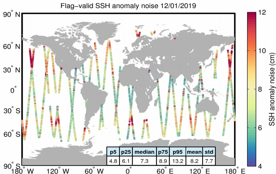
Figure 8. Geographical distribution of flag-valid 20-Hz SSH anomaly measurement noise over oceans and lakes for 12/01/2019. The statistical values shown in the table refer to the SSH anomaly noise and are calculated over all measurements shown in the figure.
