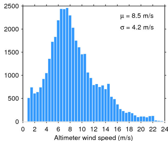
Figure 35. Histogram of science-valid wind over oceans and lakes for 12/01/2019. The mean ( \mu ) and standard deviation ( \sigma ) are also shown. Note that values larger than 24 m/s are excluded from the histogram for the sake of readability but not from the computation of \mu and \sigma .
