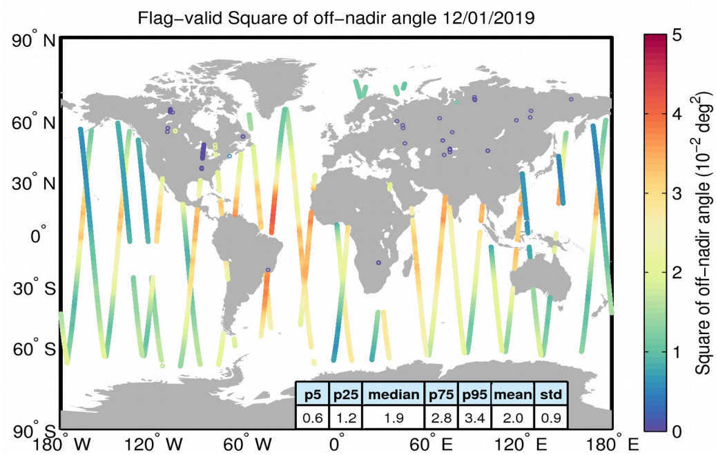
Figure 37. Geographical distribution of flag-valid mispointing data over oceans and lakes for 12/01/2019. The statistical values shown in the table refer to the mispointing in 10^{-2} deg 2 and are calculated over all measurements shown in the figure.
