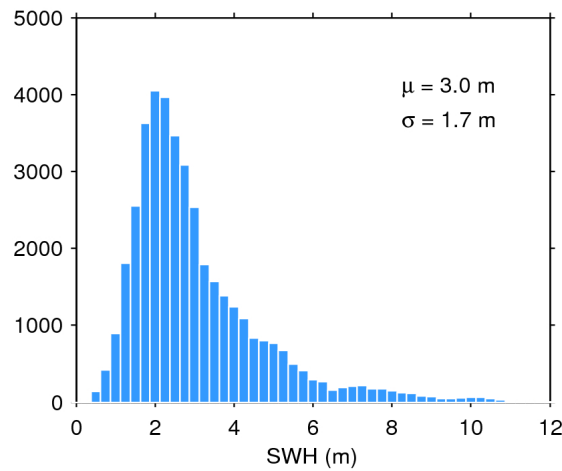
Figure 17. Histogram of flag-valid SWH over oceans and lakes for 12/01/2019. The mean ( \mu ) and standard deviation ( \sigma ) are also shown. Note that values larger than 12 m are excluded from the histogram for the sake of readability but not from the computation of \mu and \sigma .
