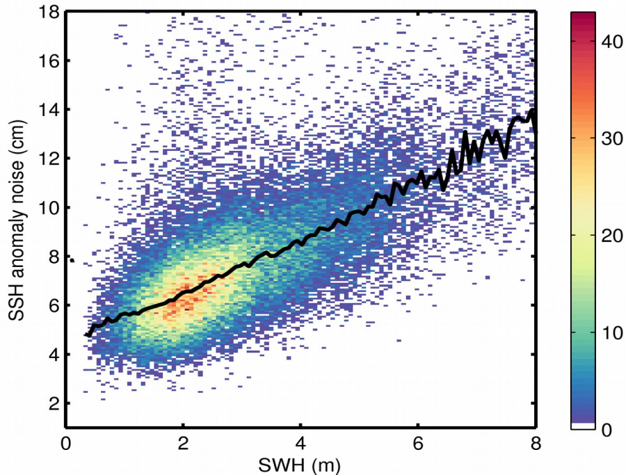
Figure 9. 2D histogram showing flag-valid SSH anomaly noise as a function of SWH for 12/01/2019. The black line denotes the median SSH anomaly noise as a function of SWH.
