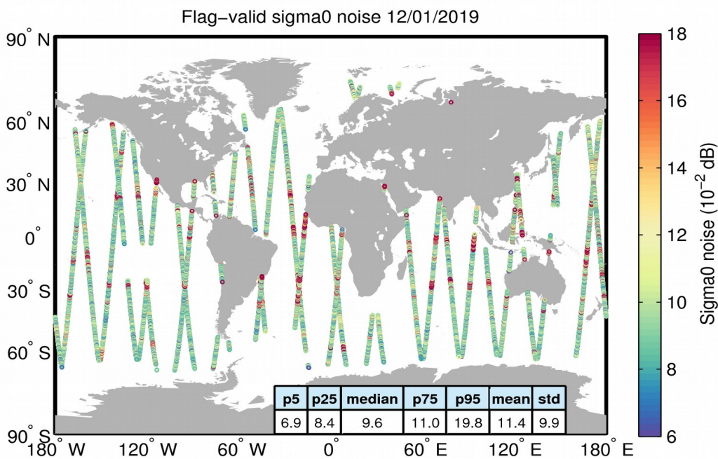
Figure 26. Geographical distribution of flag-valid 20-Hz sigma0 measurement noise over oceans and lakes for 12/01/2019. The statistical values shown in the table refer to the sigma0 noise and are calculated over all measurements shown in the figure.
