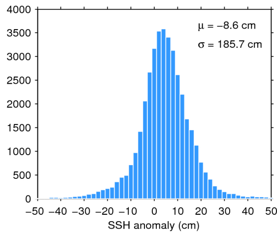
Figure 7. Histogram of flag-valid SSH anomaly over oceans and lakes for 11/01/2019. The mean ( \mu ) and standard deviation ( \sigma ) are also shown. Note that values outside [-50 50] cm are excluded from the histogram for the sake of readability but not from the computation of \mu and \sigma .
