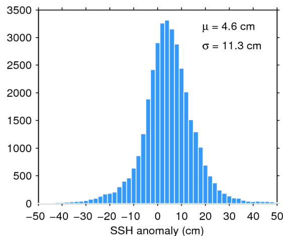
Figure 11. Histogram of science-valid SSH anomaly over oceans and lakes for 11/01/2019. The mean ( \mu ) and standard deviation ( \sigma ) are also shown. Note that values outside [-50 50] cm are excluded from the histogram for the sake of readability but not from the computation of \mu and \sigma .
