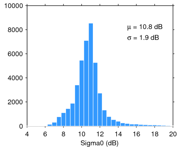
Figure 25. Histogram of flag-valid sigma0 over oceans and lakes for 11/01/2019. The mean ( \mu ) and standard deviation ( \sigma ) are also shown. Note that values outside [4 20] dB are excluded from the histogram for the sake of readability but not from the computation of \mu and \sigma .
