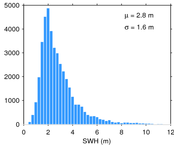
Figure 20. Histogram of science-valid SWH over oceans and lakes for 11/01/2019. The mean ( \mu ) and standard deviation ( \sigma ) are also shown. Note that values larger than 12 m are excluded from the histogram for the sake of readability but not from the computation of \mu and \sigma .
