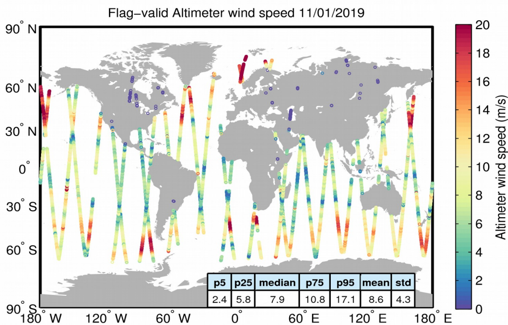
Figure 31. Geographical distribution of flag-valid wind data over oceans and lakes for 11/01/2019. The statistical values shown in the table refer to the wind in m/s and are calculated over all measurements shown in the figure.
