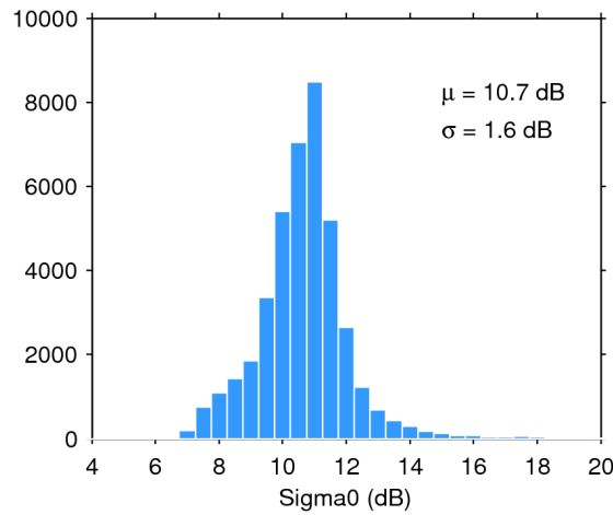
Figure 28. Histogram of science-valid sigma0 over oceans and lakes for 11/01/2019. The mean ( \mu ) and standard deviation ( \sigma ) are also shown. Note that values outside [4 20] dB are excluded from the histogram for the sake of readability but not from the computation of \mu and \sigma .
