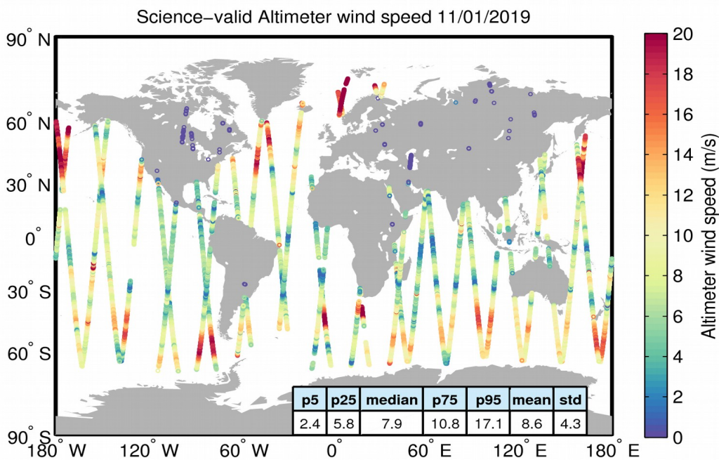
Figure 34. Geographical distribution of science-valid wind data over oceans and lakes for 11/01/2019. The statistical values shown in the table refer to the wind in m/s and are calculated over all measurements shown in the figure. Gray circles denote records that have been rejected based on the editing criteria described in Table 5.
