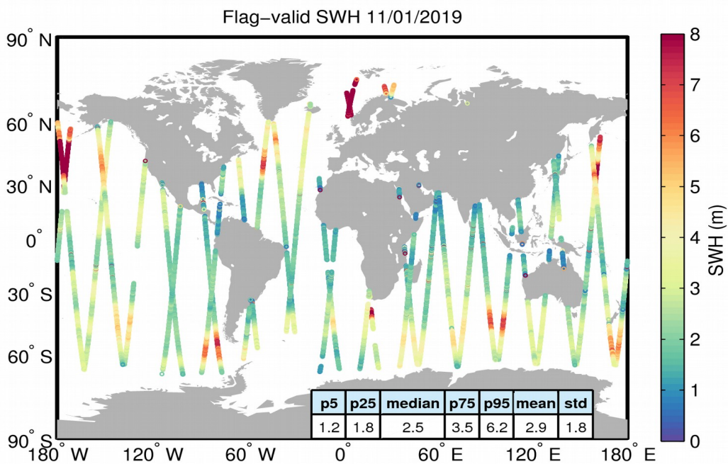
Figure 15. Geographical distribution of flag-valid SWH data over oceans and lakes for 11/01/2019. The statistical values shown in the table refer to the SWH in m and are calculated over all measurements shown in the figure.
