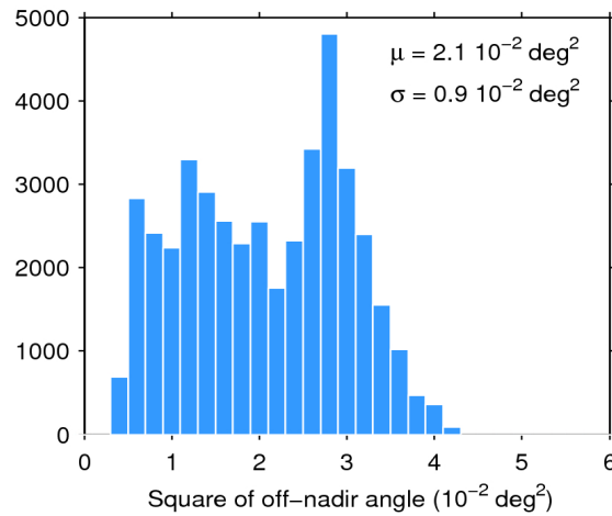
Figure 39. Histogram of flag-valid mispointing over oceans and lakes for 11/01/2019. The mean ( \mu ) and standard deviation ( \sigma ) are also shown. Note that values larger than 6 \cdot 10^{-2} \text{ deg}^2 are excluded from the histogram for the sake of readability but not from the computation of \mu and \sigma .
