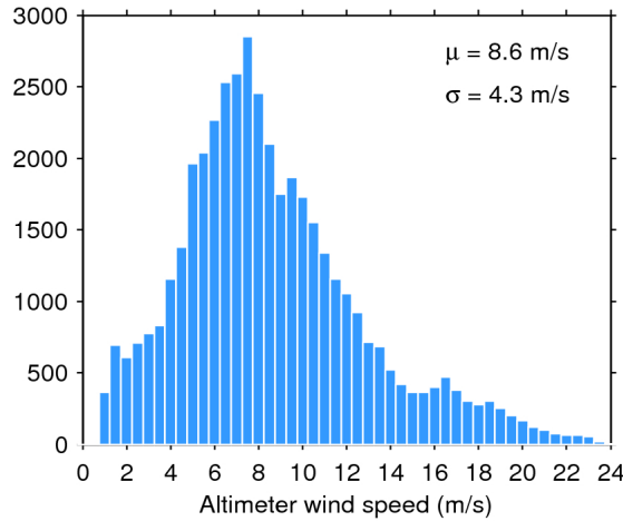
Figure 33. Histogram of flag-valid wind over oceans and lakes for 11/01/2019. The mean ( \mu ) and standard deviation ( \sigma ) are also shown. Note that values larger than 24 m/s are excluded from the histogram for the sake of readability but not from the computation of \mu and \sigma .
