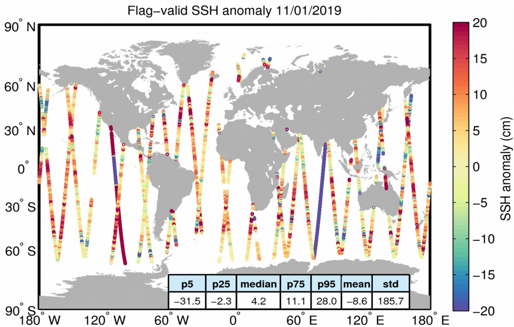
Figure 5. Geographical distribution of flag-valid 1-Hz SSH anomaly data over oceans and lakes for 11/01/2019. The statistical values shown in the table refer to the SSH anomaly in cm and are calculated over all measurements shown in the figure.
