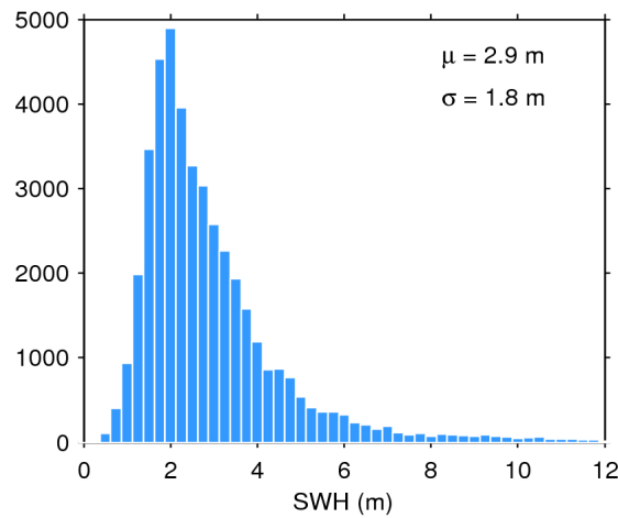
Figure 17. Histogram of flag-valid SWH over oceans and lakes for 11/01/2019. The mean ( \mu ) and standard deviation ( \sigma ) are also shown. Note that values larger than 12 m are excluded from the histogram for the sake of readability but not from the computation of \mu and \sigma .
