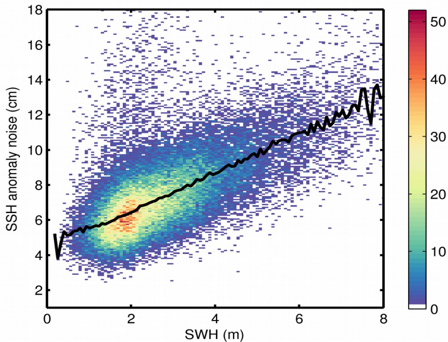
Figure 9. 2D histogram showing flag-valid SSH anomaly noise as a function of SWH for 11/01/2019. The black line denotes the median SSH anomaly noise as a function of SWH.
