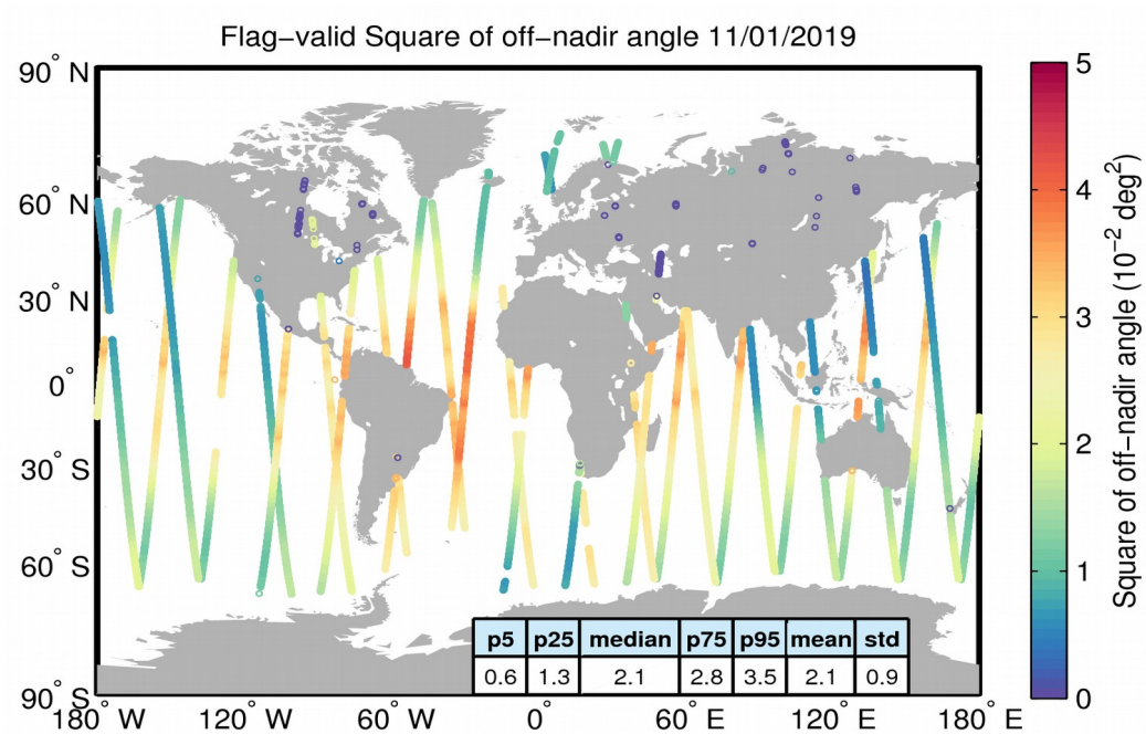
Figure 37. Geographical distribution of flag-valid mispointing data over oceans and lakes for 11/01/2019. The statistical values shown in the table refer to the mispointing in 10^{-2} \text{deg}^2 and are calculated over all measurements shown in the figure.
