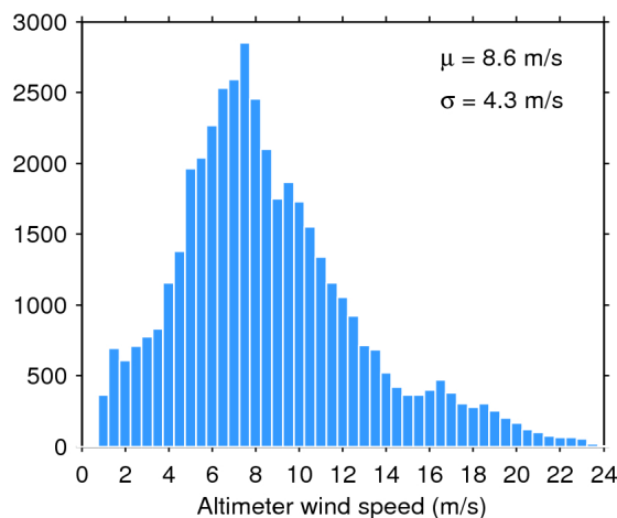
Figure 35. Histogram of science-valid wind over oceans and lakes for 11/01/2019. The mean ( \mu ) and standard deviation ( \sigma ) are also shown. Note that values larger than 24 m/s are excluded from the histogram for the sake of readability but not from the computation of \mu and \sigma .
