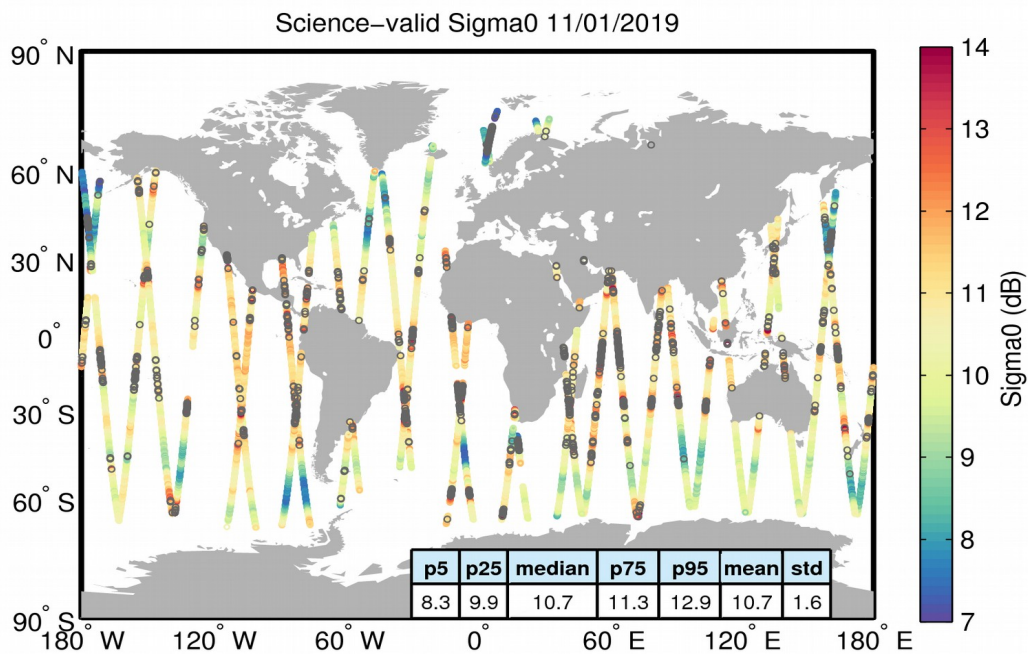
Figure 27. Geographical distribution of science-valid sigma0 data over oceans and lakes for 11/01/2019. The statistical values shown in the table refer to the sigma0 in dB and are calculated over all measurements shown in the figure. Gray circles denote records that have been rejected based on the editing criteria described in Table 4.
