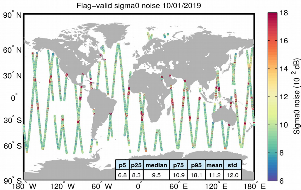
Figure 26. Geographical distribution of flag-valid 20-Hz sigma0 measurement noise over oceans and lakes for 10/01/2019. The statistical values shown in the table refer to the sigma0 noise and are calculated over all measurements shown in the figure.
