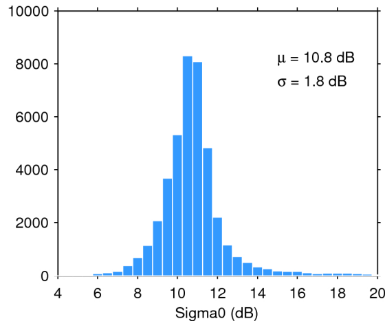
Figure 25. Histogram of flag-valid sigma0 over oceans and lakes for 10/01/2019. The mean ( \mu ) and standard deviation ( \sigma ) are also shown. Note that values outside [4 20] dB are excluded from the histogram for the sake of readability but not from the computation of \mu and \sigma .
