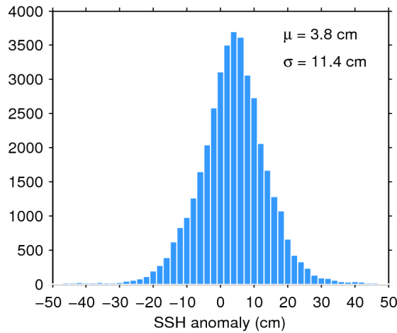
Figure 11. Histogram of science-valid SSH anomaly over oceans and lakes for 10/01/2019. The mean ( \mu ) and standard deviation ( \sigma ) are also shown. Note that values outside [-50 50] cm are excluded from the histogram for the sake of readability but not from the computation of \mu and \sigma .
