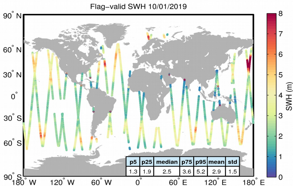
Figure 15. Geographical distribution of flag-valid SWH data over oceans and lakes for 10/01/2019. The statistical values shown in the table refer to the SWH in m and are calculated over all measurements shown in the figure.
