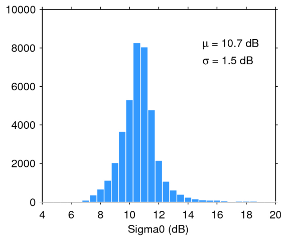
Figure 28. Histogram of science-valid sigma0 over oceans and lakes for 10/01/2019. The mean ( \mu ) and standard deviation ( \sigma ) are also shown. Note that values outside [4 20] dB are excluded from the histogram for the sake of readability but not from the computation of \mu and \sigma .
