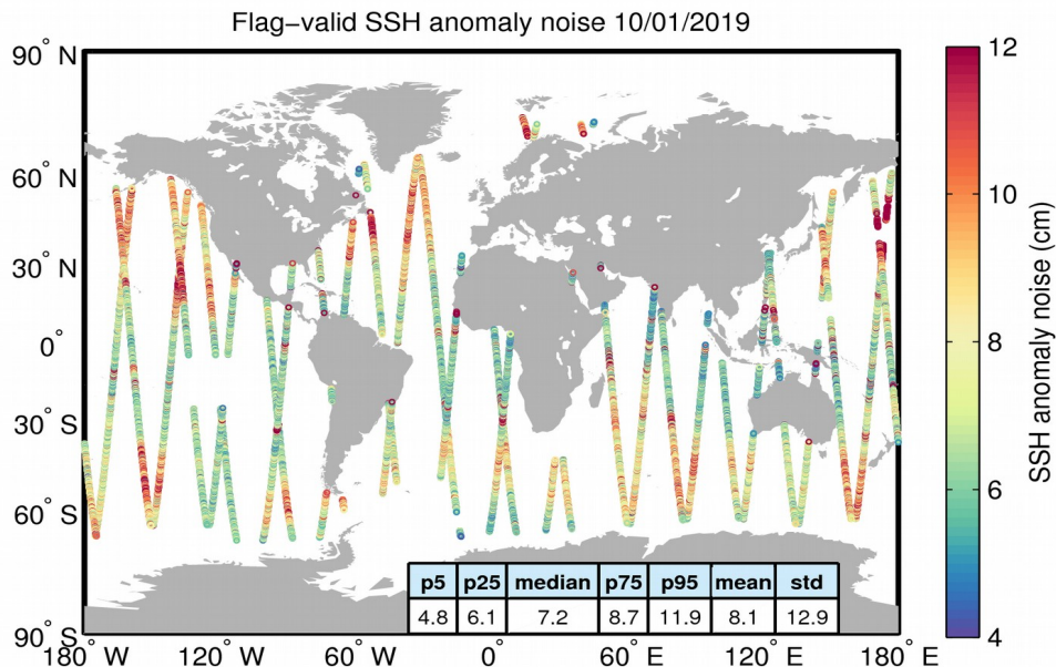
Figure 8. Geographical distribution of flag-valid 20-Hz SSH anomaly measurement noise over oceans and lakes for 10/01/2019. The statistical values shown in the table refer to the SSH anomaly noise and are calculated over all measurements shown in the figure.
