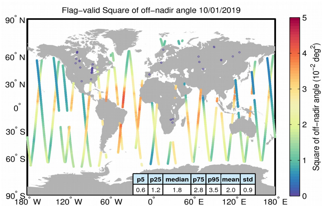
Figure 37. Geographical distribution of flag-valid mispointing data over oceans and lakes for 10/01/2019. The statistical values shown in the table refer to the mispointing in 10^{-2} deg 2 and are calculated over all measurements shown in the figure.
