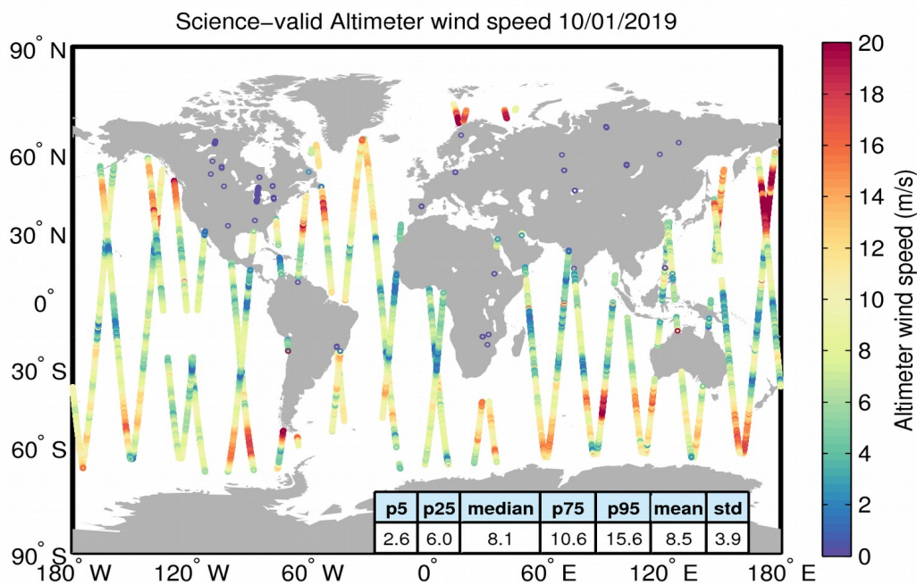
Figure 34. Geographical distribution of science-valid wind data over oceans and lakes for 10/01/2019. The statistical values shown in the table refer to the wind in m/s and are calculated over all measurements shown in the figure. Gray circles denote records that have been rejected based on the editing criteria described in Table 5.
