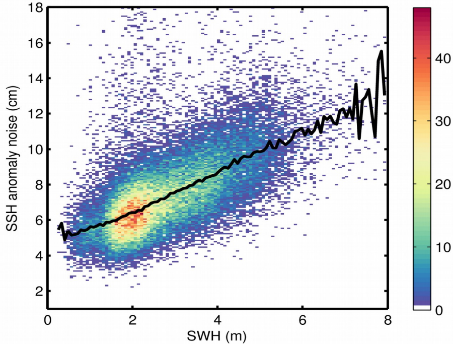
Figure 9. 2D histogram showing flag-valid SSH anomaly noise as a function of SWH for 10/01/2019. The black line denotes the median SSH anomaly noise as a function of SWH.
