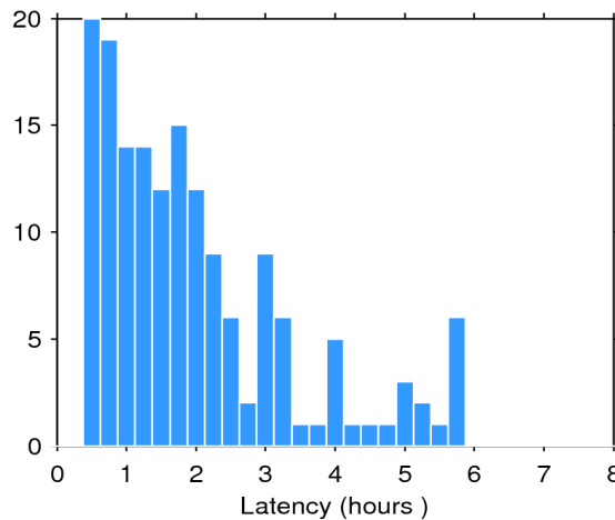
Figure 2. Histogram of the data latency for 10/01/2019. The y-axis denotes the number of files that are made available with a delay of x-hours with respect to the mean time of the records stored in the file.
