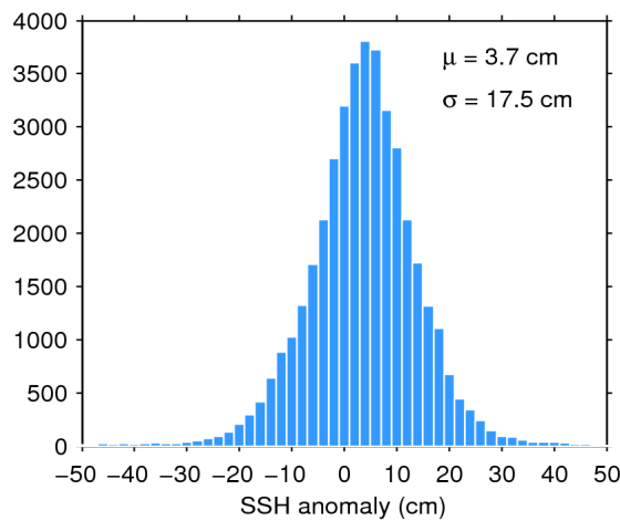
Figure 7. Histogram of flag-valid SSH anomaly over oceans and lakes for 10/01/2019. The mean ( \mu ) and standard deviation ( \sigma ) are also shown. Note that values outside [-50\ 50] cm are excluded from the histogram for the sake of readability but not from the computation of \mu and \sigma .
