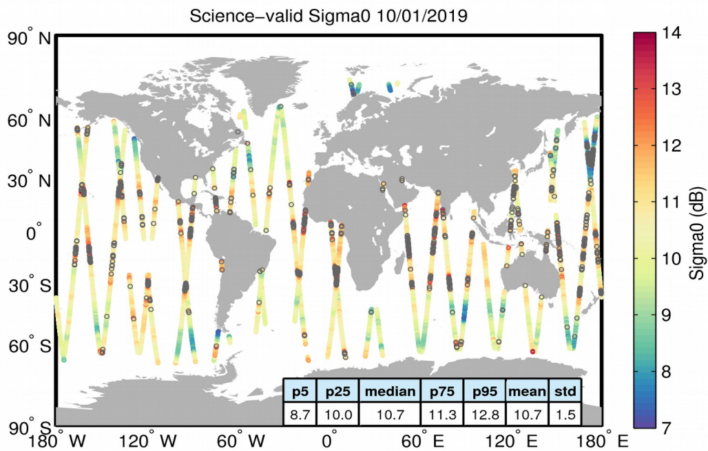
Figure 27. Geographical distribution of science-valid sigma0 data over oceans and lakes for 10/01/2019. The statistical values shown in the table refer to the sigma0 in dB and are calculated over all measurements shown in the figure. Gray circles denote records that have been rejected based on the editing criteria described in Table 4.
