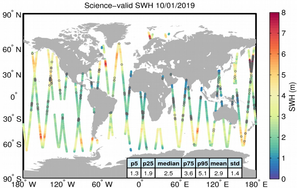
Figure 19. Geographical distribution of science-valid SWH data over oceans and lakes for 10/01/2019. The statistical values shown in the table refer to the SWH in m and are calculated over all measurements shown in the figure. Gray circles denote records that have been rejected based on the editing criteria described in Table 3.
