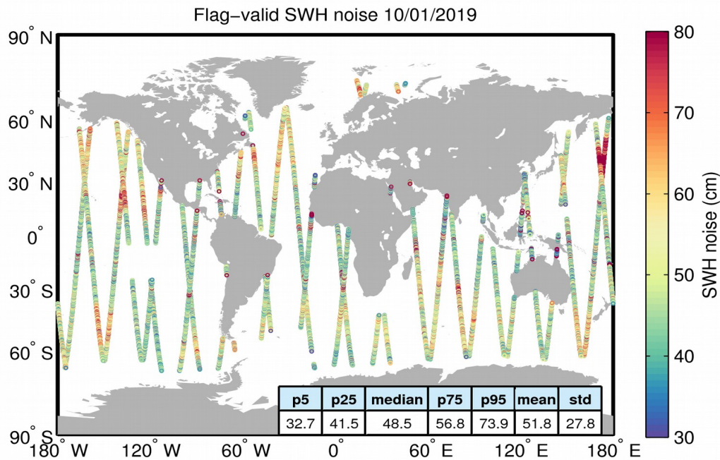
Figure 18. Geographical distribution of flag-valid 20-Hz SWH measurement noise over oceans and lakes for 10/01/2019. The statistical values shown in the figure refer to the SWH noise and are calculated over all measurements shown in the figure.
