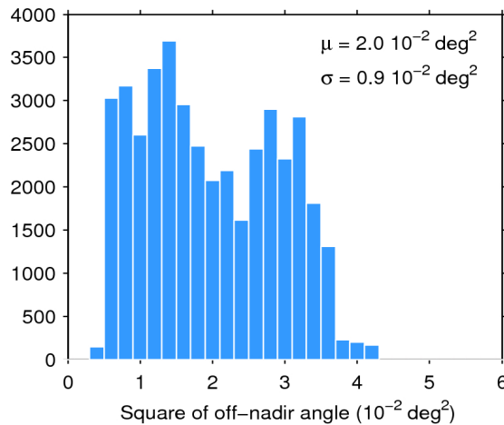
Figure 39. Histogram of flag-valid mispointing over oceans and lakes for 10/01/2019. The mean ( \mu ) and standard deviation ( \sigma ) are also shown. Note that values larger than 6 \cdot 10^{-2} \text{ deg}^2 are excluded from the histogram for the sake of readability but not from the computation of \mu and \sigma .
