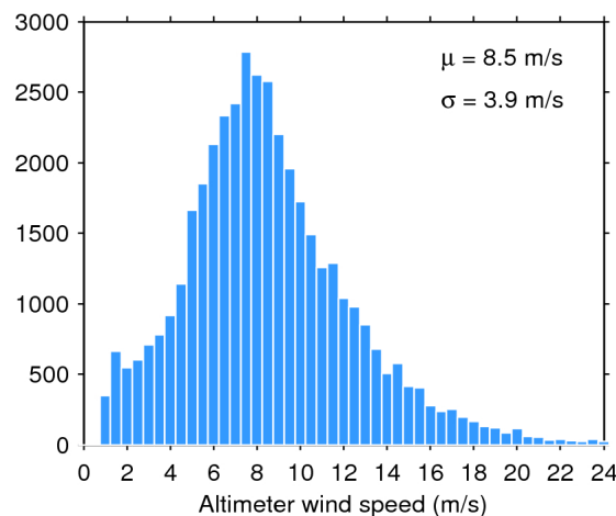
Figure 35. Histogram of science-valid wind over oceans and lakes for 10/01/2019. The mean ( \mu ) and standard deviation ( \sigma ) are also shown. Note that values larger than 24 m/s are excluded from the histogram for the sake of readability but not from the computation of \mu and \sigma .
