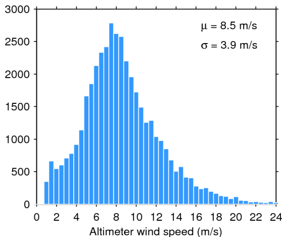
Figure 33. Histogram of flag-valid wind over oceans and lakes for 10/01/2019. The mean ( \mu ) and standard deviation ( \sigma ) are also shown. Note that values larger than 24 m/s are excluded from the histogram for the sake of readability but not from the computation of \mu and \sigma .
