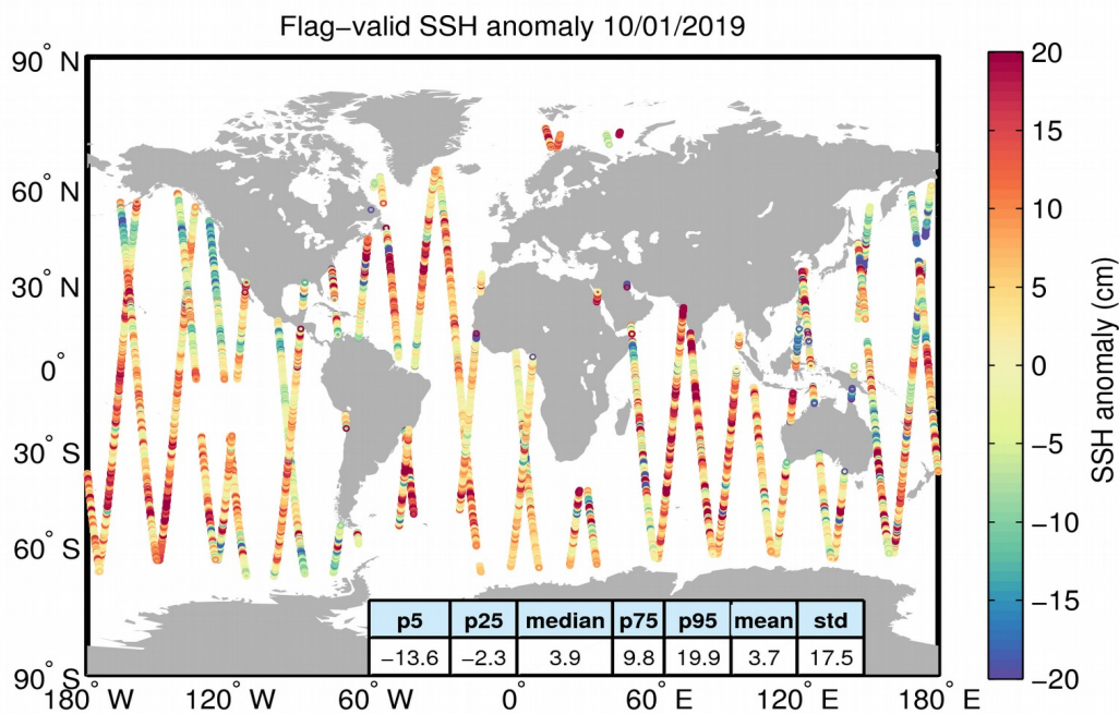
Figure 5. Geographical distribution of flag-valid 1-Hz SSH anomaly data over oceans and lakes for 10/01/2019. The statistical values shown in the table refer to the SSH anomaly in cm and are calculated over all measurements shown in the figure.
