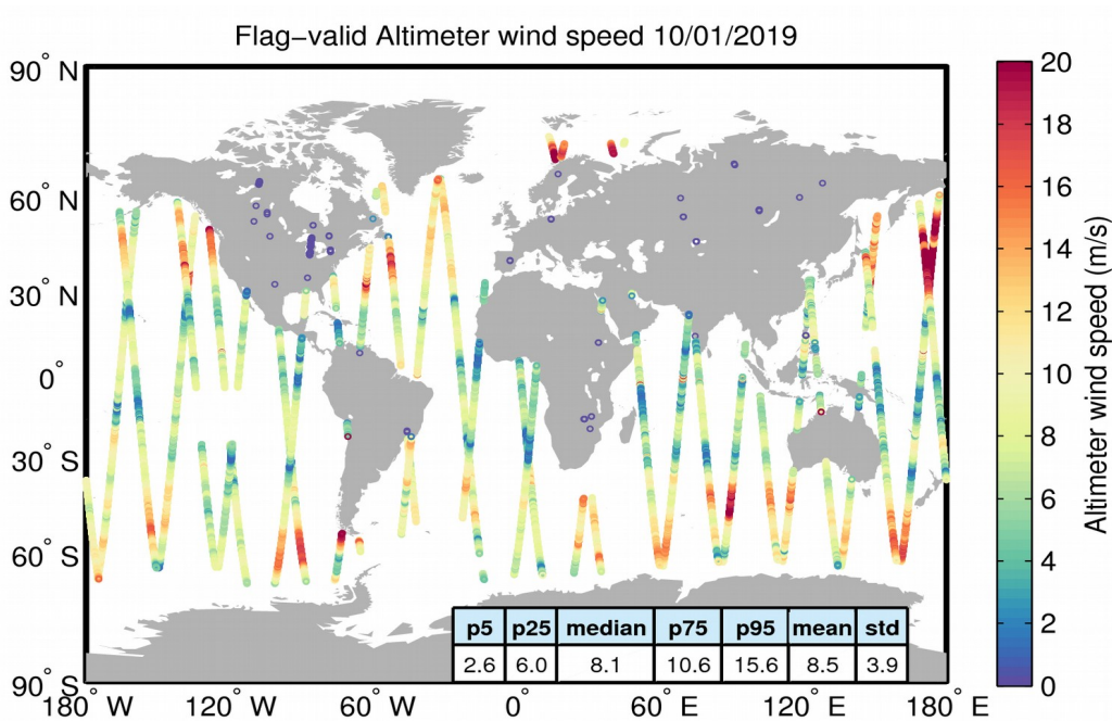
Figure 31. Geographical distribution of flag-valid wind data over oceans and lakes for 10/01/2019. The statistical values shown in the table refer to the wind in m/s and are calculated over all measurements shown in the figure.
