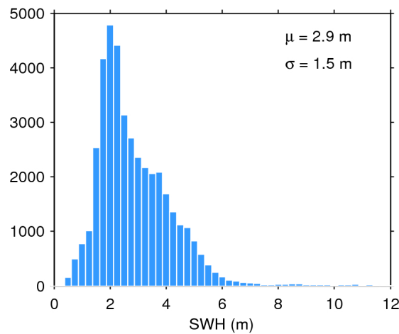
Figure 17. Histogram of flag-valid SWH over oceans and lakes for 10/01/2019. The mean ( \mu ) and standard deviation ( \sigma ) are also shown. Note that values larger than 12 m are excluded from the histogram for the sake of readability but not from the computation of \mu and \sigma .
