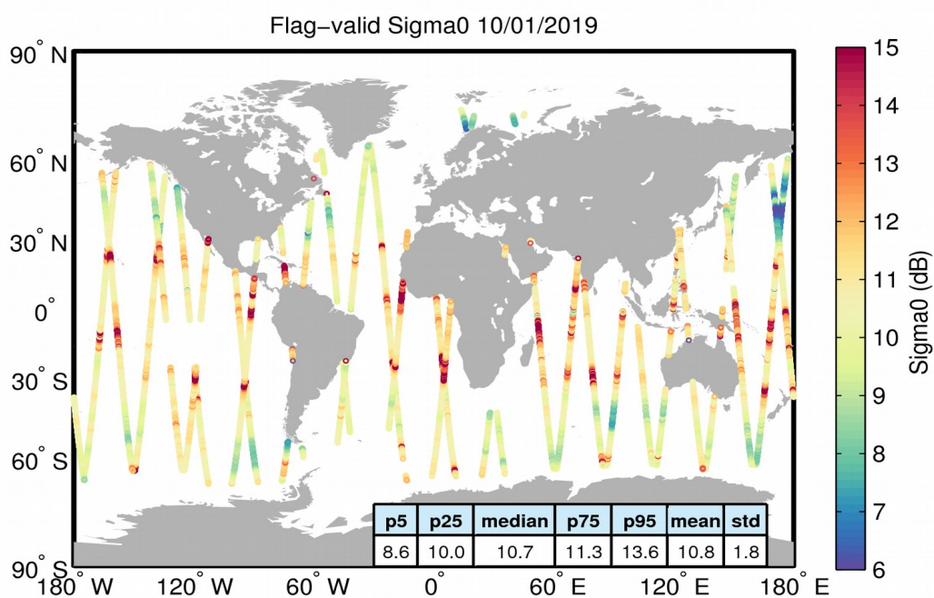
Figure 23. Geographical distribution of flag-valid sigma0 data over oceans and lakes for 10/01/2019. The statistical values shown in the table refer to the sigma0 in dB and are calculated over all measurements shown in the figure.
