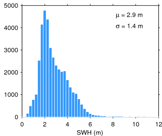
Figure 20. Histogram of science-valid SWH over oceans and lakes for 10/01/2019. The mean ( \mu ) and standard deviation ( \sigma ) are also shown. Note that values larger than 12 m are excluded from the histogram for the sake of readability but not from the computation of \mu and \sigma .
