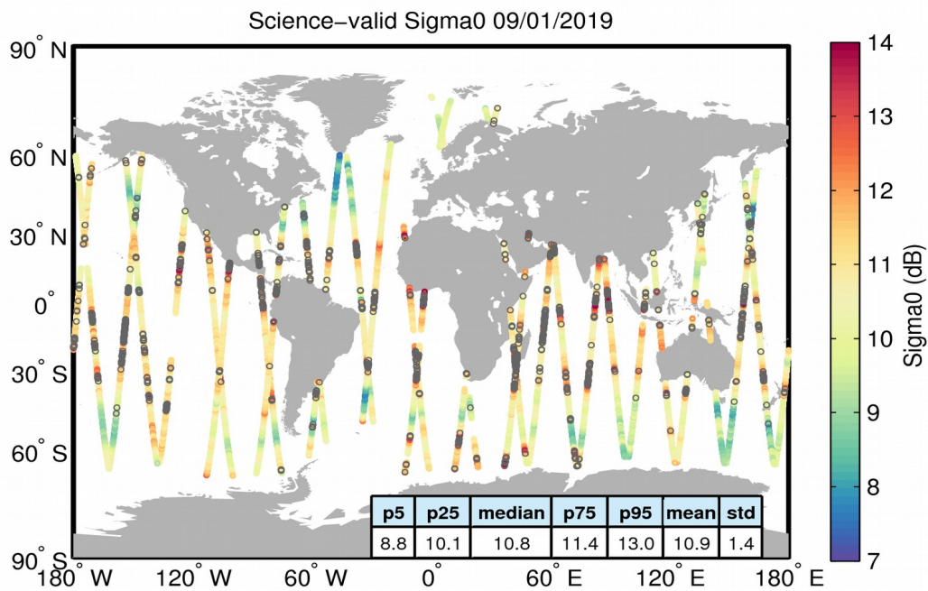
Figure 27. Geographical distribution of science-valid sigma0 data over oceans and lakes for 09/01/2019. The statistical values shown in the table refer to the sigma0 in dB and are calculated over all measurements shown in the figure. Gray circles denote records that have been rejected based on the editing criteria described in Table 4.
