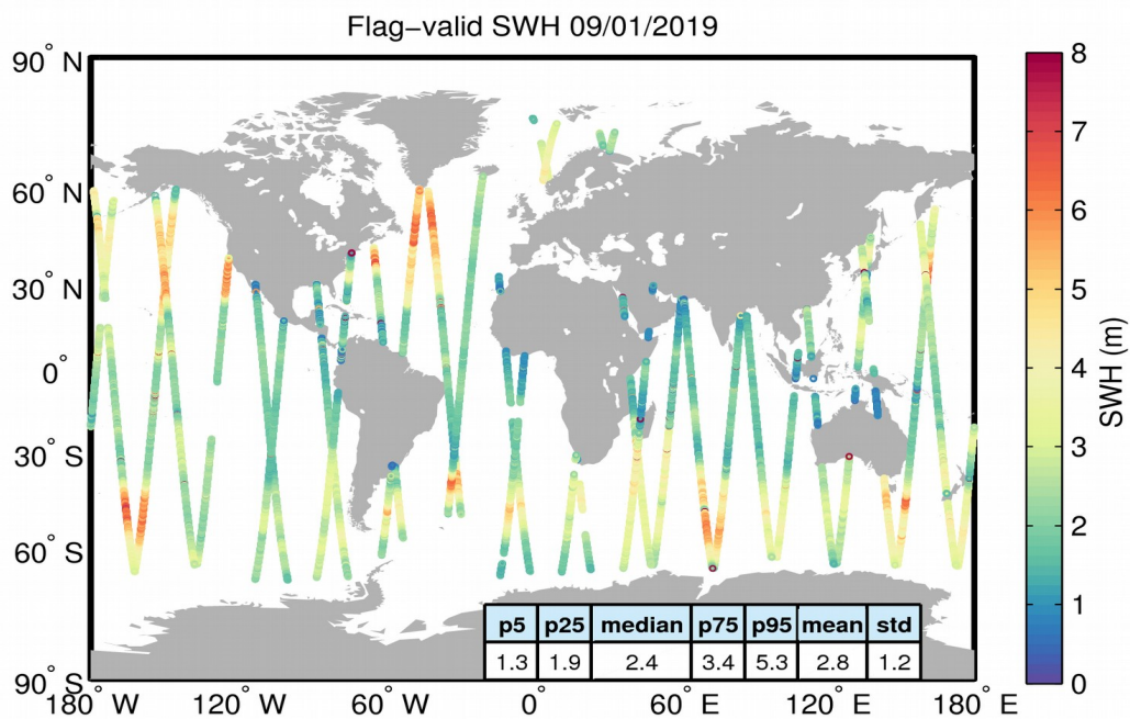
Figure 15. Geographical distribution of flag-valid SWH data over oceans and lakes for 09/01/2019. The statistical values shown in the table refer to the SWH in m and are calculated over all measurements shown in the figure.
