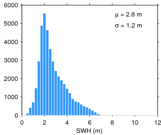
Figure 17. Histogram of flag-valid SWH over oceans and lakes for 09/01/2019. The mean ( \mu ) and standard deviation ( \sigma ) are also shown. Note that values larger than 12 m are excluded from the histogram for the sake of readability but not from the computation of \mu and \sigma .
