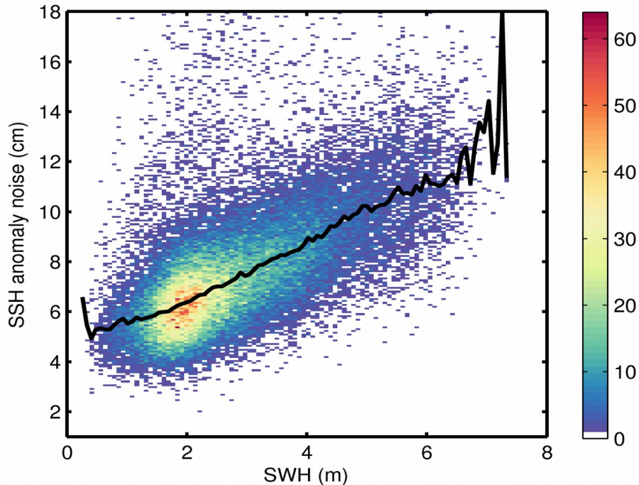
Figure 9. 2D histogram showing flag-valid SSH anomaly noise as a function of SWH for 09/01/2019. The black line denotes the median SSH anomaly noise as a function of SWH.
