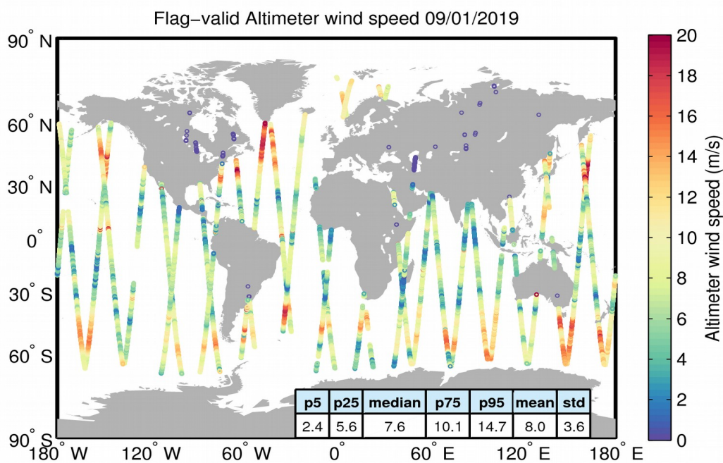
Figure 31. Geographical distribution of flag-valid wind data over oceans and lakes for 09/01/2019. The statistical values shown in the table refer to the wind in m/s and are calculated over all measurements shown in the figure.
