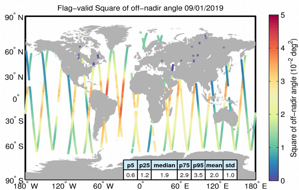
Figure 37. Geographical distribution of flag-valid mispointing data over oceans and lakes for 09/01/2019. The statistical values shown in the table refer to the mispointing in 10^{-2} \text{ deg}^2 and are calculated over all measurements shown in the figure.
