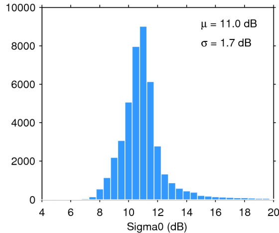
Figure 25. Histogram of flag-valid sigma0 over oceans and lakes for 09/01/2019. The mean ( \mu ) and standard deviation ( \sigma ) are also shown. Note that values outside [4 20] dB are excluded from the histogram for the sake of readability but not from the computation of \mu and \sigma .
