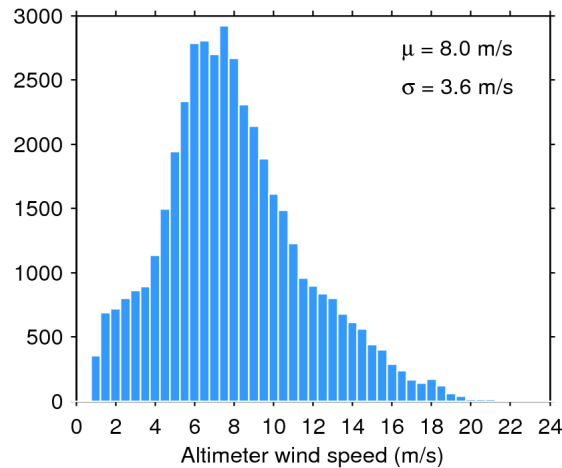
Figure 33. Histogram of flag-valid wind over oceans and lakes for 09/01/2019. The mean ( \mu ) and standard deviation ( \sigma ) are also shown. Note that values larger than 24 m/s are excluded from the histogram for the sake of readability but not from the computation of \mu and \sigma .
