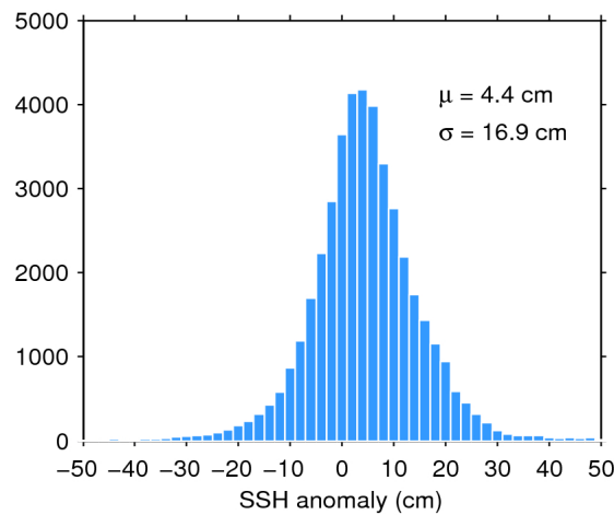
Figure 7. Histogram of flag-valid SSH anomaly over oceans and lakes for 09/01/2019. The mean ( \mu ) and standard deviation ( \sigma ) are also shown. Note that values outside [-50\ 50] cm are excluded from the histogram for the sake of readability but not from the computation of \mu and \sigma .
