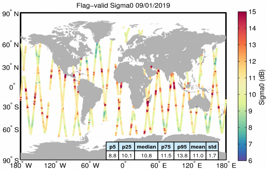
Figure 23. Geographical distribution of flag-valid sigma0 data over oceans and lakes for 09/01/2019. The statistical values shown in the table refer to the sigma0 in dB and are calculated over all measurements shown in the figure.
