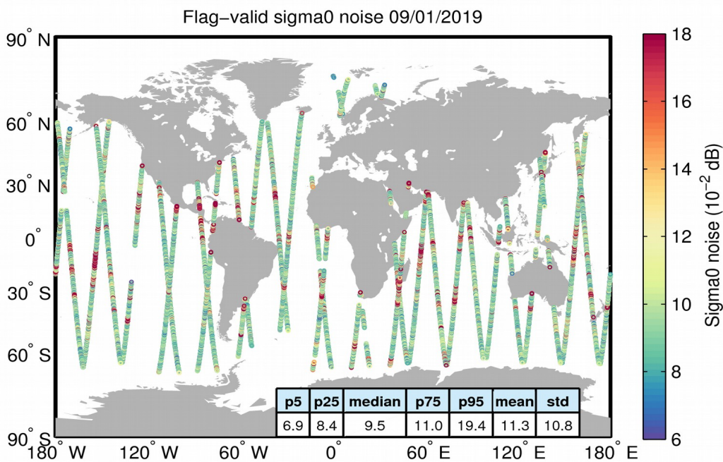
Figure 26. Geographical distribution of flag-valid 20-Hz sigma0 measurement noise over oceans and lakes for 09/01/2019. The statistical values shown in the table refer to the sigma0 noise and are calculated over all measurements shown in the figure.
