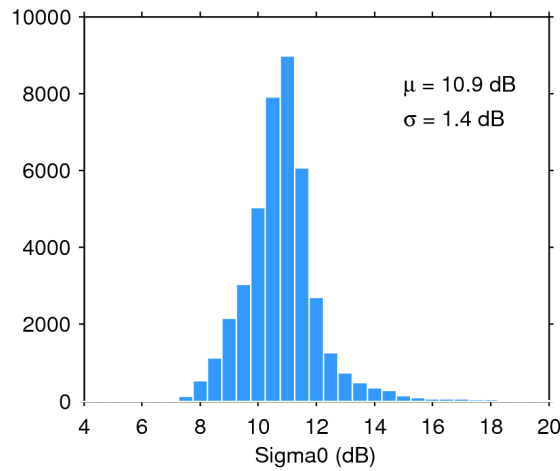
Figure 28. Histogram of science-valid sigma0 over oceans and lakes for 09/01/2019. The mean ( \mu ) and standard deviation ( \sigma ) are also shown. Note that values outside [4 20] dB are excluded from the histogram for the sake of readability but not from the computation of \mu and \sigma .
