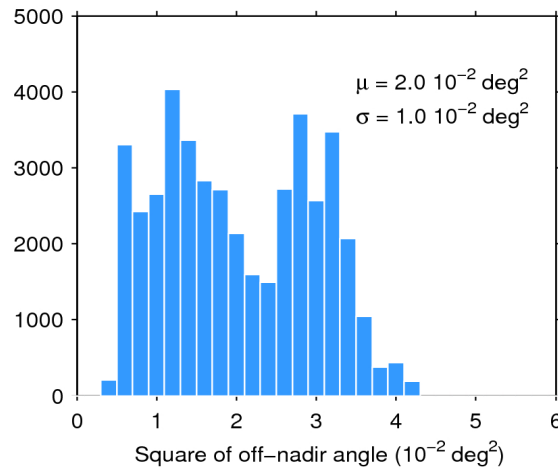
Figure 39. Histogram of flag-valid mispointing over oceans and lakes for 09/01/2019. The mean ( \mu ) and standard deviation ( \sigma ) are also shown. Note that values larger than 6 \cdot 10^{-2} \text{ deg}^2 are excluded from the histogram for the sake of readability but not from the computation of \mu and \sigma .
