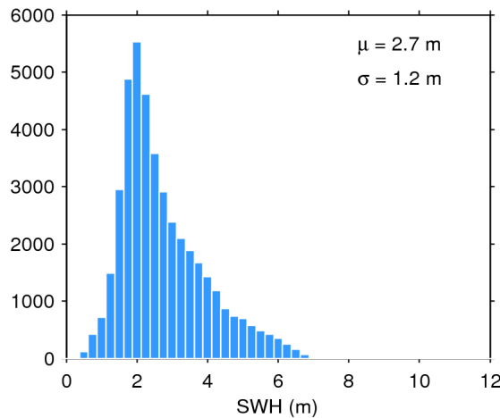
Figure 20. Histogram of science-valid SWH over oceans and lakes for 09/01/2019. The mean ( \mu ) and standard deviation ( \sigma ) are also shown. Note that values larger than 12 m are excluded from the histogram for the sake of readability but not from the computation of \mu and \sigma .
