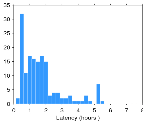
Figure 2. Histogram of the data latency for 08/01/2019. The y-axis denotes the number of files that are made available with a delay of x-hours with respect to the mean time of the records stored in the file.
