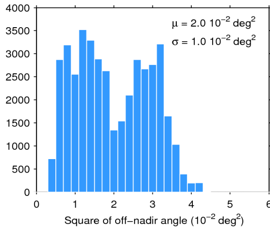
Figure 39. Histogram of flag-valid mispointing over oceans and lakes for 08/01/2019. The mean ( \mu ) and standard deviation ( \sigma ) are also shown. Note that values larger than 6 \cdot 10^{-2} \text{ deg}^2 are excluded from the histogram for the sake of readability but not from the computation of \mu and \sigma .
