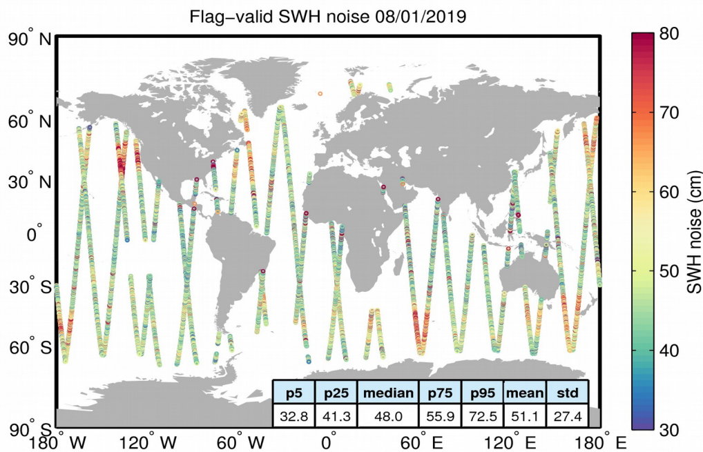
Figure 18. Geographical distribution of flag-valid 20-Hz SWH measurement noise over oceans and lakes for 08/01/2019. The statistical values shown in the figure refer to the SWH noise and are calculated over all measurements shown in the figure.
