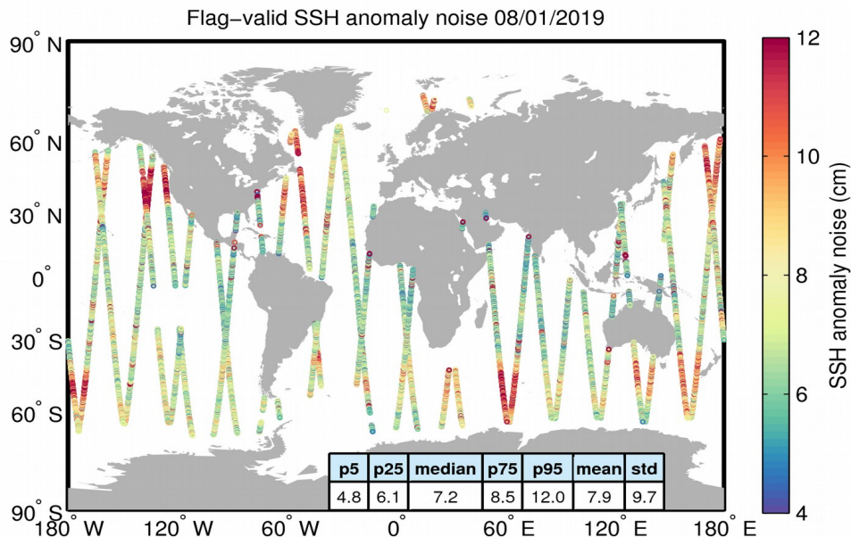
Figure 8. Geographical distribution of flag-valid 20-Hz SSH anomaly measurement noise over oceans and lakes for 08/01/2019. The statistical values shown in the table refer to the SSH anomaly noise and are calculated over all measurements shown in the figure.
