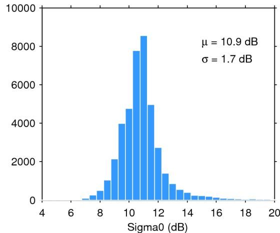
Figure 25. Histogram of flag-valid sigma0 over oceans and lakes for 08/01/2019. The mean ( \mu ) and standard deviation ( \sigma ) are also shown. Note that values outside [4 20] dB are excluded from the histogram for the sake of readability but not from the computation of \mu and \sigma .
