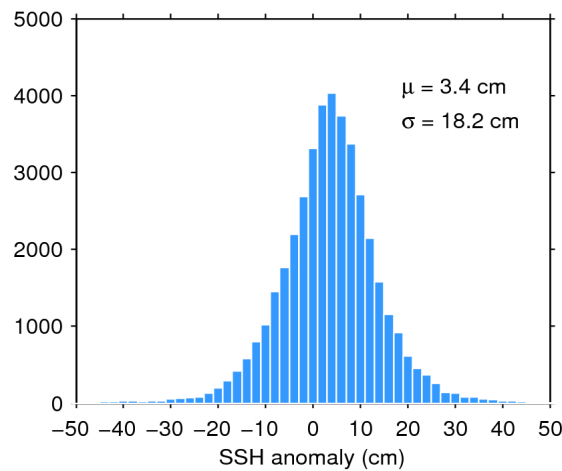
Figure 7. Histogram of flag-valid SSH anomaly over oceans and lakes for 08/01/2019. The mean ( \mu ) and standard deviation ( \sigma ) are also shown. Note that values outside [-50\ 50] cm are excluded from the histogram for the sake of readability but not from the computation of \mu and \sigma .
