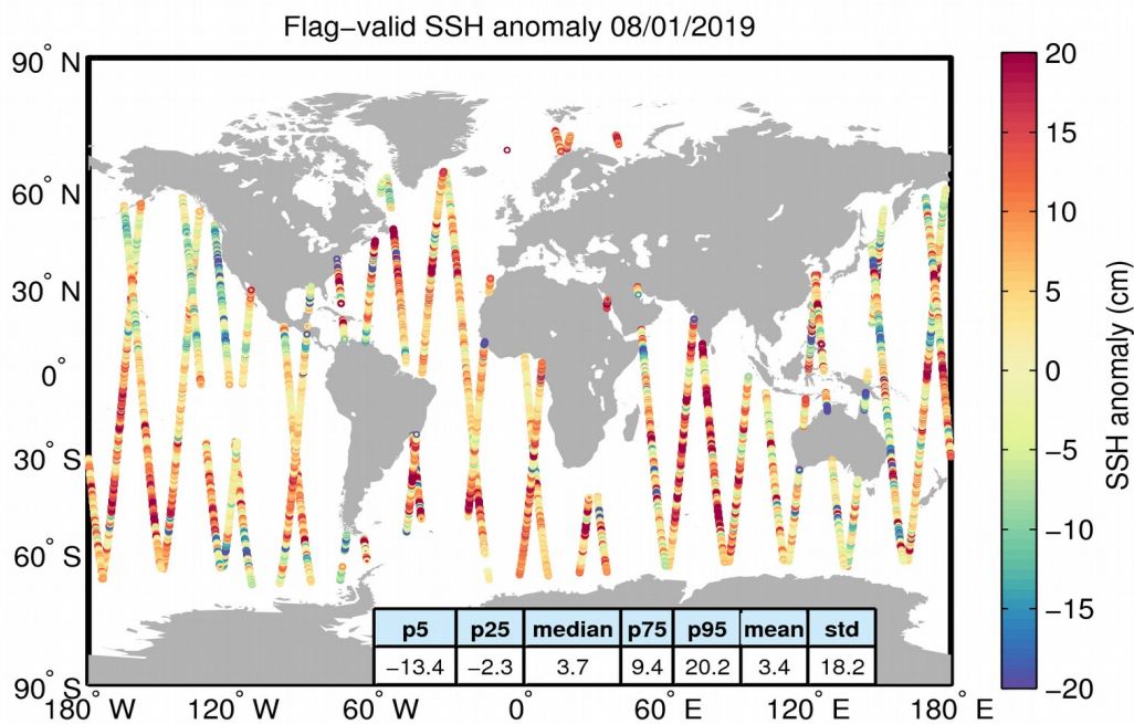
Figure 5. Geographical distribution of flag-valid 1-Hz SSH anomaly data over oceans and lakes for 08/01/2019. The statistical values shown in the table refer to the SSH anomaly in cm and are calculated over all measurements shown in the figure.
