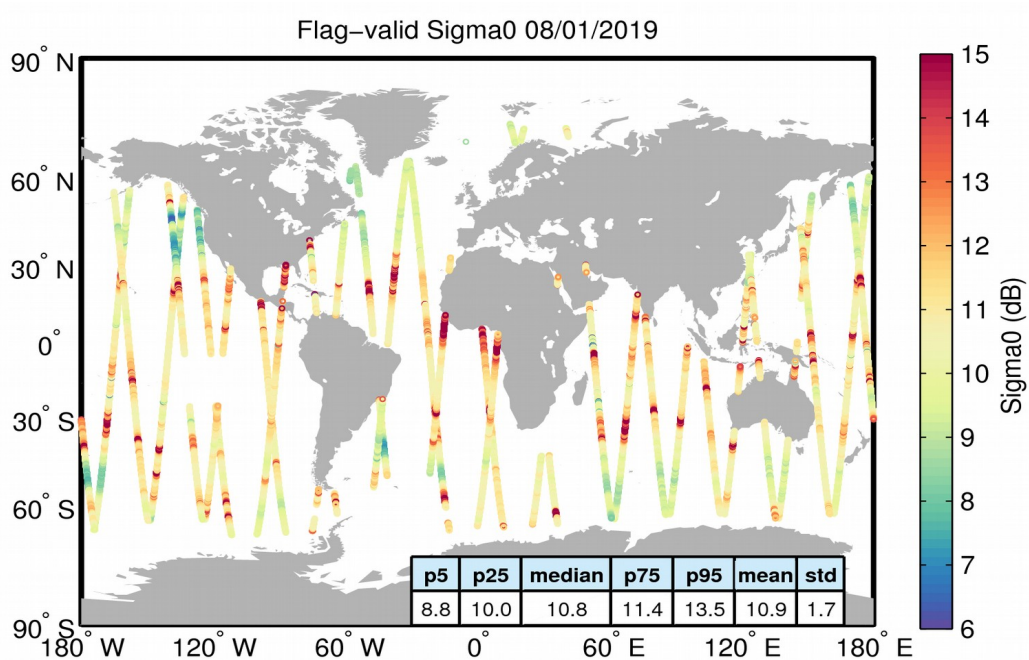
Figure 23. Geographical distribution of flag-valid sigma0 data over oceans and lakes for 08/01/2019. The statistical values shown in the table refer to the sigma0 in dB and are calculated over all measurements shown in the figure.
