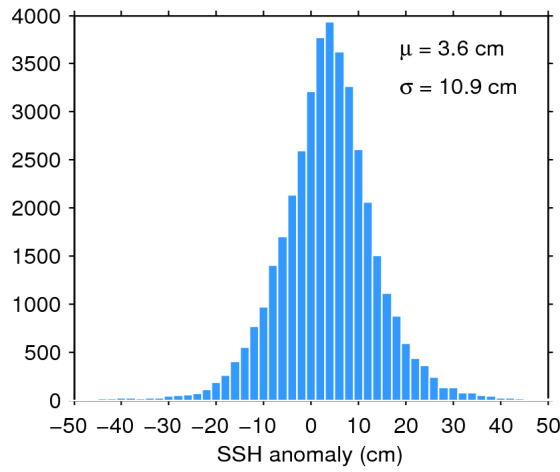
Figure 11. Histogram of science-valid SSH anomaly over oceans and lakes for 08/01/2019. The mean ( \mu ) and standard deviation ( \sigma ) are also shown. Note that values outside [-50 50] cm are excluded from the histogram for the sake of readability but not from the computation of \mu and \sigma .
