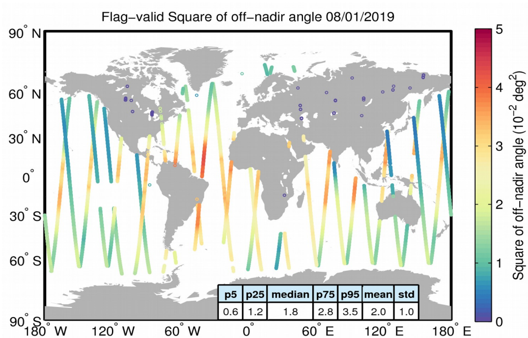
Figure 37. Geographical distribution of flag-valid mispointing data over oceans and lakes for 08/01/2019. The statistical values shown in the table refer to the mispointing in 10^{-2} \text{ deg}^2 and are calculated over all measurements shown in the figure.
