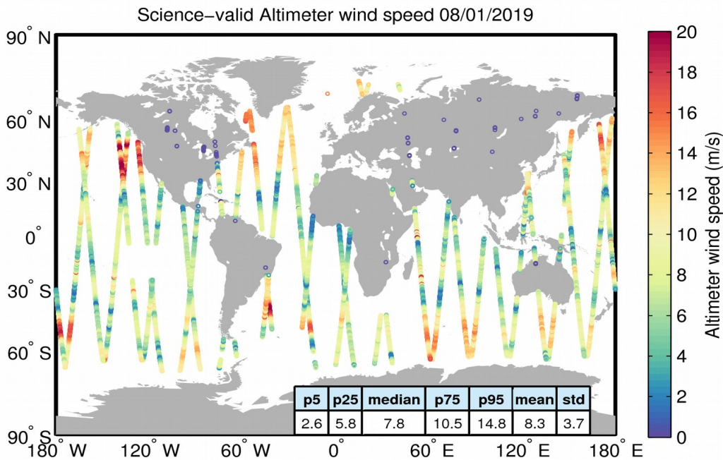
Figure 34. Geographical distribution of science-valid wind data over oceans and lakes for 08/01/2019. The statistical values shown in the table refer to the wind in m/s and are calculated over all measurements shown in the figure. Gray circles denote records that have been rejected based on the editing criteria described in Table 5.
