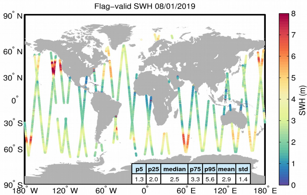
Figure 15. Geographical distribution of flag-valid SWH data over oceans and lakes for 08/01/2019. The statistical values shown in the table refer to the SWH in m and are calculated over all measurements shown in the figure.
