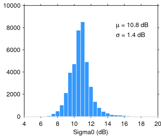
Figure 28. Histogram of science-valid sigma0 over oceans and lakes for 08/01/2019. The mean ( \mu ) and standard deviation ( \sigma ) are also shown. Note that values outside [4 20] dB are excluded from the histogram for the sake of readability but not from the computation of \mu and \sigma .
