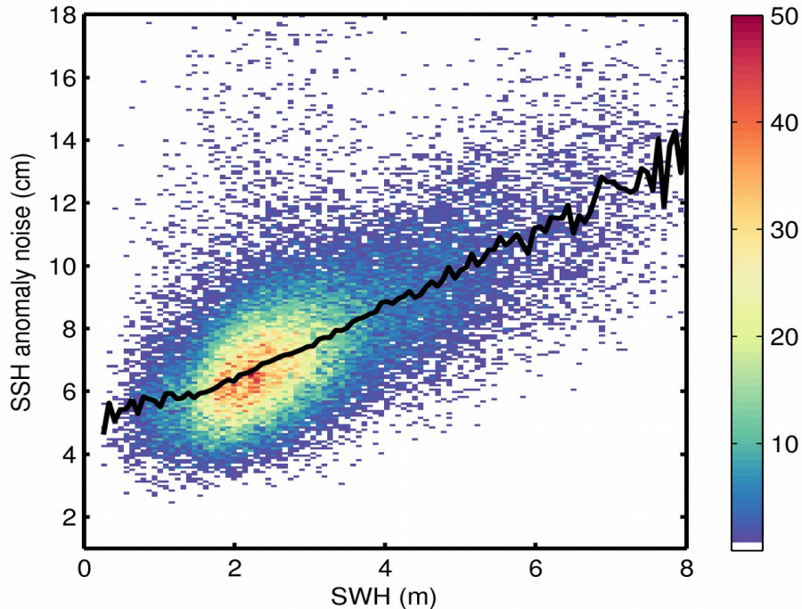
Figure 9. 2D histogram showing flag-valid SSH anomaly noise as a function of SWH for 08/01/2019. The black line denotes the median SSH anomaly noise as a function of SWH.
