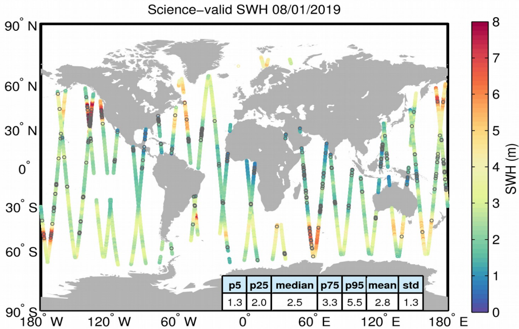
Figure 19. Geographical distribution of science-valid SWH data over oceans and lakes for 08/01/2019. The statistical values shown in the table refer to the SWH in m and are calculated over all measurements shown in the figure. Gray circles denote records that have been rejected based on the editing criteria described in Table 3.
