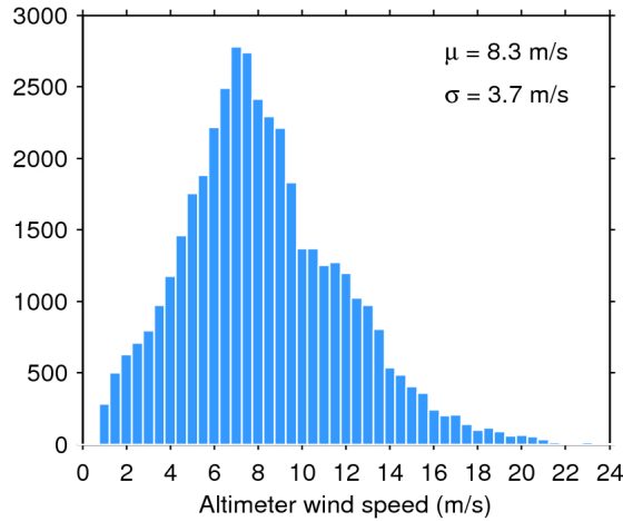
Figure 33. Histogram of flag-valid wind over oceans and lakes for 08/01/2019. The mean ( \mu ) and standard deviation ( \sigma ) are also shown. Note that values larger than 24 m/s are excluded from the histogram for the sake of readability but not from the computation of \mu and \sigma .
