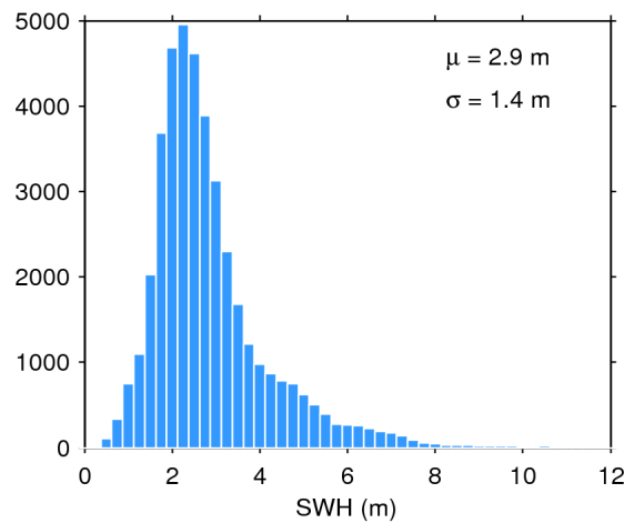
Figure 17. Histogram of flag-valid SWH over oceans and lakes for 08/01/2019. The mean ( \mu ) and standard deviation ( \sigma ) are also shown. Note that values larger than 12 m are excluded from the histogram for the sake of readability but not from the computation of \mu and \sigma .
