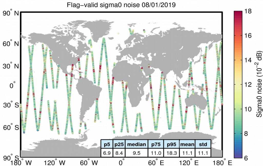
Figure 26. Geographical distribution of flag-valid 20-Hz sigma0 measurement noise over oceans and lakes for 08/01/2019. The statistical values shown in the table refer to the sigma0 noise and are calculated over all measurements shown in the figure.
