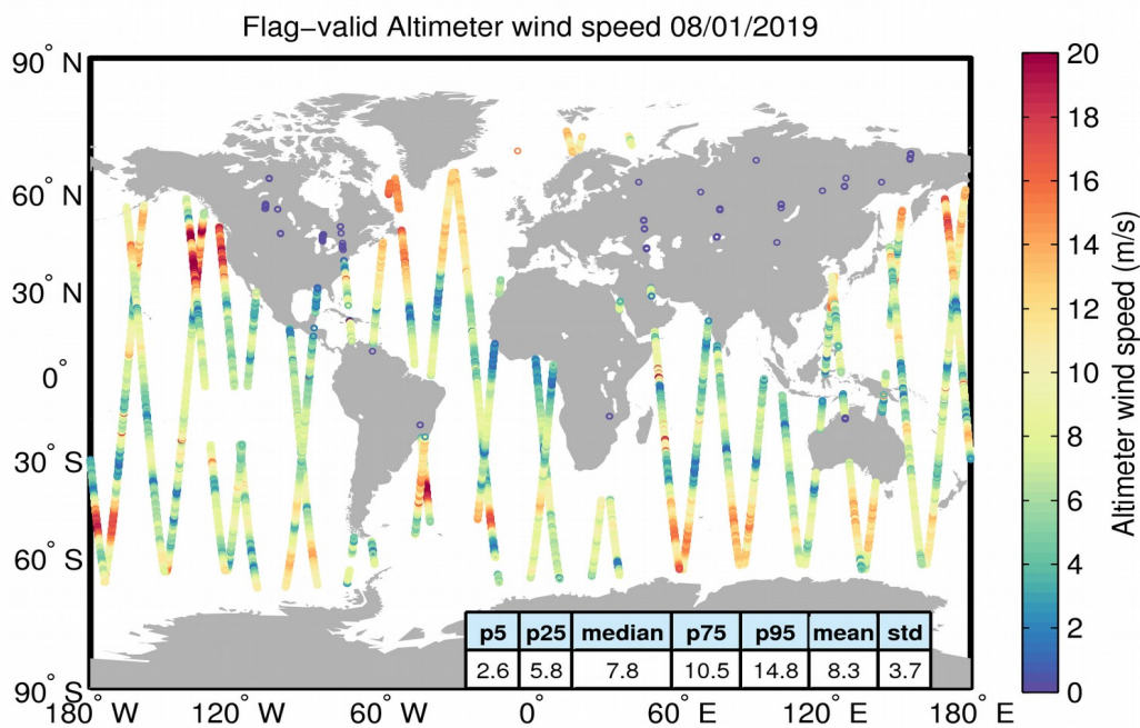
Figure 31. Geographical distribution of flag-valid wind data over oceans and lakes for 08/01/2019. The statistical values shown in the table refer to the wind in m/s and are calculated over all measurements shown in the figure.
