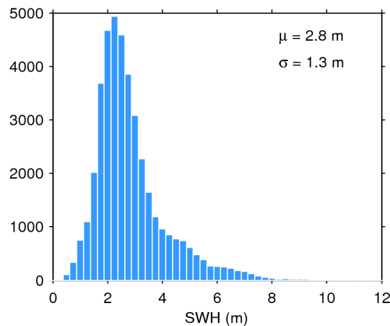
Figure 20. Histogram of science-valid SWH over oceans and lakes for 08/01/2019. The mean ( \mu ) and standard deviation ( \sigma ) are also shown. Note that values larger than 12 m are excluded from the histogram for the sake of readability but not from the computation of \mu and \sigma .
