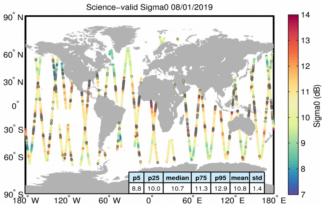
Figure 27. Geographical distribution of science-valid sigma0 data over oceans and lakes for 08/01/2019. The statistical values shown in the table refer to the sigma0 in dB and are calculated over all measurements shown in the figure. Gray circles denote records that have been rejected based on the editing criteria described in Table 4.
