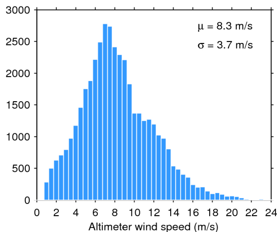
Figure 35. Histogram of science-valid wind over oceans and lakes for 08/01/2019. The mean ( \mu ) and standard deviation ( \sigma ) are also shown. Note that values larger than 24 m/s are excluded from the histogram for the sake of readability but not from the computation of \mu and \sigma .
