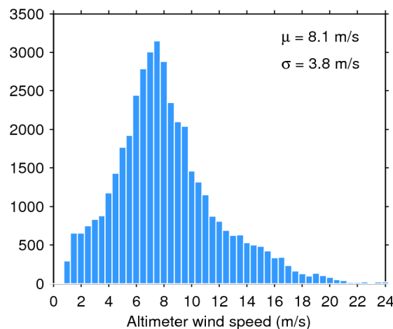
Figure 35. Histogram of science-valid wind over oceans and lakes for 07/01/2019. The mean ( \mu ) and standard deviation ( \sigma ) are also shown. Note that values larger than 24 m/s are excluded from the histogram for the sake of readability but not from the computation of \mu and \sigma .
