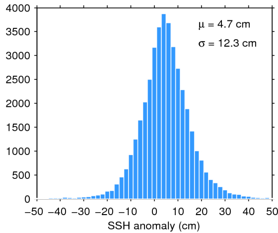
Figure 11. Histogram of science-valid SSH anomaly over oceans and lakes for 07/01/2019. The mean ( \mu ) and standard deviation ( \sigma ) are also shown. Note that values outside [-50 50] cm are excluded from the histogram for the sake of readability but not from the computation of \mu and \sigma .
