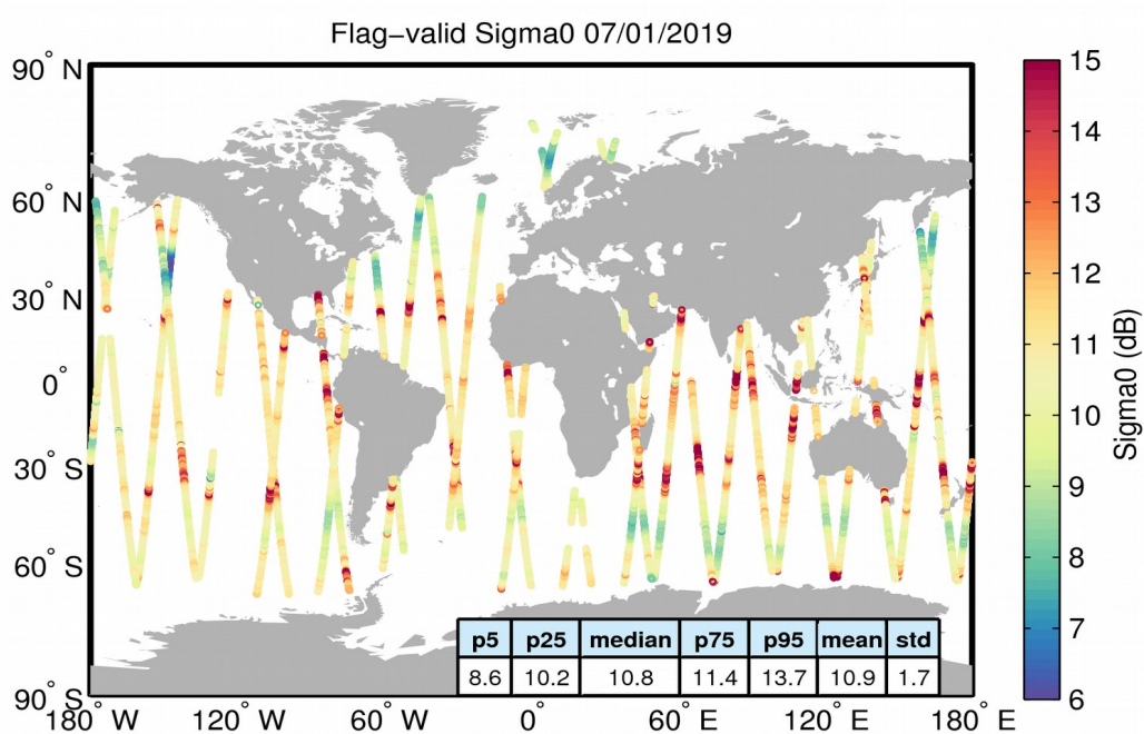
Figure 23. Geographical distribution of flag-valid sigma0 data over oceans and lakes for 07/01/2019. The statistical values shown in the table refer to the sigma0 in dB and are calculated over all measurements shown in the figure.
