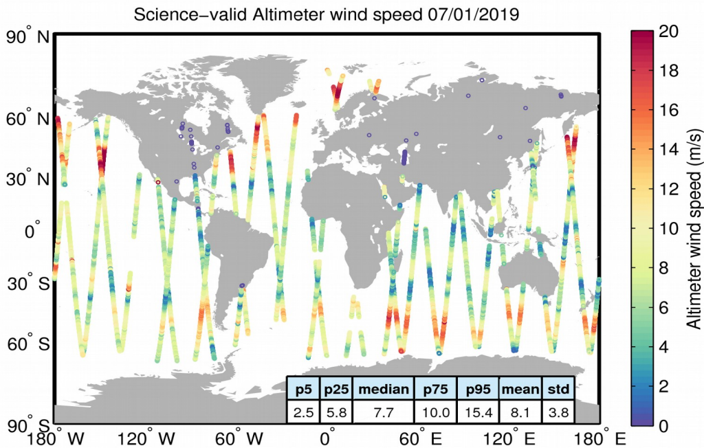
Figure 34. Geographical distribution of science-valid wind data over oceans and lakes for 07/01/2019. The statistical values shown in the table refer to the wind in m/s and are calculated over all measurements shown in the figure. Gray circles denote records that have been rejected based on the editing criteria described in Table 5.
