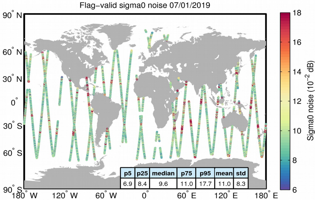
Figure 26. Geographical distribution of flag-valid 20-Hz sigma0 measurement noise over oceans and lakes for 07/01/2019. The statistical values shown in the table refer to the sigma0 noise and are calculated over all measurements shown in the figure.
