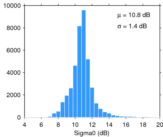
Figure 28. Histogram of science-valid sigma0 over oceans and lakes for 07/01/2019. The mean ( \mu ) and standard deviation ( \sigma ) are also shown. Note that values outside [4 20] dB are excluded from the histogram for the sake of readability but not from the computation of \mu and \sigma .
