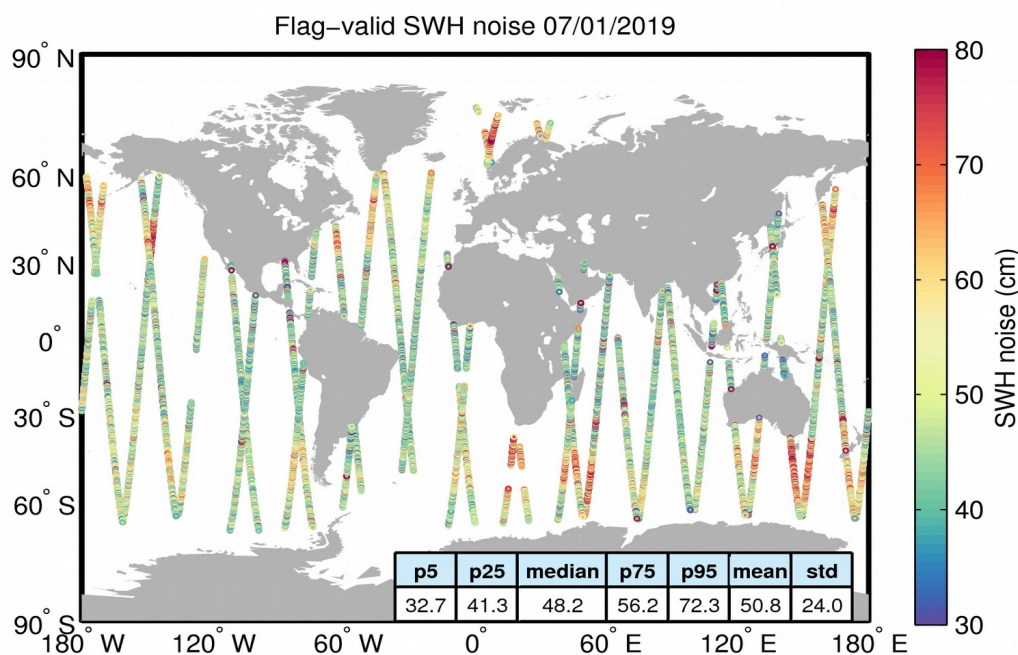
Figure 18. Geographical distribution of flag-valid 20-Hz SWH measurement noise over oceans and lakes for 07/01/2019. The statistical values shown in the figure refer to the SWH noise and are calculated over all measurements shown in the figure.
