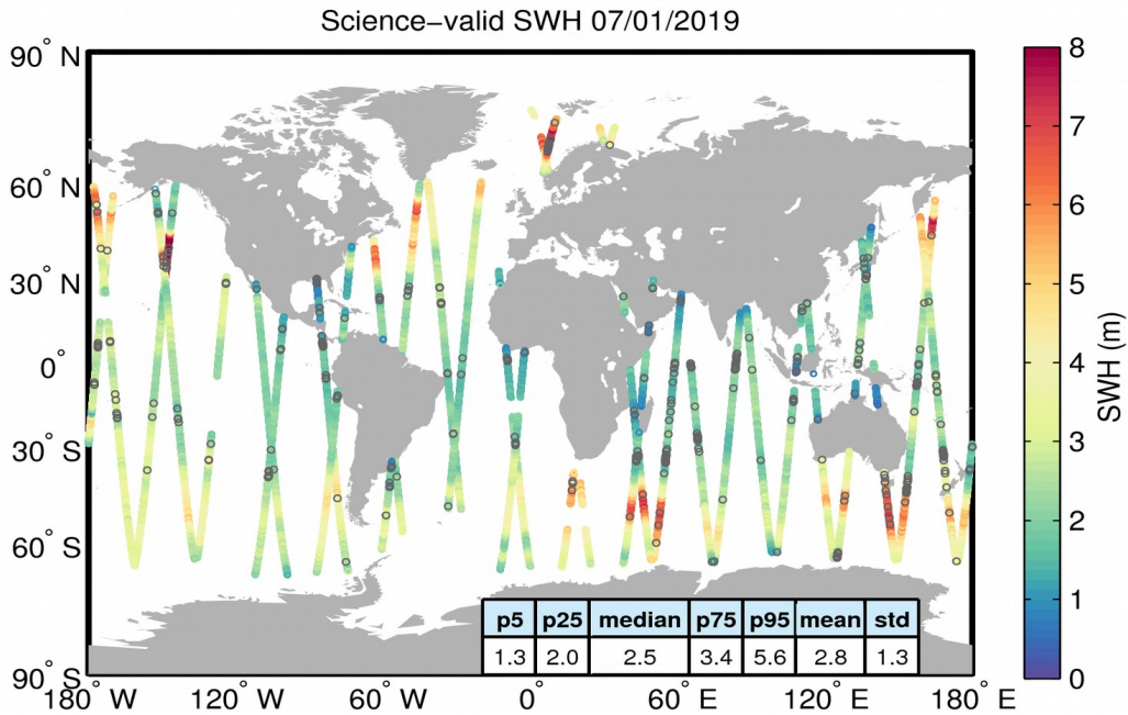
Figure 19. Geographical distribution of science-valid SWH data over oceans and lakes for 07/01/2019. The statistical values shown in the table refer to the SWH in m and are calculated over all measurements shown in the figure. Gray circles denote records that have been rejected based on the editing criteria described in Table 3.
