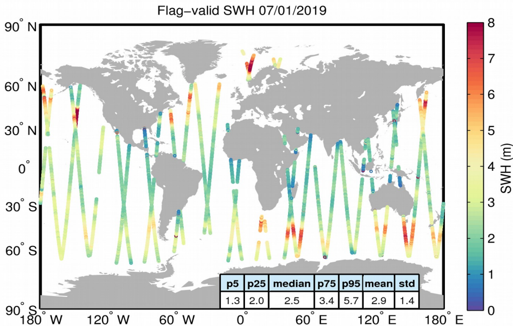
Figure 15. Geographical distribution of flag-valid SWH data over oceans and lakes for 07/01/2019. The statistical values shown in the table refer to the SWH in m and are calculated over all measurements shown in the figure.
