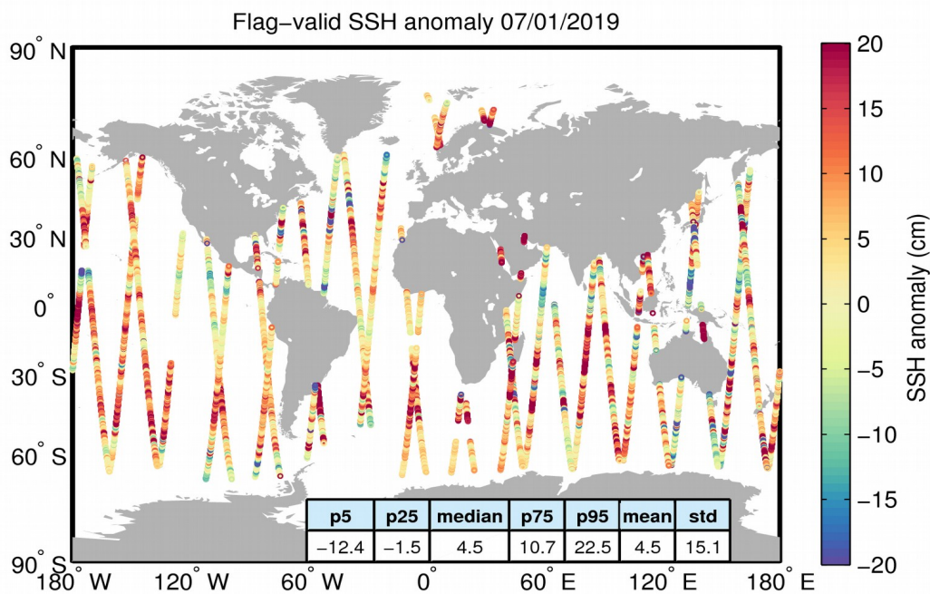
Figure 5. Geographical distribution of flag-valid 1-Hz SSH anomaly data over oceans and lakes for 07/01/2019. The statistical values shown in the table refer to the SSH anomaly in cm and are calculated over all measurements shown in the figure.
