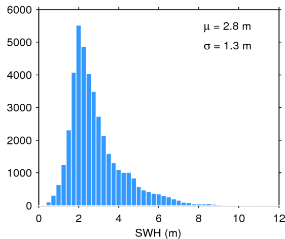
Figure 20. Histogram of science-valid SWH over oceans and lakes for 07/01/2019. The mean ( \mu ) and standard deviation ( \sigma ) are also shown. Note that values larger than 12 m are excluded from the histogram for the sake of readability but not from the computation of \mu and \sigma .
