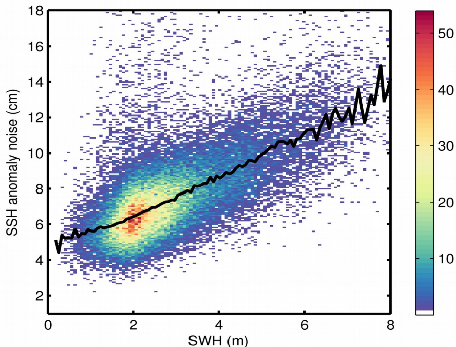
Figure 9. 2D histogram showing flag-valid SSH anomaly noise as a function of SWH for 07/01/2019. The black line denotes the median SSH anomaly noise as a function of SWH.
