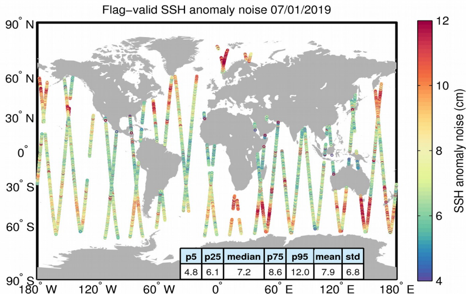
Figure 8. Geographical distribution of flag-valid 20-Hz SSH anomaly measurement noise over oceans and lakes for 07/01/2019. The statistical values shown in the table refer to the SSH anomaly noise and are calculated over all measurements shown in the figure.
