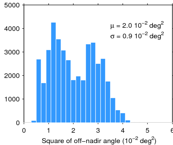
Figure 39. Histogram of flag-valid mispointing over oceans and lakes for 07/01/2019. The mean ( \mu ) and standard deviation ( \sigma ) are also shown. Note that values larger than 6 \cdot 10^{-2} \text{ deg}^2 are excluded from the histogram for the sake of readability but not from the computation of \mu and \sigma .
