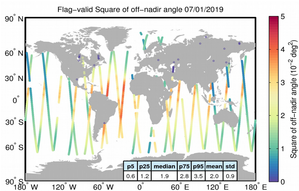
Figure 37. Geographical distribution of flag-valid mispointing data over oceans and lakes for 07/01/2019. The statistical values shown in the table refer to the mispointing in 10^{-2} \text{deg}^2 and are calculated over all measurements shown in the figure.
