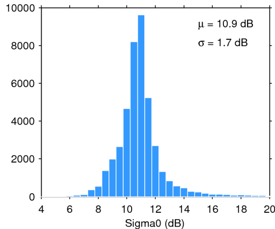
Figure 25. Histogram of flag-valid sigma0 over oceans and lakes for 07/01/2019. The mean ( \mu ) and standard deviation ( \sigma ) are also shown. Note that values outside [4 20] dB are excluded from the histogram for the sake of readability but not from the computation of \mu and \sigma .
