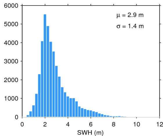
Figure 17. Histogram of flag-valid SWH over oceans and lakes for 07/01/2019. The mean ( \mu ) and standard deviation ( \sigma ) are also shown. Note that values larger than 12 m are excluded from the histogram for the sake of readability but not from the computation of \mu and \sigma .
