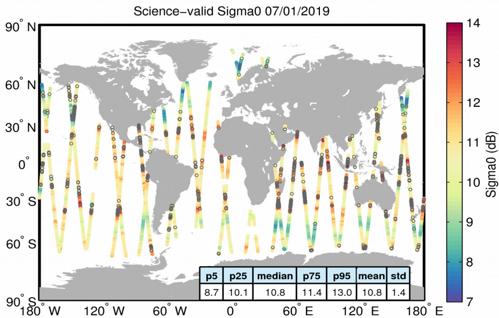
Figure 27. Geographical distribution of science-valid sigma0 data over oceans and lakes for 07/01/2019. The statistical values shown in the table refer to the sigma0 in dB and are calculated over all measurements shown in the figure. Gray circles denote records that have been rejected based on the editing criteria described in Table 4.
