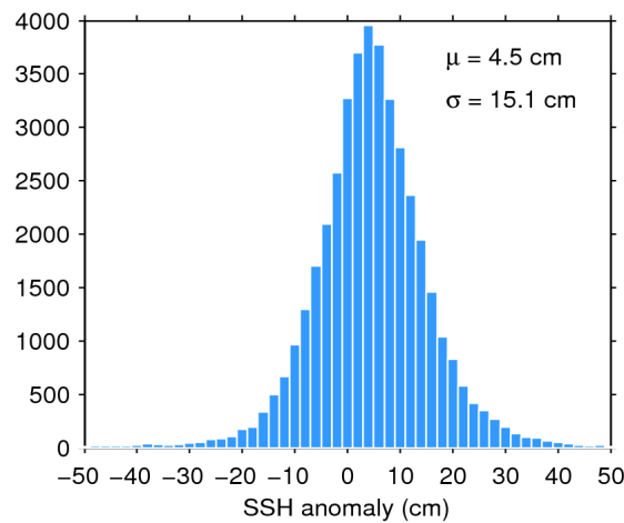
Figure 7. Histogram of flag-valid SSH anomaly over oceans and lakes for 07/01/2019. The mean ( \mu ) and standard deviation ( \sigma ) are also shown. Note that values outside [-50 50] cm are excluded from the histogram for the sake of readability but not from the computation of \mu and \sigma .
