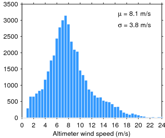
Figure 33. Histogram of flag-valid wind over oceans and lakes for 07/01/2019. The mean ( \mu ) and standard deviation ( \sigma ) are also shown. Note that values larger than 24 m/s are excluded from the histogram for the sake of readability but not from the computation of \mu and \sigma .
