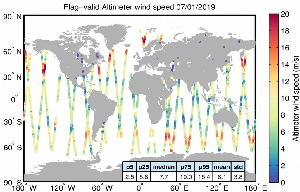
Figure 31. Geographical distribution of flag-valid wind data over oceans and lakes for 07/01/2019. The statistical values shown in the table refer to the wind in m/s and are calculated over all measurements shown in the figure.
