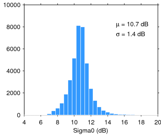
Figure 28. Histogram of science-valid sigma0 over oceans and lakes for 06/01/2019. The mean ( \mu ) and standard deviation ( \sigma ) are also shown. Note that values outside [4 20] dB are excluded from the histogram for the sake of readability but not from the computation of \mu and \sigma .
