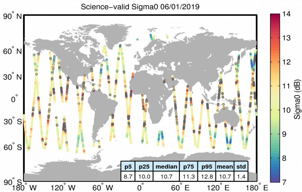
Figure 27. Geographical distribution of science-valid sigma0 data over oceans and lakes for 06/01/2019. The statistical values shown in the table refer to the sigma0 in dB and are calculated over all measurements shown in the figure. Gray circles denote records that have been rejected based on the editing criteria described in Table 4.
