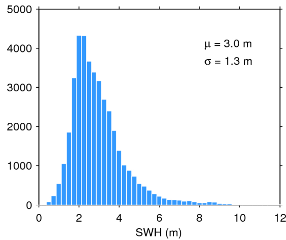
Figure 17. Histogram of flag-valid SWH over oceans and lakes for 06/01/2019. The mean ( \mu ) and standard deviation ( \sigma ) are also shown. Note that values larger than 12 m are excluded from the histogram for the sake of readability but not from the computation of \mu and \sigma .
