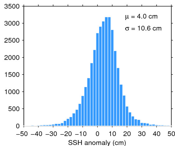
Figure 11. Histogram of science-valid SSH anomaly over oceans and lakes for 06/01/2019. The mean ( \mu ) and standard deviation ( \sigma ) are also shown. Note that values outside [-50 50] cm are excluded from the histogram for the sake of readability but not from the computation of \mu and \sigma .
