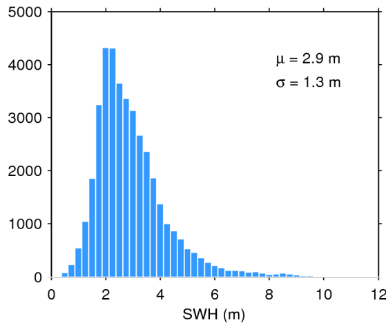
Figure 20. Histogram of science-valid SWH over oceans and lakes for 06/01/2019. The mean ( \mu ) and standard deviation ( \sigma ) are also shown. Note that values larger than 12 m are excluded from the histogram for the sake of readability but not from the computation of \mu and \sigma .
