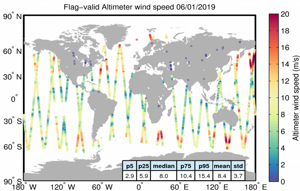
Figure 31. Geographical distribution of flag-valid wind data over oceans and lakes for 06/01/2019. The statistical values shown in the table refer to the wind in m/s and are calculated over all measurements shown in the figure.
