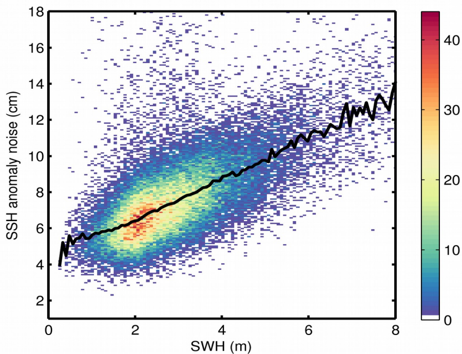
Figure 9. 2D histogram showing flag-valid SSH anomaly noise as a function of SWH for 06/01/2019. The black line denotes the median SSH anomaly noise as a function of SWH.
