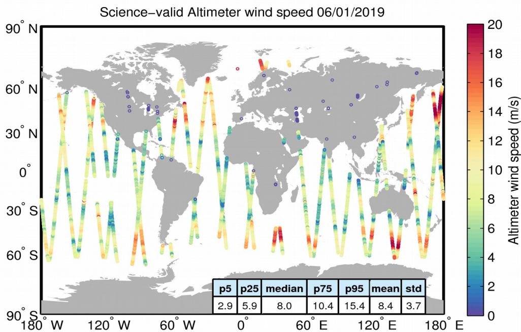
Figure 34. Geographical distribution of science-valid wind data over oceans and lakes for 06/01/2019. The statistical values shown in the table refer to the wind in m/s and are calculated over all measurements shown in the figure. Gray circles denote records that have been rejected based on the editing criteria described in Table 5.
