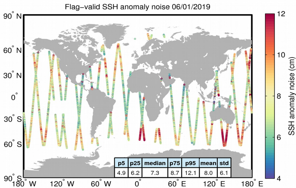
Figure 8. Geographical distribution of flag-valid 20-Hz SSH anomaly measurement noise over oceans and lakes for 06/01/2019. The statistical values shown in the table refer to the SSH anomaly noise and are calculated over all measurements shown in the figure.
