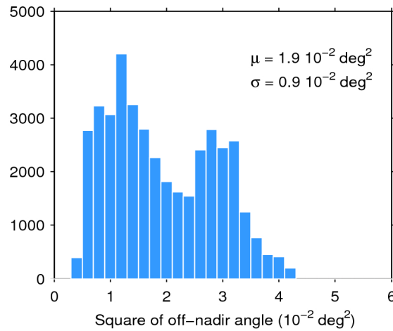
Figure 39. Histogram of flag-valid mispointing over oceans and lakes for 06/01/2019. The mean ( \mu ) and standard deviation ( \sigma ) are also shown. Note that values larger than 6 \cdot 10^{-2} \text{ deg}^2 are excluded from the histogram for the sake of readability but not from the computation of \mu and \sigma .
