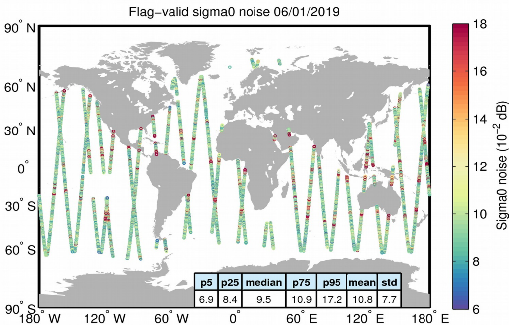
Figure 26. Geographical distribution of flag-valid 20-Hz sigma0 measurement noise over oceans and lakes for 06/01/2019. The statistical values shown in the table refer to the sigma0 noise and are calculated over all measurements shown in the figure.
