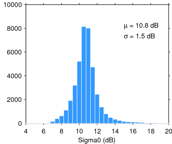
Figure 25. Histogram of flag-valid sigma0 over oceans and lakes for 06/01/2019. The mean ( \mu ) and standard deviation ( \sigma ) are also shown. Note that values outside [4 20] dB are excluded from the histogram for the sake of readability but not from the computation of \mu and \sigma .
