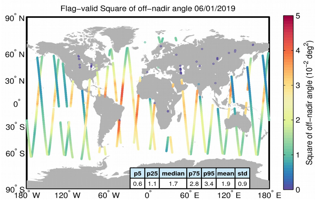
Figure 37. Geographical distribution of flag-valid mispointing data over oceans and lakes for 06/01/2019. The statistical values shown in the table refer to the mispointing in 10^{-2} deg 2 and are calculated over all measurements shown in the figure.
