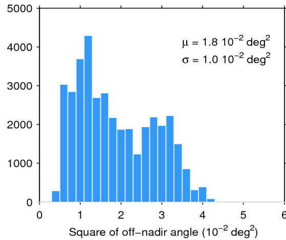
Figure 39. Histogram of flag-valid mispointing over oceans and lakes for 04/01/2019. The mean ( \mu ) and standard deviation ( \sigma ) are also shown. Note that values larger than 6 \cdot 10^{-2} \text{ deg}^2 are excluded from the histogram for the sake of readability but not from the computation of \mu and \sigma .
