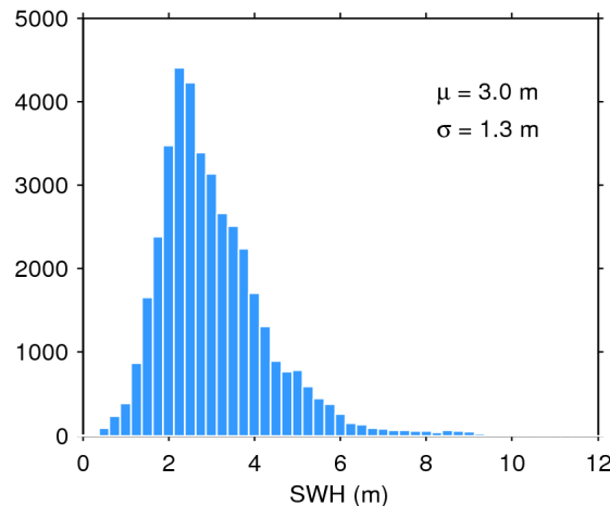
Figure 20. Histogram of science-valid SWH over oceans and lakes for 04/01/2019. The mean ( \mu ) and standard deviation ( \sigma ) are also shown. Note that values larger than 12 m are excluded from the histogram for the sake of readability but not from the computation of \mu and \sigma .
