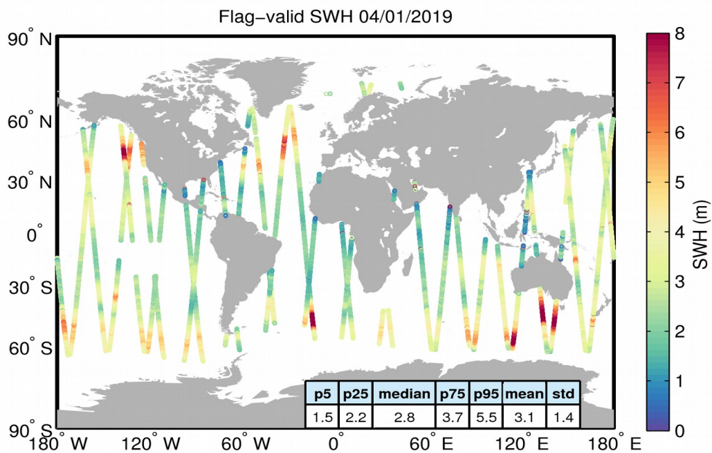
Figure 15. Geographical distribution of flag-valid SWH data over oceans and lakes for 04/01/2019. The statistical values shown in the table refer to the SWH in m and are calculated over all measurements shown in the figure.
