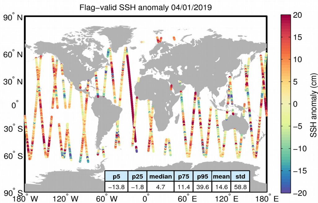
Figure 5. Geographical distribution of flag-valid 1-Hz SSH anomaly data over oceans and lakes for 04/01/2019. The statistical values shown in the table refer to the SSH anomaly in cm and are calculated over all measurements shown in the figure.
