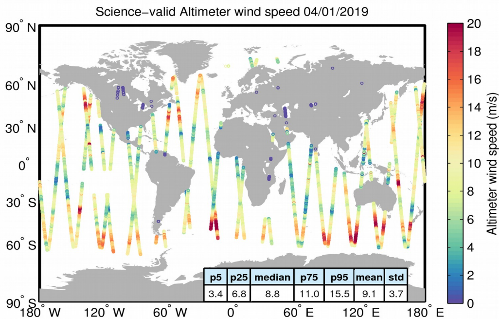
Figure 34. Geographical distribution of science-valid wind data over oceans and lakes for 04/01/2019. The statistical values shown in the table refer to the wind in m/s and are calculated over all measurements shown in the figure. Gray circles denote records that have been rejected based on the editing criteria described in Table 5.
