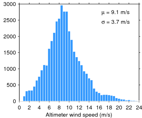
Figure 33. Histogram of flag-valid wind over oceans and lakes for 04/01/2019. The mean ( \mu ) and standard deviation ( \sigma ) are also shown. Note that values larger than 24 m/s are excluded from the histogram for the sake of readability but not from the computation of \mu and \sigma .
