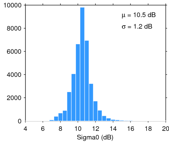
Figure 28. Histogram of science-valid sigma0 over oceans and lakes for 04/01/2019. The mean ( \mu ) and standard deviation ( \sigma ) are also shown. Note that values outside [4 20] dB are excluded from the histogram for the sake of readability but not from the computation of \mu and \sigma .
