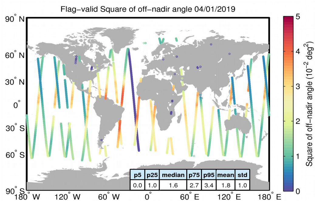
Figure 37. Geographical distribution of flag-valid mispointing data over oceans and lakes for 04/01/2019. The statistical values shown in the table refer to the mispointing in 10^{-2} deg 2 and are calculated over all measurements shown in the figure.
