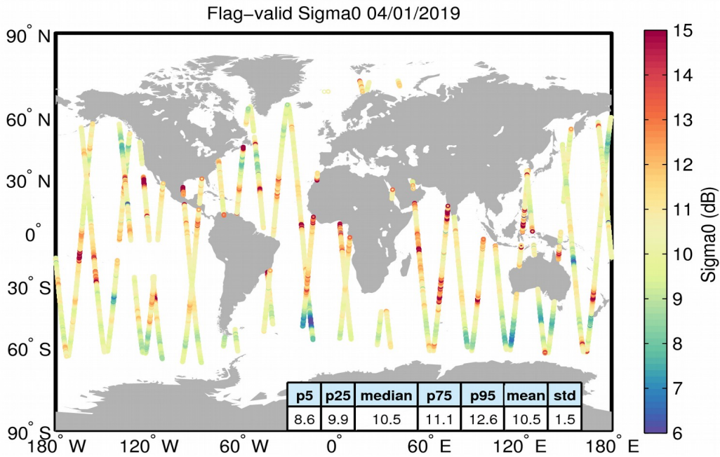
Figure 23. Geographical distribution of flag-valid sigma0 data over oceans and lakes for 04/01/2019. The statistical values shown in the table refer to the sigma0 in dB and are calculated over all measurements shown in the figure.
