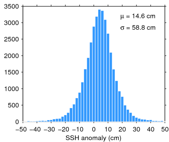
Figure 7. Histogram of flag-valid SSH anomaly over oceans and lakes for 04/01/2019. The mean ( \mu ) and standard deviation ( \sigma ) are also shown. Note that values outside [-50 50] cm are excluded from the histogram for the sake of readability but not from the computation of \mu and \sigma .
