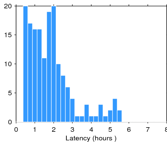
Figure 2. Histogram of the data latency for 04/01/2019. The y-axis denotes the number of files that are made available with a delay of x-hours with respect to the mean time of the records stored in the file.
