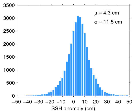
Figure 11. Histogram of science-valid SSH anomaly over oceans and lakes for 04/01/2019. The mean ( \mu ) and standard deviation ( \sigma ) are also shown. Note that values outside [-50 50] cm are excluded from the histogram for the sake of readability but not from the computation of \mu and \sigma .
