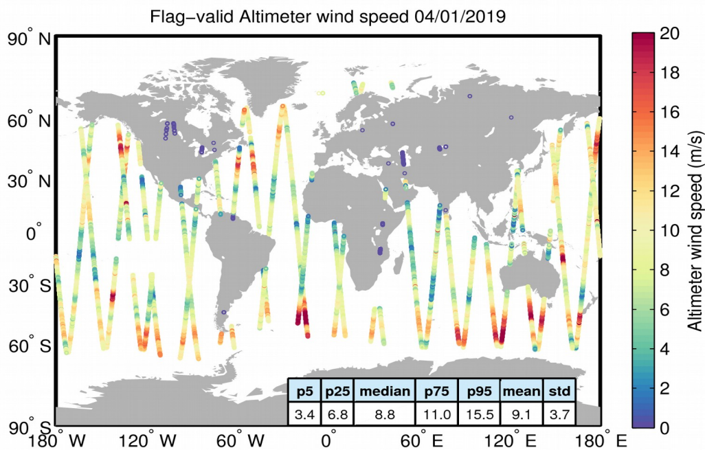
Figure 31. Geographical distribution of flag-valid wind data over oceans and lakes for 04/01/2019. The statistical values shown in the table refer to the wind in m/s and are calculated over all measurements shown in the figure.
