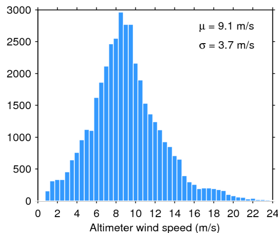
Figure 35. Histogram of science-valid wind over oceans and lakes for 04/01/2019. The mean ( \mu ) and standard deviation ( \sigma ) are also shown. Note that values larger than 24 m/s are excluded from the histogram for the sake of readability but not from the computation of \mu and \sigma .
