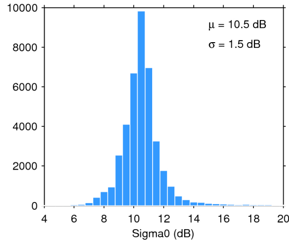
Figure 25. Histogram of flag-valid sigma0 over oceans and lakes for 04/01/2019. The mean ( \mu ) and standard deviation ( \sigma ) are also shown. Note that values outside [4 20] dB are excluded from the histogram for the sake of readability but not from the computation of \mu and \sigma .
