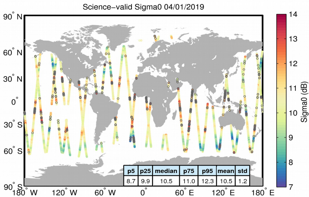
Figure 27. Geographical distribution of science-valid sigma0 data over oceans and lakes for 04/01/2019. The statistical values shown in the table refer to the sigma0 in dB and are calculated over all measurements shown in the figure. Gray circles denote records that have been rejected based on the editing criteria described in Table 4.
