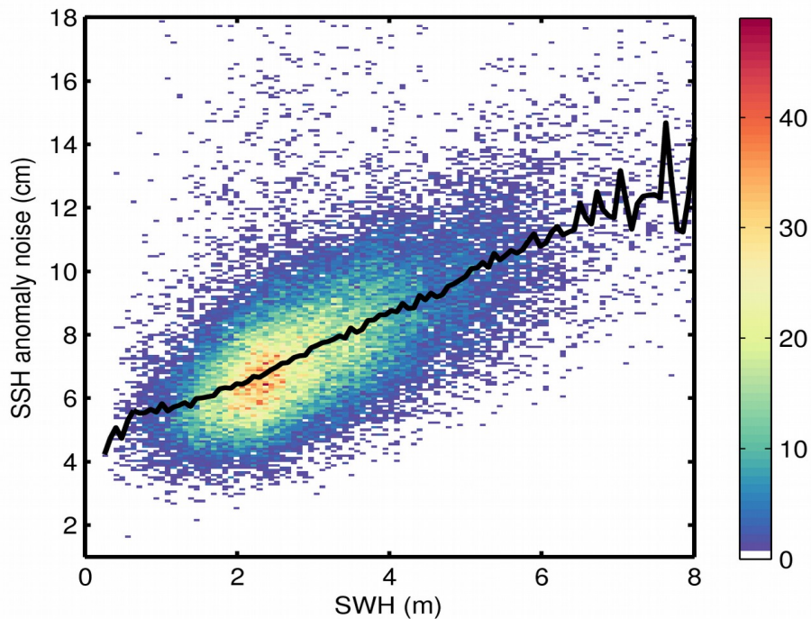
Figure 9. 2D histogram showing flag-valid SSH anomaly noise as a function of SWH for 04/01/2019. The black line denotes the median SSH anomaly noise as a function of SWH.
