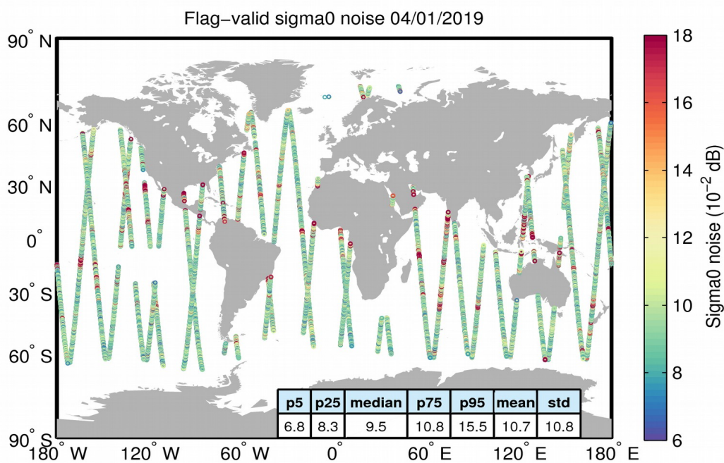
Figure 26. Geographical distribution of flag-valid 20-Hz sigma0 measurement noise over oceans and lakes for 04/01/2019. The statistical values shown in the figure refer to the sigma0 noise and are calculated over all measurements shown in the figure.
