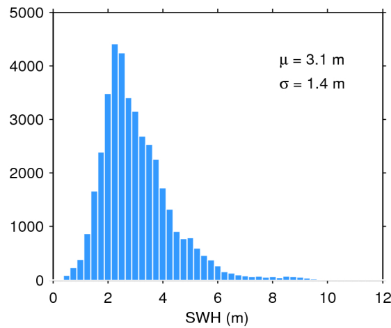
Figure 17. Histogram of flag-valid SWH over oceans and lakes for 04/01/2019. The mean ( \mu ) and standard deviation ( \sigma ) are also shown. Note that values larger than 12 m are excluded from the histogram for the sake of readability but not from the computation of \mu and \sigma .
