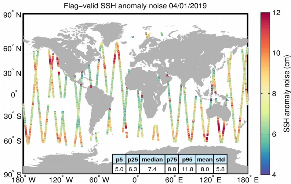
Figure 8. Geographical distribution of flag-valid 20-Hz SSH anomaly measurement noise over oceans and lakes for 04/01/2019. The statistical values shown in the table refer to the SSH anomaly noise and are calculated over all measurements shown in the figure.
