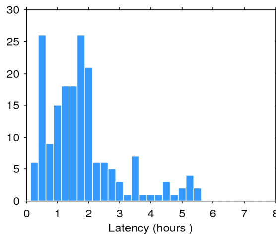
Figure 2. Histogram of the data latency for 02/01/2019. The y-axis denotes the number of files that are made available with a delay of x-hours with respect to the mean time of the records stored in the file.
