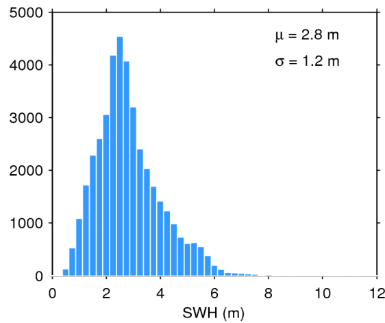
Figure 17. Histogram of flag-valid SWH over oceans and lakes for 01/01/2019. The mean ( \mu ) and standard deviation ( \sigma ) are also shown. Note that values larger than 12 m are excluded from the histogram for the sake of readability but not from the computation of \mu and \sigma .
