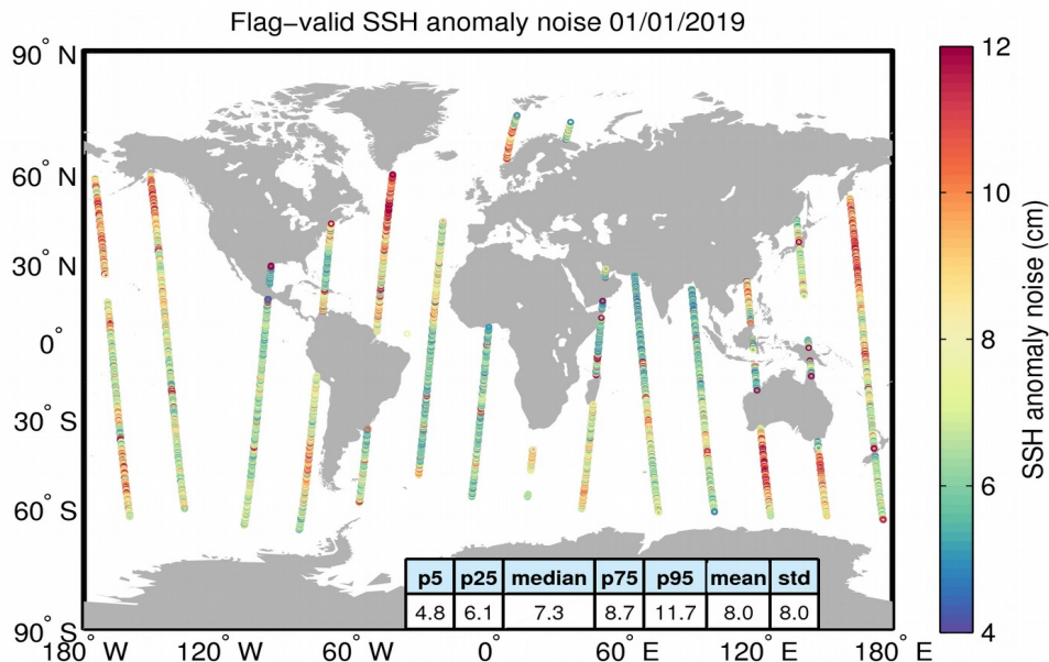
Figure 8. Geographical distribution of flag-valid 20-Hz SSH anomaly measurement noise over oceans and lakes for 01/01/2019. The statistical values shown in the table refer to the SSH anomaly noise and are calculated over all measurements shown in the figure.
