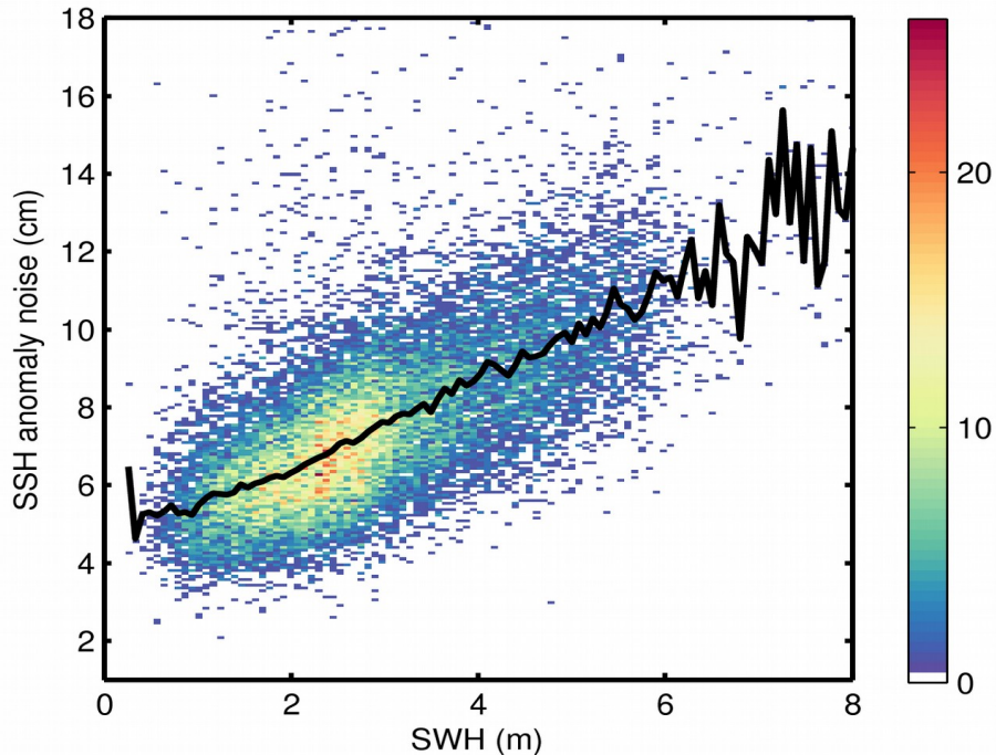
Figure 9. 2D histogram showing flag-valid SSH anomaly noise as a function of SWH for 01/01/2019. The black line denotes the median SSH anomaly noise as a function of SWH.
