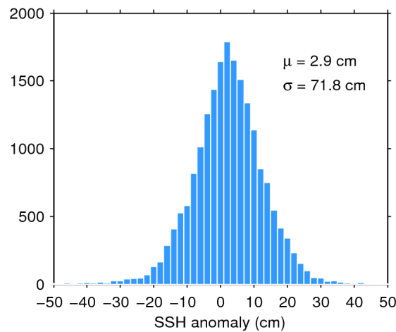
Figure 7. Histogram of flag-valid SSH anomaly over oceans and lakes for 01/01/2019. The mean ( \mu ) and standard deviation ( \sigma ) are also shown. Note that values outside [-50\ 50] cm are excluded from the histogram for the sake of readability but not from the computation of \mu and \sigma .
