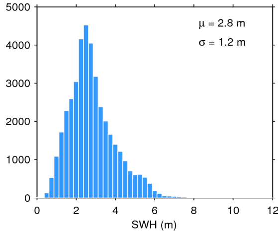
Figure 20. Histogram of science-valid SWH over oceans and lakes for 01/01/2019. The mean ( \mu ) and standard deviation ( \sigma ) are also shown. Note that values larger than 12 m are excluded from the histogram for the sake of readability but not from the computation of \mu and \sigma .
