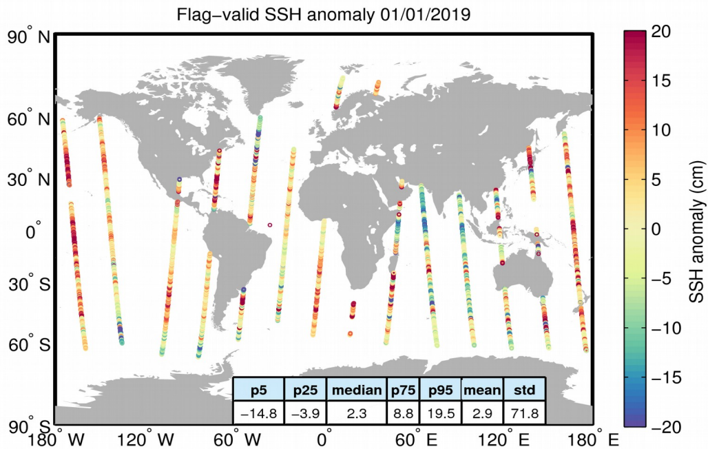
Figure 5. Geographical distribution of flag-valid 1-Hz SSH anomaly data over oceans and lakes for 01/01/2019. The statistical values shown in the table refer to the SSH anomaly in cm and are calculated over all measurements shown in the figure.
