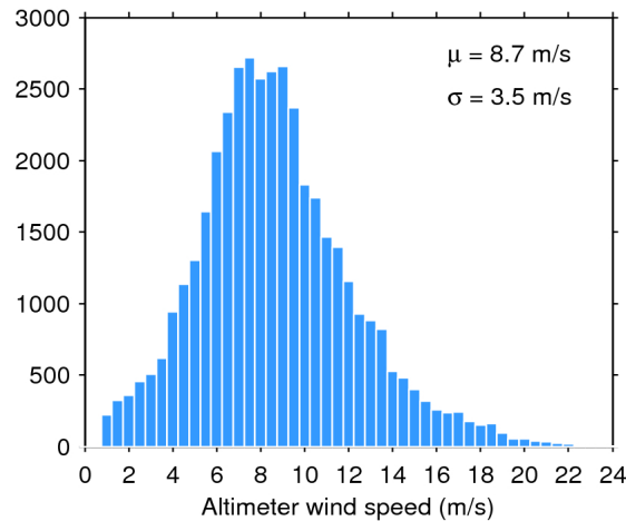
Figure 33. Histogram of flag-valid wind over oceans and lakes for 01/01/2019. The mean ( \mu ) and standard deviation ( \sigma ) are also shown. Note that values larger than 24 m/s are excluded from the histogram for the sake of readability but not from the computation of \mu and \sigma .
