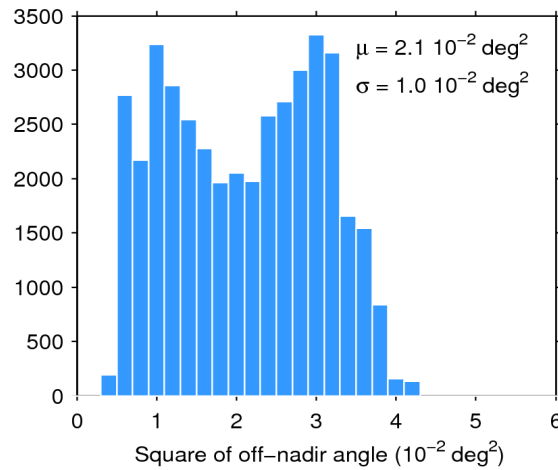
Figure 39. Histogram of flag-valid mispointing over oceans and lakes for 01/01/2019. The mean ( \mu ) and standard deviation ( \sigma ) are also shown. Note that values larger than 6 \cdot 10^{-2} \text{ deg}^2 are excluded from the histogram for the sake of readability but not from the computation of \mu and \sigma .
