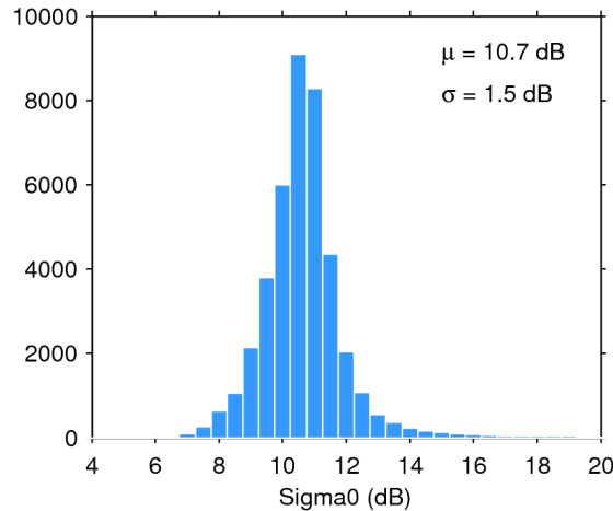
Figure 25. Histogram of flag-valid sigma0 over oceans and lakes for 01/01/2019. The mean ( \mu ) and standard deviation ( \sigma ) are also shown. Note that values outside [4 20] dB are excluded from the histogram for the sake of readability but not from the computation of \mu and \sigma .
