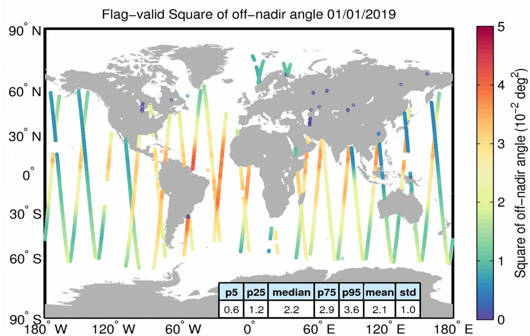
Figure 37. Geographical distribution of flag-valid mispointing data over oceans and lakes for 01/01/2019. The statistical values shown in the table refer to the mispointing in 10^{-2} \text{ deg}^2 and are calculated over all measurements shown in the figure.
