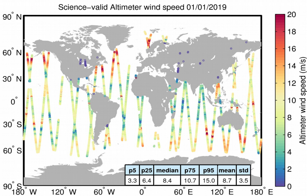
Figure 34. Geographical distribution of science-valid wind data over oceans and lakes for 01/01/2019. The statistical values shown in the table refer to the wind in m/s and are calculated over all measurements shown in the figure. Gray circles denote records that have been rejected based on the editing criteria described in Table 5.
