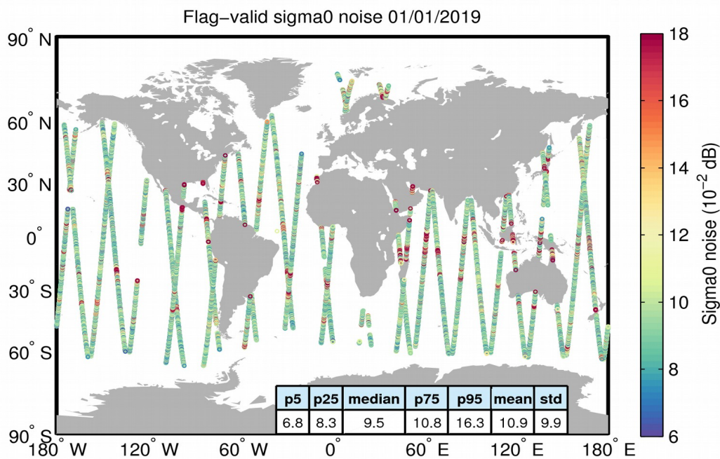
Figure 26. Geographical distribution of flag-valid 20-Hz sigma0 measurement noise over oceans and lakes for 01/01/2019. The statistical values shown in the table refer to the sigma0 noise and are calculated over all measurements shown in the figure.
