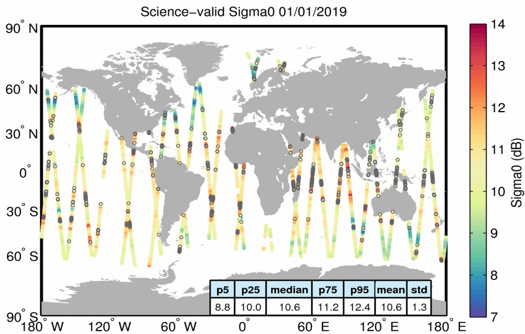
Figure 27. Geographical distribution of science-valid sigma0 data over oceans and lakes for 01/01/2019. The statistical values shown in the table refer to the sigma0 in dB and are calculated over all measurements shown in the figure. Gray circles denote records that have been rejected based on the editing criteria described in Table 4.
