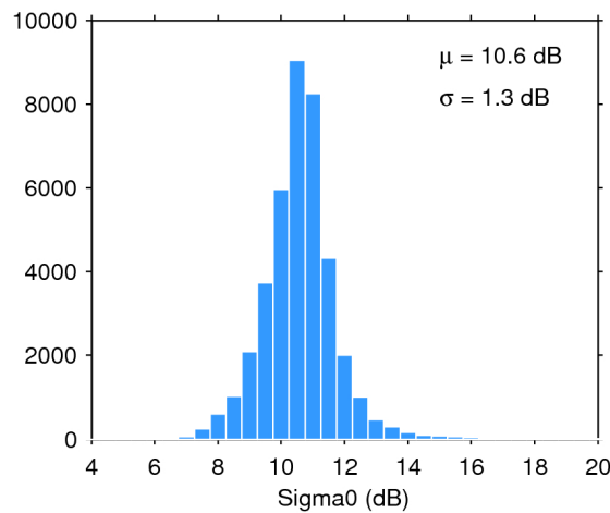
Figure 28. Histogram of science-valid sigma0 over oceans and lakes for 01/01/2019. The mean ( \mu ) and standard deviation ( \sigma ) are also shown. Note that values outside [4 20] dB are excluded from the histogram for the sake of readability but not from the computation of \mu and \sigma .
