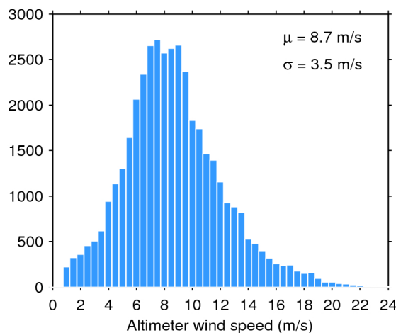
Figure 35. Histogram of science-valid wind over oceans and lakes for 01/01/2019. The mean ( \mu ) and standard deviation ( \sigma ) are also shown. Note that values larger than 24 m/s are excluded from the histogram for the sake of readability but not from the computation of \mu and \sigma .
