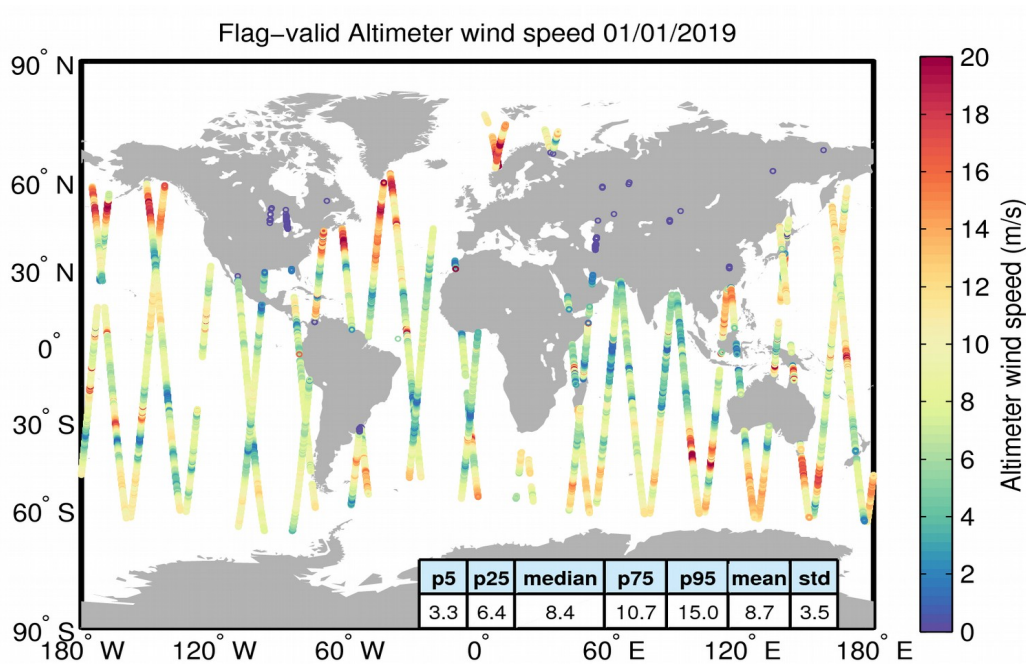
Figure 31. Geographical distribution of flag-valid wind data over oceans and lakes for 01/01/2019. The statistical values shown in the table refer to the wind in m/s and are calculated over all measurements shown in the figure.
