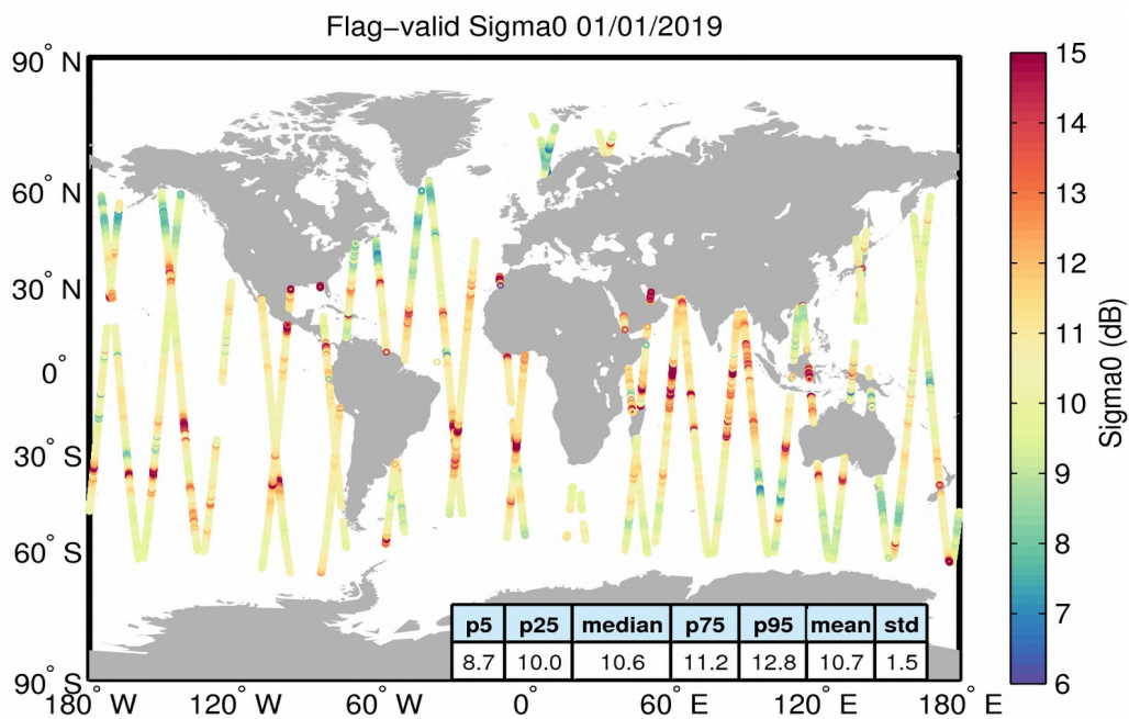
Figure 23. Geographical distribution of flag-valid sigma0 data over oceans and lakes for 01/01/2019. The statistical values shown in the table refer to the sigma0 in dB and are calculated over all measurements shown in the figure.
