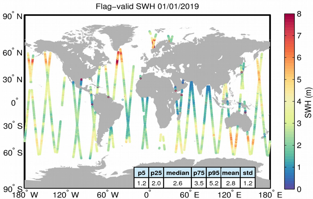
Figure 15. Geographical distribution of flag-valid SWH data over oceans and lakes for 01/01/2019. The statistical values shown in the table refer to the SWH in m and are calculated over all measurements shown in the figure.
