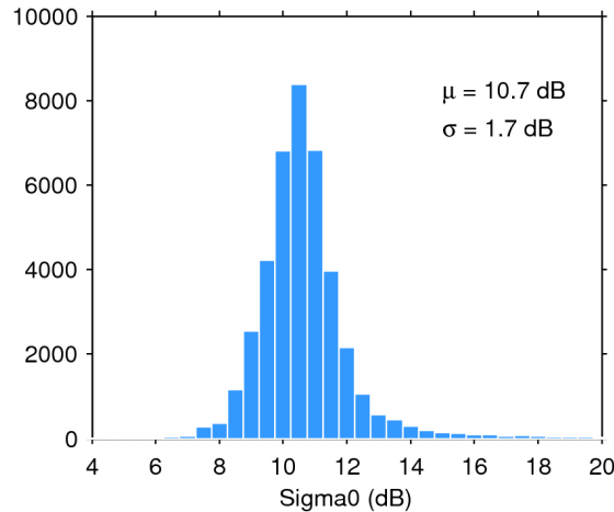
Figure 25. Histogram of flag-valid sigma0 over oceans and lakes for 31/12/2018. The mean ( \mu ) and standard deviation ( \sigma ) are also shown. Note that values outside [4 20] dB are excluded from the histogram for the sake of readability but not from the computation of \mu and \sigma .
