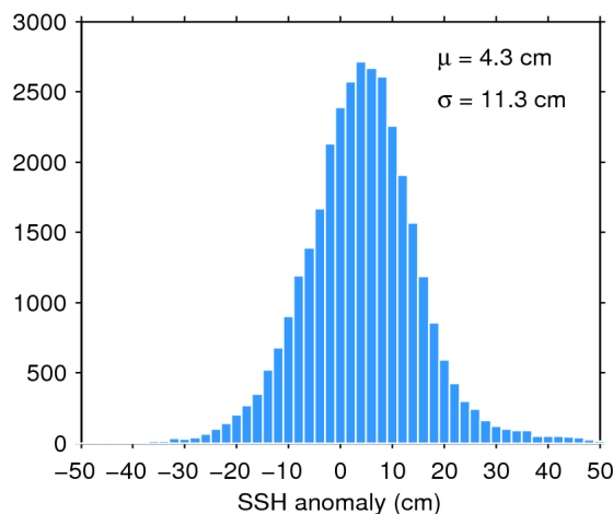
Figure 11. Histogram of science-valid SSH anomaly over oceans and lakes for 31/12/2018. The mean ( \mu ) and standard deviation ( \sigma ) are also shown. Note that values outside [-50 50] cm are excluded from the histogram for the sake of readability but not from the computation of \mu and \sigma .
