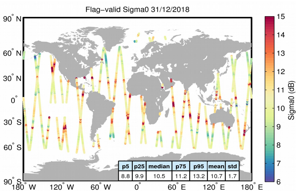
Figure 23. Geographical distribution of flag-valid sigma0 data over oceans and lakes for 31/12/2018. The statistical values shown in the table refer to the sigma0 in dB and are calculated over all measurements shown in the figure.
