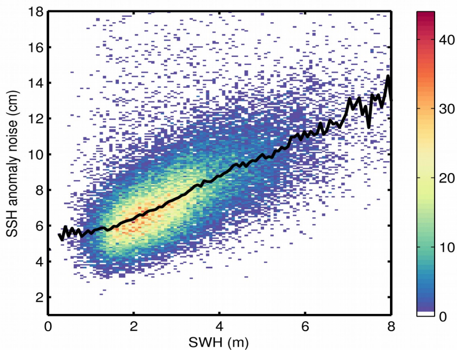
Figure 9. 2D histogram showing flag-valid SSH anomaly noise as a function of SWH for 31/12/2018. The black line denotes the median SSH anomaly noise as a function of SWH.
