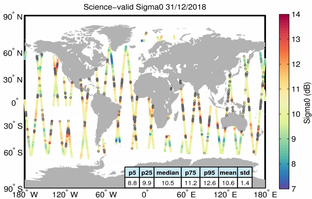
Figure 27. Geographical distribution of science-valid sigma0 data over oceans and lakes for 31/12/2018. The statistical values shown in the table refer to the sigma0 in dB and are calculated over all measurements shown in the figure. Gray circles denote records that have been rejected based on the editing criteria described in Table 4.
