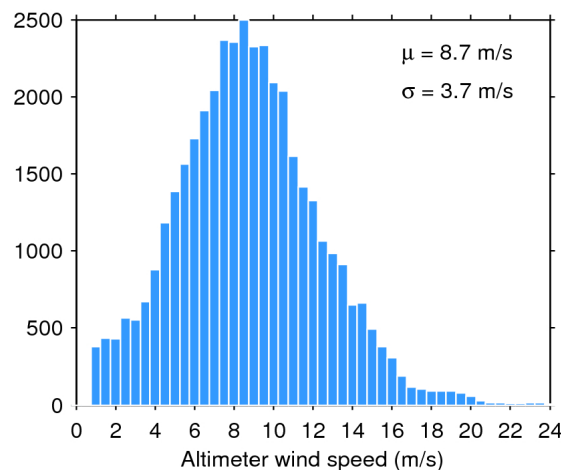
Figure 35. Histogram of science-valid wind over oceans and lakes for 31/12/2018. The mean ( \mu ) and standard deviation ( \sigma ) are also shown. Note that values larger than 24 m/s are excluded from the histogram for the sake of readability but not from the computation of \mu and \sigma .
