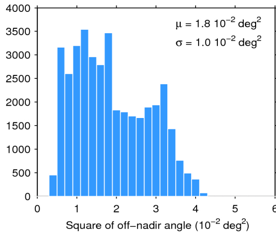
Figure 39. Histogram of flag-valid mispointing over oceans and lakes for 31/12/2018. The mean ( \mu ) and standard deviation ( \sigma ) are also shown. Note that values larger than 6 \cdot 10^{-2} \text{ deg}^2 are excluded from the histogram for the sake of readability but not from the computation of \mu and \sigma .
