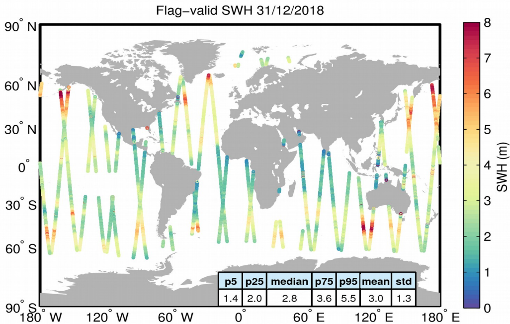
Figure 15. Geographical distribution of flag-valid SWH data over oceans and lakes for 31/12/2018. The statistical values shown in the table refer to the SWH in m and are calculated over all measurements shown in the figure.
