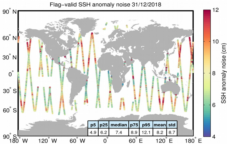
Figure 8. Geographical distribution of flag-valid 20-Hz SSH anomaly measurement noise over oceans and lakes for 31/12/2018. The statistical values shown in the table refer to the SSH anomaly noise and are calculated over all measurements shown in the figure.
