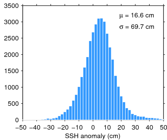
Figure 7. Histogram of flag-valid SSH anomaly over oceans and lakes for 31/12/2018. The mean ( \mu ) and standard deviation ( \sigma ) are also shown. Note that values outside [-50 50] cm are excluded from the histogram for the sake of readability but not from the computation of \mu and \sigma .
