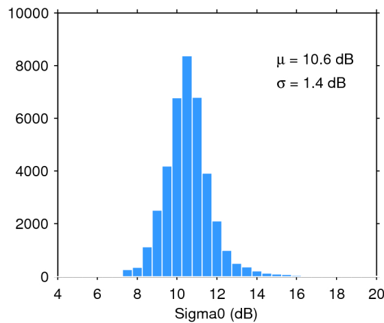
Figure 28. Histogram of science-valid sigma0 over oceans and lakes for 31/12/2018. The mean ( \mu ) and standard deviation ( \sigma ) are also shown. Note that values outside [4 20] dB are excluded from the histogram for the sake of readability but not from the computation of \mu and \sigma .
