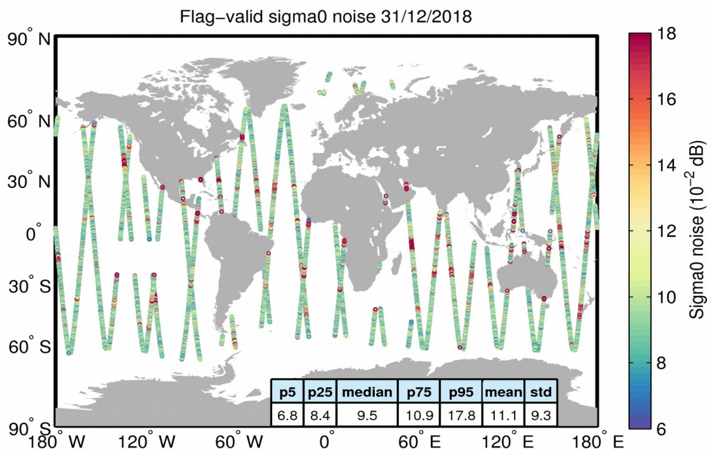
Figure 26. Geographical distribution of flag-valid 20-Hz sigma0 measurement noise over oceans and lakes for 31/12/2018. The statistical values shown in the figure refer to the sigma0 noise and are calculated over all measurements shown in the figure.
