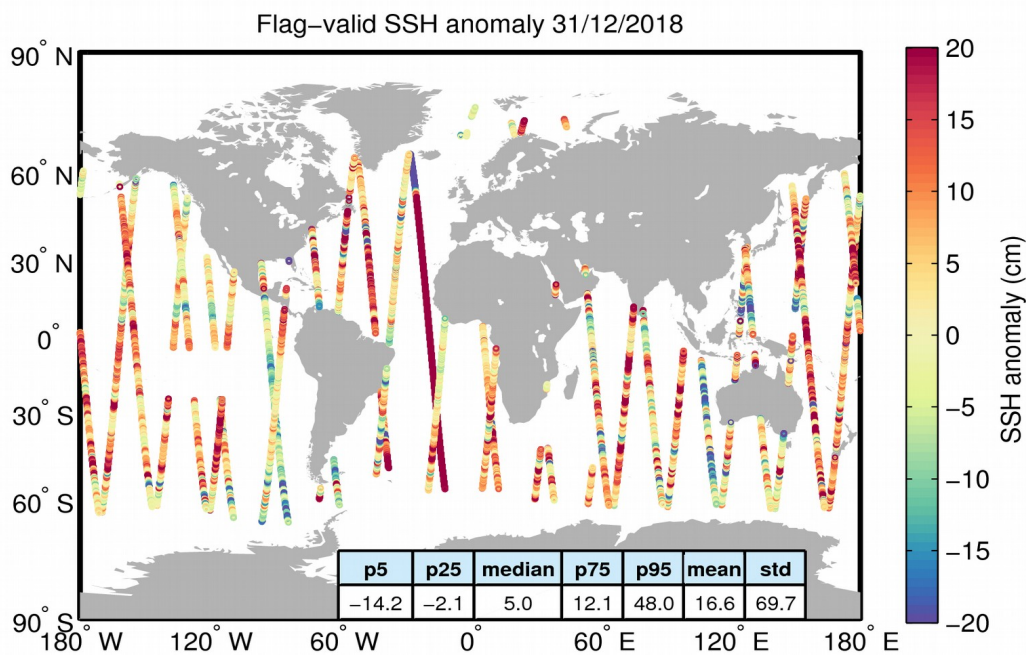
Figure 5. Geographical distribution of flag-valid 1-Hz SSH anomaly data over oceans and lakes for 31/12/2018. The statistical values shown in the table refer to the SSH anomaly in cm and are calculated over all measurements shown in the figure.
