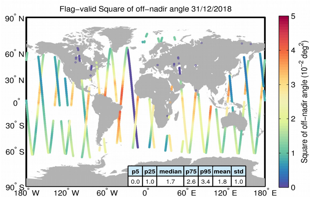
Figure 37. Geographical distribution of flag-valid mispointing data over oceans and lakes for 31/12/2018. The statistical values shown in the table refer to the mispointing in 10^{-2} \text{ deg}^2 and are calculated over all measurements shown in the figure.
