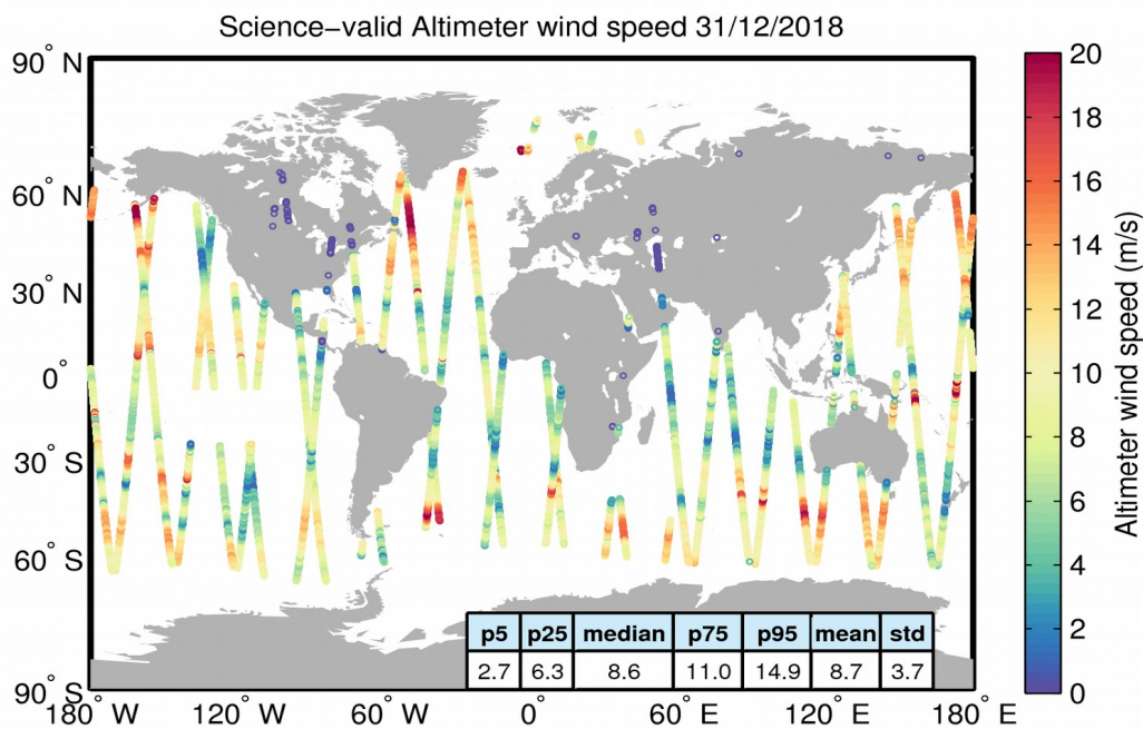
Figure 34. Geographical distribution of science-valid wind data over oceans and lakes for 31/12/2018. The statistical values shown in the table refer to the wind in m/s and are calculated over all measurements shown in the figure. Gray circles denote records that have been rejected based on the editing criteria described in Table 5.
