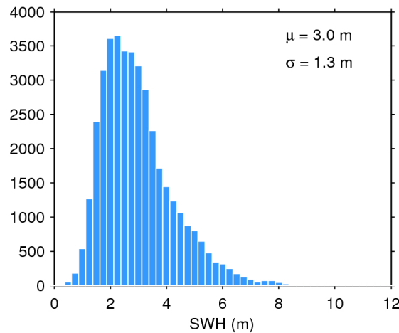
Figure 20. Histogram of science-valid SWH over oceans and lakes for 31/12/2018. The mean ( \mu ) and standard deviation ( \sigma ) are also shown. Note that values larger than 12 m are excluded from the histogram for the sake of readability but not from the computation of \mu and \sigma .
