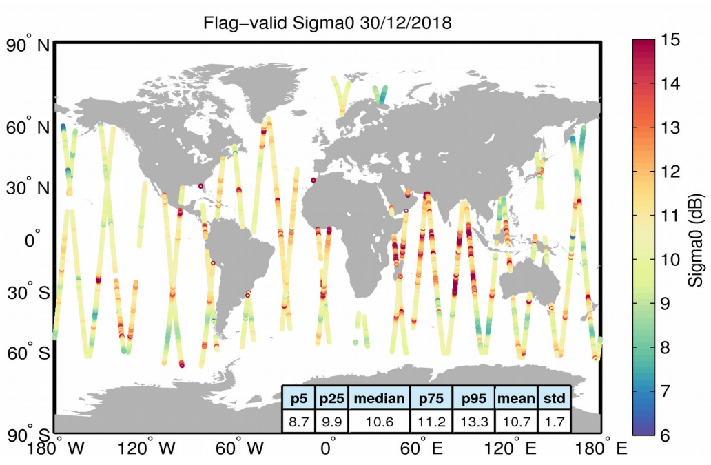
Figure 23. Geographical distribution of flag-valid sigma0 data over oceans and lakes for 30/12/2018. The statistical values shown in the table refer to the sigma0 in dB and are calculated over all measurements shown in the figure.
