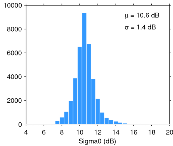
Figure 28. Histogram of science-valid sigma0 over oceans and lakes for 30/12/2018. The mean ( \mu ) and standard deviation ( \sigma ) are also shown. Note that values outside [4 20] dB are excluded from the histogram for the sake of readability but not from the computation of \mu and \sigma .
