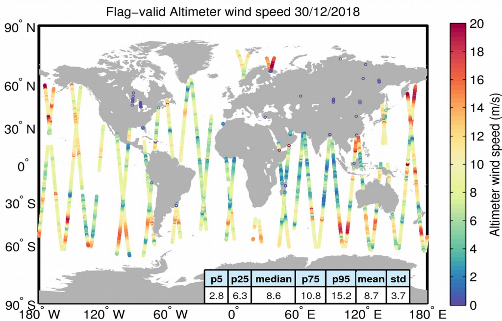
Figure 31. Geographical distribution of flag-valid wind data over oceans and lakes for 30/12/2018. The statistical values shown in the table refer to the wind in m/s and are calculated over all measurements shown in the figure.
