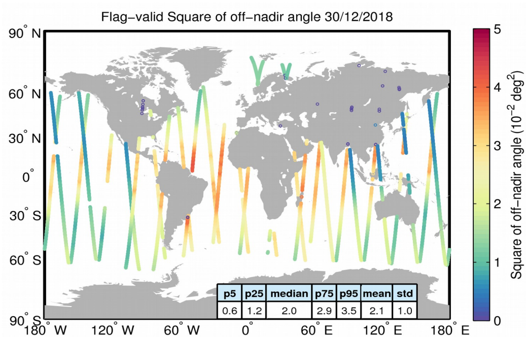
Figure 37. Geographical distribution of flag-valid mispointing data over oceans and lakes for 30/12/2018. The statistical values shown in the table refer to the mispointing in 10^{-2} deg 2 and are calculated over all measurements shown in the figure.
