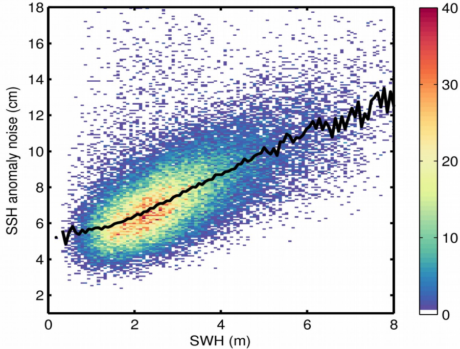
Figure 9. 2D histogram showing flag-valid SSH anomaly noise as a function of SWH for 30/12/2018. The black line denotes the median SSH anomaly noise as a function of SWH.
