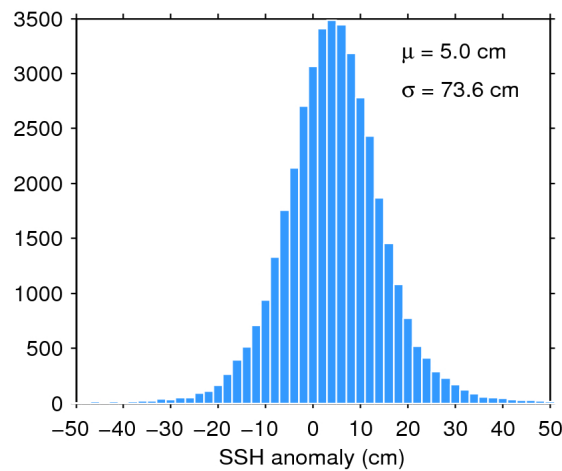
Figure 7. Histogram of flag-valid SSH anomaly over oceans and lakes for 30/12/2018. The mean ( \mu ) and standard deviation ( \sigma ) are also shown. Note that values outside [-50\ 50] cm are excluded from the histogram for the sake of readability but not from the computation of \mu and \sigma .
