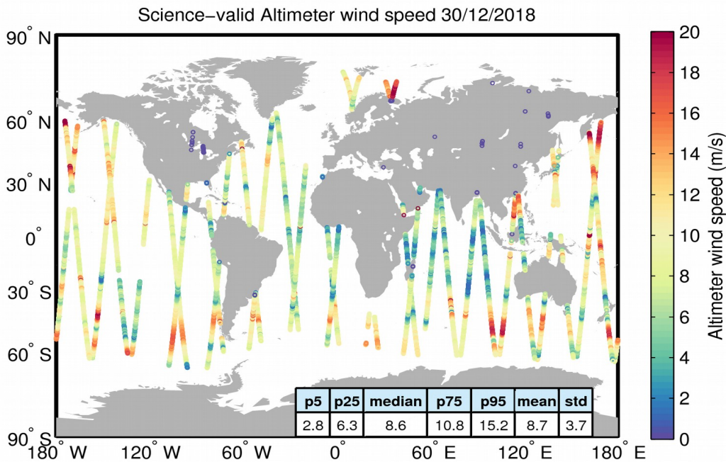
Figure 34. Geographical distribution of science-valid wind data over oceans and lakes for 30/12/2018. The statistical values shown in the table refer to the wind in m/s and are calculated over all measurements shown in the figure. Gray circles denote records that have been rejected based on the editing criteria described in Table 5.
