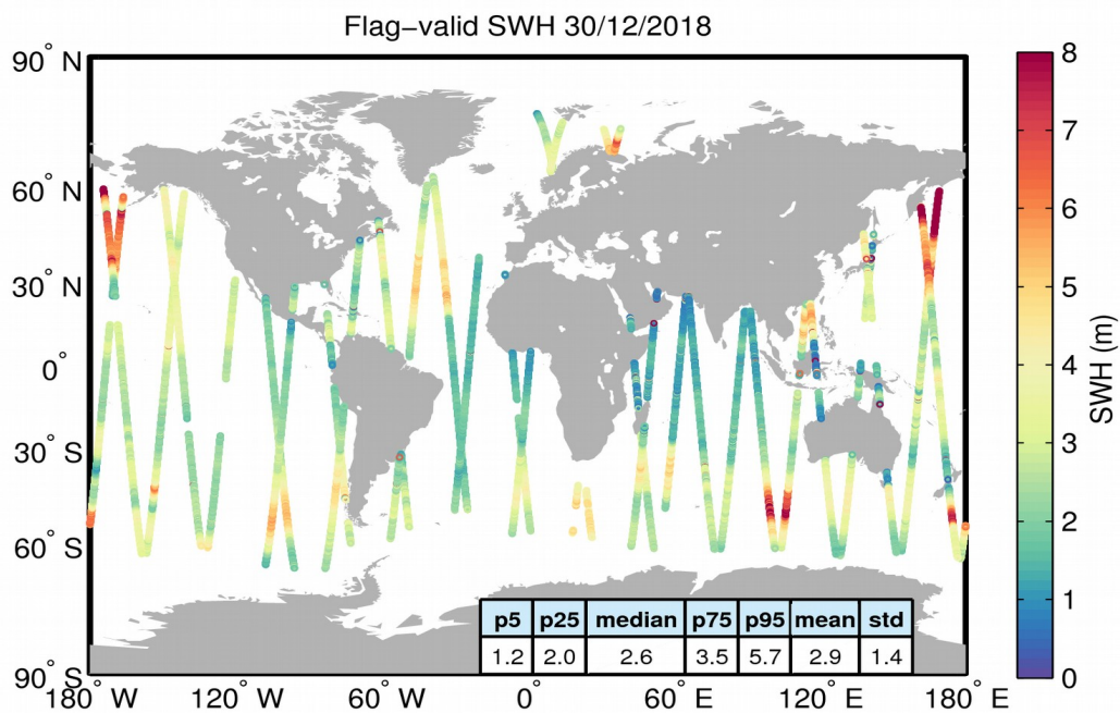
Figure 15. Geographical distribution of flag-valid SWH data over oceans and lakes for 30/12/2018. The statistical values shown in the table refer to the SWH in m and are calculated over all measurements shown in the figure.
