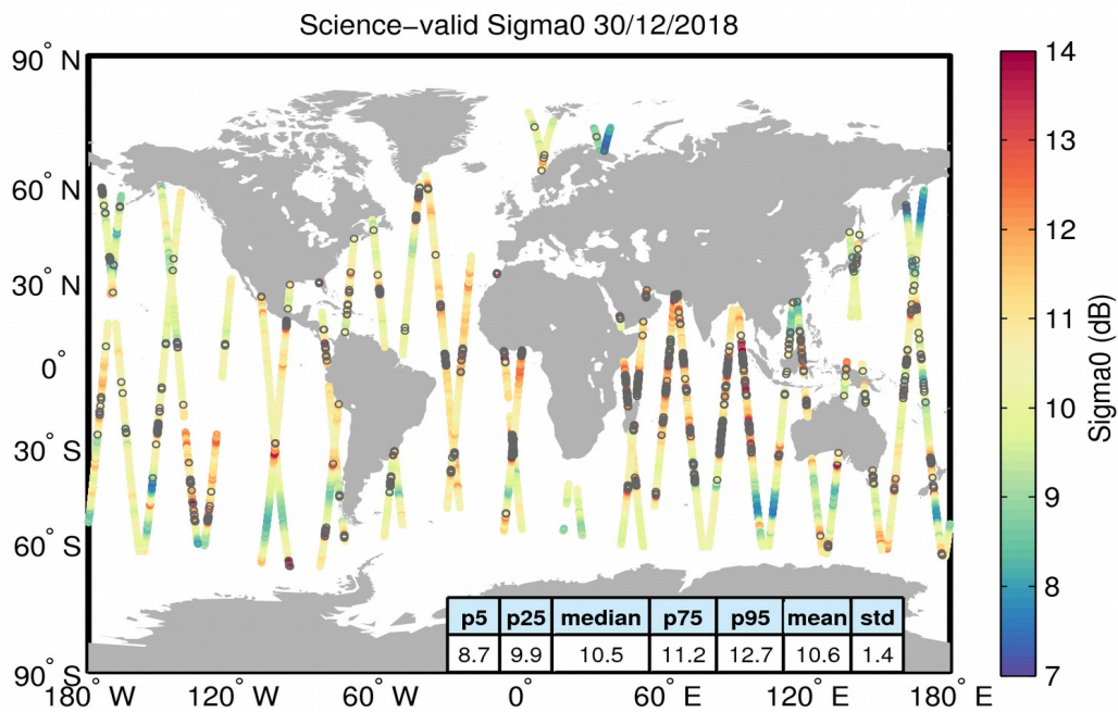
Figure 27. Geographical distribution of science-valid sigma0 data over oceans and lakes for 30/12/2018. The statistical values shown in the table refer to the sigma0 in dB and are calculated over all measurements shown in the figure. Gray circles denote records that have been rejected based on the editing criteria described in Table 4.
