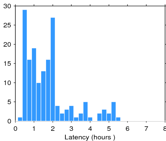
Figure 2. Histogram of the data latency for 30/12/2018. The y-axis denotes the number of files that are made available with a delay of x-hours with respect to the mean time of the records stored in the file.
