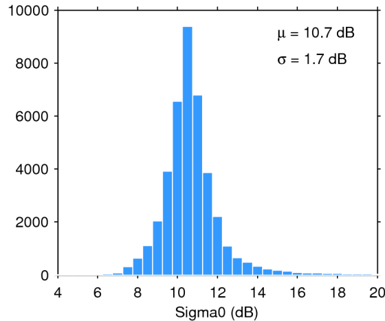
Figure 25. Histogram of flag-valid sigma0 over oceans and lakes for 30/12/2018. The mean ( \mu ) and standard deviation ( \sigma ) are also shown. Note that values outside [4 20] dB are excluded from the histogram for the sake of readability but not from the computation of \mu and \sigma .
