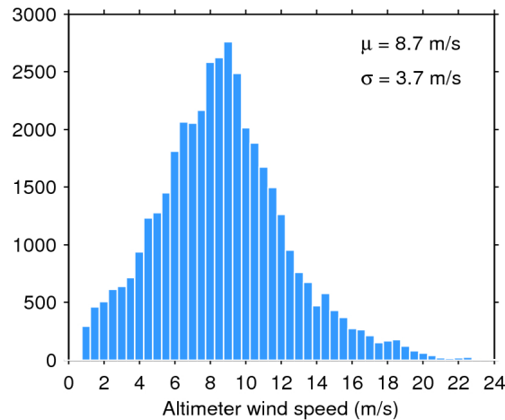
Figure 33. Histogram of flag-valid wind over oceans and lakes for 30/12/2018. The mean ( \mu ) and standard deviation ( \sigma ) are also shown. Note that values larger than 24 m/s are excluded from the histogram for the sake of readability but not from the computation of \mu and \sigma .
