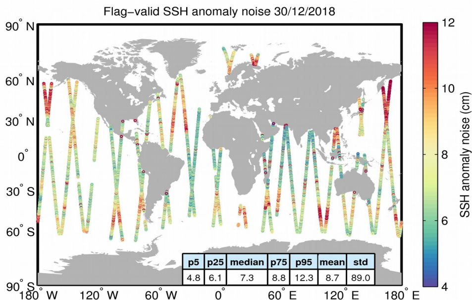
Figure 8. Geographical distribution of flag-valid 20-Hz SSH anomaly measurement noise over oceans and lakes for 30/12/2018. The statistical values shown in the table refer to the SSH anomaly noise and are calculated over all measurements shown in the figure.
