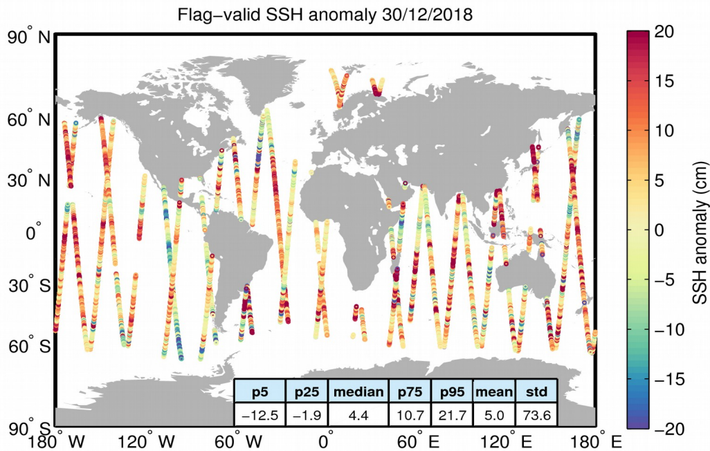
Figure 5. Geographical distribution of flag-valid 1-Hz SSH anomaly data over oceans and lakes for 30/12/2018. The statistical values shown in the table refer to the SSH anomaly in cm and are calculated over all measurements shown in the figure.
