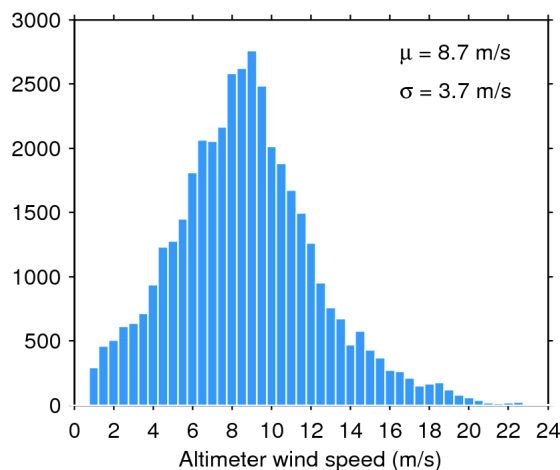
Figure 35. Histogram of science-valid wind over oceans and lakes for 30/12/2018. The mean ( \mu ) and standard deviation ( \sigma ) are also shown. Note that values larger than 24 m/s are excluded from the histogram for the sake of readability but not from the computation of \mu and \sigma .
