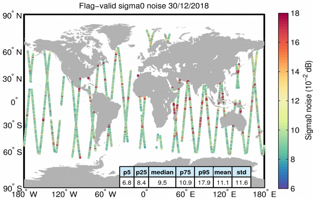
Figure 26. Geographical distribution of flag-valid 20-Hz sigma0 measurement noise over oceans and lakes for 30/12/2018. The statistical values shown in the table refer to the sigma0 noise and are calculated over all measurements shown in the figure.
