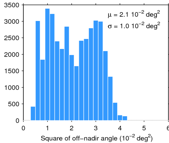
Figure 39. Histogram of flag-valid mispointing over oceans and lakes for 30/12/2018. The mean ( \mu ) and standard deviation ( \sigma ) are also shown. Note that values larger than 6 \cdot 10^{-2} \text{ deg}^2 are excluded from the histogram for the sake of readability but not from the computation of \mu and \sigma .
