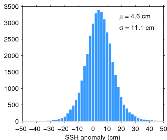
Figure 11. Histogram of science-valid SSH anomaly over oceans and lakes for 30/12/2018. The mean ( \mu ) and standard deviation ( \sigma ) are also shown. Note that values outside [-50 50] cm are excluded from the histogram for the sake of readability but not from the computation of \mu and \sigma .
