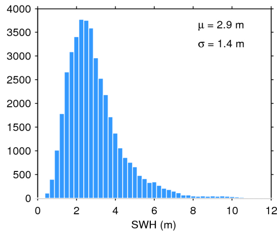
Figure 17. Histogram of flag-valid SWH over oceans and lakes for 30/12/2018. The mean ( \mu ) and standard deviation ( \sigma ) are also shown. Note that values larger than 12 m are excluded from the histogram for the sake of readability but not from the computation of \mu and \sigma .
