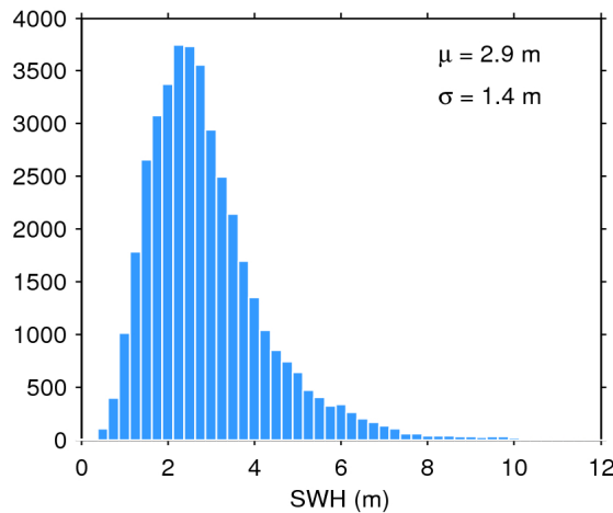
Figure 20. Histogram of science-valid SWH over oceans and lakes for 30/12/2018. The mean ( \mu ) and standard deviation ( \sigma ) are also shown. Note that values larger than 12 m are excluded from the histogram for the sake of readability but not from the computation of \mu and \sigma .
