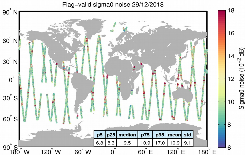
Figure 26. Geographical distribution of flag-valid 20-Hz sigma0 measurement noise over oceans and lakes for 29/12/2018. The statistical values shown in the table refer to the sigma0 noise and are calculated over all measurements shown in the figure.
