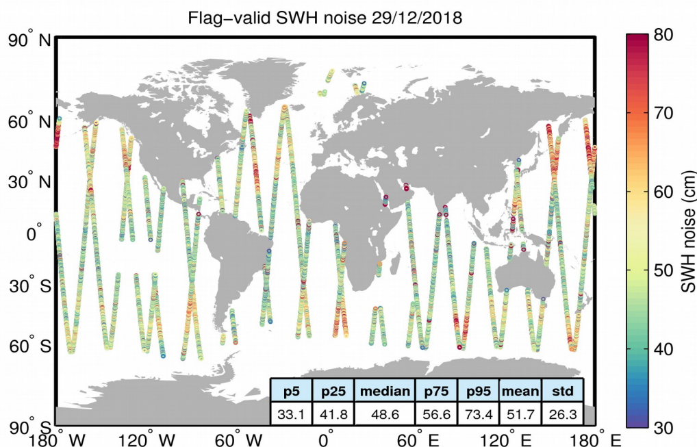
Figure 18. Geographical distribution of flag-valid 20-Hz SWH measurement noise over oceans and lakes for 29/12/2018. The statistical values shown in the figure refer to the SWH noise and are calculated over all measurements shown in the figure.
