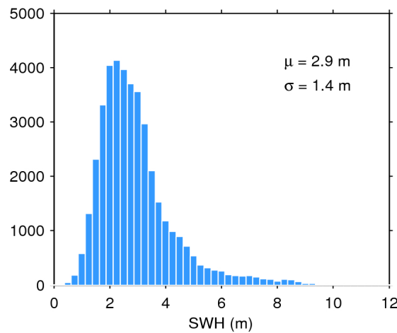
Figure 17. Histogram of flag-valid SWH over oceans and lakes for 29/12/2018. The mean ( \mu ) and standard deviation ( \sigma ) are also shown. Note that values larger than 12 m are excluded from the histogram for the sake of readability but not from the computation of \mu and \sigma .
