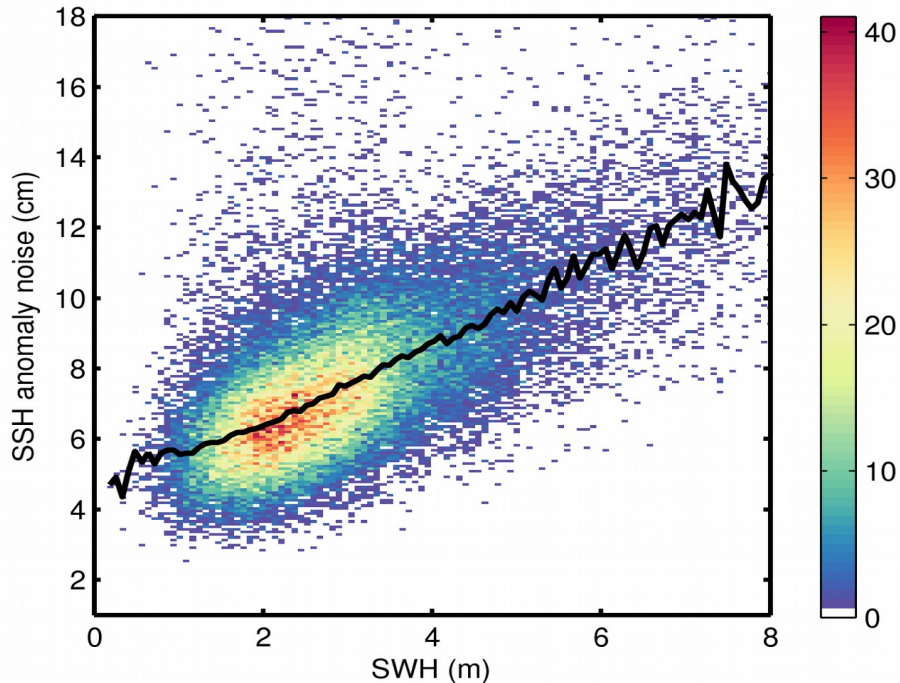
Figure 9. 2D histogram showing flag-valid SSH anomaly noise as a function of SWH for 29/12/2018. The black line denotes the median SSH anomaly noise as a function of SWH.
