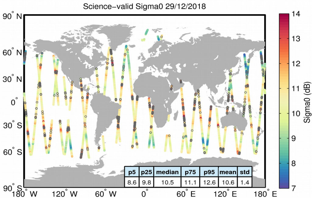
Figure 27. Geographical distribution of science-valid sigma0 data over oceans and lakes for 29/12/2018. The statistical values shown in the table refer to the sigma0 in dB and are calculated over all measurements shown in the figure. Gray circles denote records that have been rejected based on the editing criteria described in Table 4.
