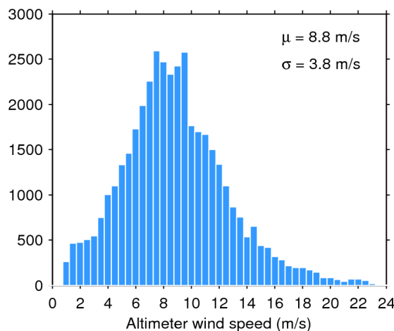
Figure 35. Histogram of science-valid wind over oceans and lakes for 29/12/2018. The mean ( \mu ) and standard deviation ( \sigma ) are also shown. Note that values larger than 24 m/s are excluded from the histogram for the sake of readability but not from the computation of \mu and \sigma .
