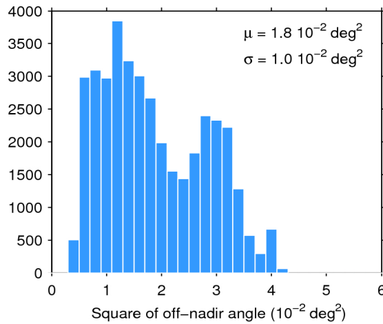
Figure 39. Histogram of flag-valid mispointing over oceans and lakes for 29/12/2018. The mean ( \mu ) and standard deviation ( \sigma ) are also shown. Note that values larger than 6 \cdot 10^{-2} \text{ deg}^2 are excluded from the histogram for the sake of readability but not from the computation of \mu and \sigma .
