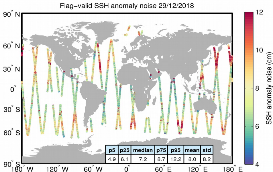
Figure 8. Geographical distribution of flag-valid 20-Hz SSH anomaly measurement noise over oceans and lakes for 29/12/2018. The statistical values shown in the table refer to the SSH anomaly noise and are calculated over all measurements shown in the figure.
