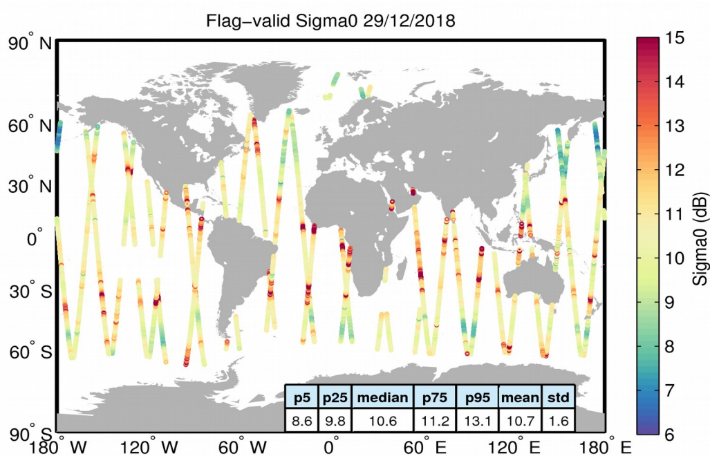
Figure 23. Geographical distribution of flag-valid sigma0 data over oceans and lakes for 29/12/2018. The statistical values shown in the table refer to the sigma0 in dB and are calculated over all measurements shown in the figure.
