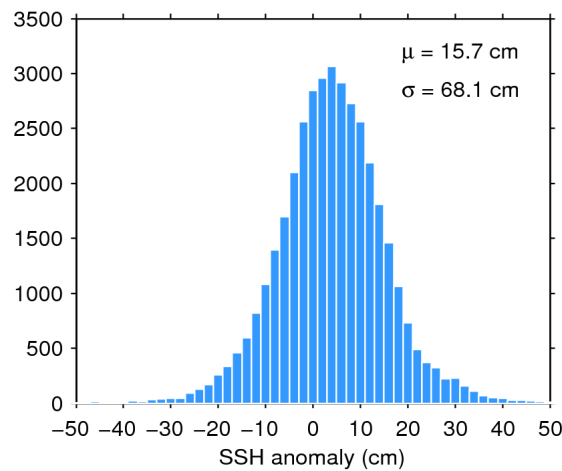
Figure 7. Histogram of flag-valid SSH anomaly over oceans and lakes for 29/12/2018. The mean ( \mu ) and standard deviation ( \sigma ) are also shown. Note that values outside [-50\ 50] cm are excluded from the histogram for the sake of readability but not from the computation of \mu and \sigma .
