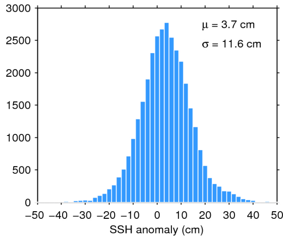
Figure 11. Histogram of science-valid SSH anomaly over oceans and lakes for 29/12/2018. The mean ( \mu ) and standard deviation ( \sigma ) are also shown. Note that values outside [-50 50] cm are excluded from the histogram for the sake of readability but not from the computation of \mu and \sigma .
