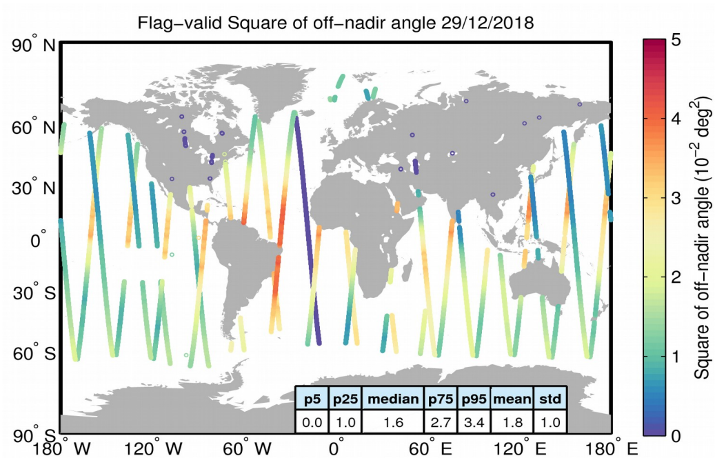
Figure 37. Geographical distribution of flag-valid mispointing data over oceans and lakes for 29/12/2018. The statistical values shown in the table refer to the mispointing in 10^{-2} \text{deg}^2 and are calculated over all measurements shown in the figure.
