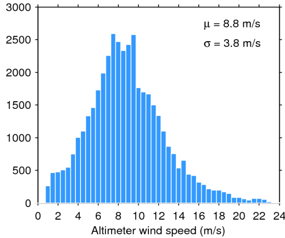
Figure 33. Histogram of flag-valid wind over oceans and lakes for 29/12/2018. The mean ( \mu ) and standard deviation ( \sigma ) are also shown. Note that values larger than 24 m/s are excluded from the histogram for the sake of readability but not from the computation of \mu and \sigma .
