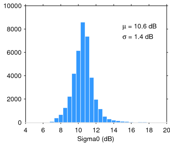
Figure 28. Histogram of science-valid sigma0 over oceans and lakes for 29/12/2018. The mean ( \mu ) and standard deviation ( \sigma ) are also shown. Note that values outside [4 20] dB are excluded from the histogram for the sake of readability but not from the computation of \mu and \sigma .
