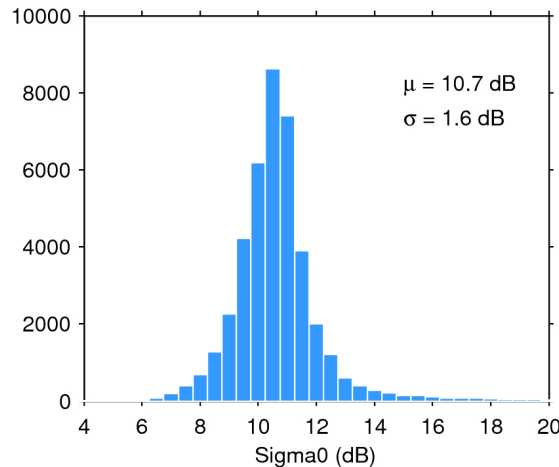
Figure 25. Histogram of flag-valid sigma0 over oceans and lakes for 29/12/2018. The mean ( \mu ) and standard deviation ( \sigma ) are also shown. Note that values outside [4 20] dB are excluded from the histogram for the sake of readability but not from the computation of \mu and \sigma .
