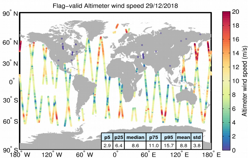
Figure 31. Geographical distribution of flag-valid wind data over oceans and lakes for 29/12/2018. The statistical values shown in the table refer to the wind in m/s and are calculated over all measurements shown in the figure.
