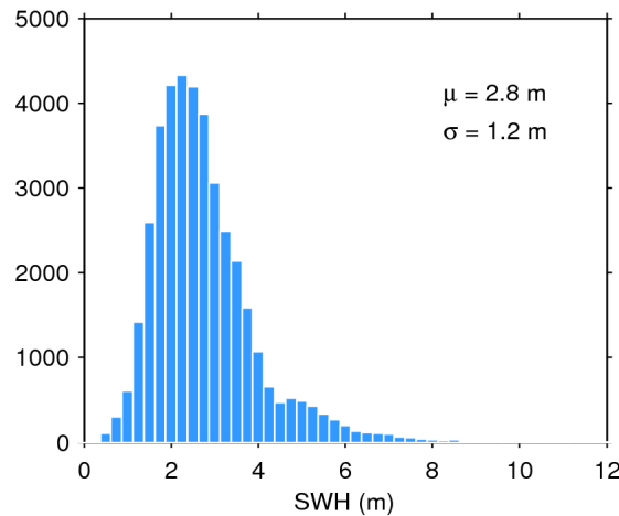
Figure 20. Histogram of science-valid SWH over oceans and lakes for 28/12/2018. The mean ( \mu ) and standard deviation ( \sigma ) are also shown. Note that values larger than 12 m are excluded from the histogram for the sake of readability but not from the computation of \mu and \sigma .
