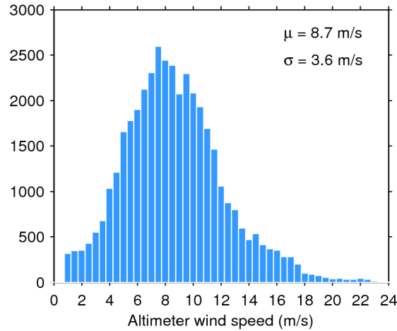
Figure 33. Histogram of flag-valid wind over oceans and lakes for 28/12/2018. The mean ( \mu ) and standard deviation ( \sigma ) are also shown. Note that values larger than 24 m/s are excluded from the histogram for the sake of readability but not from the computation of \mu and \sigma .
