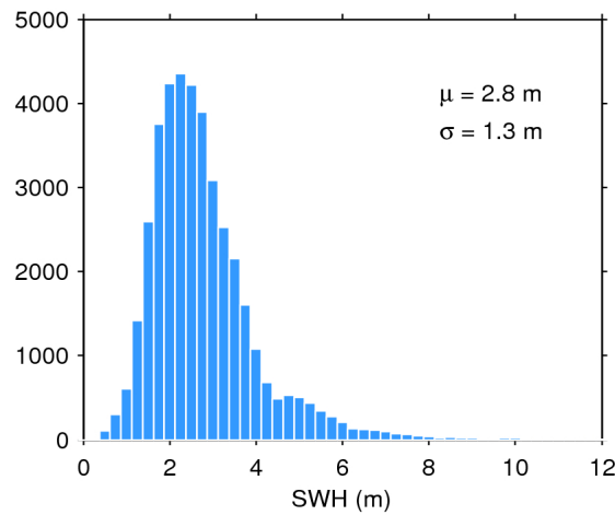
Figure 17. Histogram of flag-valid SWH over oceans and lakes for 28/12/2018. The mean ( \mu ) and standard deviation ( \sigma ) are also shown. Note that values larger than 12 m are excluded from the histogram for the sake of readability but not from the computation of \mu and \sigma .
