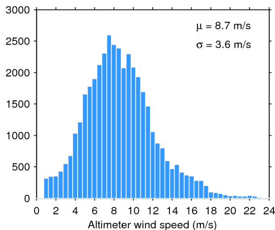
Figure 35. Histogram of science-valid wind over oceans and lakes for 28/12/2018. The mean ( \mu ) and standard deviation ( \sigma ) are also shown. Note that values larger than 24 m/s are excluded from the histogram for the sake of readability but not from the computation of \mu and \sigma .
