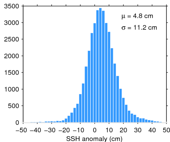
Figure 11. Histogram of science-valid SSH anomaly over oceans and lakes for 28/12/2018. The mean ( \mu ) and standard deviation ( \sigma ) are also shown. Note that values outside [-50 50] cm are excluded from the histogram for the sake of readability but not from the computation of \mu and \sigma .
