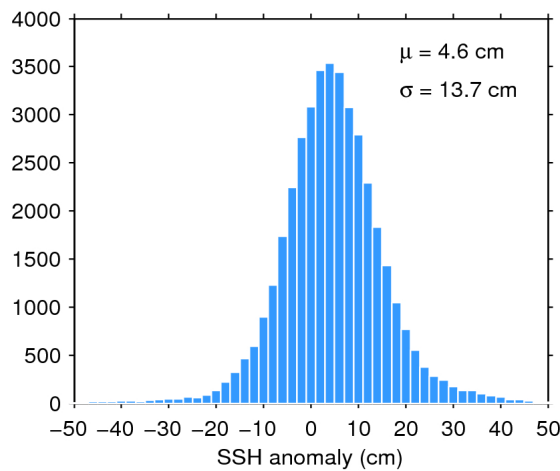
Figure 7. Histogram of flag-valid SSH anomaly over oceans and lakes for 28/12/2018. The mean ( \mu ) and standard deviation ( \sigma ) are also shown. Note that values outside [-50 50] cm are excluded from the histogram for the sake of readability but not from the computation of \mu and \sigma .
