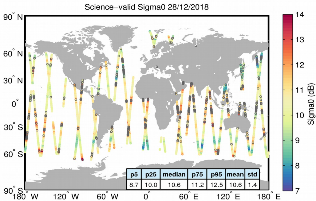
Figure 27. Geographical distribution of science-valid sigma0 data over oceans and lakes for 28/12/2018. The statistical values shown in the table refer to the sigma0 in dB and are calculated over all measurements shown in the figure. Gray circles denote records that have been rejected based on the editing criteria described in Table 4.
