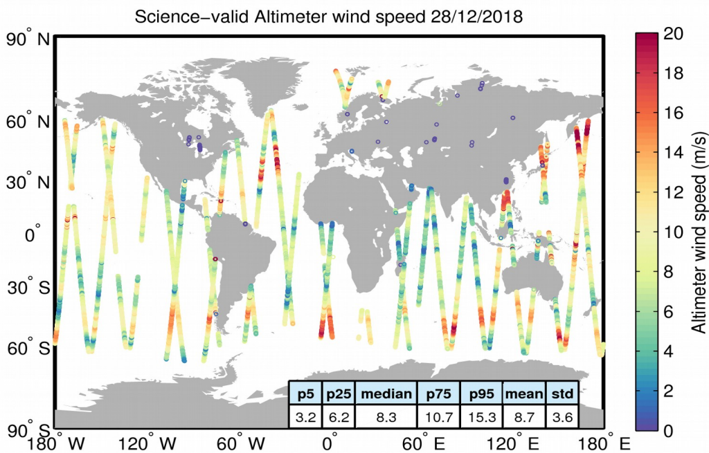
Figure 34. Geographical distribution of science-valid wind data over oceans and lakes for 28/12/2018. The statistical values shown in the table refer to the wind in m/s and are calculated over all measurements shown in the figure. Gray circles denote records that have been rejected based on the editing criteria described in Table 5.
