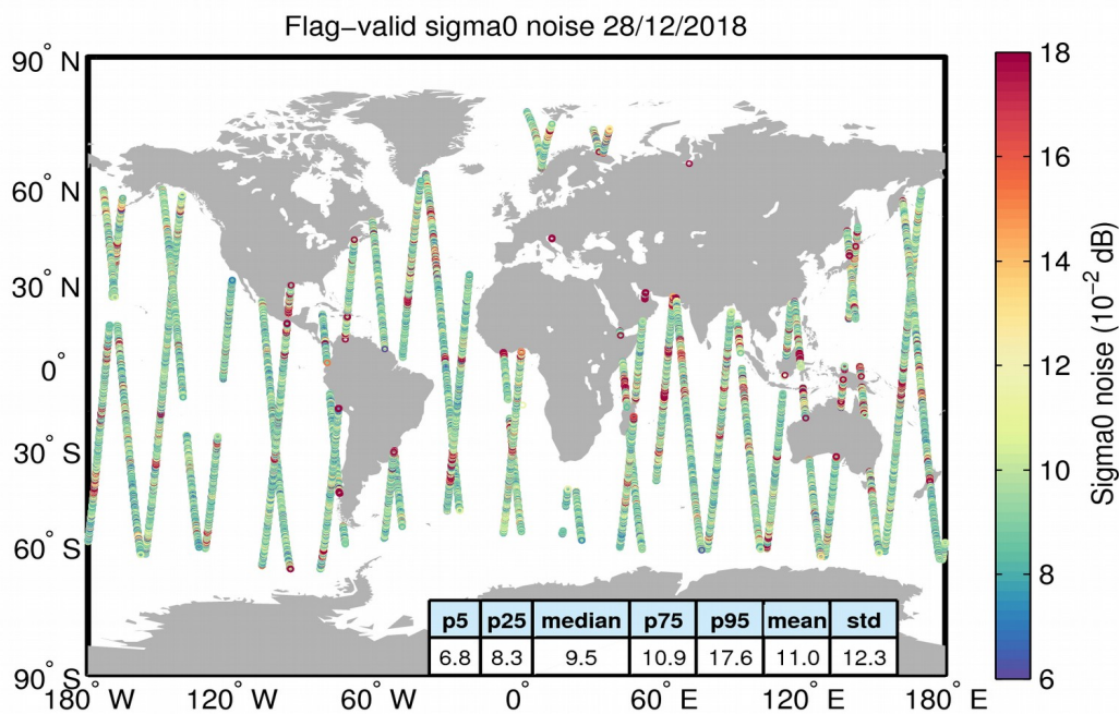
Figure 26. Geographical distribution of flag-valid 20-Hz sigma0 measurement noise over oceans and lakes for 28/12/2018. The statistical values shown in the table refer to the sigma0 noise and are calculated over all measurements shown in the figure.
