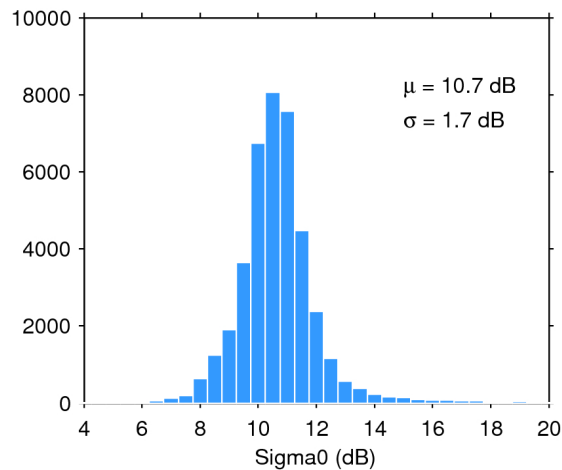
Figure 25. Histogram of flag-valid sigma0 over oceans and lakes for 28/12/2018. The mean ( \mu ) and standard deviation ( \sigma ) are also shown. Note that values outside [4 20] dB are excluded from the histogram for the sake of readability but not from the computation of \mu and \sigma .
