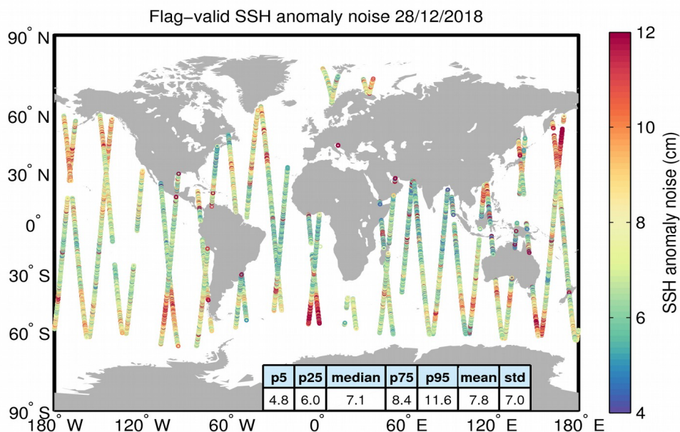
Figure 8. Geographical distribution of flag-valid 20-Hz SSH anomaly measurement noise over oceans and lakes for 28/12/2018. The statistical values shown in the table refer to the SSH anomaly noise and are calculated over all measurements shown in the figure.
