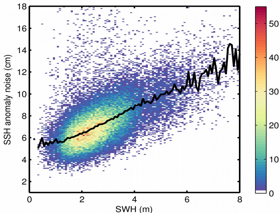
Figure 9. 2D histogram showing flag-valid SSH anomaly noise as a function of SWH for 28/12/2018. The black line denotes the median SSH anomaly noise as a function of SWH.
