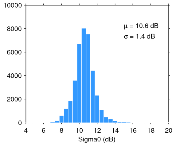
Figure 28. Histogram of science-valid sigma0 over oceans and lakes for 28/12/2018. The mean ( \mu ) and standard deviation ( \sigma ) are also shown. Note that values outside [4 20] dB are excluded from the histogram for the sake of readability but not from the computation of \mu and \sigma .
