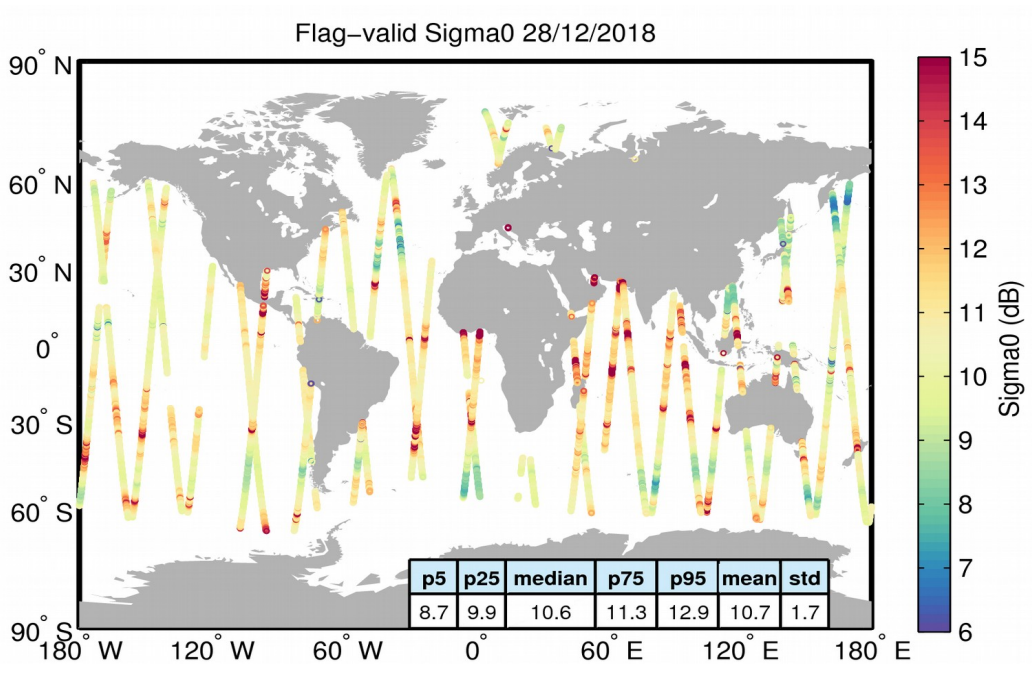
Figure 23. Geographical distribution of flag-valid sigma0 data over oceans and lakes for 28/12/2018. The statistical values shown in the table refer to the sigma0 in dB and are calculated over all measurements shown in the figure.
