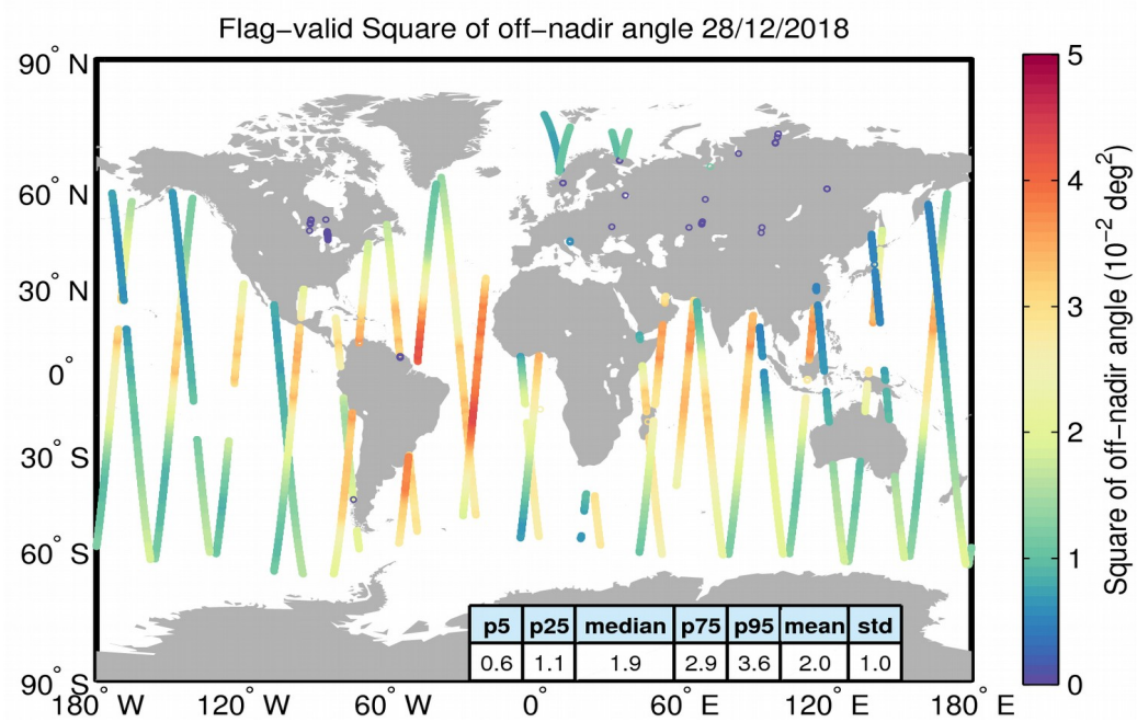
Figure 37. Geographical distribution of flag-valid mispointing data over oceans and lakes for 28/12/2018. The statistical values shown in the table refer to the mispointing in 10^{-2} \text{ deg}^2 and are calculated over all measurements shown in the figure.
