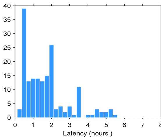
Figure 2. Histogram of the data latency for 28/12/2018. The y-axis denotes the number of files that are made available with a delay of x-hours with respect to the mean time of the records stored in the file.
