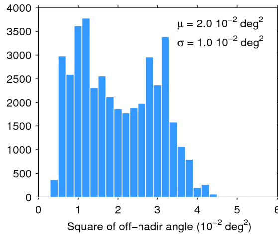
Figure 39. Histogram of flag-valid mispointing over oceans and lakes for 28/12/2018. The mean ( \mu ) and standard deviation ( \sigma ) are also shown. Note that values larger than 6 \cdot 10^{-2} \text{ deg}^2 are excluded from the histogram for the sake of readability but not from the computation of \mu and \sigma .
