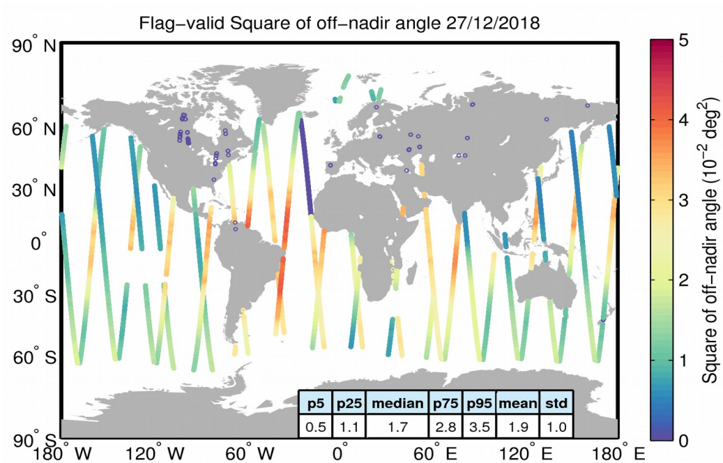
Figure 37. Geographical distribution of flag-valid mispointing data over oceans and lakes for 27/12/2018. The statistical values shown in the table refer to the mispointing in 10^{-2} deg 2 and are calculated over all measurements shown in the figure.
