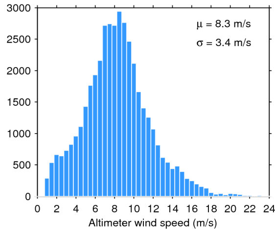
Figure 33. Histogram of flag-valid wind over oceans and lakes for 27/12/2018. The mean ( \mu ) and standard deviation ( \sigma ) are also shown. Note that values larger than 24 m/s are excluded from the histogram for the sake of readability but not from the computation of \mu and \sigma .
