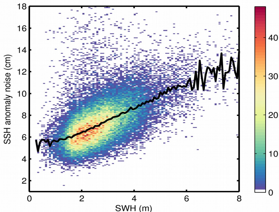
Figure 9. 2D histogram showing flag-valid SSH anomaly noise as a function of SWH for 27/12/2018. The black line denotes the median SSH anomaly noise as a function of SWH.
