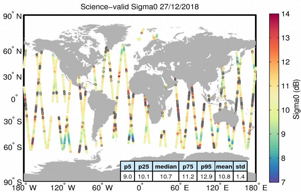
Figure 27. Geographical distribution of science-valid sigma0 data over oceans and lakes for 27/12/2018. The statistical values shown in the table refer to the sigma0 in dB and are calculated over all measurements shown in the figure. Gray circles denote records that have been rejected based on the editing criteria described in Table 4.
