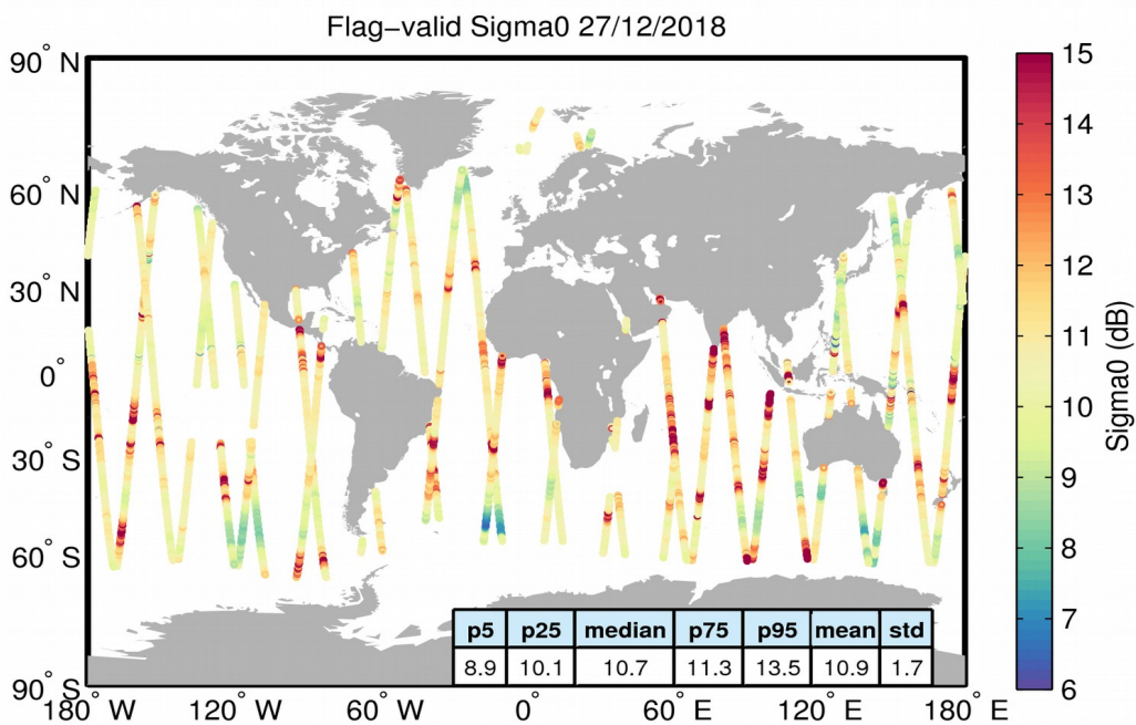
Figure 23. Geographical distribution of flag-valid sigma0 data over oceans and lakes for 27/12/2018. The statistical values shown in the table refer to the sigma0 in dB and are calculated over all measurements shown in the figure.
