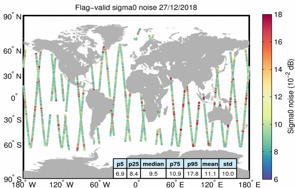
Figure 26. Geographical distribution of flag-valid 20-Hz sigma0 measurement noise over oceans and lakes for 27/12/2018. The statistical values shown in the table refer to the sigma0 noise and are calculated over all measurements shown in the figure.
