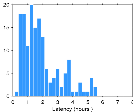
Figure 2. Histogram of the data latency for 27/12/2018. The y-axis denotes the number of files that are made available with a delay of x-hours with respect to the mean time of the records stored in the file.
