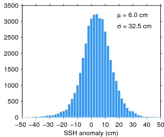
Figure 7. Histogram of flag-valid SSH anomaly over oceans and lakes for 27/12/2018. The mean ( \mu ) and standard deviation ( \sigma ) are also shown. Note that values outside [-50 50] cm are excluded from the histogram for the sake of readability but not from the computation of \mu and \sigma .
