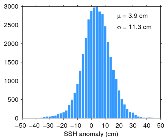
Figure 11. Histogram of science-valid SSH anomaly over oceans and lakes for 27/12/2018. The mean ( \mu ) and standard deviation ( \sigma ) are also shown. Note that values outside [-50 50] cm are excluded from the histogram for the sake of readability but not from the computation of \mu and \sigma .
