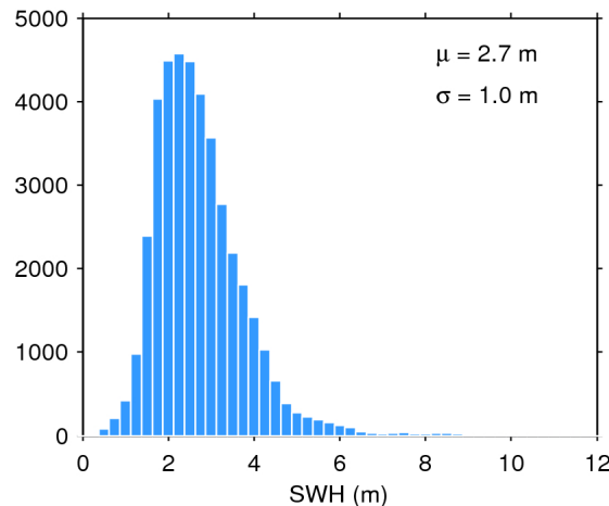
Figure 20. Histogram of science-valid SWH over oceans and lakes for 27/12/2018. The mean ( \mu ) and standard deviation ( \sigma ) are also shown. Note that values larger than 12 m are excluded from the histogram for the sake of readability but not from the computation of \mu and \sigma .
