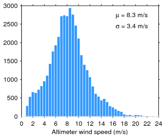
Figure 35. Histogram of science-valid wind over oceans and lakes for 27/12/2018. The mean ( \mu ) and standard deviation ( \sigma ) are also shown. Note that values larger than 24 m/s are excluded from the histogram for the sake of readability but not from the computation of \mu and \sigma .
