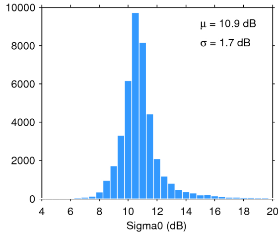
Figure 25. Histogram of flag-valid sigma0 over oceans and lakes for 27/12/2018. The mean ( \mu ) and standard deviation ( \sigma ) are also shown. Note that values outside [4 20] dB are excluded from the histogram for the sake of readability but not from the computation of \mu and \sigma .
