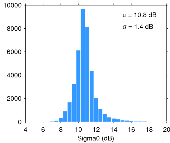
Figure 28. Histogram of science-valid sigma0 over oceans and lakes for 27/12/2018. The mean ( \mu ) and standard deviation ( \sigma ) are also shown. Note that values outside [4 20] dB are excluded from the histogram for the sake of readability but not from the computation of \mu and \sigma .
