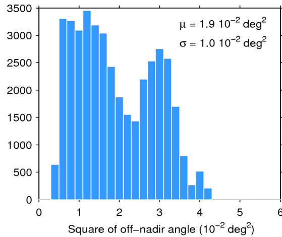
Figure 39. Histogram of flag-valid mispointing over oceans and lakes for 27/12/2018. The mean ( \mu ) and standard deviation ( \sigma ) are also shown. Note that values larger than 6 \cdot 10^{-2} \text{ deg}^2 are excluded from the histogram for the sake of readability but not from the computation of \mu and \sigma .
