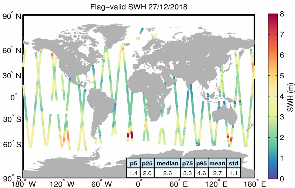
Figure 15. Geographical distribution of flag-valid SWH data over oceans and lakes for 27/12/2018. The statistical values shown in the table refer to the SWH in m and are calculated over all measurements shown in the figure.
