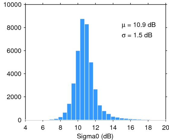
Figure 25. Histogram of flag-valid sigma0 over oceans and lakes for 26/12/2018. The mean ( \mu ) and standard deviation ( \sigma ) are also shown. Note that values outside [4 20] dB are excluded from the histogram for the sake of readability but not from the computation of \mu and \sigma .
