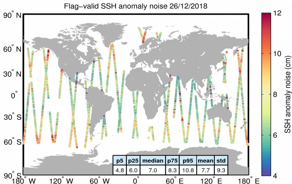
Figure 8. Geographical distribution of flag-valid 20-Hz SSH anomaly measurement noise over oceans and lakes for 26/12/2018. The statistical values shown in the table refer to the SSH anomaly noise and are calculated over all measurements shown in the figure.
