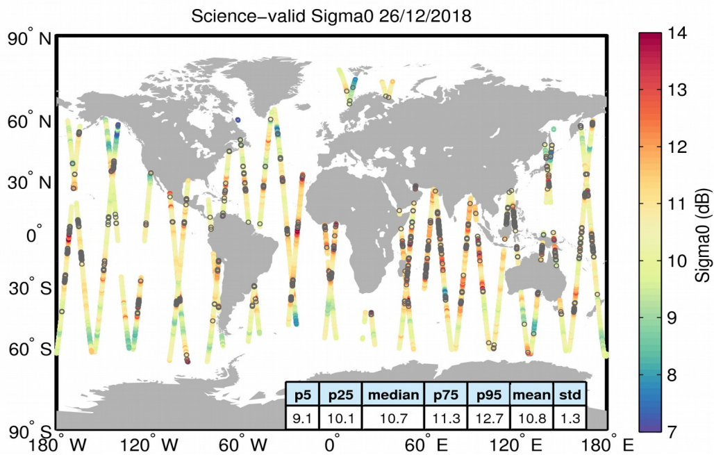
Figure 27. Geographical distribution of science-valid sigma0 data over oceans and lakes for 26/12/2018. The statistical values shown in the table refer to the sigma0 in dB and are calculated over all measurements shown in the figure. Gray circles denote records that have been rejected based on the editing criteria described in Table 4.
