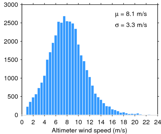
Figure 33. Histogram of flag-valid wind over oceans and lakes for 26/12/2018. The mean ( \mu ) and standard deviation ( \sigma ) are also shown. Note that values larger than 24 m/s are excluded from the histogram for the sake of readability but not from the computation of \mu and \sigma .
