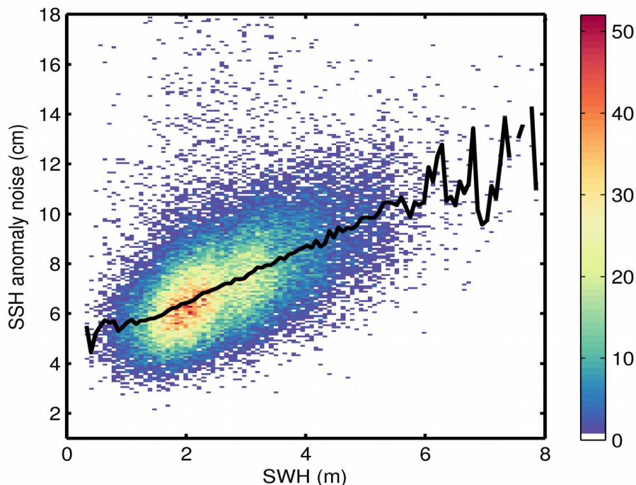
Figure 9. 2D histogram showing flag-valid SSH anomaly noise as a function of SWH for 26/12/2018. The black line denotes the median SSH anomaly noise as a function of SWH.
