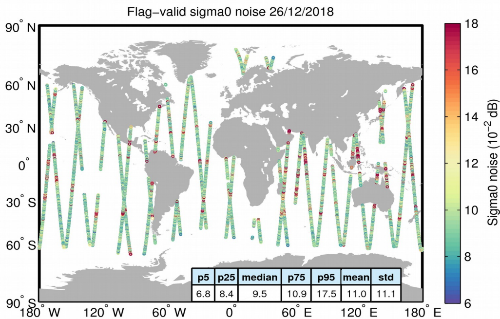
Figure 26. Geographical distribution of flag-valid 20-Hz sigma0 measurement noise over oceans and lakes for 26/12/2018. The statistical values shown in the table refer to the sigma0 noise and are calculated over all measurements shown in the figure.
