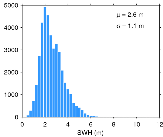
Figure 17. Histogram of flag-valid SWH over oceans and lakes for 26/12/2018. The mean ( \mu ) and standard deviation ( \sigma ) are also shown. Note that values larger than 12 m are excluded from the histogram for the sake of readability but not from the computation of \mu and \sigma .
