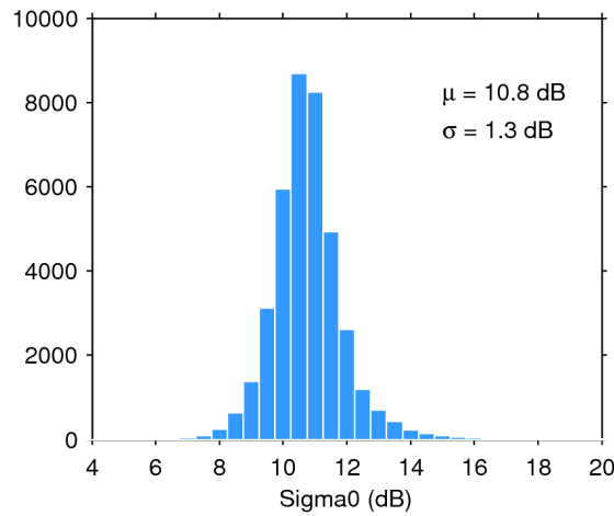
Figure 28. Histogram of science-valid sigma0 over oceans and lakes for 26/12/2018. The mean ( \mu ) and standard deviation ( \sigma ) are also shown. Note that values outside [4 20] dB are excluded from the histogram for the sake of readability but not from the computation of \mu and \sigma .
