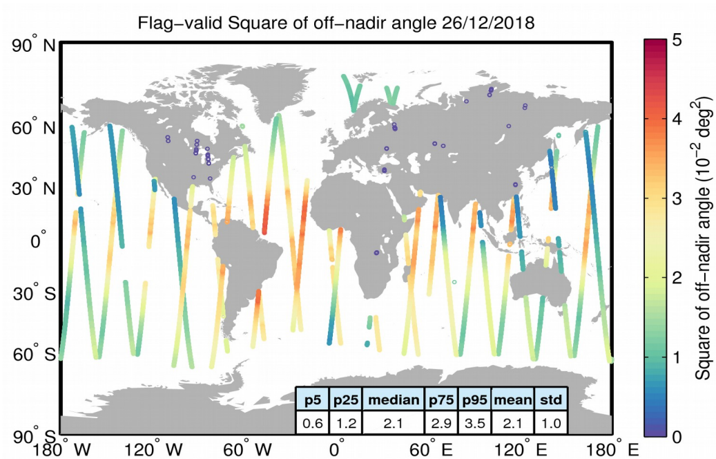
Figure 37. Geographical distribution of flag-valid mispointing data over oceans and lakes for 26/12/2018. The statistical values shown in the table refer to the mispointing in 10^{-2} deg 2 and are calculated over all measurements shown in the figure.
