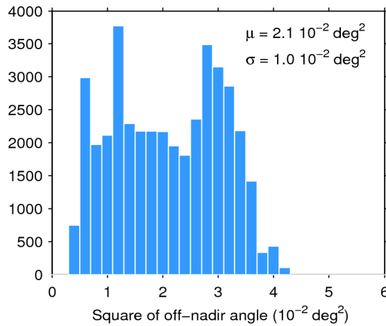
Figure 39. Histogram of flag-valid mispointing over oceans and lakes for 26/12/2018. The mean ( \mu ) and standard deviation ( \sigma ) are also shown. Note that values larger than 6 \cdot 10^{-2} \text{ deg}^2 are excluded from the histogram for the sake of readability but not from the computation of \mu and \sigma .
