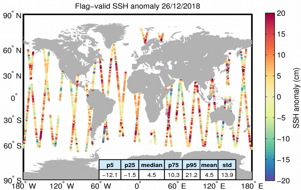
Figure 5. Geographical distribution of flag-valid 1-Hz SSH anomaly data over oceans and lakes for 26/12/2018. The statistical values shown in the table refer to the SSH anomaly in cm and are calculated over all measurements shown in the figure.
