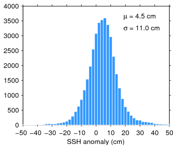
Figure 11. Histogram of science-valid SSH anomaly over oceans and lakes for 26/12/2018. The mean ( \mu ) and standard deviation ( \sigma ) are also shown. Note that values outside [-50 50] cm are excluded from the histogram for the sake of readability but not from the computation of \mu and \sigma .
