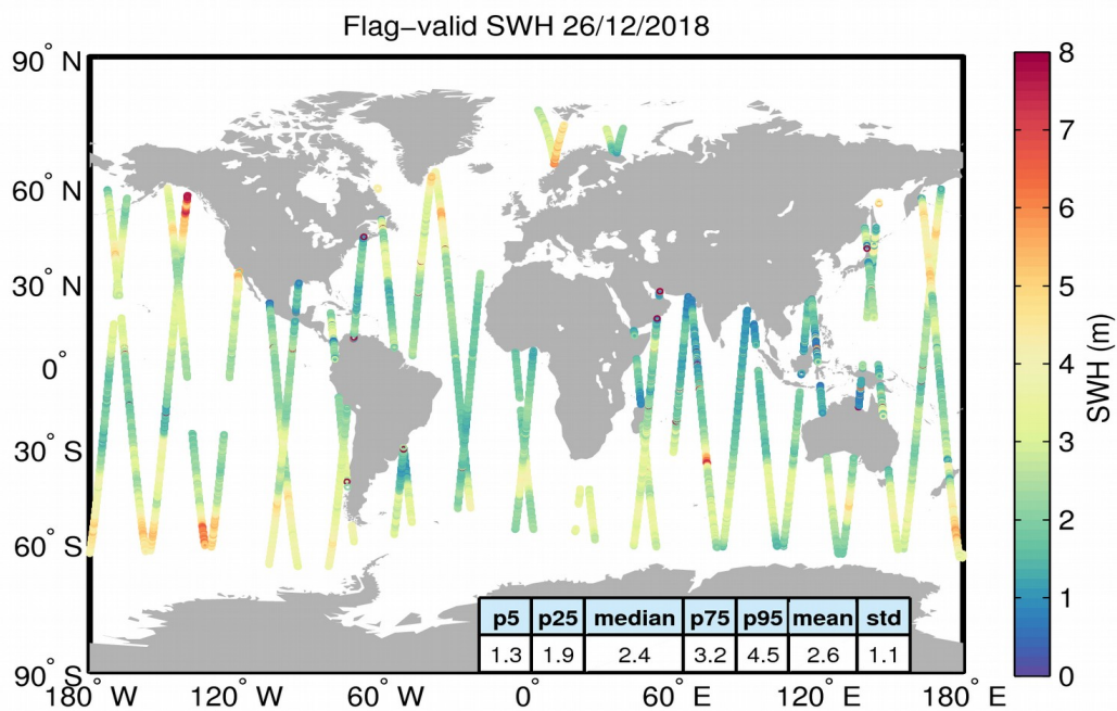
Figure 15. Geographical distribution of flag-valid SWH data over oceans and lakes for 26/12/2018. The statistical values shown in the table refer to the SWH in m and are calculated over all measurements shown in the figure.
