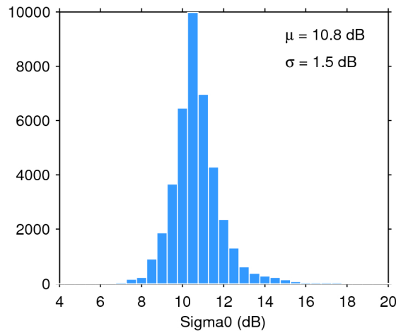
Figure 28. Histogram of science-valid sigma0 over oceans and lakes for 25/12/2018. The mean ( \mu ) and standard deviation ( \sigma ) are also shown. Note that values outside [4 20] dB are excluded from the histogram for the sake of readability but not from the computation of \mu and \sigma .
