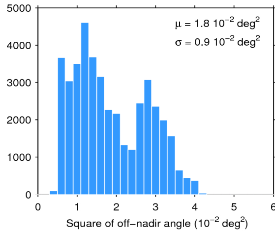
Figure 39. Histogram of flag-valid mispointing over oceans and lakes for 25/12/2018. The mean ( \mu ) and standard deviation ( \sigma ) are also shown. Note that values larger than 6 \cdot 10^{-2} \text{ deg}^2 are excluded from the histogram for the sake of readability but not from the computation of \mu and \sigma .
