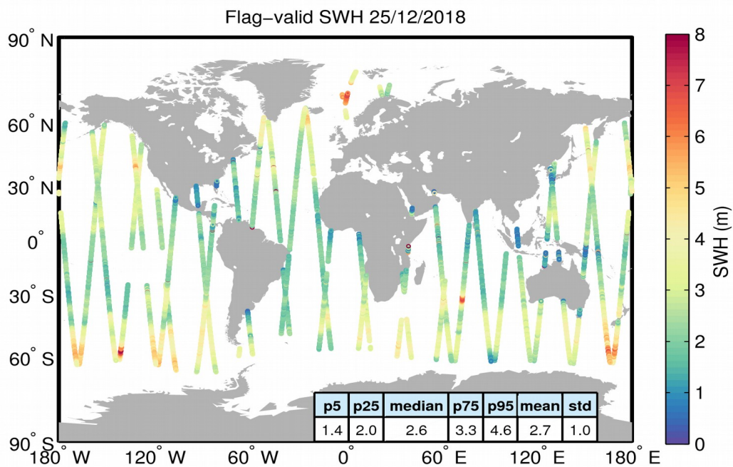
Figure 15. Geographical distribution of flag-valid SWH data over oceans and lakes for 25/12/2018. The statistical values shown in the table refer to the SWH in m and are calculated over all measurements shown in the figure.
