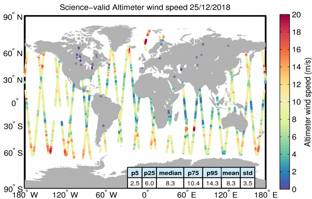
Figure 34. Geographical distribution of science-valid wind data over oceans and lakes for 25/12/2018. The statistical values shown in the table refer to the wind in m/s and are calculated over all measurements shown in the figure. Gray circles denote records that have been rejected based on the editing criteria described in Table 5.
