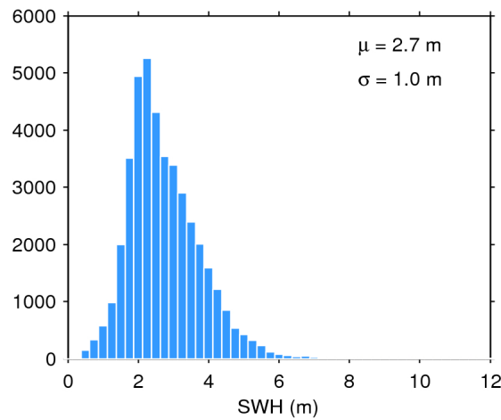
Figure 17. Histogram of flag-valid SWH over oceans and lakes for 25/12/2018. The mean ( \mu ) and standard deviation ( \sigma ) are also shown. Note that values larger than 12 m are excluded from the histogram for the sake of readability but not from the computation of \mu and \sigma .
