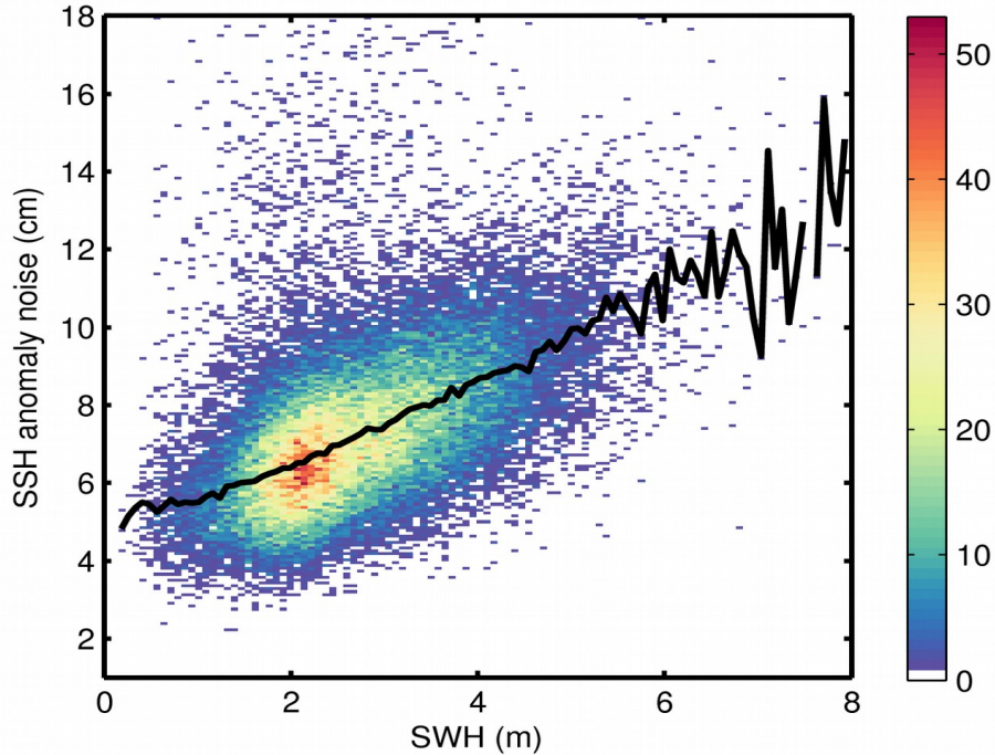
Figure 9. 2D histogram showing flag-valid SSH anomaly noise as a function of SWH for 25/12/2018. The black line denotes the median SSH anomaly noise as a function of SWH.
