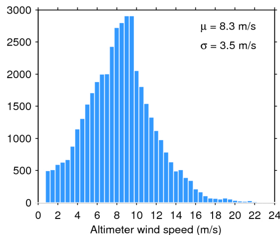
Figure 35. Histogram of science-valid wind over oceans and lakes for 25/12/2018. The mean ( \mu ) and standard deviation ( \sigma ) are also shown. Note that values larger than 24 m/s are excluded from the histogram for the sake of readability but not from the computation of \mu and \sigma .
