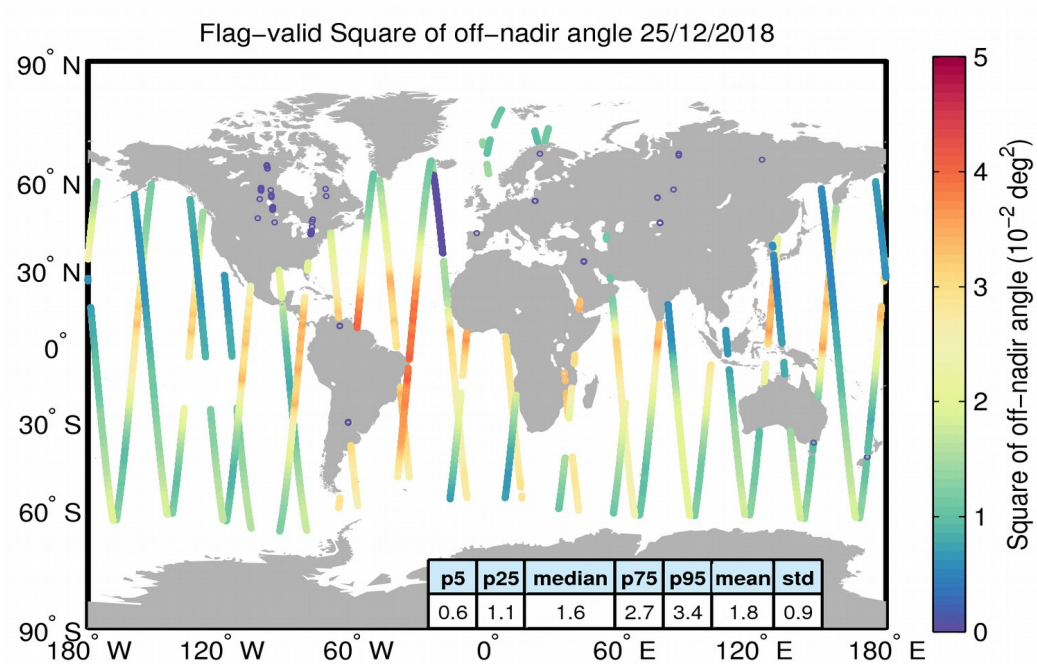
Figure 37. Geographical distribution of flag-valid mispointing data over oceans and lakes for 25/12/2018. The statistical values shown in the table refer to the mispointing in 10^{-2} deg 2 and are calculated over all measurements shown in the figure.
