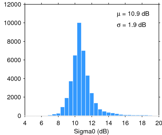
Figure 25. Histogram of flag-valid sigma0 over oceans and lakes for 25/12/2018. The mean ( \mu ) and standard deviation ( \sigma ) are also shown. Note that values outside [4 20] dB are excluded from the histogram for the sake of readability but not from the computation of \mu and \sigma .
