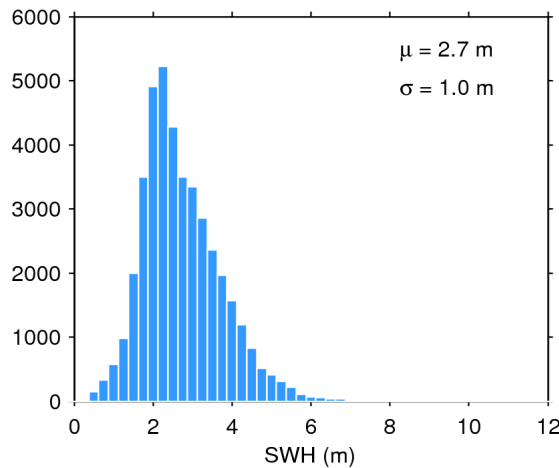
Figure 20. Histogram of science-valid SWH over oceans and lakes for 25/12/2018. The mean ( \mu ) and standard deviation ( \sigma ) are also shown. Note that values larger than 12 m are excluded from the histogram for the sake of readability but not from the computation of \mu and \sigma .
