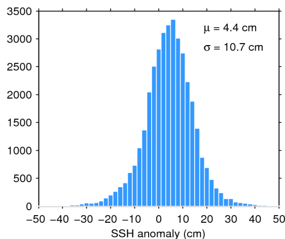
Figure 11. Histogram of science-valid SSH anomaly over oceans and lakes for 25/12/2018. The mean ( \mu ) and standard deviation ( \sigma ) are also shown. Note that values outside [-50 50] cm are excluded from the histogram for the sake of readability but not from the computation of \mu and \sigma .
