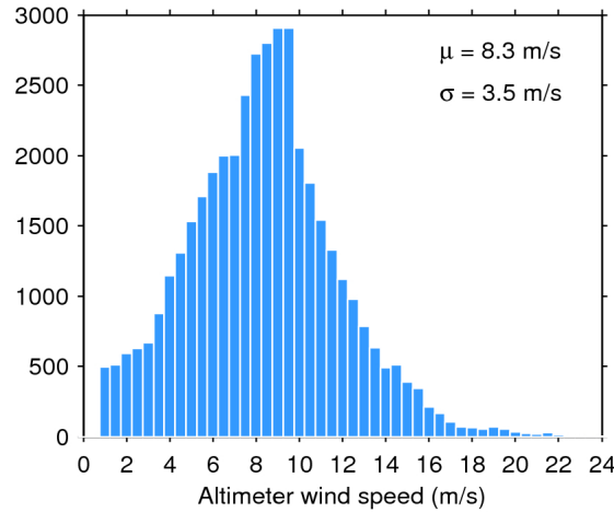
Figure 33. Histogram of flag-valid wind over oceans and lakes for 25/12/2018. The mean ( \mu ) and standard deviation ( \sigma ) are also shown. Note that values larger than 24 m/s are excluded from the histogram for the sake of readability but not from the computation of \mu and \sigma .
