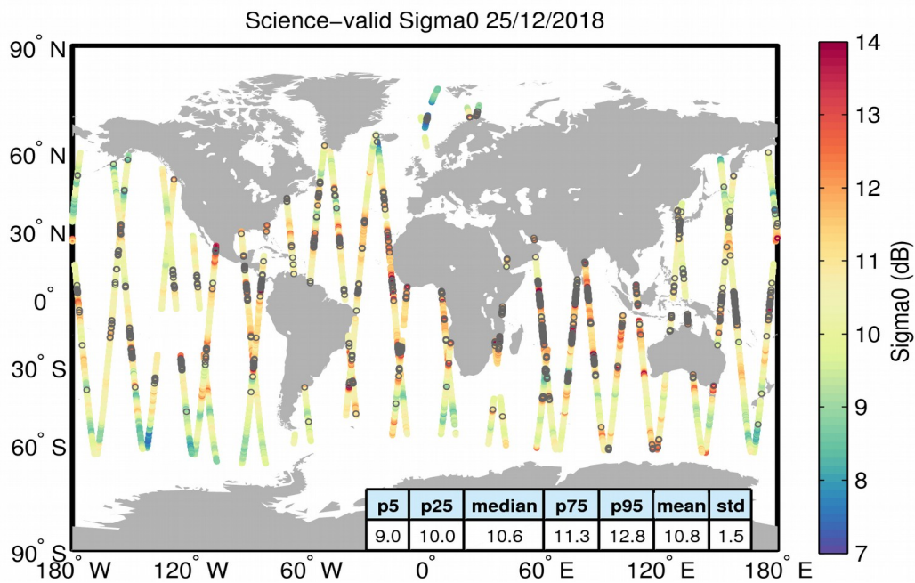
Figure 27. Geographical distribution of science-valid sigma0 data over oceans and lakes for 25/12/2018. The statistical values shown in the table refer to the sigma0 in dB and are calculated over all measurements shown in the figure. Gray circles denote records that have been rejected based on the editing criteria described in Table 4.
