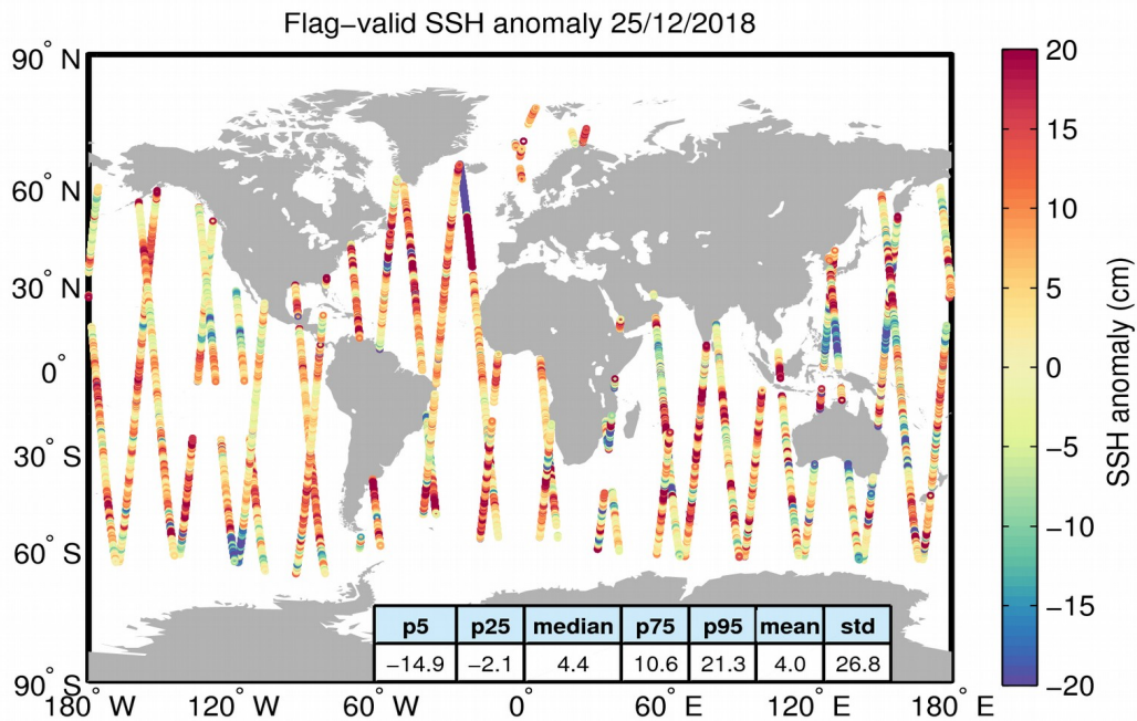
Figure 5. Geographical distribution of flag-valid 1-Hz SSH anomaly data over oceans and lakes for 25/12/2018. The statistical values shown in the table refer to the SSH anomaly in cm and are calculated over all measurements shown in the figure.
