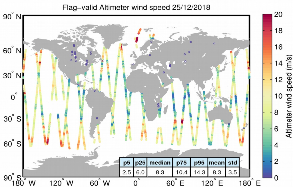
Figure 31. Geographical distribution of flag-valid wind data over oceans and lakes for 25/12/2018. The statistical values shown in the table refer to the wind in m/s and are calculated over all measurements shown in the figure.
