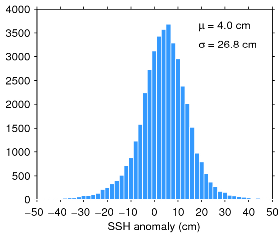
Figure 7. Histogram of flag-valid SSH anomaly over oceans and lakes for 25/12/2018. The mean ( \mu ) and standard deviation ( \sigma ) are also shown. Note that values outside [-50 50] cm are excluded from the histogram for the sake of readability but not from the computation of \mu and \sigma .
