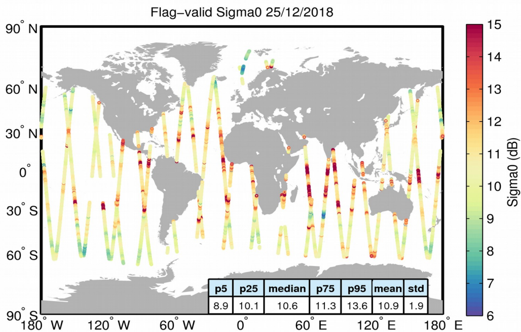
Figure 23. Geographical distribution of flag-valid sigma0 data over oceans and lakes for 25/12/2018. The statistical values shown in the table refer to the sigma0 in dB and are calculated over all measurements shown in the figure.
