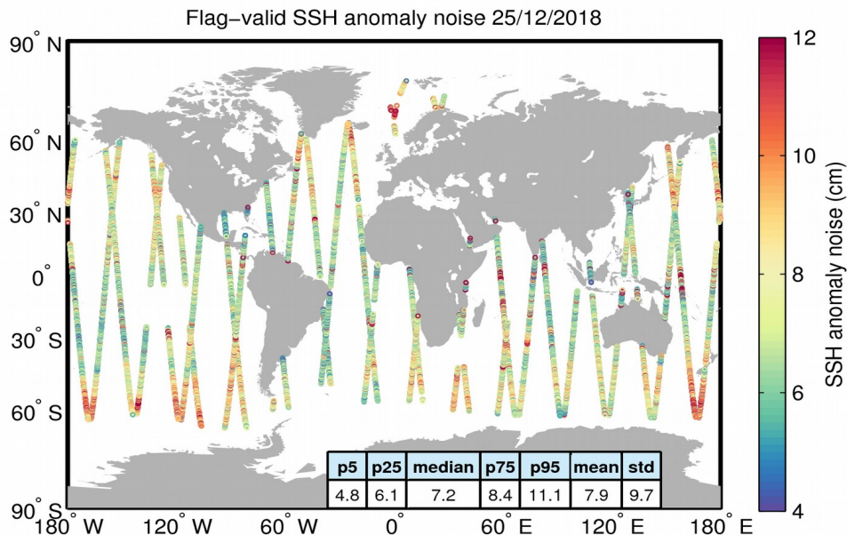
Figure 8. Geographical distribution of flag-valid 20-Hz SSH anomaly measurement noise over oceans and lakes for 25/12/2018. The statistical values shown in the table refer to the SSH anomaly noise and are calculated over all measurements shown in the figure.
