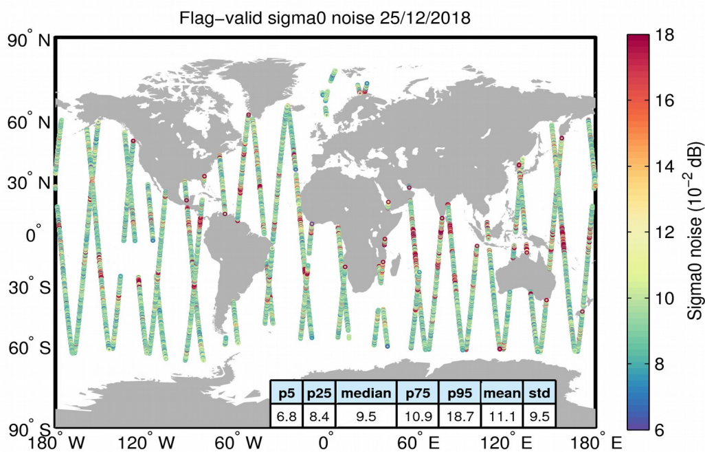
Figure 26. Geographical distribution of flag-valid 20-Hz sigma0 measurement noise over oceans and lakes for 25/12/2018. The statistical values shown in the table refer to the sigma0 noise and are calculated over all measurements shown in the figure.
