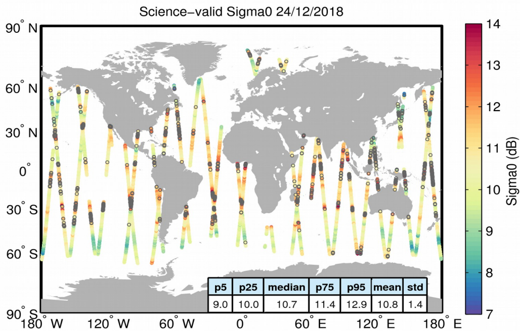
Figure 27. Geographical distribution of science-valid sigma0 data over oceans and lakes for 24/12/2018. The statistical values shown in the table refer to the sigma0 in dB and are calculated over all measurements shown in the figure. Gray circles denote records that have been rejected based on the editing criteria described in Table 4.
