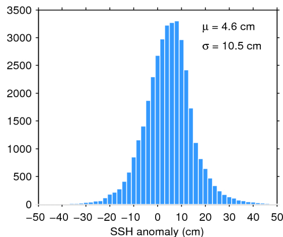
Figure 11. Histogram of science-valid SSH anomaly over oceans and lakes for 24/12/2018. The mean ( \mu ) and standard deviation ( \sigma ) are also shown. Note that values outside [-50 50] cm are excluded from the histogram for the sake of readability but not from the computation of \mu and \sigma .
