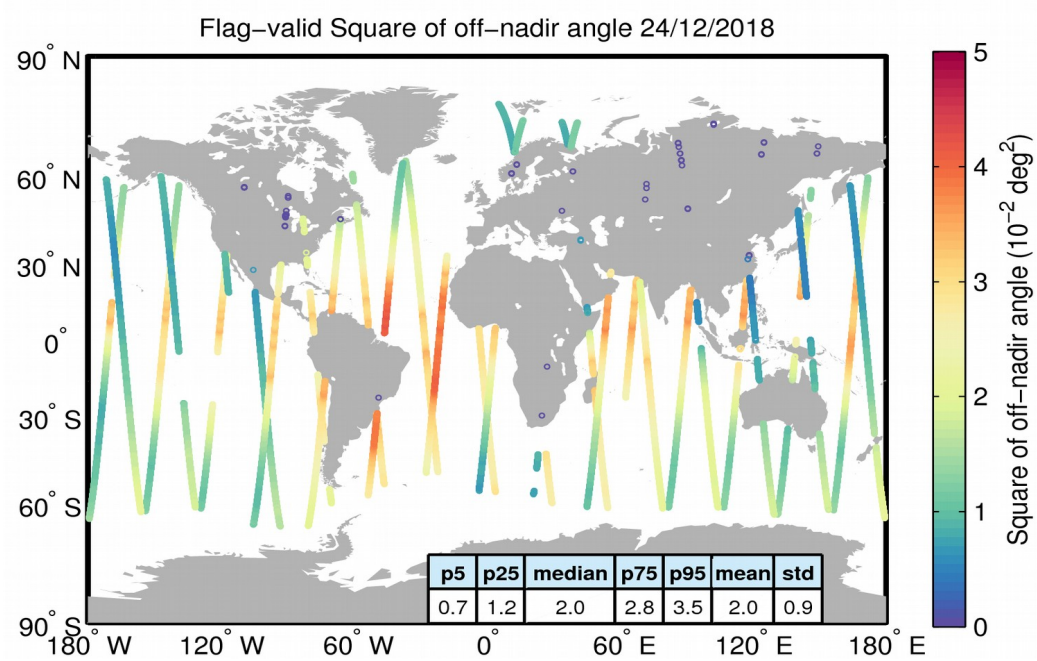
Figure 37. Geographical distribution of flag-valid mispointing data over oceans and lakes for 24/12/2018. The statistical values shown in the table refer to the mispointing in 10^{-2} \text{ deg}^2 and are calculated over all measurements shown in the figure.
