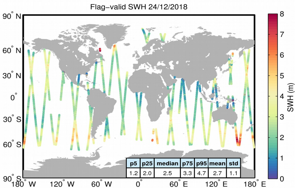
Figure 15. Geographical distribution of flag-valid SWH data over oceans and lakes for 24/12/2018. The statistical values shown in the table refer to the SWH in m and are calculated over all measurements shown in the figure.
