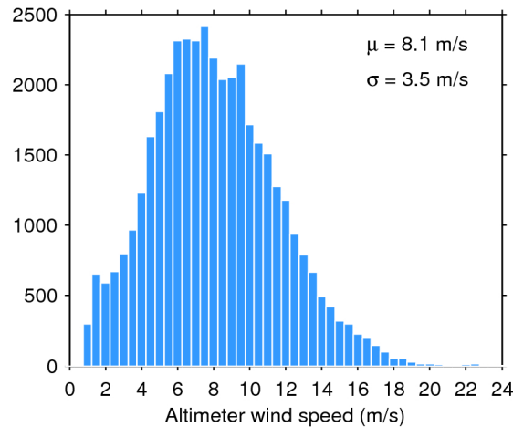
Figure 33. Histogram of flag-valid wind over oceans and lakes for 24/12/2018. The mean ( \mu ) and standard deviation ( \sigma ) are also shown. Note that values larger than 24 m/s are excluded from the histogram for the sake of readability but not from the computation of \mu and \sigma .
