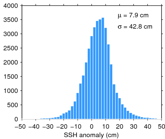
Figure 7. Histogram of flag-valid SSH anomaly over oceans and lakes for 24/12/2018. The mean ( \mu ) and standard deviation ( \sigma ) are also shown. Note that values outside [-50 50] cm are excluded from the histogram for the sake of readability but not from the computation of \mu and \sigma .
