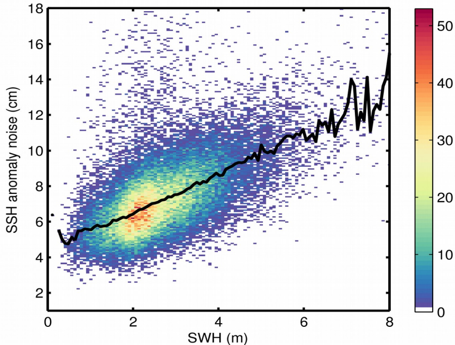
Figure 9. 2D histogram showing flag-valid SSH anomaly noise as a function of SWH for 24/12/2018. The black line denotes the median SSH anomaly noise as a function of SWH.
