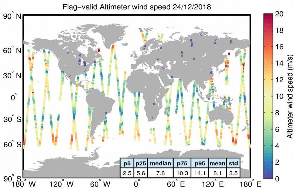
Figure 31. Geographical distribution of flag-valid wind data over oceans and lakes for 24/12/2018. The statistical values shown in the table refer to the wind in m/s and are calculated over all measurements shown in the figure.
