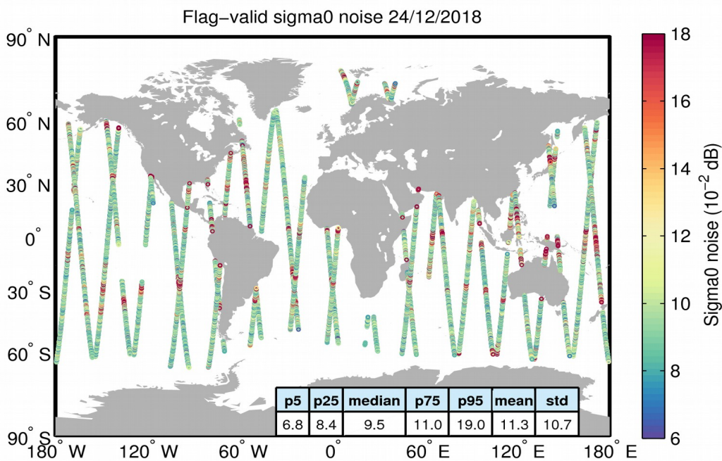
Figure 26. Geographical distribution of flag-valid 20-Hz sigma0 measurement noise over oceans and lakes for 24/12/2018. The statistical values shown in the table refer to the sigma0 noise and are calculated over all measurements shown in the figure.
