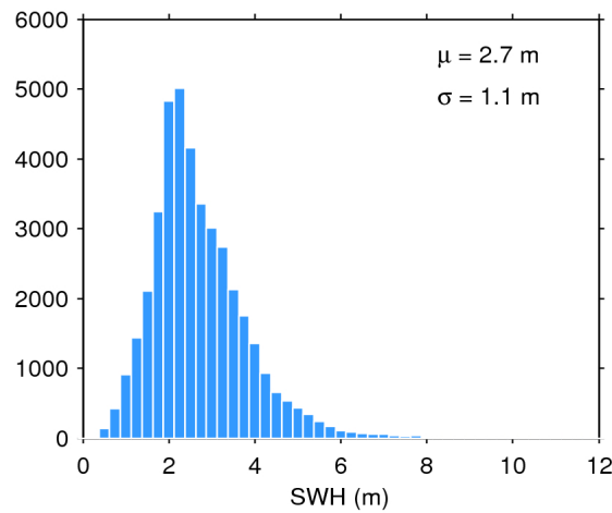
Figure 17. Histogram of flag-valid SWH over oceans and lakes for 24/12/2018. The mean ( \mu ) and standard deviation ( \sigma ) are also shown. Note that values larger than 12 m are excluded from the histogram for the sake of readability but not from the computation of \mu and \sigma .
