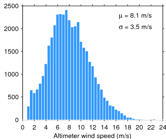
Figure 35. Histogram of science-valid wind over oceans and lakes for 24/12/2018. The mean ( \mu ) and standard deviation ( \sigma ) are also shown. Note that values larger than 24 m/s are excluded from the histogram for the sake of readability but not from the computation of \mu and \sigma .
