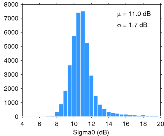
Figure 25. Histogram of flag-valid sigma0 over oceans and lakes for 24/12/2018. The mean ( \mu ) and standard deviation ( \sigma ) are also shown. Note that values outside [4 20] dB are excluded from the histogram for the sake of readability but not from the computation of \mu and \sigma .
