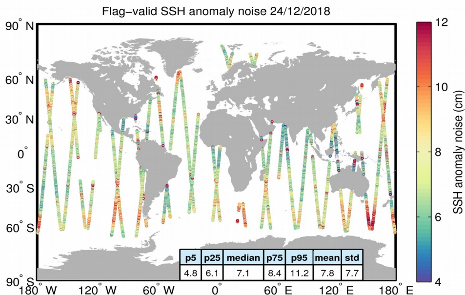
Figure 8. Geographical distribution of flag-valid 20-Hz SSH anomaly measurement noise over oceans and lakes for 24/12/2018. The statistical values shown in the table refer to the SSH anomaly noise and are calculated over all measurements shown in the figure.
