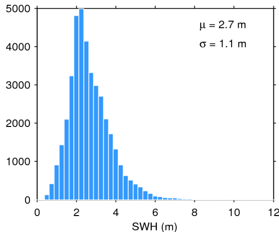
Figure 20. Histogram of science-valid SWH over oceans and lakes for 24/12/2018. The mean ( \mu ) and standard deviation ( \sigma ) are also shown. Note that values larger than 12 m are excluded from the histogram for the sake of readability but not from the computation of \mu and \sigma .
