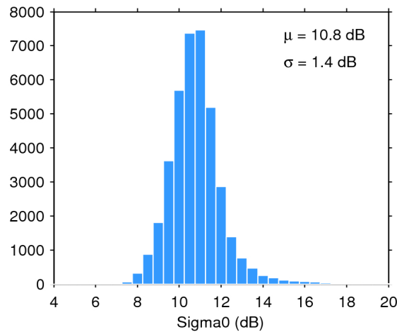
Figure 28. Histogram of science-valid sigma0 over oceans and lakes for 24/12/2018. The mean ( \mu ) and standard deviation ( \sigma ) are also shown. Note that values outside [4 20] dB are excluded from the histogram for the sake of readability but not from the computation of \mu and \sigma .
