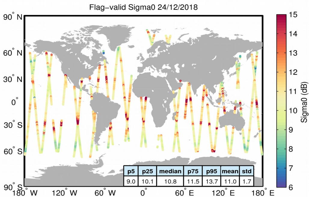
Figure 23. Geographical distribution of flag-valid sigma0 data over oceans and lakes for 24/12/2018. The statistical values shown in the table refer to the sigma0 in dB and are calculated over all measurements shown in the figure.
