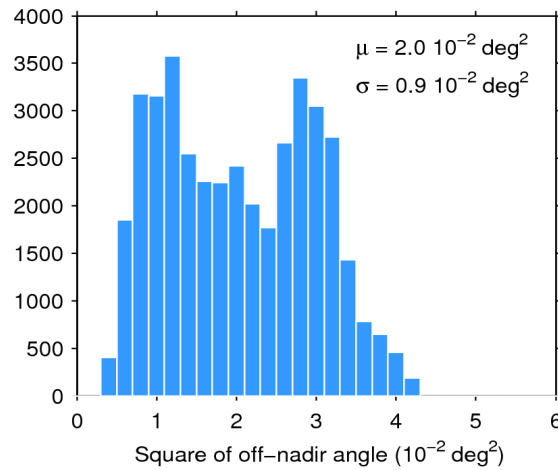
Figure 39. Histogram of flag-valid mispointing over oceans and lakes for 24/12/2018. The mean ( \mu ) and standard deviation ( \sigma ) are also shown. Note that values larger than 6 \cdot 10^{-2} \text{ deg}^2 are excluded from the histogram for the sake of readability but not from the computation of \mu and \sigma .
