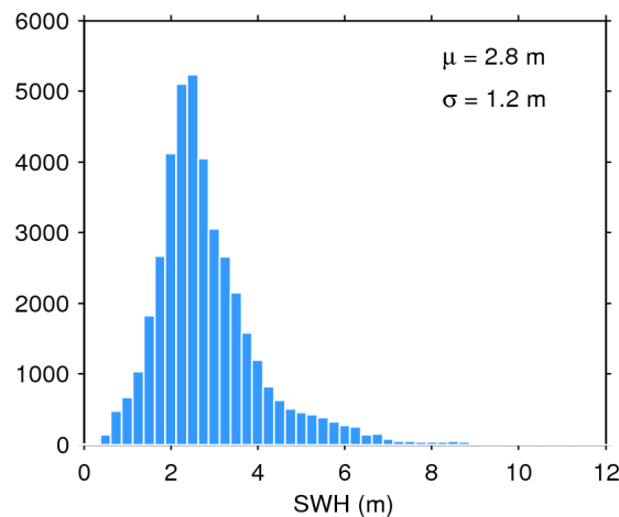
Figure 20. Histogram of science-valid SWH over oceans and lakes for 23/12/2018. The mean ( \mu ) and standard deviation ( \sigma ) are also shown. Note that values larger than 12 m are excluded from the histogram for the sake of readability but not from the computation of \mu and \sigma .
