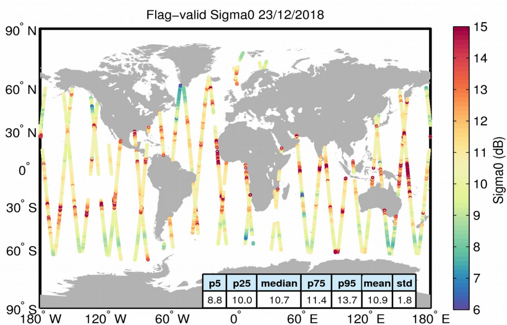
Figure 23. Geographical distribution of flag-valid sigma0 data over oceans and lakes for 23/12/2018. The statistical values shown in the table refer to the sigma0 in dB and are calculated over all measurements shown in the figure.
