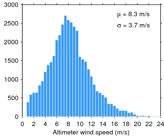
Figure 33. Histogram of flag-valid wind over oceans and lakes for 23/12/2018. The mean ( \mu ) and standard deviation ( \sigma ) are also shown. Note that values larger than 24 m/s are excluded from the histogram for the sake of readability but not from the computation of \mu and \sigma .
