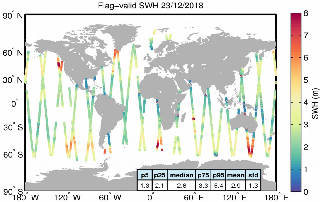
Figure 15. Geographical distribution of flag-valid SWH data over oceans and lakes for 23/12/2018. The statistical values shown in the table refer to the SWH in m and are calculated over all measurements shown in the figure.
