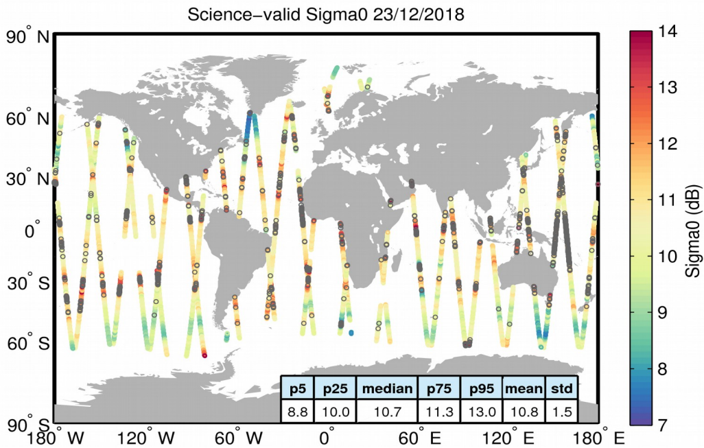
Figure 27. Geographical distribution of science-valid sigma0 data over oceans and lakes for 23/12/2018. The statistical values shown in the table refer to the sigma0 in dB and are calculated over all measurements shown in the figure. Gray circles denote records that have been rejected based on the editing criteria described in Table 4.
