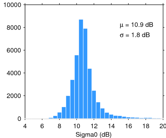
Figure 25. Histogram of flag-valid sigma0 over oceans and lakes for 23/12/2018. The mean ( \mu ) and standard deviation ( \sigma ) are also shown. Note that values outside [4 20] dB are excluded from the histogram for the sake of readability but not from the computation of \mu and \sigma .
