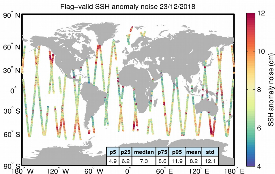
Figure 8. Geographical distribution of flag-valid 20-Hz SSH anomaly measurement noise over oceans and lakes for 23/12/2018. The statistical values shown in the table refer to the SSH anomaly noise and are calculated over all measurements shown in the figure.
