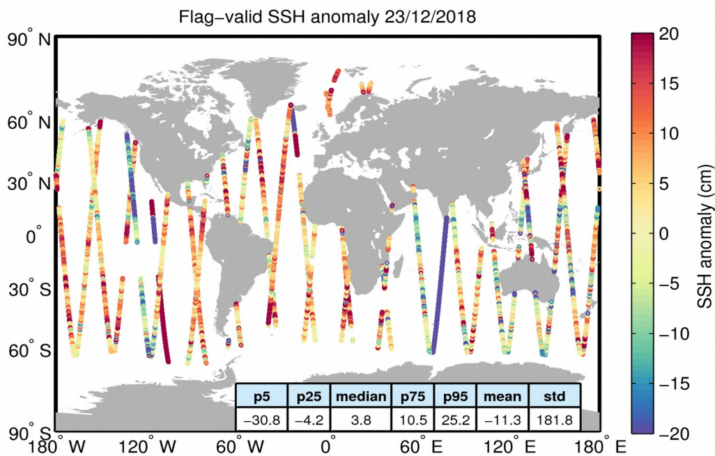
Figure 5. Geographical distribution of flag-valid 1-Hz SSH anomaly data over oceans and lakes for 23/12/2018. The statistical values shown in the table refer to the SSH anomaly in cm and are calculated over all measurements shown in the figure.
