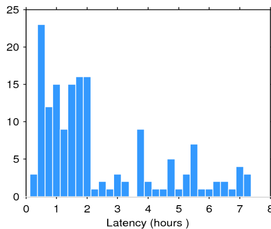
Figure 2. Histogram of the data latency for 23/12/2018. The y-axis denotes the number of files that are made available with a delay of x-hours with respect to the mean time of the records stored in the file.
