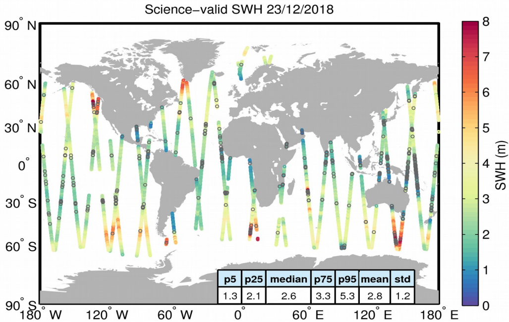
Figure 19. Geographical distribution of science-valid SWH data over oceans and lakes for 23/12/2018. The statistical values shown in the table refer to the SWH in m and are calculated over all measurements shown in the figure. Gray circles denote records that have been rejected based on the editing criteria described in Table 3.
