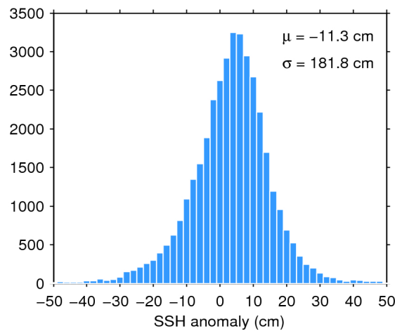
Figure 7. Histogram of flag-valid SSH anomaly over oceans and lakes for 23/12/2018. The mean ( \mu ) and standard deviation ( \sigma ) are also shown. Note that values outside [-50 50] cm are excluded from the histogram for the sake of readability but not from the computation of \mu and \sigma .
