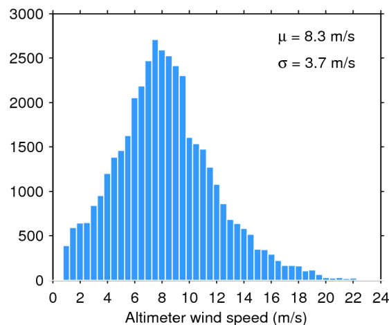
Figure 35. Histogram of science-valid wind over oceans and lakes for 23/12/2018. The mean ( \mu ) and standard deviation ( \sigma ) are also shown. Note that values larger than 24 m/s are excluded from the histogram for the sake of readability but not from the computation of \mu and \sigma .
