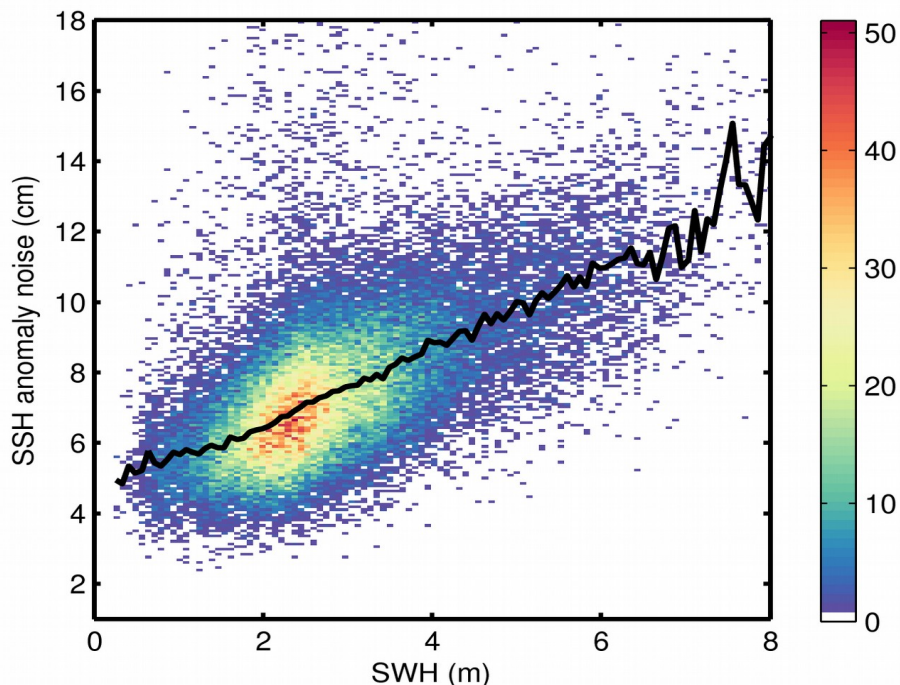
Figure 9. 2D histogram showing flag-valid SSH anomaly noise as a function of SWH for 23/12/2018. The black line denotes the median SSH anomaly noise as a function of SWH.
