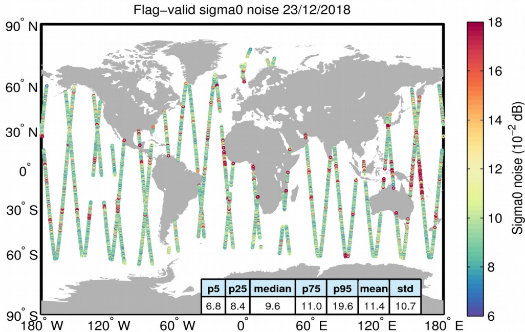
Figure 26. Geographical distribution of flag-valid 20-Hz sigma0 measurement noise over oceans and lakes for 23/12/2018. The statistical values shown in the table refer to the sigma0 noise and are calculated over all measurements shown in the figure.
