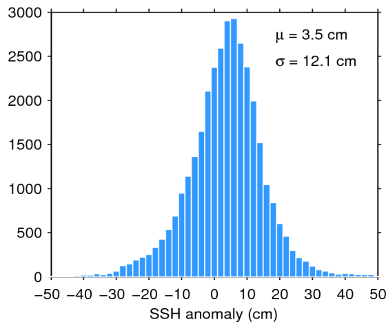
Figure 11. Histogram of science-valid SSH anomaly over oceans and lakes for 23/12/2018. The mean ( \mu ) and standard deviation ( \sigma ) are also shown. Note that values outside [-50 50] cm are excluded from the histogram for the sake of readability but not from the computation of \mu and \sigma .
