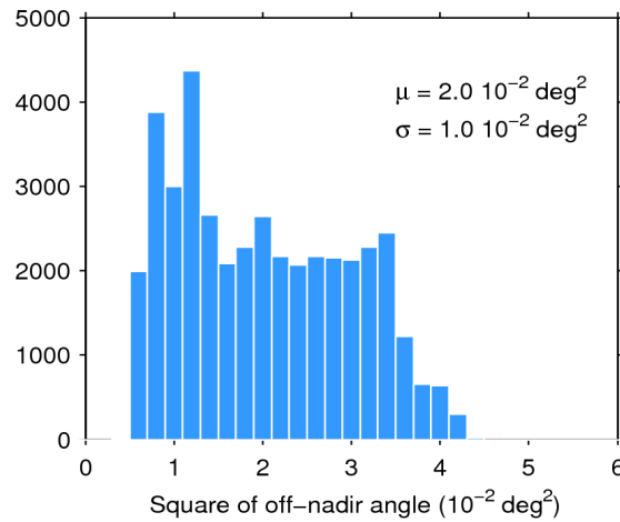
Figure 39. Histogram of flag-valid mispointing over oceans and lakes for 23/12/2018. The mean ( \mu ) and standard deviation ( \sigma ) are also shown. Note that values larger than 6 \cdot 10^{-2} \text{ deg}^2 are excluded from the histogram for the sake of readability but not from the computation of \mu and \sigma .
