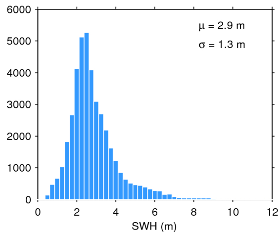
Figure 17. Histogram of flag-valid SWH over oceans and lakes for 23/12/2018. The mean ( \mu ) and standard deviation ( \sigma ) are also shown. Note that values larger than 12 m are excluded from the histogram for the sake of readability but not from the computation of \mu and \sigma .
