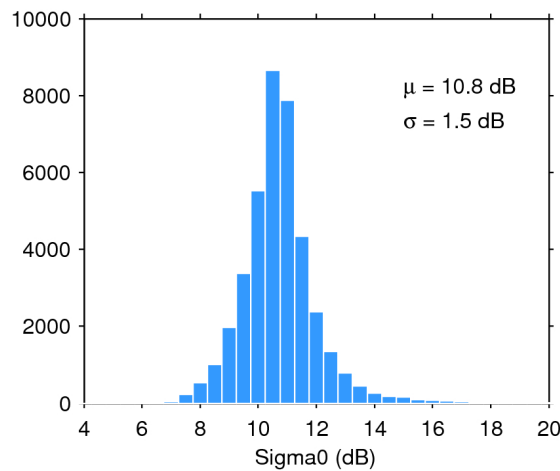
Figure 28. Histogram of science-valid sigma0 over oceans and lakes for 23/12/2018. The mean ( \mu ) and standard deviation ( \sigma ) are also shown. Note that values outside [4 20] dB are excluded from the histogram for the sake of readability but not from the computation of \mu and \sigma .
