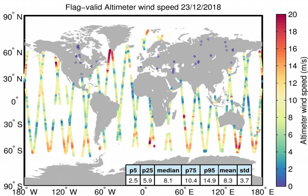
Figure 31. Geographical distribution of flag-valid wind data over oceans and lakes for 23/12/2018. The statistical values shown in the table refer to the wind in m/s and are calculated over all measurements shown in the figure.
