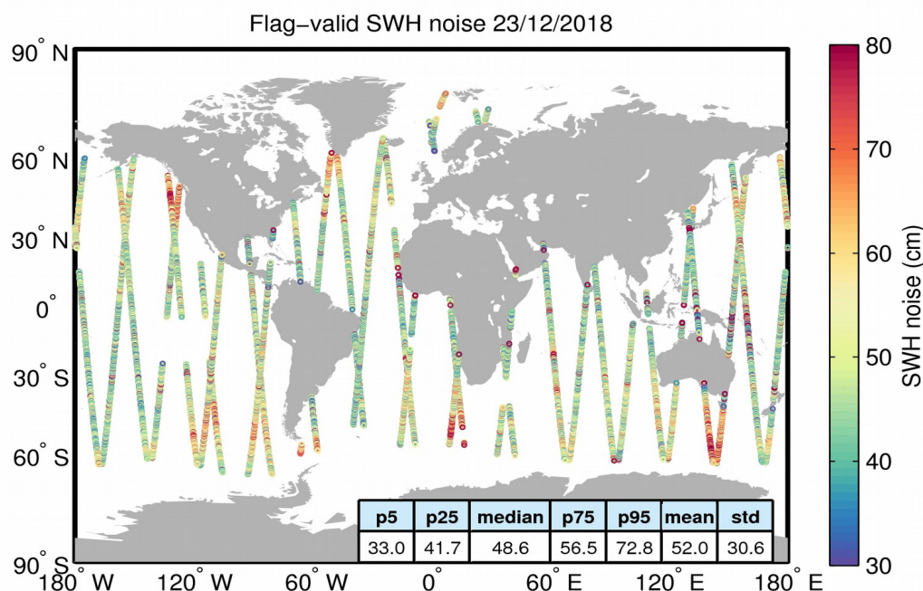
Figure 18. Geographical distribution of flag-valid 20-Hz SWH measurement noise over oceans and lakes for 23/12/2018. The statistical values shown in the figure refer to the SWH noise and are calculated over all measurements shown in the figure.
