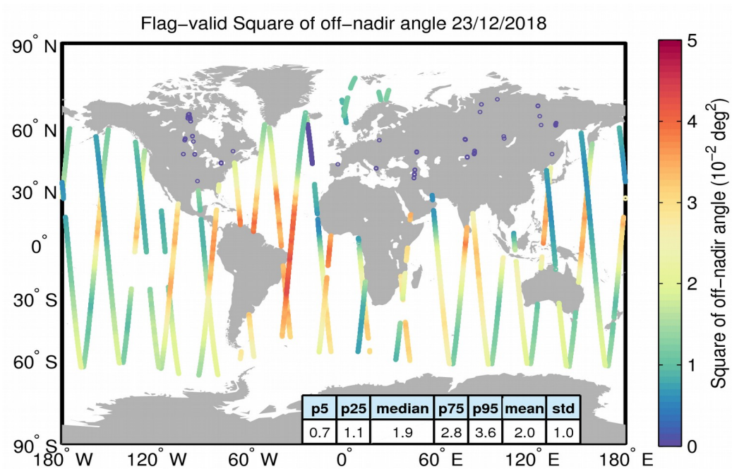
Figure 37. Geographical distribution of flag-valid mispointing data over oceans and lakes for 23/12/2018. The statistical values shown in the table refer to the mispointing in 10^{-2} \text{ deg}^2 and are calculated over all measurements shown in the figure.
