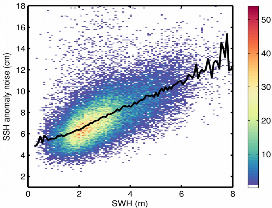
Figure 9. 2D histogram showing flag-valid SSH anomaly noise as a function of SWH for 21/12/2018. The black line denotes the median SSH anomaly noise as a function of SWH.
