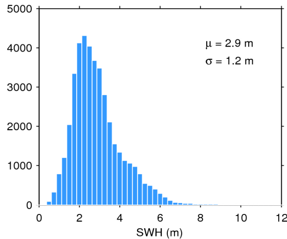
Figure 20. Histogram of science-valid SWH over oceans and lakes for 21/12/2018. The mean ( \mu ) and standard deviation ( \sigma ) are also shown. Note that values larger than 12 m are excluded from the histogram for the sake of readability but not from the computation of \mu and \sigma .
