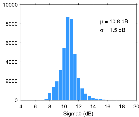
Figure 28. Histogram of science-valid sigma0 over oceans and lakes for 21/12/2018. The mean ( \mu ) and standard deviation ( \sigma ) are also shown. Note that values outside [4 20] dB are excluded from the histogram for the sake of readability but not from the computation of \mu and \sigma .
