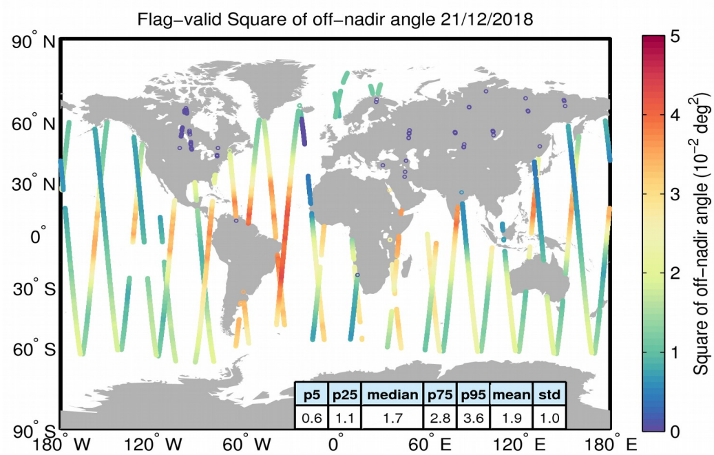
Figure 37. Geographical distribution of flag-valid mispointing data over oceans and lakes for 21/12/2018. The statistical values shown in the table refer to the mispointing in 10^{-2} deg 2 and are calculated over all measurements shown in the figure.
