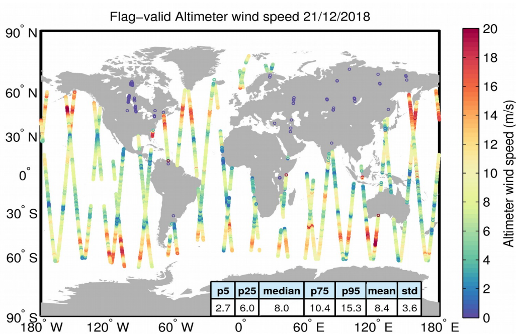
Figure 31. Geographical distribution of flag-valid wind data over oceans and lakes for 21/12/2018. The statistical values shown in the table refer to the wind in m/s and are calculated over all measurements shown in the figure.
