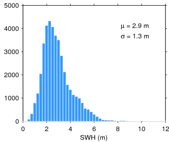
Figure 17. Histogram of flag-valid SWH over oceans and lakes for 21/12/2018. The mean ( \mu ) and standard deviation ( \sigma ) are also shown. Note that values larger than 12 m are excluded from the histogram for the sake of readability but not from the computation of \mu and \sigma .
