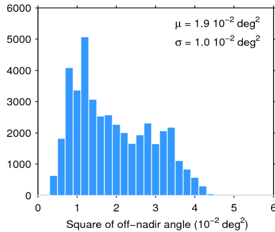
Figure 39. Histogram of flag-valid mispointing over oceans and lakes for 21/12/2018. The mean ( \mu ) and standard deviation ( \sigma ) are also shown. Note that values larger than 6 \cdot 10^{-2} \text{ deg}^2 are excluded from the histogram for the sake of readability but not from the computation of \mu and \sigma .
