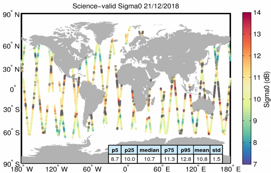
Figure 27. Geographical distribution of science-valid sigma0 data over oceans and lakes for 21/12/2018. The statistical values shown in the table refer to the sigma0 in dB and are calculated over all measurements shown in the figure. Gray circles denote records that have been rejected based on the editing criteria described in Table 4.
