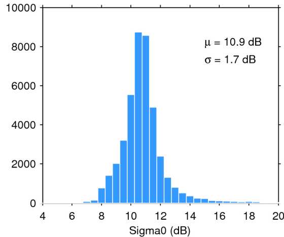
Figure 25. Histogram of flag-valid sigma0 over oceans and lakes for 21/12/2018. The mean ( \mu ) and standard deviation ( \sigma ) are also shown. Note that values outside [4 20] dB are excluded from the histogram for the sake of readability but not from the computation of \mu and \sigma .
