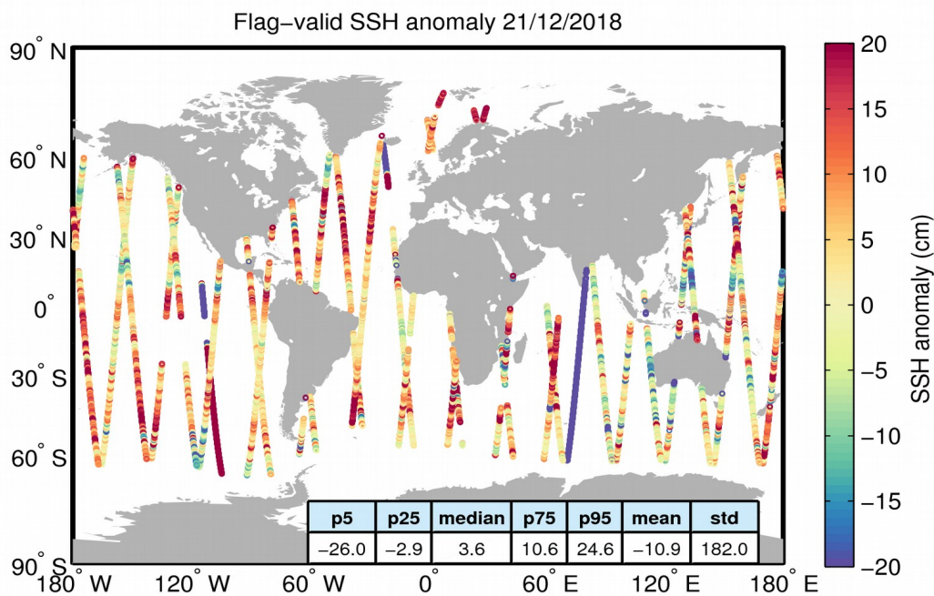
Figure 5. Geographical distribution of flag-valid 1-Hz SSH anomaly data over oceans and lakes for 21/12/2018. The statistical values shown in the table refer to the SSH anomaly in cm and are calculated over all measurements shown in the figure.
