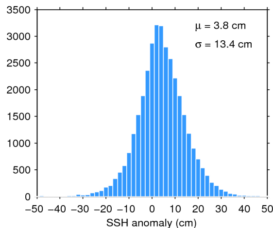
Figure 11. Histogram of science-valid SSH anomaly over oceans and lakes for 21/12/2018. The mean ( \mu ) and standard deviation ( \sigma ) are also shown. Note that values outside [-50 50] cm are excluded from the histogram for the sake of readability but not from the computation of \mu and \sigma .
