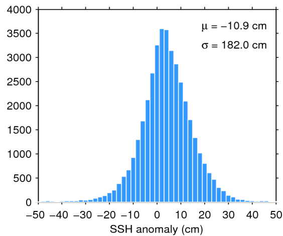
Figure 7. Histogram of flag-valid SSH anomaly over oceans and lakes for 21/12/2018. The mean ( \mu ) and standard deviation ( \sigma ) are also shown. Note that values outside [-50 50] cm are excluded from the histogram for the sake of readability but not from the computation of \mu and \sigma .
