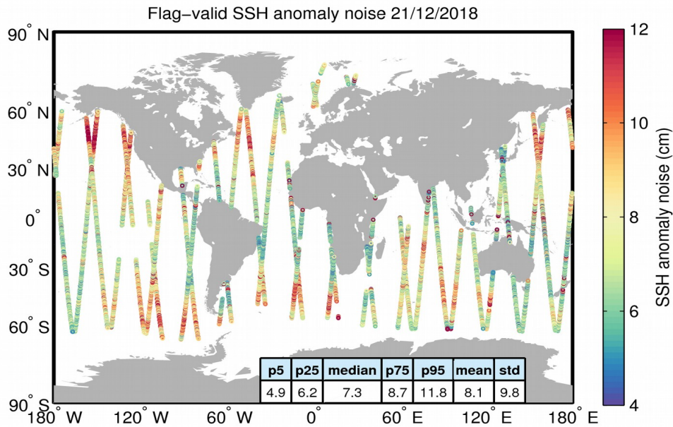
Figure 8. Geographical distribution of flag-valid 20-Hz SSH anomaly measurement noise over oceans and lakes for 21/12/2018. The statistical values shown in the table refer to the SSH anomaly noise and are calculated over all measurements shown in the figure.
