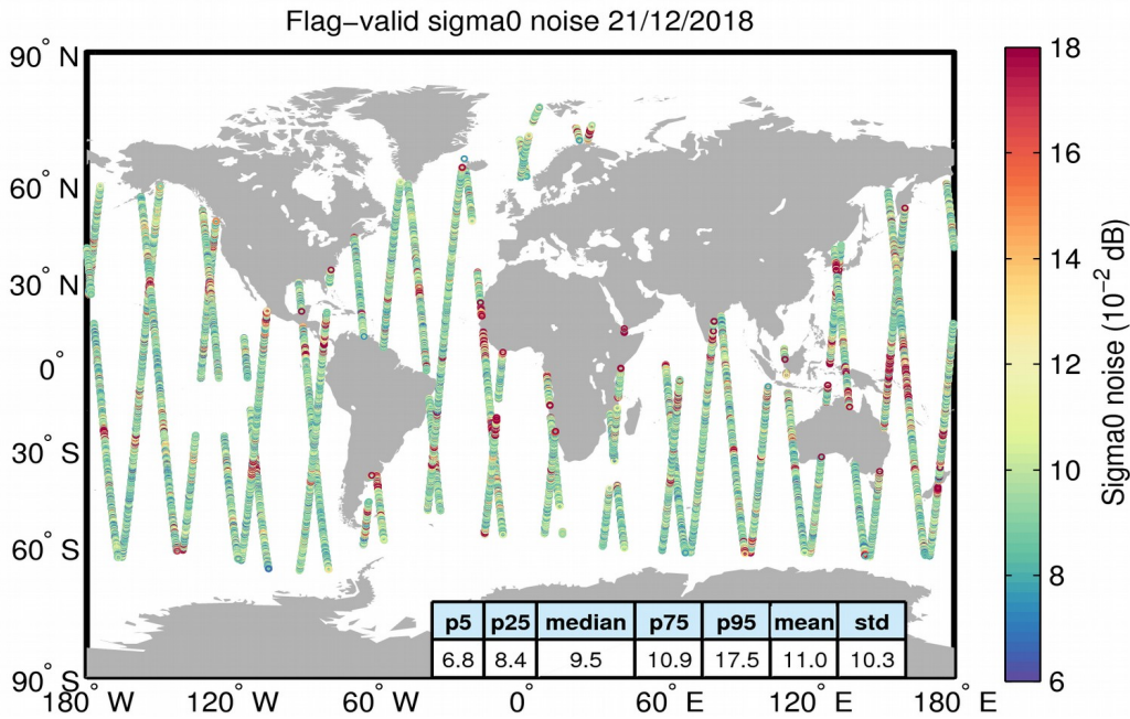
Figure 26. Geographical distribution of flag-valid 20-Hz sigma0 measurement noise over oceans and lakes for 21/12/2018. The statistical values shown in the table refer to the sigma0 noise and are calculated over all measurements shown in the figure.
