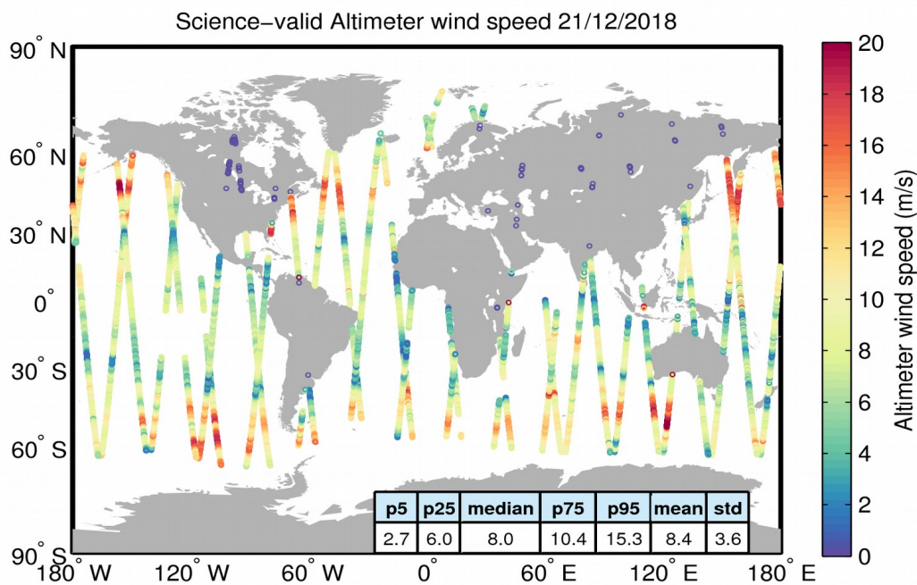
Figure 34. Geographical distribution of science-valid wind data over oceans and lakes for 21/12/2018. The statistical values shown in the table refer to the wind in m/s and are calculated over all measurements shown in the figure. Gray circles denote records that have been rejected based on the editing criteria described in Table 5.
