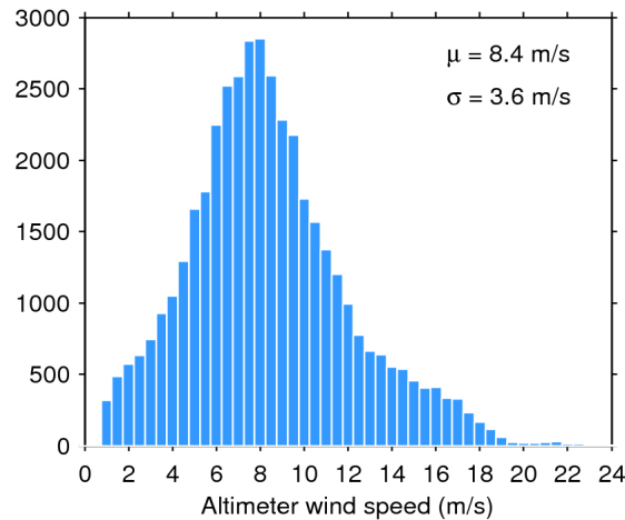
Figure 33. Histogram of flag-valid wind over oceans and lakes for 21/12/2018. The mean ( \mu ) and standard deviation ( \sigma ) are also shown. Note that values larger than 24 m/s are excluded from the histogram for the sake of readability but not from the computation of \mu and \sigma .
