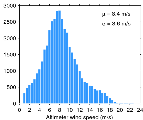
Figure 35. Histogram of science-valid wind over oceans and lakes for 21/12/2018. The mean ( \mu ) and standard deviation ( \sigma ) are also shown. Note that values larger than 24 m/s are excluded from the histogram for the sake of readability but not from the computation of \mu and \sigma .
