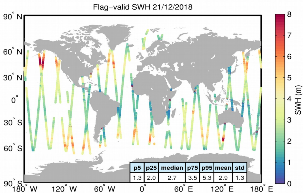
Figure 15. Geographical distribution of flag-valid SWH data over oceans and lakes for 21/12/2018. The statistical values shown in the table refer to the SWH in m and are calculated over all measurements shown in the figure.
