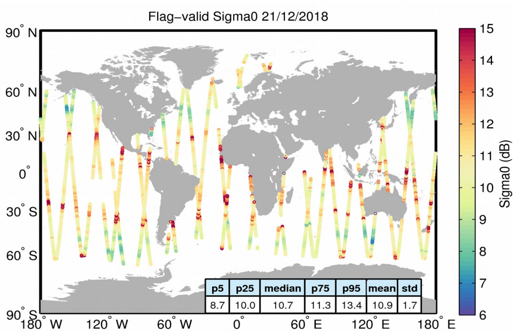
Figure 23. Geographical distribution of flag-valid sigma0 data over oceans and lakes for 21/12/2018. The statistical values shown in the table refer to the sigma0 in dB and are calculated over all measurements shown in the figure.
