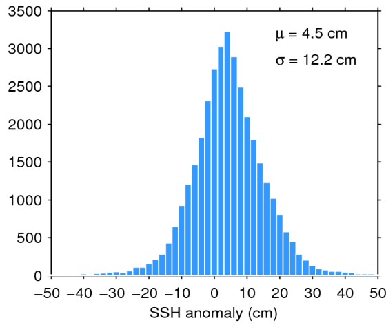
Figure 11. Histogram of science-valid SSH anomaly over oceans and lakes for 20/12/2018. The mean ( \mu ) and standard deviation ( \sigma ) are also shown. Note that values outside [-50 50] cm are excluded from the histogram for the sake of readability but not from the computation of \mu and \sigma .
