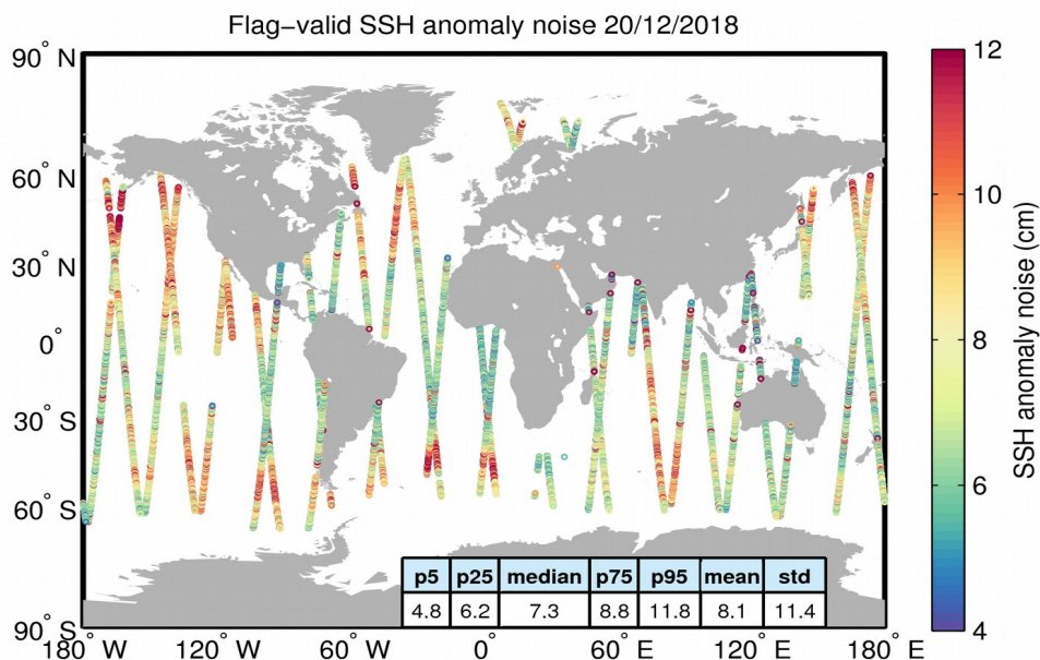
Figure 8. Geographical distribution of flag-valid 20-Hz SSH anomaly measurement noise over oceans and lakes for 20/12/2018. The statistical values shown in the table refer to the SSH anomaly noise and are calculated over all measurements shown in the figure.
