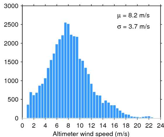
Figure 35. Histogram of science-valid wind over oceans and lakes for 20/12/2018. The mean ( \mu ) and standard deviation ( \sigma ) are also shown. Note that values larger than 24 m/s are excluded from the histogram for the sake of readability but not from the computation of \mu and \sigma .
