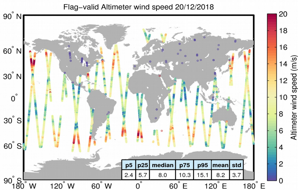
Figure 31. Geographical distribution of flag-valid wind data over oceans and lakes for 20/12/2018. The statistical values shown in the table refer to the wind in m/s and are calculated over all measurements shown in the figure.
