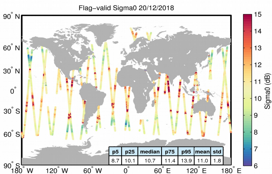
Figure 23. Geographical distribution of flag-valid sigma0 data over oceans and lakes for 20/12/2018. The statistical values shown in the table refer to the sigma0 in dB and are calculated over all measurements shown in the figure.
