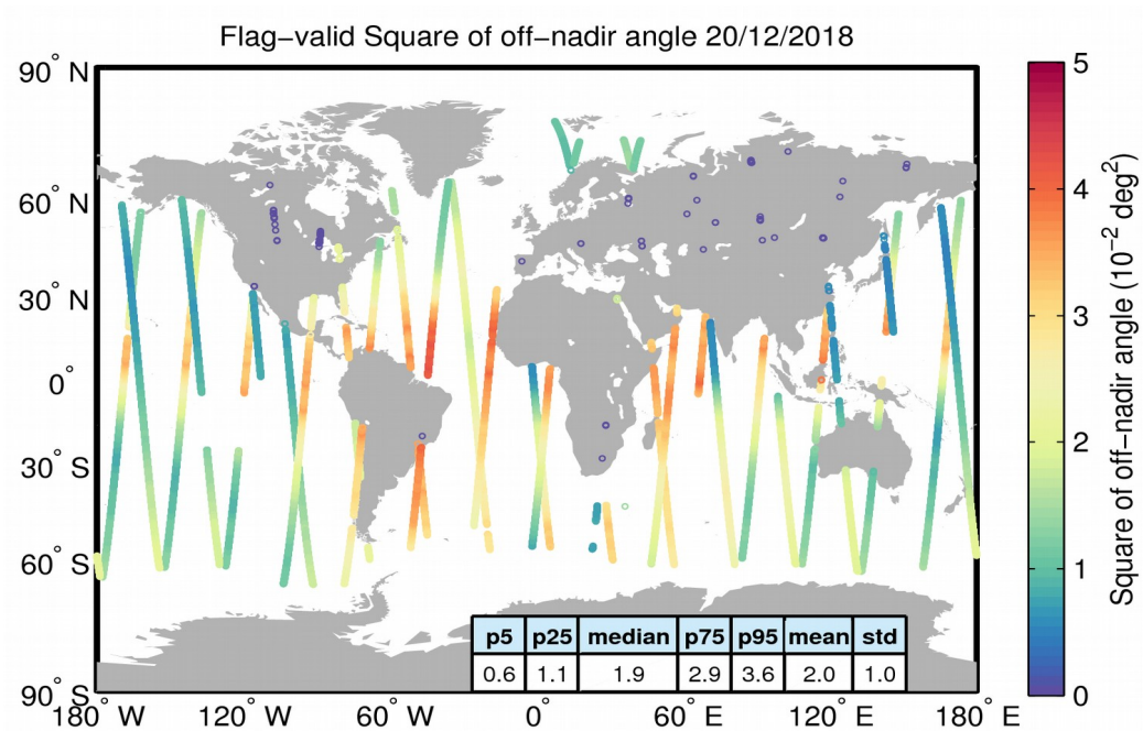
Figure 37. Geographical distribution of flag-valid mispointing data over oceans and lakes for 20/12/2018. The statistical values shown in the table refer to the mispointing in 10^{-2} deg 2 and are calculated over all measurements shown in the figure.
