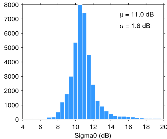
Figure 25. Histogram of flag-valid sigma0 over oceans and lakes for 20/12/2018. The mean ( \mu ) and standard deviation ( \sigma ) are also shown. Note that values outside [4 20] dB are excluded from the histogram for the sake of readability but not from the computation of \mu and \sigma .
