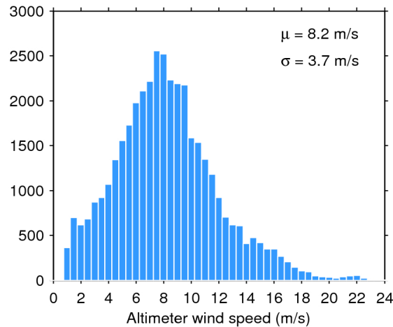
Figure 33. Histogram of flag-valid wind over oceans and lakes for 20/12/2018. The mean ( \mu ) and standard deviation ( \sigma ) are also shown. Note that values larger than 24 m/s are excluded from the histogram for the sake of readability but not from the computation of \mu and \sigma .
