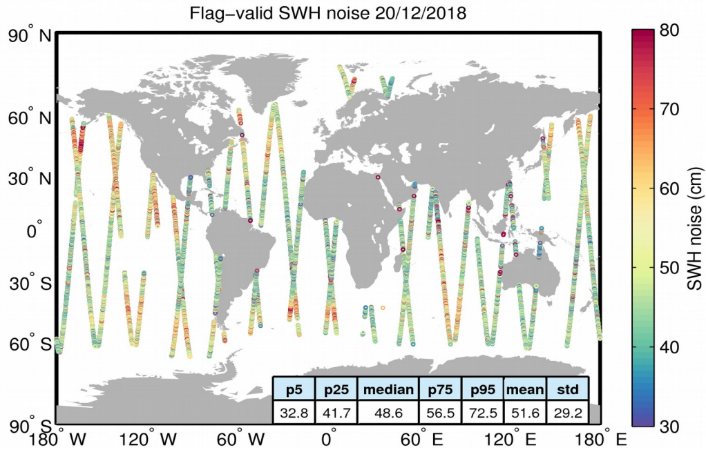
Figure 18. Geographical distribution of flag-valid 20-Hz SWH measurement noise over oceans and lakes for 20/12/2018. The statistical values shown in the figure refer to the SWH noise and are calculated over all measurements shown in the figure.
