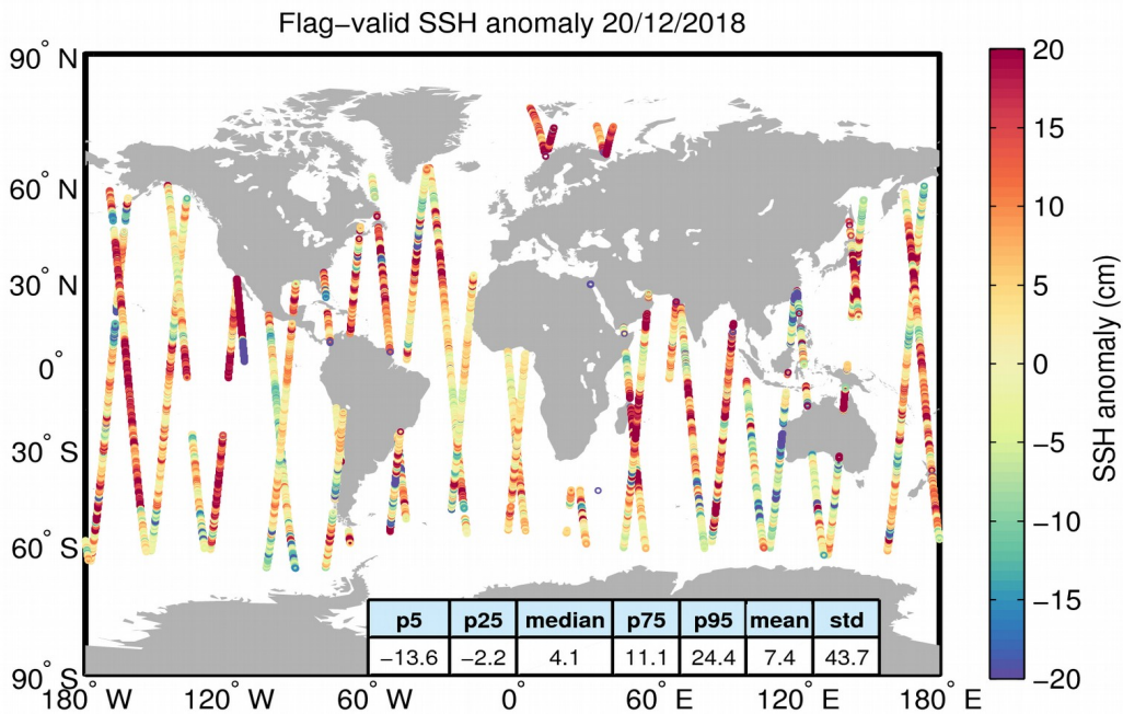
Figure 5. Geographical distribution of flag-valid 1-Hz SSH anomaly data over oceans and lakes for 20/12/2018. The statistical values shown in the table refer to the SSH anomaly in cm and are calculated over all measurements shown in the figure.
