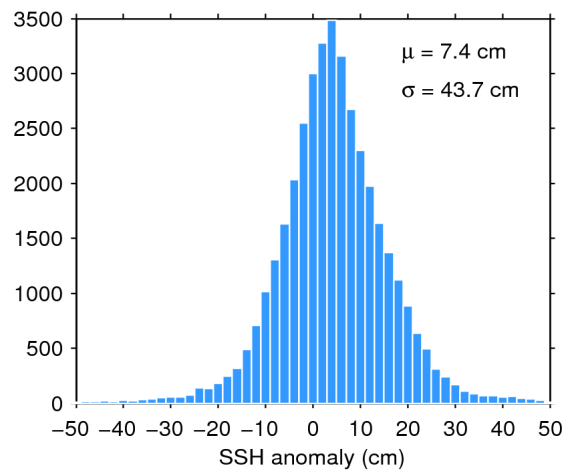
Figure 7. Histogram of flag-valid SSH anomaly over oceans and lakes for 20/12/2018. The mean ( \mu ) and standard deviation ( \sigma ) are also shown. Note that values outside [-50\ 50] cm are excluded from the histogram for the sake of readability but not from the computation of \mu and \sigma .
