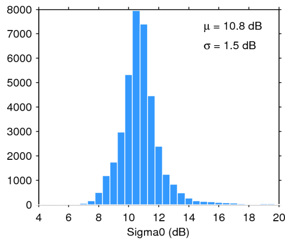
Figure 28. Histogram of science-valid sigma0 over oceans and lakes for 20/12/2018. The mean ( \mu ) and standard deviation ( \sigma ) are also shown. Note that values outside [4 20] dB are excluded from the histogram for the sake of readability but not from the computation of \mu and \sigma .
