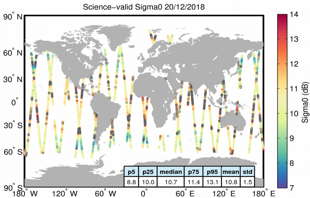
Figure 27. Geographical distribution of science-valid sigma0 data over oceans and lakes for 20/12/2018. The statistical values shown in the table refer to the sigma0 in dB and are calculated over all measurements shown in the figure. Gray circles denote records that have been rejected based on the editing criteria described in Table 4.
