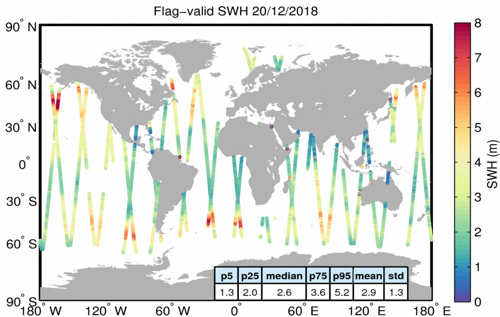
Figure 15. Geographical distribution of flag-valid SWH data over oceans and lakes for 20/12/2018. The statistical values shown in the table refer to the SWH in m and are calculated over all measurements shown in the figure.
