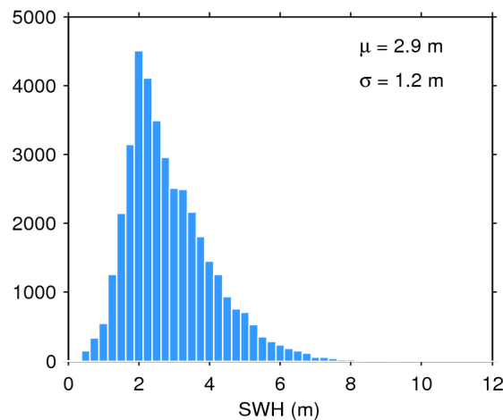
Figure 20. Histogram of science-valid SWH over oceans and lakes for 20/12/2018. The mean ( \mu ) and standard deviation ( \sigma ) are also shown. Note that values larger than 12 m are excluded from the histogram for the sake of readability but not from the computation of \mu and \sigma .
