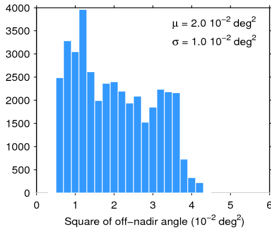
Figure 39. Histogram of flag-valid mispointing over oceans and lakes for 20/12/2018. The mean ( \mu ) and standard deviation ( \sigma ) are also shown. Note that values larger than 6 \cdot 10^{-2} \text{ deg}^2 are excluded from the histogram for the sake of readability but not from the computation of \mu and \sigma .
