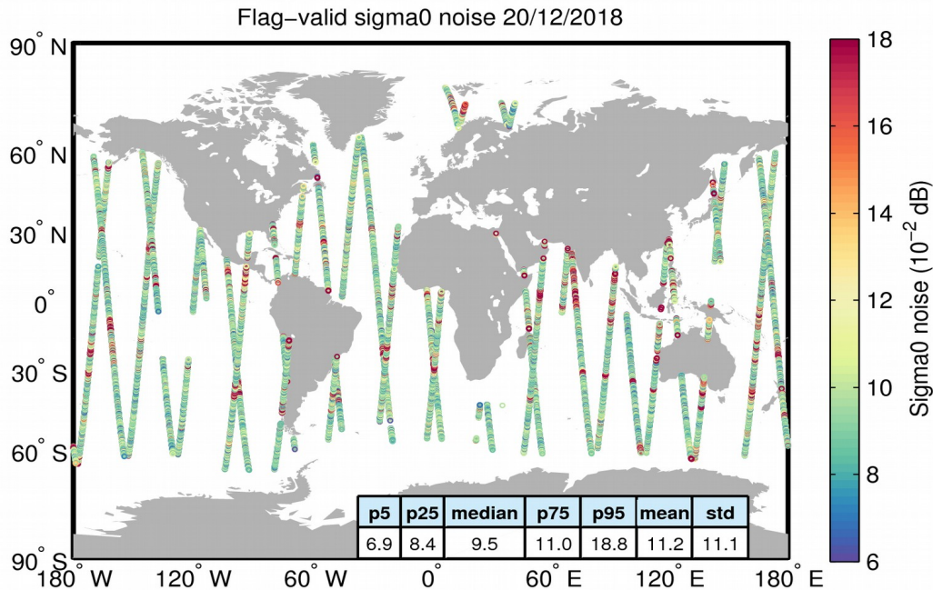
Figure 26. Geographical distribution of flag-valid 20-Hz sigma0 measurement noise over oceans and lakes for 20/12/2018. The statistical values shown in the table refer to the sigma0 noise and are calculated over all measurements shown in the figure.
