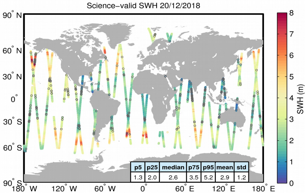
Figure 19. Geographical distribution of science-valid SWH data over oceans and lakes for 20/12/2018. The statistical values shown in the table refer to the SWH in m and are calculated over all measurements shown in the figure. Gray circles denote records that have been rejected based on the editing criteria described in Table 3.
