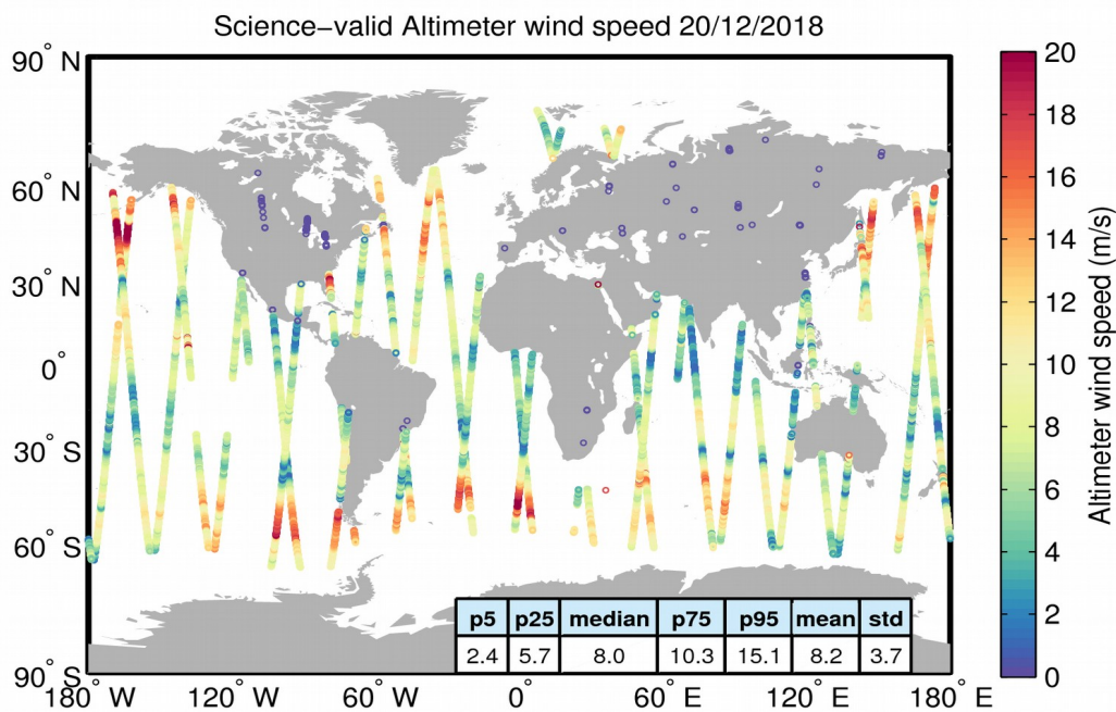
Figure 34. Geographical distribution of science-valid wind data over oceans and lakes for 20/12/2018. The statistical values shown in the table refer to the wind in m/s and are calculated over all measurements shown in the figure. Gray circles denote records that have been rejected based on the editing criteria described in Table 5.
