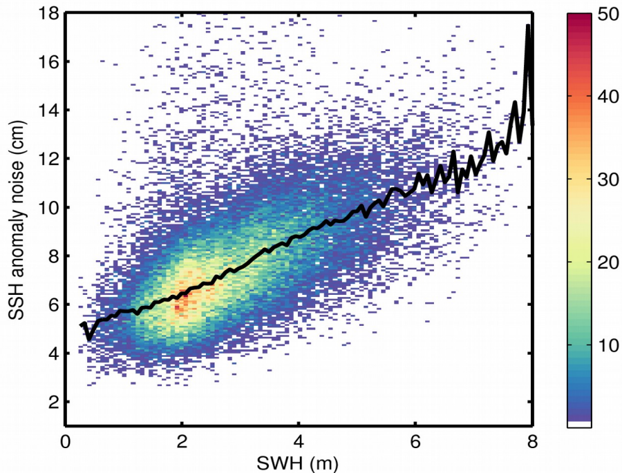
Figure 9. 2D histogram showing flag-valid SSH anomaly noise as a function of SWH for 20/12/2018. The black line denotes the median SSH anomaly noise as a function of SWH.
