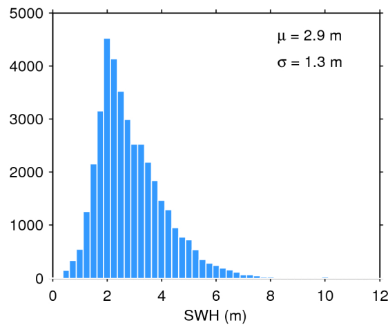
Figure 17. Histogram of flag-valid SWH over oceans and lakes for 20/12/2018. The mean ( \mu ) and standard deviation ( \sigma ) are also shown. Note that values larger than 12 m are excluded from the histogram for the sake of readability but not from the computation of \mu and \sigma .
