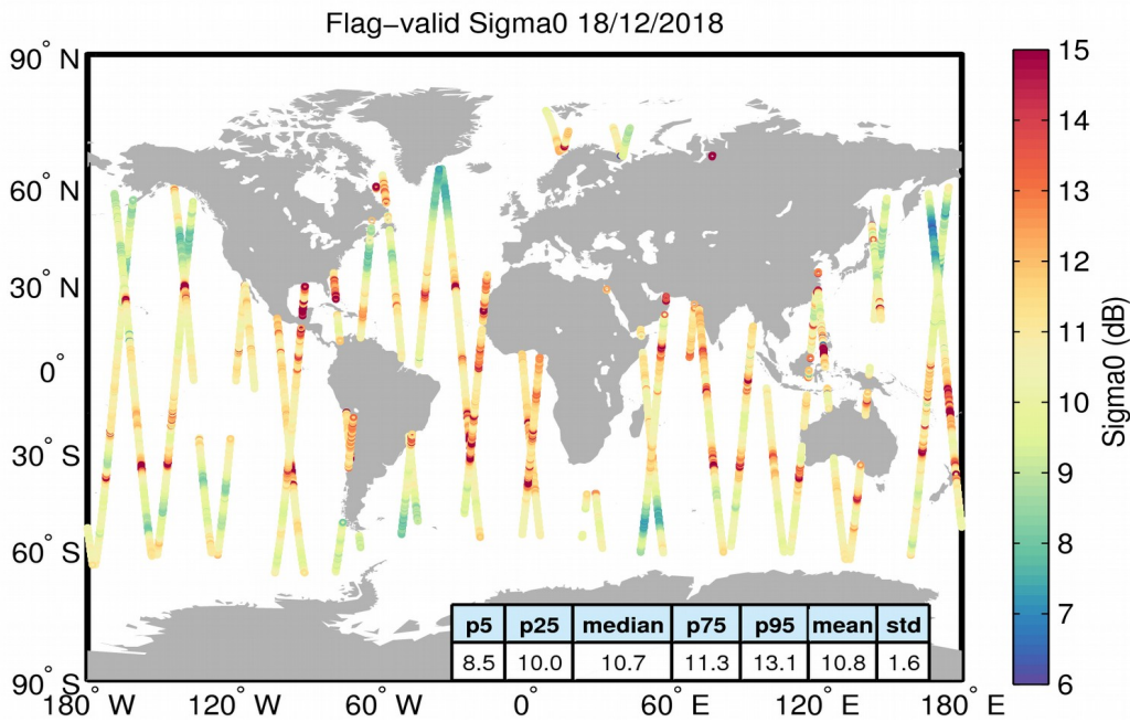
Figure 23. Geographical distribution of flag-valid sigma0 data over oceans and lakes for 18/12/2018. The statistical values shown in the table refer to the sigma0 in dB and are calculated over all measurements shown in the figure.
