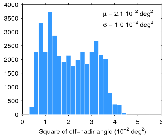
Figure 39. Histogram of flag-valid mispointing over oceans and lakes for 18/12/2018. The mean ( \mu ) and standard deviation ( \sigma ) are also shown. Note that values larger than 6 \cdot 10^{-2} \text{ deg}^2 are excluded from the histogram for the sake of readability but not from the computation of \mu and \sigma .
