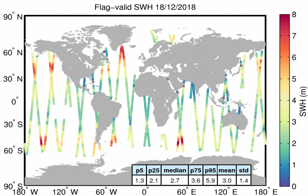
Figure 15. Geographical distribution of flag-valid SWH data over oceans and lakes for 18/12/2018. The statistical values shown in the table refer to the SWH in m and are calculated over all measurements shown in the figure.
