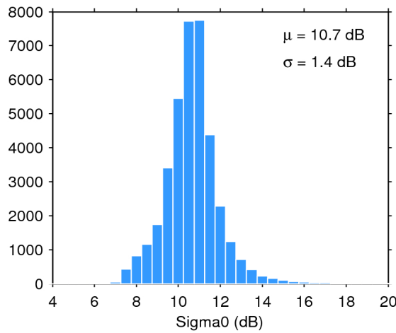
Figure 28. Histogram of science-valid sigma0 over oceans and lakes for 18/12/2018. The mean ( \mu ) and standard deviation ( \sigma ) are also shown. Note that values outside [4 20] dB are excluded from the histogram for the sake of readability but not from the computation of \mu and \sigma .
