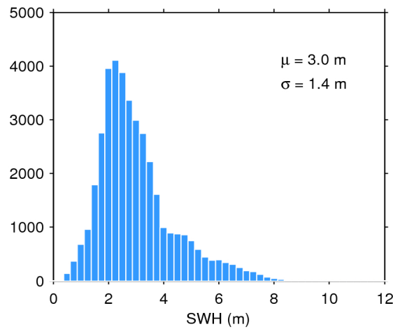
Figure 17. Histogram of flag-valid SWH over oceans and lakes for 18/12/2018. The mean ( \mu ) and standard deviation ( \sigma ) are also shown. Note that values larger than 12 m are excluded from the histogram for the sake of readability but not from the computation of \mu and \sigma .
