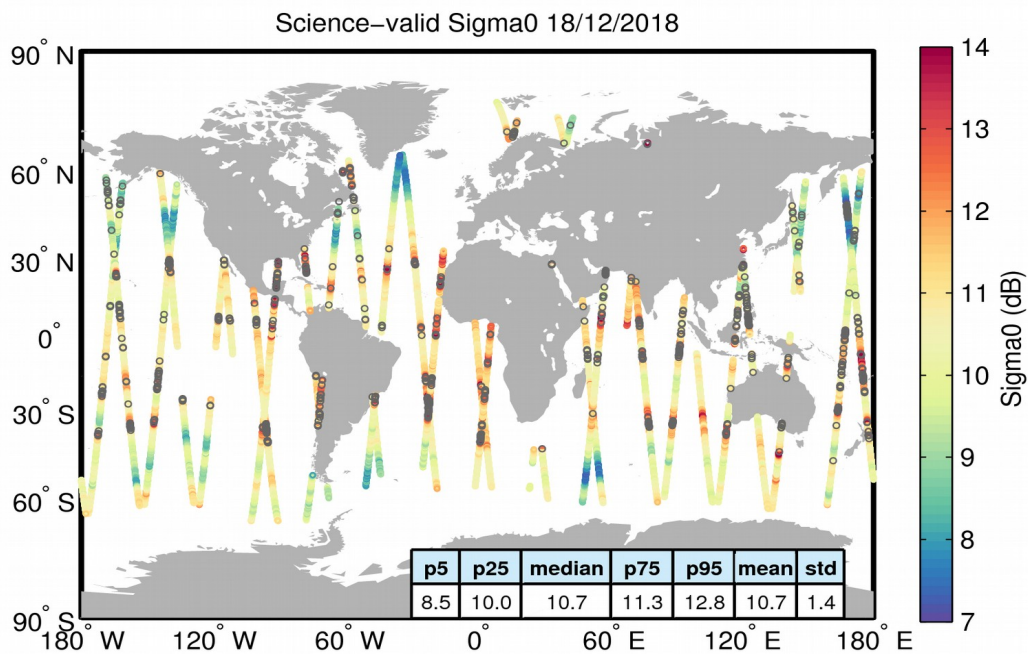
Figure 27. Geographical distribution of science-valid sigma0 data over oceans and lakes for 18/12/2018. The statistical values shown in the table refer to the sigma0 in dB and are calculated over all measurements shown in the figure. Gray circles denote records that have been rejected based on the editing criteria described in Table 4.
