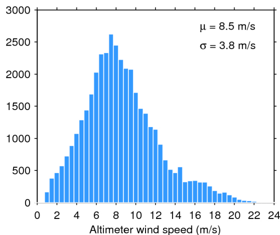
Figure 35. Histogram of science-valid wind over oceans and lakes for 18/12/2018. The mean ( \mu ) and standard deviation ( \sigma ) are also shown. Note that values larger than 24 m/s are excluded from the histogram for the sake of readability but not from the computation of \mu and \sigma .
