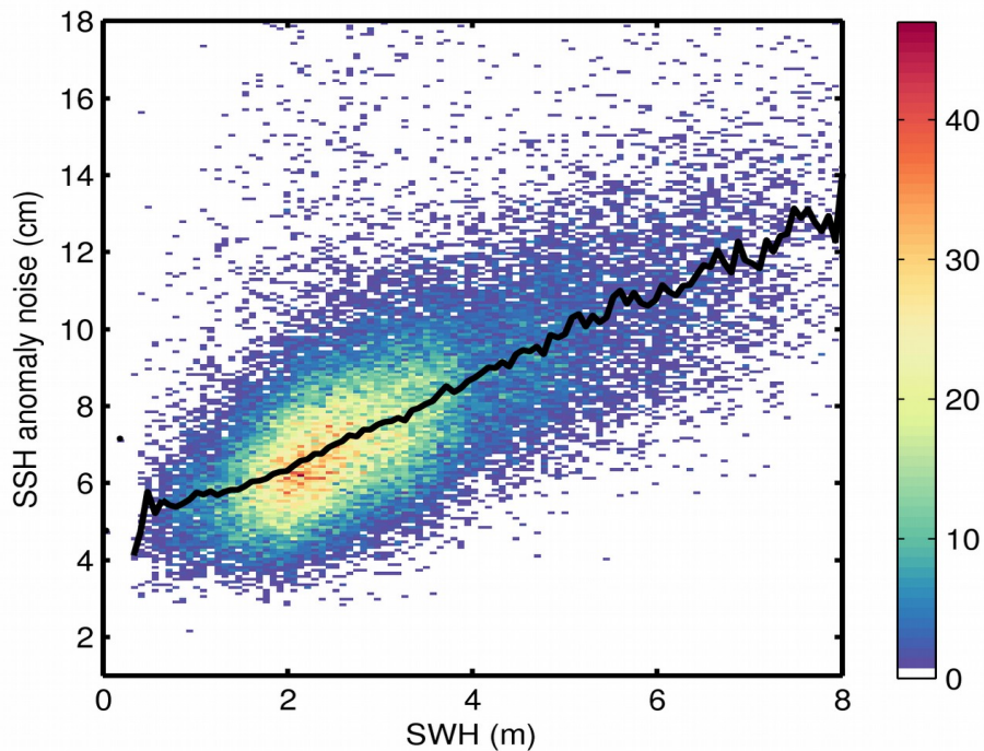
Figure 9. 2D histogram showing flag-valid SSH anomaly noise as a function of SWH for 18/12/2018. The black line denotes the median SSH anomaly noise as a function of SWH.
