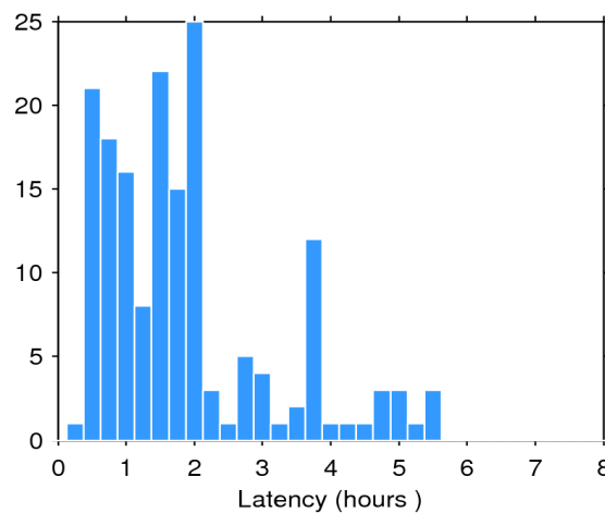
Figure 2. Histogram of the data latency for 18/12/2018. The y-axis denotes the number of files that are made available with a delay of x-hours with respect to the mean time of the records stored in the file.
