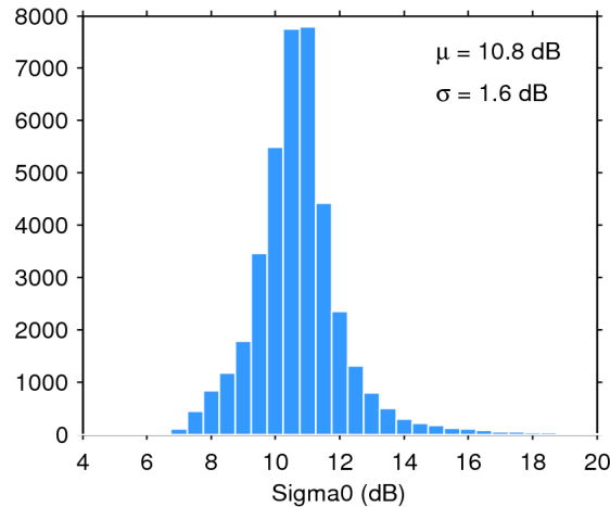
Figure 25. Histogram of flag-valid sigma0 over oceans and lakes for 18/12/2018. The mean ( \mu ) and standard deviation ( \sigma ) are also shown. Note that values outside [4 20] dB are excluded from the histogram for the sake of readability but not from the computation of \mu and \sigma .
