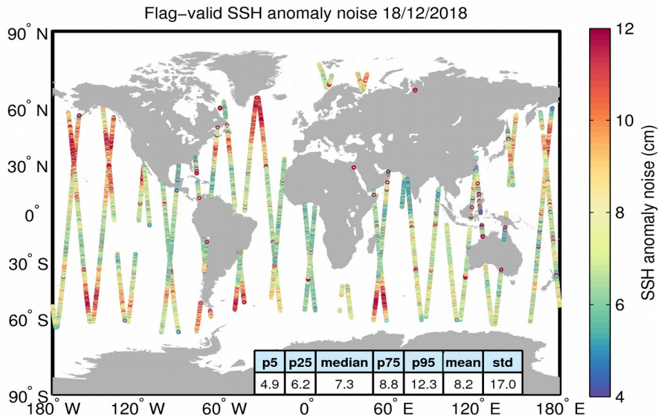
Figure 8. Geographical distribution of flag-valid 20-Hz SSH anomaly measurement noise over oceans and lakes for 18/12/2018. The statistical values shown in the table refer to the SSH anomaly noise and are calculated over all measurements shown in the figure.
