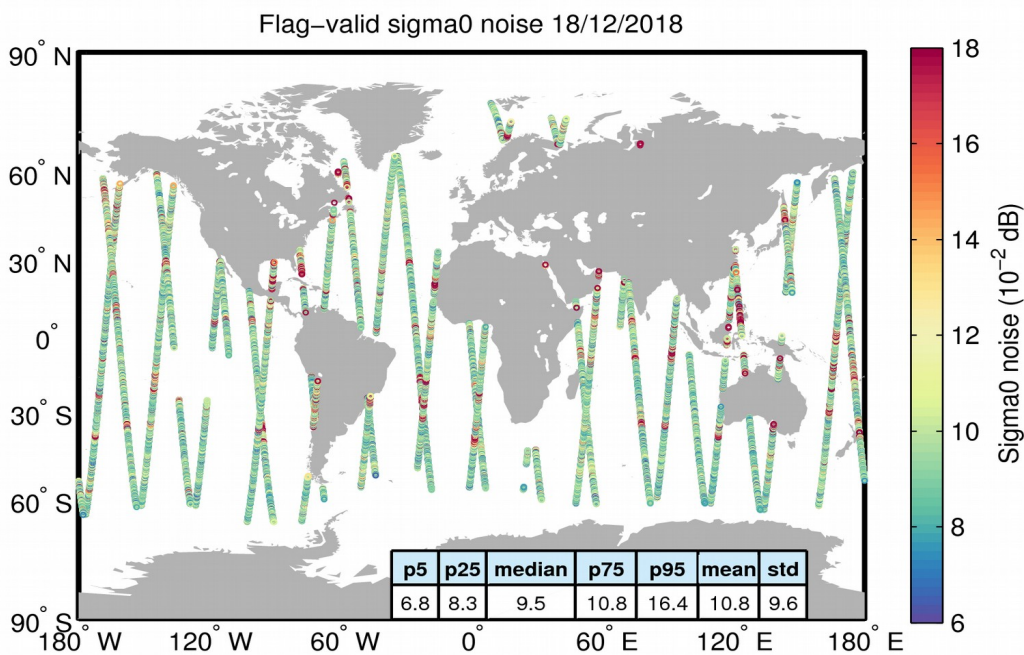
Figure 26. Geographical distribution of flag-valid 20-Hz sigma0 measurement noise over oceans and lakes for 18/12/2018. The statistical values shown in the table refer to the sigma0 noise and are calculated over all measurements shown in the figure.
