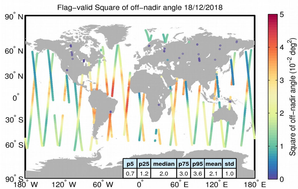
Figure 37. Geographical distribution of flag-valid mispointing data over oceans and lakes for 18/12/2018. The statistical values shown in the table refer to the mispointing in 10^{-2} deg 2 and are calculated over all measurements shown in the figure.
