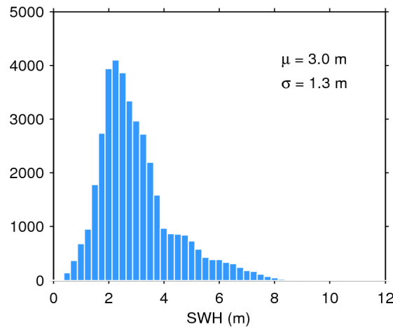
Figure 20. Histogram of science-valid SWH over oceans and lakes for 18/12/2018. The mean ( \mu ) and standard deviation ( \sigma ) are also shown. Note that values larger than 12 m are excluded from the histogram for the sake of readability but not from the computation of \mu and \sigma .
