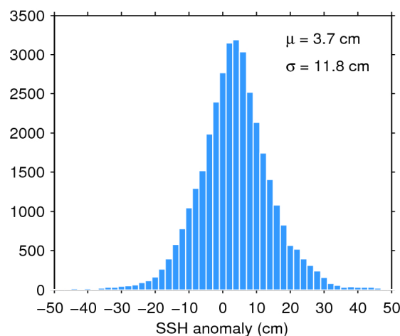
Figure 11. Histogram of science-valid SSH anomaly over oceans and lakes for 18/12/2018. The mean ( \mu ) and standard deviation ( \sigma ) are also shown. Note that values outside [-50 50] cm are excluded from the histogram for the sake of readability but not from the computation of \mu and \sigma .
