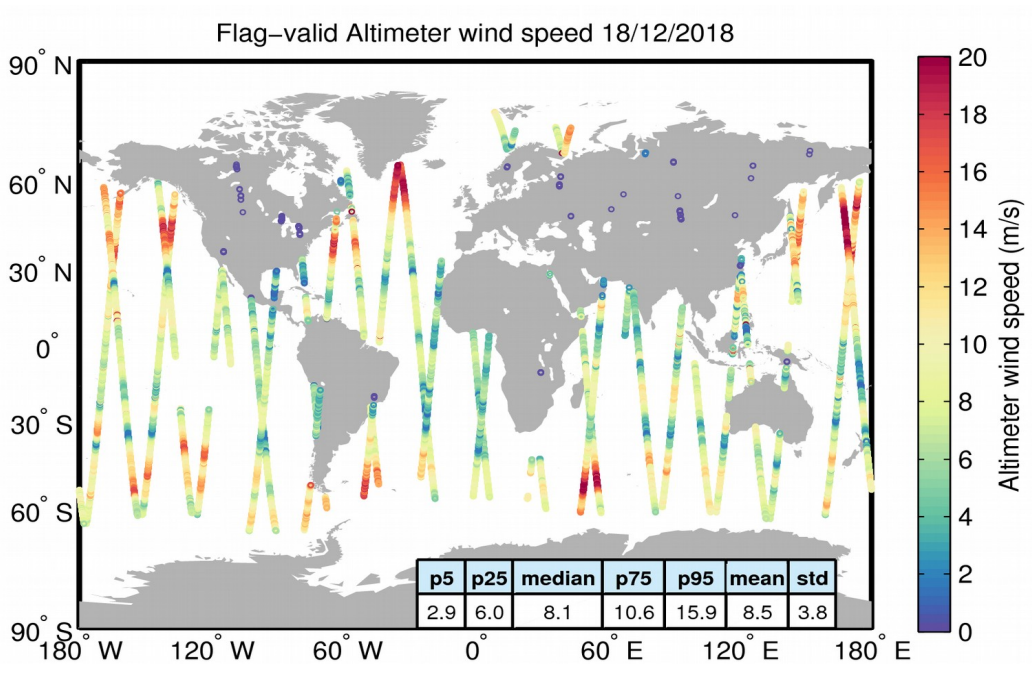
Figure 31. Geographical distribution of flag-valid wind data over oceans and lakes for 18/12/2018. The statistical values shown in the table refer to the wind in m/s and are calculated over all measurements shown in the figure.
