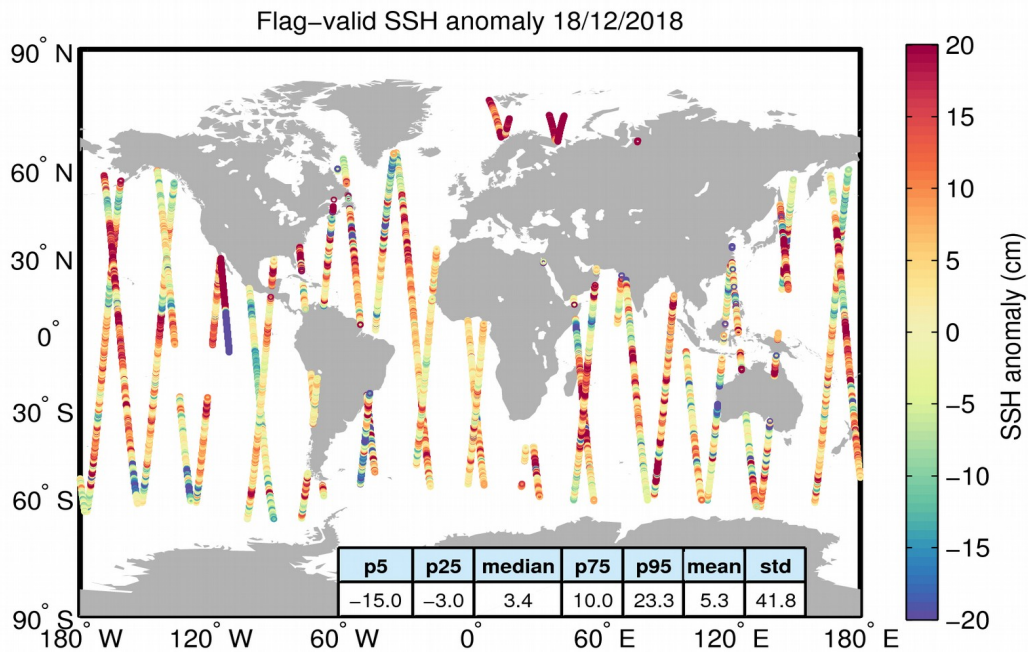
Figure 5. Geographical distribution of flag-valid 1-Hz SSH anomaly data over oceans and lakes for 18/12/2018. The statistical values shown in the table refer to the SSH anomaly in cm and are calculated over all measurements shown in the figure.
