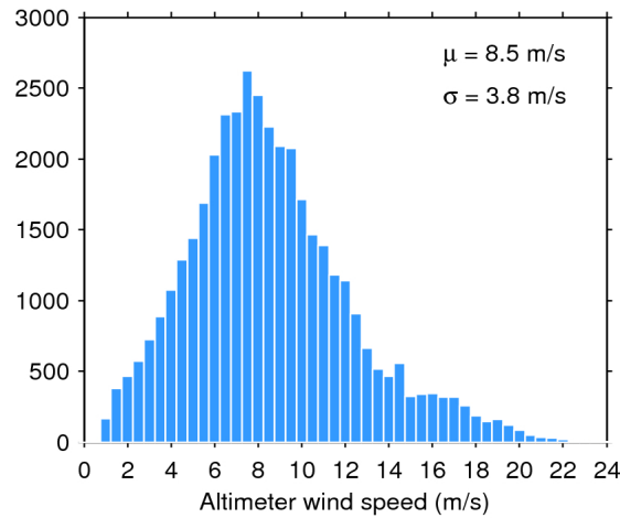
Figure 33. Histogram of flag-valid wind over oceans and lakes for 18/12/2018. The mean ( \mu ) and standard deviation ( \sigma ) are also shown. Note that values larger than 24 m/s are excluded from the histogram for the sake of readability but not from the computation of \mu and \sigma .
