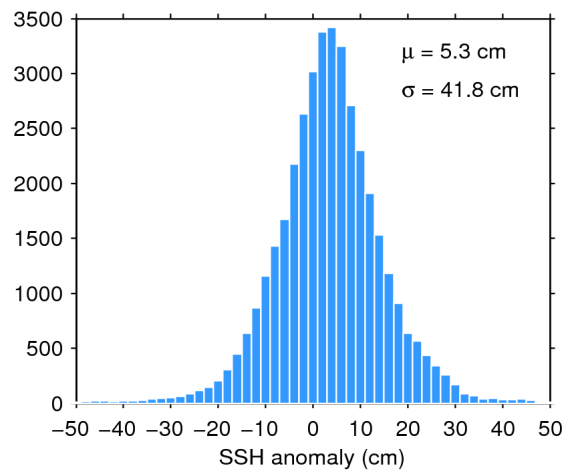
Figure 7. Histogram of flag-valid SSH anomaly over oceans and lakes for 18/12/2018. The mean ( \mu ) and standard deviation ( \sigma ) are also shown. Note that values outside [-50 50] cm are excluded from the histogram for the sake of readability but not from the computation of \mu and \sigma .
