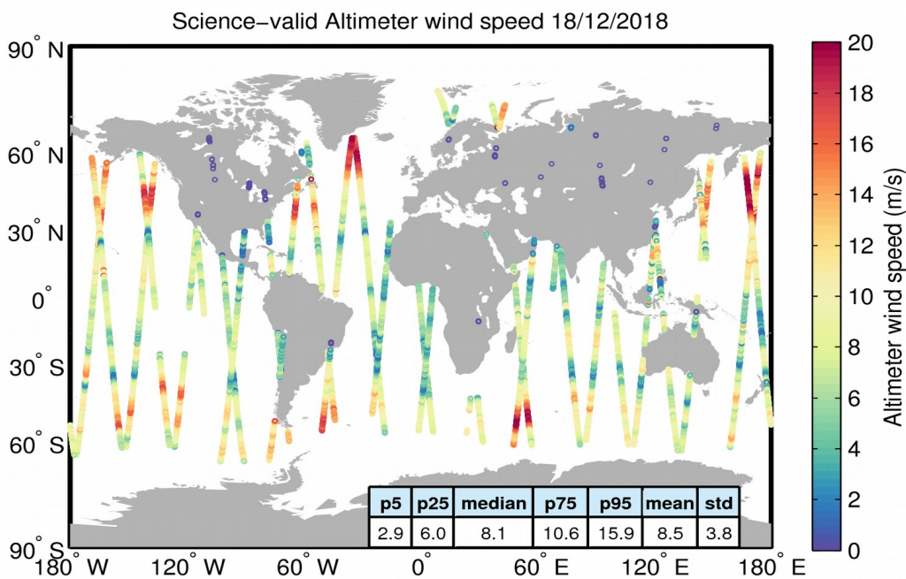
Figure 34. Geographical distribution of science-valid wind data over oceans and lakes for 18/12/2018. The statistical values shown in the table refer to the wind in m/s and are calculated over all measurements shown in the figure. Gray circles denote records that have been rejected based on the editing criteria described in Table 5.
