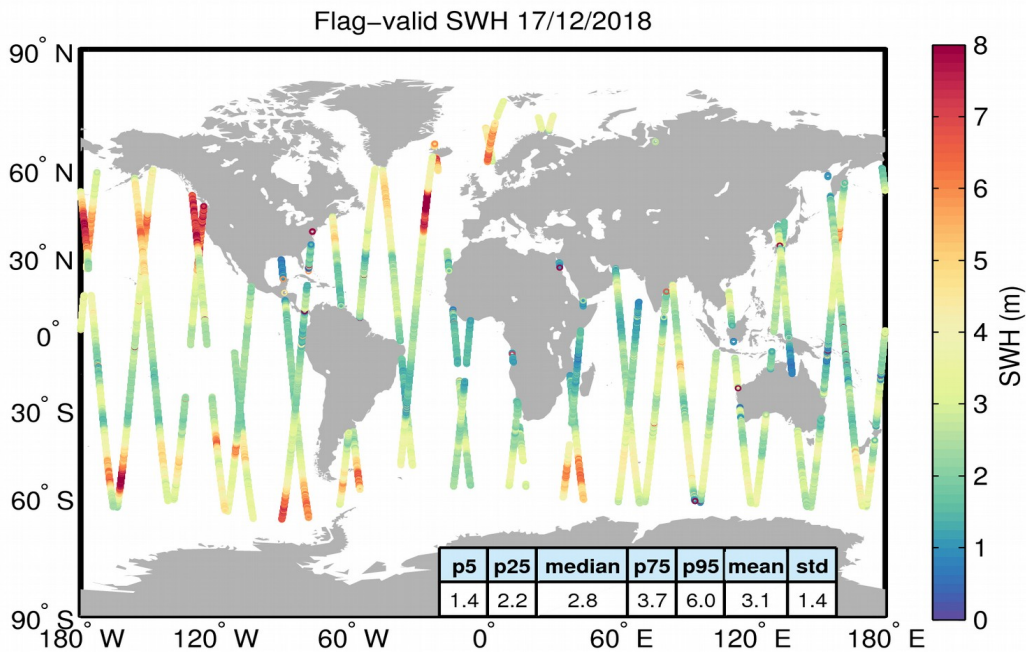
Figure 15. Geographical distribution of flag-valid SWH data over oceans and lakes for 17/12/2018. The statistical values shown in the table refer to the SWH in m and are calculated over all measurements shown in the figure.
