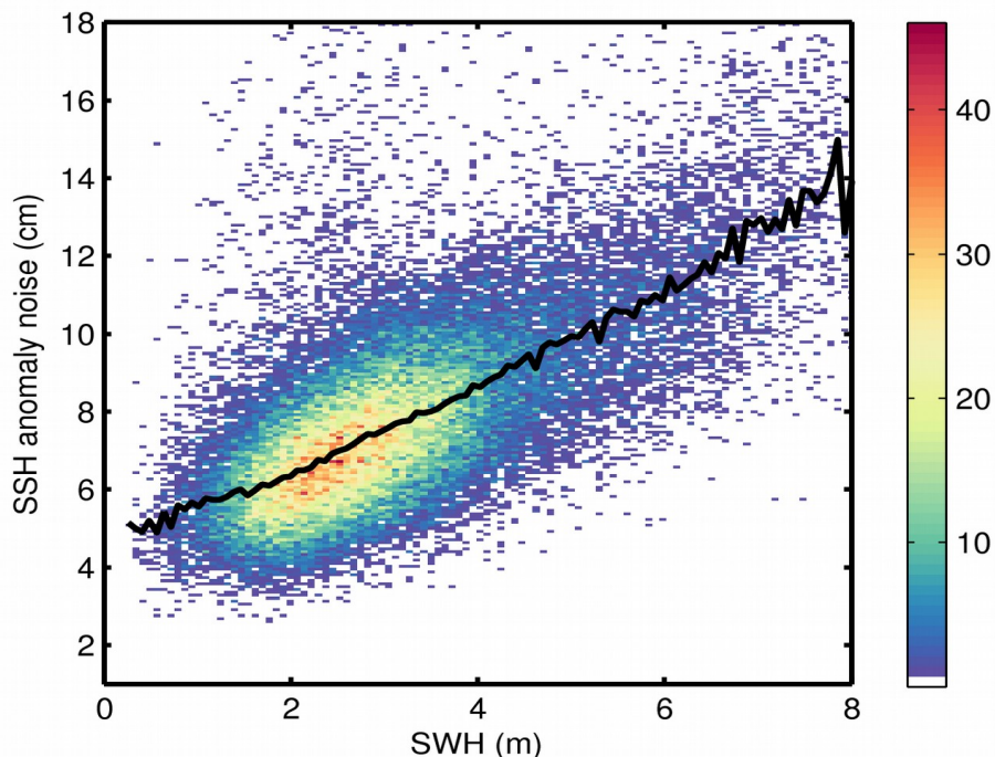
Figure 9. 2D histogram showing flag-valid SSH anomaly noise as a function of SWH for 17/12/2018. The black line denotes the median SSH anomaly noise as a function of SWH.
