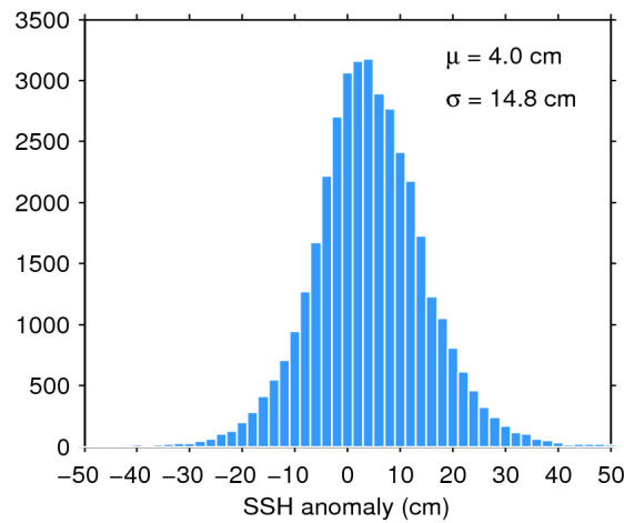
Figure 11. Histogram of science-valid SSH anomaly over oceans and lakes for 17/12/2018. The mean ( \mu ) and standard deviation ( \sigma ) are also shown. Note that values outside [-50 50] cm are excluded from the histogram for the sake of readability but not from the computation of \mu and \sigma .
