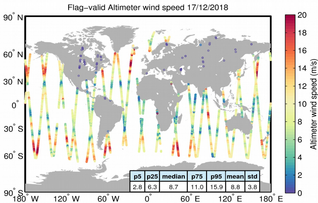
Figure 31. Geographical distribution of flag-valid wind data over oceans and lakes for 17/12/2018. The statistical values shown in the table refer to the wind in m/s and are calculated over all measurements shown in the figure.
