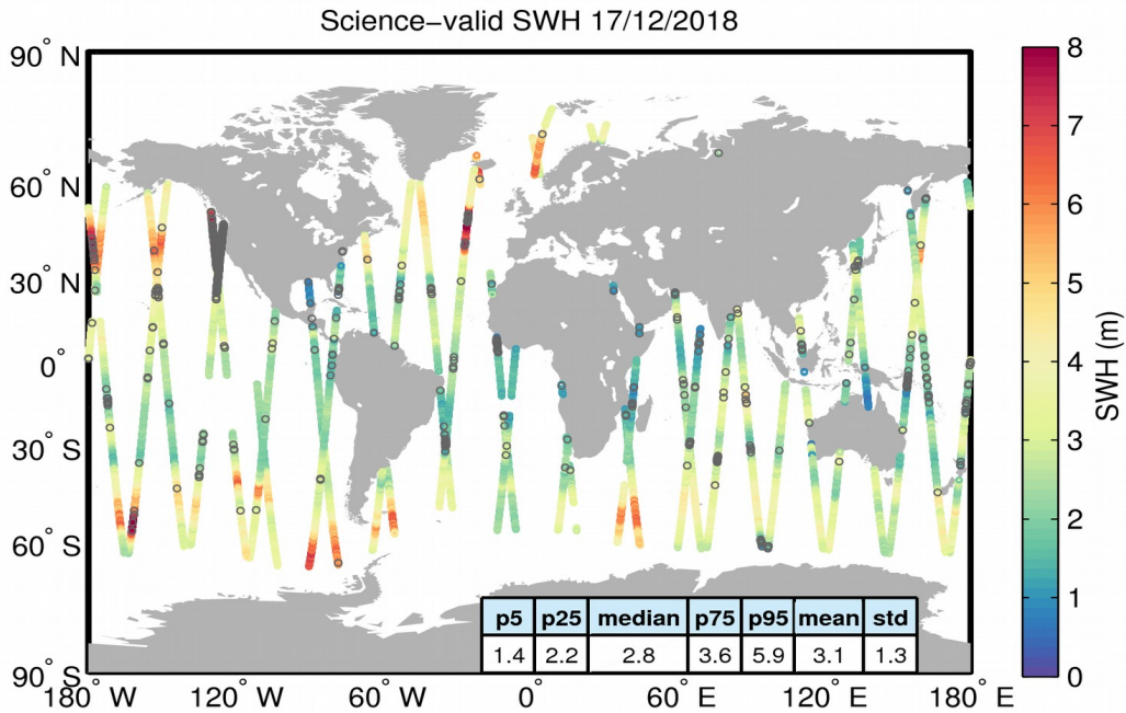
Figure 19. Geographical distribution of science-valid SWH data over oceans and lakes for 17/12/2018. The statistical values shown in the table refer to the SWH in m and are calculated over all measurements shown in the figure. Gray circles denote records that have been rejected based on the editing criteria described in Table 3.
