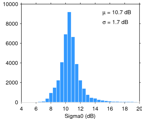
Figure 25. Histogram of flag-valid sigma0 over oceans and lakes for 17/12/2018. The mean ( \mu ) and standard deviation ( \sigma ) are also shown. Note that values outside [4 20] dB are excluded from the histogram for the sake of readability but not from the computation of \mu and \sigma .
