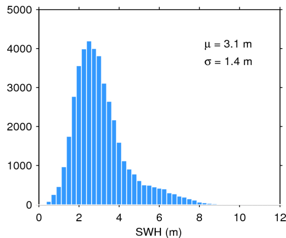
Figure 17. Histogram of flag-valid SWH over oceans and lakes for 17/12/2018. The mean ( \mu ) and standard deviation ( \sigma ) are also shown. Note that values larger than 12 m are excluded from the histogram for the sake of readability but not from the computation of \mu and \sigma .
