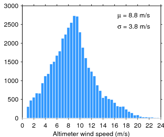
Figure 35. Histogram of science-valid wind over oceans and lakes for 17/12/2018. The mean ( \mu ) and standard deviation ( \sigma ) are also shown. Note that values larger than 24 m/s are excluded from the histogram for the sake of readability but not from the computation of \mu and \sigma .
