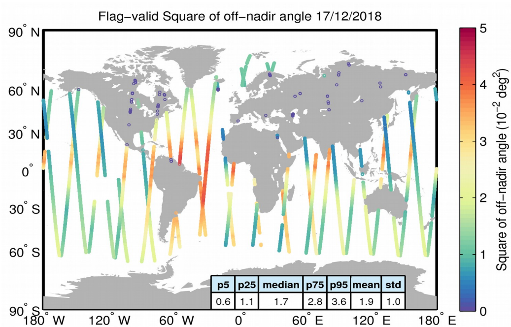
Figure 37. Geographical distribution of flag-valid mispointing data over oceans and lakes for 17/12/2018. The statistical values shown in the table refer to the mispointing in 10^{-2} deg 2 and are calculated over all measurements shown in the figure.
