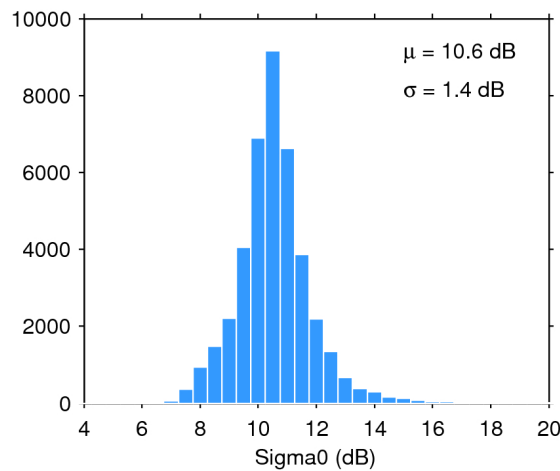
Figure 28. Histogram of science-valid sigma0 over oceans and lakes for 17/12/2018. The mean ( \mu ) and standard deviation ( \sigma ) are also shown. Note that values outside [4 20] dB are excluded from the histogram for the sake of readability but not from the computation of \mu and \sigma .
