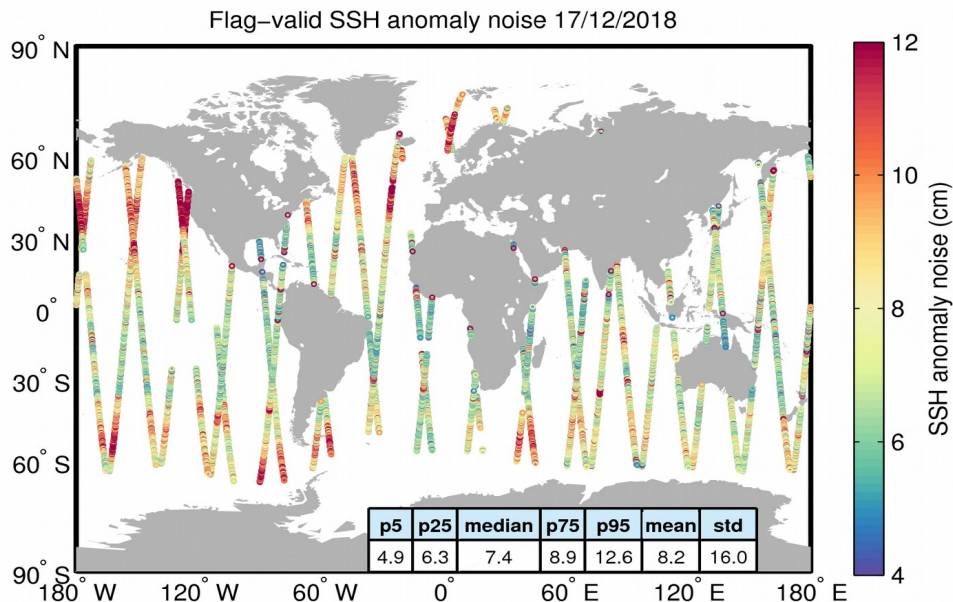
Figure 8. Geographical distribution of flag-valid 20-Hz SSH anomaly measurement noise over oceans and lakes for 17/12/2018. The statistical values shown in the table refer to the SSH anomaly noise and are calculated over all measurements shown in the figure.
