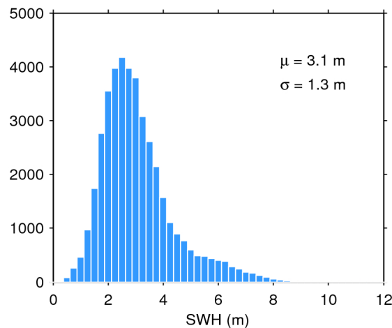
Figure 20. Histogram of science-valid SWH over oceans and lakes for 17/12/2018. The mean ( \mu ) and standard deviation ( \sigma ) are also shown. Note that values larger than 12 m are excluded from the histogram for the sake of readability but not from the computation of \mu and \sigma .
