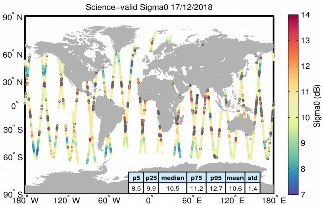
Figure 27. Geographical distribution of science-valid sigma0 data over oceans and lakes for 17/12/2018. The statistical values shown in the table refer to the sigma0 in dB and are calculated over all measurements shown in the figure. Gray circles denote records that have been rejected based on the editing criteria described in Table 4.
