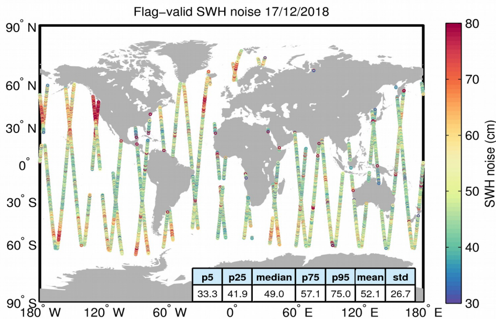
Figure 18. Geographical distribution of flag-valid 20-Hz SWH measurement noise over oceans and lakes for 17/12/2018. The statistical values shown in the figure refer to the SWH noise and are calculated over all measurements shown in the figure.
