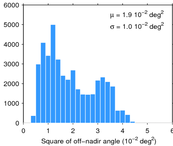
Figure 39. Histogram of flag-valid mispointing over oceans and lakes for 17/12/2018. The mean ( \mu ) and standard deviation ( \sigma ) are also shown. Note that values larger than 6 \cdot 10^{-2} \text{ deg}^2 are excluded from the histogram for the sake of readability but not from the computation of \mu and \sigma .
