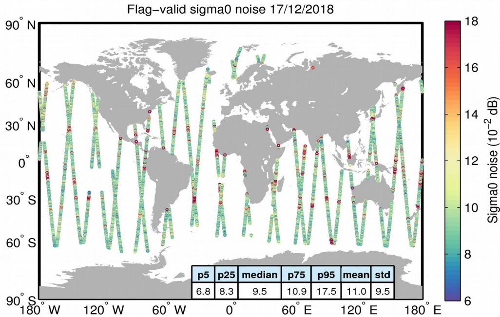
Figure 26. Geographical distribution of flag-valid 20-Hz sigma0 measurement noise over oceans and lakes for 17/12/2018. The statistical values shown in the table refer to the sigma0 noise and are calculated over all measurements shown in the figure.
