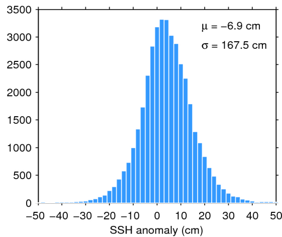
Figure 7. Histogram of flag-valid SSH anomaly over oceans and lakes for 17/12/2018. The mean ( \mu ) and standard deviation ( \sigma ) are also shown. Note that values outside [-50 50] cm are excluded from the histogram for the sake of readability but not from the computation of \mu and \sigma .
