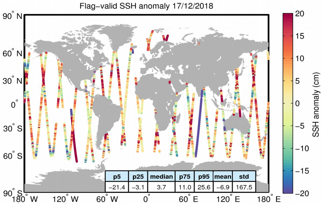
Figure 5. Geographical distribution of flag-valid 1-Hz SSH anomaly data over oceans and lakes for 17/12/2018. The statistical values shown in the table refer to the SSH anomaly in cm and are calculated over all measurements shown in the figure.
