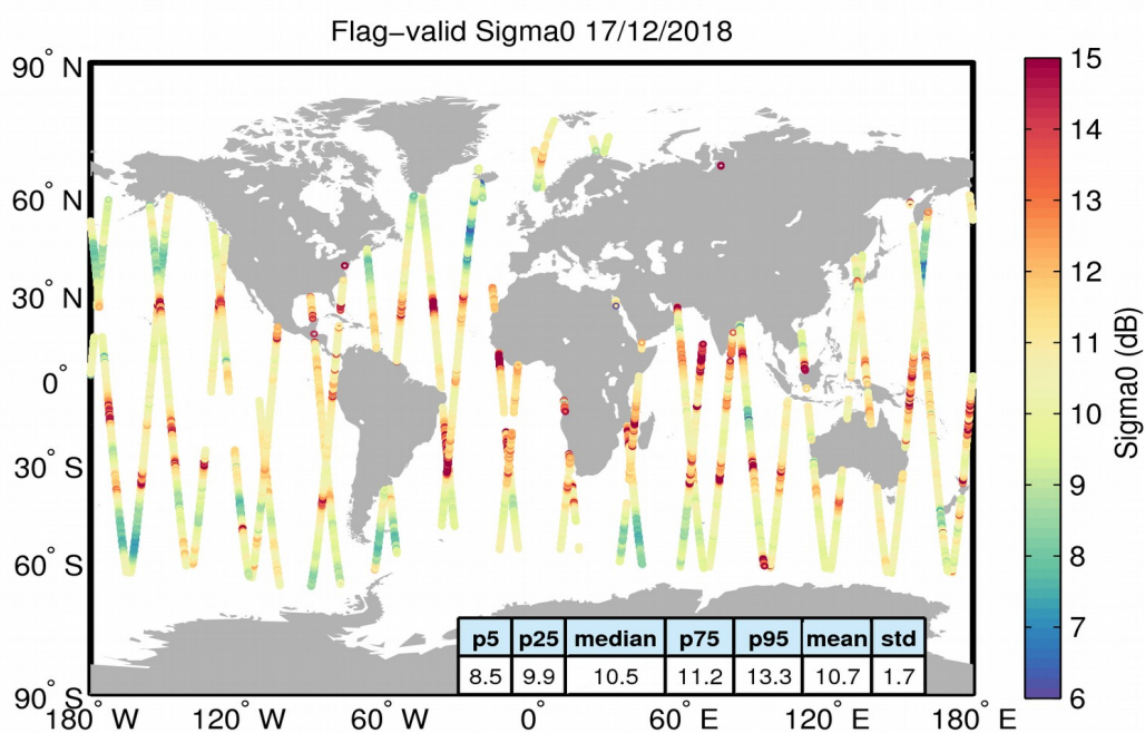
Figure 23. Geographical distribution of flag-valid sigma0 data over oceans and lakes for 17/12/2018. The statistical values shown in the table refer to the sigma0 in dB and are calculated over all measurements shown in the figure.
