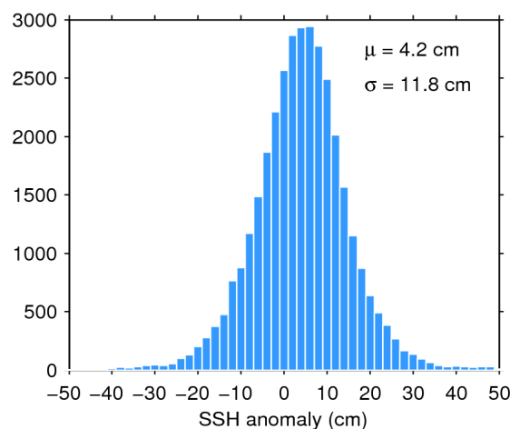
Figure 11. Histogram of science-valid SSH anomaly over oceans and lakes for 16/12/2018. The mean ( \mu ) and standard deviation ( \sigma ) are also shown. Note that values outside [-50 50] cm are excluded from the histogram for the sake of readability but not from the computation of \mu and \sigma .
