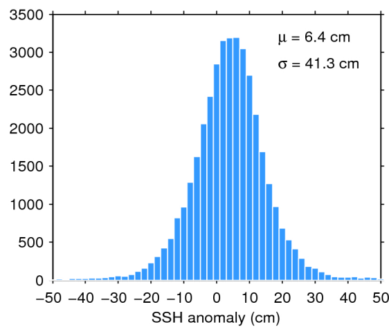
Figure 7. Histogram of flag-valid SSH anomaly over oceans and lakes for 16/12/2018. The mean ( \mu ) and standard deviation ( \sigma ) are also shown. Note that values outside [-50 50] cm are excluded from the histogram for the sake of readability but not from the computation of \mu and \sigma .
