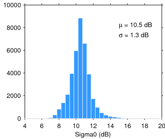
Figure 28. Histogram of science-valid sigma0 over oceans and lakes for 16/12/2018. The mean ( \mu ) and standard deviation ( \sigma ) are also shown. Note that values outside [4 20] dB are excluded from the histogram for the sake of readability but not from the computation of \mu and \sigma .
