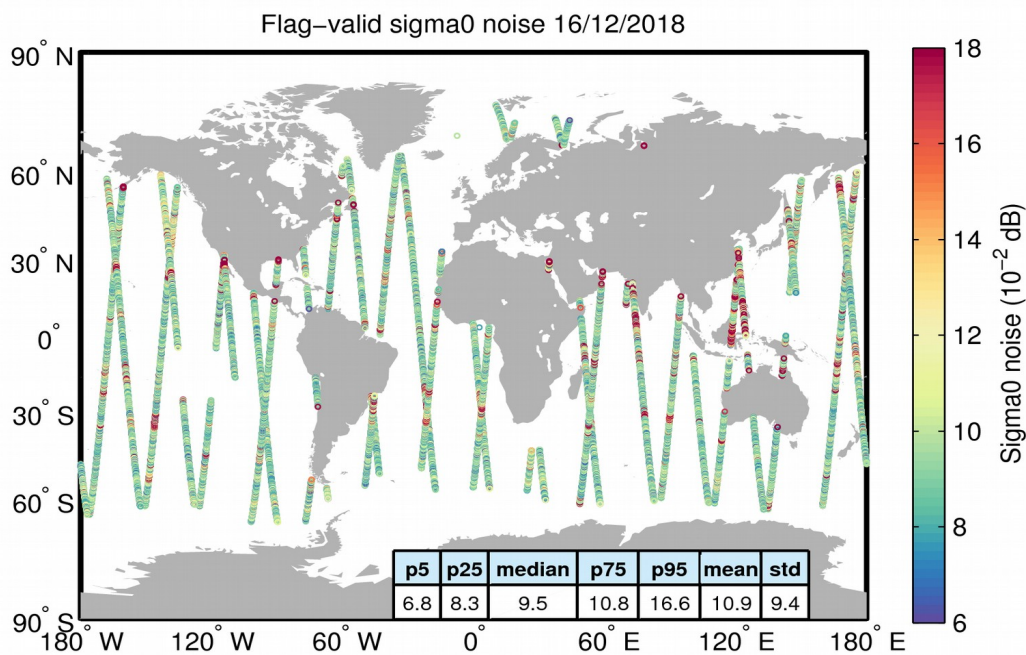
Figure 26. Geographical distribution of flag-valid 20-Hz sigma0 measurement noise over oceans and lakes for 16/12/2018. The statistical values shown in the table refer to the sigma0 noise and are calculated over all measurements shown in the figure.
