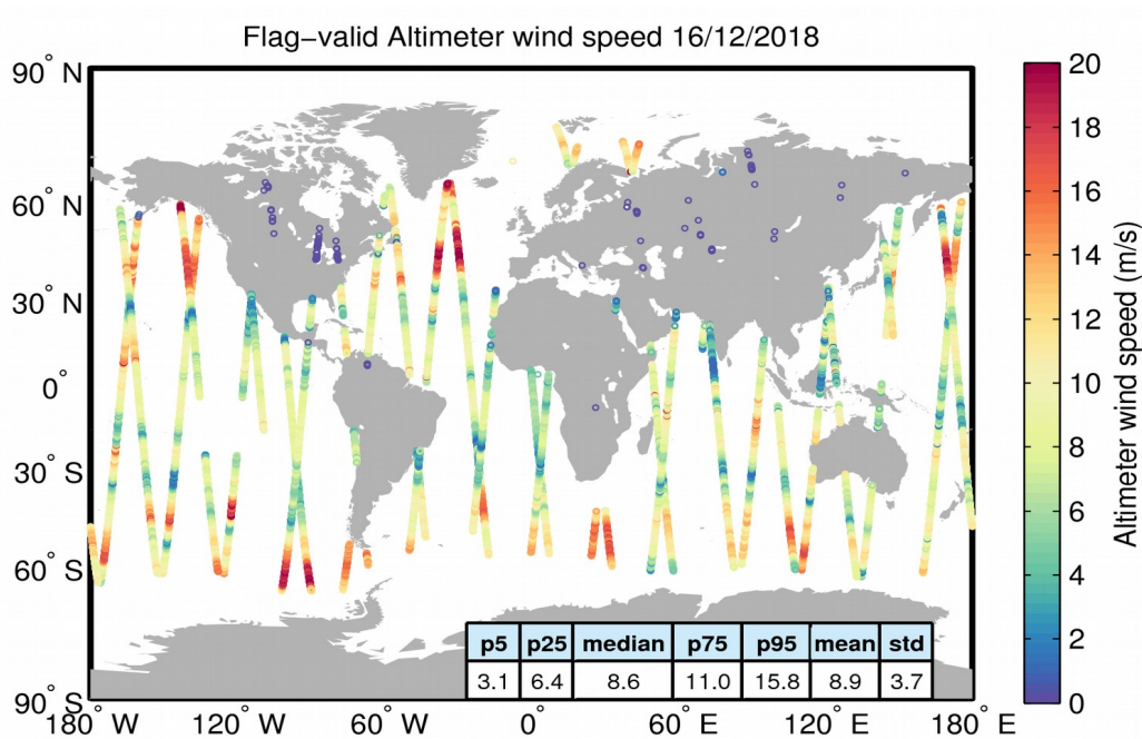
Figure 31. Geographical distribution of flag-valid wind data over oceans and lakes for 16/12/2018. The statistical values shown in the table refer to the wind in m/s and are calculated over all measurements shown in the figure.
