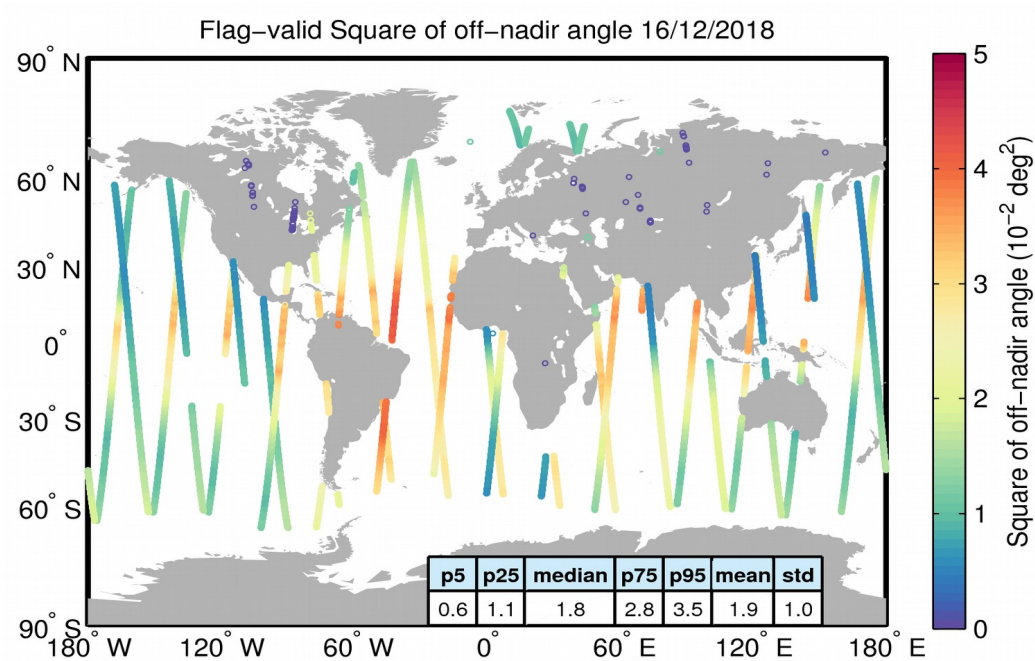
Figure 37. Geographical distribution of flag-valid mispointing data over oceans and lakes for 16/12/2018. The statistical values shown in the table refer to the mispointing in 10^{-2} \text{ deg}^2 and are calculated over all measurements shown in the figure.
