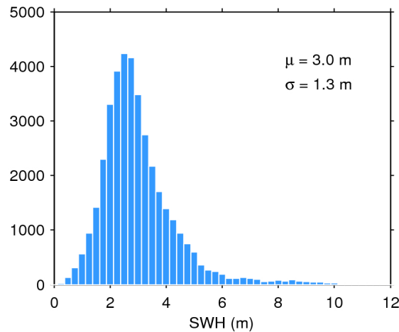
Figure 20. Histogram of science-valid SWH over oceans and lakes for 16/12/2018. The mean ( \mu ) and standard deviation ( \sigma ) are also shown. Note that values larger than 12 m are excluded from the histogram for the sake of readability but not from the computation of \mu and \sigma .
