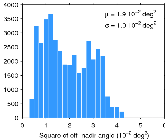
Figure 39. Histogram of flag-valid mispointing over oceans and lakes for 16/12/2018. The mean ( \mu ) and standard deviation ( \sigma ) are also shown. Note that values larger than 6 \cdot 10^{-2} \text{ deg}^2 are excluded from the histogram for the sake of readability but not from the computation of \mu and \sigma .
