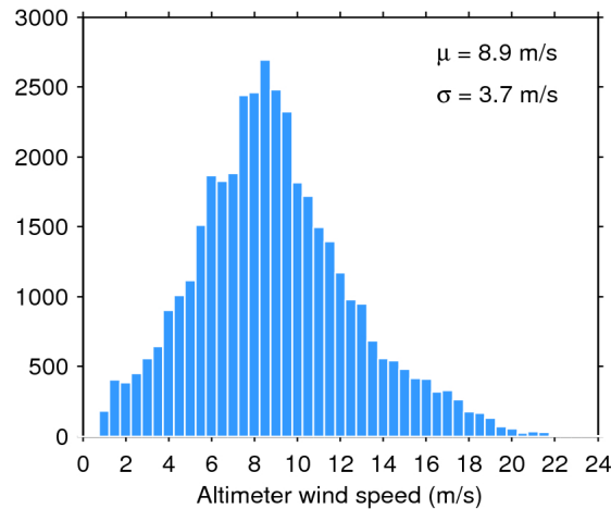
Figure 33. Histogram of flag-valid wind over oceans and lakes for 16/12/2018. The mean ( \mu ) and standard deviation ( \sigma ) are also shown. Note that values larger than 24 m/s are excluded from the histogram for the sake of readability but not from the computation of \mu and \sigma .
