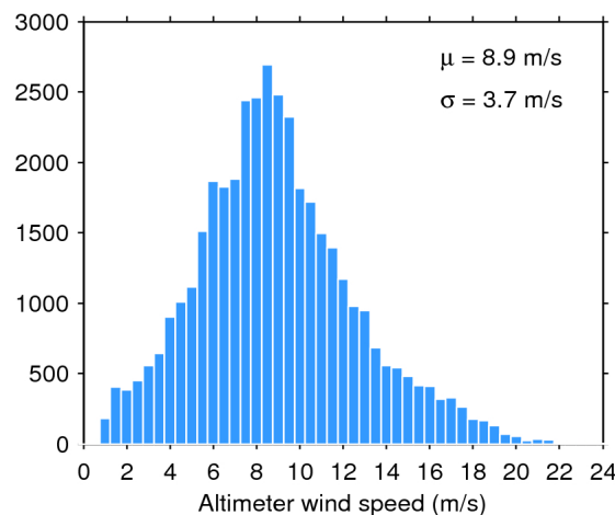
Figure 35. Histogram of science-valid wind over oceans and lakes for 16/12/2018. The mean ( \mu ) and standard deviation ( \sigma ) are also shown. Note that values larger than 24 m/s are excluded from the histogram for the sake of readability but not from the computation of \mu and \sigma .
