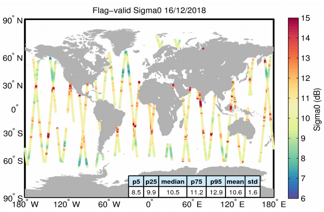
Figure 23. Geographical distribution of flag-valid sigma0 data over oceans and lakes for 16/12/2018. The statistical values shown in the table refer to the sigma0 in dB and are calculated over all measurements shown in the figure.
