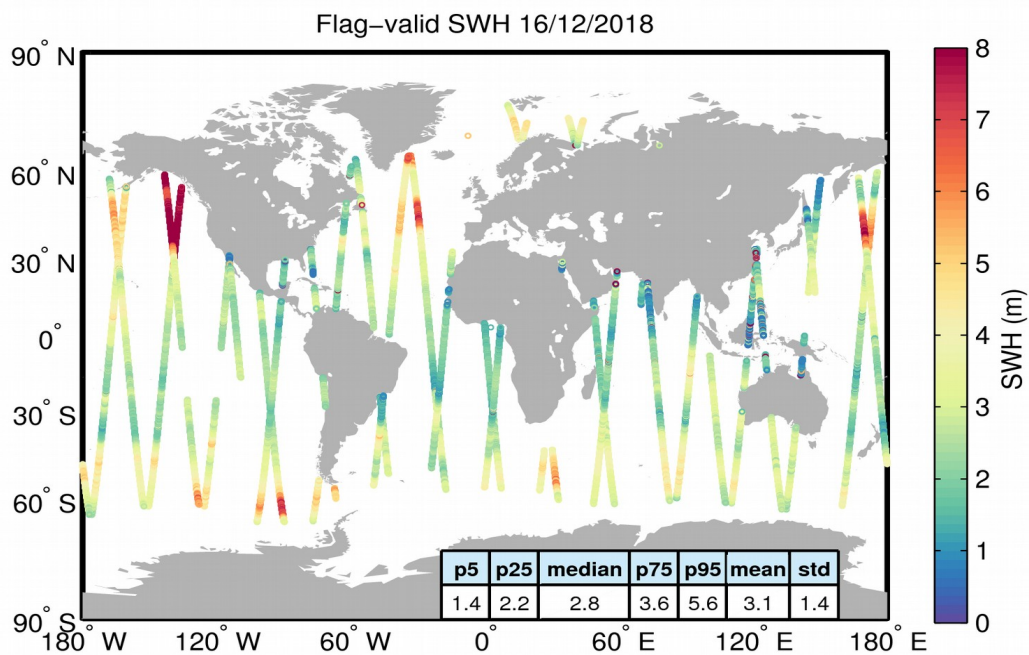
Figure 15. Geographical distribution of flag-valid SWH data over oceans and lakes for 16/12/2018. The statistical values shown in the table refer to the SWH in m and are calculated over all measurements shown in the figure.
