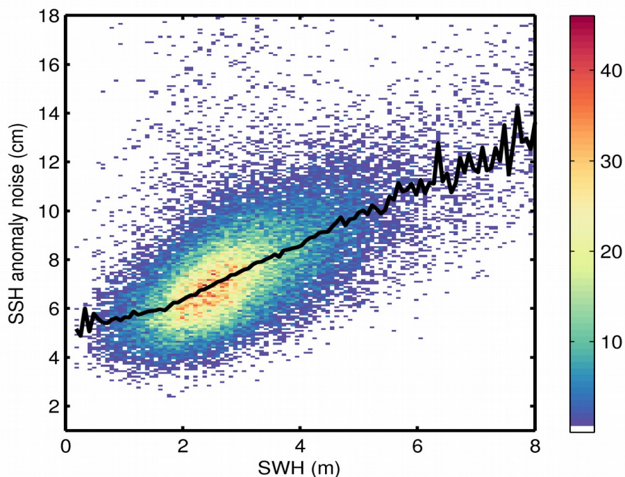
Figure 9. 2D histogram showing flag-valid SSH anomaly noise as a function of SWH for 16/12/2018. The black line denotes the median SSH anomaly noise as a function of SWH.
