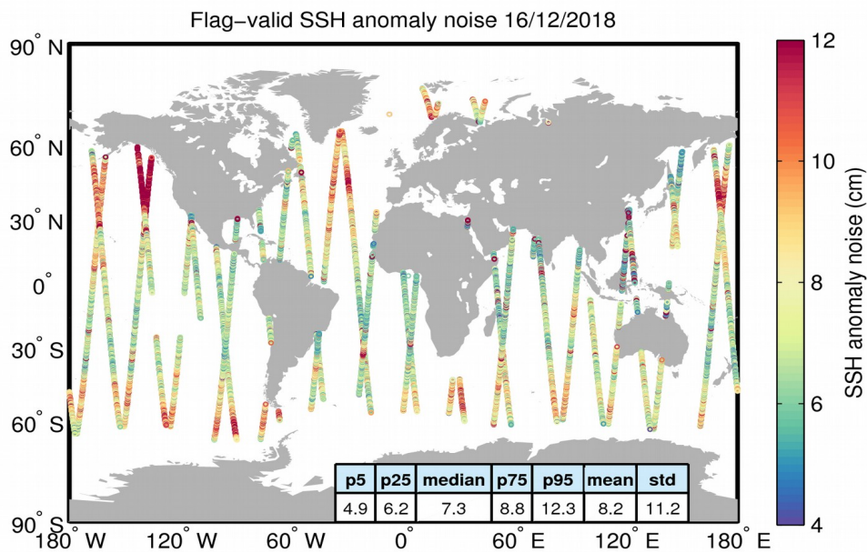
Figure 8. Geographical distribution of flag-valid 20-Hz SSH anomaly measurement noise over oceans and lakes for 16/12/2018. The statistical values shown in the table refer to the SSH anomaly noise and are calculated over all measurements shown in the figure.
