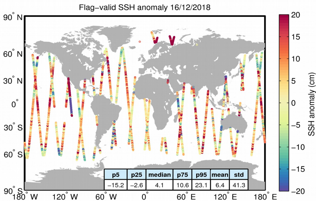
Figure 5. Geographical distribution of flag-valid 1-Hz SSH anomaly data over oceans and lakes for 16/12/2018. The statistical values shown in the table refer to the SSH anomaly in cm and are calculated over all measurements shown in the figure.
