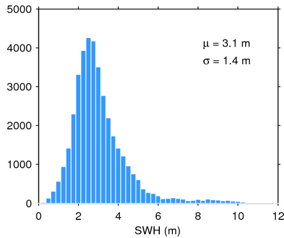
Figure 17. Histogram of flag-valid SWH over oceans and lakes for 16/12/2018. The mean ( \mu ) and standard deviation ( \sigma ) are also shown. Note that values larger than 12 m are excluded from the histogram for the sake of readability but not from the computation of \mu and \sigma .
