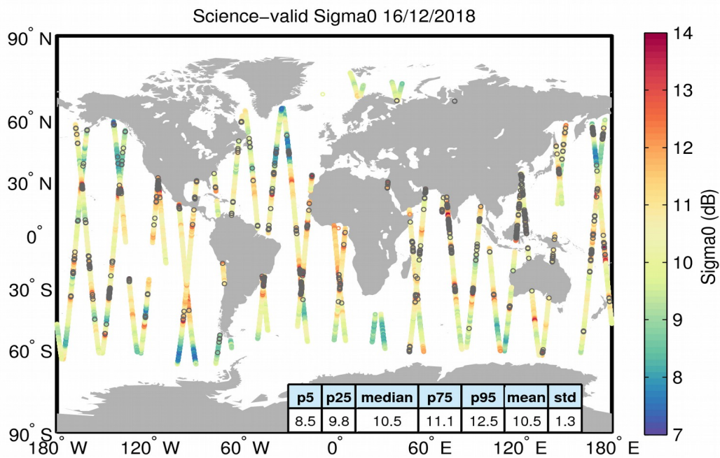
Figure 27. Geographical distribution of science-valid sigma0 data over oceans and lakes for 16/12/2018. The statistical values shown in the table refer to the sigma0 in dB and are calculated over all measurements shown in the figure. Gray circles denote records that have been rejected based on the editing criteria described in Table 4.
