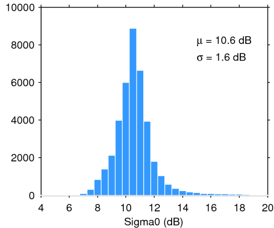
Figure 25. Histogram of flag-valid sigma0 over oceans and lakes for 16/12/2018. The mean ( \mu ) and standard deviation ( \sigma ) are also shown. Note that values outside [4 20] dB are excluded from the histogram for the sake of readability but not from the computation of \mu and \sigma .
