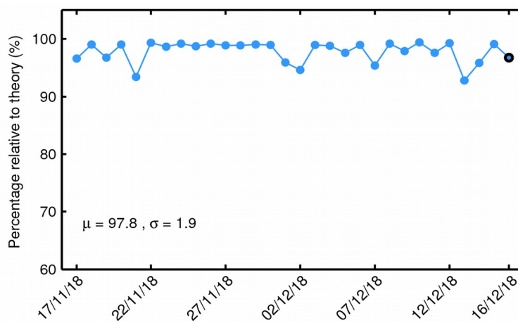
Figure 24. Percentage of flag-valid 1-Hz sigma0 records over ocean and lakes relative to theory for each day in last 30-day window. The mean ( \mu ) and standard deviation ( \sigma ) are also shown.
