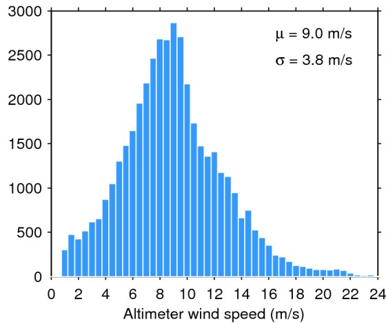
Figure 33. Histogram of flag-valid wind over oceans and lakes for 15/12/2018. The mean ( \mu ) and standard deviation ( \sigma ) are also shown. Note that values larger than 24 m/s are excluded from the histogram for the sake of readability but not from the computation of \mu and \sigma .
