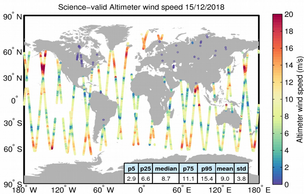
Figure 34. Geographical distribution of science-valid wind data over oceans and lakes for 15/12/2018. The statistical values shown in the table refer to the wind in m/s and are calculated over all measurements shown in the figure. Gray circles denote records that have been rejected based on the editing criteria described in Table 5.
