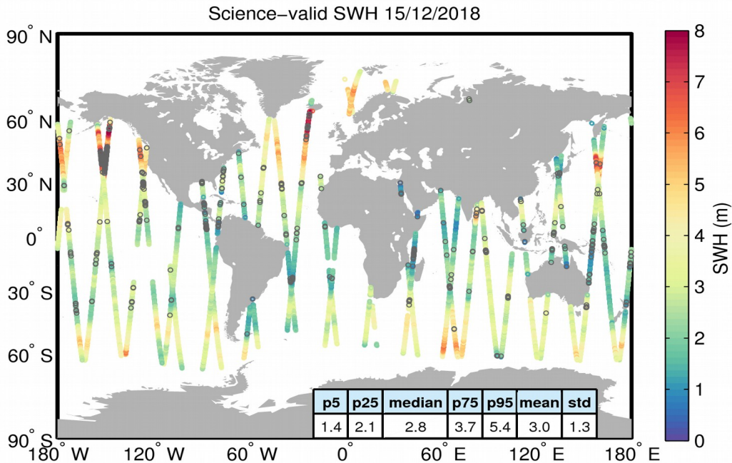
Figure 19. Geographical distribution of science-valid SWH data over oceans and lakes for 15/12/2018. The statistical values shown in the table refer to the SWH in m and are calculated over all measurements shown in the figure. Gray circles denote records that have been rejected based on the editing criteria described in Table 3.
