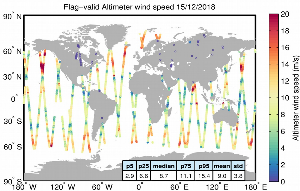
Figure 31. Geographical distribution of flag-valid wind data over oceans and lakes for 15/12/2018. The statistical values shown in the table refer to the wind in m/s and are calculated over all measurements shown in the figure.
