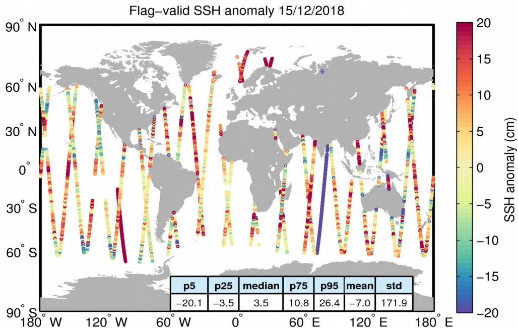
Figure 5. Geographical distribution of flag-valid 1-Hz SSH anomaly data over oceans and lakes for 15/12/2018. The statistical values shown in the table refer to the SSH anomaly in cm and are calculated over all measurements shown in the figure.
