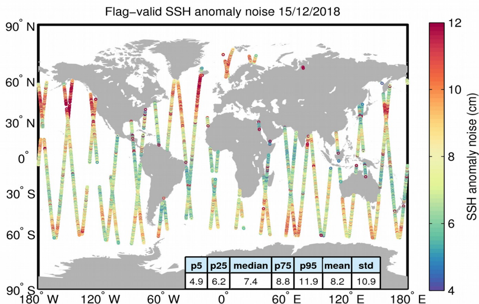
Figure 8. Geographical distribution of flag-valid 20-Hz SSH anomaly measurement noise over oceans and lakes for 15/12/2018. The statistical values shown in the table refer to the SSH anomaly noise and are calculated over all measurements shown in the figure.
