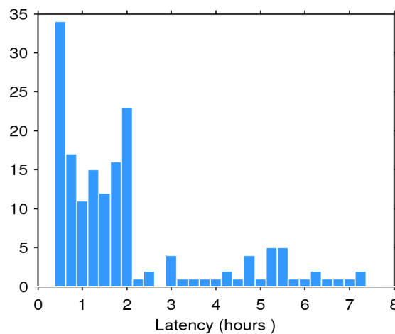
Figure 2. Histogram of the data latency for 15/12/2018. The y-axis denotes the number of files that are made available with a delay of x-hours with respect to the mean time of the records stored in the file.
