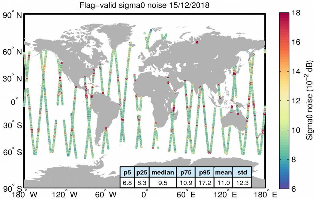
Figure 26. Geographical distribution of flag-valid 20-Hz sigma0 measurement noise over oceans and lakes for 15/12/2018. The statistical values shown in the table refer to the sigma0 noise and are calculated over all measurements shown in the figure.
