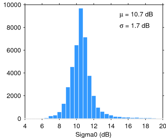
Figure 25. Histogram of flag-valid sigma0 over oceans and lakes for 15/12/2018. The mean ( \mu ) and standard deviation ( \sigma ) are also shown. Note that values outside [4 20] dB are excluded from the histogram for the sake of readability but not from the computation of \mu and \sigma .
