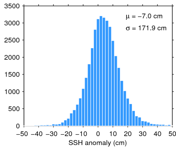
Figure 7. Histogram of flag-valid SSH anomaly over oceans and lakes for 15/12/2018. The mean ( \mu ) and standard deviation ( \sigma ) are also shown. Note that values outside [-50\ 50] cm are excluded from the histogram for the sake of readability but not from the computation of \mu and \sigma .
