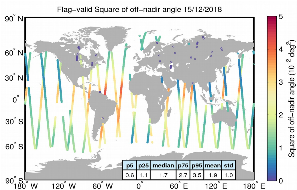
Figure 37. Geographical distribution of flag-valid mispointing data over oceans and lakes for 15/12/2018. The statistical values shown in the table refer to the mispointing in 10^{-2} deg 2 and are calculated over all measurements shown in the figure.
