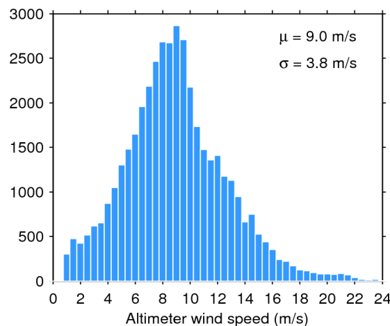
Figure 35. Histogram of science-valid wind over oceans and lakes for 15/12/2018. The mean ( \mu ) and standard deviation ( \sigma ) are also shown. Note that values larger than 24 m/s are excluded from the histogram for the sake of readability but not from the computation of \mu and \sigma .
