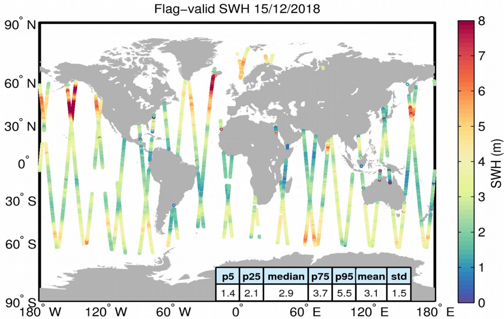
Figure 15. Geographical distribution of flag-valid SWH data over oceans and lakes for 15/12/2018. The statistical values shown in the table refer to the SWH in m and are calculated over all measurements shown in the figure.
