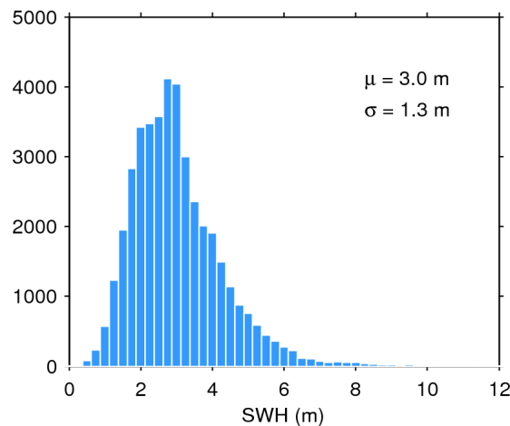
Figure 20. Histogram of science-valid SWH over oceans and lakes for 15/12/2018. The mean ( \mu ) and standard deviation ( \sigma ) are also shown. Note that values larger than 12 m are excluded from the histogram for the sake of readability but not from the computation of \mu and \sigma .
