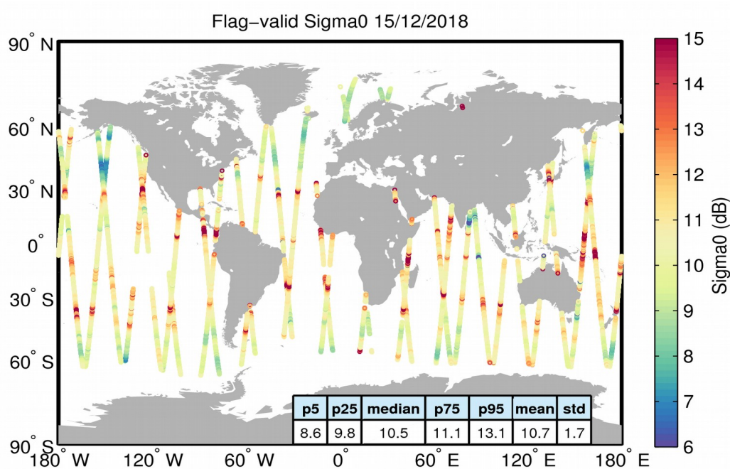
Figure 23. Geographical distribution of flag-valid sigma0 data over oceans and lakes for 15/12/2018. The statistical values shown in the table refer to the sigma0 in dB and are calculated over all measurements shown in the figure.
