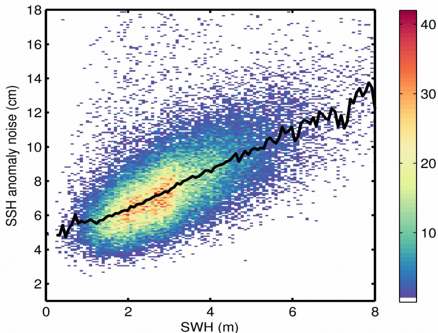
Figure 9. 2D histogram showing flag-valid SSH anomaly noise as a function of SWH for 15/12/2018. The black line denotes the median SSH anomaly noise as a function of SWH.
