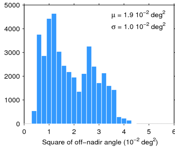
Figure 39. Histogram of flag-valid mispointing over oceans and lakes for 15/12/2018. The mean ( \mu ) and standard deviation ( \sigma ) are also shown. Note that values larger than 6 \cdot 10^{-2} \text{ deg}^2 are excluded from the histogram for the sake of readability but not from the computation of \mu and \sigma .
