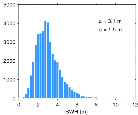
Figure 17. Histogram of flag-valid SWH over oceans and lakes for 15/12/2018. The mean ( \mu ) and standard deviation ( \sigma ) are also shown. Note that values larger than 12 m are excluded from the histogram for the sake of readability but not from the computation of \mu and \sigma .
