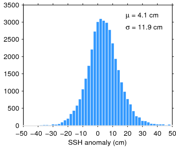
Figure 11. Histogram of science-valid SSH anomaly over oceans and lakes for 15/12/2018. The mean ( \mu ) and standard deviation ( \sigma ) are also shown. Note that values outside [-50 50] cm are excluded from the histogram for the sake of readability but not from the computation of \mu and \sigma .
