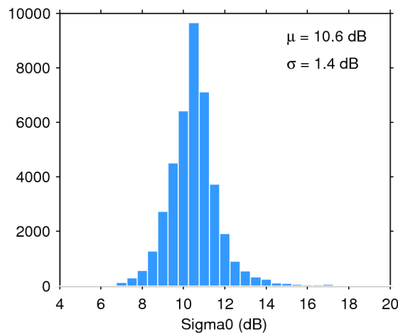
Figure 28. Histogram of science-valid sigma0 over oceans and lakes for 15/12/2018. The mean ( \mu ) and standard deviation ( \sigma ) are also shown. Note that values outside [4 20] dB are excluded from the histogram for the sake of readability but not from the computation of \mu and \sigma .
