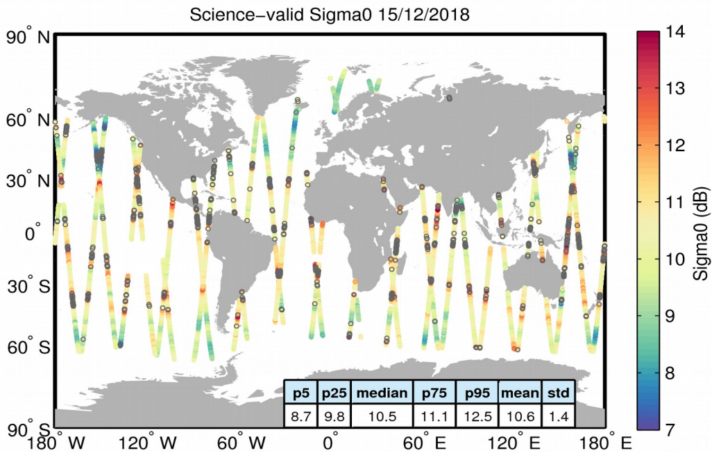
Figure 27. Geographical distribution of science-valid sigma0 data over oceans and lakes for 15/12/2018. The statistical values shown in the table refer to the sigma0 in dB and are calculated over all measurements shown in the figure. Gray circles denote records that have been rejected based on the editing criteria described in Table 4.
