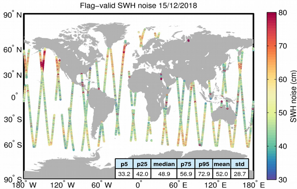
Figure 18. Geographical distribution of flag-valid 20-Hz SWH measurement noise over oceans and lakes for 15/12/2018. The statistical values shown in the figure refer to the SWH noise and are calculated over all measurements shown in the figure.
