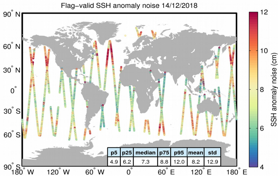
Figure 8. Geographical distribution of flag-valid 20-Hz SSH anomaly measurement noise over oceans and lakes for 14/12/2018. The statistical values shown in the table refer to the SSH anomaly noise and are calculated over all measurements shown in the figure.
