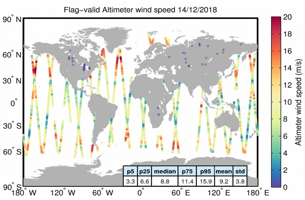
Figure 31. Geographical distribution of flag-valid wind data over oceans and lakes for 14/12/2018. The statistical values shown in the table refer to the wind in m/s and are calculated over all measurements shown in the figure.
