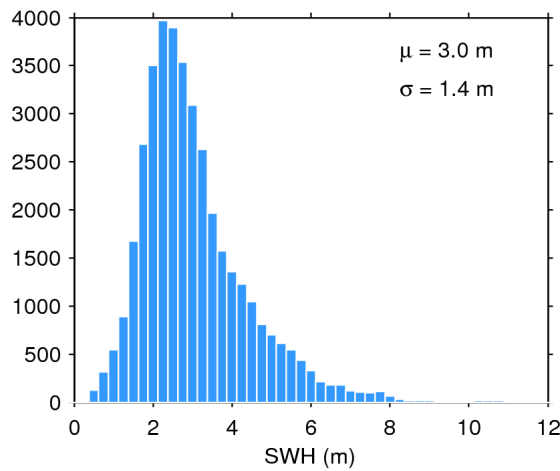
Figure 17. Histogram of flag-valid SWH over oceans and lakes for 14/12/2018. The mean ( \mu ) and standard deviation ( \sigma ) are also shown. Note that values larger than 12 m are excluded from the histogram for the sake of readability but not from the computation of \mu and \sigma .
