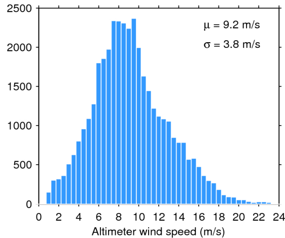
Figure 33. Histogram of flag-valid wind over oceans and lakes for 14/12/2018. The mean ( \mu ) and standard deviation ( \sigma ) are also shown. Note that values larger than 24 m/s are excluded from the histogram for the sake of readability but not from the computation of \mu and \sigma .
