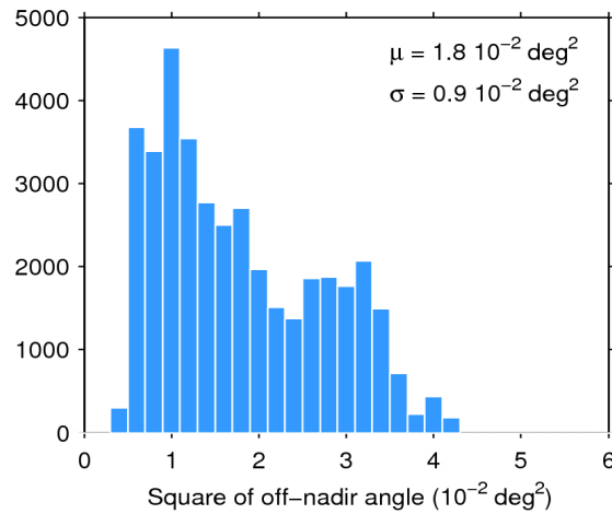
Figure 39. Histogram of flag-valid mispointing over oceans and lakes for 14/12/2018. The mean ( \mu ) and standard deviation ( \sigma ) are also shown. Note that values larger than 6 \cdot 10^{-2} \text{ deg}^2 are excluded from the histogram for the sake of readability but not from the computation of \mu and \sigma .
