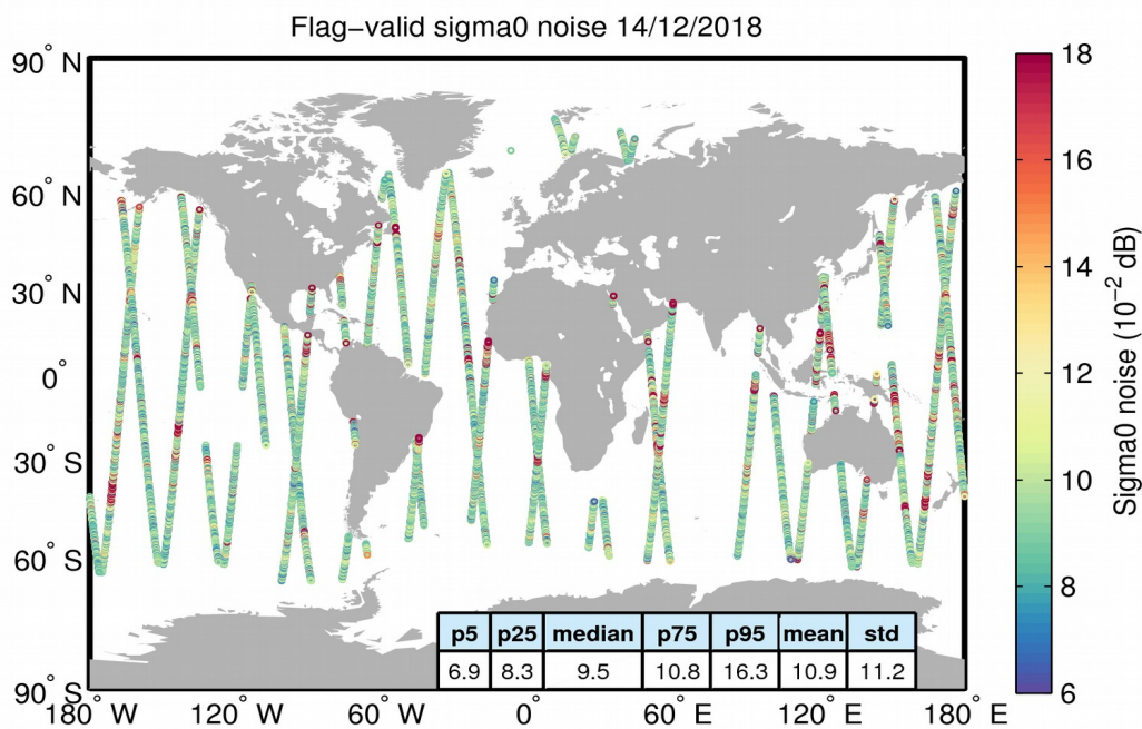
Figure 26. Geographical distribution of flag-valid 20-Hz sigma0 measurement noise over oceans and lakes for 14/12/2018. The statistical values shown in the table refer to the sigma0 noise and are calculated over all measurements shown in the figure.
