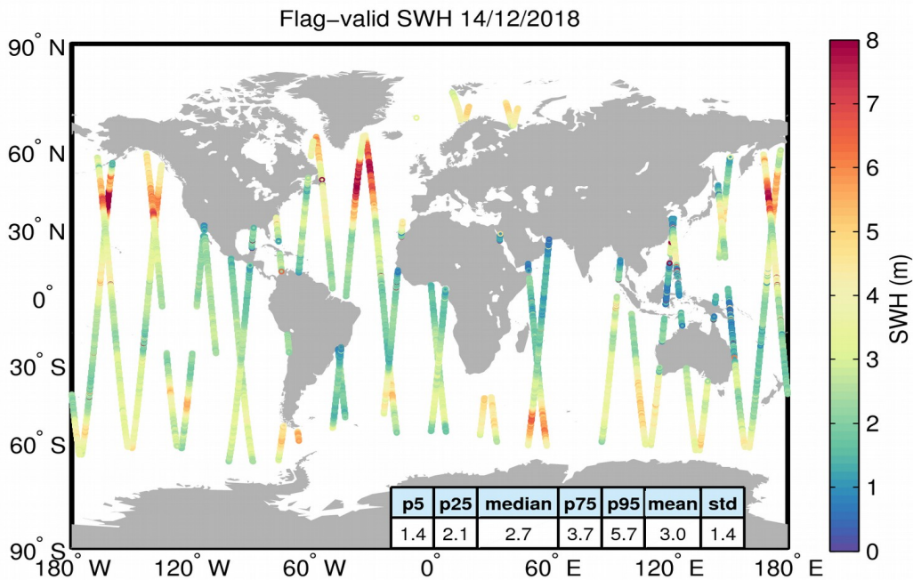
Figure 15. Geographical distribution of flag-valid SWH data over oceans and lakes for 14/12/2018. The statistical values shown in the table refer to the SWH in m and are calculated over all measurements shown in the figure.
