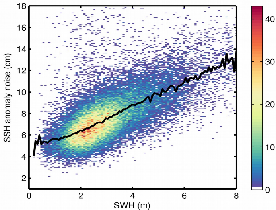
Figure 9. 2D histogram showing flag-valid SSH anomaly noise as a function of SWH for 14/12/2018. The black line denotes the median SSH anomaly noise as a function of SWH.
