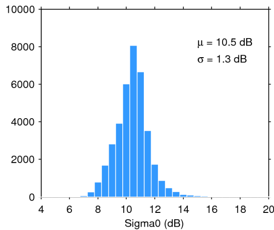
Figure 28. Histogram of science-valid sigma0 over oceans and lakes for 14/12/2018. The mean ( \mu ) and standard deviation ( \sigma ) are also shown. Note that values outside [4 20] dB are excluded from the histogram for the sake of readability but not from the computation of \mu and \sigma .
