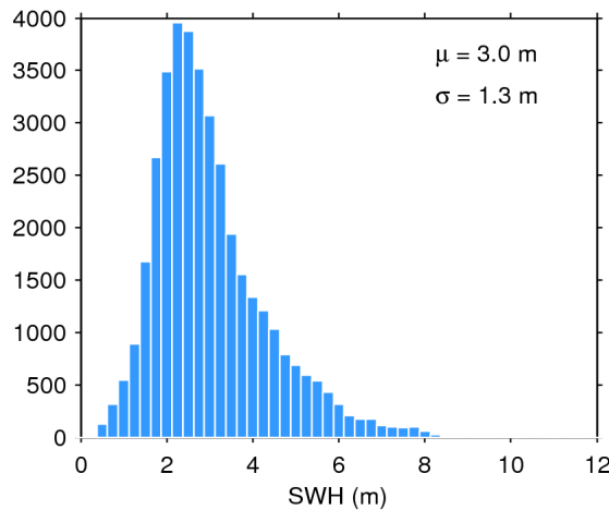
Figure 20. Histogram of science-valid SWH over oceans and lakes for 14/12/2018. The mean ( \mu ) and standard deviation ( \sigma ) are also shown. Note that values larger than 12 m are excluded from the histogram for the sake of readability but not from the computation of \mu and \sigma .
