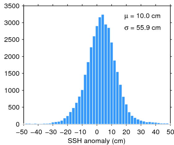
Figure 7. Histogram of flag-valid SSH anomaly over oceans and lakes for 14/12/2018. The mean ( \mu ) and standard deviation ( \sigma ) are also shown. Note that values outside [-50 50] cm are excluded from the histogram for the sake of readability but not from the computation of \mu and \sigma .
