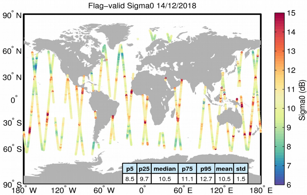
Figure 23. Geographical distribution of flag-valid sigma0 data over oceans and lakes for 14/12/2018. The statistical values shown in the table refer to the sigma0 in dB and are calculated over all measurements shown in the figure.
