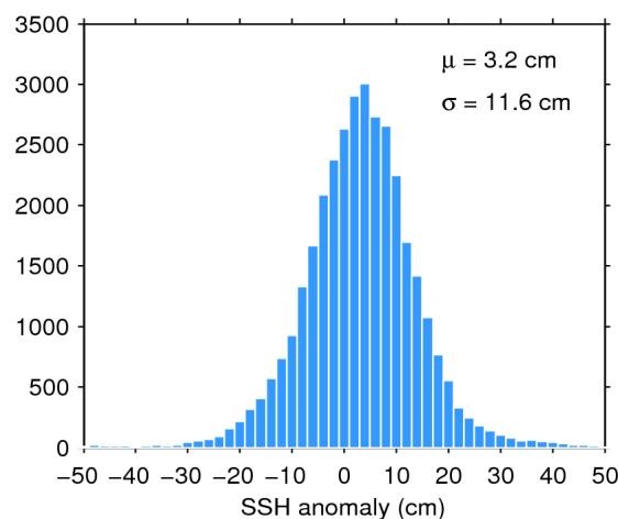
Figure 11. Histogram of science-valid SSH anomaly over oceans and lakes for 14/12/2018. The mean ( \mu ) and standard deviation ( \sigma ) are also shown. Note that values outside [-50 50] cm are excluded from the histogram for the sake of readability but not from the computation of \mu and \sigma .
