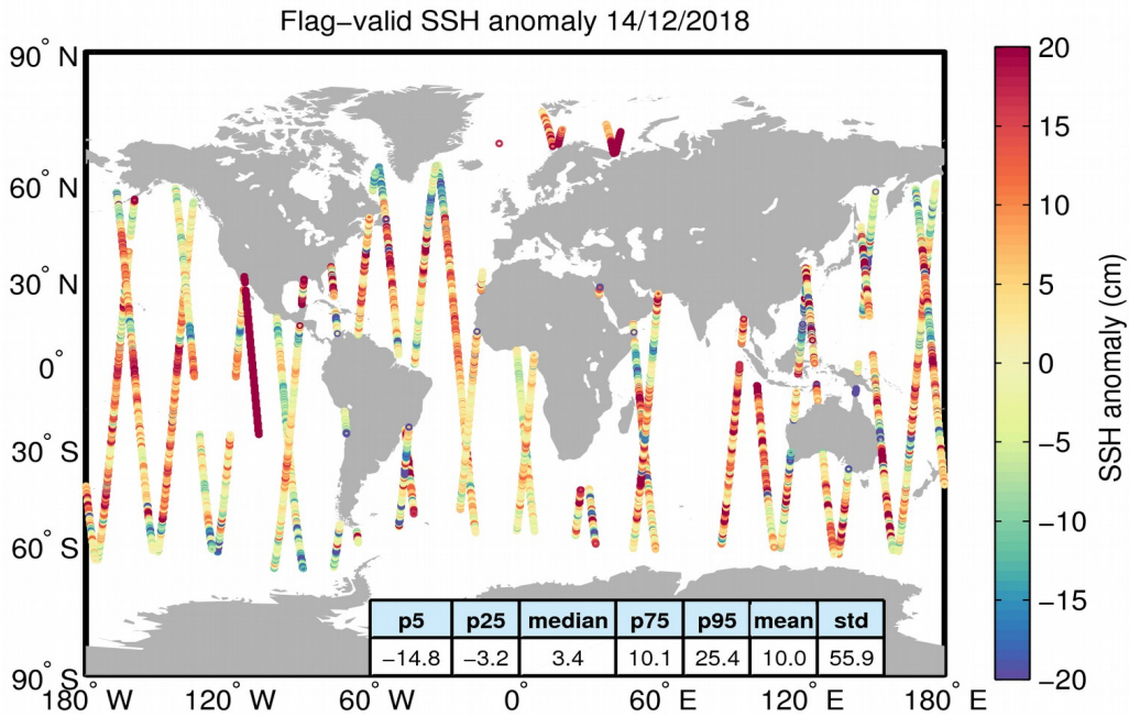
Figure 5. Geographical distribution of flag-valid 1-Hz SSH anomaly data over oceans and lakes for 14/12/2018. The statistical values shown in the table refer to the SSH anomaly in cm and are calculated over all measurements shown in the figure.
