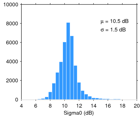
Figure 25. Histogram of flag-valid sigma0 over oceans and lakes for 14/12/2018. The mean ( \mu ) and standard deviation ( \sigma ) are also shown. Note that values outside [4 20] dB are excluded from the histogram for the sake of readability but not from the computation of \mu and \sigma .
