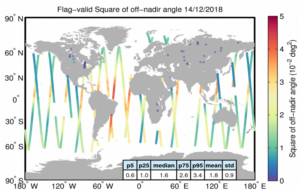
Figure 37. Geographical distribution of flag-valid mispointing data over oceans and lakes for 14/12/2018. The statistical values shown in the table refer to the mispointing in 10^{-2} deg 2 and are calculated over all measurements shown in the figure.
