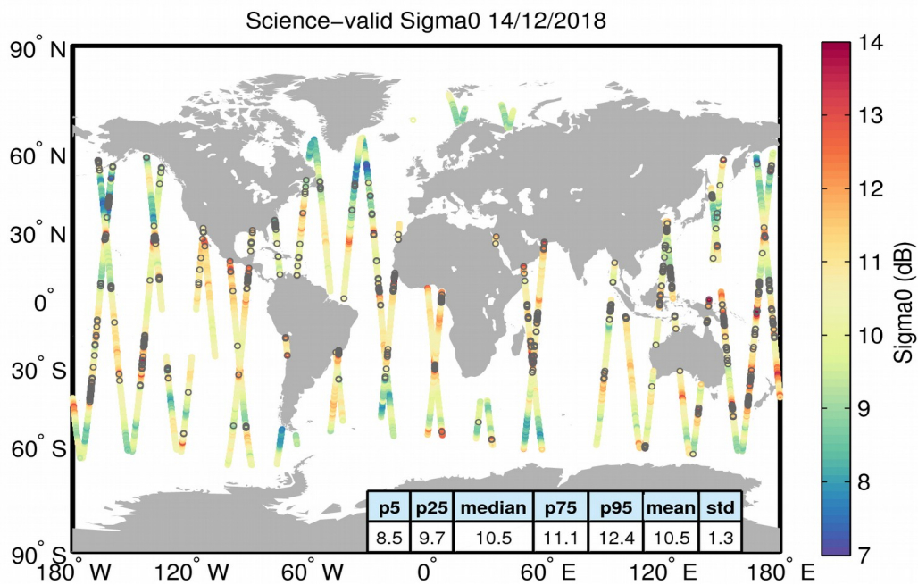
Figure 27. Geographical distribution of science-valid sigma0 data over oceans and lakes for 14/12/2018. The statistical values shown in the table refer to the sigma0 in dB and are calculated over all measurements shown in the figure. Gray circles denote records that have been rejected based on the editing criteria described in Table 4.
