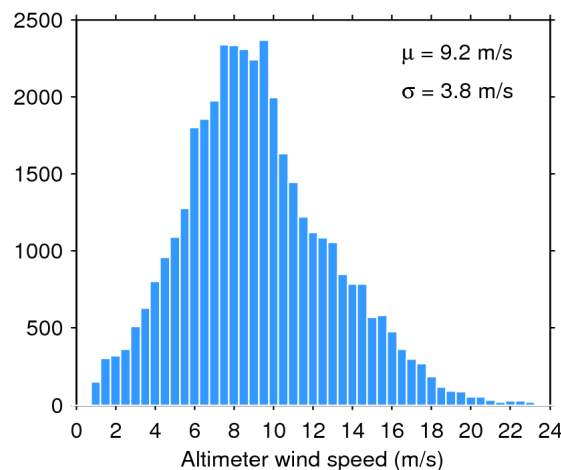
Figure 35. Histogram of science-valid wind over oceans and lakes for 14/12/2018. The mean ( \mu ) and standard deviation ( \sigma ) are also shown. Note that values larger than 24 m/s are excluded from the histogram for the sake of readability but not from the computation of \mu and \sigma .
