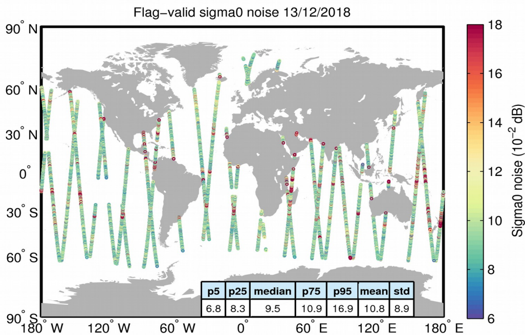
Figure 26. Geographical distribution of flag-valid 20-Hz sigma0 measurement noise over oceans and lakes for 13/12/2018. The statistical values shown in the table refer to the sigma0 noise and are calculated over all measurements shown in the figure.
