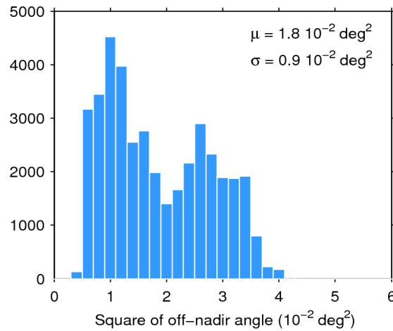
Figure 39. Histogram of flag-valid mispointing over oceans and lakes for 13/12/2018. The mean ( \mu ) and standard deviation ( \sigma ) are also shown. Note that values larger than 6 \cdot 10^{-2} \text{ deg}^2 are excluded from the histogram for the sake of readability but not from the computation of \mu and \sigma .
