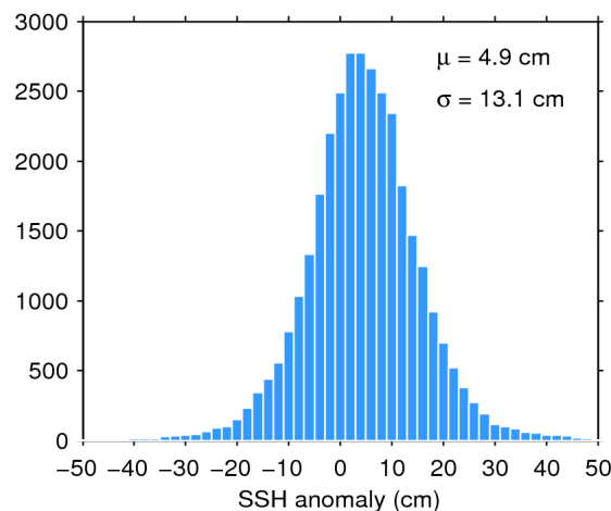
Figure 11. Histogram of science-valid SSH anomaly over oceans and lakes for 13/12/2018. The mean ( \mu ) and standard deviation ( \sigma ) are also shown. Note that values outside [-50 50] cm are excluded from the histogram for the sake of readability but not from the computation of \mu and \sigma .
