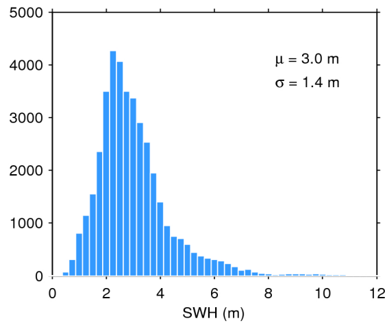
Figure 17. Histogram of flag-valid SWH over oceans and lakes for 13/12/2018. The mean ( \mu ) and standard deviation ( \sigma ) are also shown. Note that values larger than 12 m are excluded from the histogram for the sake of readability but not from the computation of \mu and \sigma .
