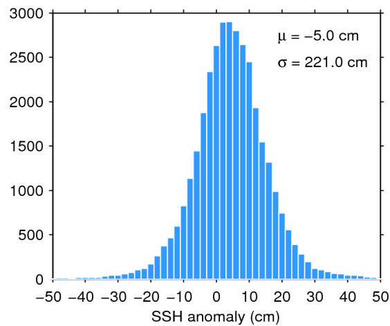
Figure 7. Histogram of flag-valid SSH anomaly over oceans and lakes for 13/12/2018. The mean ( \mu ) and standard deviation ( \sigma ) are also shown. Note that values outside [-50 50] cm are excluded from the histogram for the sake of readability but not from the computation of \mu and \sigma .
