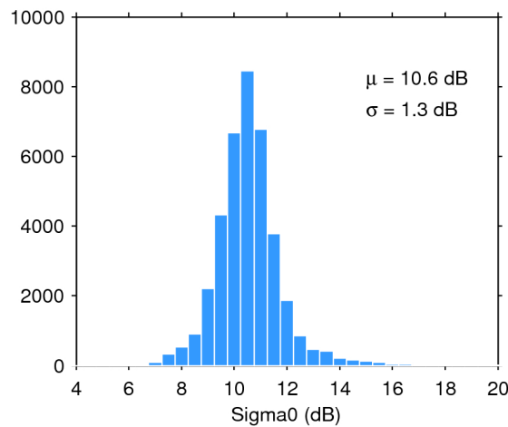
Figure 28. Histogram of science-valid sigma0 over oceans and lakes for 13/12/2018. The mean ( \mu ) and standard deviation ( \sigma ) are also shown. Note that values outside [4 20] dB are excluded from the histogram for the sake of readability but not from the computation of \mu and \sigma .
