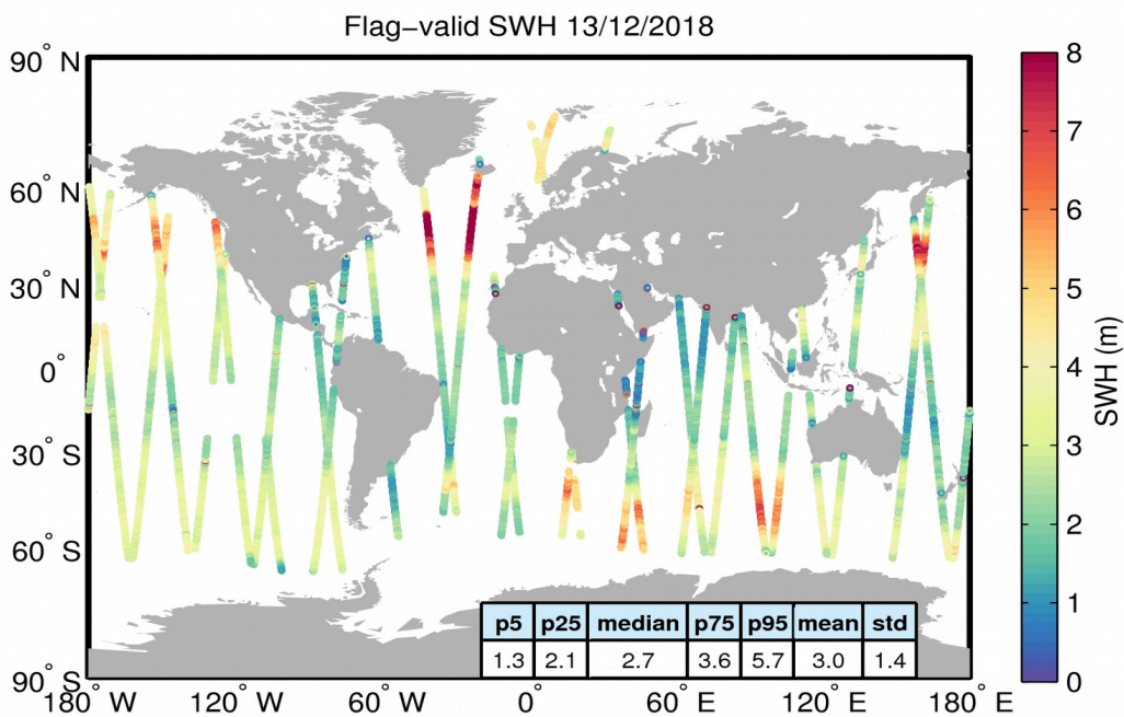
Figure 15. Geographical distribution of flag-valid SWH data over oceans and lakes for 13/12/2018. The statistical values shown in the table refer to the SWH in m and are calculated over all measurements shown in the figure.
