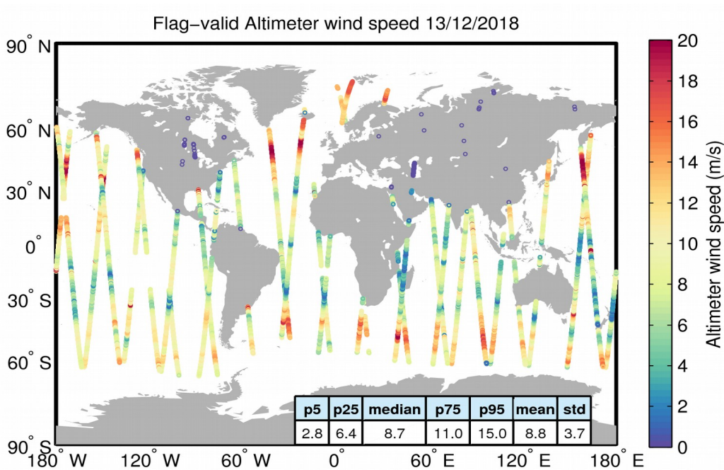
Figure 31. Geographical distribution of flag-valid wind data over oceans and lakes for 13/12/2018. The statistical values shown in the table refer to the wind in m/s and are calculated over all measurements shown in the figure.
