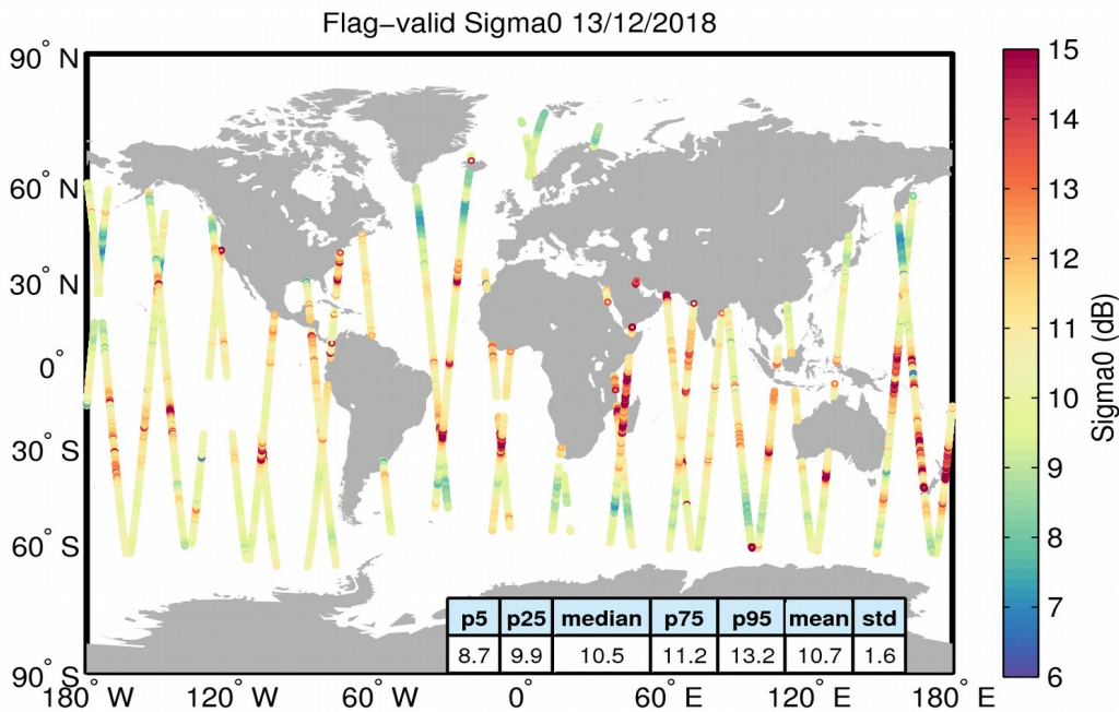
Figure 23. Geographical distribution of flag-valid sigma0 data over oceans and lakes for 13/12/2018. The statistical values shown in the table refer to the sigma0 in dB and are calculated over all measurements shown in the figure.
