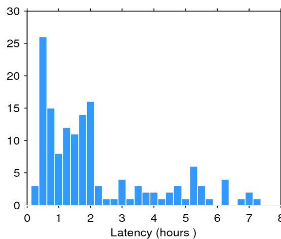
Figure 2. Histogram of the data latency for 13/12/2018. The y-axis denotes the number of files that are made available with a delay of x-hours with respect to the mean time of the records stored in the file.
