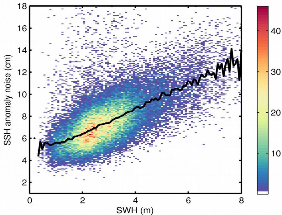
Figure 9. 2D histogram showing flag-valid SSH anomaly noise as a function of SWH for 13/12/2018. The black line denotes the median SSH anomaly noise as a function of SWH.
