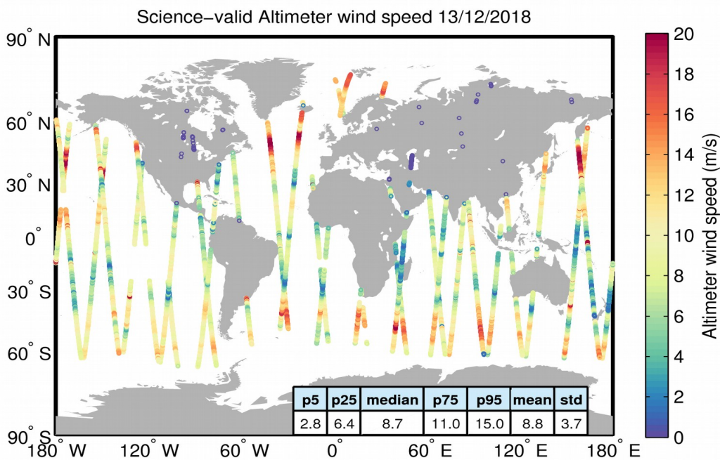
Figure 34. Geographical distribution of science-valid wind data over oceans and lakes for 13/12/2018. The statistical values shown in the table refer to the wind in m/s and are calculated over all measurements shown in the figure. Gray circles denote records that have been rejected based on the editing criteria described in Table 5.
