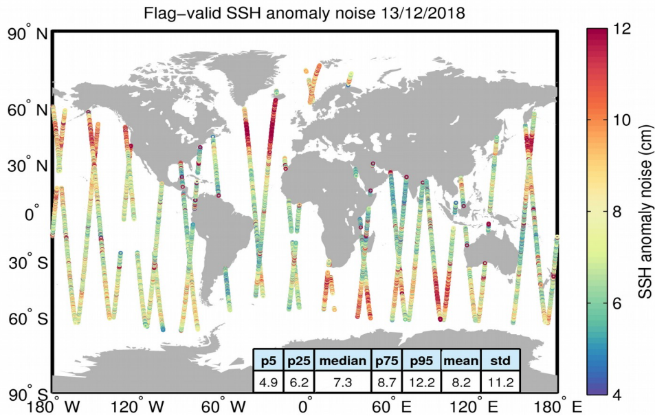
Figure 8. Geographical distribution of flag-valid 20-Hz SSH anomaly measurement noise over oceans and lakes for 13/12/2018. The statistical values shown in the table refer to the SSH anomaly noise and are calculated over all measurements shown in the figure.
