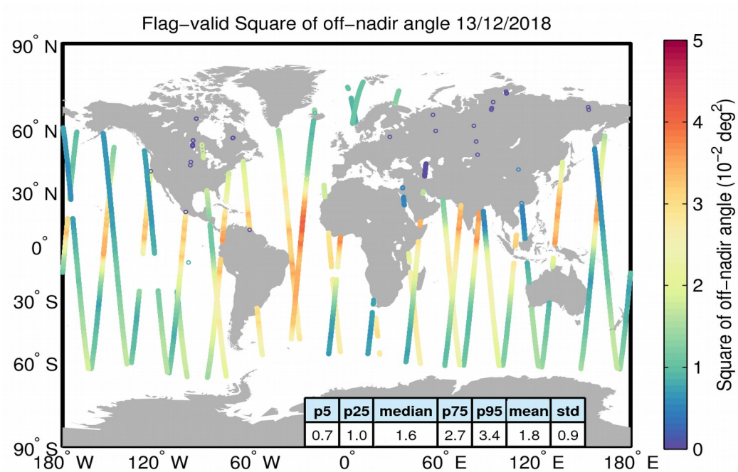
Figure 37. Geographical distribution of flag-valid mispointing data over oceans and lakes for 13/12/2018. The statistical values shown in the table refer to the mispointing in 10^{-2} deg 2 and are calculated over all measurements shown in the figure.
