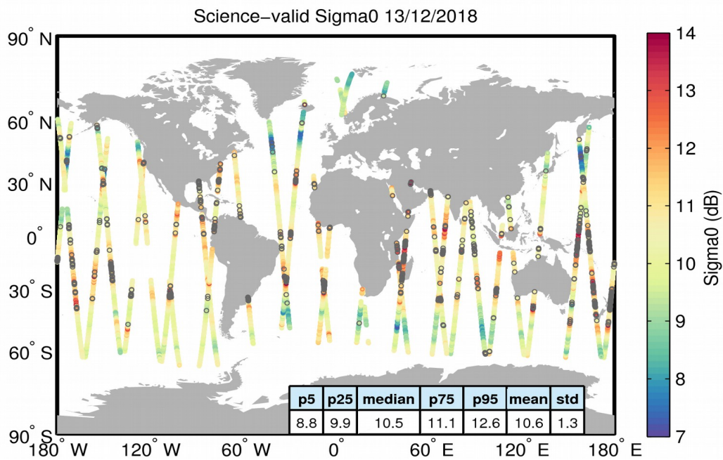
Figure 27. Geographical distribution of science-valid sigma0 data over oceans and lakes for 13/12/2018. The statistical values shown in the table refer to the sigma0 in dB and are calculated over all measurements shown in the figure. Gray circles denote records that have been rejected based on the editing criteria described in Table 4.
