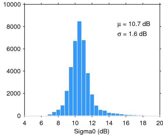
Figure 25. Histogram of flag-valid sigma0 over oceans and lakes for 13/12/2018. The mean ( \mu ) and standard deviation ( \sigma ) are also shown. Note that values outside [4 20] dB are excluded from the histogram for the sake of readability but not from the computation of \mu and \sigma .
