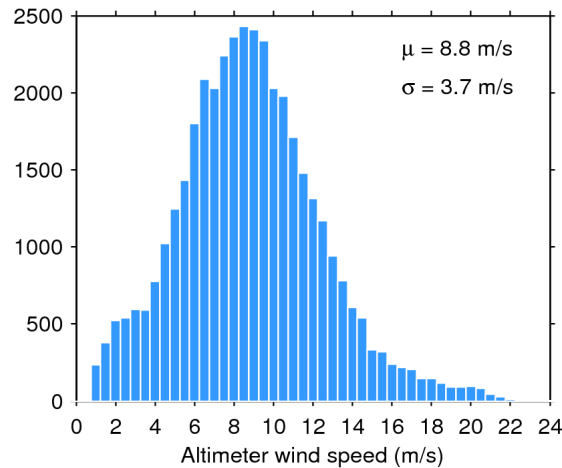
Figure 33. Histogram of flag-valid wind over oceans and lakes for 13/12/2018. The mean ( \mu ) and standard deviation ( \sigma ) are also shown. Note that values larger than 24 m/s are excluded from the histogram for the sake of readability but not from the computation of \mu and \sigma .
