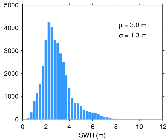
Figure 20. Histogram of science-valid SWH over oceans and lakes for 13/12/2018. The mean ( \mu ) and standard deviation ( \sigma ) are also shown. Note that values larger than 12 m are excluded from the histogram for the sake of readability but not from the computation of \mu and \sigma .
