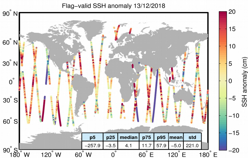
Figure 5. Geographical distribution of flag-valid 1-Hz SSH anomaly data over oceans and lakes for 13/12/2018. The statistical values shown in the table refer to the SSH anomaly in cm and are calculated over all measurements shown in the figure.
