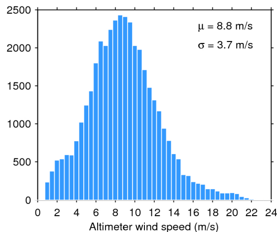
Figure 35. Histogram of science-valid wind over oceans and lakes for 13/12/2018. The mean ( \mu ) and standard deviation ( \sigma ) are also shown. Note that values larger than 24 m/s are excluded from the histogram for the sake of readability but not from the computation of \mu and \sigma .
