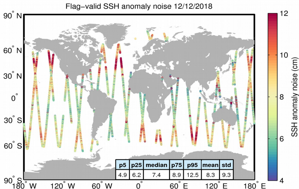
Figure 8. Geographical distribution of flag-valid 20-Hz SSH anomaly measurement noise over oceans and lakes for 12/12/2018. The statistical values shown in the table refer to the SSH anomaly noise and are calculated over all measurements shown in the figure.
