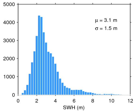
Figure 17. Histogram of flag-valid SWH over oceans and lakes for 12/12/2018. The mean ( \mu ) and standard deviation ( \sigma ) are also shown. Note that values larger than 12 m are excluded from the histogram for the sake of readability but not from the computation of \mu and \sigma .
