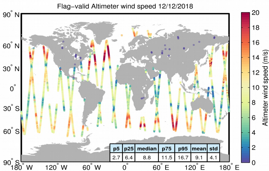
Figure 31. Geographical distribution of flag-valid wind data over oceans and lakes for 12/12/2018. The statistical values shown in the table refer to the wind in m/s and are calculated over all measurements shown in the figure.
