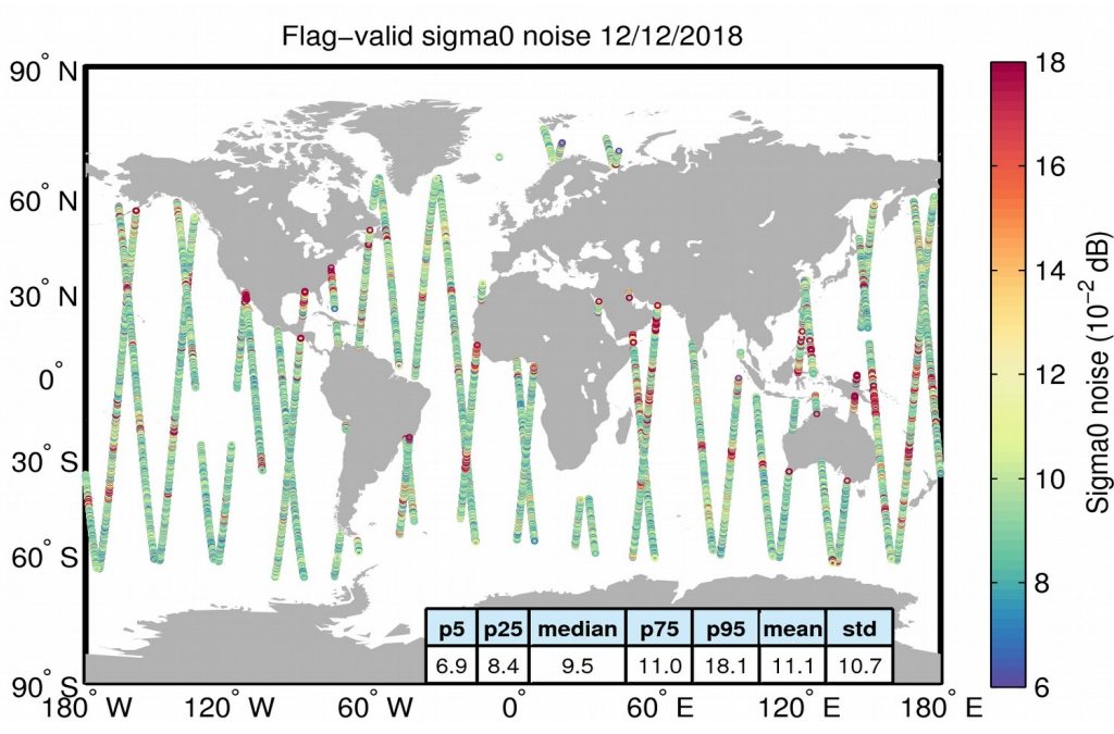
Figure 26. Geographical distribution of flag-valid 20-Hz sigma0 measurement noise over oceans and lakes for 12/12/2018. The statistical values shown in the table refer to the sigma0 noise and are calculated over all measurements shown in the figure.
