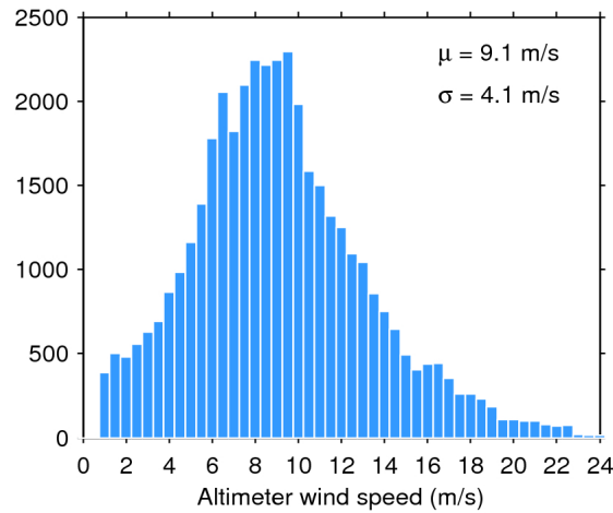
Figure 33. Histogram of flag-valid wind over oceans and lakes for 12/12/2018. The mean ( \mu ) and standard deviation ( \sigma ) are also shown. Note that values larger than 24 m/s are excluded from the histogram for the sake of readability but not from the computation of \mu and \sigma .
