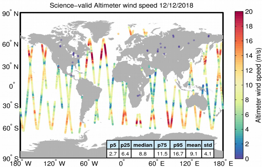
Figure 34. Geographical distribution of science-valid wind data over oceans and lakes for 12/12/2018. The statistical values shown in the table refer to the wind in m/s and are calculated over all measurements shown in the figure. Gray circles denote records that have been rejected based on the editing criteria described in Table 5.
