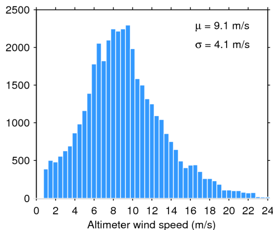
Figure 35. Histogram of science-valid wind over oceans and lakes for 12/12/2018. The mean ( \mu ) and standard deviation ( \sigma ) are also shown. Note that values larger than 24 m/s are excluded from the histogram for the sake of readability but not from the computation of \mu and \sigma .
