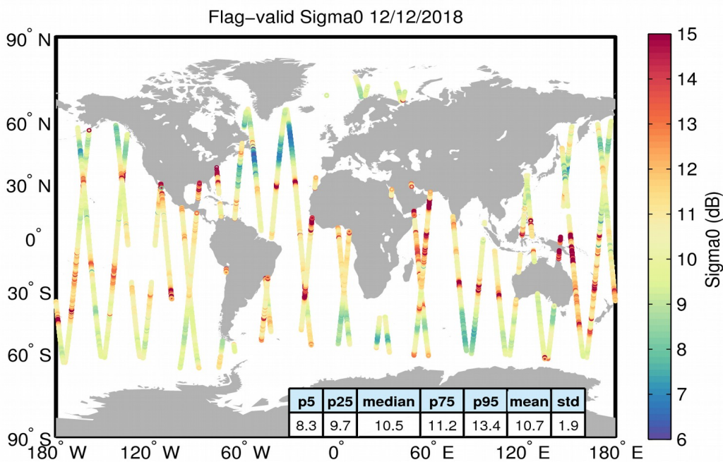
Figure 23. Geographical distribution of flag-valid sigma0 data over oceans and lakes for 12/12/2018. The statistical values shown in the table refer to the sigma0 in dB and are calculated over all measurements shown in the figure.
