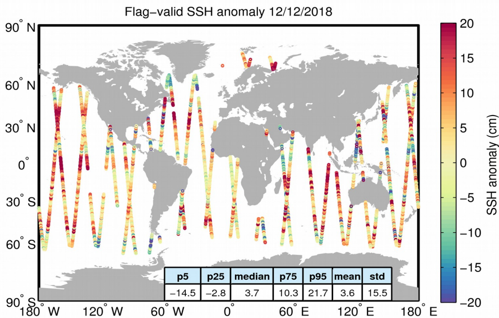
Figure 5. Geographical distribution of flag-valid 1-Hz SSH anomaly data over oceans and lakes for 12/12/2018. The statistical values shown in the table refer to the SSH anomaly in cm and are calculated over all measurements shown in the figure.
