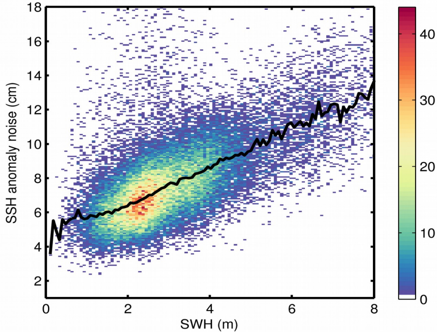
Figure 9. 2D histogram showing flag-valid SSH anomaly noise as a function of SWH for 12/12/2018. The black line denotes the median SSH anomaly noise as a function of SWH.
