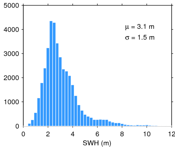
Figure 20. Histogram of science-valid SWH over oceans and lakes for 12/12/2018. The mean ( \mu ) and standard deviation ( \sigma ) are also shown. Note that values larger than 12 m are excluded from the histogram for the sake of readability but not from the computation of \mu and \sigma .
