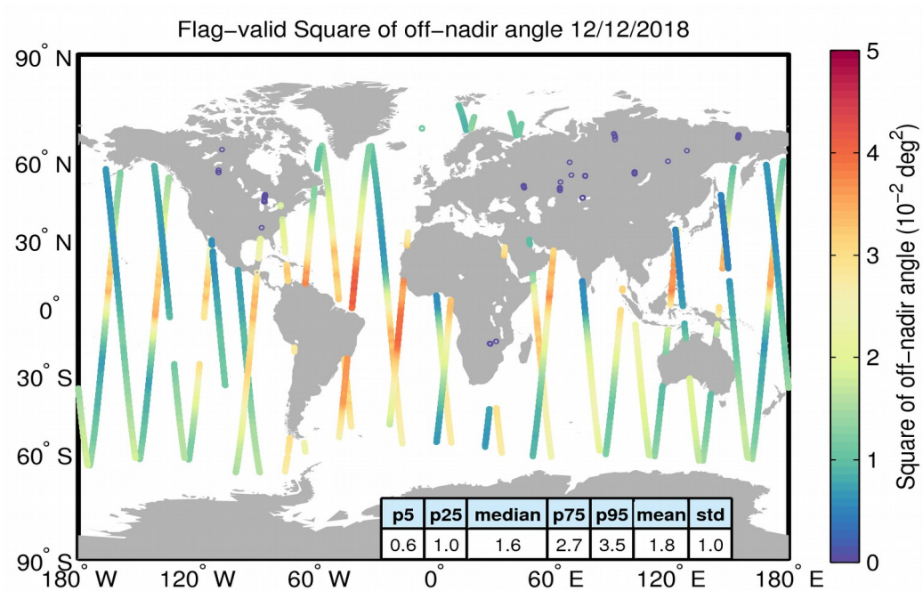
Figure 37. Geographical distribution of flag-valid mispointing data over oceans and lakes for 12/12/2018. The statistical values shown in the table refer to the mispointing in 10^{-2} \text{deg}^2 and are calculated over all measurements shown in the figure.
