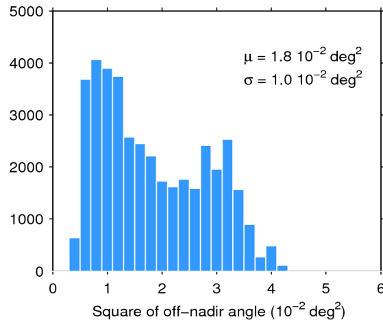
Figure 39. Histogram of flag-valid mispointing over oceans and lakes for 12/12/2018. The mean ( \mu ) and standard deviation ( \sigma ) are also shown. Note that values larger than 6 \cdot 10^{-2} \text{ deg}^2 are excluded from the histogram for the sake of readability but not from the computation of \mu and \sigma .
