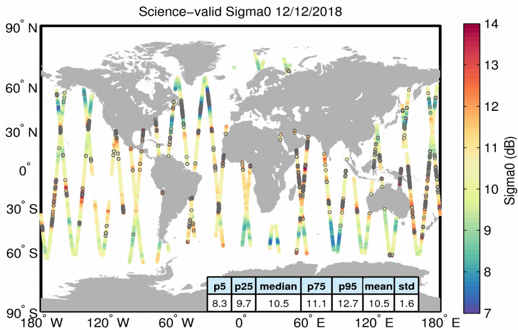
Figure 27. Geographical distribution of science-valid sigma0 data over oceans and lakes for 12/12/2018. The statistical values shown in the table refer to the sigma0 in dB and are calculated over all measurements shown in the figure. Gray circles denote records that have been rejected based on the editing criteria described in Table 4.
