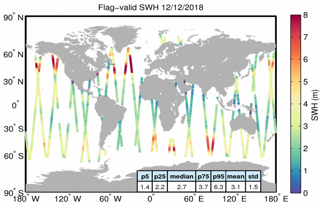
Figure 15. Geographical distribution of flag-valid SWH data over oceans and lakes for 12/12/2018. The statistical values shown in the table refer to the SWH in m and are calculated over all measurements shown in the figure.
