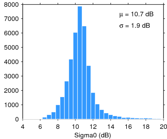
Figure 25. Histogram of flag-valid sigma0 over oceans and lakes for 12/12/2018. The mean ( \mu ) and standard deviation ( \sigma ) are also shown. Note that values outside [4 20] dB are excluded from the histogram for the sake of readability but not from the computation of \mu and \sigma .
