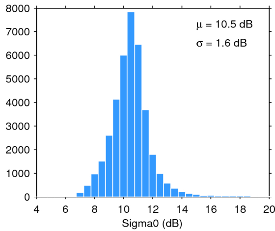
Figure 28. Histogram of science-valid sigma0 over oceans and lakes for 12/12/2018. The mean ( \mu ) and standard deviation ( \sigma ) are also shown. Note that values outside [4 20] dB are excluded from the histogram for the sake of readability but not from the computation of \mu and \sigma .
