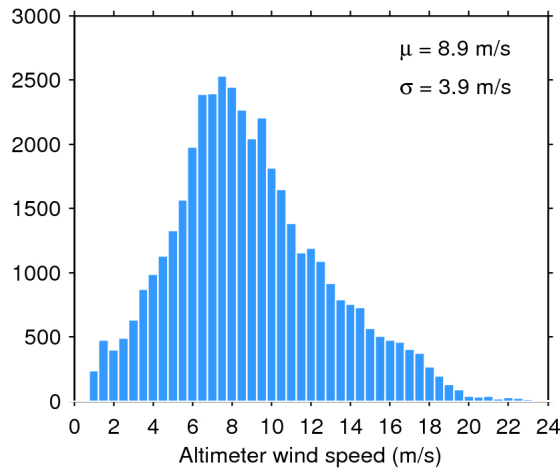
Figure 33. Histogram of flag-valid wind over oceans and lakes for 11/12/2018. The mean ( \mu ) and standard deviation ( \sigma ) are also shown. Note that values larger than 24 m/s are excluded from the histogram for the sake of readability but not from the computation of \mu and \sigma .
