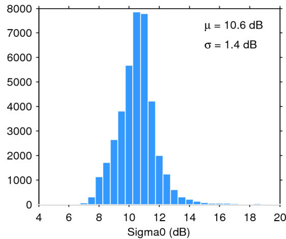
Figure 28. Histogram of science-valid sigma0 over oceans and lakes for 11/12/2018. The mean ( \mu ) and standard deviation ( \sigma ) are also shown. Note that values outside [4 20] dB are excluded from the histogram for the sake of readability but not from the computation of \mu and \sigma .
