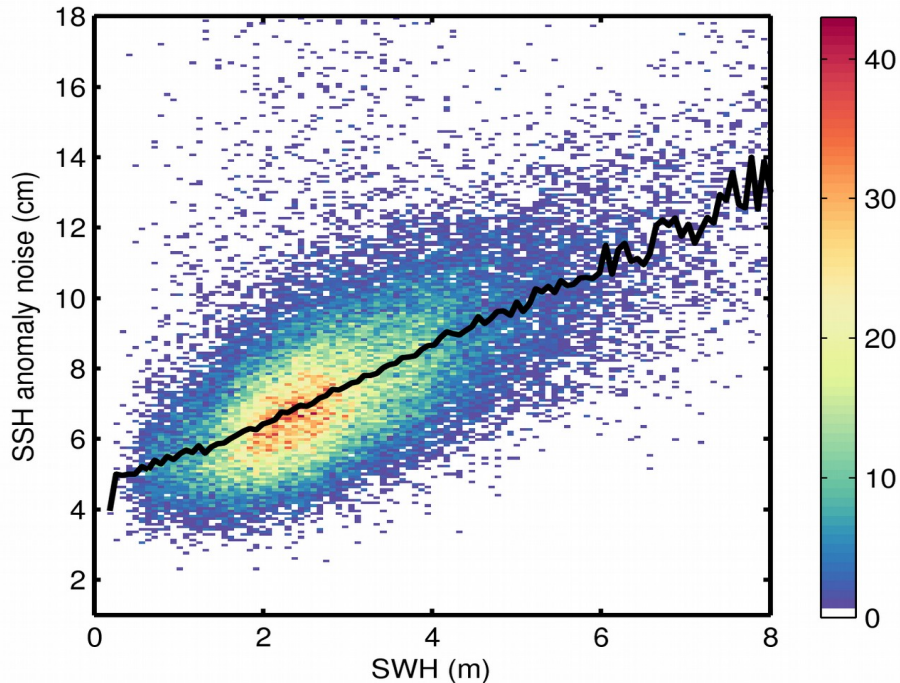
Figure 9. 2D histogram showing flag-valid SSH anomaly noise as a function of SWH for 11/12/2018. The black line denotes the median SSH anomaly noise as a function of SWH.
