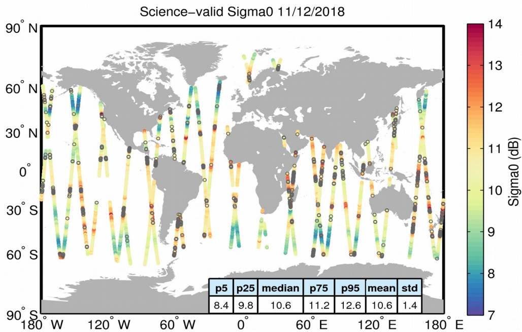
Figure 27. Geographical distribution of science-valid sigma0 data over oceans and lakes for 11/12/2018. The statistical values shown in the table refer to the sigma0 in dB and are calculated over all measurements shown in the figure. Gray circles denote records that have been rejected based on the editing criteria described in Table 4.
