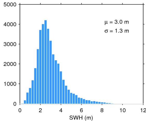
Figure 20. Histogram of science-valid SWH over oceans and lakes for 11/12/2018. The mean ( \mu ) and standard deviation ( \sigma ) are also shown. Note that values larger than 12 m are excluded from the histogram for the sake of readability but not from the computation of \mu and \sigma .
