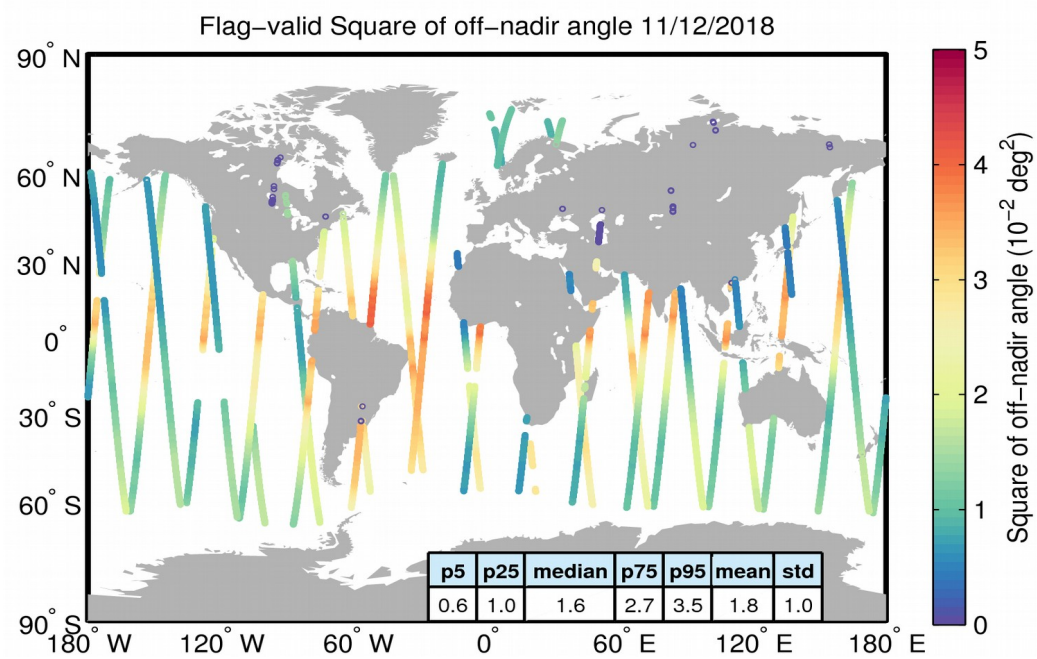
Figure 37. Geographical distribution of flag-valid mispointing data over oceans and lakes for 11/12/2018. The statistical values shown in the table refer to the mispointing in 10^{-2} \text{deg}^2 and are calculated over all measurements shown in the figure.
