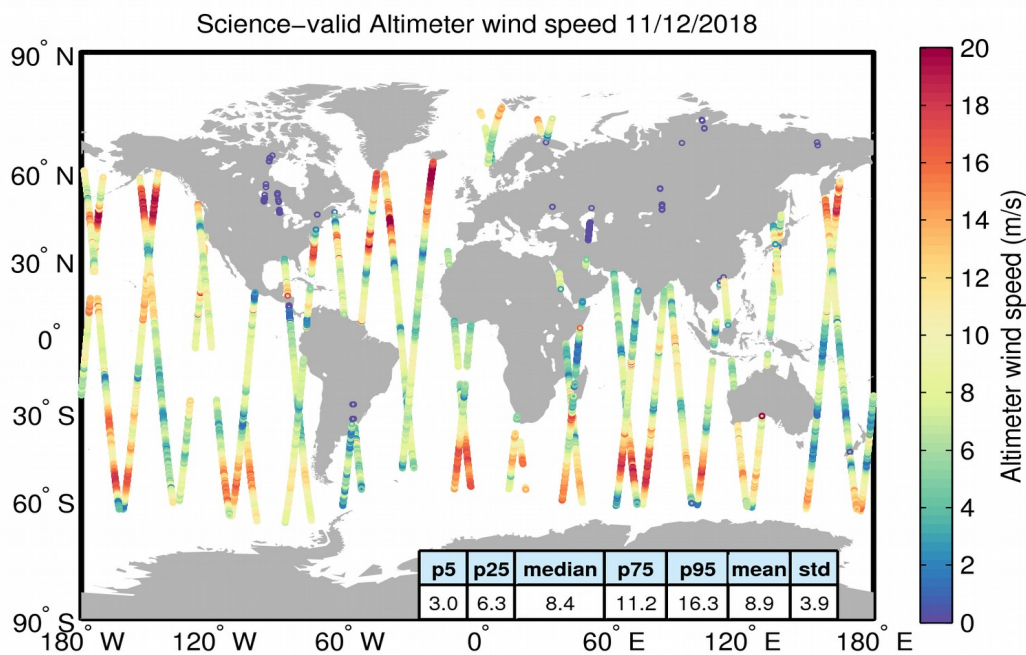
Figure 34. Geographical distribution of science-valid wind data over oceans and lakes for 11/12/2018. The statistical values shown in the table refer to the wind in m/s and are calculated over all measurements shown in the figure. Gray circles denote records that have been rejected based on the editing criteria described in Table 5.
