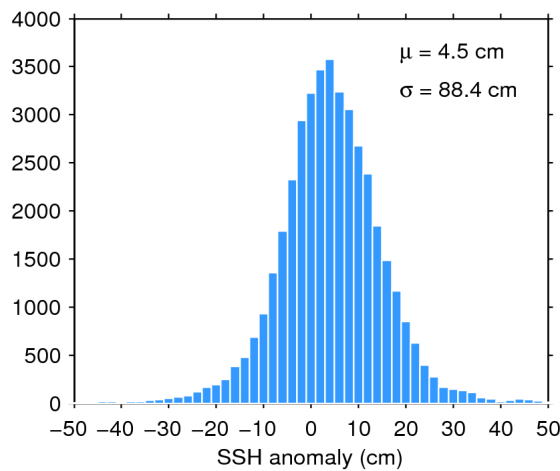
Figure 7. Histogram of flag-valid SSH anomaly over oceans and lakes for 11/12/2018. The mean ( \mu ) and standard deviation ( \sigma ) are also shown. Note that values outside [-50 50] cm are excluded from the histogram for the sake of readability but not from the computation of \mu and \sigma .
