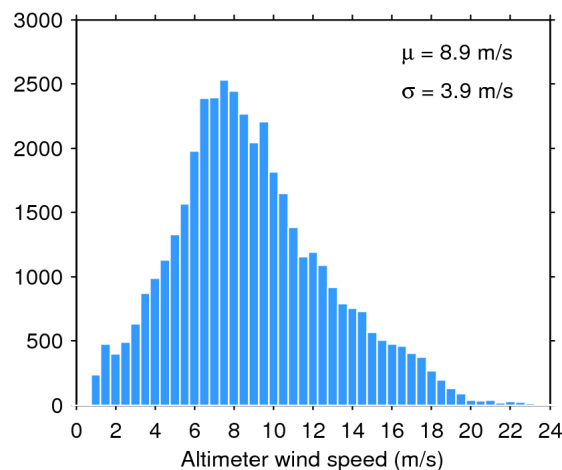
Figure 35. Histogram of science-valid wind over oceans and lakes for 11/12/2018. The mean ( \mu ) and standard deviation ( \sigma ) are also shown. Note that values larger than 24 m/s are excluded from the histogram for the sake of readability but not from the computation of \mu and \sigma .
