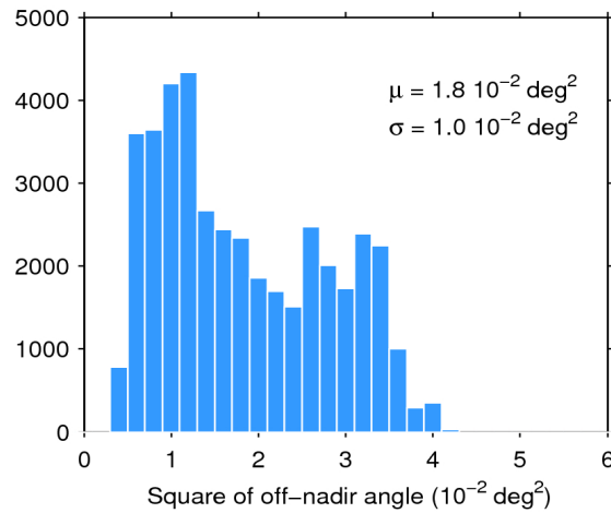
Figure 39. Histogram of flag-valid mispointing over oceans and lakes for 11/12/2018. The mean ( \mu ) and standard deviation ( \sigma ) are also shown. Note that values larger than 6 \cdot 10^{-2} \text{ deg}^2 are excluded from the histogram for the sake of readability but not from the computation of \mu and \sigma .
