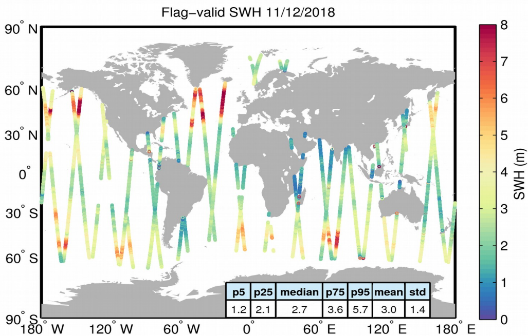
Figure 15. Geographical distribution of flag-valid SWH data over oceans and lakes for 11/12/2018. The statistical values shown in the table refer to the SWH in m and are calculated over all measurements shown in the figure.
