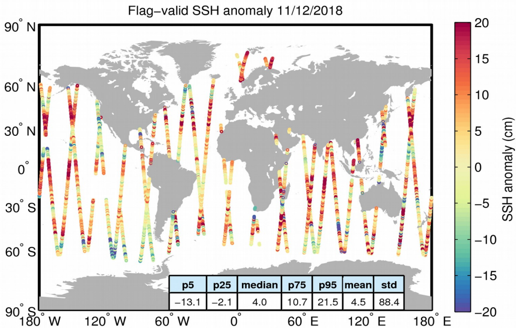
Figure 5. Geographical distribution of flag-valid 1-Hz SSH anomaly data over oceans and lakes for 11/12/2018. The statistical values shown in the table refer to the SSH anomaly in cm and are calculated over all measurements shown in the figure.
