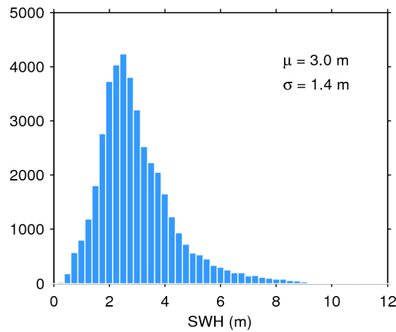
Figure 17. Histogram of flag-valid SWH over oceans and lakes for 11/12/2018. The mean ( \mu ) and standard deviation ( \sigma ) are also shown. Note that values larger than 12 m are excluded from the histogram for the sake of readability but not from the computation of \mu and \sigma .
