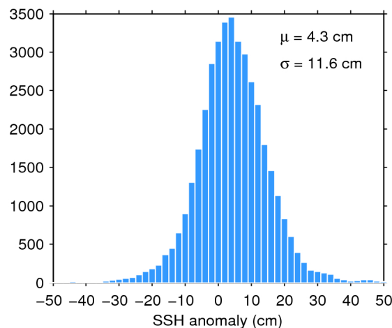
Figure 11. Histogram of science-valid SSH anomaly over oceans and lakes for 11/12/2018. The mean ( \mu ) and standard deviation ( \sigma ) are also shown. Note that values outside [-50 50] cm are excluded from the histogram for the sake of readability but not from the computation of \mu and \sigma .
