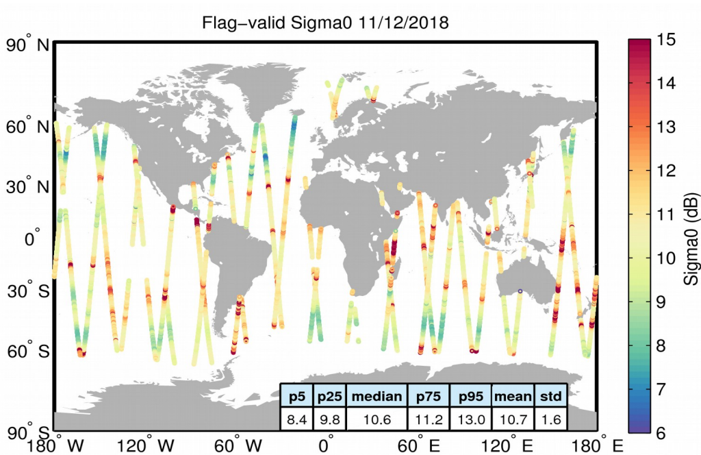
Figure 23. Geographical distribution of flag-valid sigma0 data over oceans and lakes for 11/12/2018. The statistical values shown in the table refer to the sigma0 in dB and are calculated over all measurements shown in the figure.
