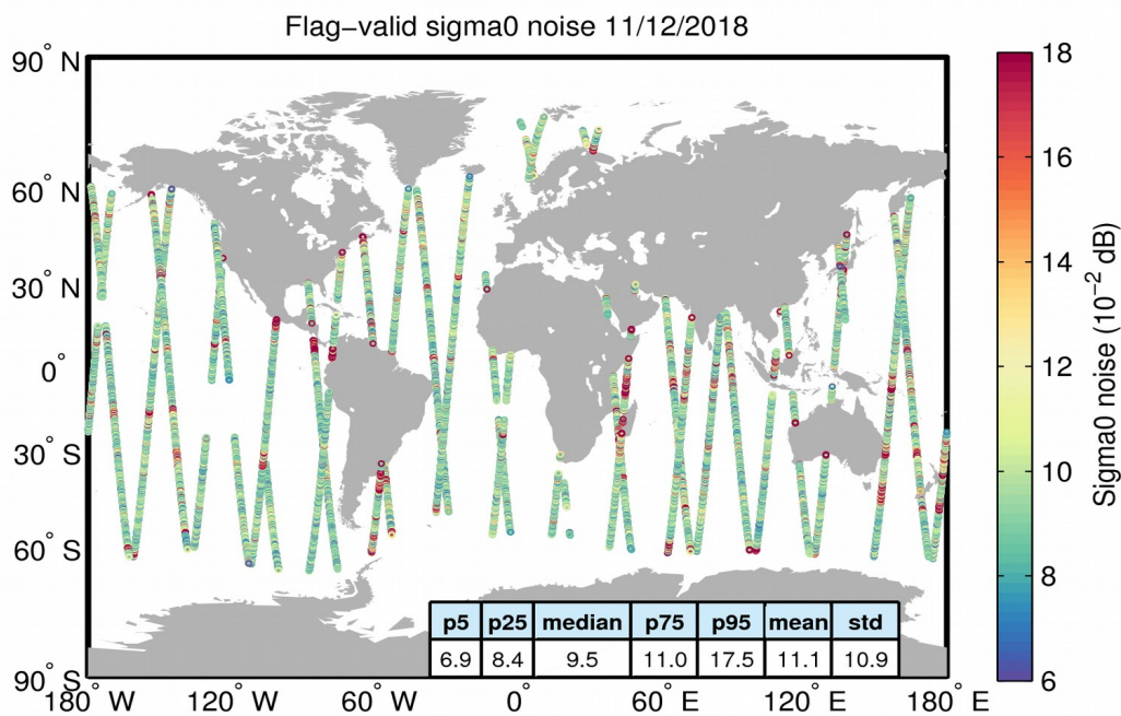
Figure 26. Geographical distribution of flag-valid 20-Hz sigma0 measurement noise over oceans and lakes for 11/12/2018. The statistical values shown in the table refer to the sigma0 noise and are calculated over all measurements shown in the figure.
