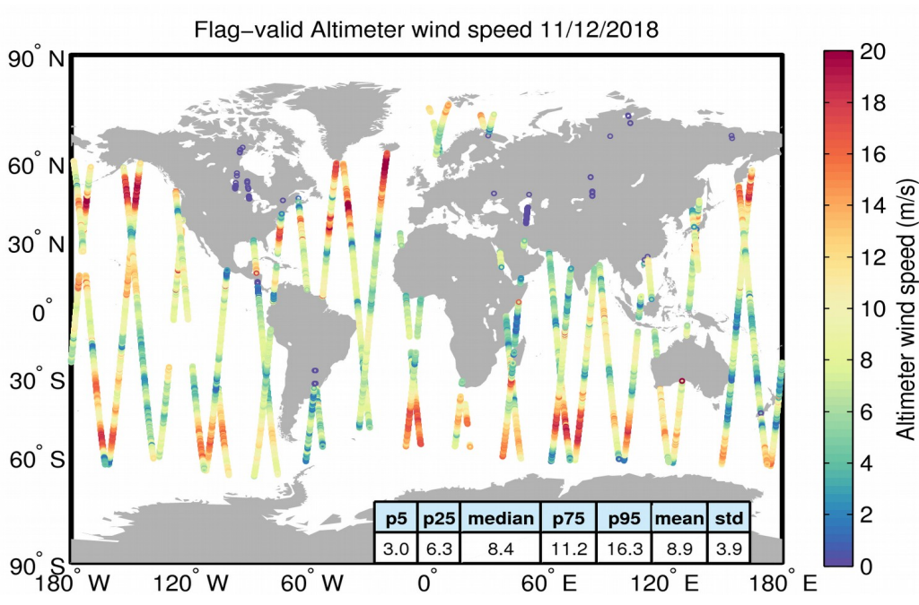
Figure 31. Geographical distribution of flag-valid wind data over oceans and lakes for 11/12/2018. The statistical values shown in the table refer to the wind in m/s and are calculated over all measurements shown in the figure.
