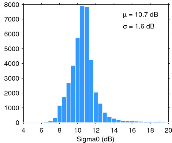
Figure 25. Histogram of flag-valid sigma0 over oceans and lakes for 11/12/2018. The mean ( \mu ) and standard deviation ( \sigma ) are also shown. Note that values outside [4 20] dB are excluded from the histogram for the sake of readability but not from the computation of \mu and \sigma .
