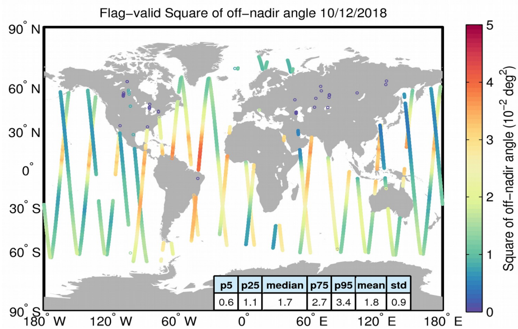
Figure 37. Geographical distribution of flag-valid mispointing data over oceans and lakes for 10/12/2018. The statistical values shown in the table refer to the mispointing in 10^{-2} deg 2 and are calculated over all measurements shown in the figure.
