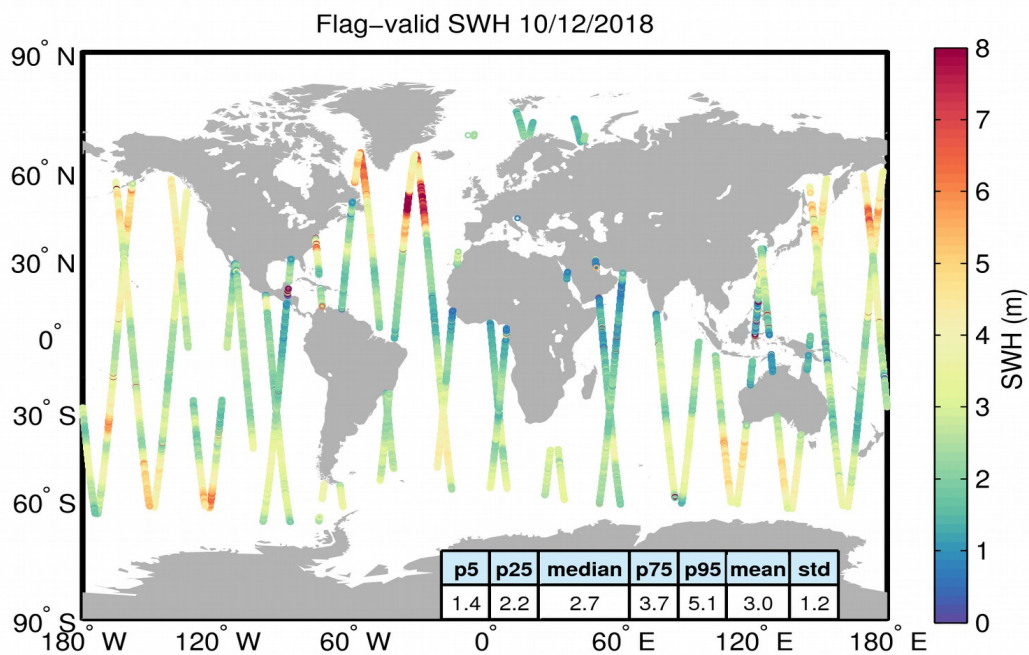
Figure 15. Geographical distribution of flag-valid SWH data over oceans and lakes for 10/12/2018. The statistical values shown in the table refer to the SWH in m and are calculated over all measurements shown in the figure.
