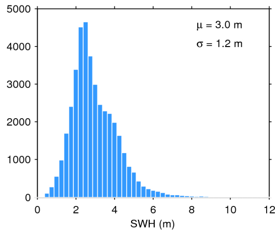
Figure 17. Histogram of flag-valid SWH over oceans and lakes for 10/12/2018. The mean ( \mu ) and standard deviation ( \sigma ) are also shown. Note that values larger than 12 m are excluded from the histogram for the sake of readability but not from the computation of \mu and \sigma .
