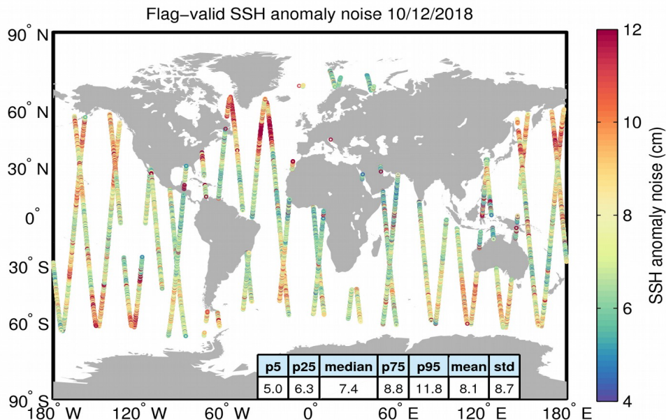
Figure 8. Geographical distribution of flag-valid 20-Hz SSH anomaly measurement noise over oceans and lakes for 10/12/2018. The statistical values shown in the table refer to the SSH anomaly noise and are calculated over all measurements shown in the figure.
