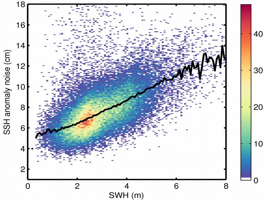
Figure 9. 2D histogram showing flag-valid SSH anomaly noise as a function of SWH for 10/12/2018. The black line denotes the median SSH anomaly noise as a function of SWH.
