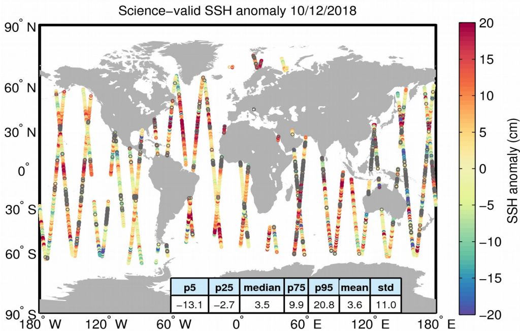
Figure 10. Geographical distribution of science-valid SSH anomaly data over oceans and lakes for 10/12/2018. The statistical values shown in the table refer to the SSH anomaly in cm and are calculated over all measurements shown in the figure. Gray circles denote records that have been rejected based on the editing criteria described in Table 2.
