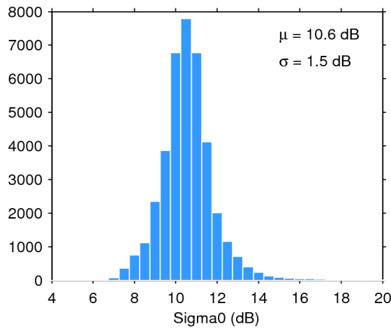
Figure 28. Histogram of science-valid sigma0 over oceans and lakes for 10/12/2018. The mean ( \mu ) and standard deviation ( \sigma ) are also shown. Note that values outside [4 20] dB are excluded from the histogram for the sake of readability but not from the computation of \mu and \sigma .
