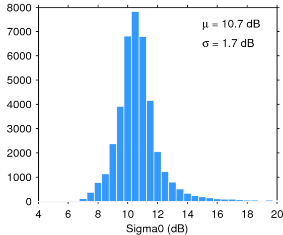
Figure 25. Histogram of flag-valid sigma0 over oceans and lakes for 10/12/2018. The mean ( \mu ) and standard deviation ( \sigma ) are also shown. Note that values outside [4 20] dB are excluded from the histogram for the sake of readability but not from the computation of \mu and \sigma .
