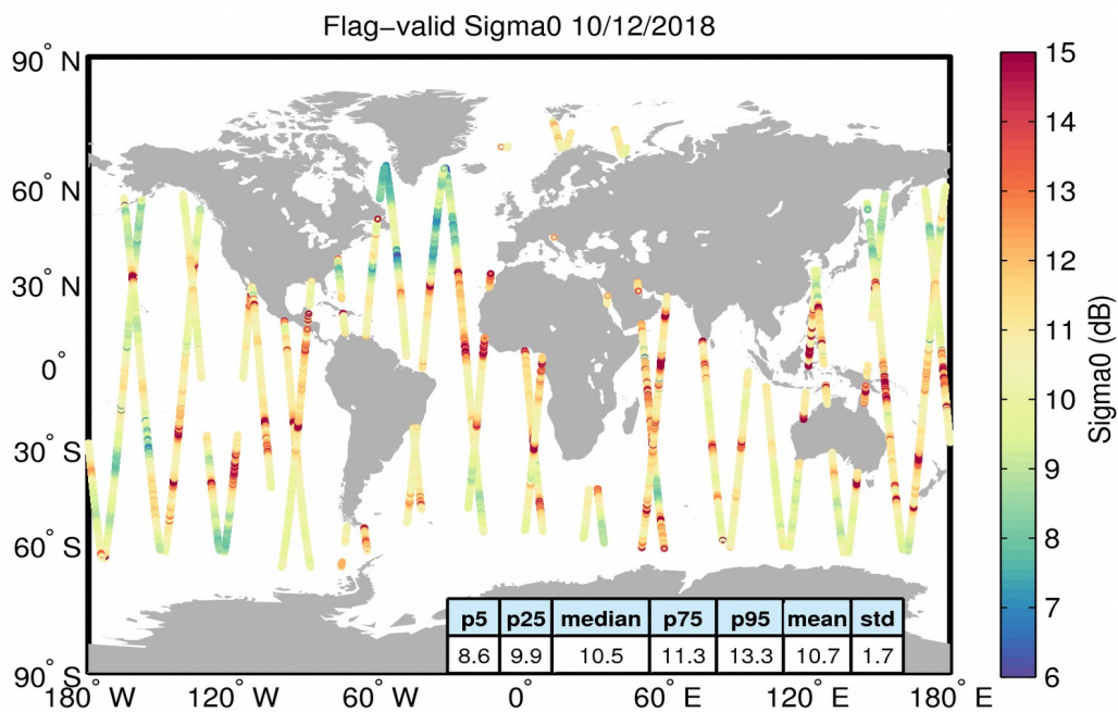
Figure 23. Geographical distribution of flag-valid sigma0 data over oceans and lakes for 10/12/2018. The statistical values shown in the table refer to the sigma0 in dB and are calculated over all measurements shown in the figure.
