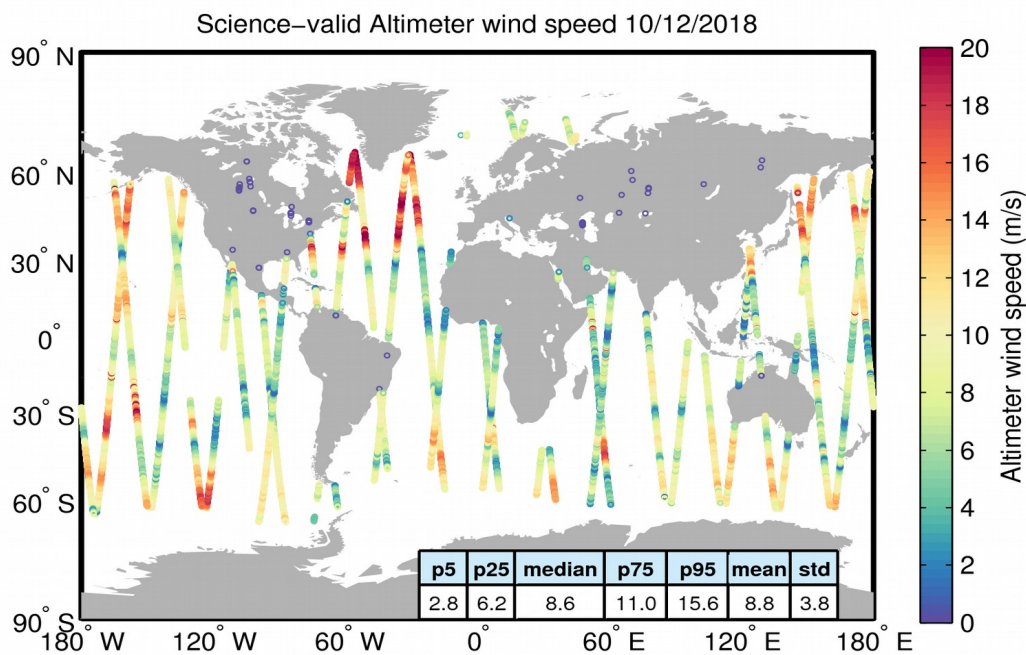
Figure 34. Geographical distribution of science-valid wind data over oceans and lakes for 10/12/2018. The statistical values shown in the table refer to the wind in m/s and are calculated over all measurements shown in the figure. Gray circles denote records that have been rejected based on the editing criteria described in Table 5.
