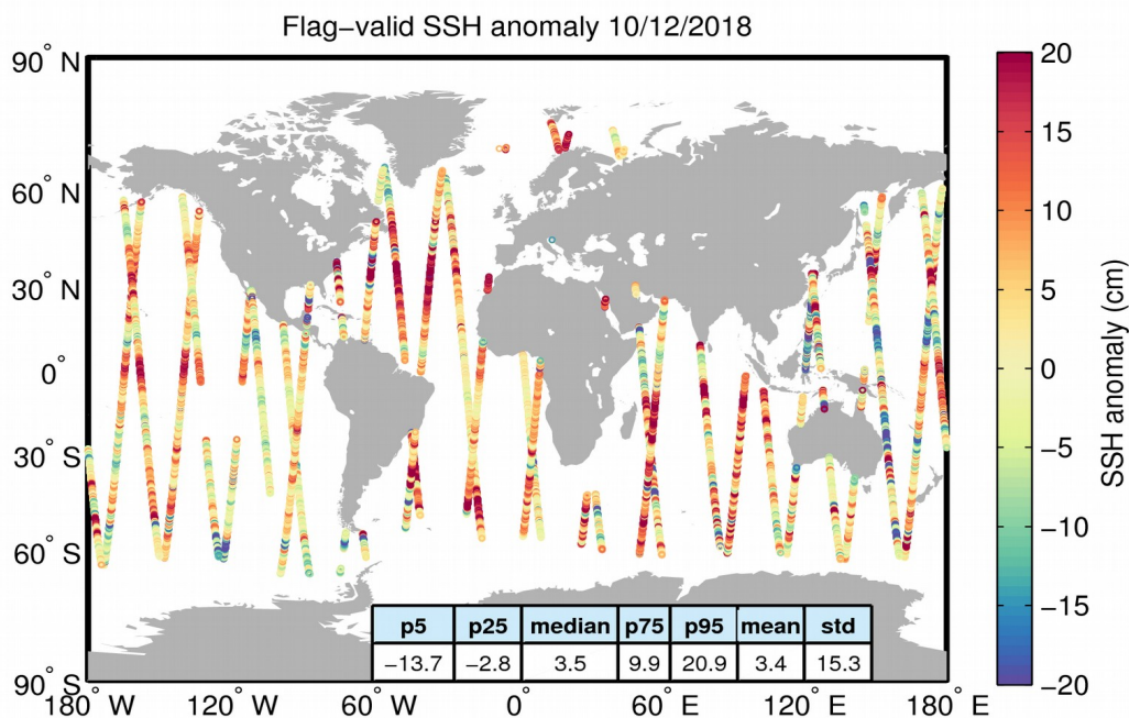
Figure 5. Geographical distribution of flag-valid 1-Hz SSH anomaly data over oceans and lakes for 10/12/2018. The statistical values shown in the table refer to the SSH anomaly in cm and are calculated over all measurements shown in the figure.
