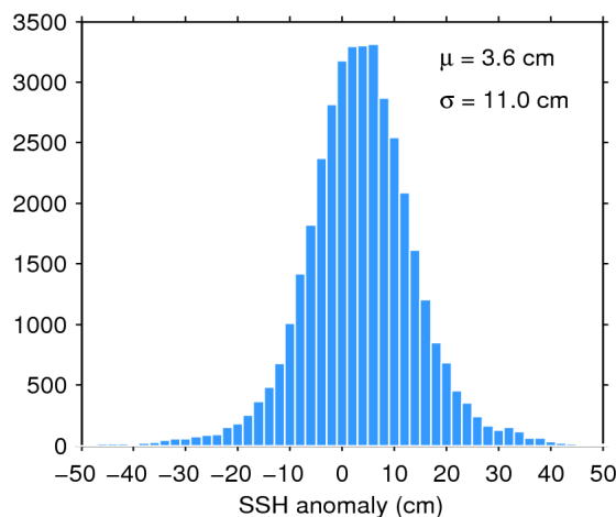
Figure 11. Histogram of science-valid SSH anomaly over oceans and lakes for 10/12/2018. The mean ( \mu ) and standard deviation ( \sigma ) are also shown. Note that values outside [-50 50] cm are excluded from the histogram for the sake of readability but not from the computation of \mu and \sigma .
