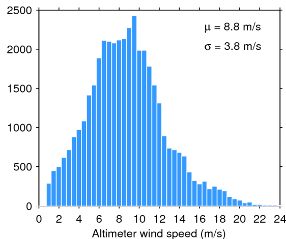
Figure 35. Histogram of science-valid wind over oceans and lakes for 10/12/2018. The mean ( \mu ) and standard deviation ( \sigma ) are also shown. Note that values larger than 24 m/s are excluded from the histogram for the sake of readability but not from the computation of \mu and \sigma .
