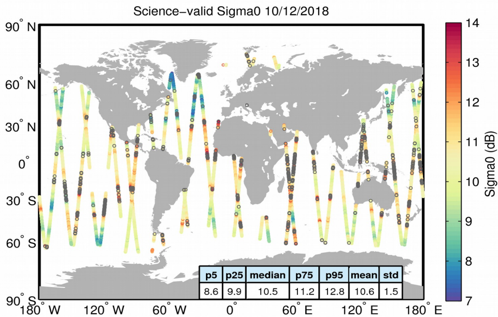
Figure 27. Geographical distribution of science-valid sigma0 data over oceans and lakes for 10/12/2018. The statistical values shown in the table refer to the sigma0 in dB and are calculated over all measurements shown in the figure. Gray circles denote records that have been rejected based on the editing criteria described in Table 4.
