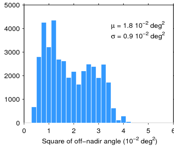
Figure 39. Histogram of flag-valid mispointing over oceans and lakes for 10/12/2018. The mean ( \mu ) and standard deviation ( \sigma ) are also shown. Note that values larger than 6 \cdot 10^{-2} \text{ deg}^2 are excluded from the histogram for the sake of readability but not from the computation of \mu and \sigma .
