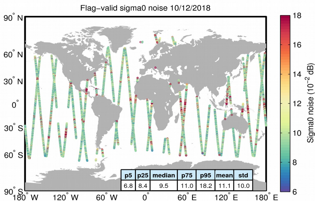
Figure 26. Geographical distribution of flag-valid 20-Hz sigma0 measurement noise over oceans and lakes for 10/12/2018. The statistical values shown in the table refer to the sigma0 noise and are calculated over all measurements shown in the figure.
