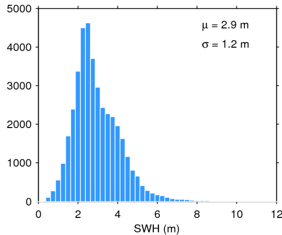
Figure 20. Histogram of science-valid SWH over oceans and lakes for 10/12/2018. The mean ( \mu ) and standard deviation ( \sigma ) are also shown. Note that values larger than 12 m are excluded from the histogram for the sake of readability but not from the computation of \mu and \sigma .
