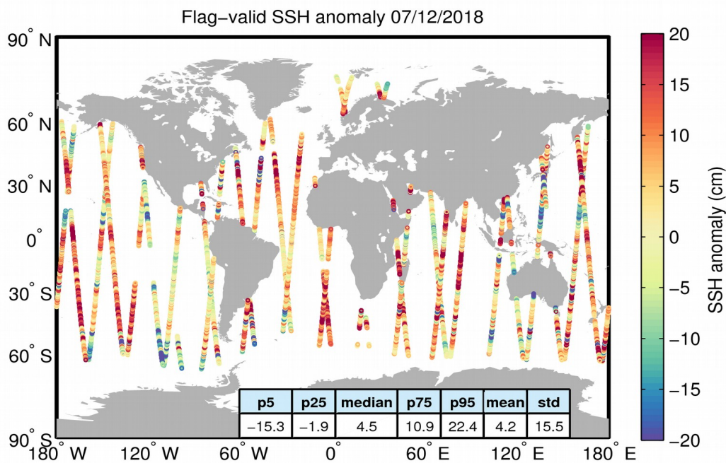
Figure 5. Geographical distribution of flag-valid 1-Hz SSH anomaly data over oceans and lakes for 07/12/2018. The statistical values shown in the table refer to the SSH anomaly in cm and are calculated over all measurements shown in the figure.
