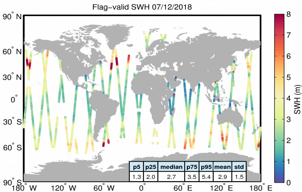
Figure 15. Geographical distribution of flag-valid SWH data over oceans and lakes for 07/12/2018. The statistical values shown in the table refer to the SWH in m and are calculated over all measurements shown in the figure.
