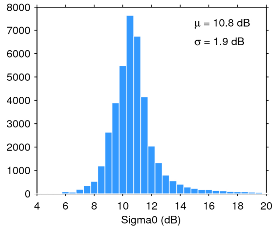
Figure 25. Histogram of flag-valid sigma0 over oceans and lakes for 07/12/2018. The mean ( \mu ) and standard deviation ( \sigma ) are also shown. Note that values outside [4 20] dB are excluded from the histogram for the sake of readability but not from the computation of \mu and \sigma .
