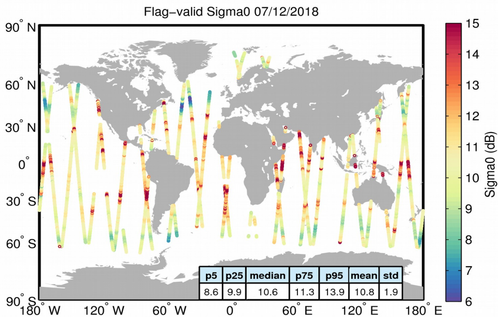
Figure 23. Geographical distribution of flag-valid sigma0 data over oceans and lakes for 07/12/2018. The statistical values shown in the table refer to the sigma0 in dB and are calculated over all measurements shown in the figure.
