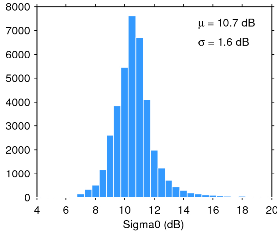
Figure 28. Histogram of science-valid sigma0 over oceans and lakes for 07/12/2018. The mean ( \mu ) and standard deviation ( \sigma ) are also shown. Note that values outside [4 20] dB are excluded from the histogram for the sake of readability but not from the computation of \mu and \sigma .
