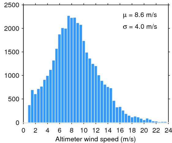
Figure 33. Histogram of flag-valid wind over oceans and lakes for 07/12/2018. The mean ( \mu ) and standard deviation ( \sigma ) are also shown. Note that values larger than 24 m/s are excluded from the histogram for the sake of readability but not from the computation of \mu and \sigma .
