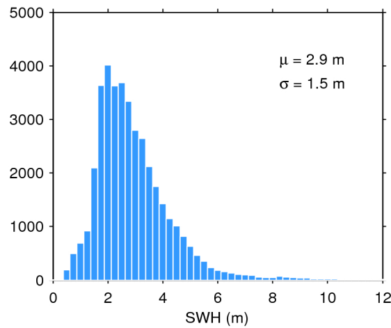
Figure 17. Histogram of flag-valid SWH over oceans and lakes for 07/12/2018. The mean ( \mu ) and standard deviation ( \sigma ) are also shown. Note that values larger than 12 m are excluded from the histogram for the sake of readability but not from the computation of \mu and \sigma .
