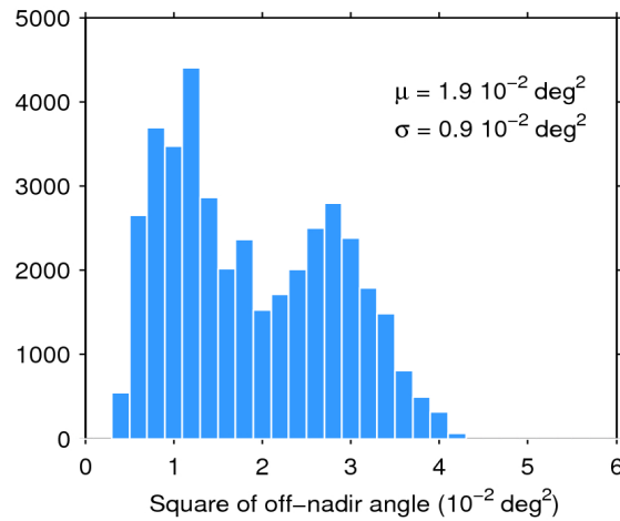
Figure 39. Histogram of flag-valid mispointing over oceans and lakes for 07/12/2018. The mean ( \mu ) and standard deviation ( \sigma ) are also shown. Note that values larger than 6 \cdot 10^{-2} \text{ deg}^2 are excluded from the histogram for the sake of readability but not from the computation of \mu and \sigma .
