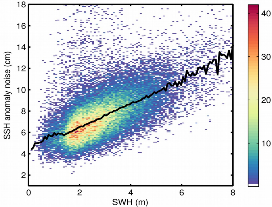
Figure 9. 2D histogram showing flag-valid SSH anomaly noise as a function of SWH for 07/12/2018. The black line denotes the median SSH anomaly noise as a function of SWH.
