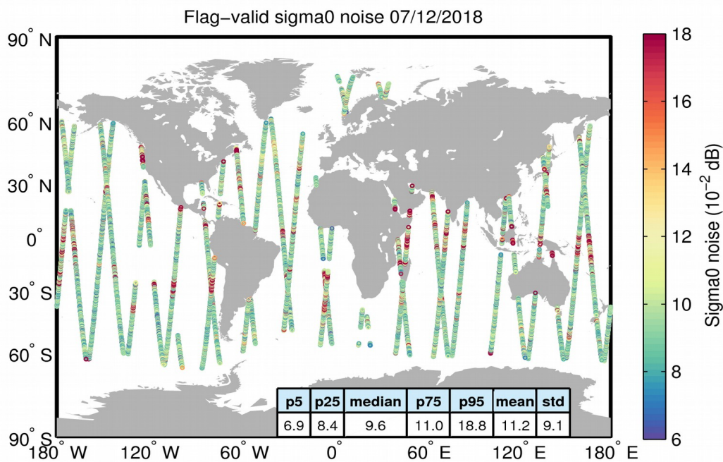
Figure 26. Geographical distribution of flag-valid 20-Hz sigma0 measurement noise over oceans and lakes for 07/12/2018. The statistical values shown in the table refer to the sigma0 noise and are calculated over all measurements shown in the figure.
