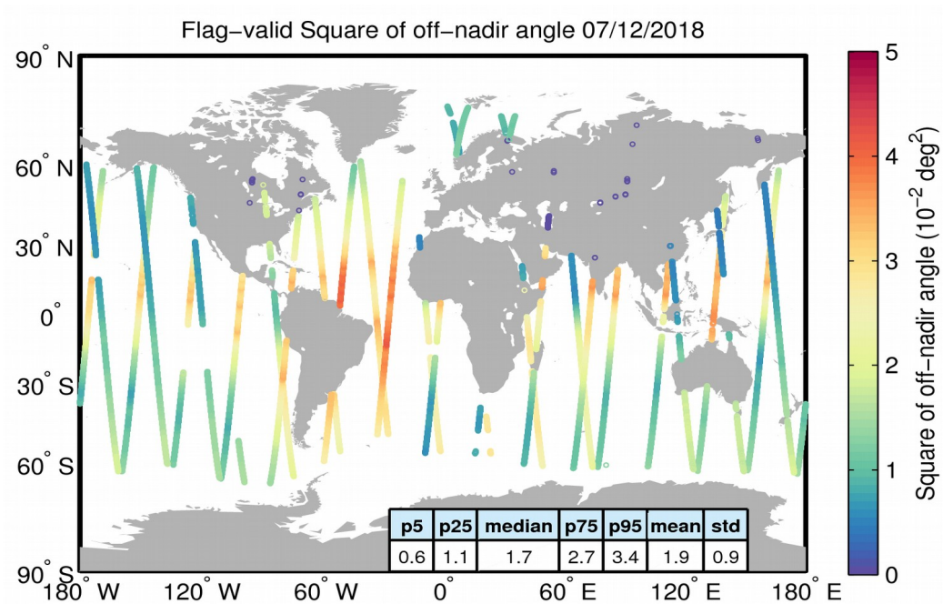
Figure 37. Geographical distribution of flag-valid mispointing data over oceans and lakes for 07/12/2018. The statistical values shown in the table refer to the mispointing in 10^{-2} \text{deg}^2 and are calculated over all measurements shown in the figure.
