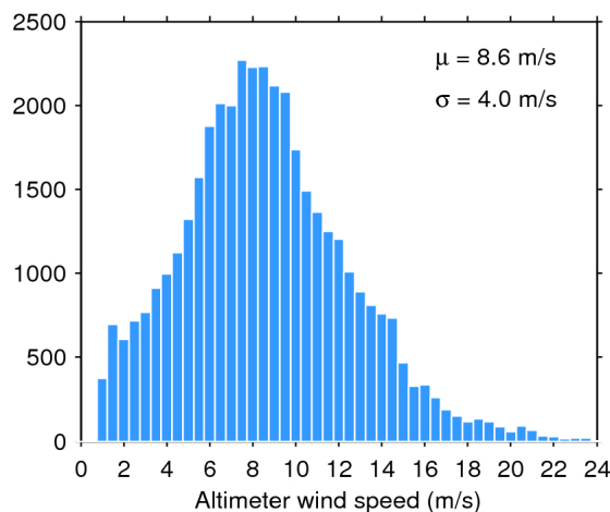
Figure 35. Histogram of science-valid wind over oceans and lakes for 07/12/2018. The mean ( \mu ) and standard deviation ( \sigma ) are also shown. Note that values larger than 24 m/s are excluded from the histogram for the sake of readability but not from the computation of \mu and \sigma .
