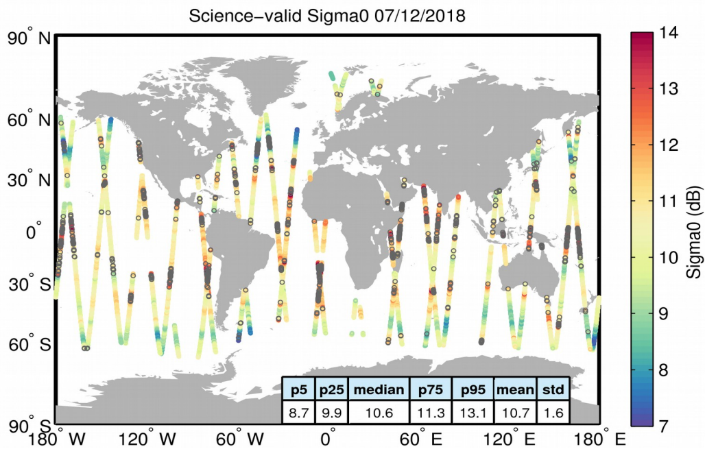
Figure 27. Geographical distribution of science-valid sigma0 data over oceans and lakes for 07/12/2018. The statistical values shown in the table refer to the sigma0 in dB and are calculated over all measurements shown in the figure. Gray circles denote records that have been rejected based on the editing criteria described in Table 4.
