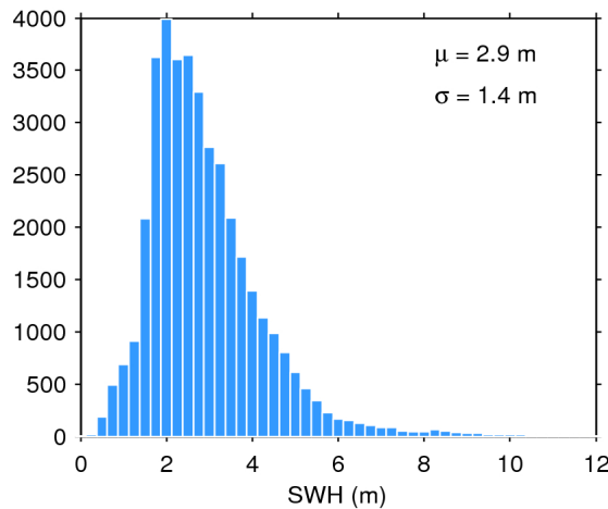
Figure 20. Histogram of science-valid SWH over oceans and lakes for 07/12/2018. The mean ( \mu ) and standard deviation ( \sigma ) are also shown. Note that values larger than 12 m are excluded from the histogram for the sake of readability but not from the computation of \mu and \sigma .
