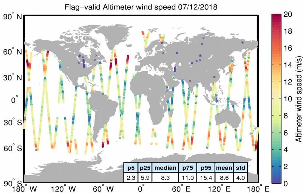
Figure 31. Geographical distribution of flag-valid wind data over oceans and lakes for 07/12/2018. The statistical values shown in the table refer to the wind in m/s and are calculated over all measurements shown in the figure.
