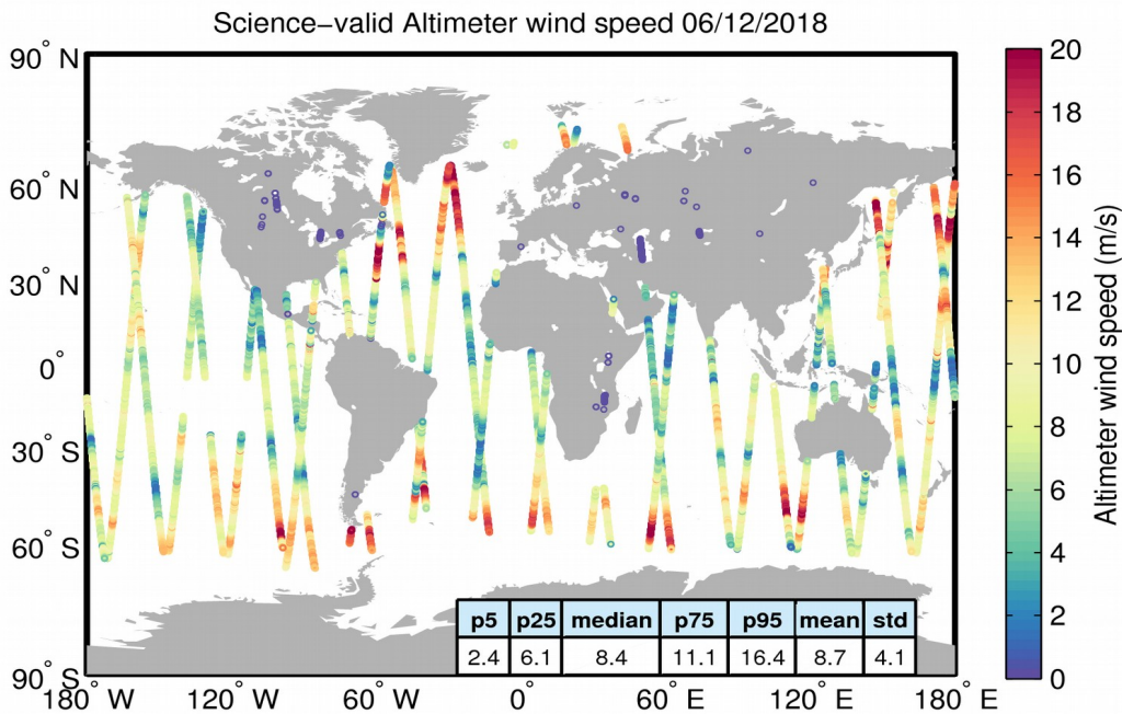
Figure 34. Geographical distribution of science-valid wind data over oceans and lakes for 06/12/2018. The statistical values shown in the table refer to the wind in m/s and are calculated over all measurements shown in the figure. Gray circles denote records that have been rejected based on the editing criteria described in Table 5.
