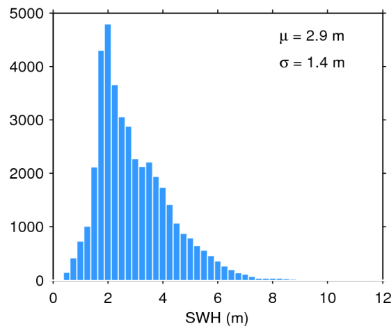
Figure 17. Histogram of flag-valid SWH over oceans and lakes for 06/12/2018. The mean ( \mu ) and standard deviation ( \sigma ) are also shown. Note that values larger than 12 m are excluded from the histogram for the sake of readability but not from the computation of \mu and \sigma .
