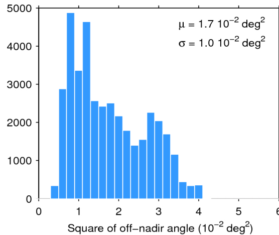
Figure 39. Histogram of flag-valid mispointing over oceans and lakes for 06/12/2018. The mean ( \mu ) and standard deviation ( \sigma ) are also shown. Note that values larger than 6 \cdot 10^{-2} \text{ deg}^2 are excluded from the histogram for the sake of readability but not from the computation of \mu and \sigma .
