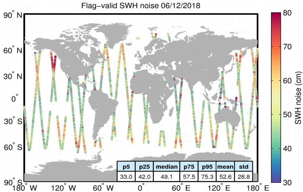
Figure 18. Geographical distribution of flag-valid 20-Hz SWH measurement noise over oceans and lakes for 06/12/2018. The statistical values shown in the figure refer to the SWH noise and are calculated over all measurements shown in the figure.
