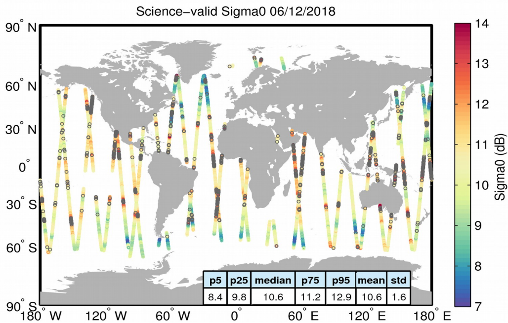
Figure 27. Geographical distribution of science-valid sigma0 data over oceans and lakes for 06/12/2018. The statistical values shown in the table refer to the sigma0 in dB and are calculated over all measurements shown in the figure. Gray circles denote records that have been rejected based on the editing criteria described in Table 4.
