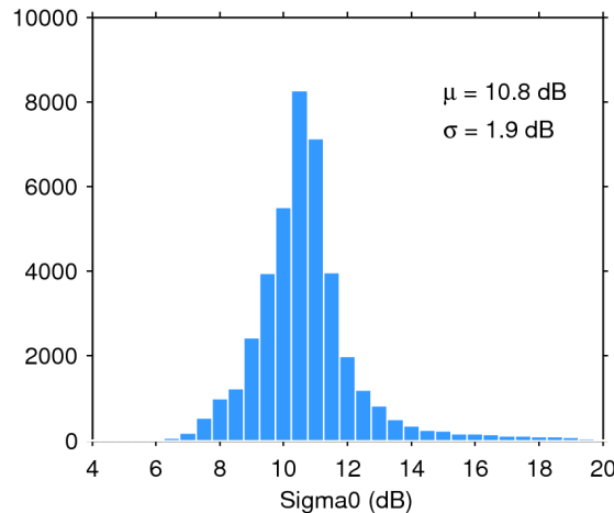
Figure 25. Histogram of flag-valid sigma0 over oceans and lakes for 06/12/2018. The mean ( \mu ) and standard deviation ( \sigma ) are also shown. Note that values outside [4 20] dB are excluded from the histogram for the sake of readability but not from the computation of \mu and \sigma .
