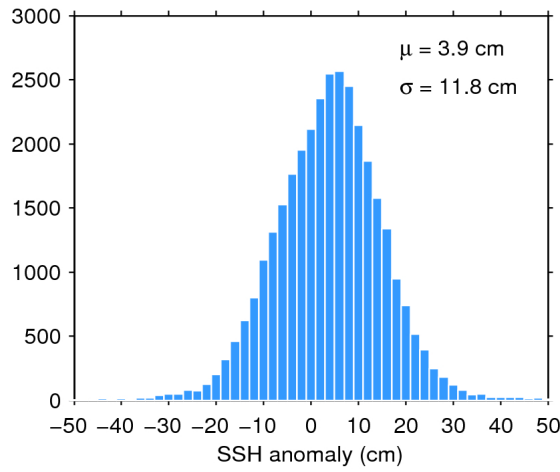
Figure 11. Histogram of science-valid SSH anomaly over oceans and lakes for 06/12/2018. The mean ( \mu ) and standard deviation ( \sigma ) are also shown. Note that values outside [-50 50] cm are excluded from the histogram for the sake of readability but not from the computation of \mu and \sigma .
