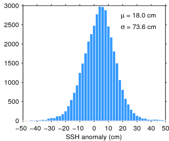
Figure 7. Histogram of flag-valid SSH anomaly over oceans and lakes for 06/12/2018. The mean ( \mu ) and standard deviation ( \sigma ) are also shown. Note that values outside [-50\ 50] cm are excluded from the histogram for the sake of readability but not from the computation of \mu and \sigma .
