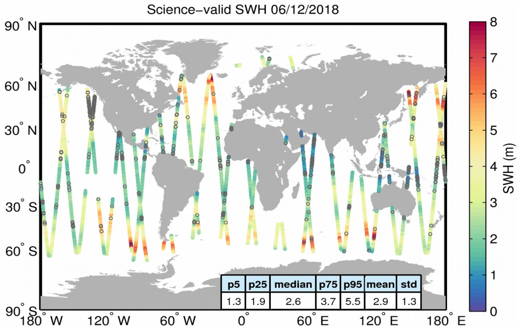
Figure 19. Geographical distribution of science-valid SWH data over oceans and lakes for 06/12/2018. The statistical values shown in the table refer to the SWH in m and are calculated over all measurements shown in the figure. Gray circles denote records that have been rejected based on the editing criteria described in Table 3.
