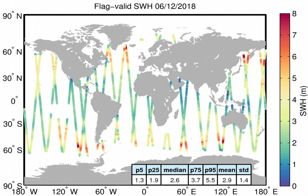
Figure 15. Geographical distribution of flag-valid SWH data over oceans and lakes for 06/12/2018. The statistical values shown in the table refer to the SWH in m and are calculated over all measurements shown in the figure.
