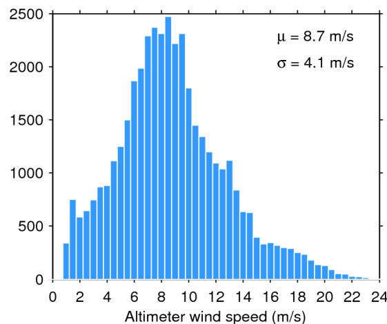
Figure 35. Histogram of science-valid wind over oceans and lakes for 06/12/2018. The mean ( \mu ) and standard deviation ( \sigma ) are also shown. Note that values larger than 24 m/s are excluded from the histogram for the sake of readability but not from the computation of \mu and \sigma .
