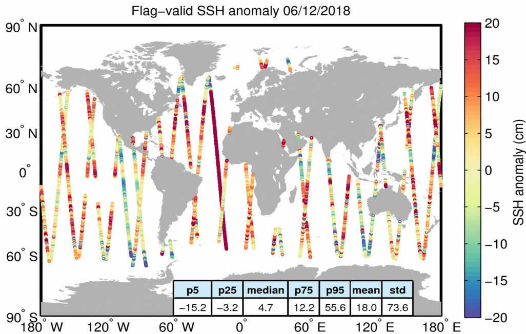
Figure 5. Geographical distribution of flag-valid 1-Hz SSH anomaly data over oceans and lakes for 06/12/2018. The statistical values shown in the table refer to the SSH anomaly in cm and are calculated over all measurements shown in the figure.
