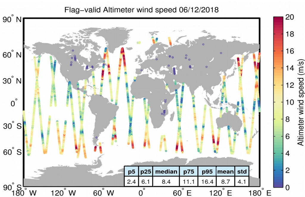
Figure 31. Geographical distribution of flag-valid wind data over oceans and lakes for 06/12/2018. The statistical values shown in the table refer to the wind in m/s and are calculated over all measurements shown in the figure.
