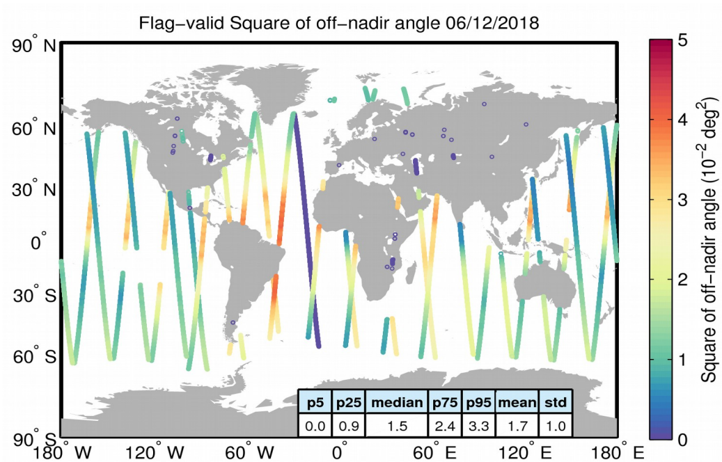
Figure 37. Geographical distribution of flag-valid mispointing data over oceans and lakes for 06/12/2018. The statistical values shown in the table refer to the mispointing in 10^{-2} deg 2 and are calculated over all measurements shown in the figure.
