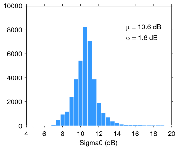
Figure 28. Histogram of science-valid sigma0 over oceans and lakes for 06/12/2018. The mean ( \mu ) and standard deviation ( \sigma ) are also shown. Note that values outside [4 20] dB are excluded from the histogram for the sake of readability but not from the computation of \mu and \sigma .
