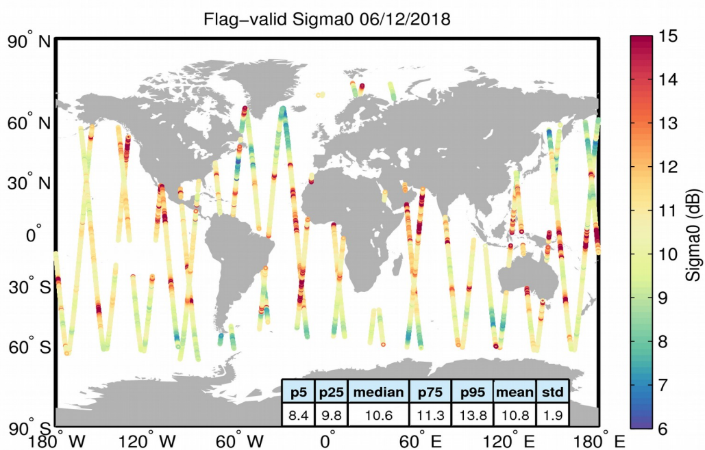
Figure 23. Geographical distribution of flag-valid sigma0 data over oceans and lakes for 06/12/2018. The statistical values shown in the table refer to the sigma0 in dB and are calculated over all measurements shown in the figure.
