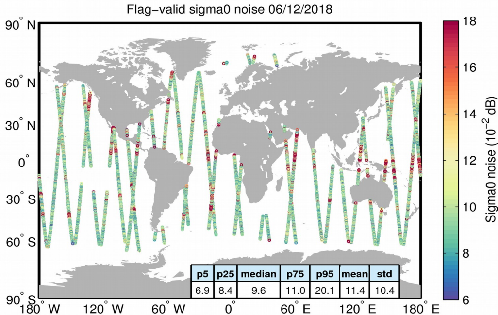
Figure 26. Geographical distribution of flag-valid 20-Hz sigma0 measurement noise over oceans and lakes for 06/12/2018. The statistical values shown in the table refer to the sigma0 noise and are calculated over all measurements shown in the figure.
