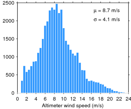
Figure 33. Histogram of flag-valid wind over oceans and lakes for 06/12/2018. The mean ( \mu ) and standard deviation ( \sigma ) are also shown. Note that values larger than 24 m/s are excluded from the histogram for the sake of readability but not from the computation of \mu and \sigma .
