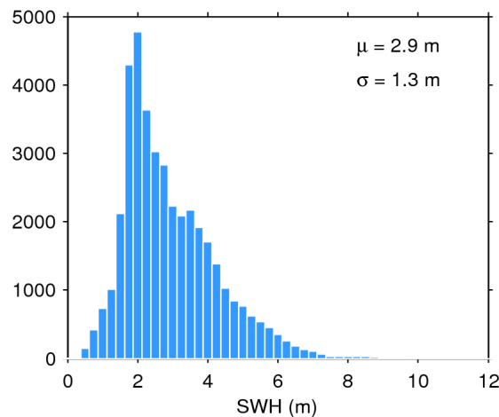
Figure 20. Histogram of science-valid SWH over oceans and lakes for 06/12/2018. The mean ( \mu ) and standard deviation ( \sigma ) are also shown. Note that values larger than 12 m are excluded from the histogram for the sake of readability but not from the computation of \mu and \sigma .
