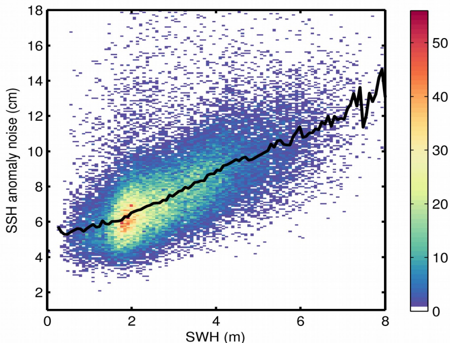
Figure 9. 2D histogram showing flag-valid SSH anomaly noise as a function of SWH for 06/12/2018. The black line denotes the median SSH anomaly noise as a function of SWH.
