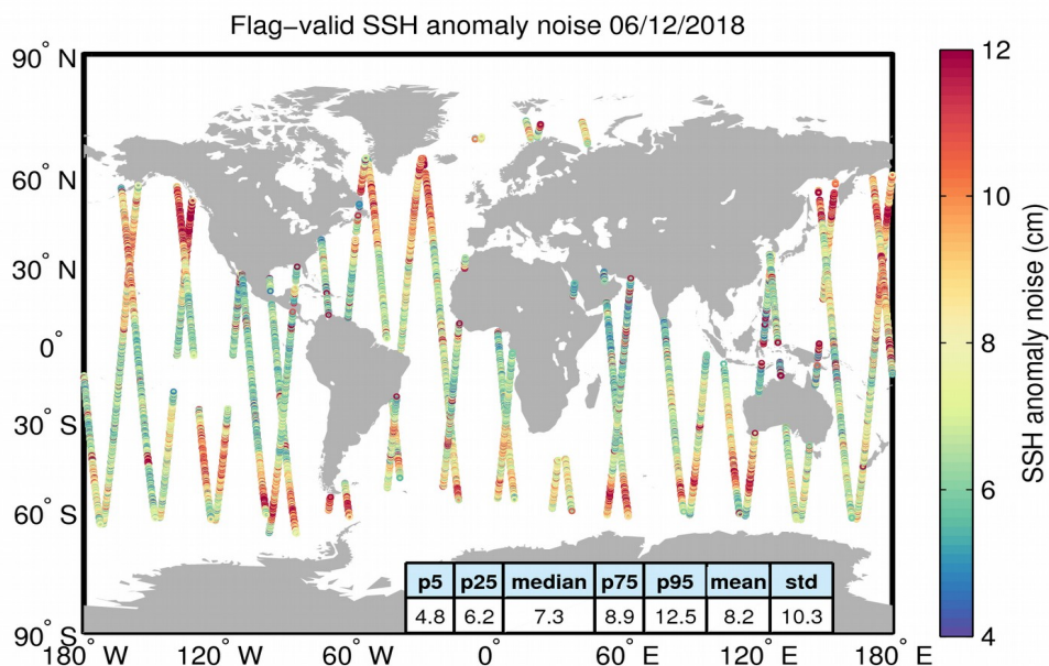
Figure 8. Geographical distribution of flag-valid 20-Hz SSH anomaly measurement noise over oceans and lakes for 06/12/2018. The statistical values shown in the table refer to the SSH anomaly noise and are calculated over all measurements shown in the figure.
