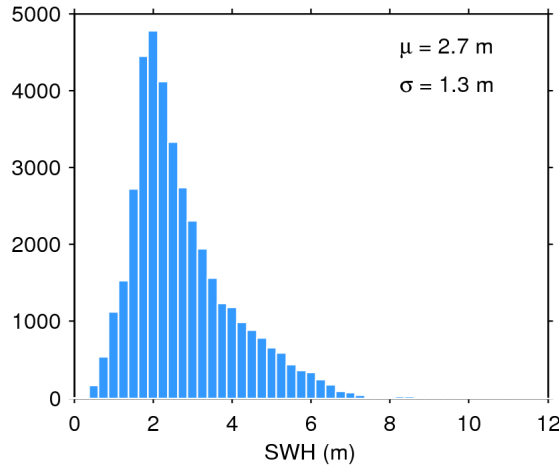
Figure 20. Histogram of science-valid SWH over oceans and lakes for 05/12/2018. The mean ( \mu ) and standard deviation ( \sigma ) are also shown. Note that values larger than 12 m are excluded from the histogram for the sake of readability but not from the computation of \mu and \sigma .
