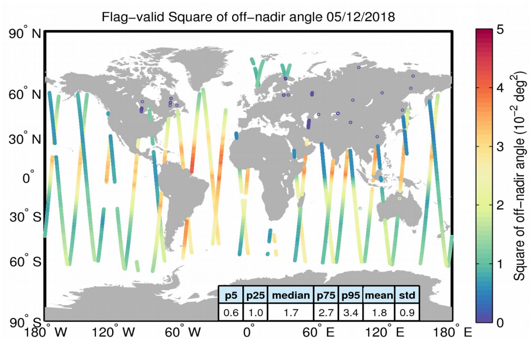
Figure 37. Geographical distribution of flag-valid mispointing data over oceans and lakes for 05/12/2018. The statistical values shown in the table refer to the mispointing in 10^{-2} deg 2 and are calculated over all measurements shown in the figure.
