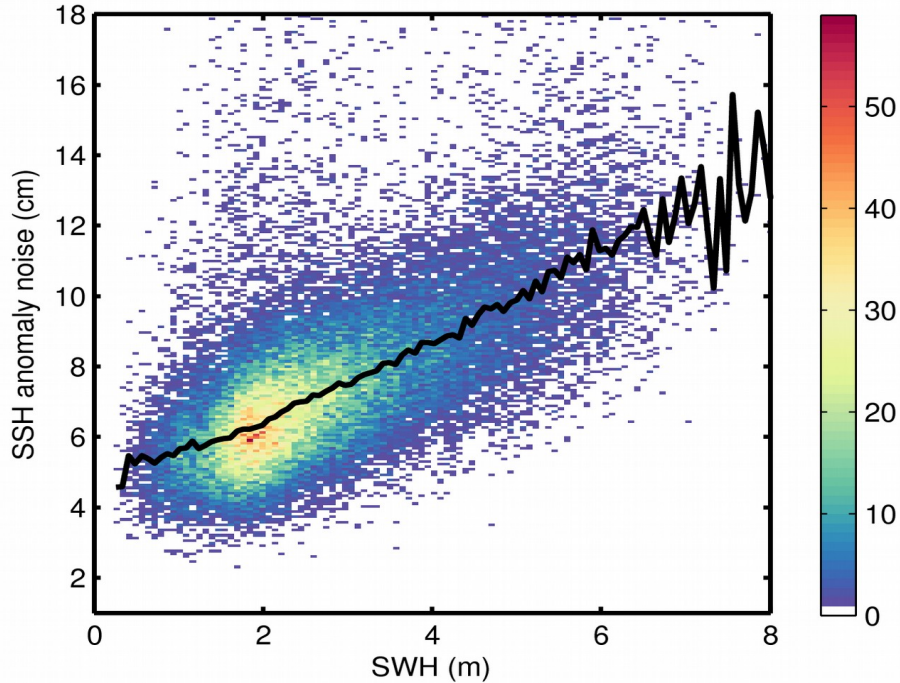
Figure 9. 2D histogram showing flag-valid SSH anomaly noise as a function of SWH for 05/12/2018. The black line denotes the median SSH anomaly noise as a function of SWH.
