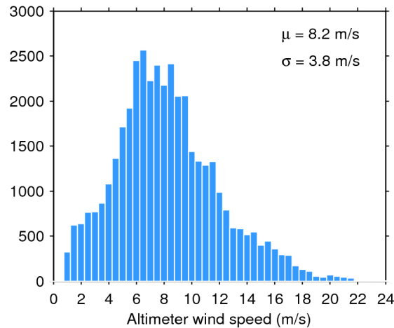
Figure 33. Histogram of flag-valid wind over oceans and lakes for 05/12/2018. The mean ( \mu ) and standard deviation ( \sigma ) are also shown. Note that values larger than 24 m/s are excluded from the histogram for the sake of readability but not from the computation of \mu and \sigma .
