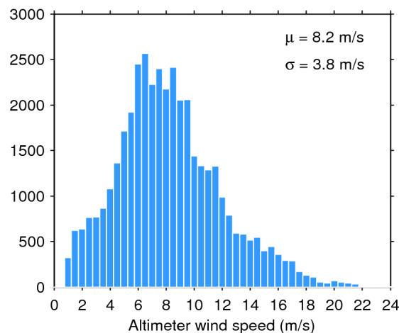
Figure 35. Histogram of science-valid wind over oceans and lakes for 05/12/2018. The mean ( \mu ) and standard deviation ( \sigma ) are also shown. Note that values larger than 24 m/s are excluded from the histogram for the sake of readability but not from the computation of \mu and \sigma .
