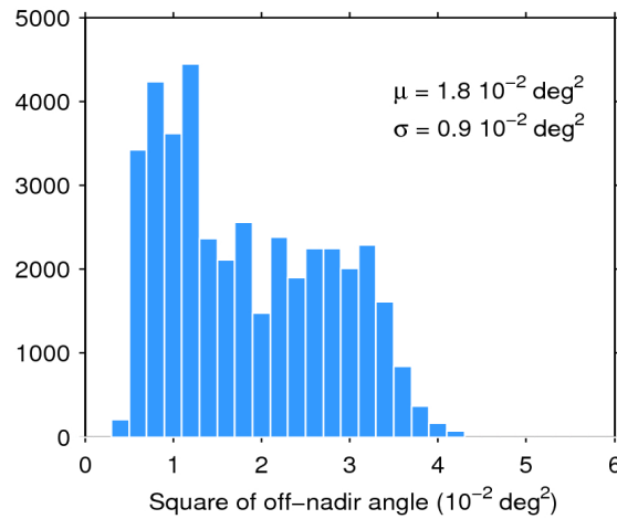
Figure 39. Histogram of flag-valid mispointing over oceans and lakes for 05/12/2018. The mean ( \mu ) and standard deviation ( \sigma ) are also shown. Note that values larger than 6 \cdot 10^{-2} \text{ deg}^2 are excluded from the histogram for the sake of readability but not from the computation of \mu and \sigma .
