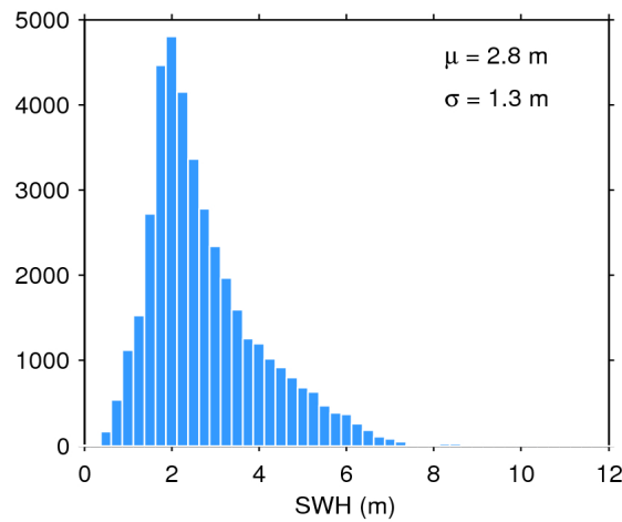
Figure 17. Histogram of flag-valid SWH over oceans and lakes for 05/12/2018. The mean ( \mu ) and standard deviation ( \sigma ) are also shown. Note that values larger than 12 m are excluded from the histogram for the sake of readability but not from the computation of \mu and \sigma .
