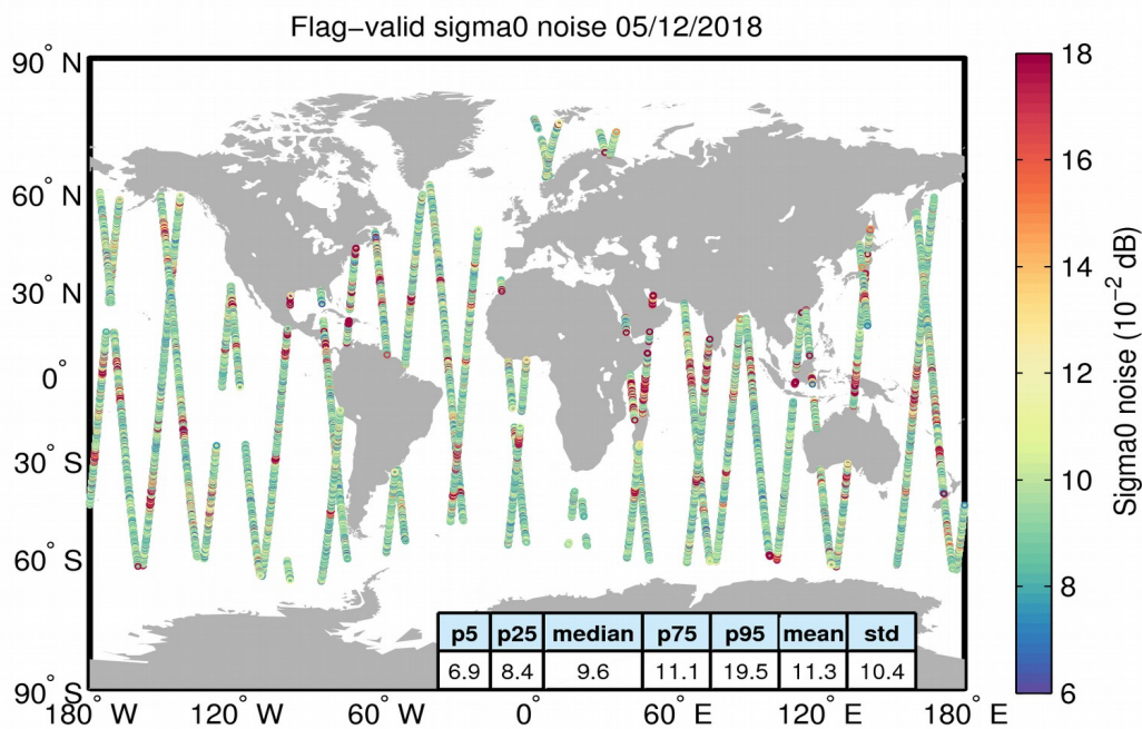
Figure 26. Geographical distribution of flag-valid 20-Hz sigma0 measurement noise over oceans and lakes for 05/12/2018. The statistical values shown in the table refer to the sigma0 noise and are calculated over all measurements shown in the figure.
