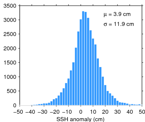
Figure 11. Histogram of science-valid SSH anomaly over oceans and lakes for 05/12/2018. The mean ( \mu ) and standard deviation ( \sigma ) are also shown. Note that values outside [-50 50] cm are excluded from the histogram for the sake of readability but not from the computation of \mu and \sigma .
