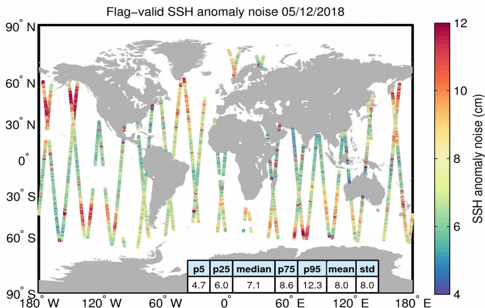
Figure 8. Geographical distribution of flag-valid 20-Hz SSH anomaly measurement noise over oceans and lakes for 05/12/2018. The statistical values shown in the table refer to the SSH anomaly noise and are calculated over all measurements shown in the figure.
