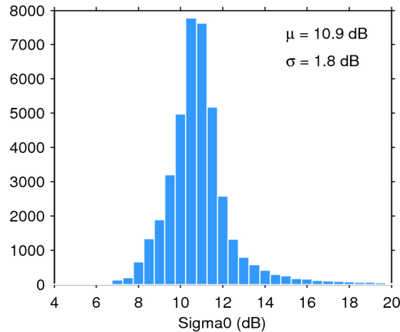
Figure 25. Histogram of flag-valid sigma0 over oceans and lakes for 05/12/2018. The mean ( \mu ) and standard deviation ( \sigma ) are also shown. Note that values outside [4 20] dB are excluded from the histogram for the sake of readability but not from the computation of \mu and \sigma .
