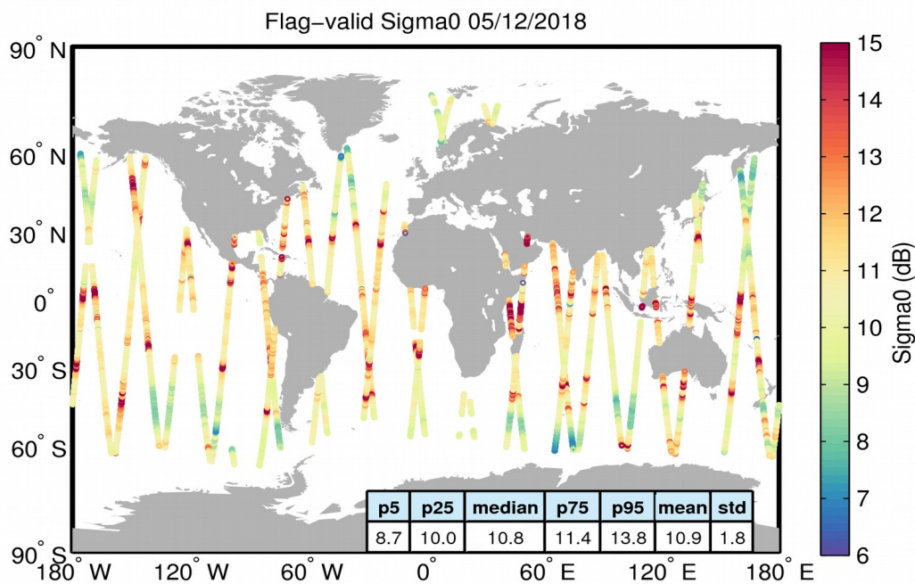
Figure 23. Geographical distribution of flag-valid sigma0 data over oceans and lakes for 05/12/2018. The statistical values shown in the table refer to the sigma0 in dB and are calculated over all measurements shown in the figure.
