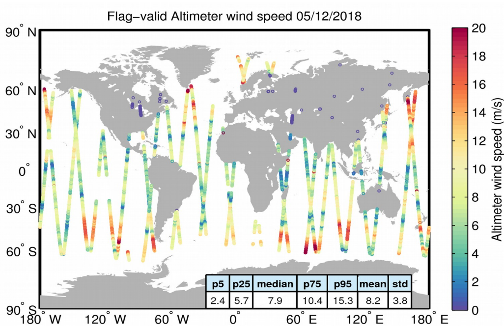
Figure 31. Geographical distribution of flag-valid wind data over oceans and lakes for 05/12/2018. The statistical values shown in the table refer to the wind in m/s and are calculated over all measurements shown in the figure.
