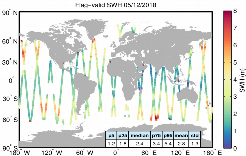
Figure 15. Geographical distribution of flag-valid SWH data over oceans and lakes for 05/12/2018. The statistical values shown in the table refer to the SWH in m and are calculated over all measurements shown in the figure.
