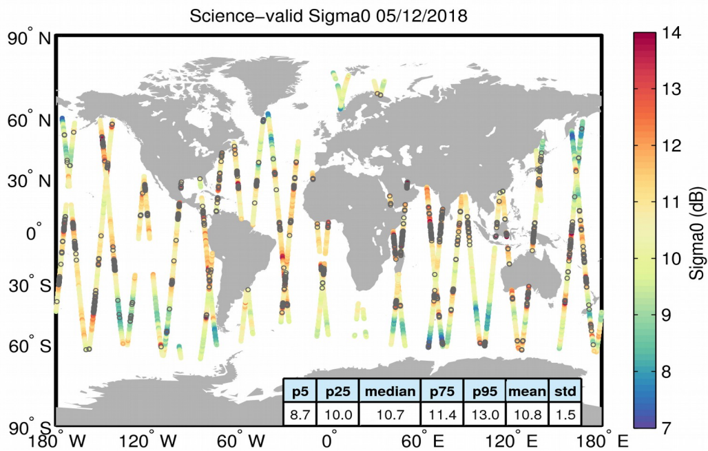
Figure 27. Geographical distribution of science-valid sigma0 data over oceans and lakes for 05/12/2018. The statistical values shown in the table refer to the sigma0 in dB and are calculated over all measurements shown in the figure. Gray circles denote records that have been rejected based on the editing criteria described in Table 4.
