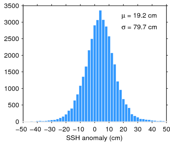
Figure 7. Histogram of flag-valid SSH anomaly over oceans and lakes for 04/12/2018. The mean ( \mu ) and standard deviation ( \sigma ) are also shown. Note that values outside [-50\ 50] cm are excluded from the histogram for the sake of readability but not from the computation of \mu and \sigma .
