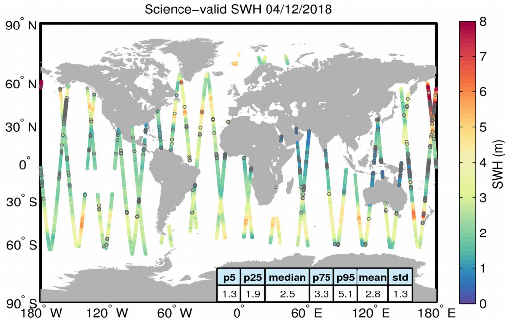
Figure 19. Geographical distribution of science-valid SWH data over oceans and lakes for 04/12/2018. The statistical values shown in the table refer to the SWH in m and are calculated over all measurements shown in the figure. Gray circles denote records that have been rejected based on the editing criteria described in Table 3.
