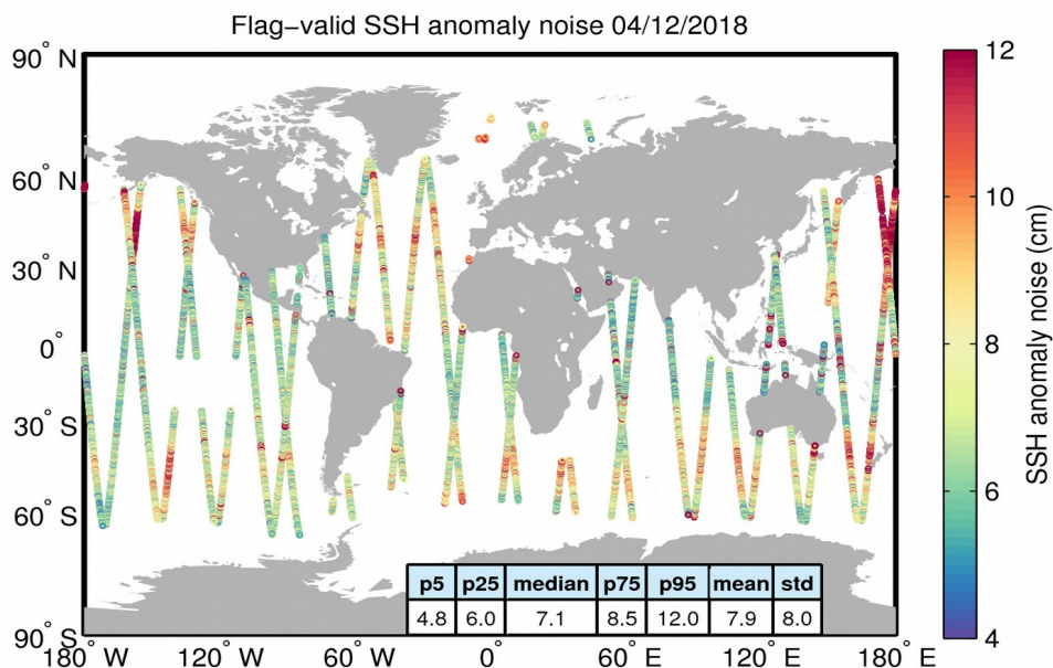
Figure 8. Geographical distribution of flag-valid 20-Hz SSH anomaly measurement noise over oceans and lakes for 04/12/2018. The statistical values shown in the table refer to the SSH anomaly noise and are calculated over all measurements shown in the figure.
