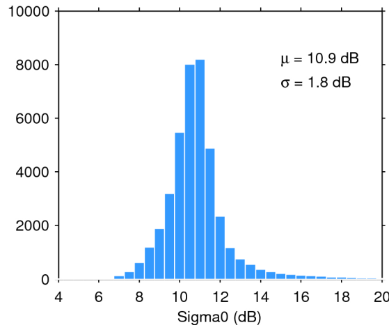
Figure 25. Histogram of flag-valid sigma0 over oceans and lakes for 04/12/2018. The mean ( \mu ) and standard deviation ( \sigma ) are also shown. Note that values outside [4 20] dB are excluded from the histogram for the sake of readability but not from the computation of \mu and \sigma .
