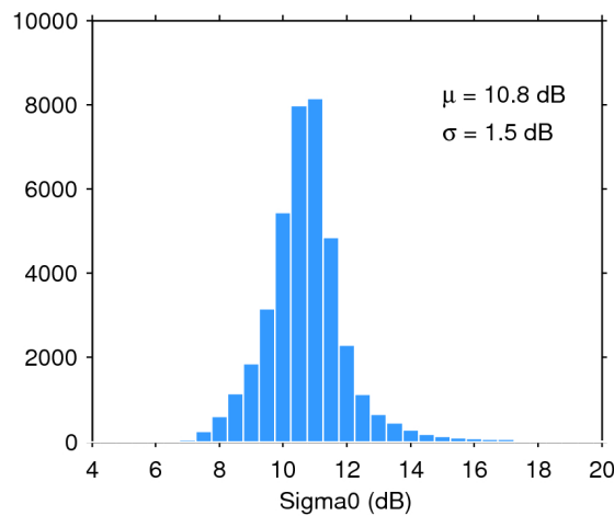
Figure 28. Histogram of science-valid sigma0 over oceans and lakes for 04/12/2018. The mean ( \mu ) and standard deviation ( \sigma ) are also shown. Note that values outside [4 20] dB are excluded from the histogram for the sake of readability but not from the computation of \mu and \sigma .
