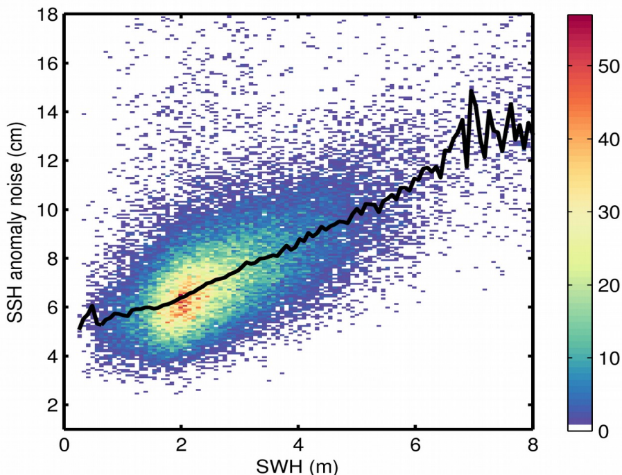
Figure 9. 2D histogram showing flag-valid SSH anomaly noise as a function of SWH for 04/12/2018. The black line denotes the median SSH anomaly noise as a function of SWH.
