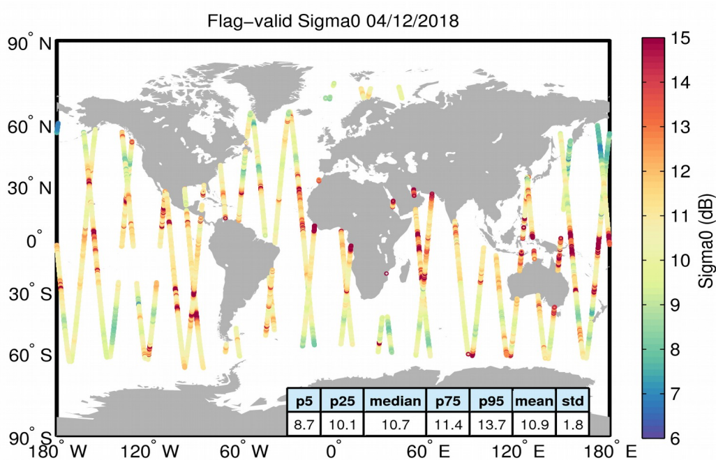
Figure 23. Geographical distribution of flag-valid sigma0 data over oceans and lakes for 04/12/2018. The statistical values shown in the table refer to the sigma0 in dB and are calculated over all measurements shown in the figure.
