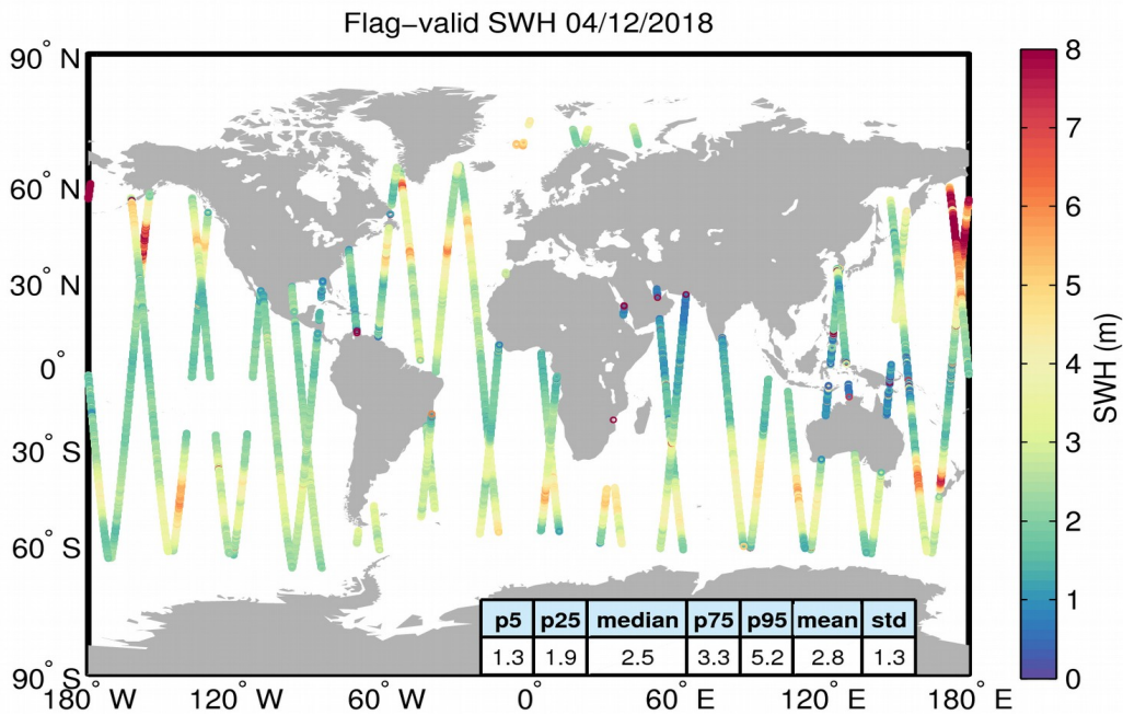
Figure 15. Geographical distribution of flag-valid SWH data over oceans and lakes for 04/12/2018. The statistical values shown in the table refer to the SWH in m and are calculated over all measurements shown in the figure.
