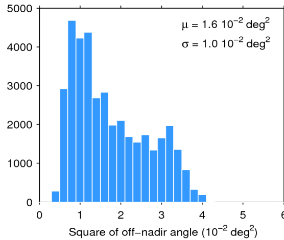
Figure 39. Histogram of flag-valid mispointing over oceans and lakes for 04/12/2018. The mean ( \mu ) and standard deviation ( \sigma ) are also shown. Note that values larger than 6 \cdot 10^{-2} \text{ deg}^2 are excluded from the histogram for the sake of readability but not from the computation of \mu and \sigma .
