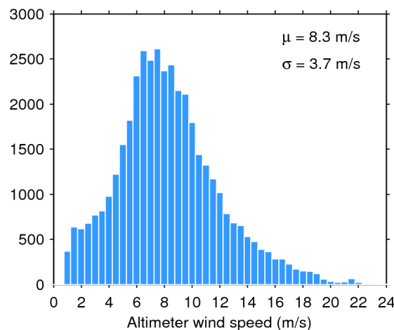
Figure 35. Histogram of science-valid wind over oceans and lakes for 04/12/2018. The mean ( \mu ) and standard deviation ( \sigma ) are also shown. Note that values larger than 24 m/s are excluded from the histogram for the sake of readability but not from the computation of \mu and \sigma .
