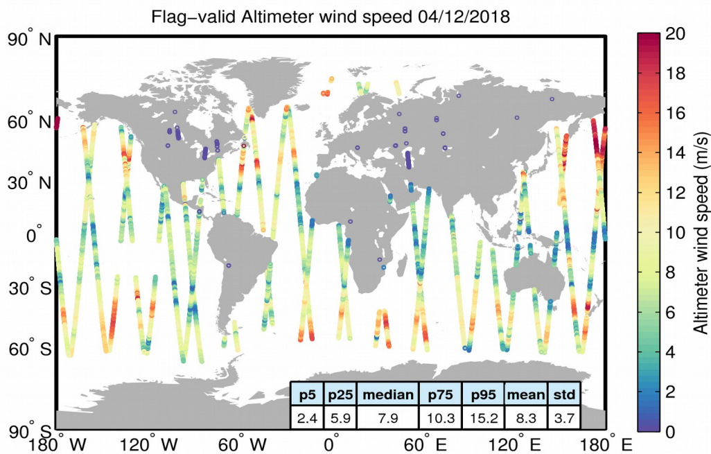
Figure 31. Geographical distribution of flag-valid wind data over oceans and lakes for 04/12/2018. The statistical values shown in the table refer to the wind in m/s and are calculated over all measurements shown in the figure.
