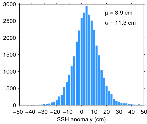
Figure 11. Histogram of science-valid SSH anomaly over oceans and lakes for 04/12/2018. The mean ( \mu ) and standard deviation ( \sigma ) are also shown. Note that values outside [-50 50] cm are excluded from the histogram for the sake of readability but not from the computation of \mu and \sigma .
