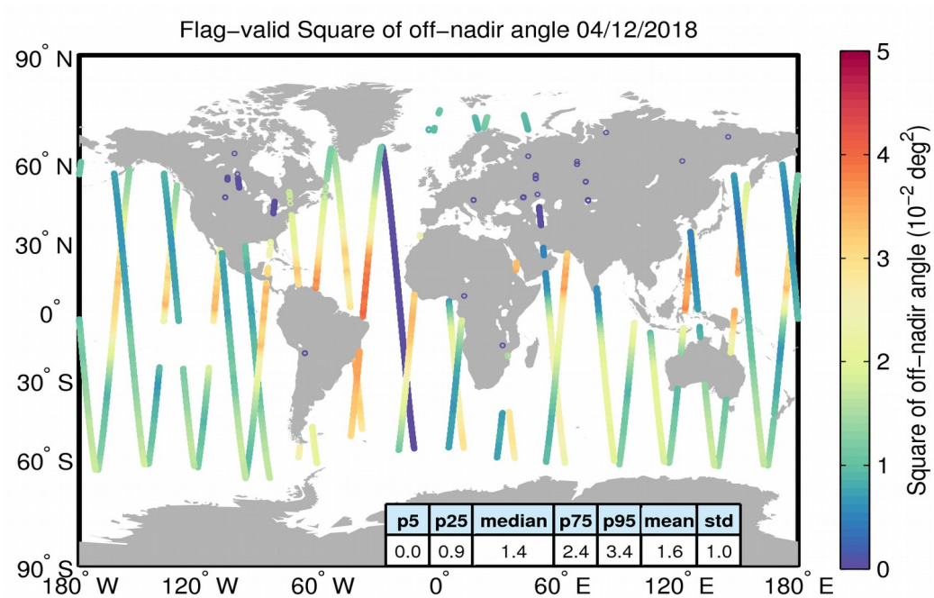
Figure 37. Geographical distribution of flag-valid mispointing data over oceans and lakes for 04/12/2018. The statistical values shown in the table refer to the mispointing in 10^{-2} deg 2 and are calculated over all measurements shown in the figure.
