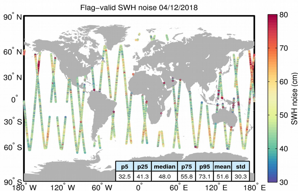
Figure 18. Geographical distribution of flag-valid 20-Hz SWH measurement noise over oceans and lakes for 04/12/2018. The statistical values shown in the figure refer to the SWH noise and are calculated over all measurements shown in the figure.
