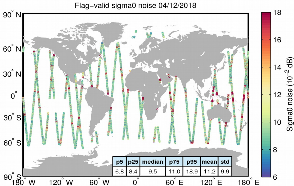
Figure 26. Geographical distribution of flag-valid 20-Hz sigma0 measurement noise over oceans and lakes for 04/12/2018. The statistical values shown in the table refer to the sigma0 noise and are calculated over all measurements shown in the figure.
