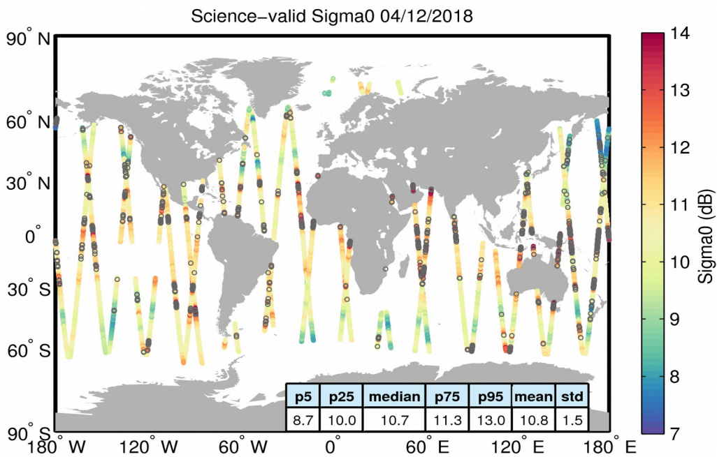
Figure 27. Geographical distribution of science-valid sigma0 data over oceans and lakes for 04/12/2018. The statistical values shown in the table refer to the sigma0 in dB and are calculated over all measurements shown in the figure. Gray circles denote records that have been rejected based on the editing criteria described in Table 4.
