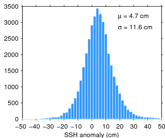
Figure 11. Histogram of science-valid SSH anomaly over oceans and lakes for 03/12/2018. The mean ( \mu ) and standard deviation ( \sigma ) are also shown. Note that values outside [-50 50] cm are excluded from the histogram for the sake of readability but not from the computation of \mu and \sigma .
