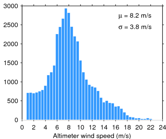
Figure 35. Histogram of science-valid wind over oceans and lakes for 03/12/2018. The mean ( \mu ) and standard deviation ( \sigma ) are also shown. Note that values larger than 24 m/s are excluded from the histogram for the sake of readability but not from the computation of \mu and \sigma .
