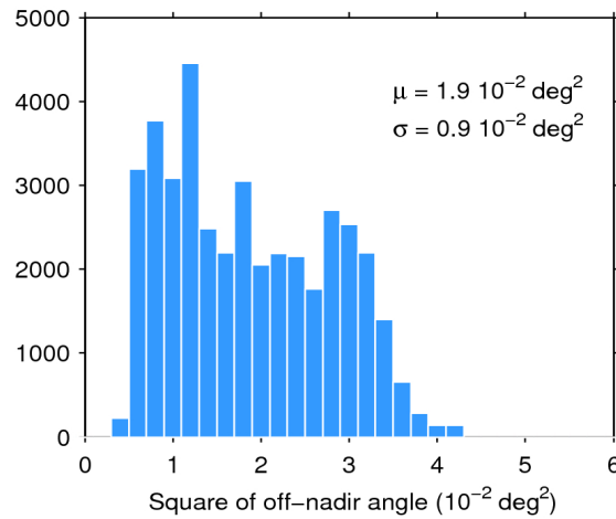
Figure 39. Histogram of flag-valid mispointing over oceans and lakes for 03/12/2018. The mean ( \mu ) and standard deviation ( \sigma ) are also shown. Note that values larger than 6 \cdot 10^{-2} \text{ deg}^2 are excluded from the histogram for the sake of readability but not from the computation of \mu and \sigma .
