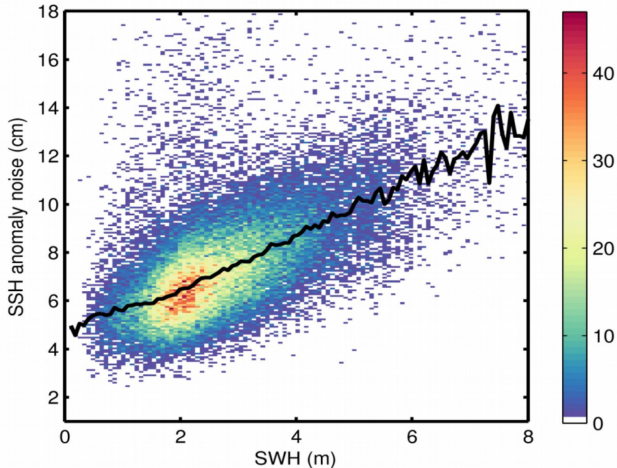
Figure 9. 2D histogram showing flag-valid SSH anomaly noise as a function of SWH for 03/12/2018. The black line denotes the median SSH anomaly noise as a function of SWH.
