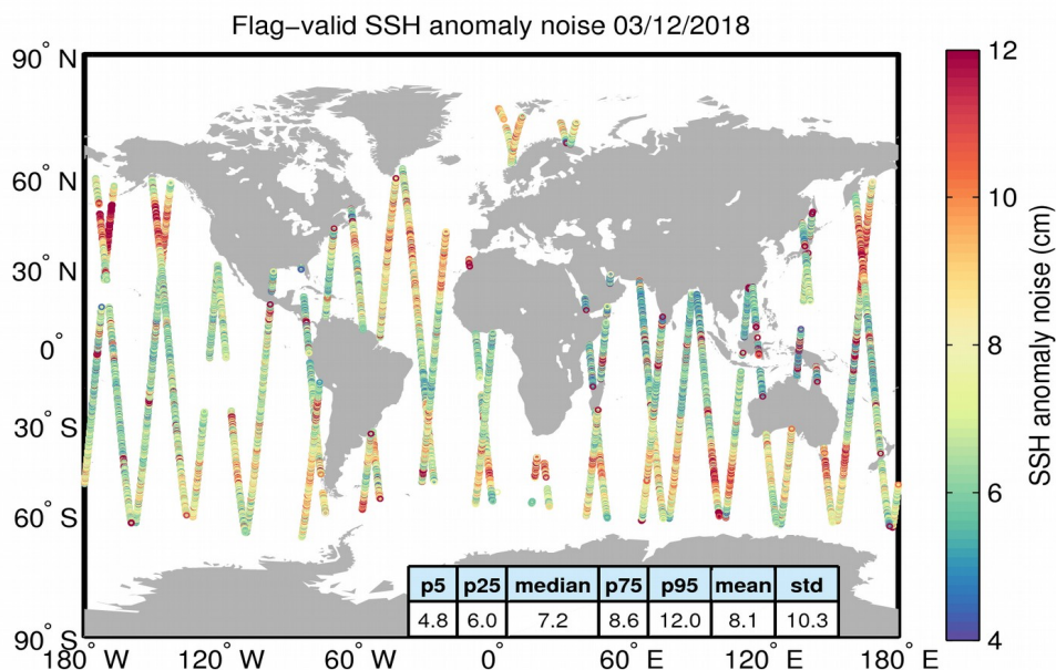
Figure 8. Geographical distribution of flag-valid 20-Hz SSH anomaly measurement noise over oceans and lakes for 03/12/2018. The statistical values shown in the table refer to the SSH anomaly noise and are calculated over all measurements shown in the figure.
