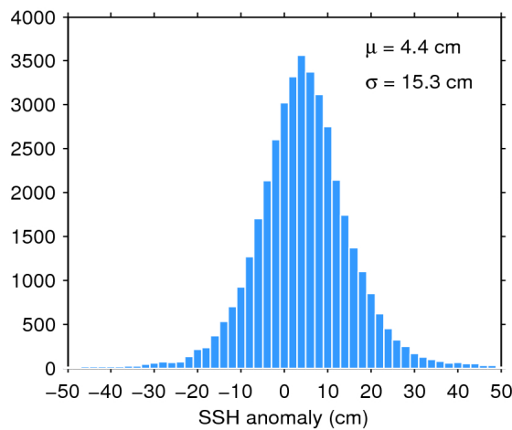
Figure 7. Histogram of flag-valid SSH anomaly over oceans and lakes for 03/12/2018. The mean ( \mu ) and standard deviation ( \sigma ) are also shown. Note that values outside [-50 50] cm are excluded from the histogram for the sake of readability but not from the computation of \mu and \sigma .
