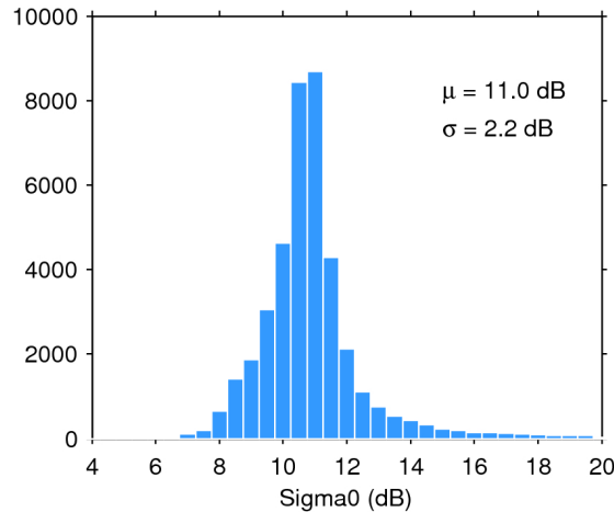
Figure 25. Histogram of flag-valid sigma0 over oceans and lakes for 03/12/2018. The mean ( \mu ) and standard deviation ( \sigma ) are also shown. Note that values outside [4 20] dB are excluded from the histogram for the sake of readability but not from the computation of \mu and \sigma .
