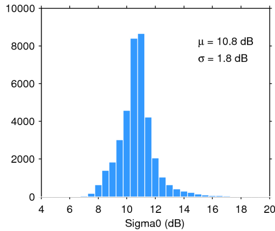
Figure 28. Histogram of science-valid sigma0 over oceans and lakes for 03/12/2018. The mean ( \mu ) and standard deviation ( \sigma ) are also shown. Note that values outside [4 20] dB are excluded from the histogram for the sake of readability but not from the computation of \mu and \sigma .
