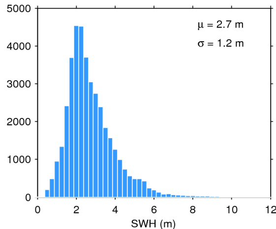
Figure 20. Histogram of science-valid SWH over oceans and lakes for 03/12/2018. The mean ( \mu ) and standard deviation ( \sigma ) are also shown. Note that values larger than 12 m are excluded from the histogram for the sake of readability but not from the computation of \mu and \sigma .
