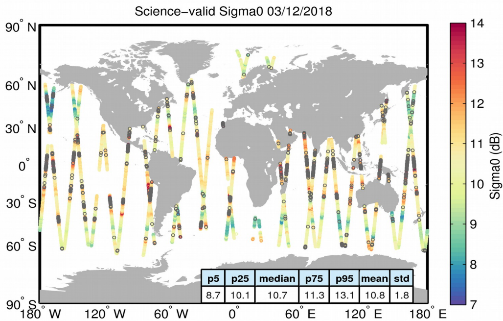
Figure 27. Geographical distribution of science-valid sigma0 data over oceans and lakes for 03/12/2018. The statistical values shown in the table refer to the sigma0 in dB and are calculated over all measurements shown in the figure. Gray circles denote records that have been rejected based on the editing criteria described in Table 4.
