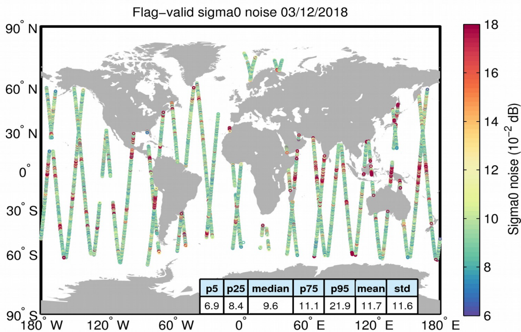
Figure 26. Geographical distribution of flag-valid 20-Hz sigma0 measurement noise over oceans and lakes for 03/12/2018. The statistical values shown in the table refer to the sigma0 noise and are calculated over all measurements shown in the figure.
