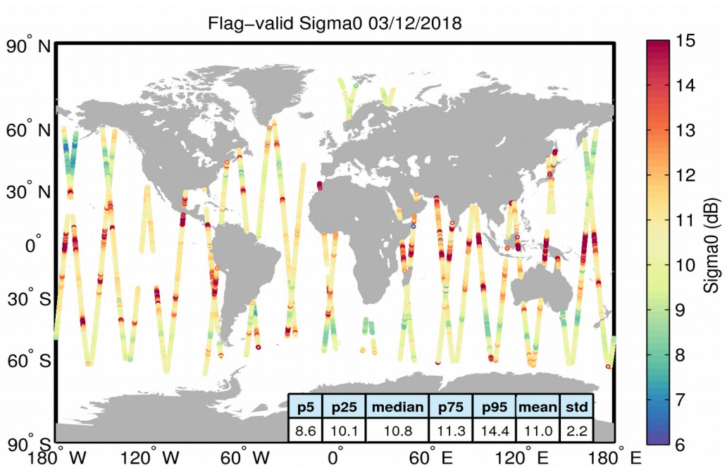
Figure 23. Geographical distribution of flag-valid sigma0 data over oceans and lakes for 03/12/2018. The statistical values shown in the table refer to the sigma0 in dB and are calculated over all measurements shown in the figure.
