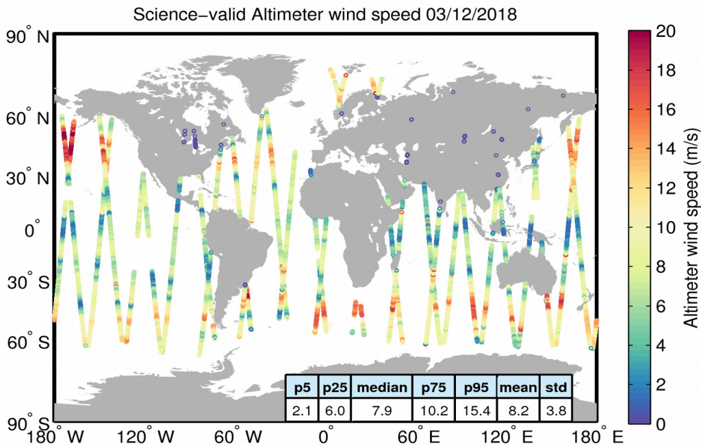
Figure 34. Geographical distribution of science-valid wind data over oceans and lakes for 03/12/2018. The statistical values shown in the table refer to the wind in m/s and are calculated over all measurements shown in the figure. Gray circles denote records that have been rejected based on the editing criteria described in Table 5.
