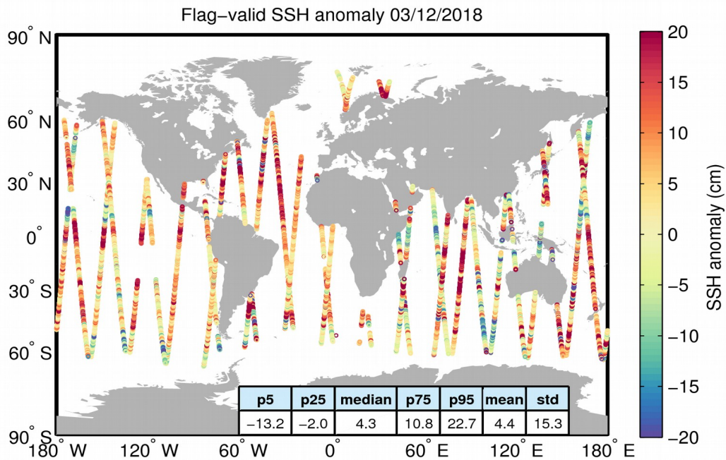
Figure 5. Geographical distribution of flag-valid 1-Hz SSH anomaly data over oceans and lakes for 03/12/2018. The statistical values shown in the table refer to the SSH anomaly in cm and are calculated over all measurements shown in the figure.
