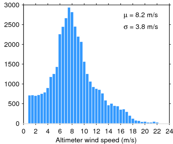
Figure 33. Histogram of flag-valid wind over oceans and lakes for 03/12/2018. The mean ( \mu ) and standard deviation ( \sigma ) are also shown. Note that values larger than 24 m/s are excluded from the histogram for the sake of readability but not from the computation of \mu and \sigma .
