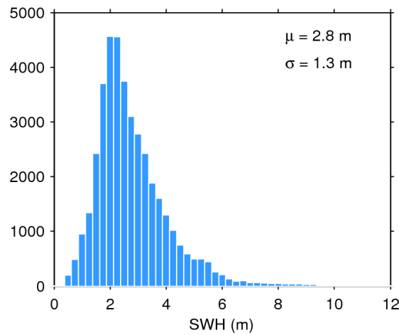
Figure 17. Histogram of flag-valid SWH over oceans and lakes for 03/12/2018. The mean ( \mu ) and standard deviation ( \sigma ) are also shown. Note that values larger than 12 m are excluded from the histogram for the sake of readability but not from the computation of \mu and \sigma .
