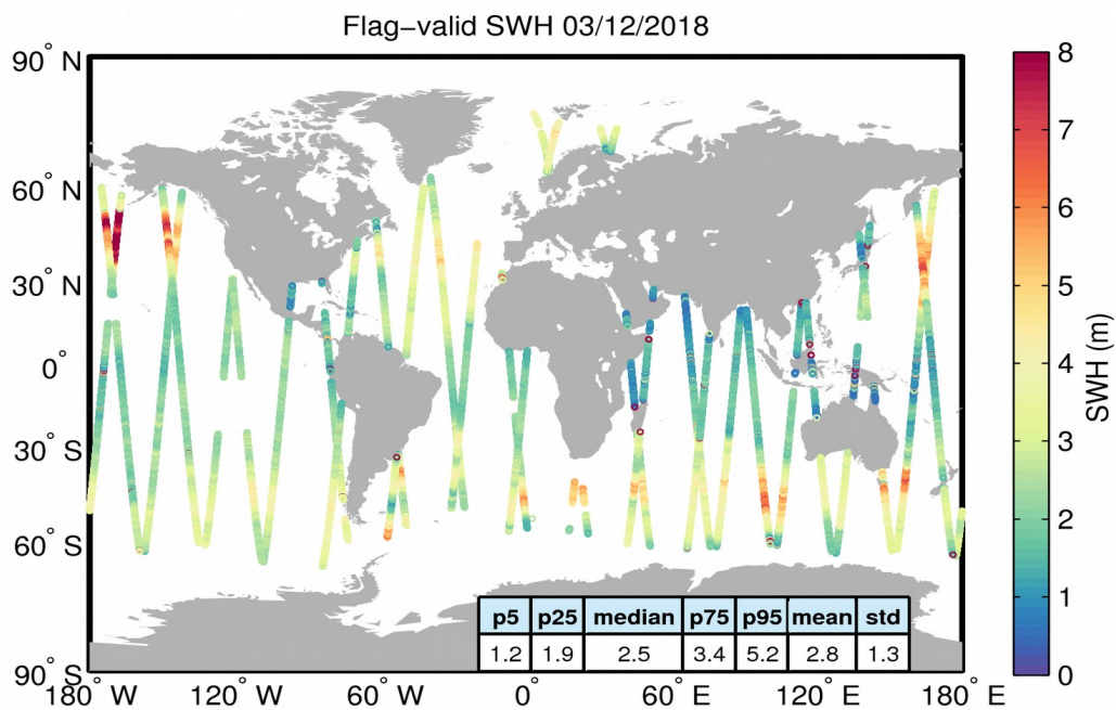
Figure 15. Geographical distribution of flag-valid SWH data over oceans and lakes for 03/12/2018. The statistical values shown in the table refer to the SWH in m and are calculated over all measurements shown in the figure.
