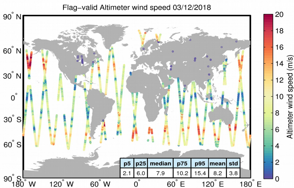
Figure 31. Geographical distribution of flag-valid wind data over oceans and lakes for 03/12/2018. The statistical values shown in the table refer to the wind in m/s and are calculated over all measurements shown in the figure.
