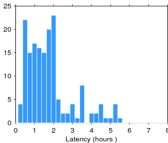
Figure 2. Histogram of the data latency for 03/12/2018. The y-axis denotes the number of files that are made available with a delay of x-hours with respect to the mean time of the records stored in the file.
