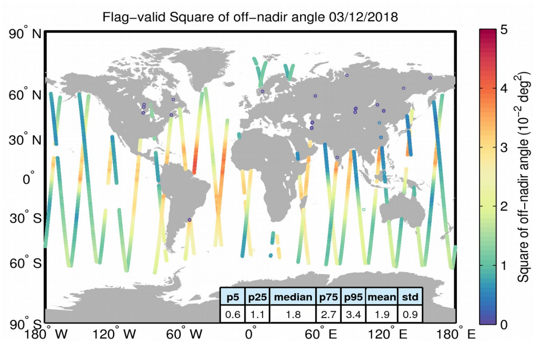
Figure 37. Geographical distribution of flag-valid mispointing data over oceans and lakes for 03/12/2018. The statistical values shown in the table refer to the mispointing in 10^{-2} deg 2 and are calculated over all measurements shown in the figure.
